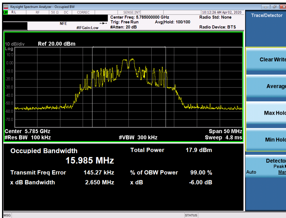
Plot 7-86. 6dB Bandwidth Plot SISO ANT1 (20MHz BW 802.11ax – 26 Tones (UNII Band 3) – Ch. 157)
