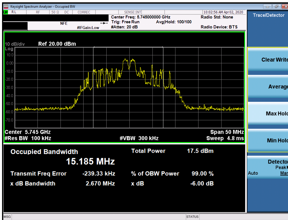
Plot 7-85. 6dB Bandwidth Plot SISO ANT1 (20MHz BW 802.11ax – 26 Tones (UNII Band 3) – Ch. 149)
