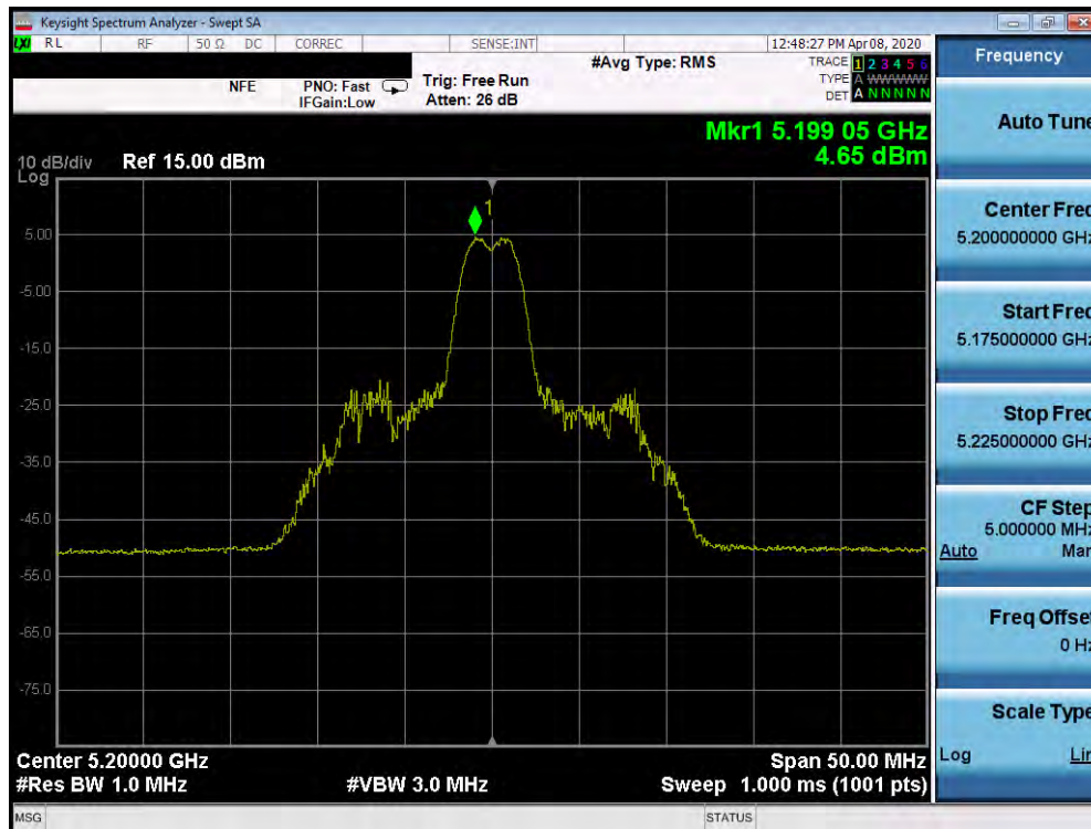
Plot 7-272. Power Spectral Density Plot MIMO ANT2 (20MHz BW 802.11ax – 26 Tones (UNII Band 1) – Ch. 40)
