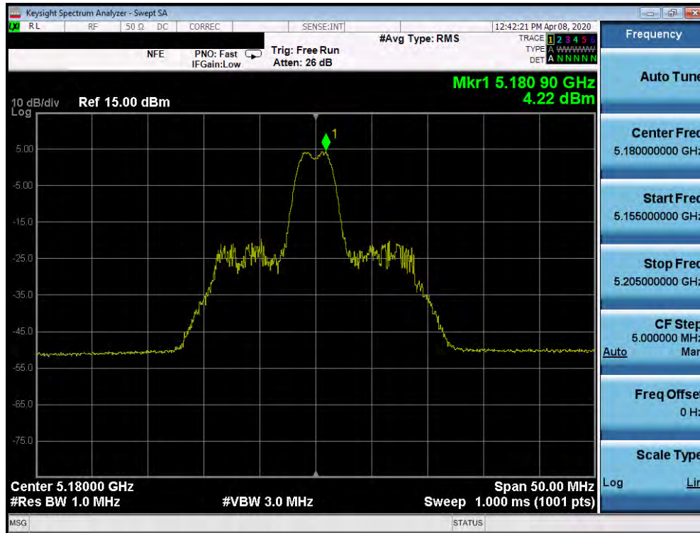
Plot 7-271. Power Spectral Density Plot MIMO ANT2 (20MHz BW 802.11ax – 26 Tones (UNII Band 1) – Ch. 36)
