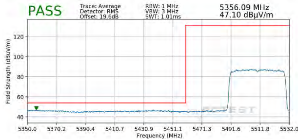
Plot 7-414. Radiated Lower Band Edge Plot MIMO (Average - UNII Band 2C - 484 Tones)
