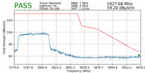
Plot 7-374. Radiated Upper Band Edge Plot SISO ANT1 (Peak – UNII Band 3 – 484 Tones)
