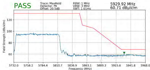
Plot 7-423. Radiated Upper Band Edge Plot MIMO (Peak - UNII Band 3 - 996 Tones)
