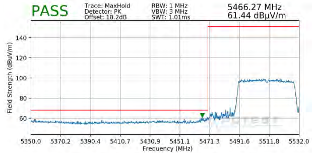
Plot 7-373. Radiated Lower Band Edge Plot SISO ANT1 (Peak – UNII Band 2C – 484 Tones)
