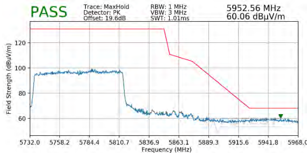
Plot 7-381. Radiated Upper Band Edge Plot SISO ANT1 (Peak – UNII Band 3 – 996 Tones)
