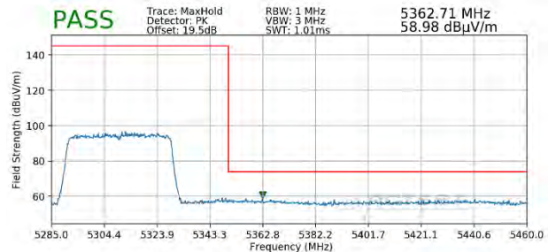
Plot 7-392. Radiated Upper Band Edge Plot SISO ANT2 (Peak - UNII Band 2A - 484 Tones)
