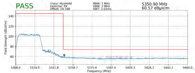
Plot 7-364. Radiated Upper Band Edge Plot SISO ANT1 (Peak - UNII Band 2A - 242 Tones)
