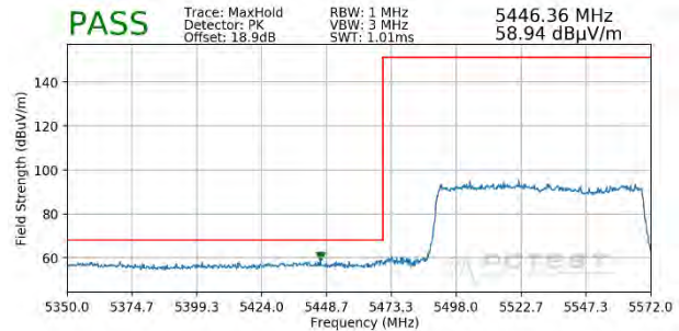
Plot 7-380. Radiated Lower Band Edge Plot SISO ANT1 (Peak – UNII Band 2C – 996 Tones)
