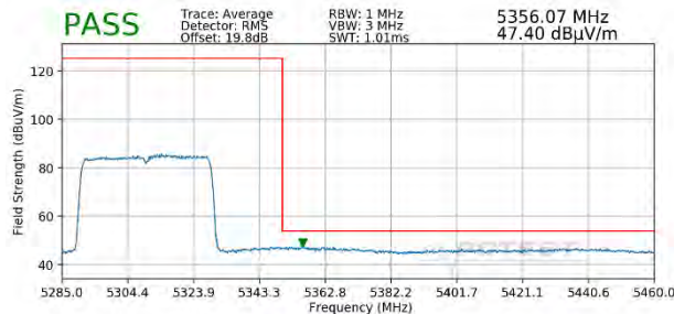
Plot 7-391. Radiated Upper Band Edge Plot SISO ANT2 (Average - UNII Band 2A - 484 Tones)
