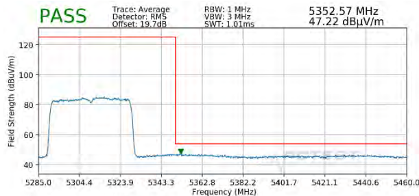
Plot 7-412. Radiated Upper Band Edge Plot MIMO (Average – UNII Band 2A – 484 Tones)
