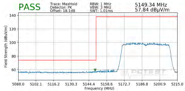
Plot 7-390. Radiated Lower Band Edge Plot SISO ANT2 (Peak - UNII Band 1 - 484 Tones)
