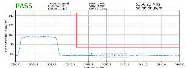
Plot 7-371. Radiated Upper Band Edge Plot SISO ANT1 (Peak - UNII Band 2A - 484 Tones)
