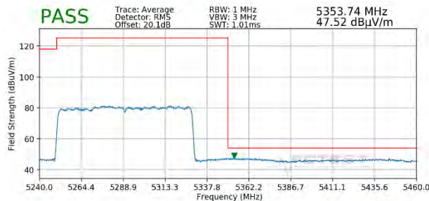
Plot 7-419. Radiated Upper Band Edge Plot MIMO (Average – UNII Band 2A – 996 Tones)
