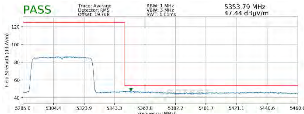
Plot 7-370. Radiated Upper Band Edge Plot SISO ANT1 (Average - UNII Band 2A - 484 Tones)
