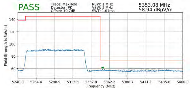
Plot 7-420. Radiated Upper Band Edge Plot MIMO (Peak – UNII Band 2A – 996 Tones)
