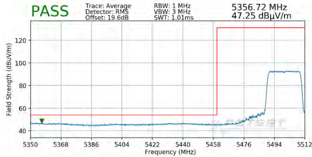
Plot 7-365. Radiated Lower Band Edge Plot SISO ANT1 (Average – UNII Band 2C – 242 Tones)
