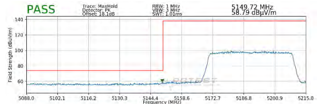
Plot 7-369. Radiated Lower Band Edge Plot SISO ANT1 (Peak - UNII Band 1 - 484 Tones)
