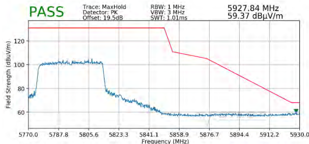
Plot 7-395. Radiated Upper Band Edge Plot SISO ANT2 (Peak - UNII Band 3 - 484 Tones)
