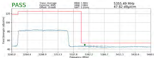
Plot 7-377. Radiated Upper Band Edge Plot SISO ANT1 (Average - UNII Band 2A - 996 Tones)
