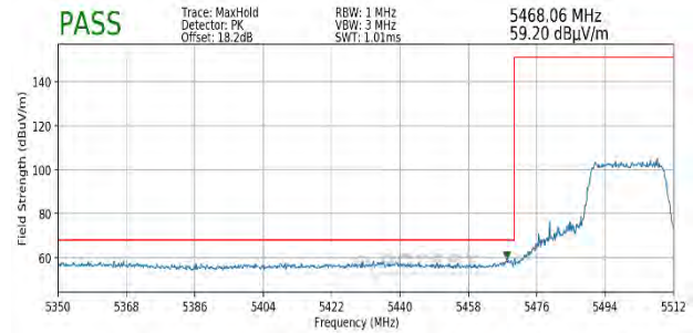
Plot 7-366. Radiated Lower Band Edge Plot SISO ANT1 (Peak – UNII Band 2C – 242 Tones)
