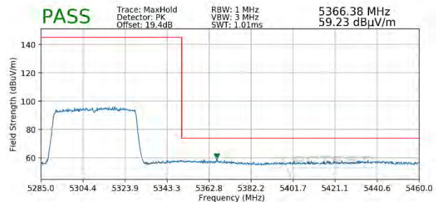
Plot 7-413. Radiated Upper Band Edge Plot MIMO (Peak – UNII Band 2A – 484 Tones)
