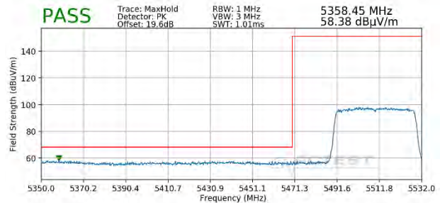
Plot 7-415. Radiated Lower Band Edge Plot MIMO (Peak - UNII Band 2C - 484 Tones)
