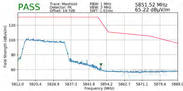
Plot 7-367. Radiated Upper Band Edge Plot SISO ANT1 (Peak – UNII Band 3 – 242 Tones)
