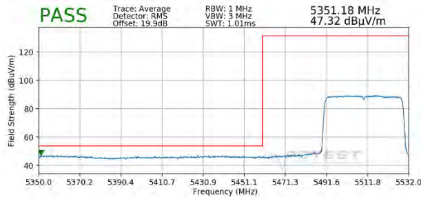
Plot 7-393. Radiated Lower Band Edge Plot SISO ANT2 (Average - UNII Band 2C - 484 Tones)
