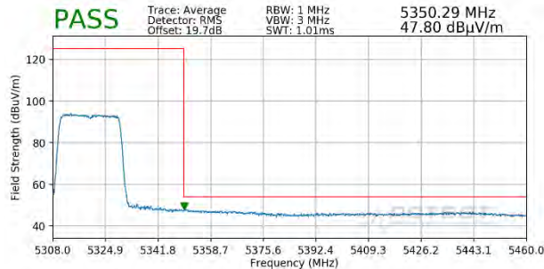
Plot 7-384. Radiated Upper Band Edge Plot SISO ANT2 (Average - UNII Band 2A - 242 Tones)
