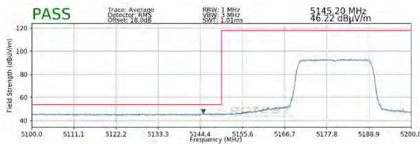
Plot 7-361. Radiated Lower Band Edge Plot SISO ANT1 (Average - UNII Band 1 - 242 Tones)
