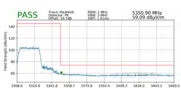
Plot 7-385. Radiated Upper Band Edge Plot SISO ANT2 (Peak - UNII Band 2A - 242 Tones)
