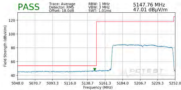
Plot 7-396. Radiated Lower Band Edge Plot SISO ANT2 (Average - UNII Band 1 - 996 Tones)
