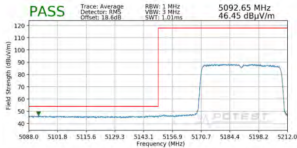
Plot 7-389. Radiated Lower Band Edge Plot SISO ANT2 (Average - UNII Band 1 - 484 Tones)
