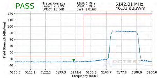
Plot 7-382. Radiated Lower Band Edge Plot SISO ANT2 (Average - UNII Band 1 - 242 Tones)
