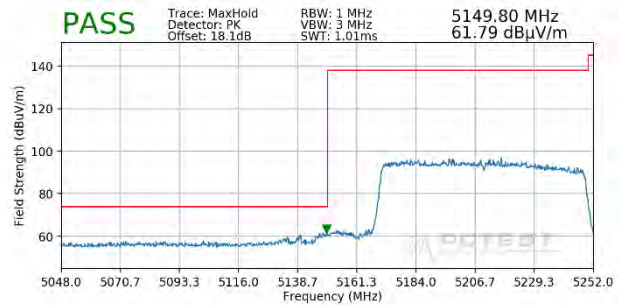
Plot 7-397. Radiated Lower Band Edge Plot SISO ANT2 (Peak - UNII Band 1 - 996 Tones)
