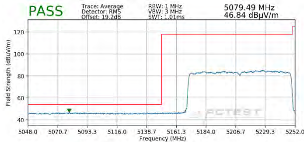
Plot 7-417. Radiated Lower Band Edge Plot MIMO (Average – UNII Band 1 – 996 Tones)
