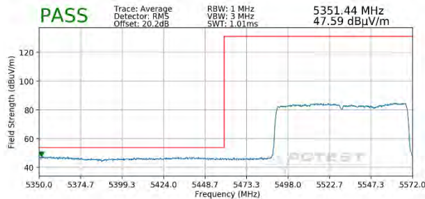
Plot 7-421. Radiated Lower Band Edge Plot MIMO (Average - UNII Band 2C - 996 Tones)
