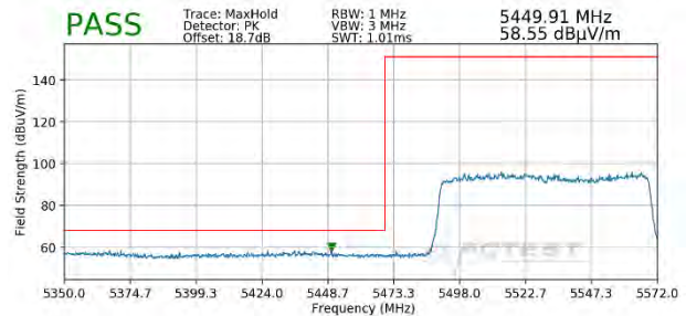
Plot 7-422. Radiated Lower Band Edge Plot MIMO (Peak - UNII Band 2C - 996 Tones)
