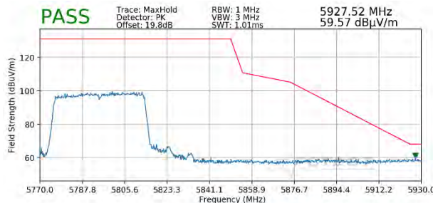
Plot 7-416. Radiated Upper Band Edge Plot MIMO (Peak - UNII Band 3 - 484 Tones)
