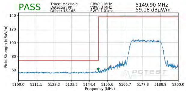
Plot 7-383. Radiated Lower Band Edge Plot SISO ANT2 (Peak - UNII Band 1 - 242 Tones)
