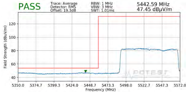
Plot 7-379. Radiated Lower Band Edge Plot SISO ANT1 (Average – UNII Band 2C – 996 Tones)
