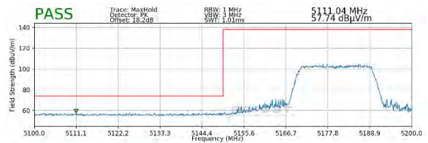
Plot 7-362. Radiated Lower Band Edge Plot SISO ANT1 (Peak - UNII Band 1 - 242 Tones)
