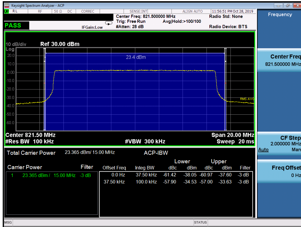
Plot 7-35. Channel Edge Plot (LTE Band 26 - 15MHz QPSK)
