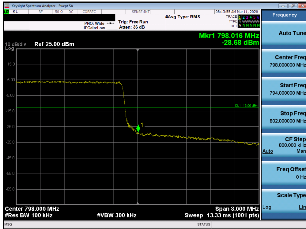
Plot 7-45. Upper Band Edge Plot (Band 14 - 10MHz QPSK - Full RB Configuration)
