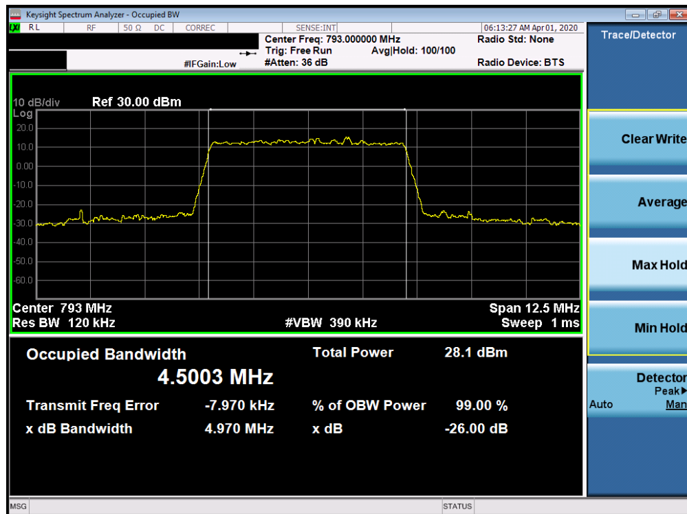
Plot 7-28. Occupied Bandwidth Plot (Band 14 - 5MHz 256-QAM - Full RB Configuration)
