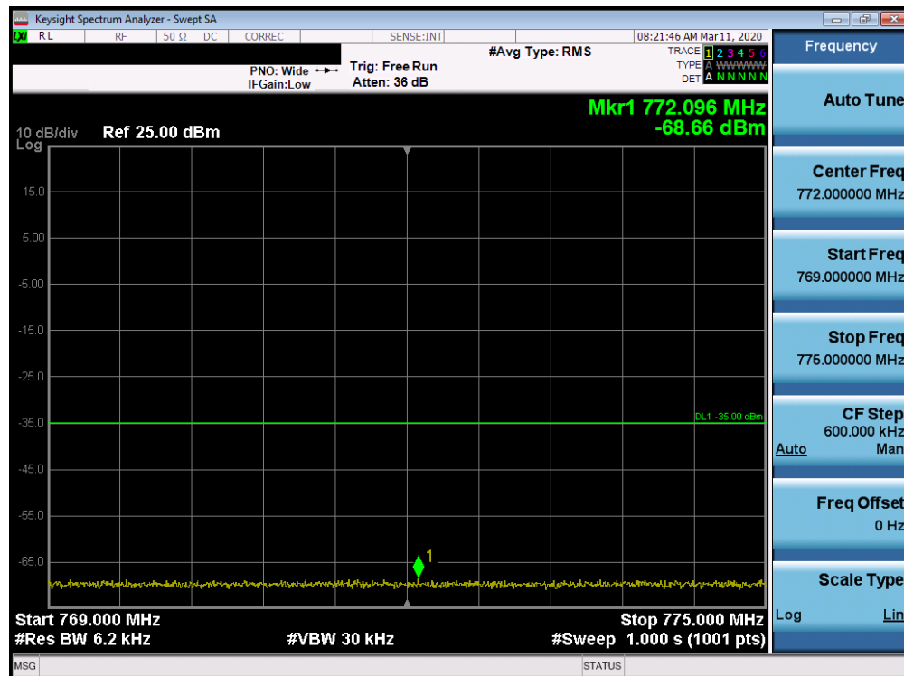
Plot 7-48. Lower Extended Band Edge Plot (Band 14 - 5MHz QPSK - Full RB Configuration)
