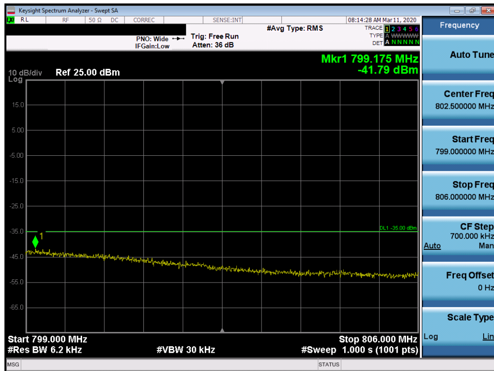
Plot 7-46. Upper Extended Band Edge Plot (Band 14 - 10MHz QPSK - Full RB Configuration)
