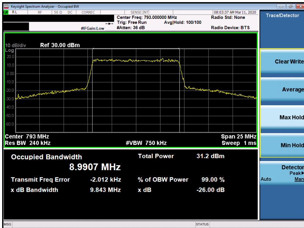
Plot 7-22. Occupied Bandwidth Plot (Band 14 - 10MHz 16-QAM - Full RB Configuration)
