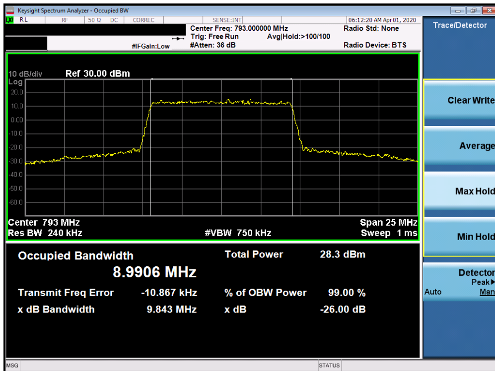
Plot 7-24. Occupied Bandwidth Plot (Band 14 - 10MHz 256-QAM - Full RB Configuration)
