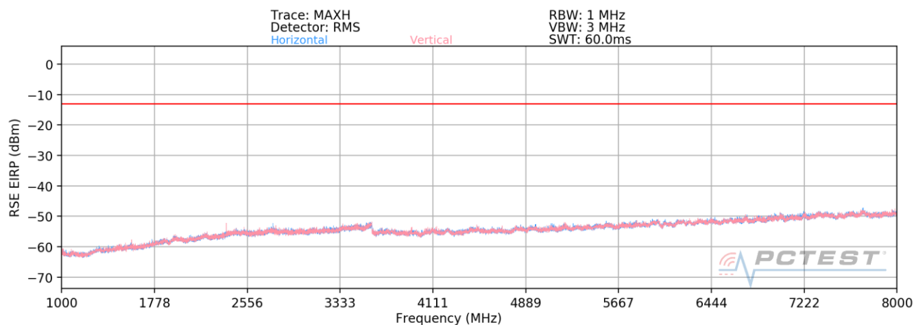
Plot 7-54. Radiated Spurious Plot (Band 14)
