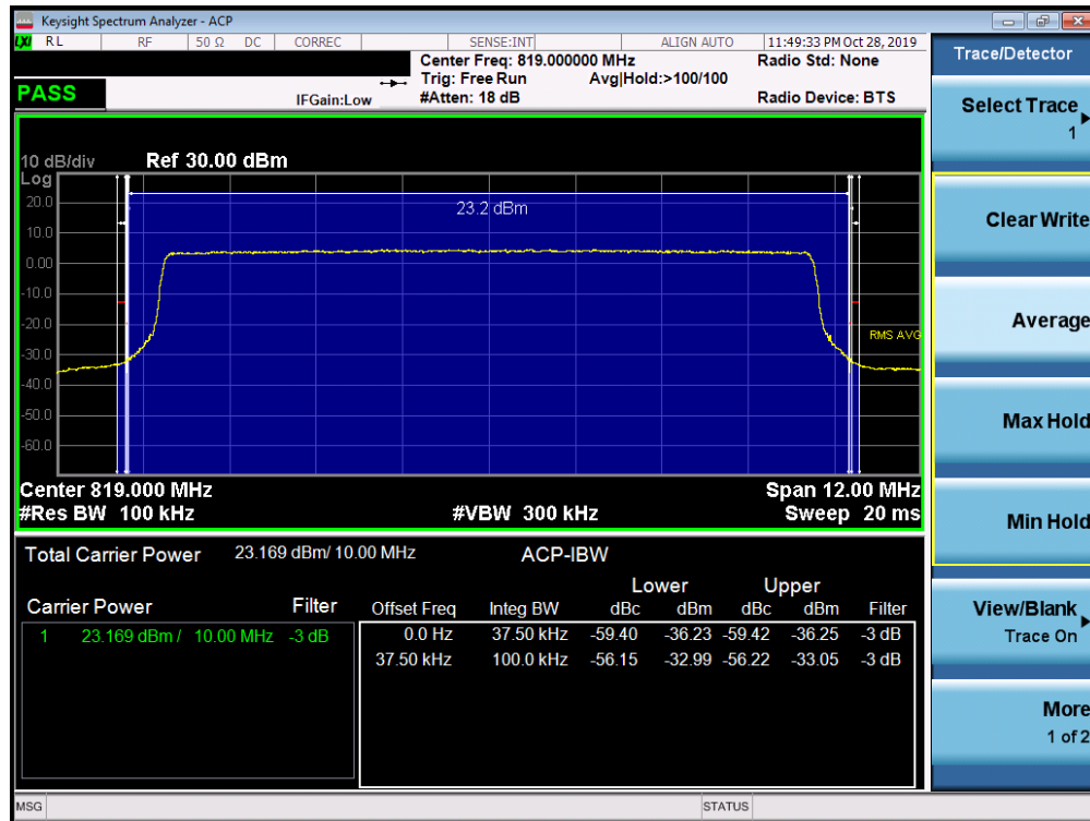
Plot 7-36. Channel Edge Plot (LTE Band 26 - 10MHz QPSK)
