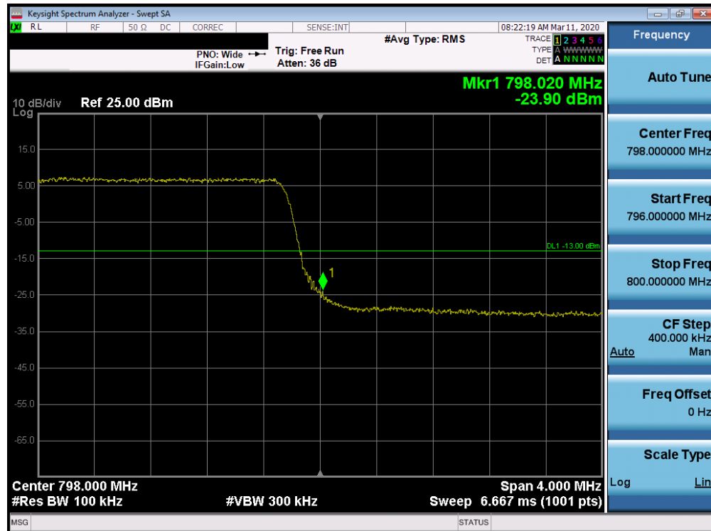
Plot 7-49. Upper Band Edge Plot (Band 14 - 5MHz QPSK - Full RB Configuration)
