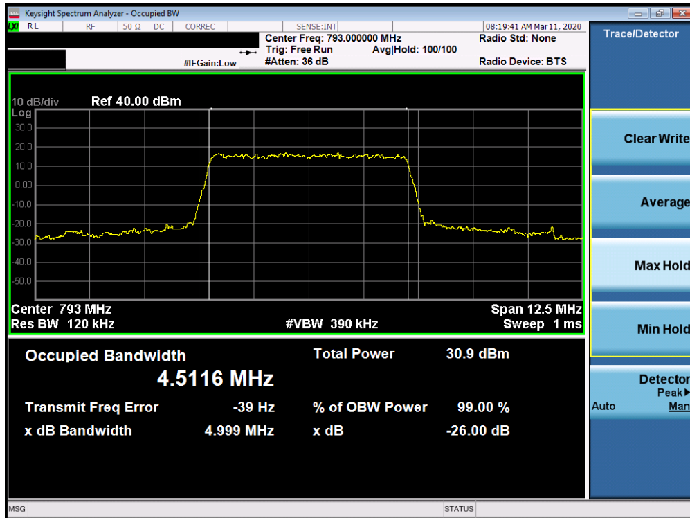
Plot 7-26. Occupied Bandwidth Plot (Band 14 - 5MHz 16-QAM - Full RB Configuration)
