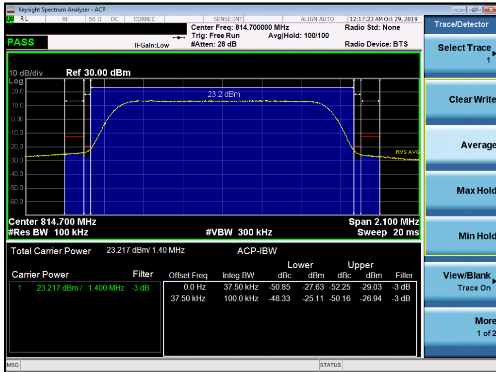
Plot 7-41. Channel Edge Plot (LTE Band 26 - 1.4MHz QPSK - Low Channel)
