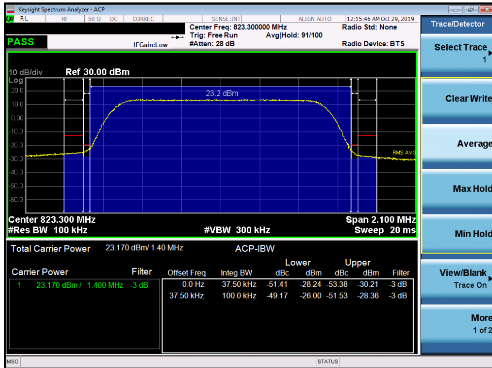
Plot 7-42. Channel Edge Plot (LTE Band 26 - 1.4MHz QPSK - High Channel)
