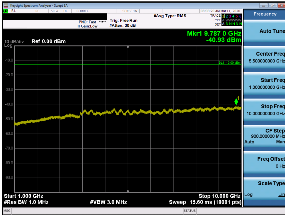
Plot 7-34. Conducted Spurious Plot (Band 14 - 10MHz QPSK - RB Size 1, RB Offset 0 - Mid Channel)
