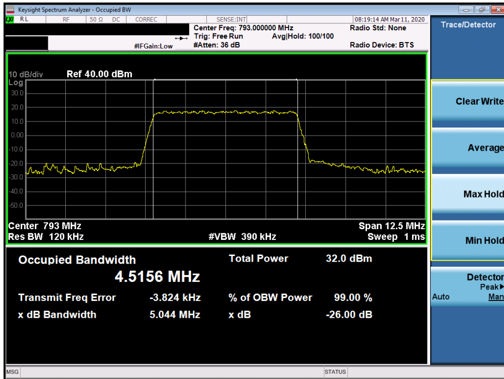
Plot 7-25. Occupied Bandwidth Plot (Band 14 - 5MHz QPSK - Full RB Configuration)
