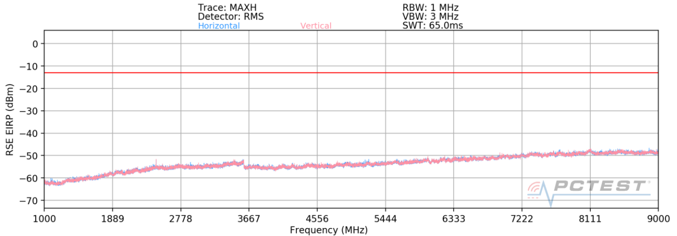
Plot 7-53. Radiated Spurious Plot (Band 26)
