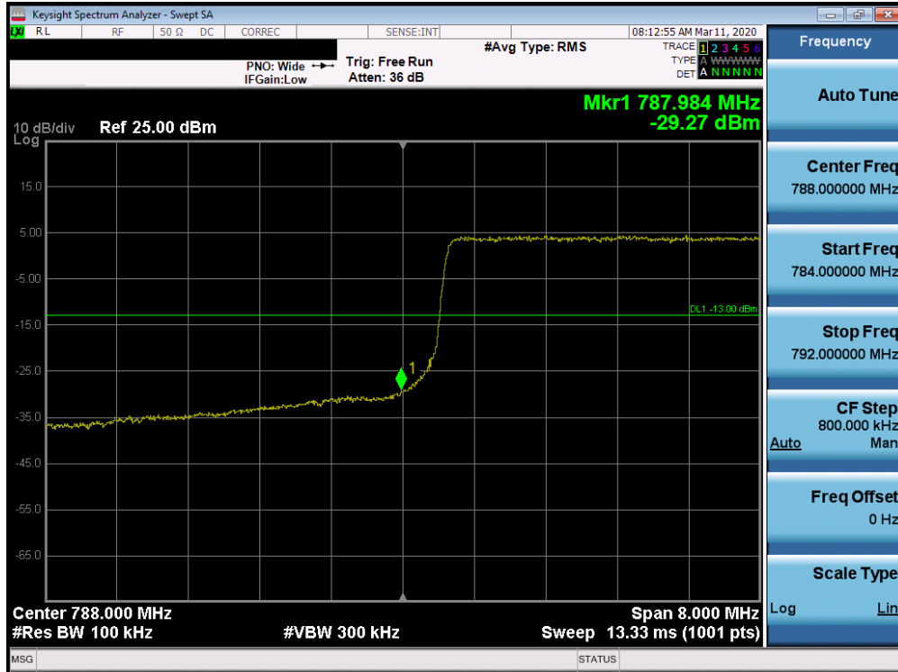
Plot 7-43. Lower Band Edge Plot (Band 14 - 10MHz QPSK - Full RB Configuration)
