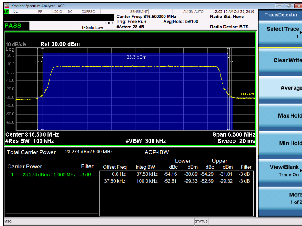
Plot 7-37. Channel Edge Plot (LTE Band 26 - 5MHz QPSK - Low Channel)
