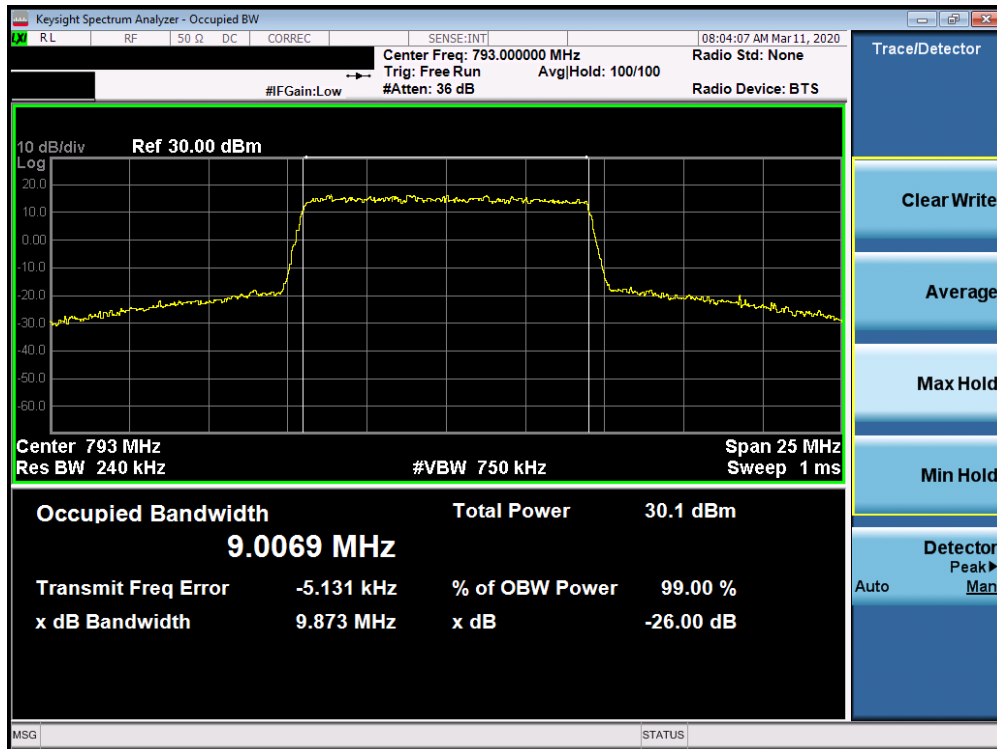
Plot 7-23. Occupied Bandwidth Plot (Band 14 - 10MHz 64-QAM - Full RB Configuration)
