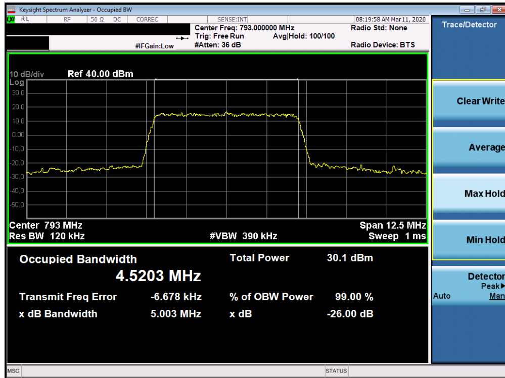
Plot 7-27. Occupied Bandwidth Plot (Band 14 - 5MHz 64-QAM - Full RB Configuration)
