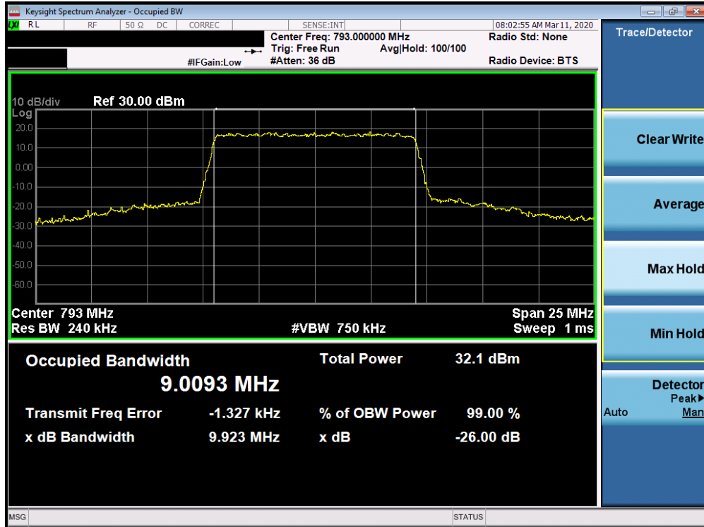
Plot 7-21. Occupied Bandwidth Plot (Band 14 - 10MHz QPSK - Full RB Configuration)
