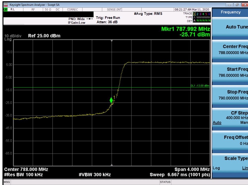
Plot 7-47. Lower Band Edge Plot (Band 14 - 5MHz QPSK - Full RB Configuration)
