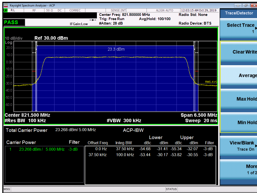
Plot 7-38. Channel Edge Plot (LTE Band 26 - 5MHz QPSK - High Channel)
