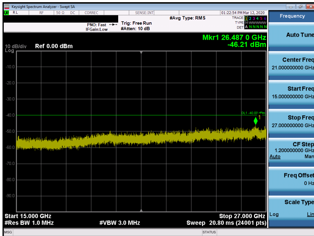
Plot 7-58. Conducted Spurious Plot (LTE Band 48 - 20.0MHz QPSK - RB Size 1, RB Offset 0 - Low Channel)
