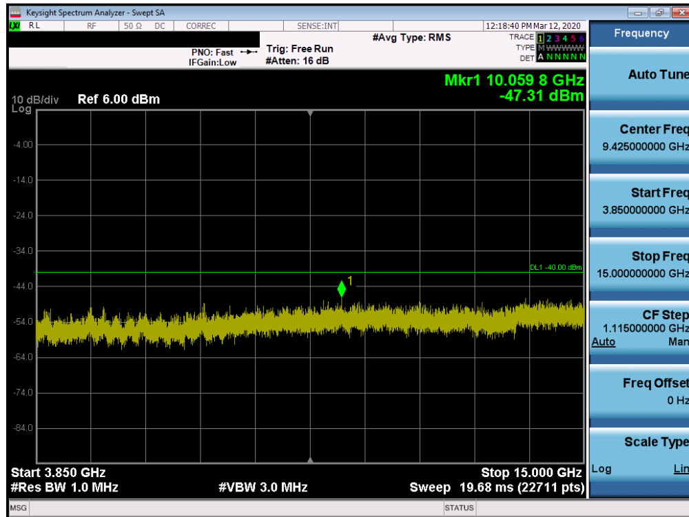
Plot 7-63. Conducted Spurious Plot (LTE Band 48 - 20.0MHz QPSK - RB Size 1, RB Offset 0 – Mid Channel)
