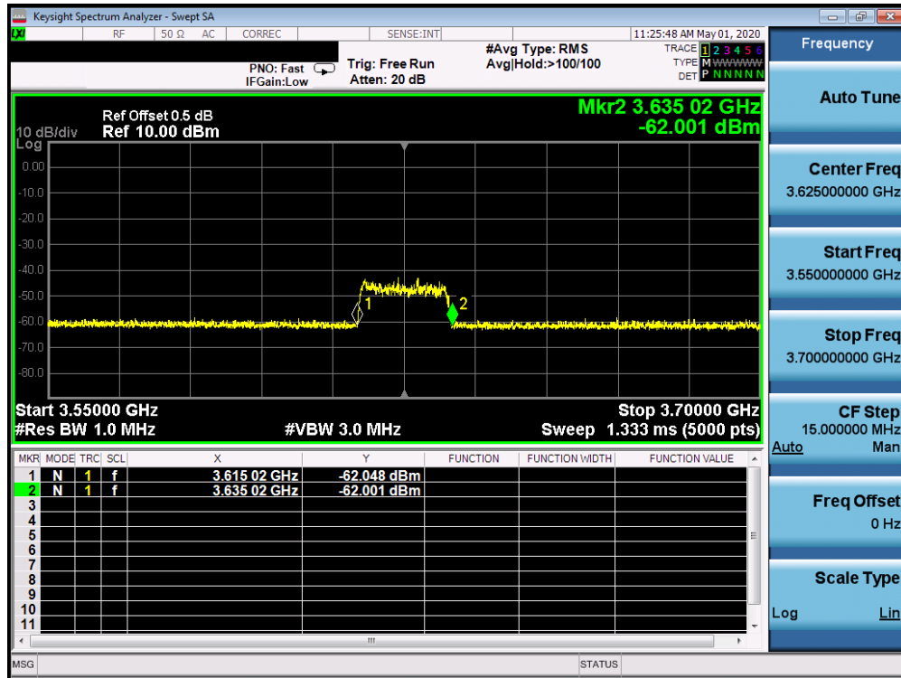
Plot 7-80. Run#1 End User Device Frequency of Operations
