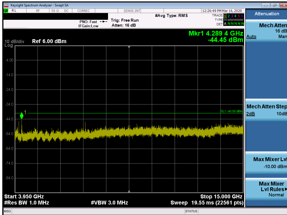
Plot 7-69. Conducted Spurious Plot (LTE Band 48 - 20.0MHz QPSK - RB Size 1, RB Offset 0 – High Channel)
