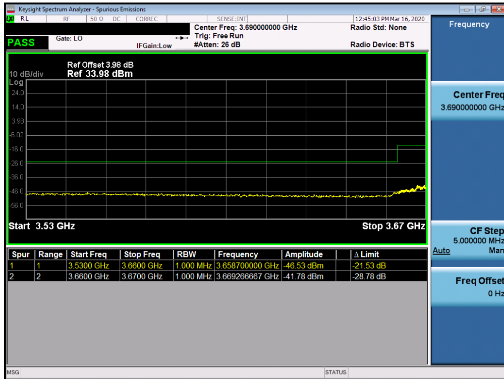
Plot 7-67. Conducted Spurious Plot (LTE Band 48 - 20.0MHz QPSK - RB Size 1, RB Offset 0 – High Channel)
