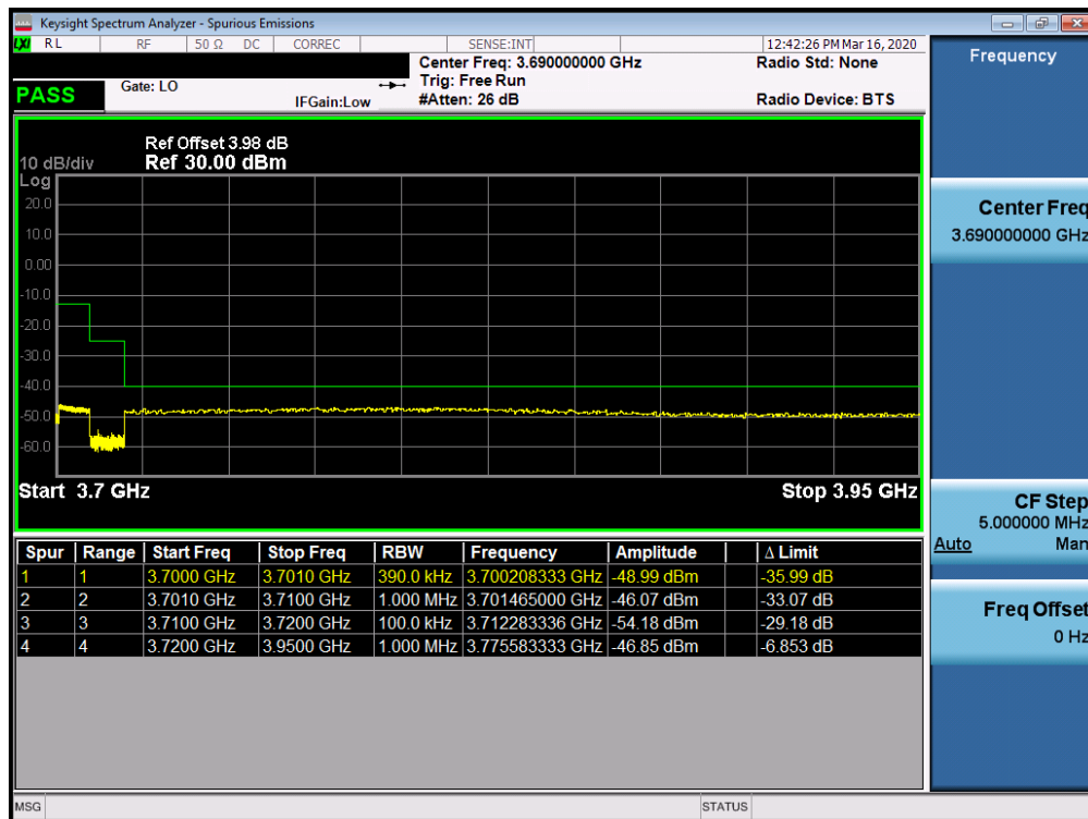
Plot 7-68. Conducted Spurious Plot (LTE Band 48 - 20.0MHz QPSK - RB Size 1, RB Offset 0 – High Channel)
