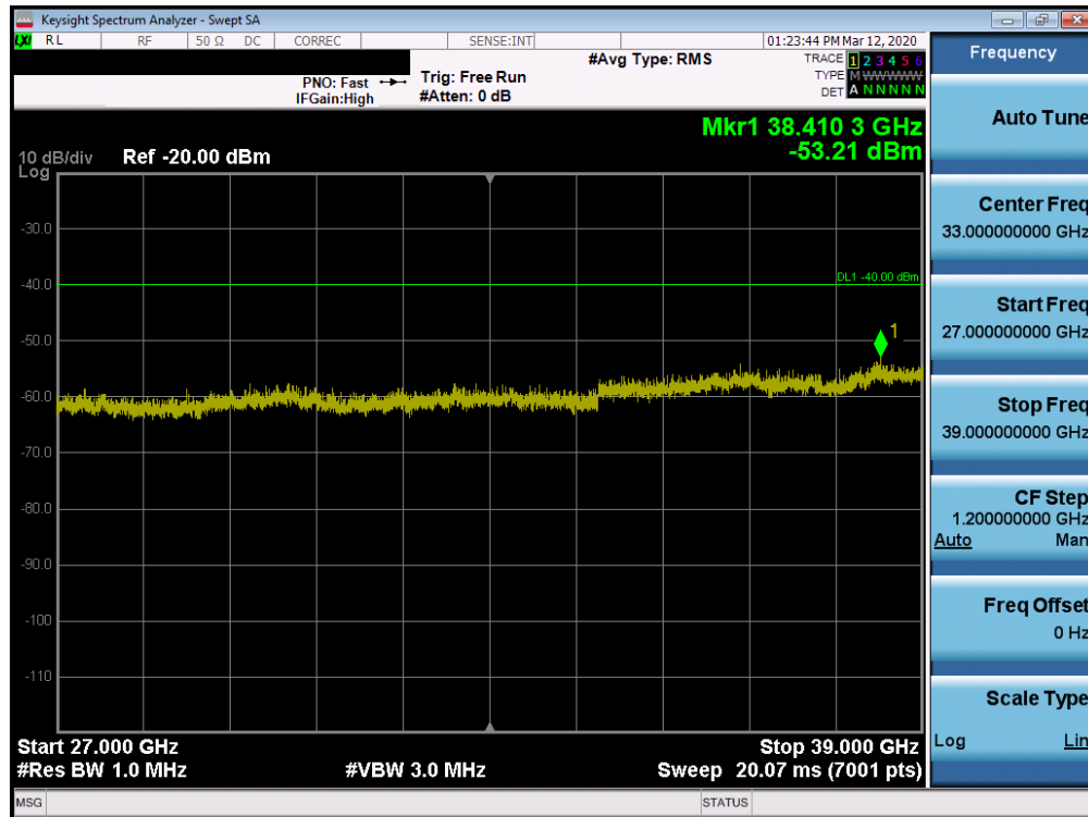
Plot 7-59. Conducted Spurious Plot (LTE Band 48 - 20.0MHz QPSK - RB Size 1, RB Offset 0 - Low Channel)
