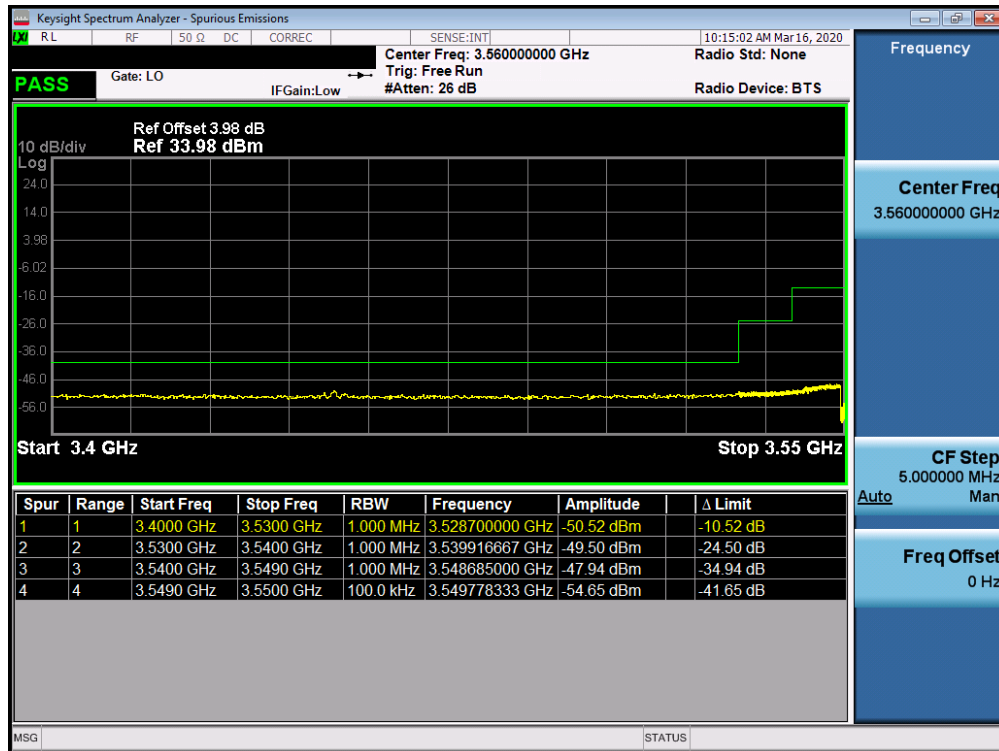
Plot 7-55. Conducted Spurious Plot (LTE Band 48 - 20.0MHz QPSK - RB Size 1, RB Offset 0 - Low Channel)
