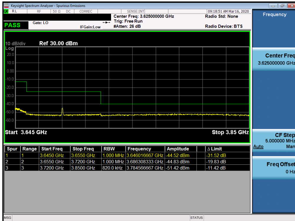
Plot 7-62. Conducted Spurious Plot (LTE Band 48 - 20.0MHz QPSK - RB Size 1, RB Offset 0 – Mid Channel)
