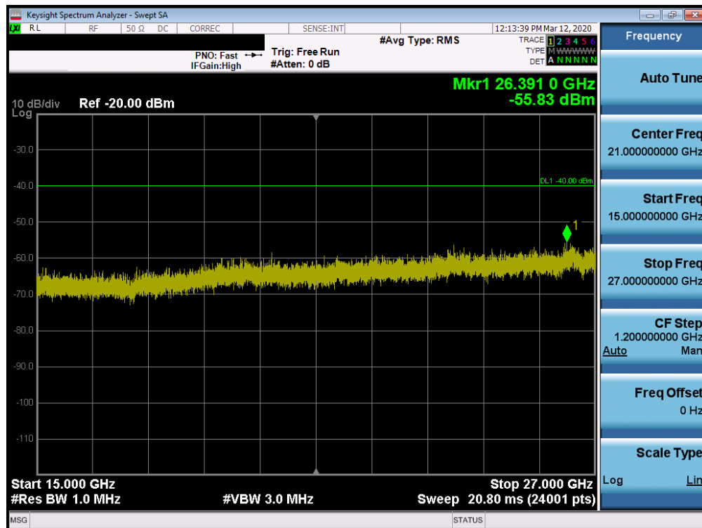
Plot 7-64. Conducted Spurious Plot (LTE Band 48 - 20.0MHz QPSK - RB Size 1, RB Offset 0 – Mid Channel)
