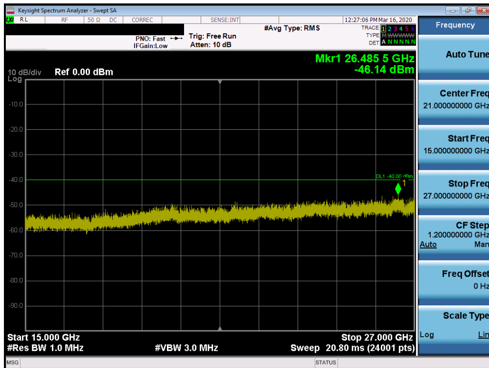
Plot 7-70. Conducted Spurious Plot (LTE Band 48 - 20.0MHz QPSK - RB Size 1, RB Offset 0 – High Channel)
