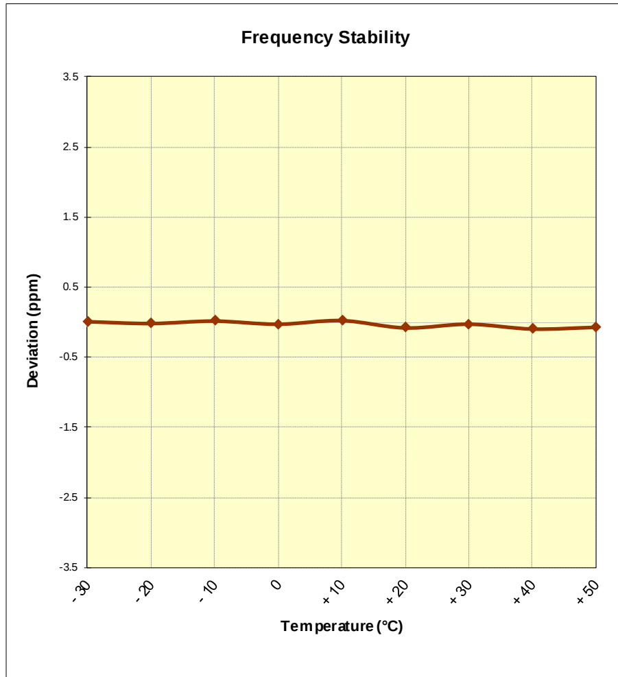
Figure 7-9. Frequency Stability Graph (LTE Band 48)
