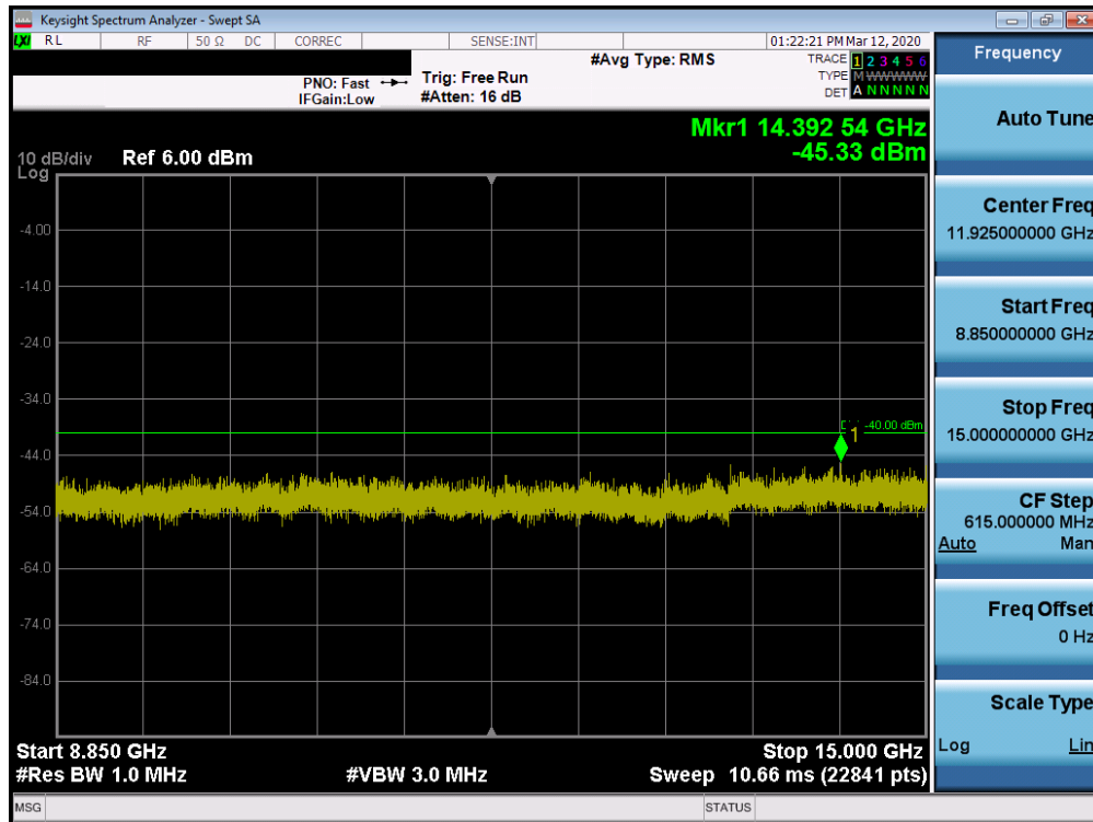
Plot 7-57. Conducted Spurious Plot (LTE Band 48 - 20.0MHz QPSK - RB Size 1, RB Offset 0 - Low Channel)
