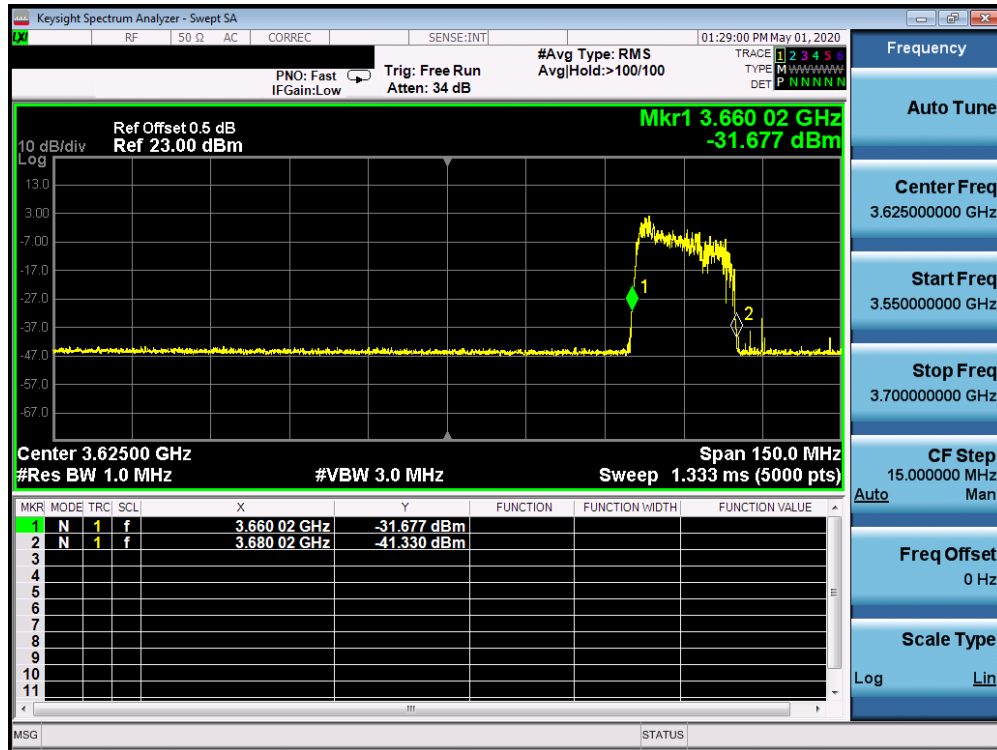
Plot 7-82. Run#2 End User Device Frequency of Operations
