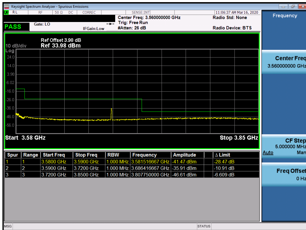
Plot 7-56. Conducted Spurious Plot (LTE Band 48 - 20.0MHz QPSK - RB Size 1, RB Offset 0 - Low Channel)
