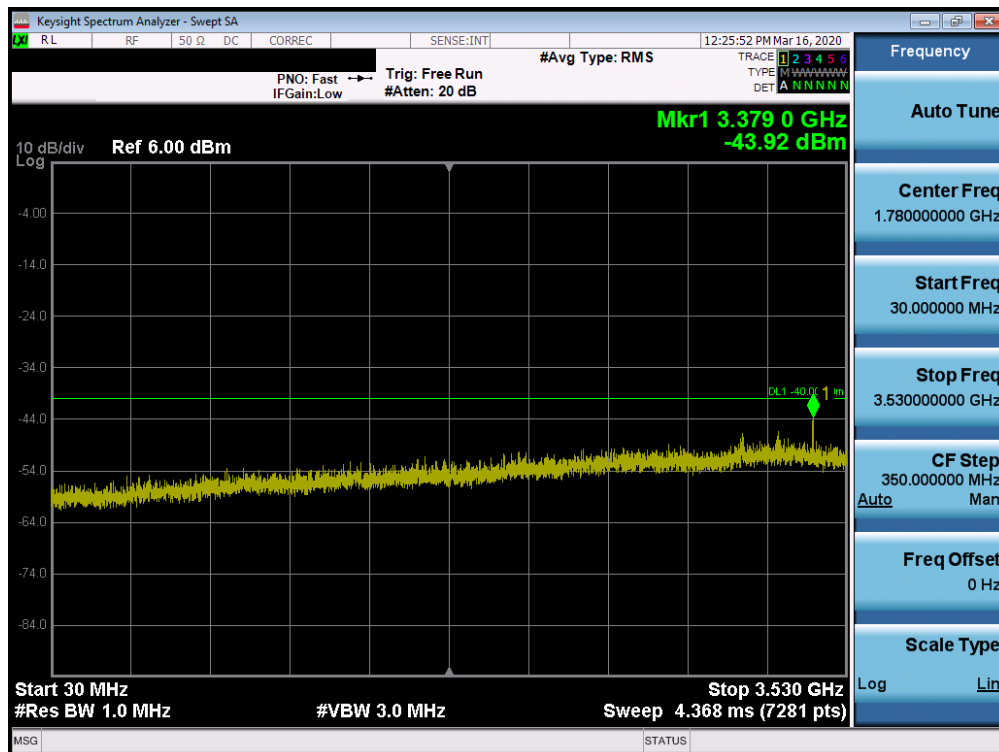
Plot 7-66. Conducted Spurious Plot (LTE Band 48 - 20.0MHz QPSK - RB Size 1, RB Offset 0 – High Channel)
