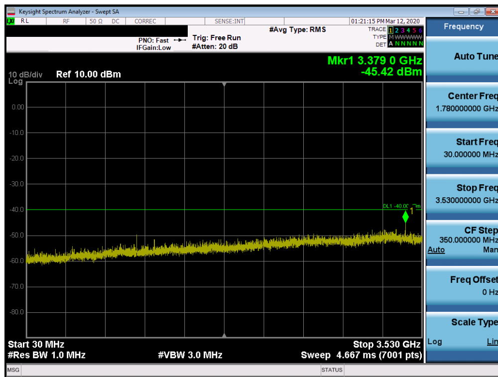
Plot 7-54. Conducted Spurious Plot (LTE Band 48 - 20.0MHz QPSK - RB Size 1, RB Offset 0 - Low Channel)
