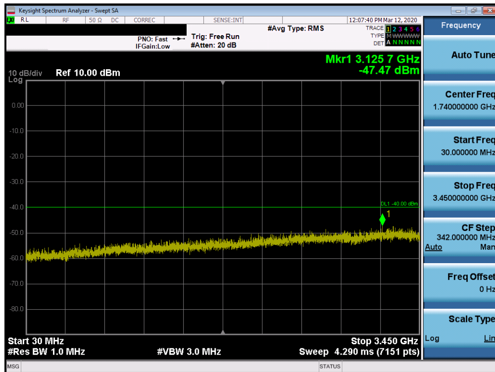
Plot 7-60. Conducted Spurious Plot (LTE Band 48 - 20.0MHz QPSK - RB Size 1, RB Offset 0 - Mid Channel)
