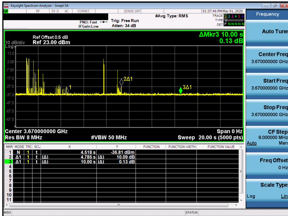
Plot 7-83. Run#2 End User Device Discontinues Operations within 10s
