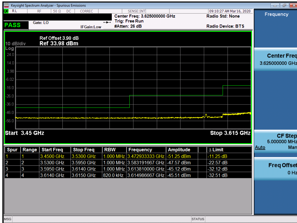
Plot 7-61. Conducted Spurious Plot (LTE Band 48 - 20.0MHz QPSK - RB Size 1, RB Offset 0 – Mid Channel)
