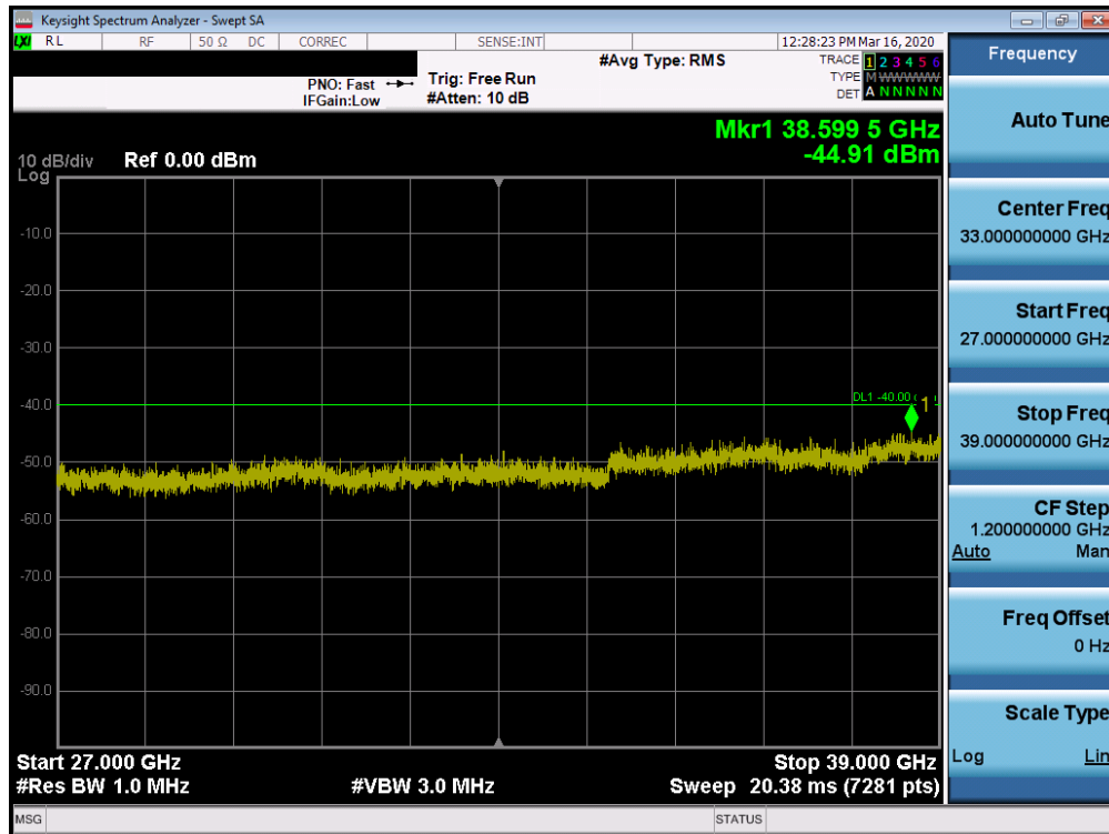
Plot 7-71. Conducted Spurious Plot (LTE Band 48 - 20.0MHz QPSK - RB Size 1, RB Offset 0 – High Channel)
