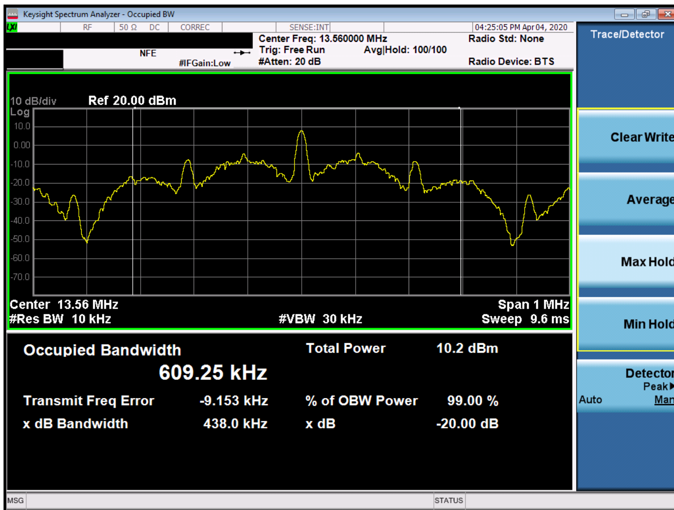
Figure 7-2. Occupied Bandwidth Plot
