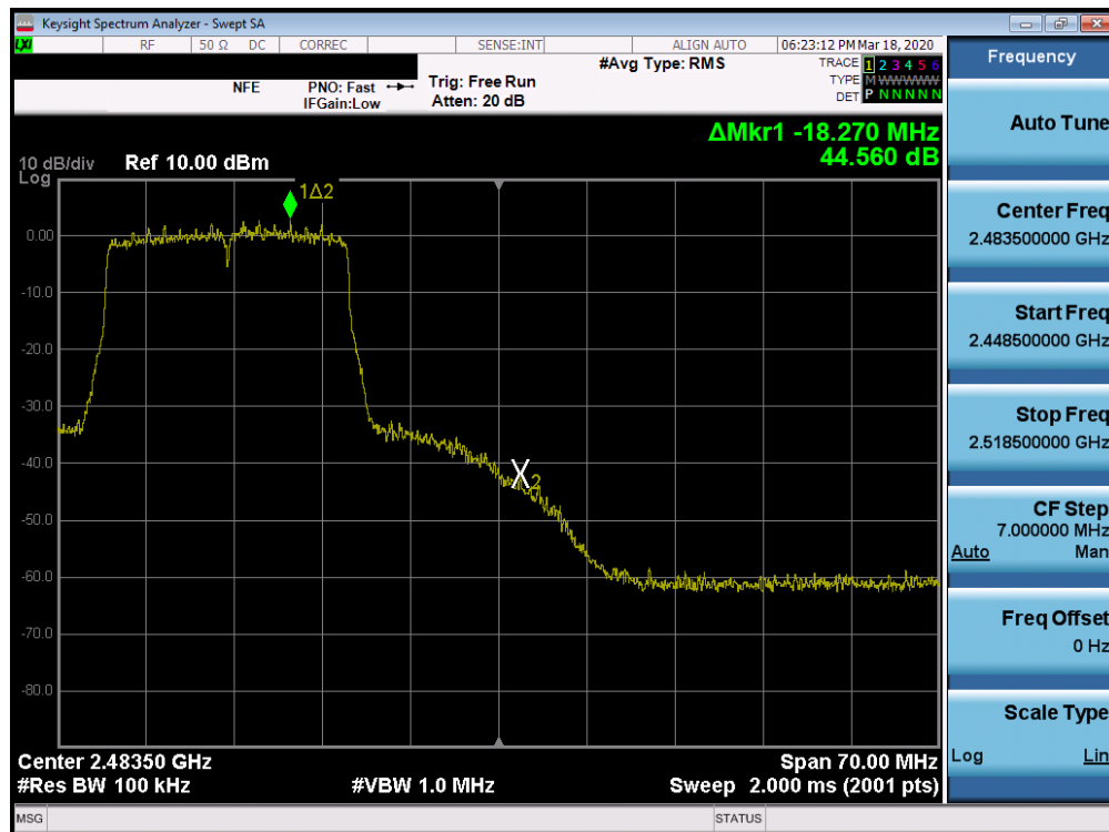
Plot 7-46. Band Edge Plot SISO ANT1 (802.11ax (2.4GHz) – Ch. 11)
