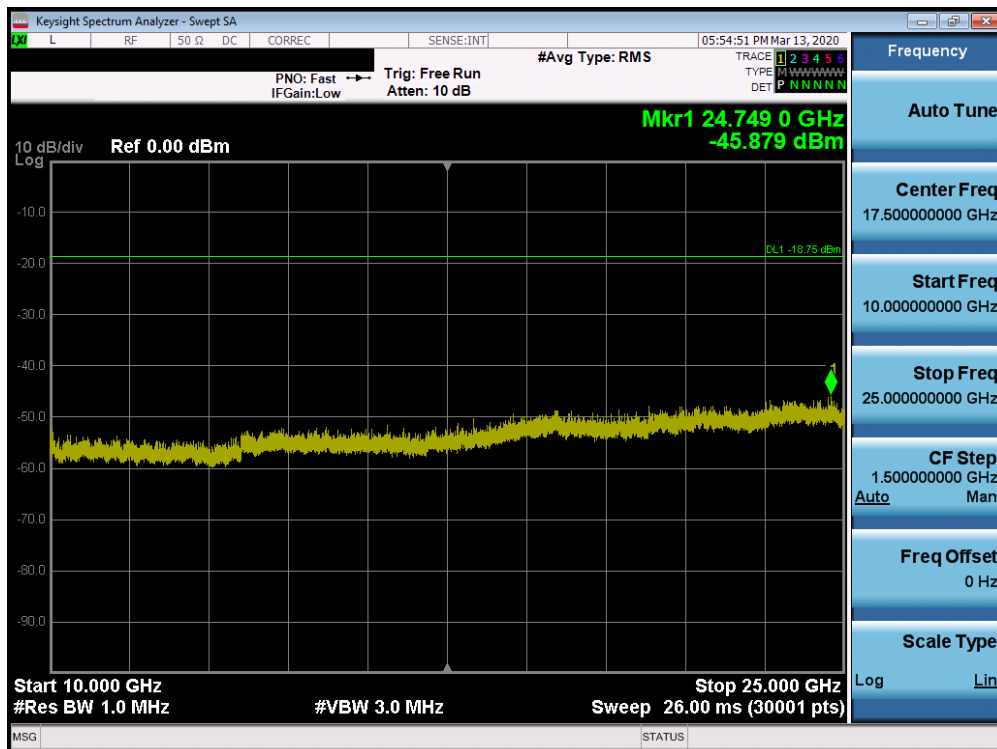
Plot 7-66. Conducted Spurious Plot SISO ANT2 (802.11b – Ch. 6)
