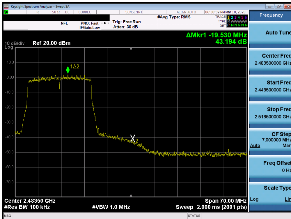
Plot 7-56. Band Edge Plot SISO ANT2 (802.11ax (2.4GHz) – Ch. 11)
