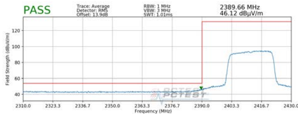
Plot 7-89. Radiated Restricted Lower Band Edge Measurement MIMO (Average)
