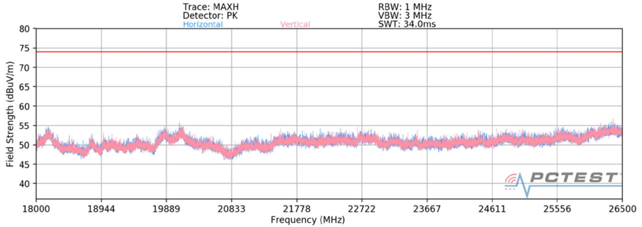
Plot 7-80. Radiated Spurious Plot above 18GHz MIMO/CDD
