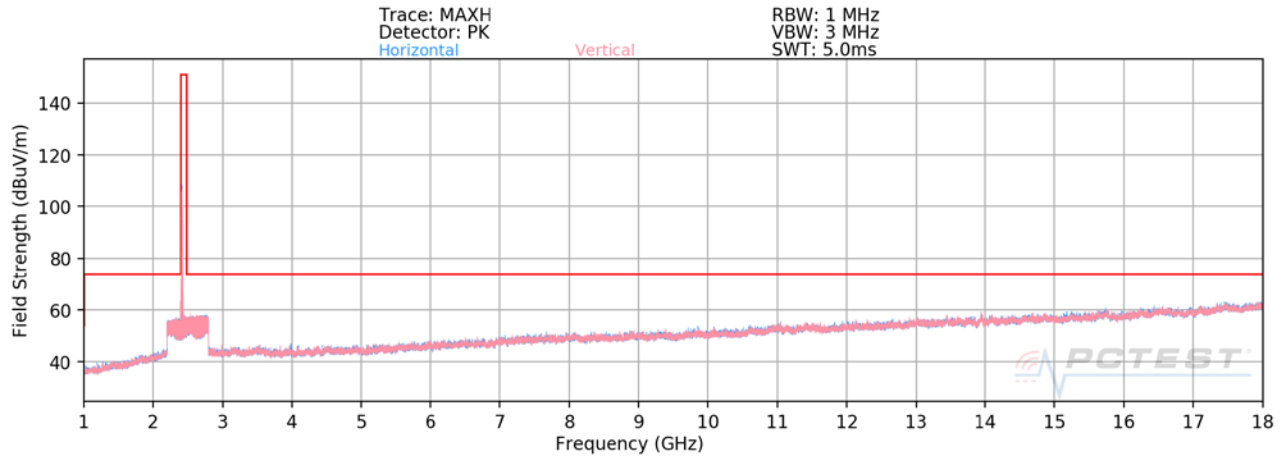
Plot 7-69. Radiated Spurious Plot above 1GHz SISO ANT1 (802.11b – Ch. 1)
