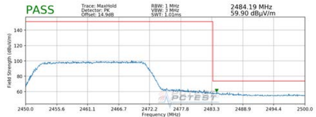
Plot 7-88. Radiated Restricted Upper Band Edge Measurement SISO ANT2 (Peak)
