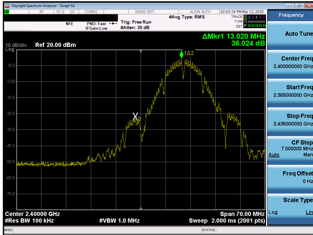
Plot 7-47. Band Edge Plot SISO ANT2 (802.11b – Ch. 1)
