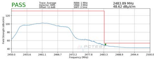
Plot 7-93. Radiated Restricted Band Edge Measurement MIMO with WCP (Average)
