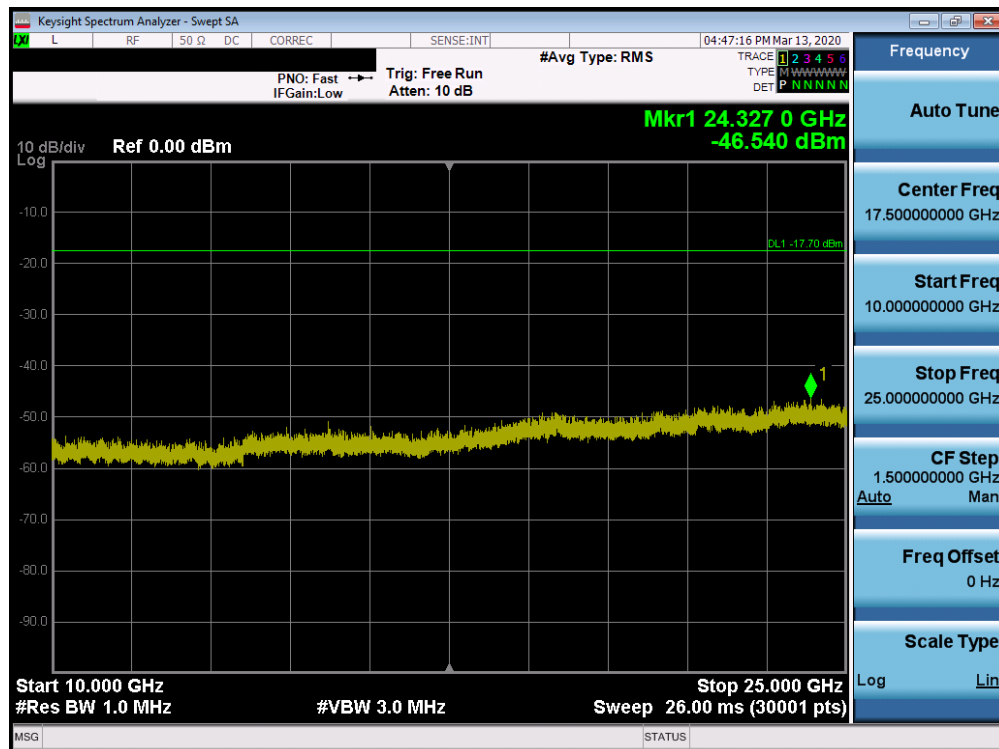
Plot 7-60. Conducted Spurious Plot SISO ANT1 (802.11b – Ch. 6)
