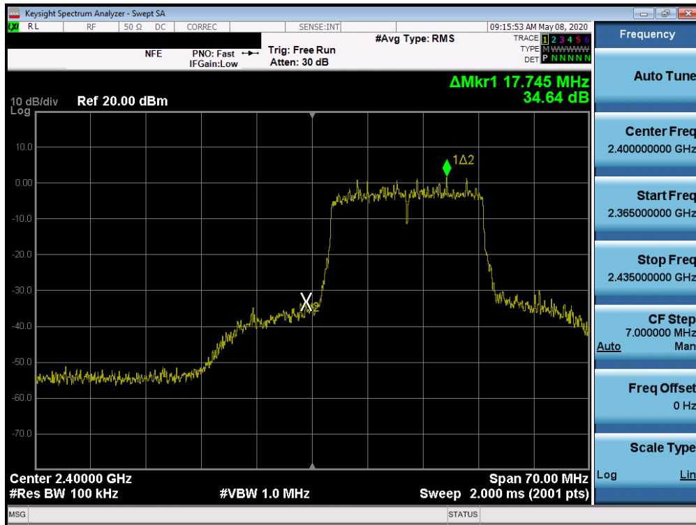
Plot 7-53. Band Edge Plot SISO ANT2 (802.11ax (2.4GHz) – Ch. 1)
