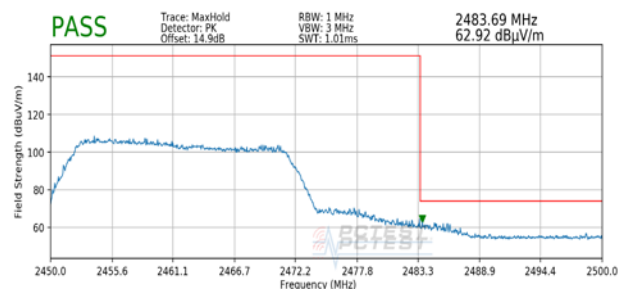
Plot 7-84. Radiated Restricted Upper Band Edge Measurement SISO ANT1 (Peak)
