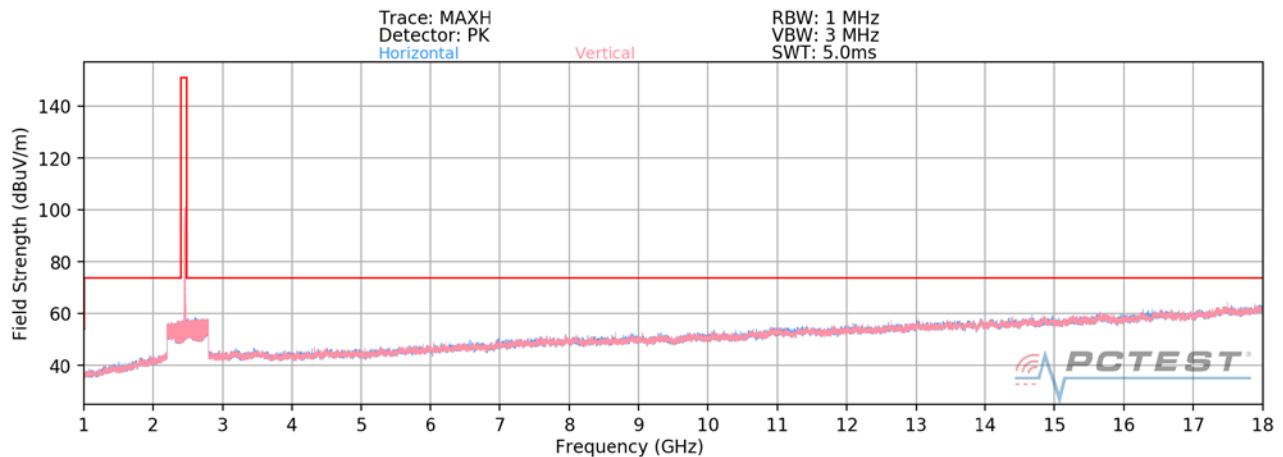
Plot 7-75. Radiated Spurious Plot above 1GHz SISO ANT2 (802.11b – Ch. 11)
