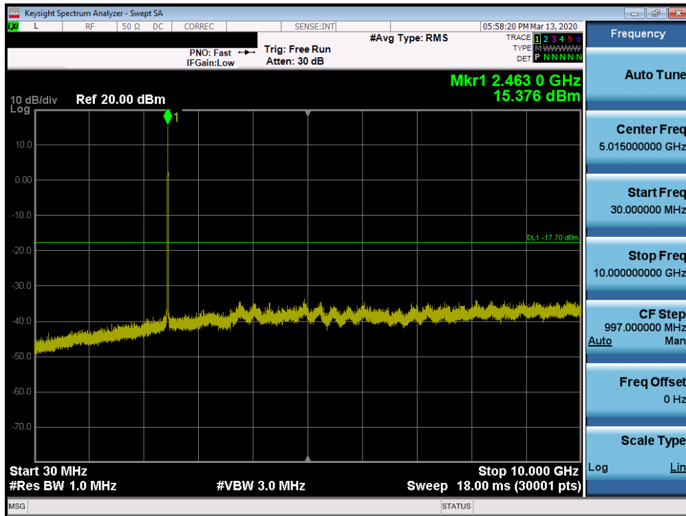
Plot 7-67. Conducted Spurious Plot SISO ANT2 (802.11b – Ch. 11)
