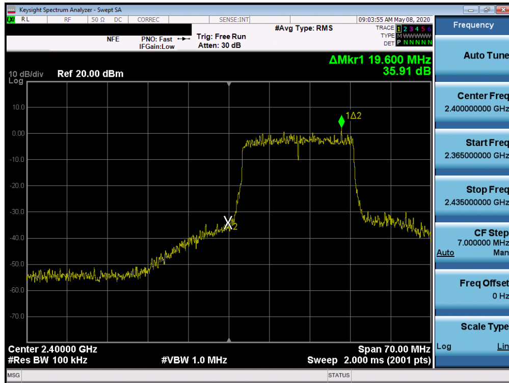
Plot 7-43. Band Edge Plot SISO ANT1 (802.11ax (2.4GHz) – Ch. 1)
