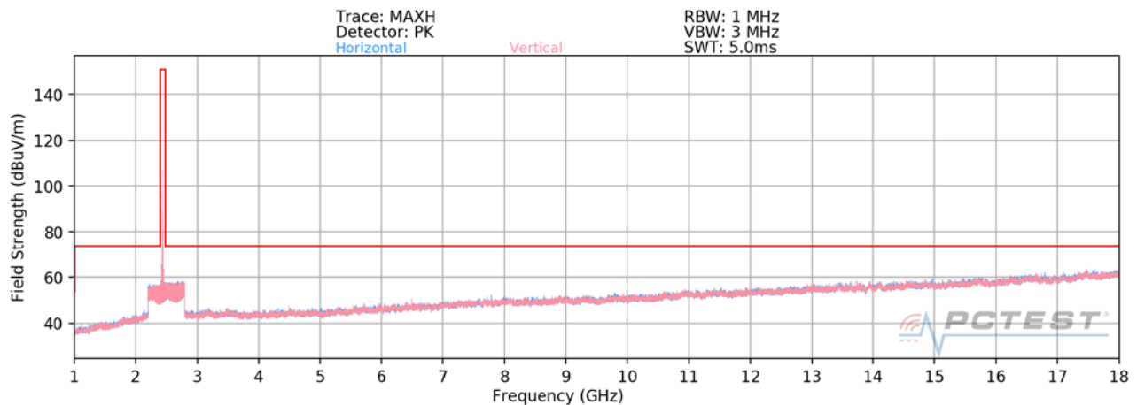
Plot 7-70. Radiated Spurious Plot above 1GHz SISO ANT1 (802.11b – Ch. 6)
