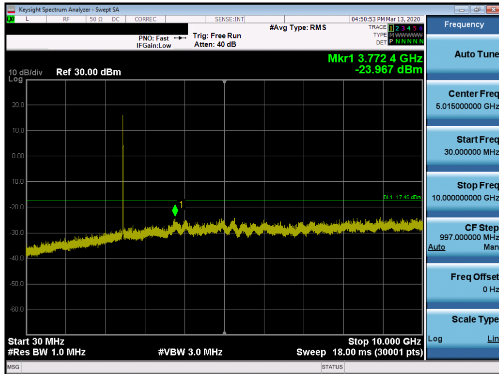
Plot 7-61. Conducted Spurious Plot SISO ANT1 (802.11b – Ch. 11)
