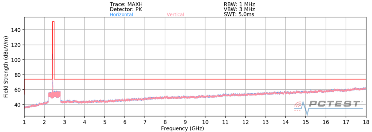
Plot 7-77. Radiated Spurious Plot above 1GHz MIMO/CDD (802.11g – Ch. 1)
