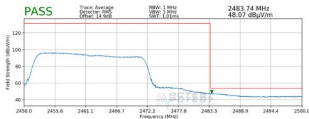
Plot 7-83. Radiated Restricted Upper Band Edge Measurement SISO ANT1 (Average)
