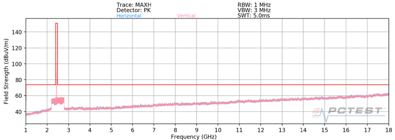
Plot 7-74. Radiated Spurious Plot above 1GHz SISO ANT2 (802.11b – Ch. 6)
