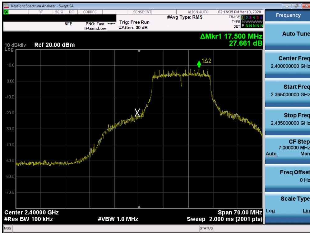
Plot 7-49. Band Edge Plot SISO ANT2 (802.11g- Ch. 1)
