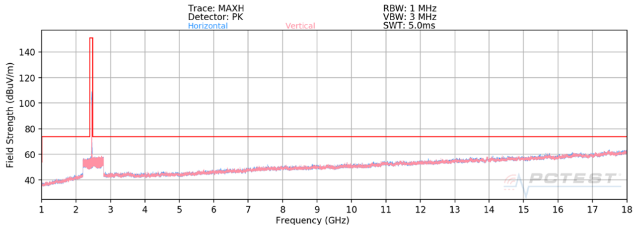
Plot 7-79. Radiated Spurious Plot above 1GHz MIMO/CDD (802.11g – Ch. 11)
