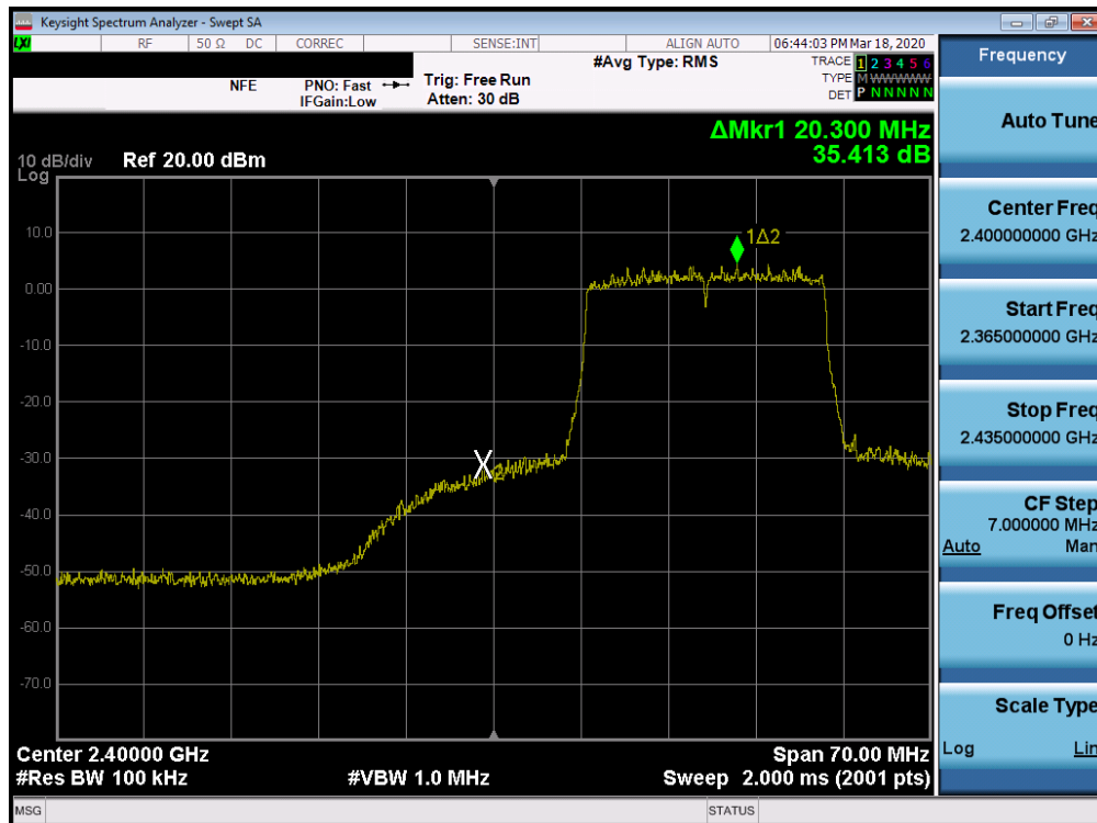
Plot 7-54. Band Edge Plot SISO ANT2 (802.11ax (2.4GHz) – Ch. 2)
