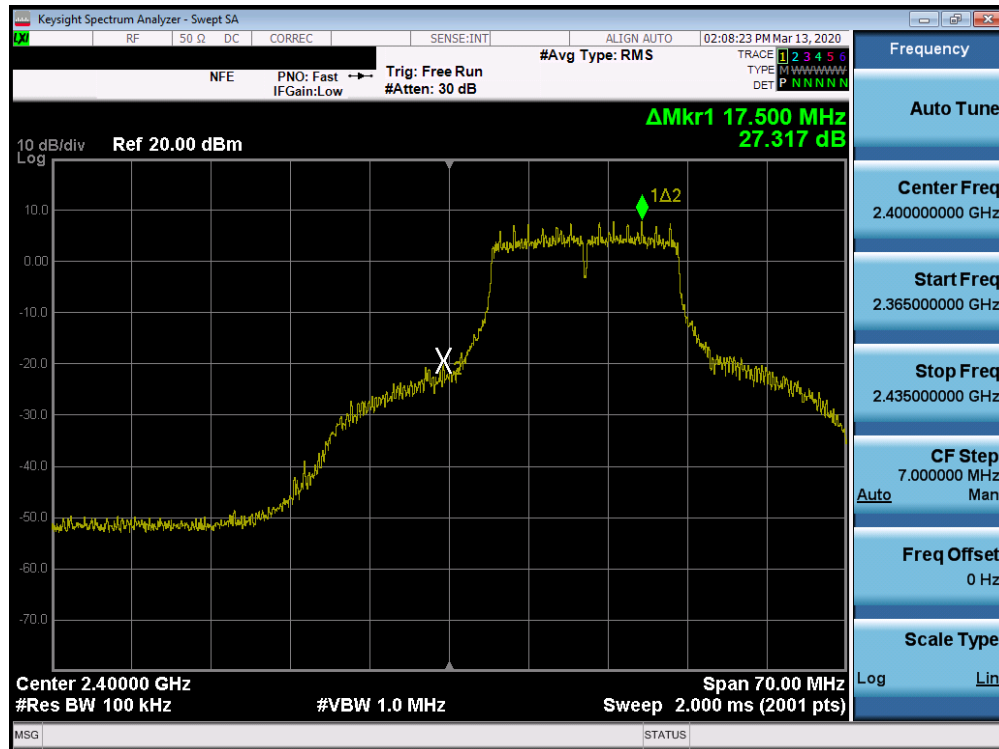
Plot 7-51. Band Edge Plot SISO ANT2 (802.11n (2.4GHz) – Ch. 1)
