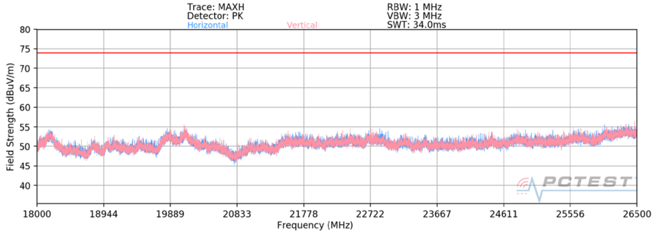
Plot 7-72. Radiated Spurious Plot above 18GHz SISO ANT1
