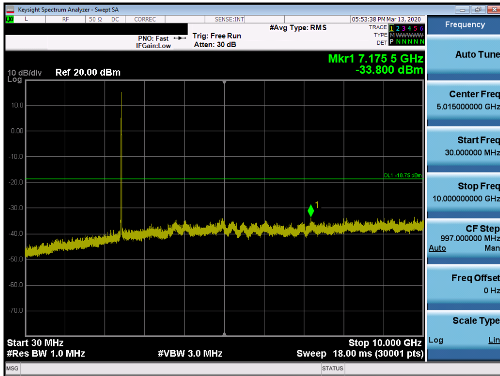
Plot 7-65. Conducted Spurious Plot SISO ANT2 (802.11b – Ch. 6)
