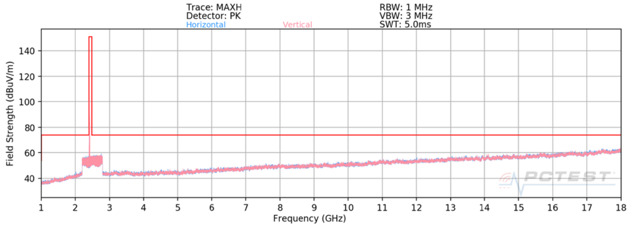
Plot 7-73. Radiated Spurious Plot above 1GHz SISO ANT2 (802.11b – Ch. 1)
