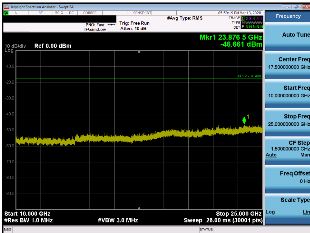
Plot 7-68. Conducted Spurious Plot SISO ANT2 (802.11b – Ch. 11)
