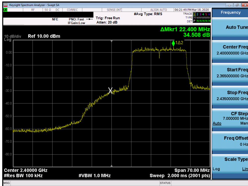
Plot 7-44. Band Edge Plot SISO ANT1 (802.11ax (2.4GHz) – Ch. 2)
