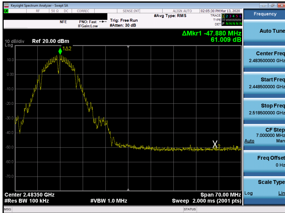
Plot 7-48. Band Edge Plot SISO ANT2 (802.11b – Ch. 11)
