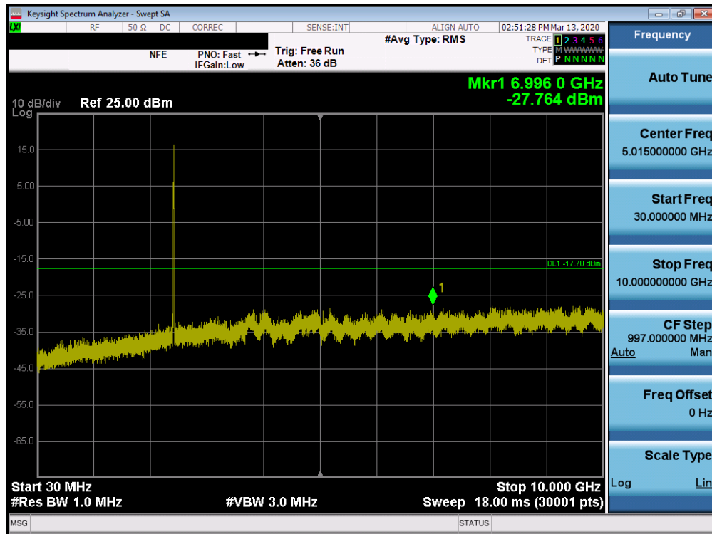
Plot 7-59. Conducted Spurious Plot SISO ANT1 (802.11b – Ch. 6)
