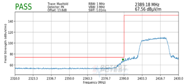
Plot 7-82. Radiated Restricted Lower Band Edge Measurement SISO ANT1 (Peak)
