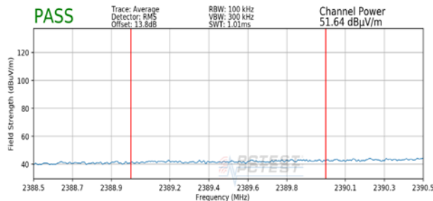
Plot 7-81. Radiated Restricted Lower Band Edge Measurement SISO ANT1 (Average)
