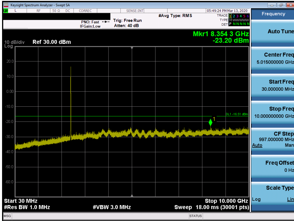
Plot 7-63. Conducted Spurious Plot SISO ANT2 (802.11b – Ch. 1)
