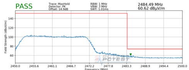
Plot 7-92. Radiated Restricted Upper Band Edge Measurement MIMO (Peak)
