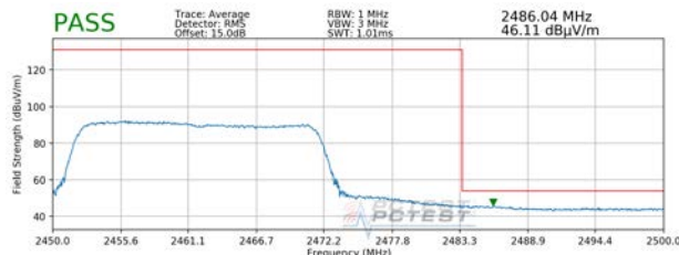
Plot 7-91. Radiated Restricted Upper Band Edge Measurement MIMO (Average)
