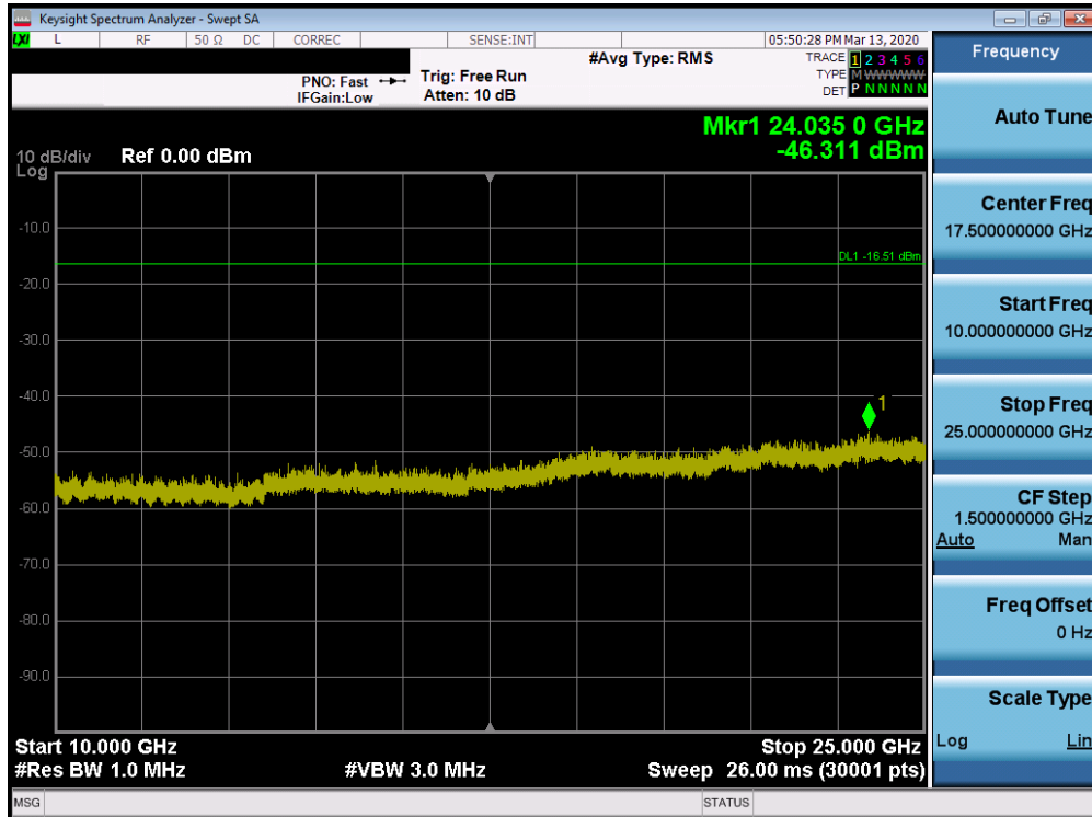
Plot 7-64. Conducted Spurious Plot SISO ANT2 (802.11b – Ch. 1)
