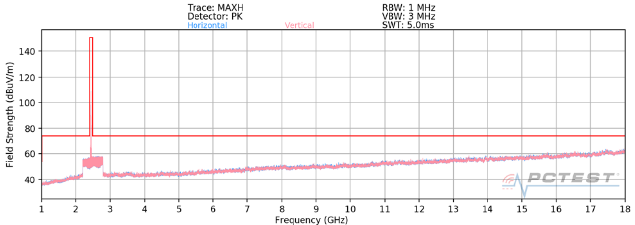
Plot 7-78. Radiated Spurious Plot above 1GHz MIMO/CDD (802.11g – Ch. 6)
