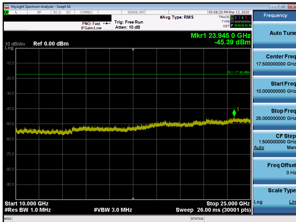
Plot 7-62. Conducted Spurious Plot SISO ANT1 (802.11b – Ch. 11)
