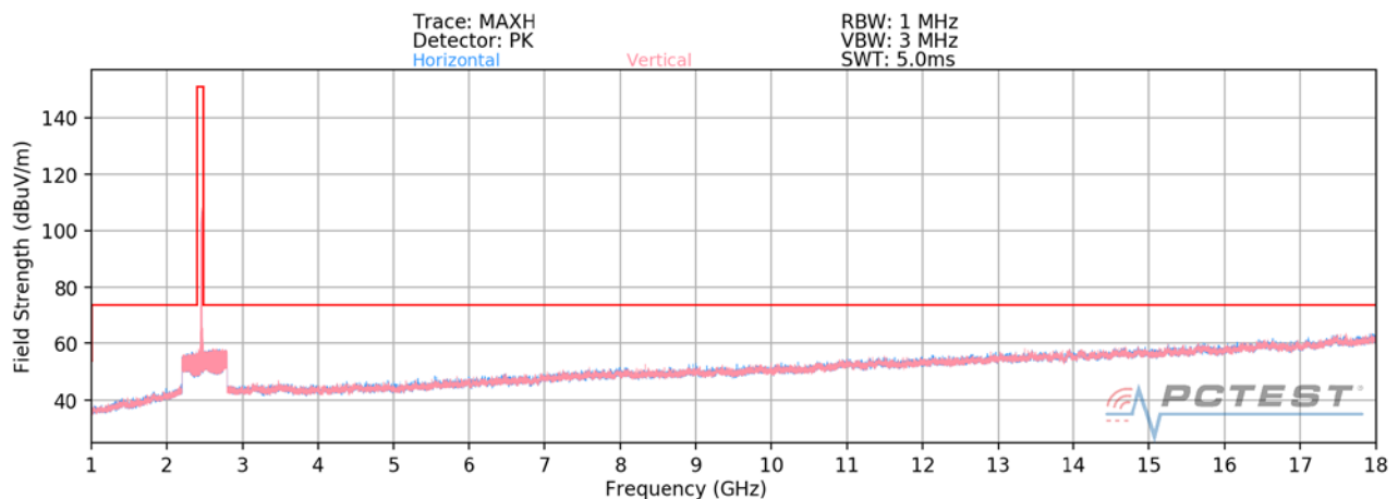
Plot 7-71. Radiated Spurious Plot above 1GHz SISO ANT1 (802.11b – Ch. 11)
