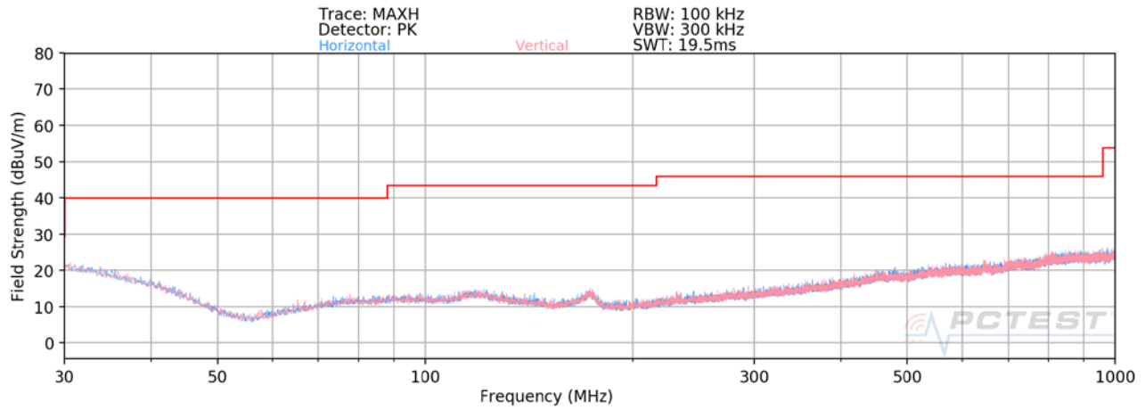
Plot 7-95. Radiated Spurious Plot below 1GHz MIMO
