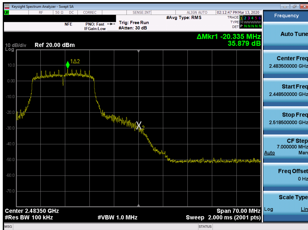
Plot 7-52. Band Edge Plot SISO ANT2 (802.11n (2.4GHz) – Ch. 11)
