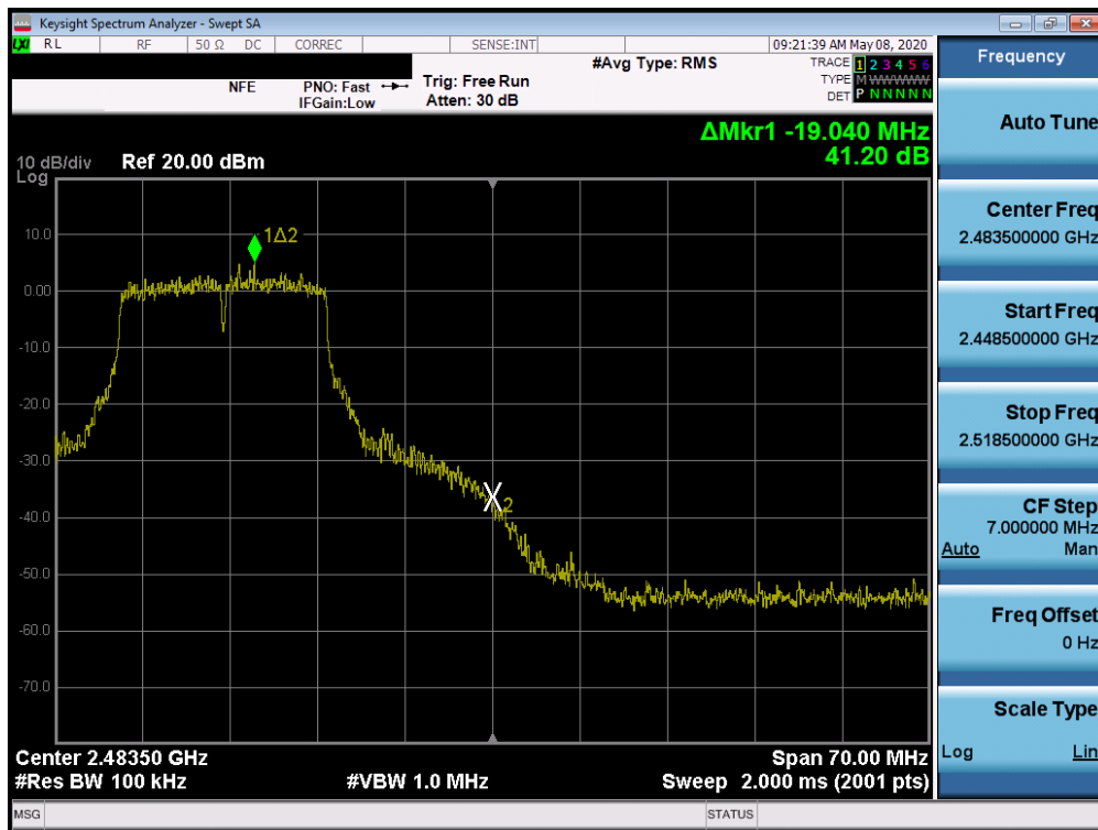
Plot 7-50. Band Edge Plot SISO ANT2 (802.11g - Ch. 11)
