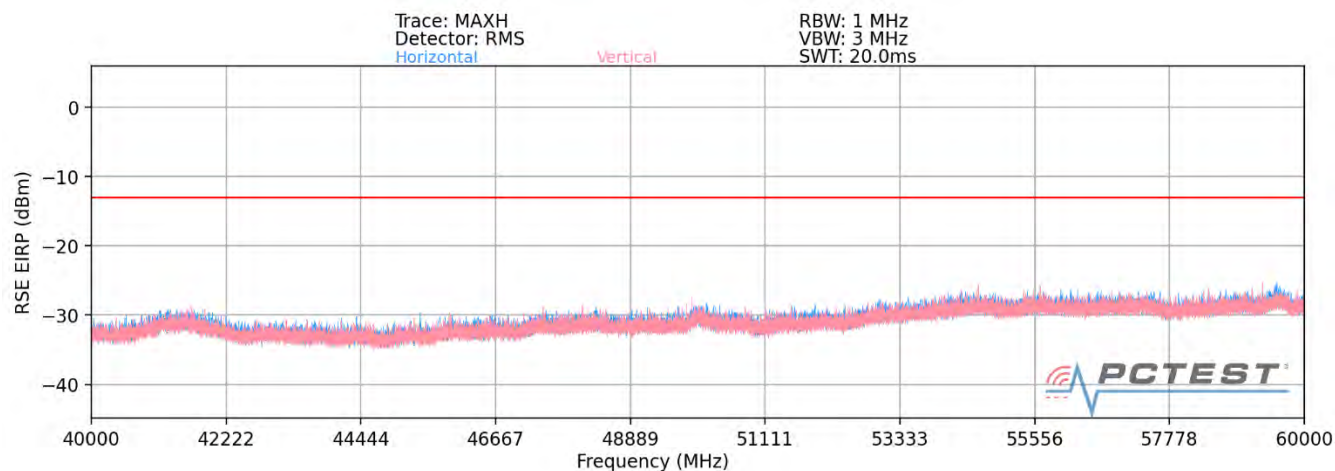
Plot 7-97. Ant1-n260 Radiated Spurious Plot (1CC QPSK Mid Channel H Beam – ENDC)
