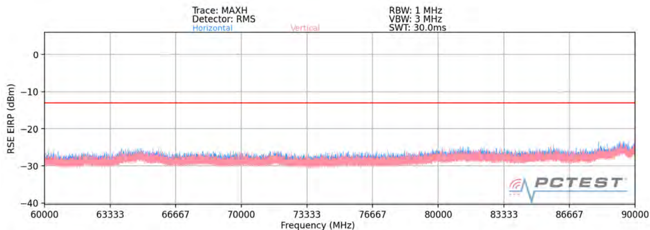
Plot 7-90. Ant2-n261 Radiated Spurious Plot (1CC QPSK Mid Channel V Beam – ENDC Anchor B2)
