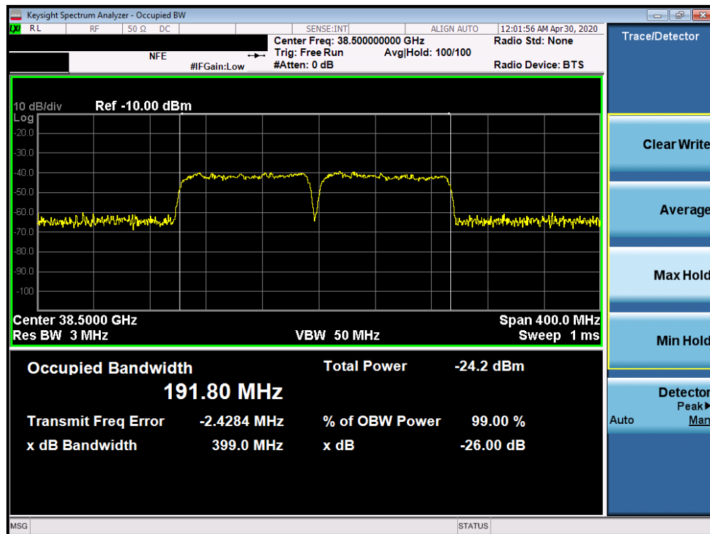
Plot 7-61. Ant2 Occupied Bandwidth Plot (100MHz-2CC – QPSK – Mid Channel)
