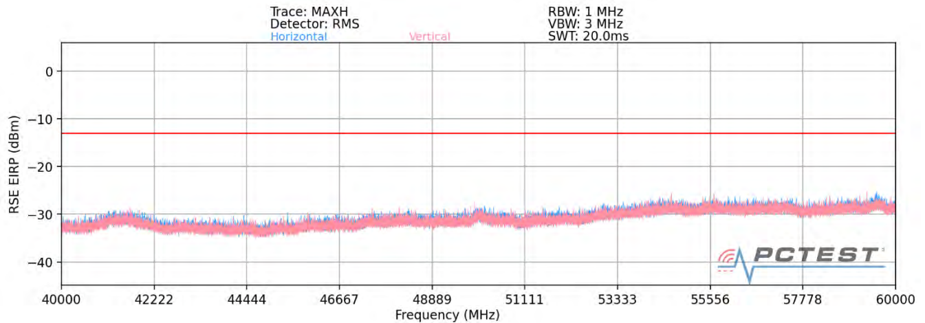
Plot 7-88. Ant2-n261 Radiated Spurious Plot (1CC QPSK Mid Channel V Beam – ENDC Anchor B2)
