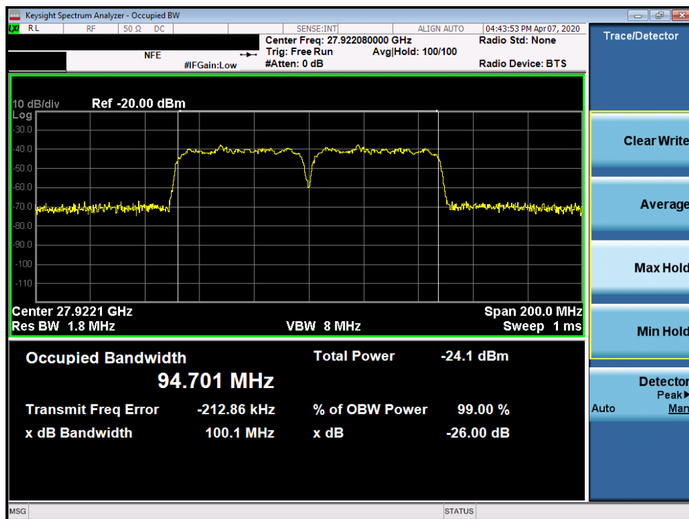
Plot 7-6. Ant1 Occupied Bandwidth Plot (50MHz-2CC – 16QAM – Mid Channel)
