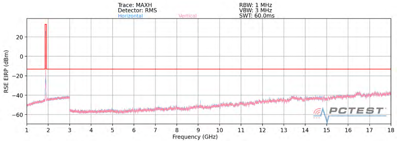
Plot 7-93. Ant1-n260 Radiated Spurious Plot 1GHz - 18GHz (1CC QPSK Mid Channel H Beam – ENDC Anchor Band 2)
