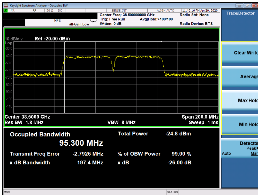
Plot 7-53. Ant2 Occupied Bandwidth Plot (50MHz-2CC – QPSK – Mid Channel)
