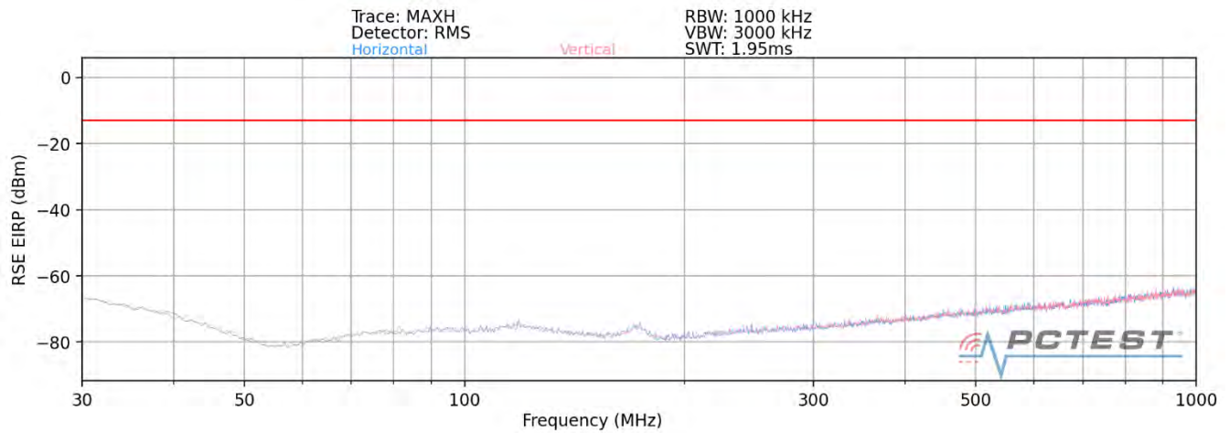
Plot 7-79. Ant2-n261 Radiated Spurious Plot (1CC QPSK Mid Channel H Beam)
