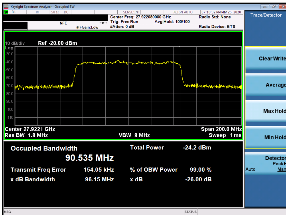
Plot 7-26. Ant2 Occupied Bandwidth Plot (100MHz-1CC – 16QAM – Mid Channel)
