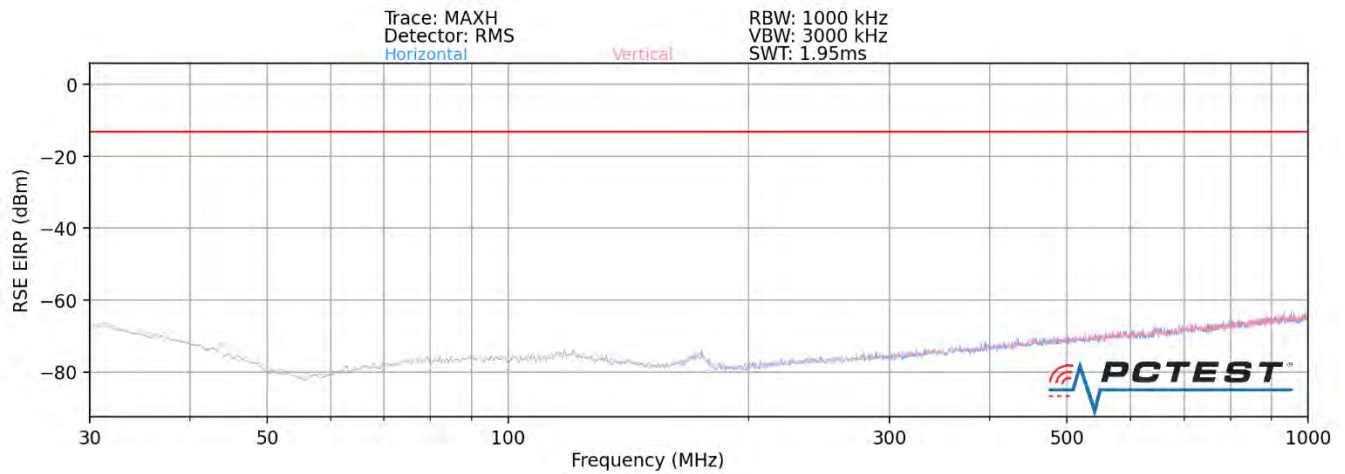
Plot 7-66. Ant1-n261 Radiated Spurious Plot (1CC QPSK Mid Channel V Beam)
