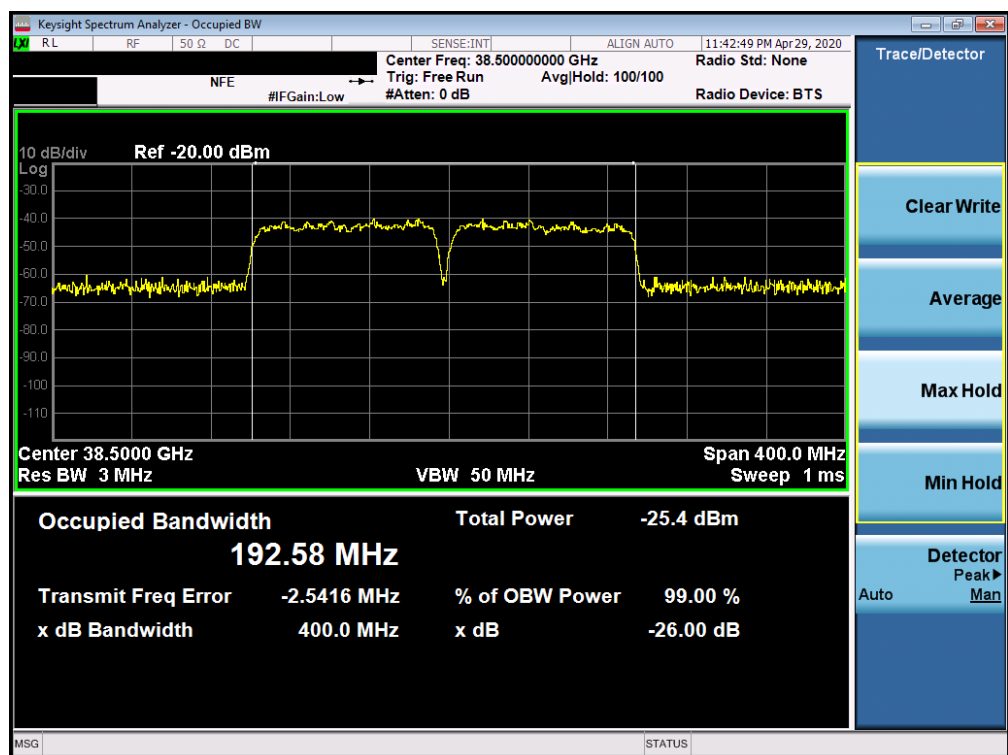
Plot 7-62. Ant2 Occupied Bandwidth Plot (100MHz-2CC – 16QAM – Mid Channel)
