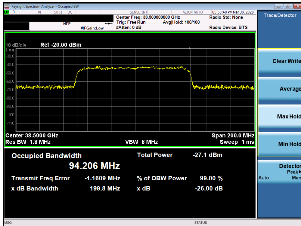
Plot 7-57. Ant2 Occupied Bandwidth Plot (100MHz-1CC – QPSK – Mid Channel)
