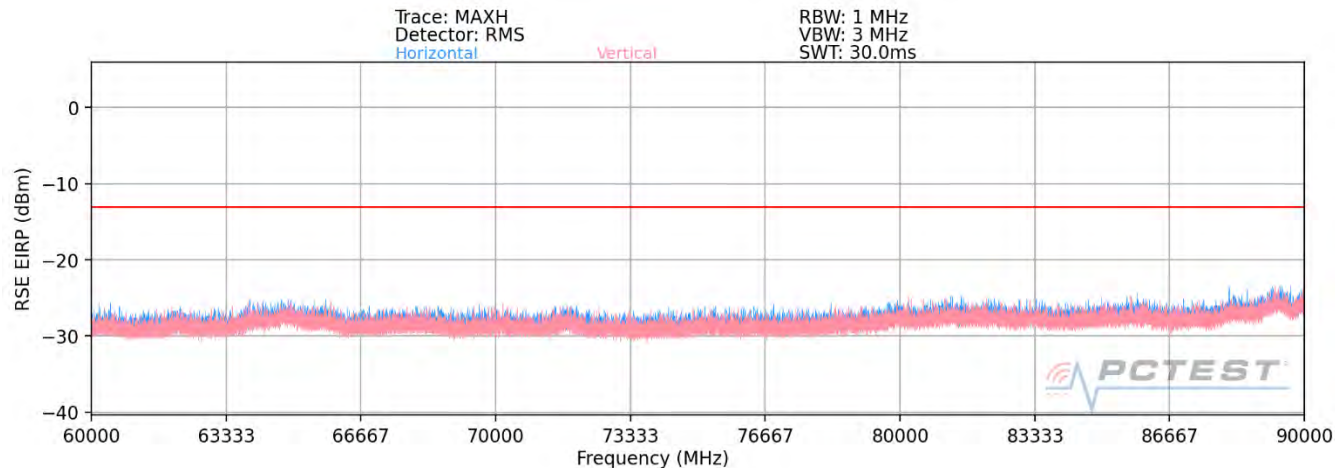
Plot 7-89. Ant2-n261 Radiated Spurious Plot (1CC QPSK Mid Channel H Beam – ENDC Anchor B2)
