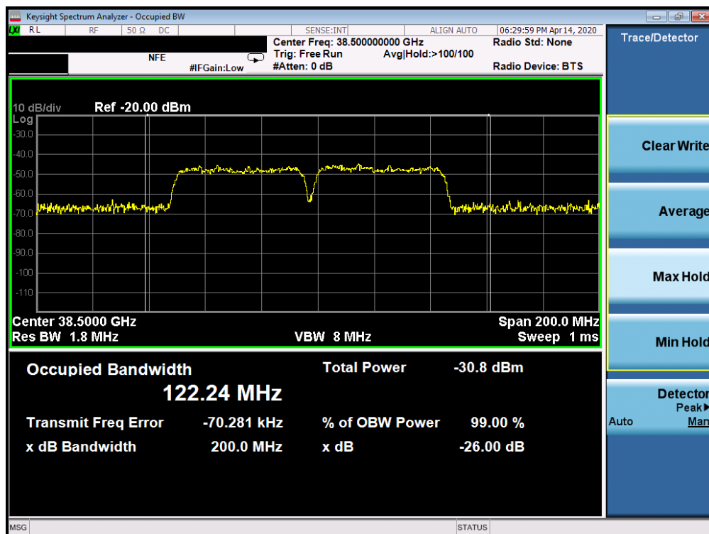
Plot 7-39. Ant1 Occupied Bandwidth Plot (50MHz-2CC – 64QAM – Mid Channel)
