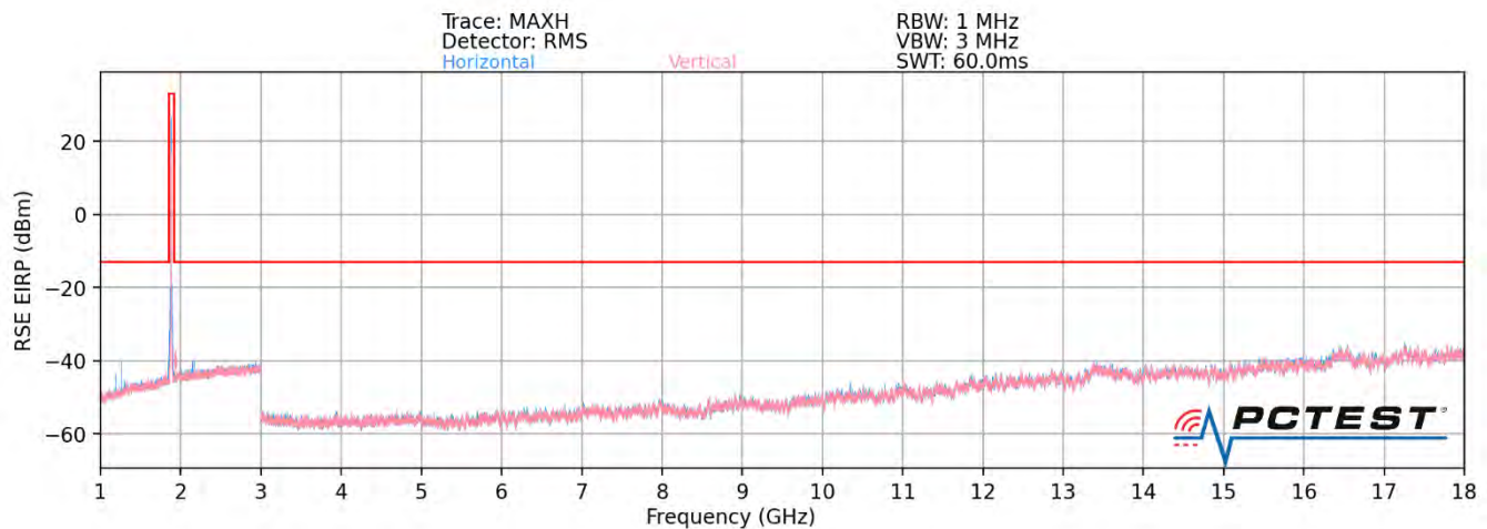
Plot 7-67. Ant1-n261 Radiated Spurious Plot 1GHz - 18GHz (1CC QPSK Mid Channel H Beam – ENDC Anchor Band 2)
