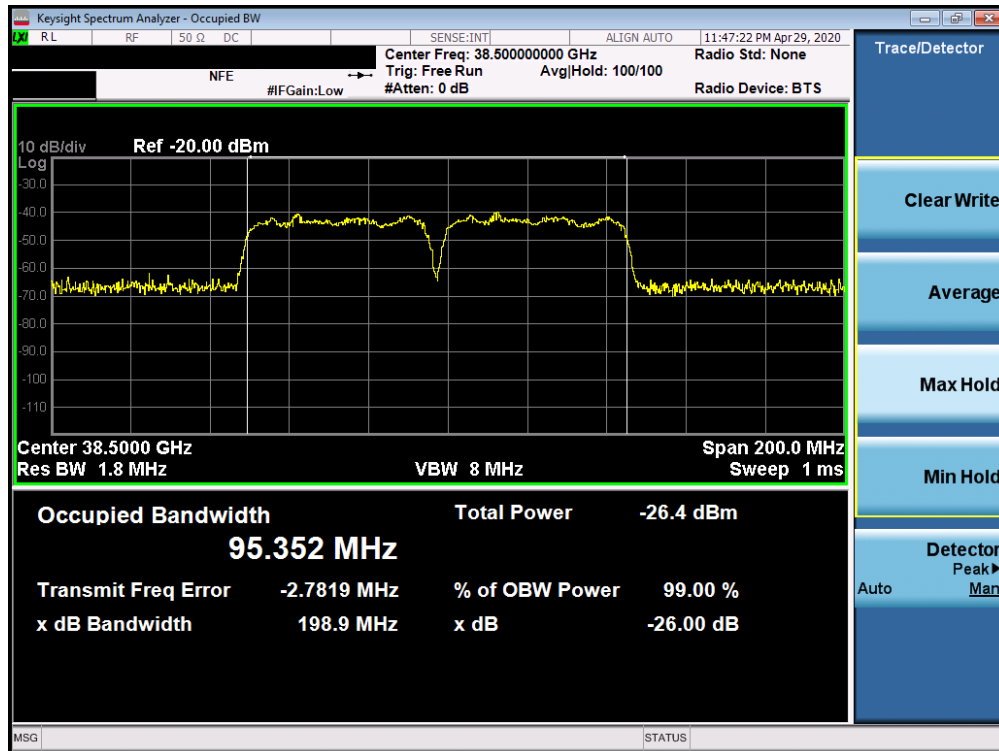
Plot 7-54. Ant2 Occupied Bandwidth Plot (50MHz-2CC – 16QAM – Mid Channel)
