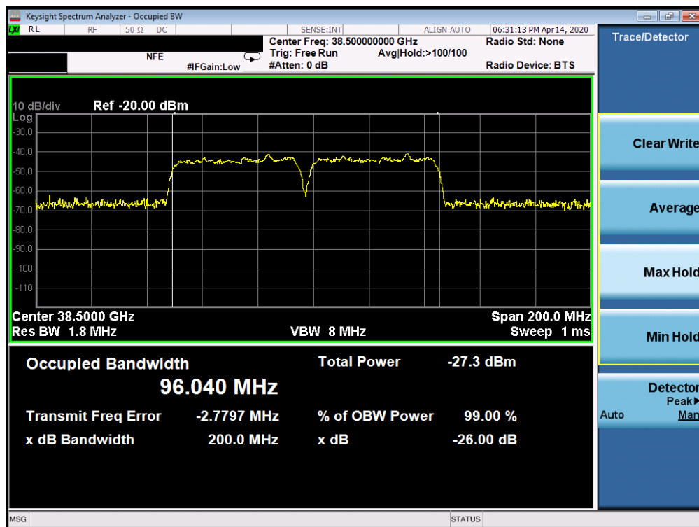
Plot 7-40. Ant1 Occupied Bandwidth Plot (50MHz-2CC – pi/2 BPSK – Mid Channel)
