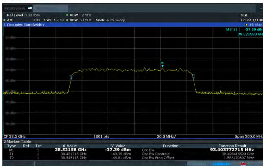
Plot 7-44. Ant1 Occupied Bandwidth Plot (100MHz-1CC – pi/2-BPSK – Mid Channel)
