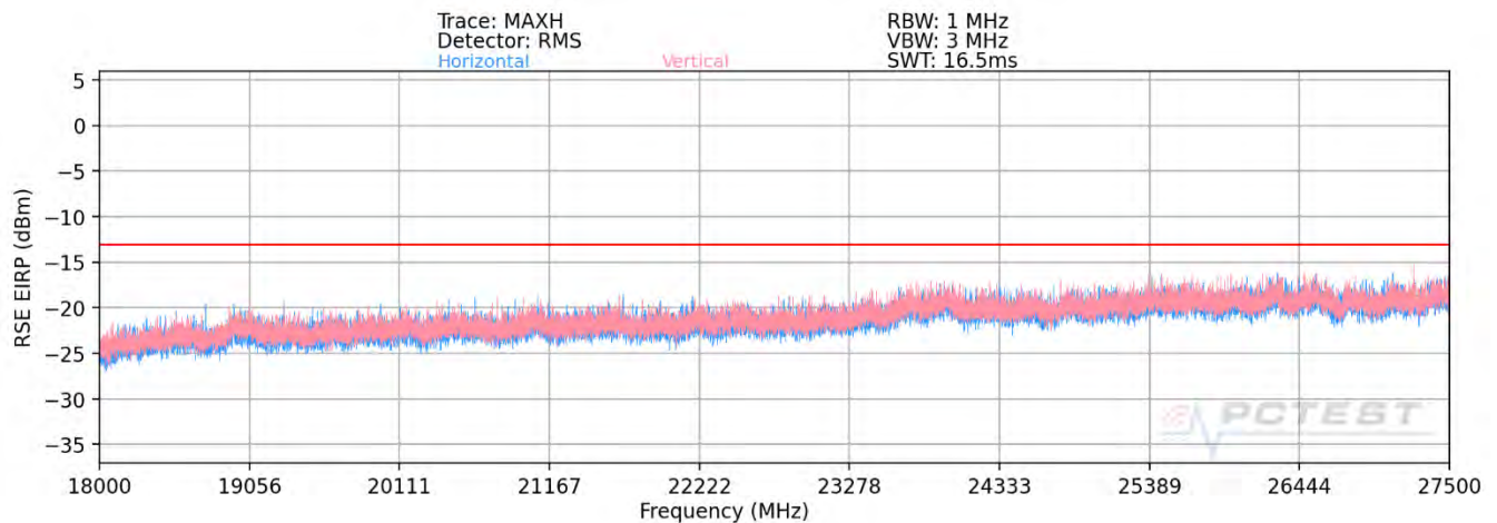
Plot 7-70. Ant1-n261 Radiated Spurious Plot (1CC QPSK Mid Channel V Beam – ENDC Anchor B2)
