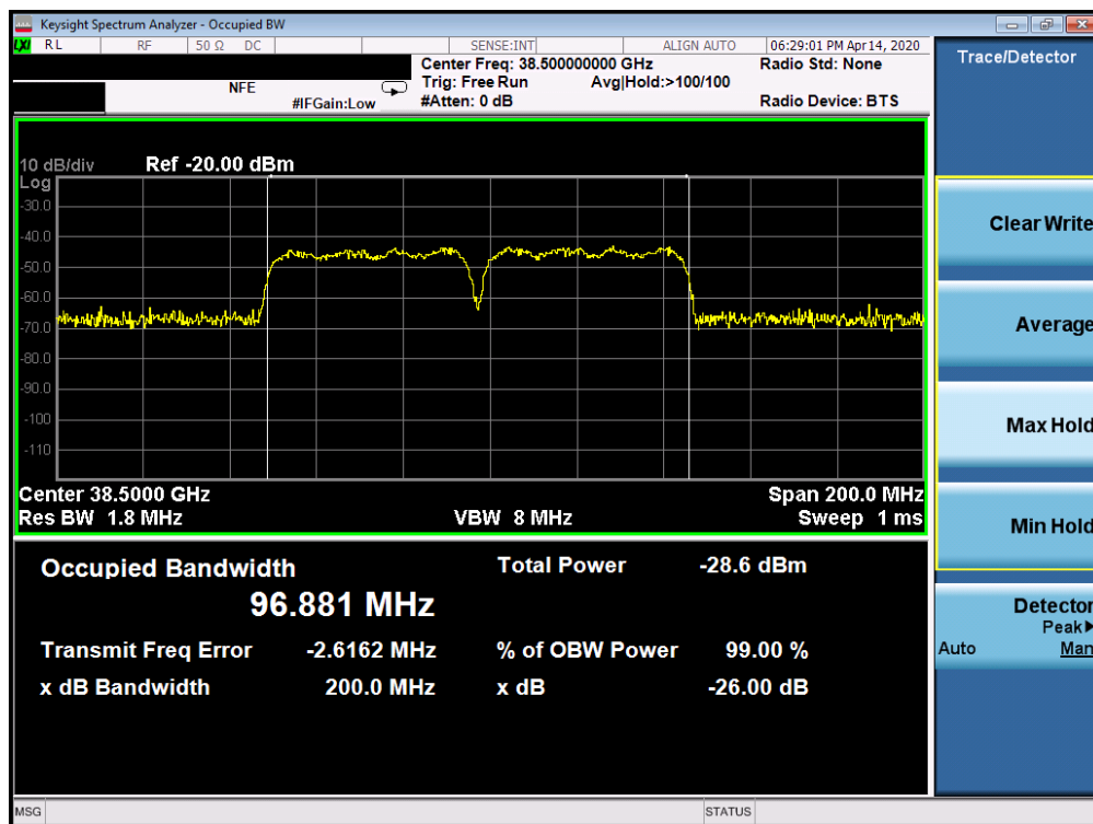
Plot 7-38. Ant1 Occupied Bandwidth Plot (50MHz-2CC – 16QAM – Mid Channel)
