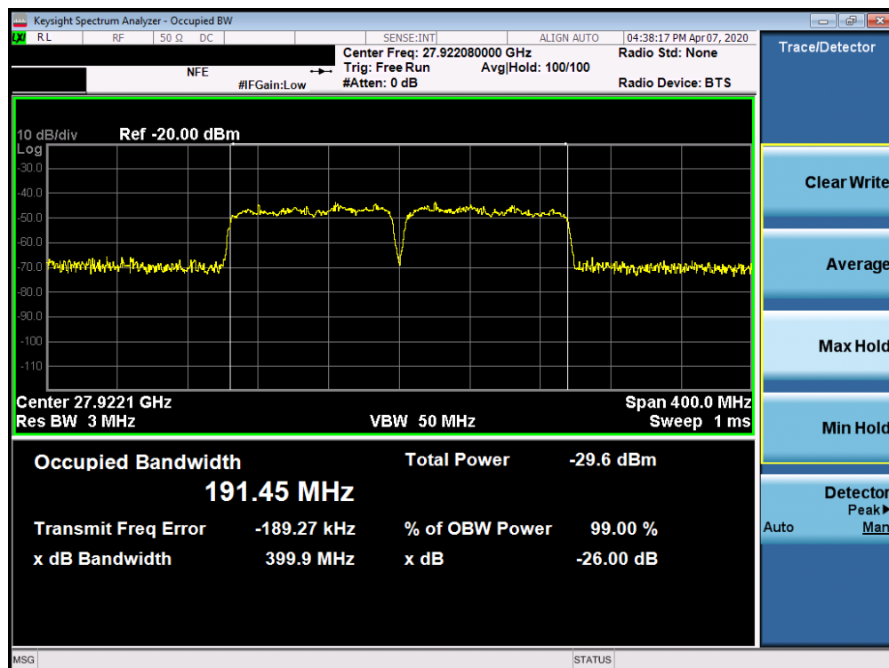
Plot 7-15. Ant1 Occupied Bandwidth Plot (100MHz-2CC – 64QAM – Mid Channel)
