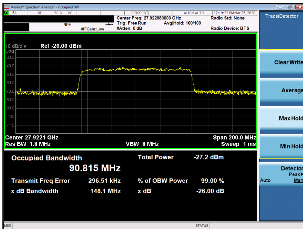
Plot 7-27. Ant2 Occupied Bandwidth Plot (100MHz-1CC – 64QAM – Mid Channel)
