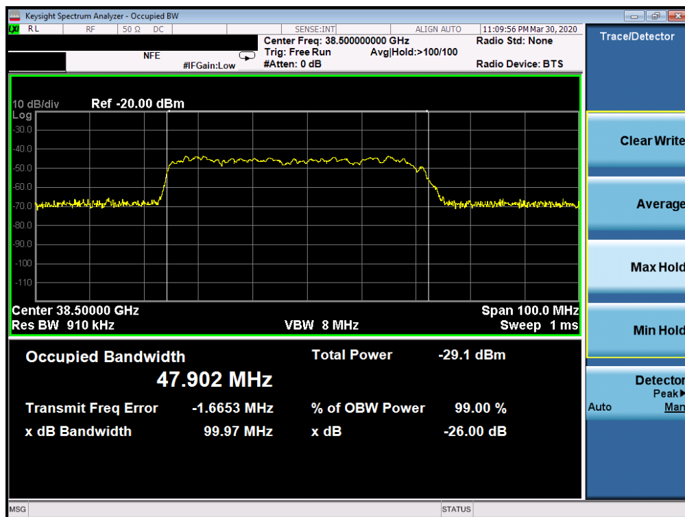
Plot 7-35. Ant1 Occupied Bandwidth Plot (50MHz-1CC – 64QAM – Mid Channel)
