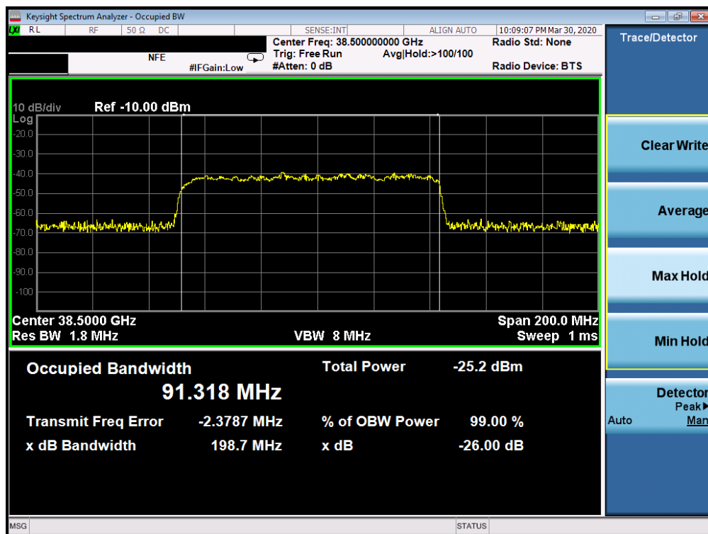
Plot 7-41. Ant1 Occupied Bandwidth Plot (100MHz-1CC – QPSK – Mid Channel)
