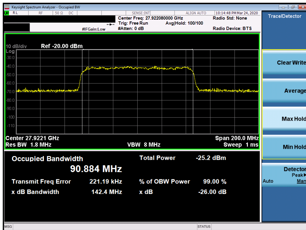
Plot 7-10. Ant1 Occupied Bandwidth Plot (100MHz-1CC – 16QAM – Mid Channel)
