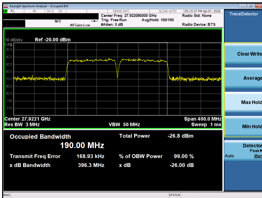
Plot 7-31. Ant2 Occupied Bandwidth Plot (100MHz-2CC – 64QAM – Mid Channel)
