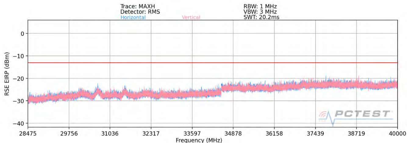
Plot 7-72. Ant1-n261 Radiated Spurious Plot (1CC QPSK Mid Channel V Beam – ENDC Anchor B2)
