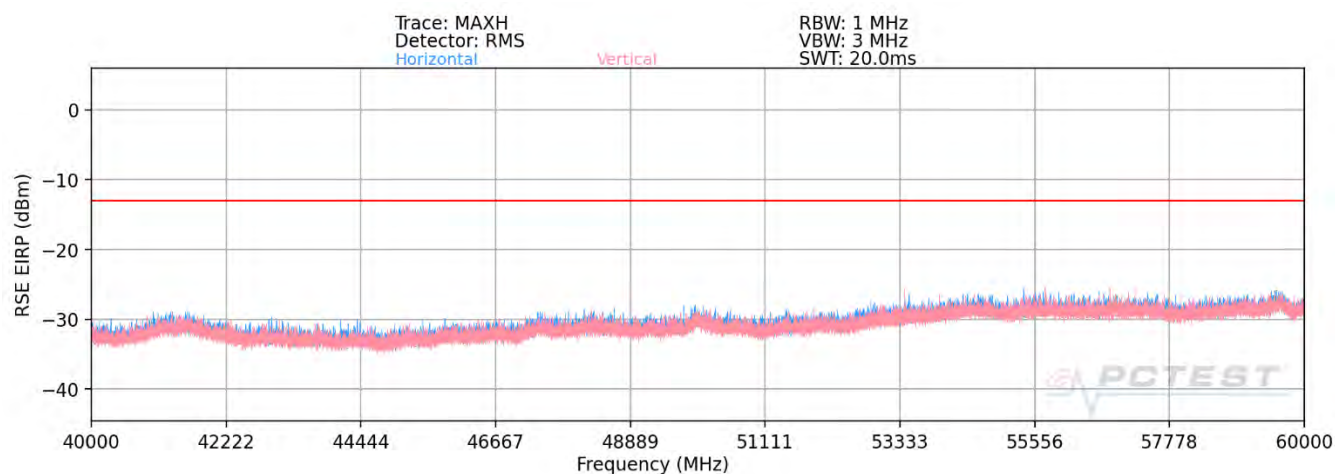
Plot 7-98. Ant1-n260 Radiated Spurious Plot (1CC QPSK Mid Channel V Beam – ENDC)
