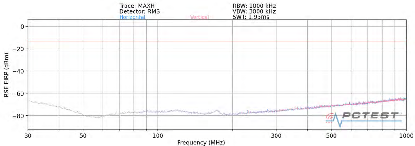
Plot 7-91. Ant1-n260 Radiated Spurious Plot (1CC QPSK Mid Channel H Beam)
