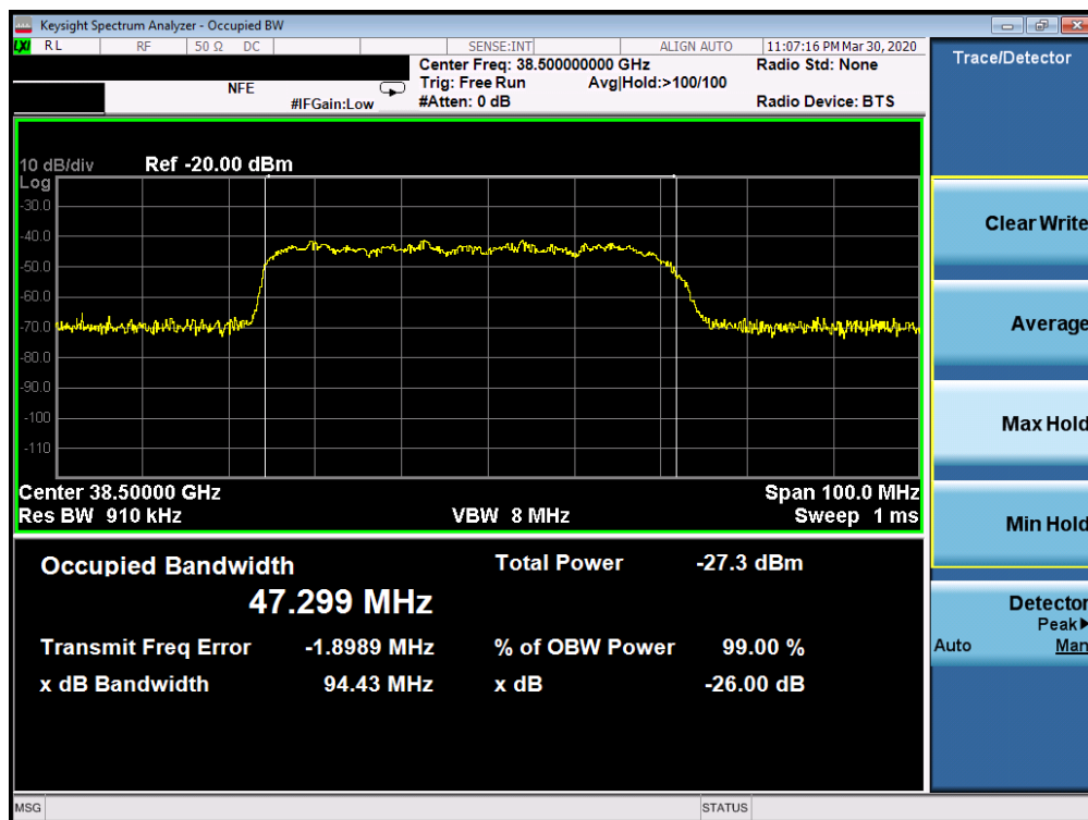
Plot 7-34. Ant1 Occupied Bandwidth Plot (50MHz-1CC – 16QAM – Mid Channel)
