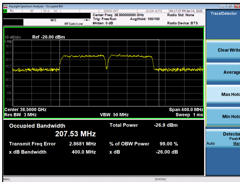
Plot 7-45. Ant1 Occupied Bandwidth Plot (100MHz-2CC – QPSK – Mid Channel)
