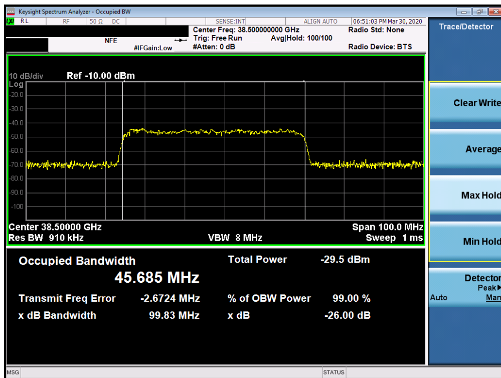
Plot 7-51. Ant2 Occupied Bandwidth Plot (50MHz-1CC – 64QAM – Mid Channel)
