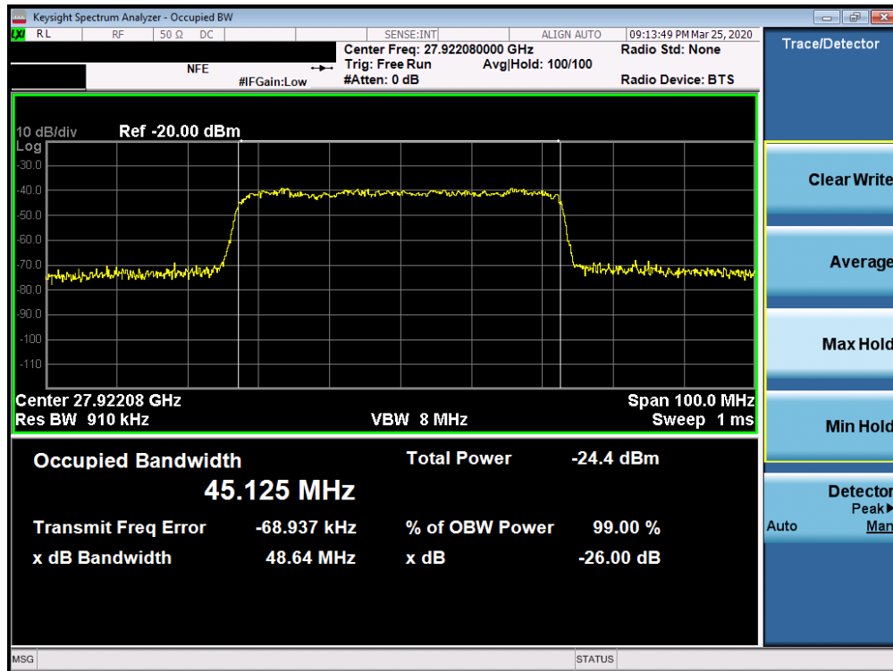
Plot 7-18. Ant2 Occupied Bandwidth Plot (50MHz-1CC – 16QAM – Mid Channel)
