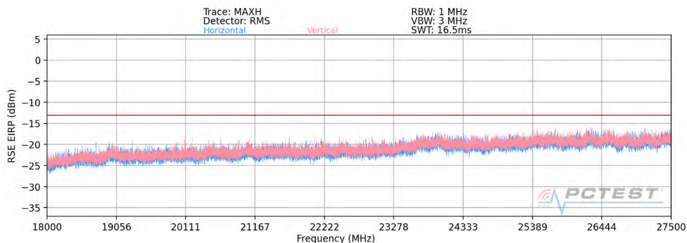
Plot 7-84. Ant2-n261 Radiated Spurious Plot (1CC QPSK Mid Channel V Beam – ENDC Anchor B2)
