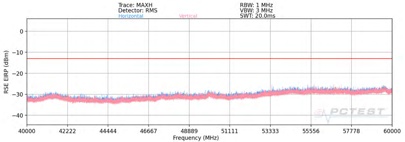
Plot 7-87. Ant2-n261 Radiated Spurious Plot (1CC QPSK Mid Channel H Beam – ENDC Anchor B2)
