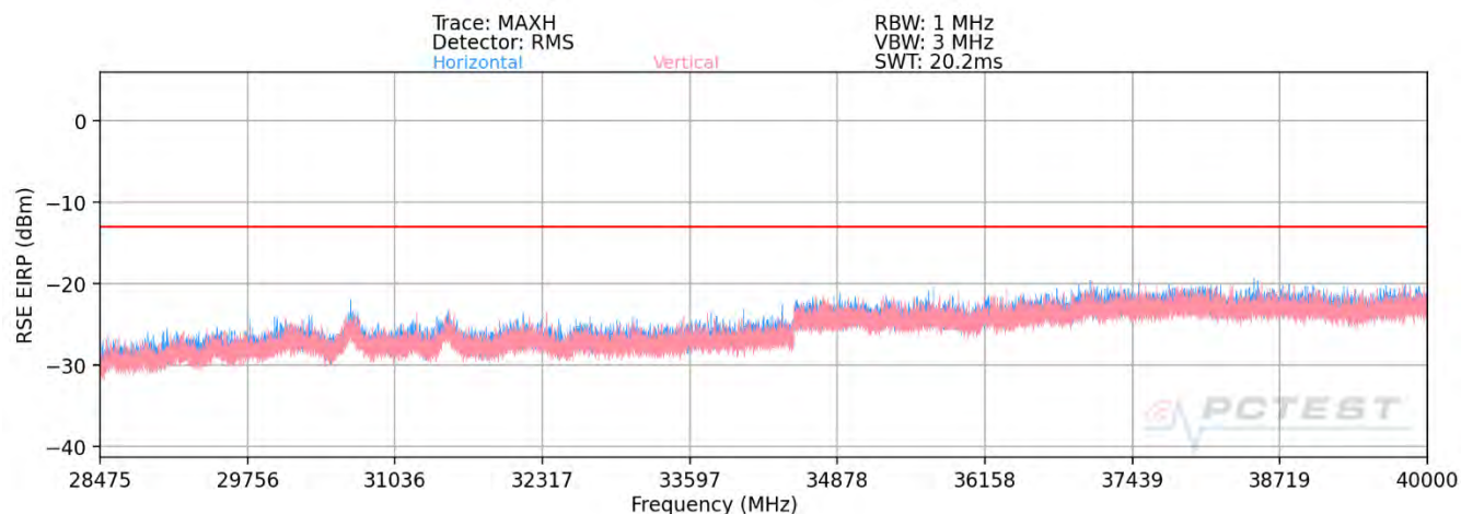
Plot 7-86. Ant2-n261 Radiated Spurious Plot (1CC QPSK Mid Channel V Beam – ENDC Anchor B2)
