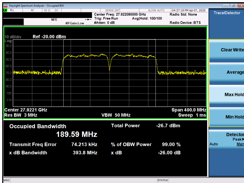
Plot 7-14. Ant1 Occupied Bandwidth Plot (100MHz-2CC – 16QAM – Mid Channel)
