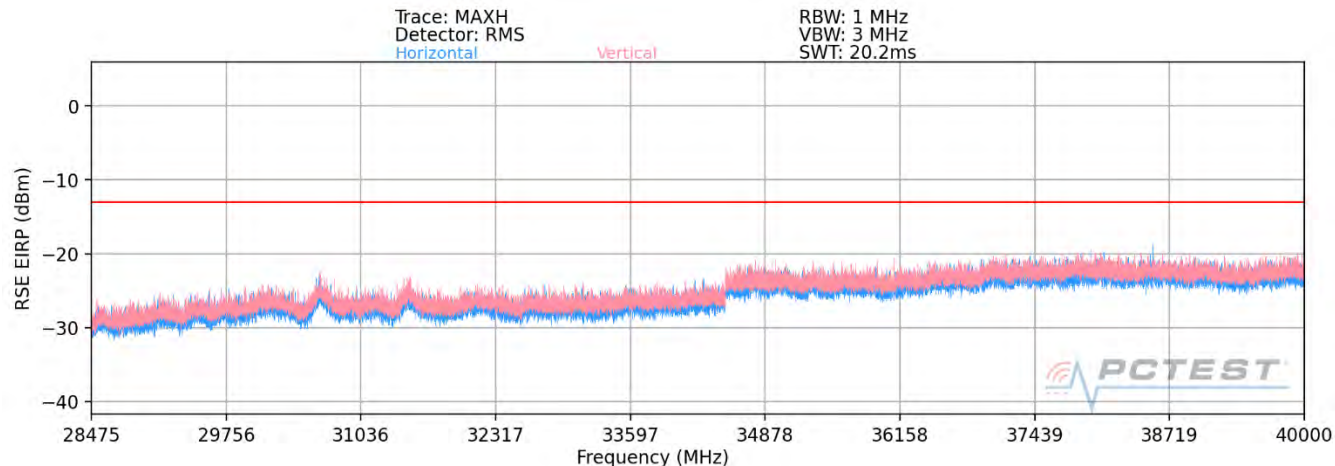
Plot 7-85. Ant2-n261 Radiated Spurious Plot (1CC QPSK Mid Channel H Beam – ENDC Anchor B2)
