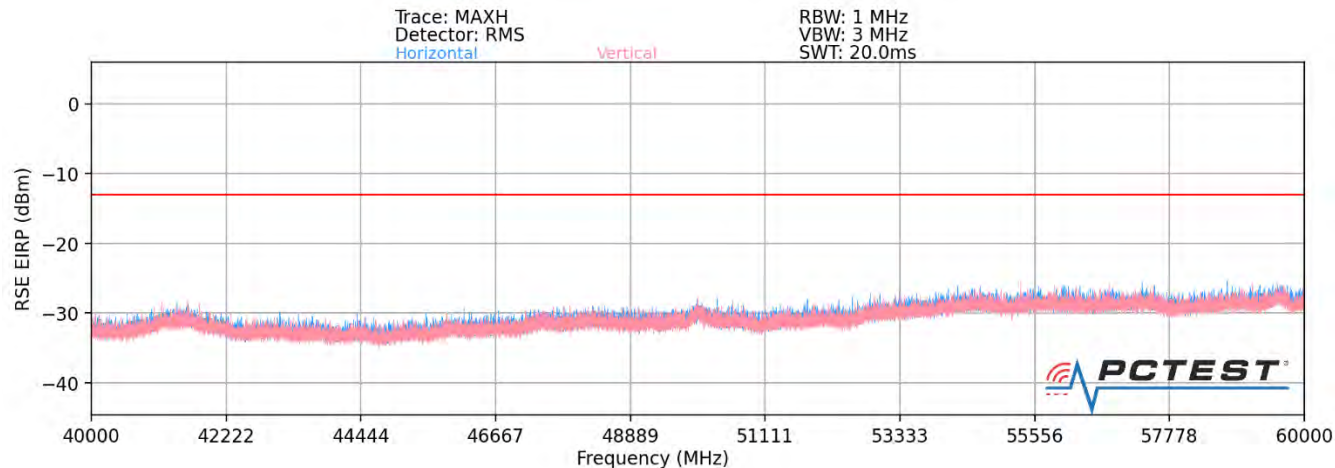
Plot 7-73. Ant1-n261 Radiated Spurious Plot (1CC QPSK Mid Channel H Beam – ENDC Anchor B2)
