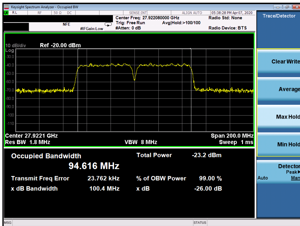
Plot 7-24. Ant2 Occupied Bandwidth Plot (50MHz-2CC – pi/2-BPSK – Mid Channel)
