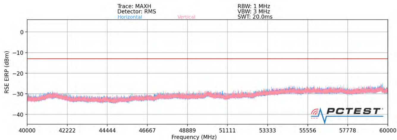
Plot 7-74. Ant1-n261 Radiated Spurious Plot (1CC QPSK Mid Channel V Beam – ENDC Anchor B2)
