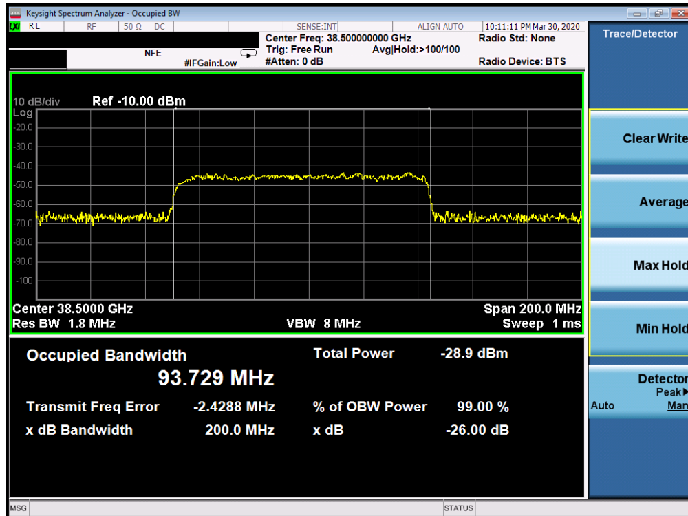
Plot 7-43. Ant1 Occupied Bandwidth Plot (100MHz-1CC – 64QAM – Mid Channel)
