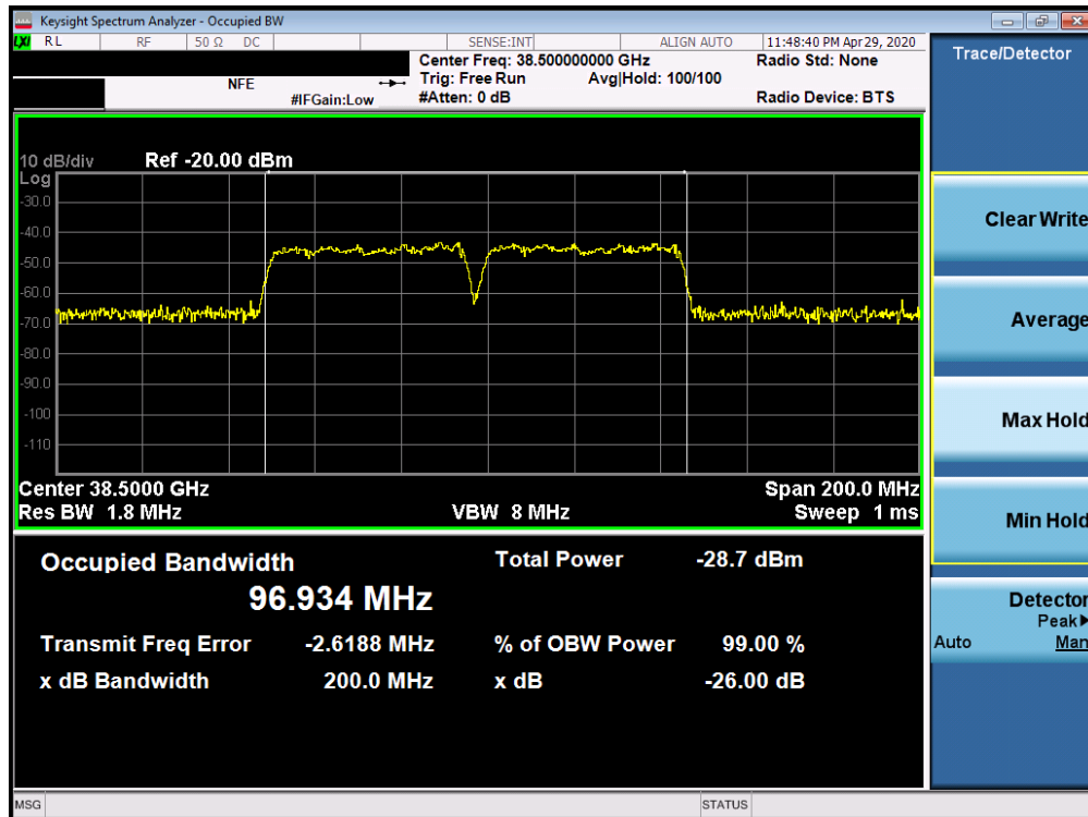
Plot 7-55. Ant2 Occupied Bandwidth Plot (50MHz-2CC – 64QAM – Mid Channel)
