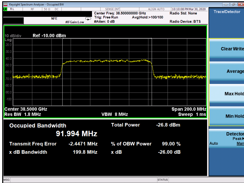
Plot 7-42. Ant1 Occupied Bandwidth Plot (100MHz-1CC – 16QAM – Mid Channel)
