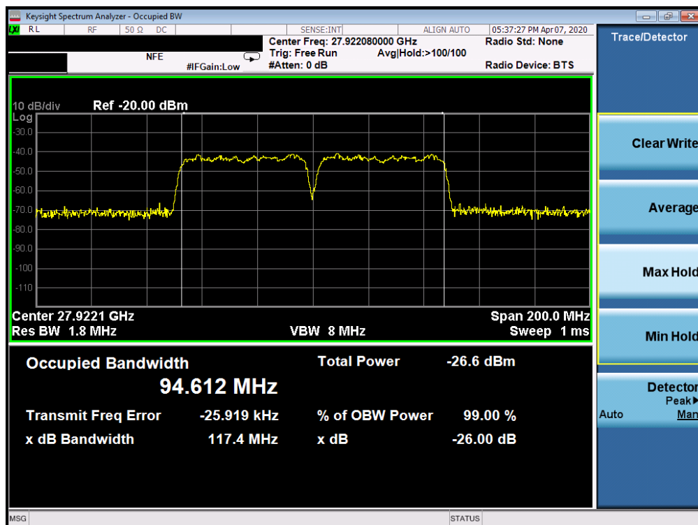
Plot 7-23. Ant2 Occupied Bandwidth Plot (50MHz-2CC – 64QAM – Mid Channel)
