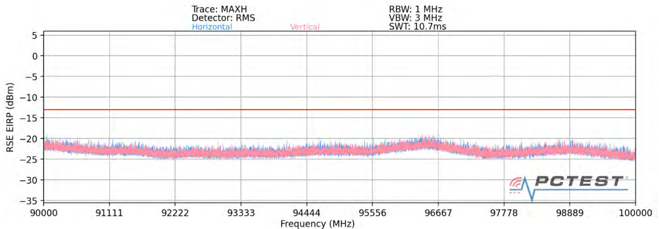
Plot 7-78. Ant1-n261 Radiated Spurious Plot (1CC QPSK Mid Channel V Beam – ENDC Anchor B2)
