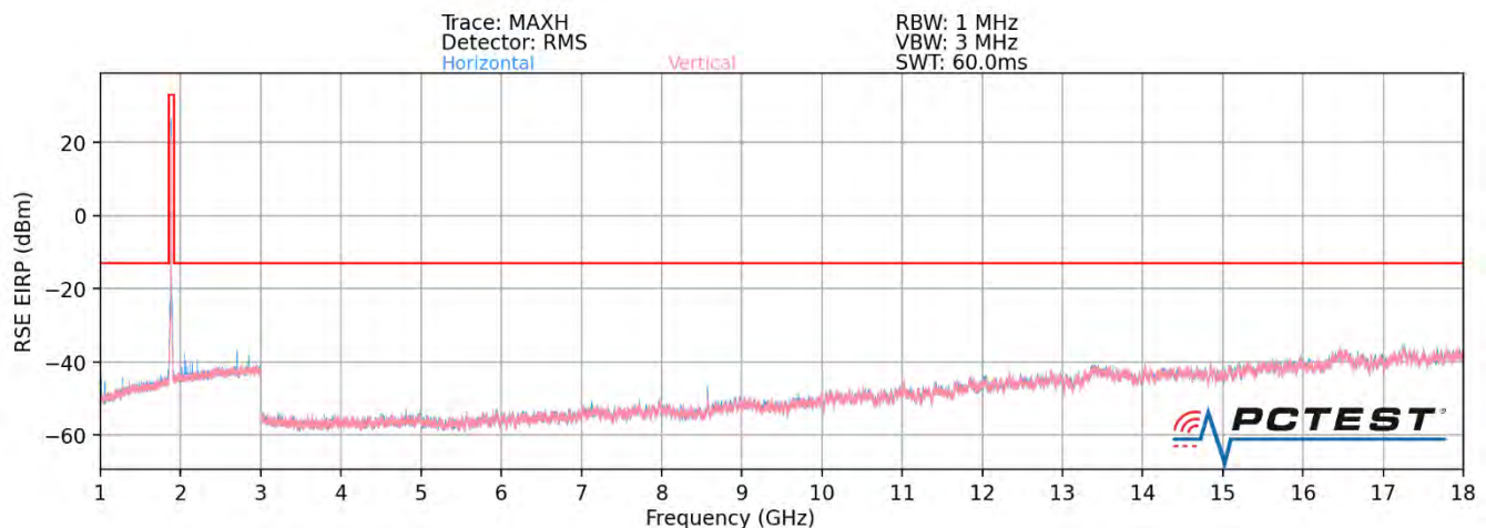
Plot 7-68. Ant1-n261 Radiated Spurious Plot 1GHz - 18GHz (1CC QPSK Mid Channel V Beam – ENDC Anchor Band 2)
