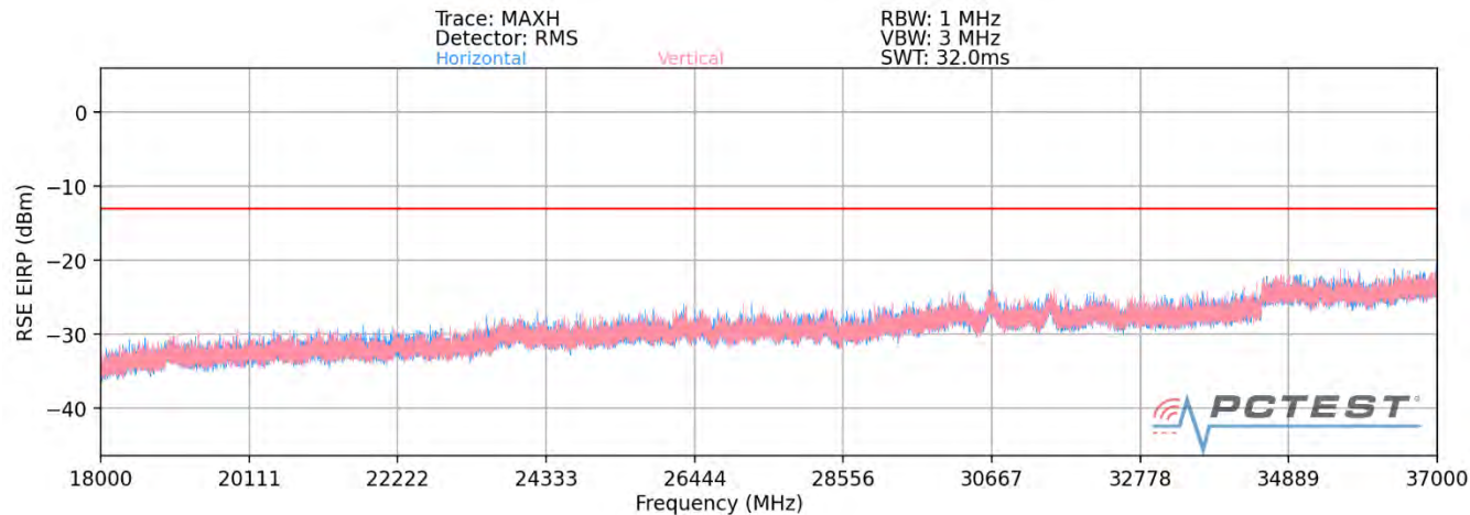
Plot 7-95. Ant1-n260 Radiated Spurious Plot (1CC QPSK Mid Channel H Beam – ENDC)
