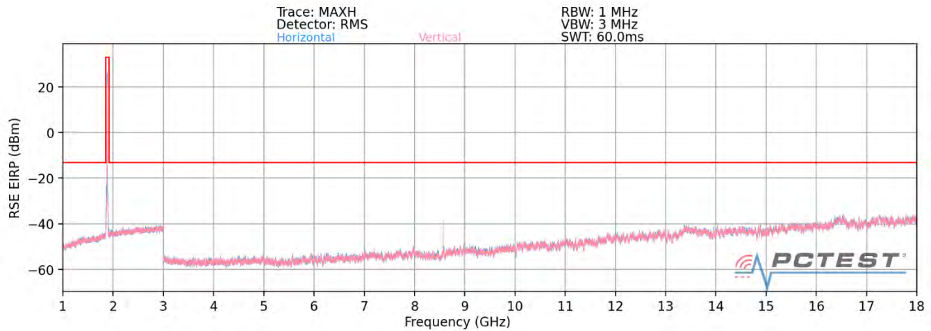
Plot 7-81. Ant2-n261 Radiated Spurious Plot 1GHz - 18GHz (1CC QPSK Mid Channel H Beam – ENDC Anchor Band 2)
