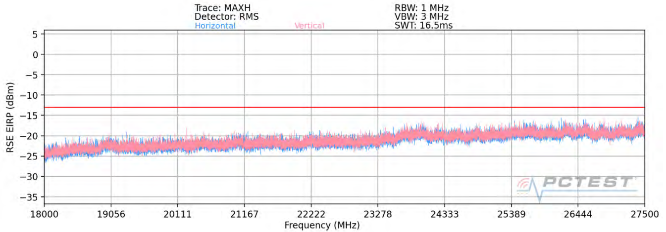
Plot 7-69. Ant1-n261 Radiated Spurious Plot (1CC QPSK Mid Channel H Beam – ENDC Anchor B2)
