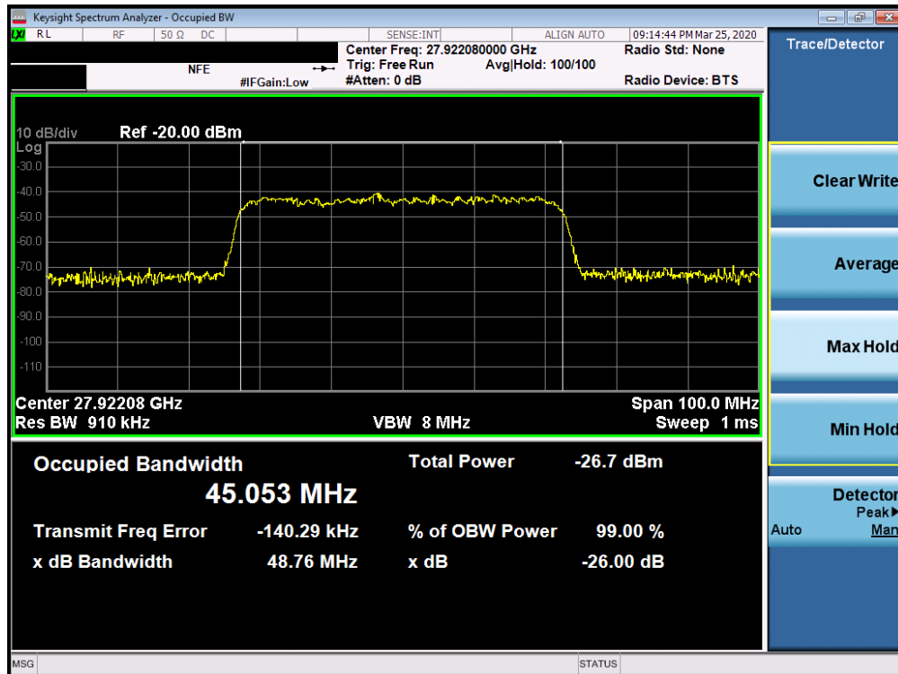
Plot 7-19. Ant2 Occupied Bandwidth Plot (50MHz-1CC – 64QAM – Mid Channel)
