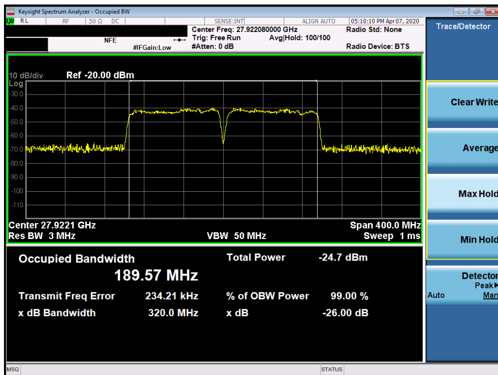
Plot 7-30. Ant2 Occupied Bandwidth Plot (100MHz-2CC – 16QAM – Mid Channel)
