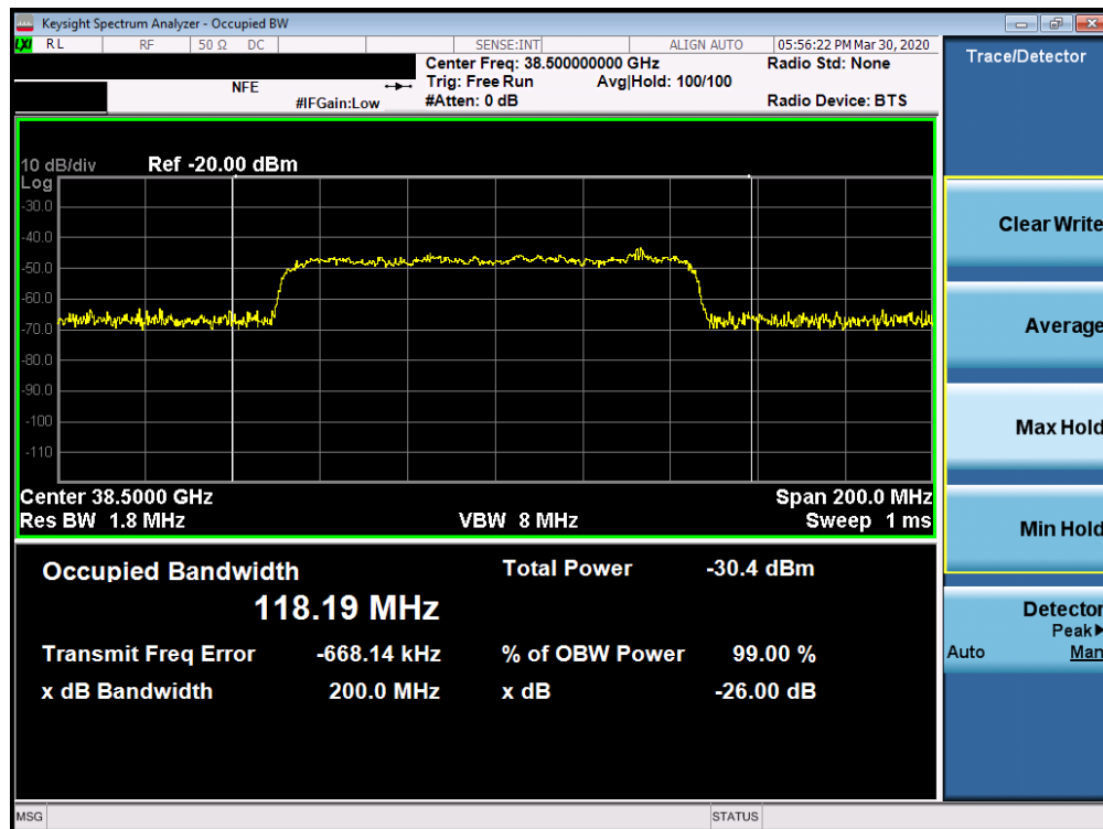
Plot 7-59. Ant2 Occupied Bandwidth Plot (100MHz-1CC – 64QAM – Mid Channel)
