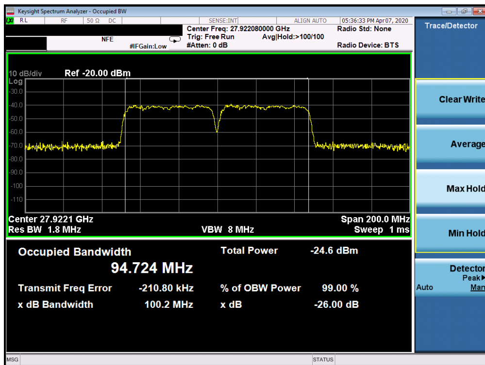
Plot 7-22. Ant2 Occupied Bandwidth Plot (50MHz-2CC – 16QAM – Mid Channel)
