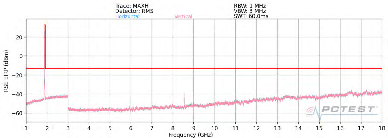
Plot 7-82. Ant2-n261 Radiated Spurious Plot 1GHz - 18GHz (1CC QPSK Mid Channel V Beam – ENDC Anchor Band 2)
