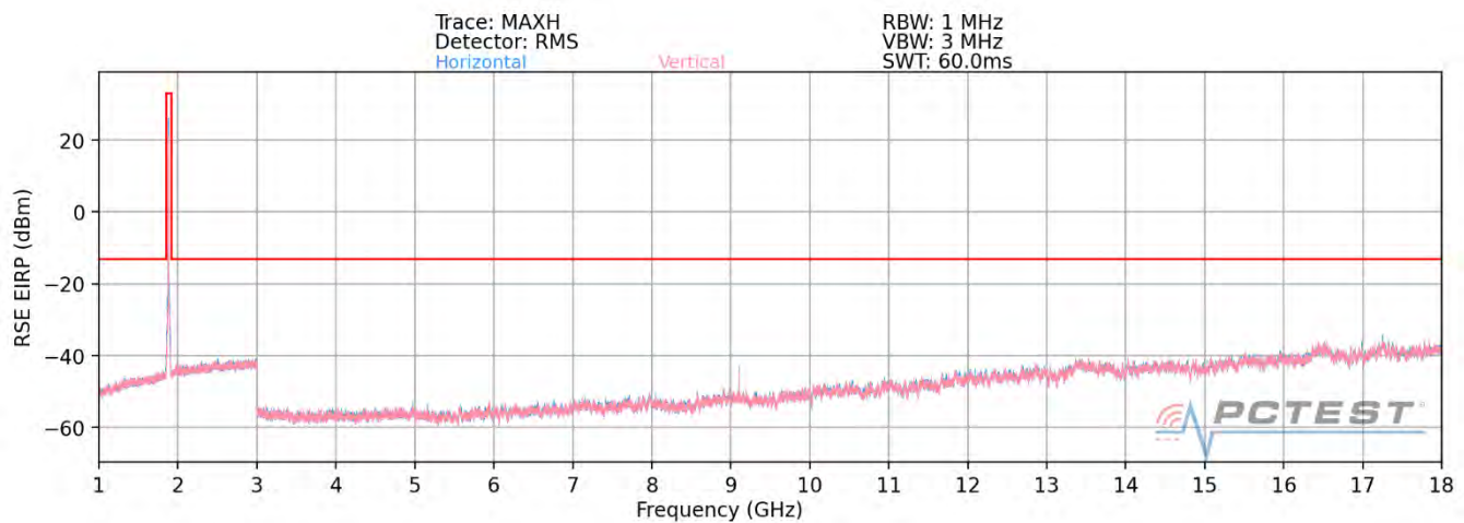
Plot 7-94. Ant1-n260 Radiated Spurious Plot 1GHz - 18GHz (1CC QPSK Mid Channel V Beam – ENDC Anchor Band 2)
