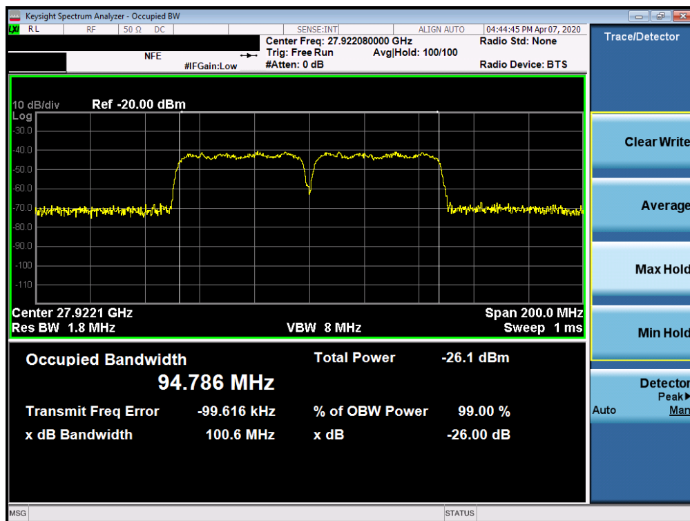
Plot 7-7. Ant1 Occupied Bandwidth Plot (50MHz-2CC – 64QAM – Mid Channel)
