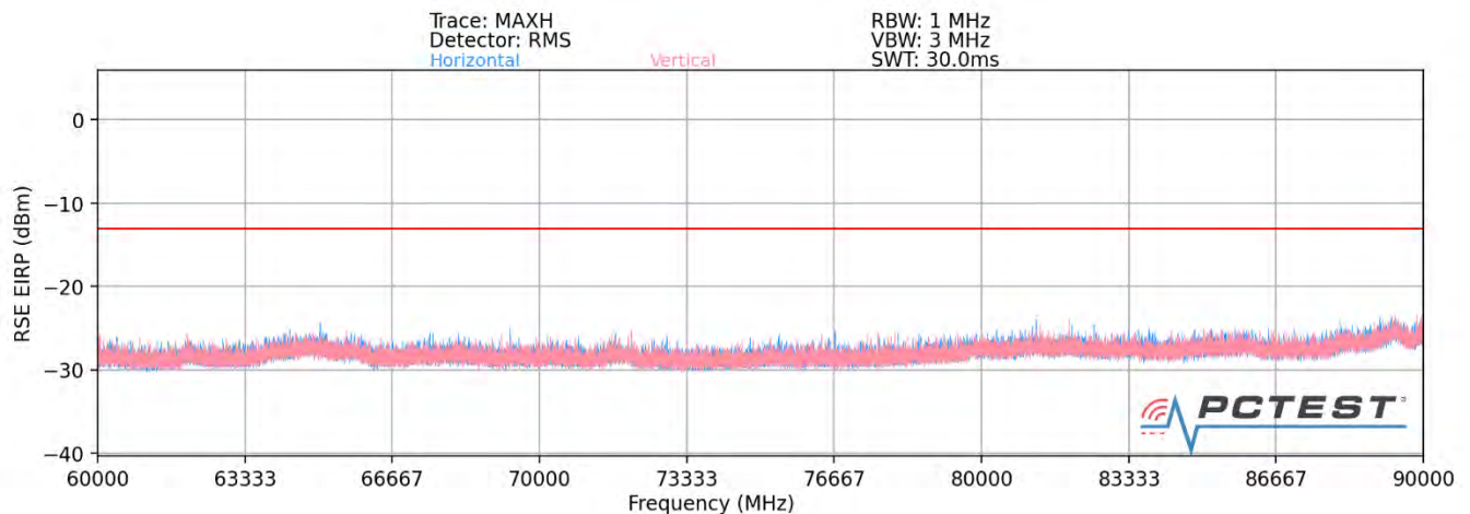
Plot 7-76. Ant1-n261 Radiated Spurious Plot (1CC QPSK Mid Channel V Beam – ENDC Anchor B2)
