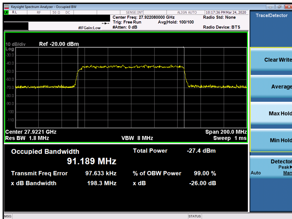
Plot 7-11. Ant1 Occupied Bandwidth Plot (100MHz-1CC – 64QAM – Mid Channel)
