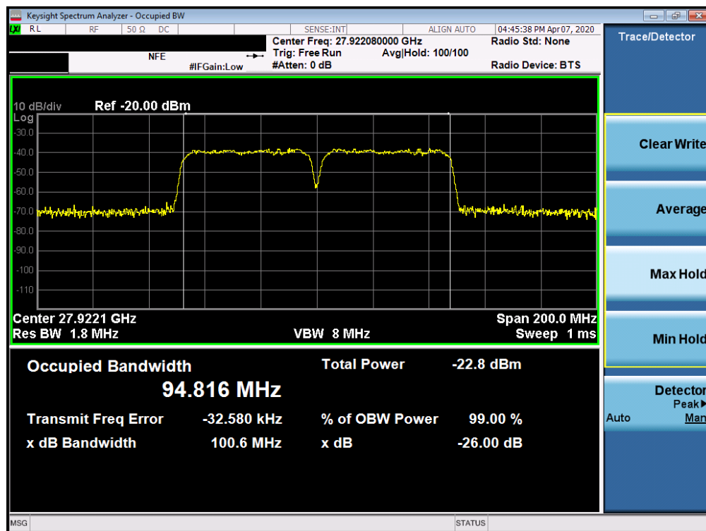
Plot 7-8. Ant1 Occupied Bandwidth Plot (50MHz-2CC – pi/2-BPSK – Mid Channel)
