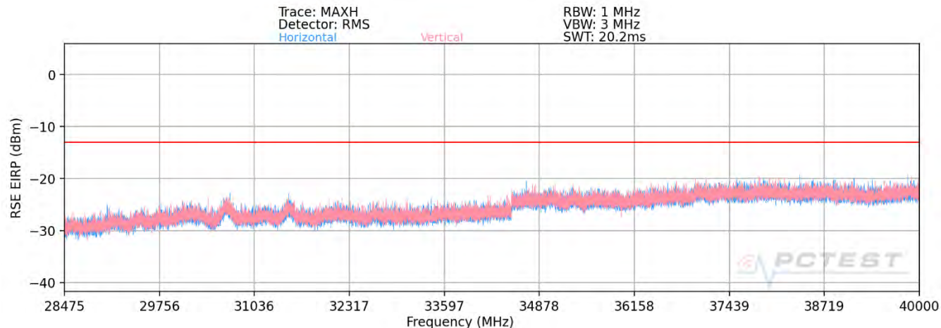
Plot 7-71. Ant1-n261 Radiated Spurious Plot (1CC QPSK Mid Channel H Beam – ENDC Anchor B2)
