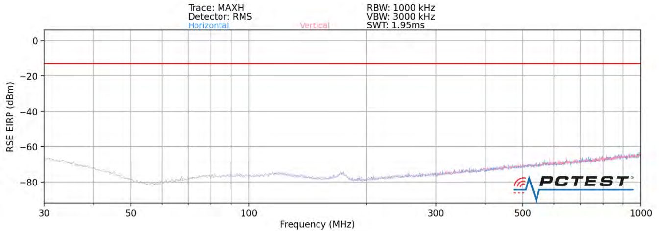
Plot 7-65. Ant1-n261 Radiated Spurious Plot (1CC QPSK Mid Channel H Beam)
