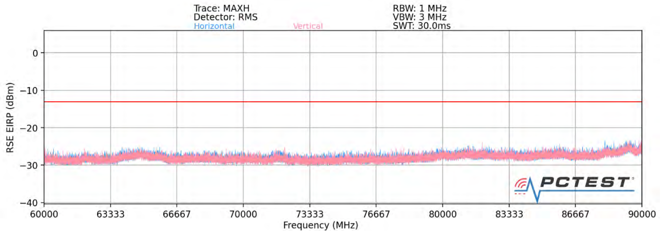
Plot 7-75. Ant1-n261 Radiated Spurious Plot (1CC QPSK Mid Channel H Beam – ENDC Anchor B2)
