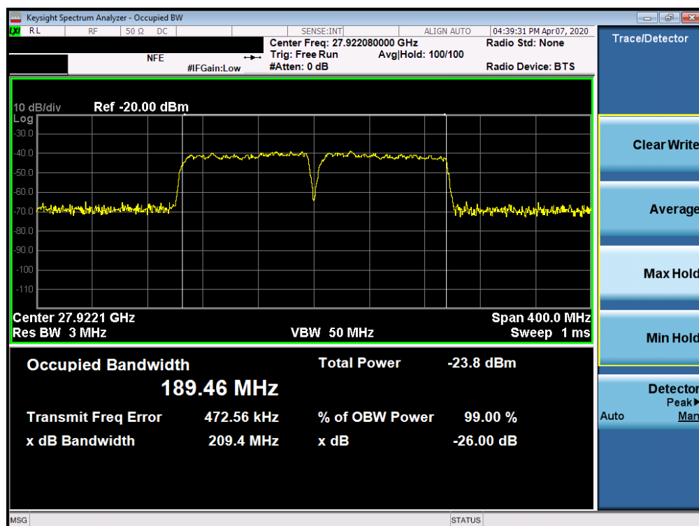
Plot 7-16. Ant1 Occupied Bandwidth Plot (100MHz-2CC – pi/2-BPSK – Mid Channel)
