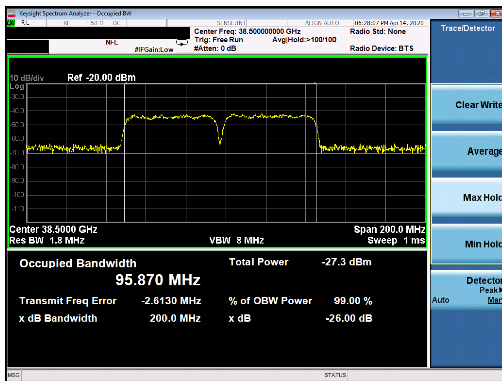
Plot 7-37. Ant1 Occupied Bandwidth Plot (50MHz-2CC – QPSK – Mid Channel)
