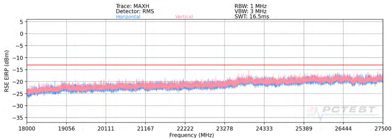
Plot 7-83. Ant2-n261 Radiated Spurious Plot (1CC QPSK Mid Channel H Beam – ENDC Anchor B2)
