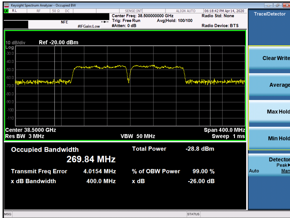
Plot 7-46. Ant1 Occupied Bandwidth Plot (100MHz-2CC – 16QAM – Mid Channel)
