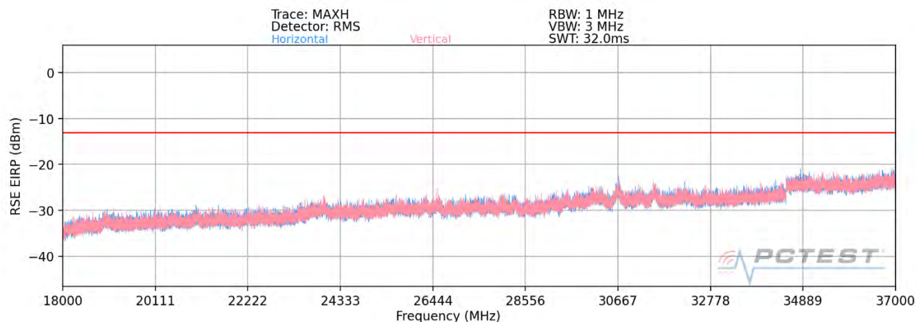
Plot 7-96. Ant1-n260 Radiated Spurious Plot (1CC QPSK Mid Channel V Beam – ENDC)
