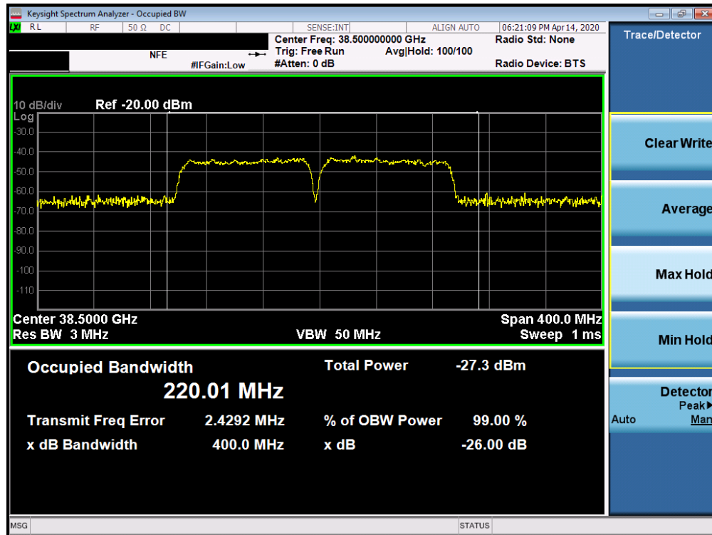
Plot 7-48. Ant1 Occupied Bandwidth Plot (100MHz-2CC – pi/2-BPSK – Mid Channel)
