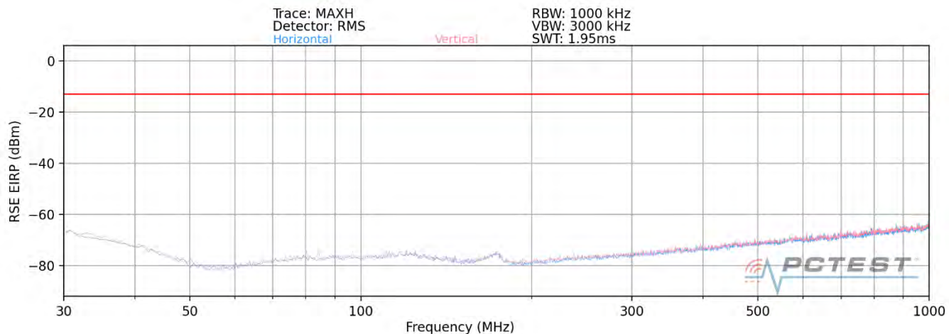
Plot 7-92. Ant1-n260 Radiated Spurious Plot (1CC QPSK Mid Channel V Beam)
