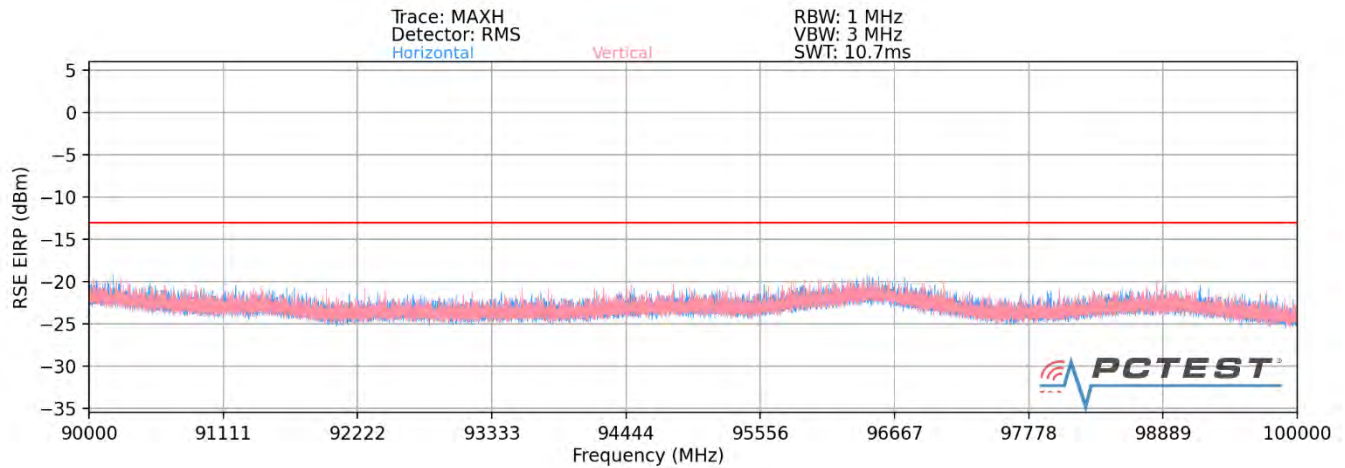
Plot 7-77. Ant1-n261 Radiated Spurious Plot (1CC QPSK Mid Channel H Beam – ENDC Anchor B2)
