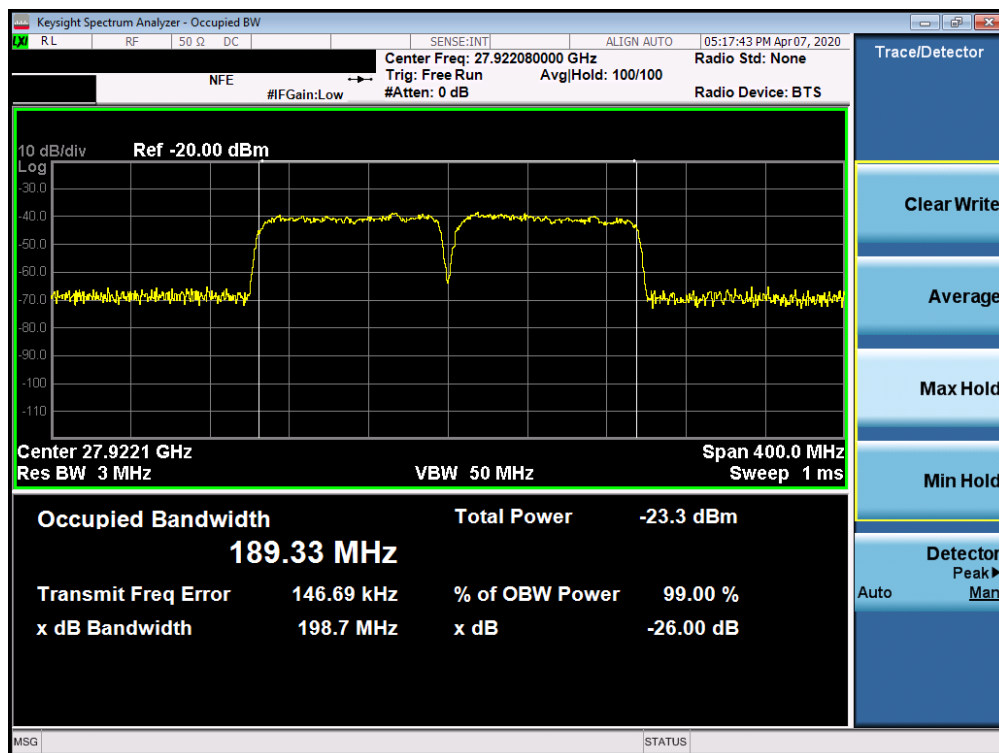
Plot 7-32. Ant2 Occupied Bandwidth Plot (100MHz-2CC – pi/2-BPSK – Mid Channel)
