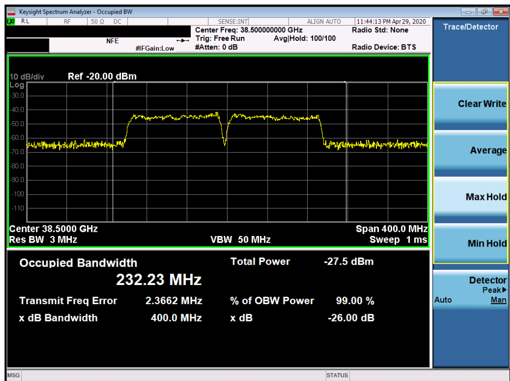
Plot 7-63. Ant2 Occupied Bandwidth Plot (100MHz-2CC – 64QAM – Mid Channel)
