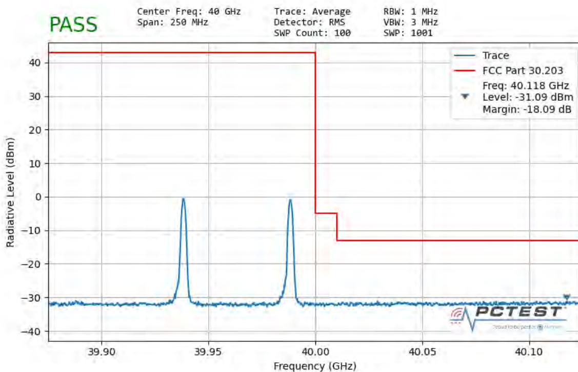
Plot 7-162. Ant1 Upper Band Edge (50MHz-2CC – QPSK 1 RB)
