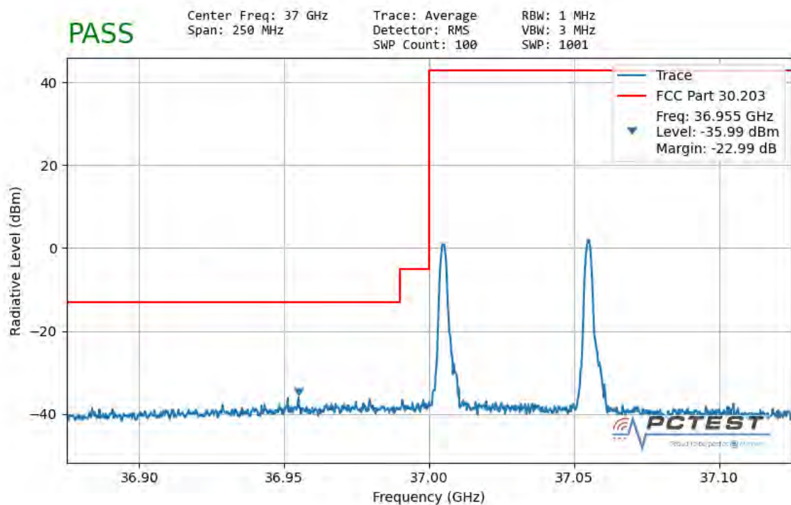
Plot 7-158. Ant1 Lower Band Edge (50MHz-2CC – QPSK 1 RB)
