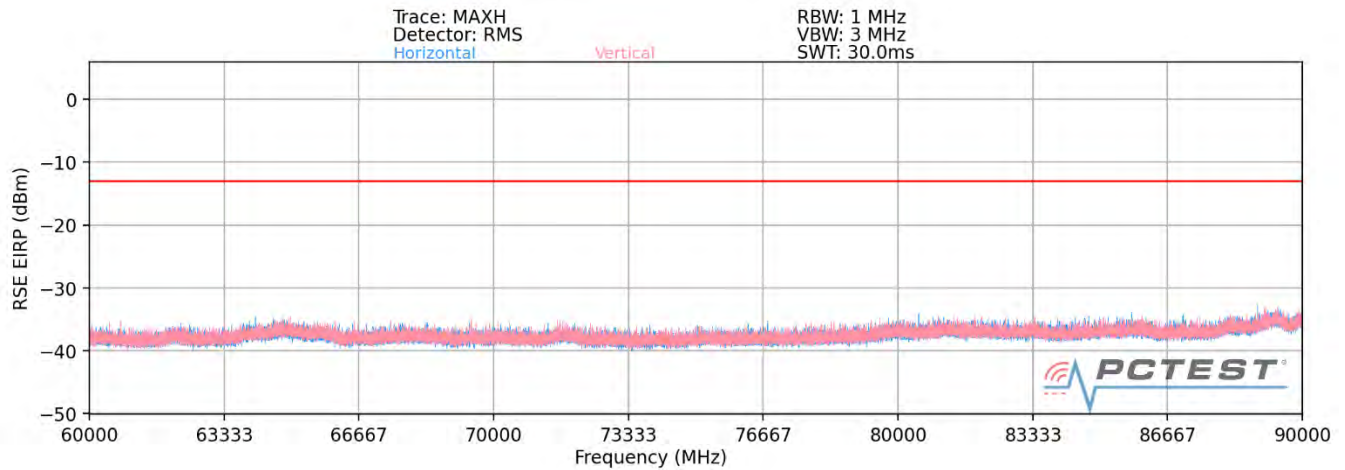
Plot 7-100. Ant1-n260 Radiated Spurious Plot (1CC QPSK Mid Channel V Beam – ENDC)
