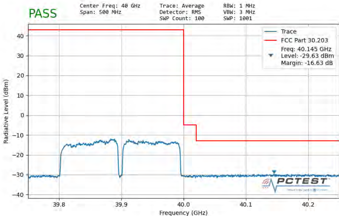
Plot 7-185. Ant2 Upper Band Edge (100MHz-2CC – QPSK Full RB)
