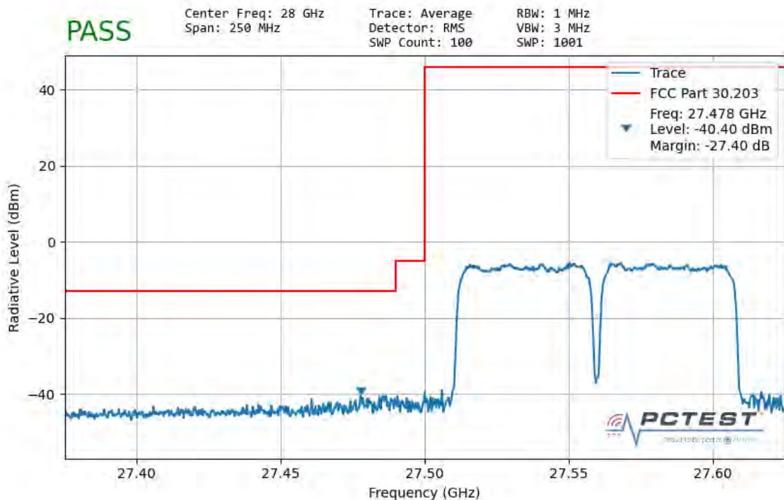
Plot 7-141. Ant2 Lower Band Edge (50MHz-2CC – QPSK Full RB)
