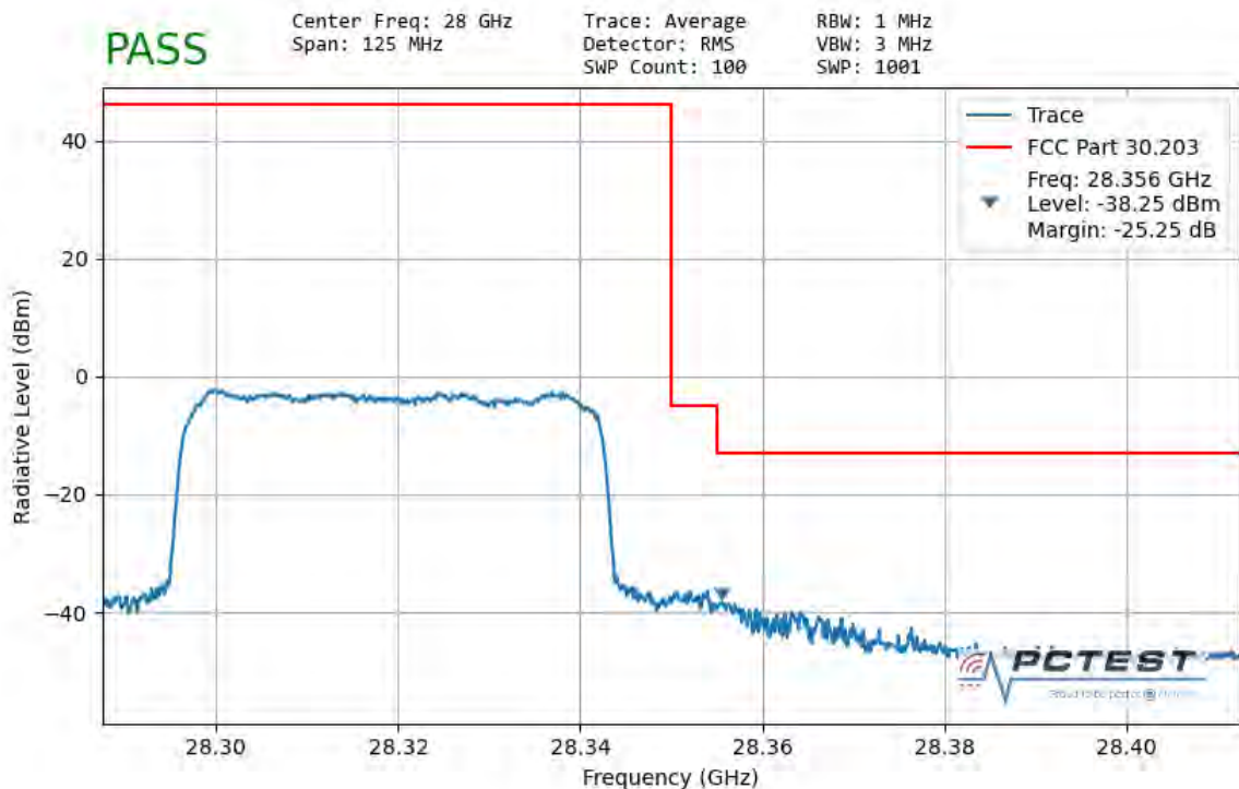
Plot 7-143. Ant2 Upper Band Edge (50MHz-1CC – QPSK Full RB)
