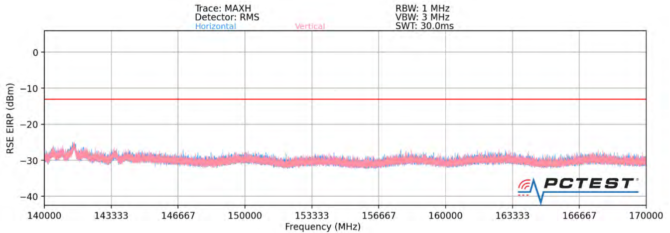
Plot 7-119. Ant2-n260 Radiated Spurious Plot (1CC QPSK Mid Channel H Beam – ENDC)
