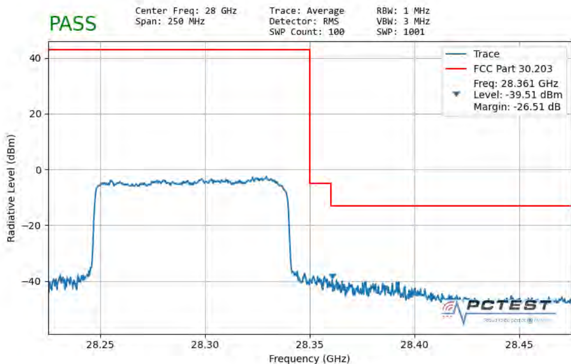
Plot 7-135. Ant1 Upper Band Edge (100MHz-1CC – QPSK Full RB)
