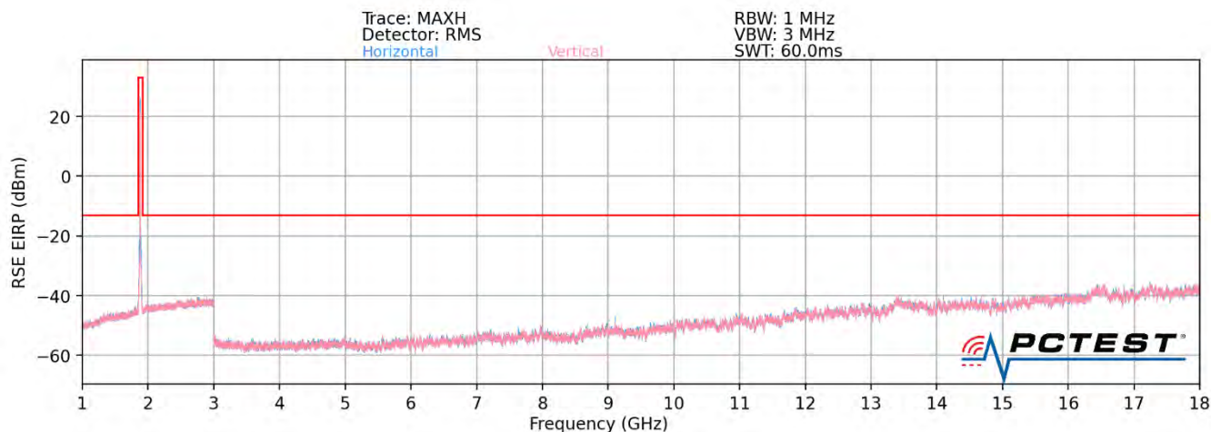
Plot 7-110. Ant2-n260 Radiated Spurious Plot 1GHz - 18GHz (1CC QPSK Mid Channel V Beam – ENDC)
