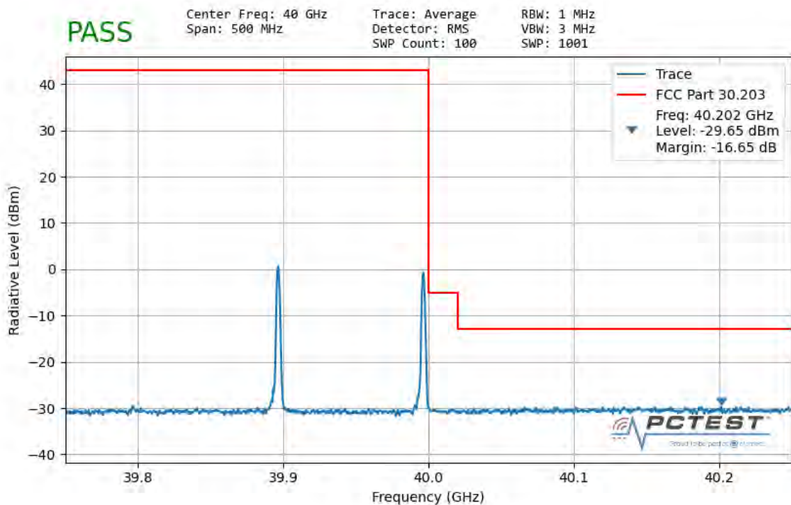
Plot 7-186. Ant2 Upper Band Edge (100MHz-2CC – QPSK 1 RB)
