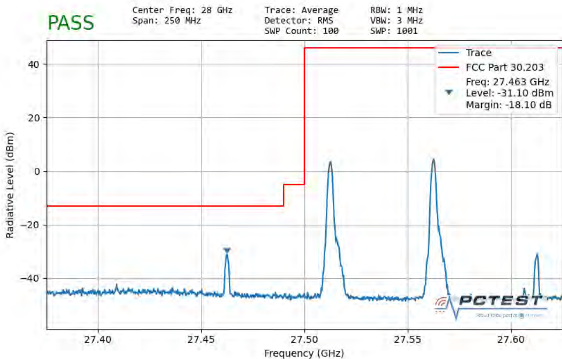
Plot 7-142. Ant2 Lower Band Edge (50MHz-2CC – QPSK 1 RB)
