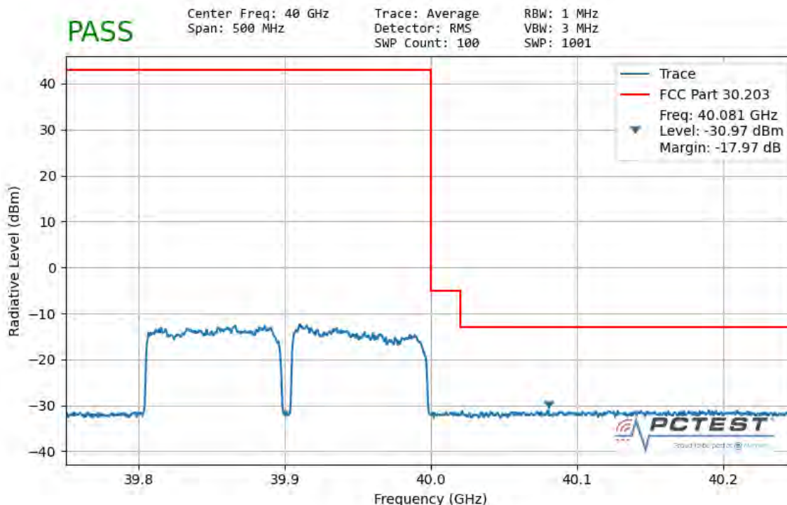
Plot 7-169. Ant1 Upper Band Edge (100MHz-2CC – QPSK Full RB)
