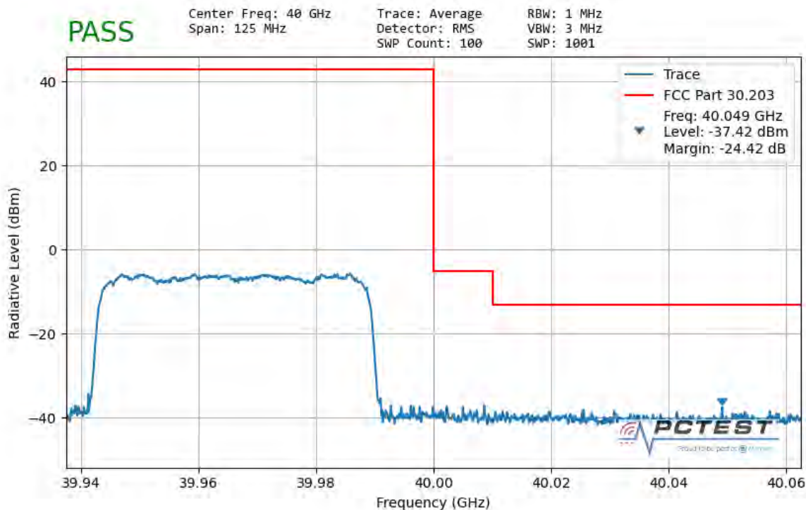
Plot 7-175. Ant2 Upper Band Edge (50MHz-1CC – QPSK Full RB)
