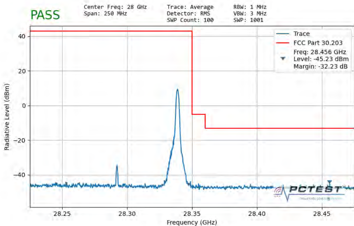
Plot 7-136. Ant1 Upper Band Edge (100MHz-1CC – QPSK 1 RB)
