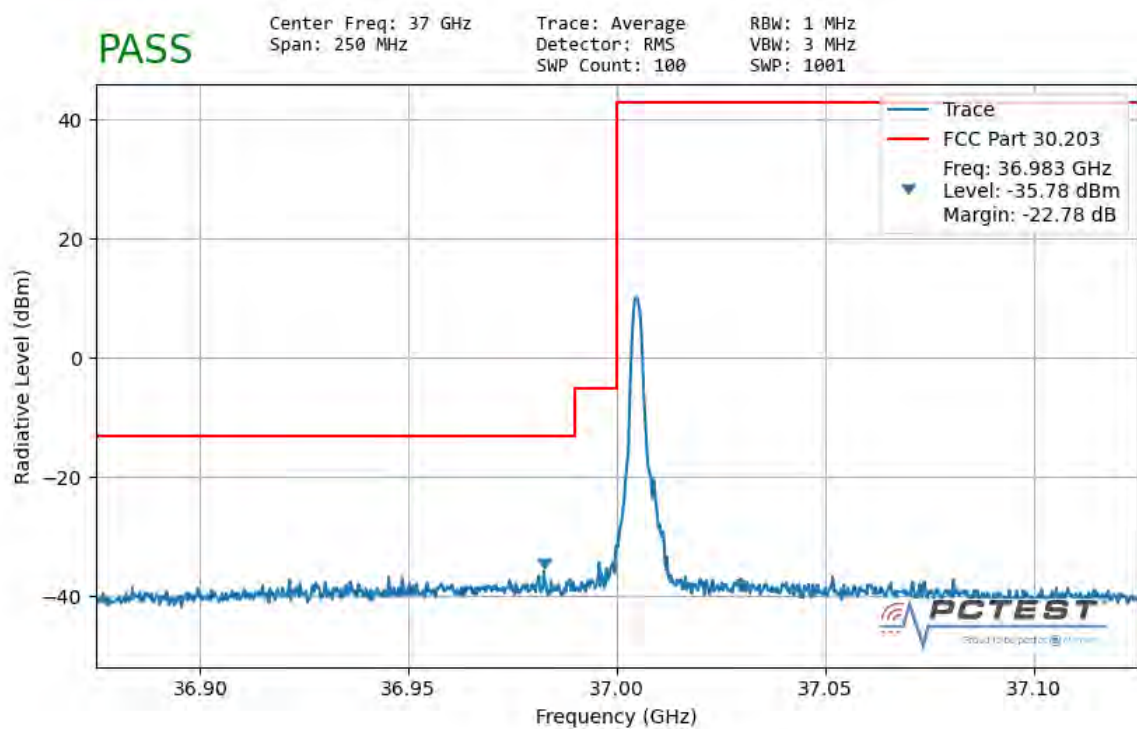
Plot 7-164. Ant1 Lower Band Edge (100MHz-1CC – QPSK 1 RB)
