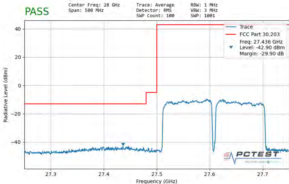
Plot 7-149. Ant2 Lower Band Edge (100MHz-2CC – QPSK Full RB)
