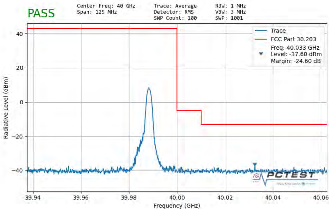
Plot 7-176. Ant2 Upper Band Edge (50MHz-1CC – QPSK 1 RB)
