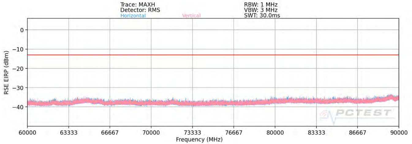
Plot 7-99. Ant1-n260 Radiated Spurious Plot (1CC QPSK Mid Channel H Beam – ENDC)
