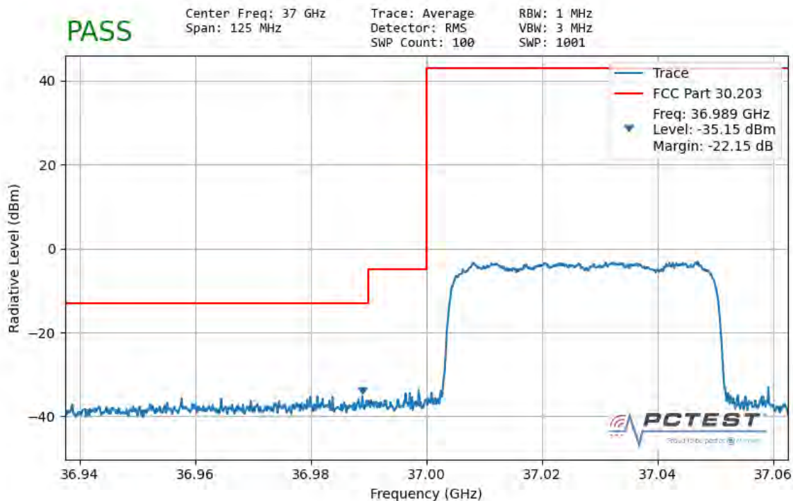
Plot 7-171. Ant2 Lower Band Edge (50MHz-1CC – QPSK Full RB)
