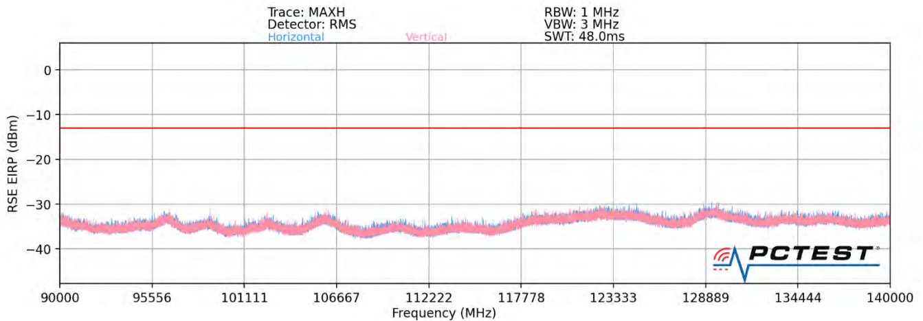
Plot 7-118. Ant2-n260 Radiated Spurious Plot (1CC QPSK Mid Channel V Beam – ENDC)
