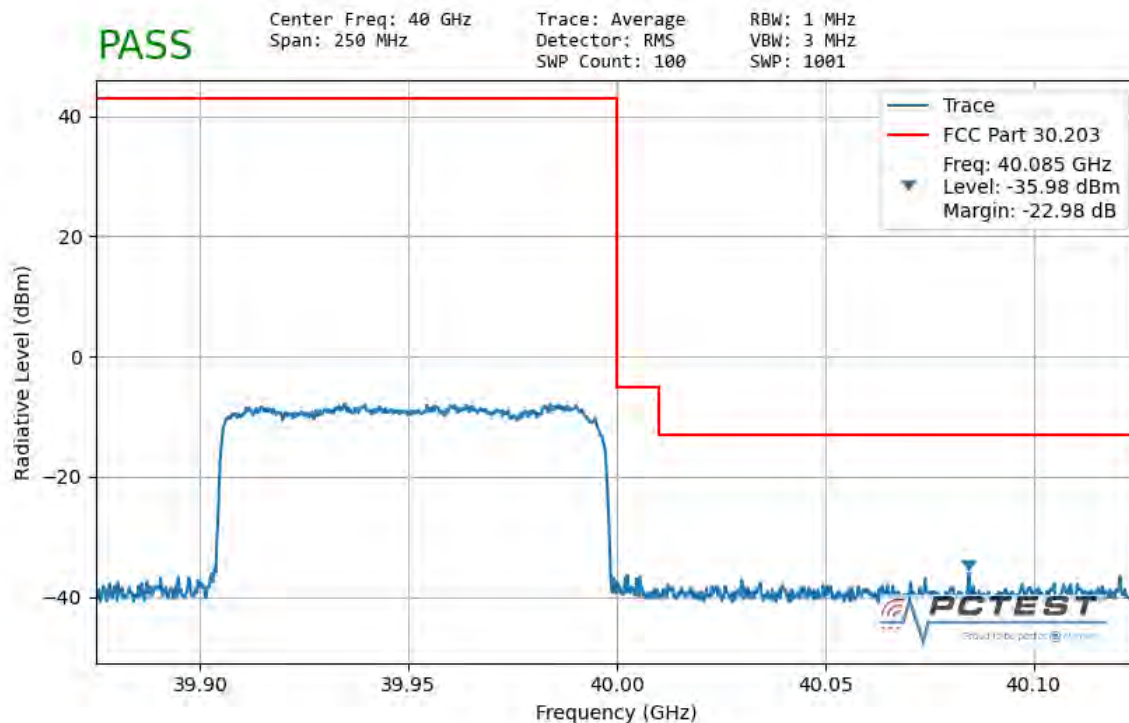
Plot 7-167. Ant1 Upper Band Edge (100MHz-1CC – QPSK Full RB)
