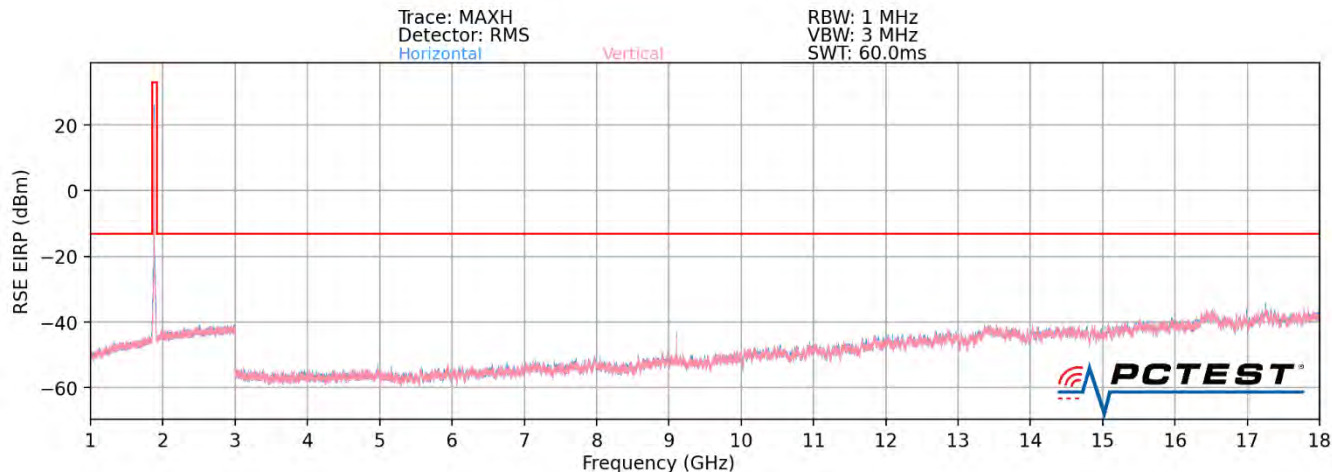
Plot 7-109. Ant2-n260 Radiated Spurious Plot 1GHz - 18GHz (1CC QPSK Mid Channel H Beam – ENDC)
