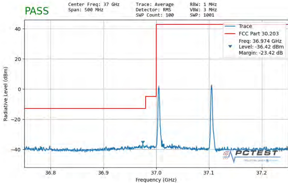
Plot 7-166. Ant1 Lower Band Edge (100MHz-2CC – QPSK 1 RB)
