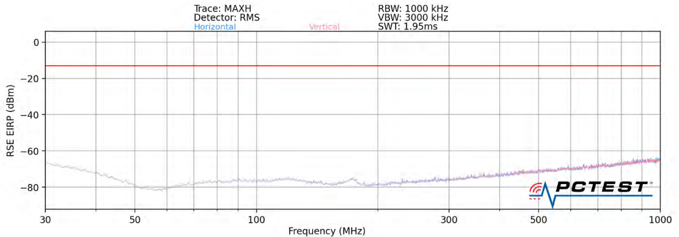
Plot 7-107. Ant2-n260 Radiated Spurious Plot (1CC QPSK Mid Channel H Beam)
