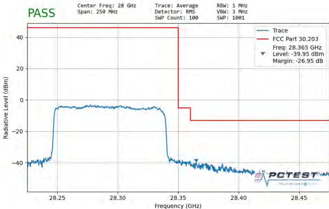
Plot 7-151. Ant2 Upper Band Edge (100MHz-1CC – QPSK Full RB)
