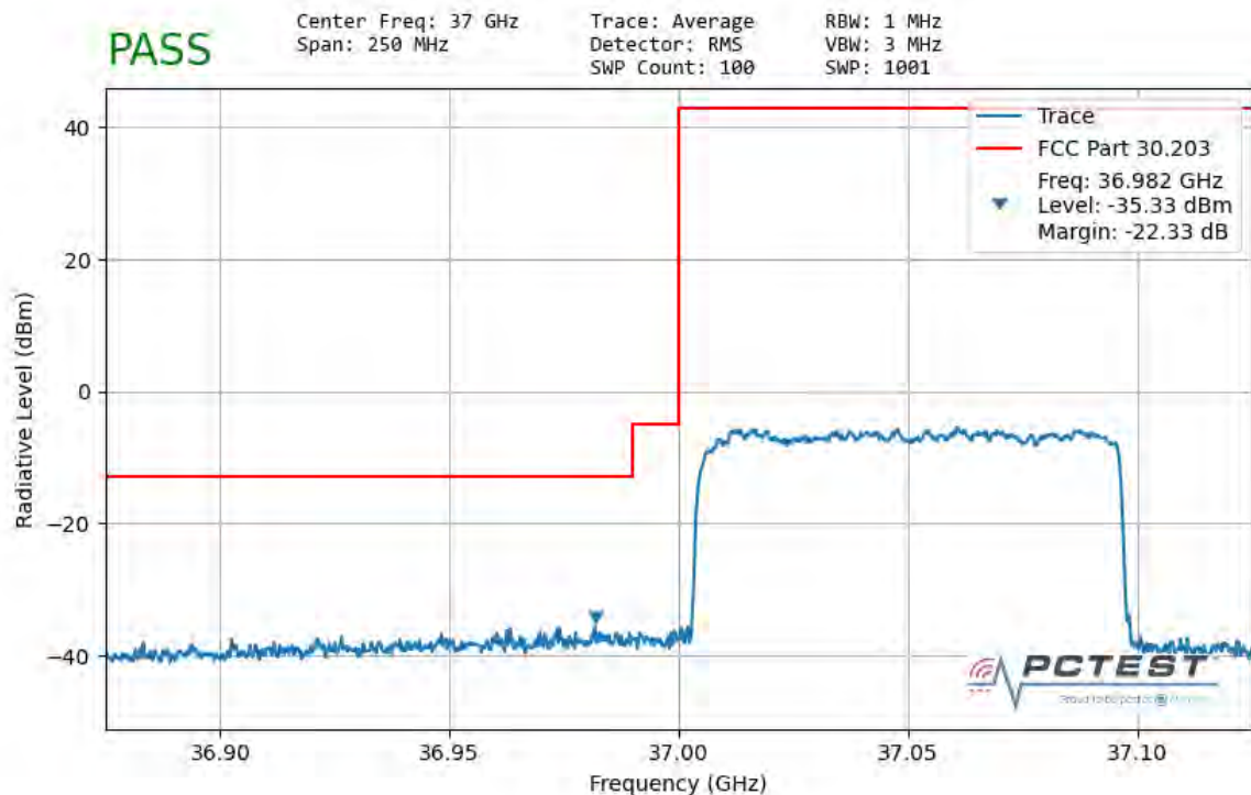
Plot 7-179. Ant2 Lower Band Edge (100MHz-1CC – QPSK Full RB)
