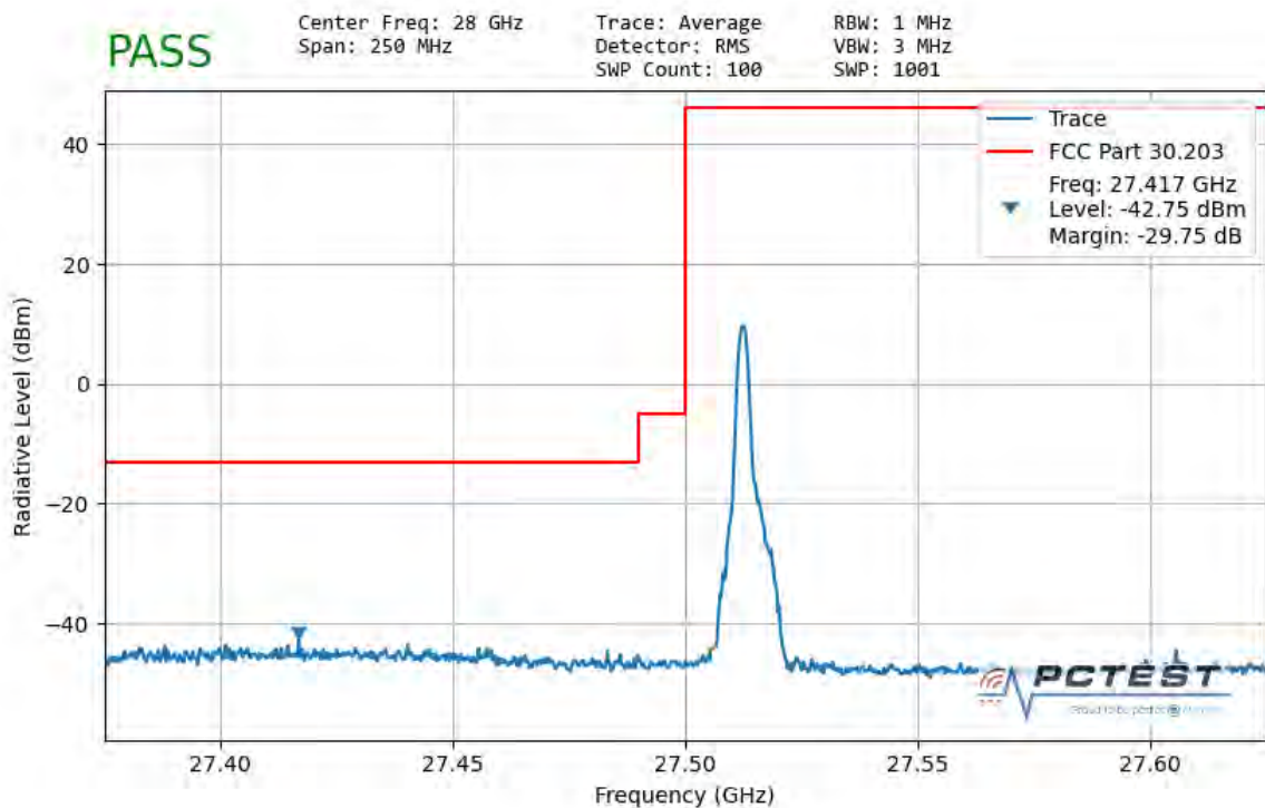
Plot 7-148. Ant2 Lower Band Edge (100MHz-1CC – QPSK 1 RB)
