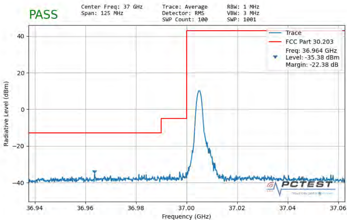
Plot 7-172. Ant2 Lower Band Edge (50MHz-1CC – QPSK 1 RB)
