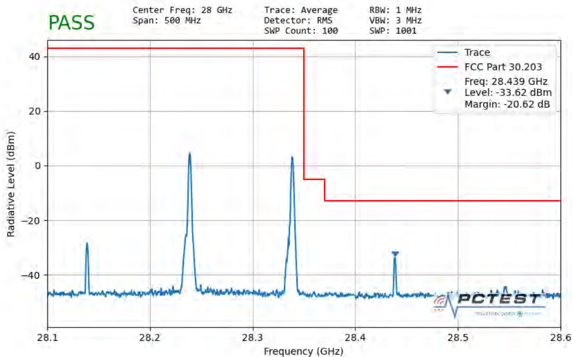
Plot 7-154. Ant2 Upper Band Edge (100MHz-2CC - QPSK 1 RB)
