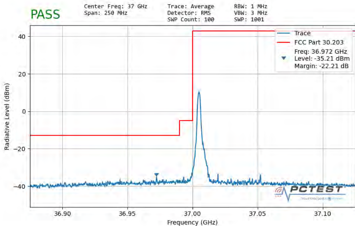
Plot 7-180. Ant2 Lower Band Edge (100MHz-1CC – QPSK 1 RB)
