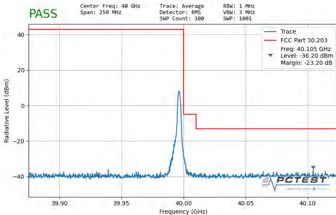
Plot 7-168. Ant1 Upper Band Edge (100MHz-1CC – QPSK 1 RB)
