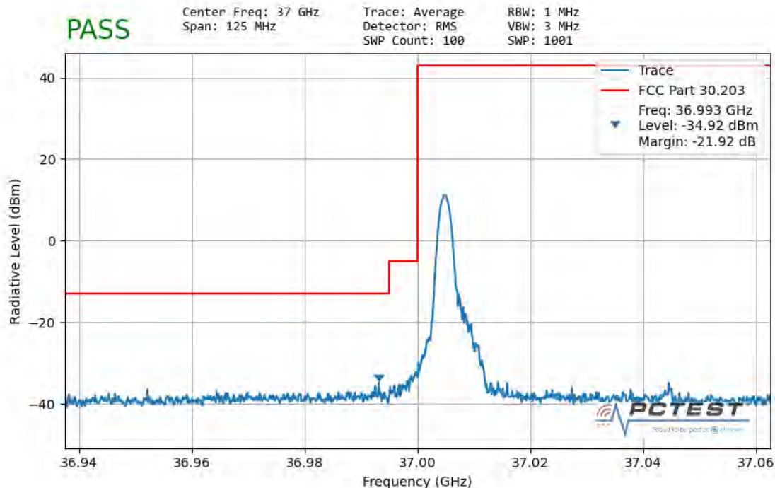
Plot 7-156. Ant1 Lower Band Edge (50MHz-1CC – QPSK 1 RB)
