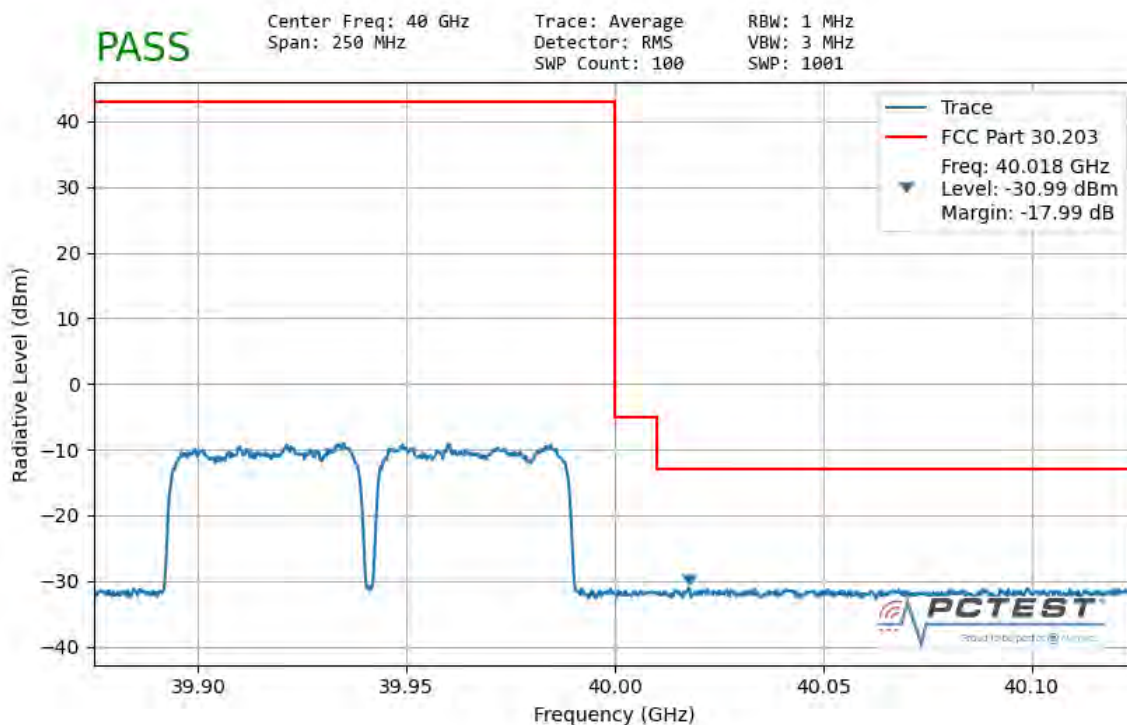
Plot 7-161. Ant1 Upper Band Edge (50MHz-2CC – QPSK Full RB)
