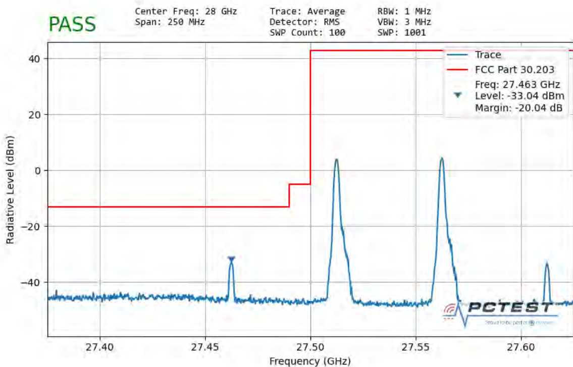
Plot 7-126. Ant1 Lower Band Edge (50MHz-2CC – QPSK 1 RB)
