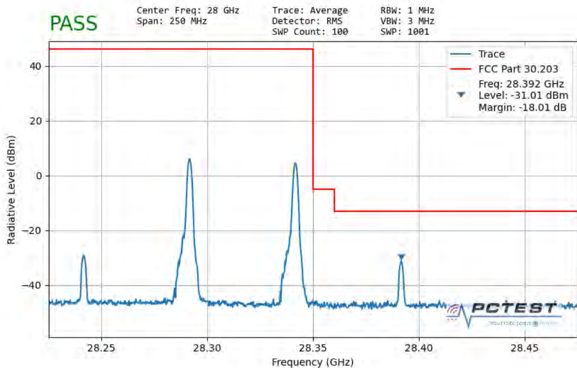
Plot 7-146. Ant2 Upper Band Edge (50MHz-2CC – QPSK 1 RB)
