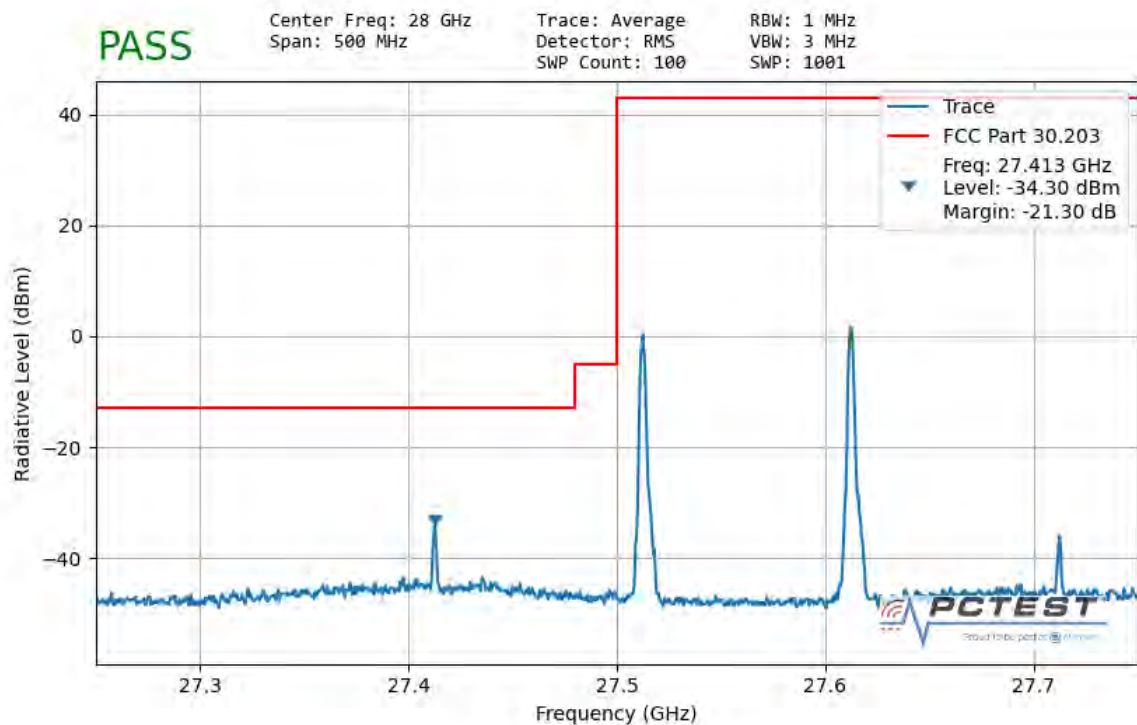
Plot 7-150. Ant2 Lower Band Edge (100MHz-2CC – QPSK 1 RB)
