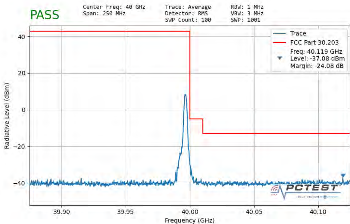
Plot 7-184. Ant2 Upper Band Edge (100MHz-1CC – QPSK 1 RB)
