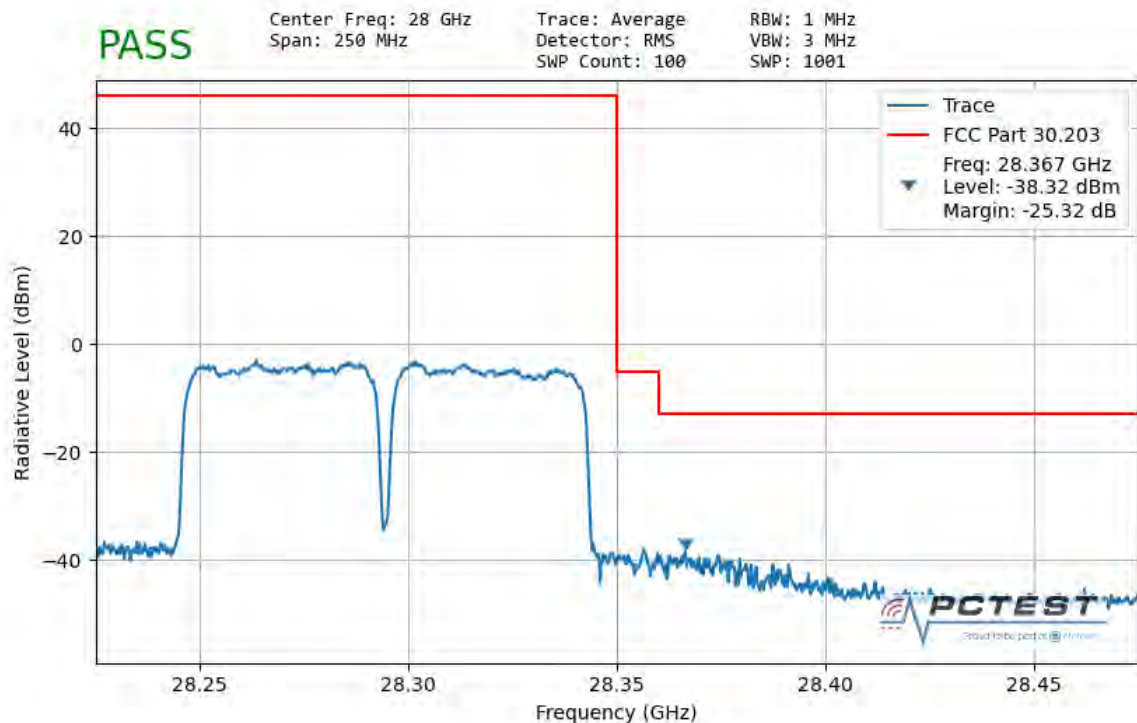
Plot 7-145. Ant2 Upper Band Edge (50MHz-2CC – QPSK Full RB)
