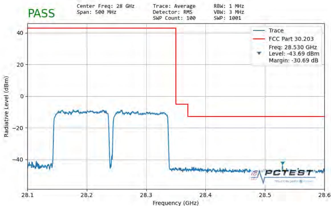
Plot 7-137. Ant1 Upper Band Edge (100MHz-2CC – QPSK Full RB)
