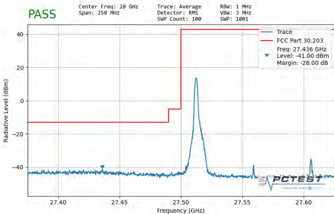
Plot 7-132. Ant1 Lower Band Edge (100MHz-1CC – QPSK 1 RB)
