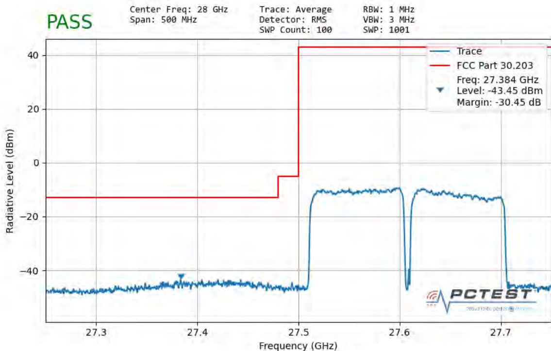
Plot 7-133. Ant1 Lower Band Edge (100MHz-2CC – QPSK Full RB)
