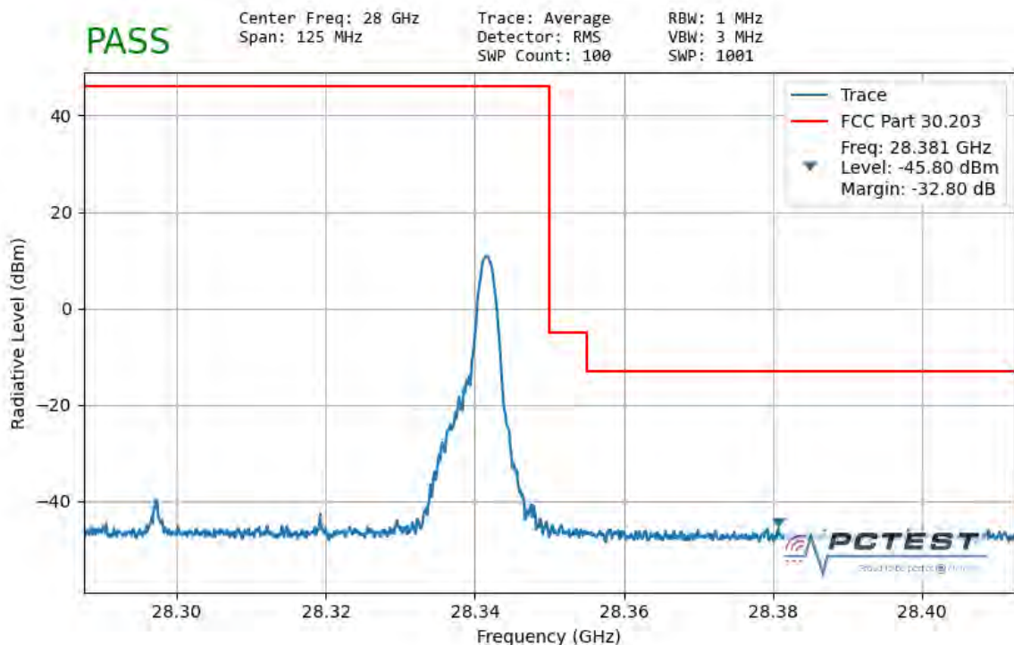
Plot 7-144. Ant2 Upper Band Edge (50MHz-1CC – QPSK 1 RB)
