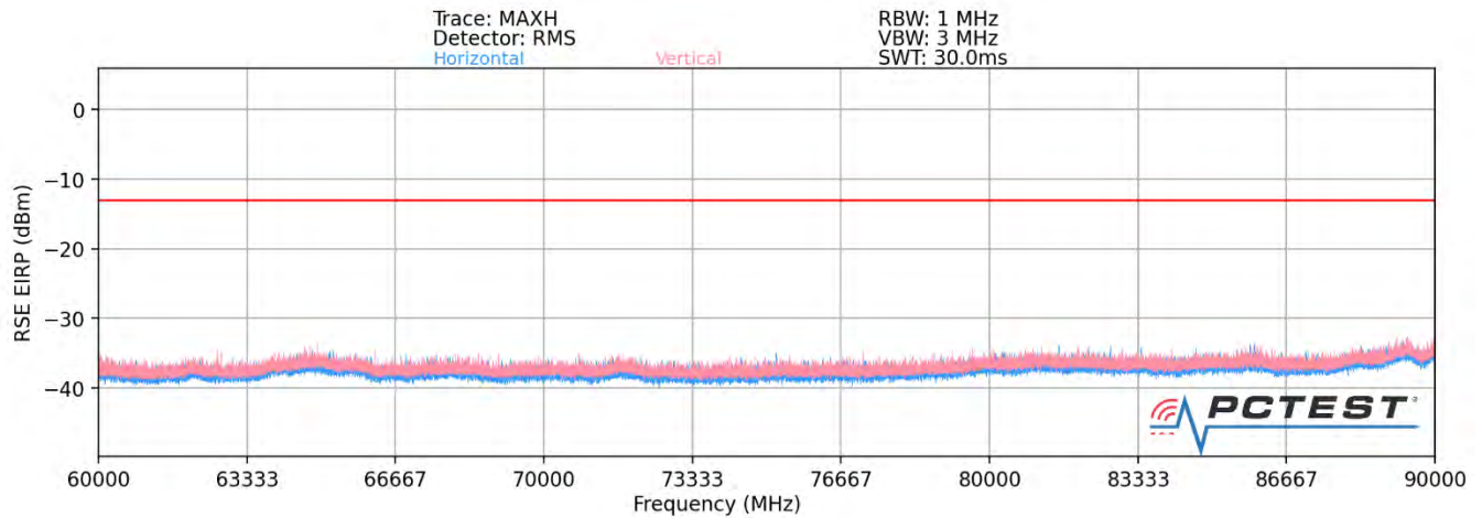
Plot 7-115. Ant2-n260 Radiated Spurious Plot (1CC QPSK Mid Channel H Beam – ENDC)
