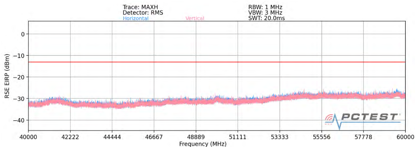
Plot 7-114. Ant2-n260 Radiated Spurious Plot (1CC QPSK Mid Channel V Beam – ENDC)
