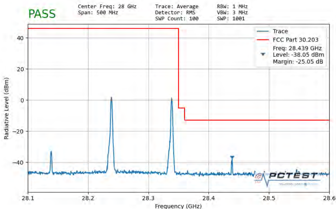
Plot 7-138. Ant1 Upper Band Edge (100MHz-2CC – QPSK 1 RB)
