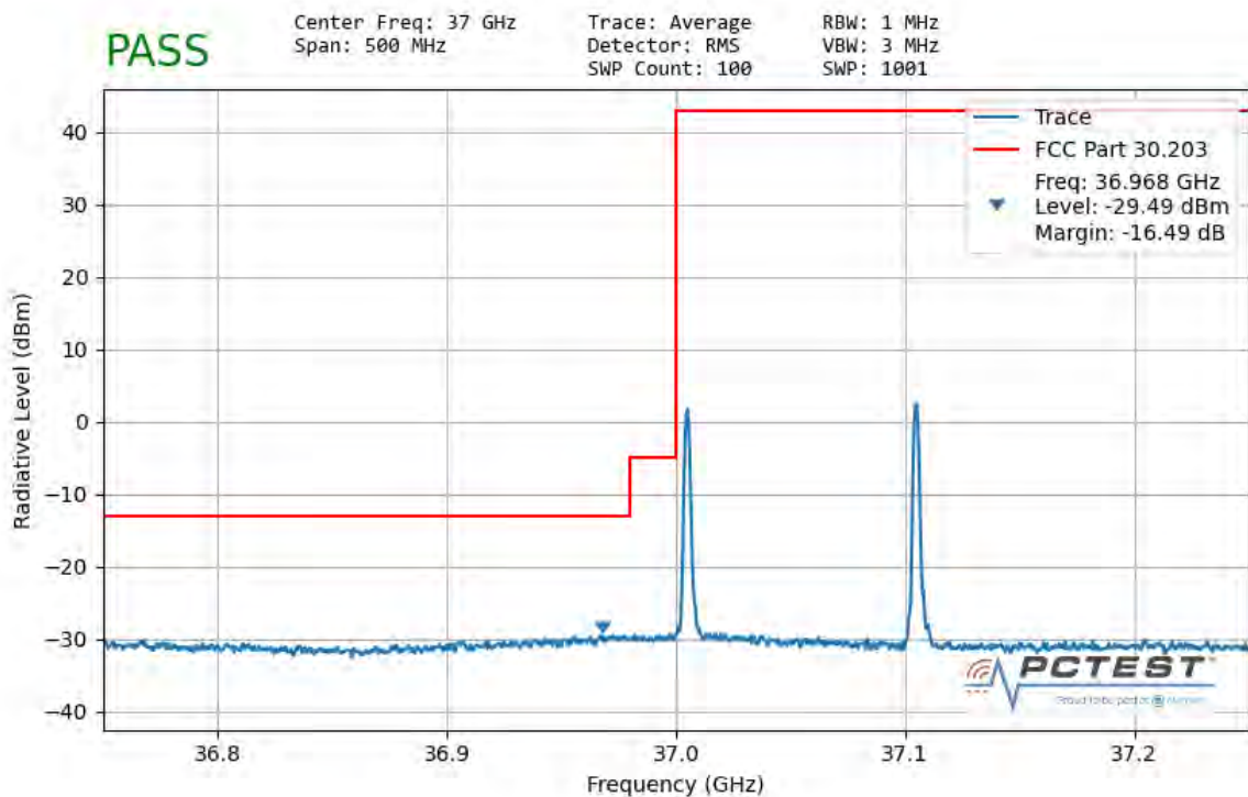
Plot 7-182. Ant2 Lower Band Edge (100MHz-2CC – QPSK 1 RB)
