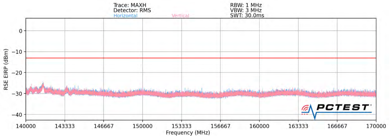
Plot 7-120. Ant2-n260 Radiated Spurious Plot (1CC QPSK Mid Channel V Beam – ENDC)
