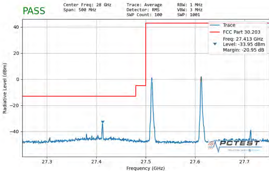
Plot 7-134. Ant1 Lower Band Edge (100MHz-2CC – QPSK 1 RB)
