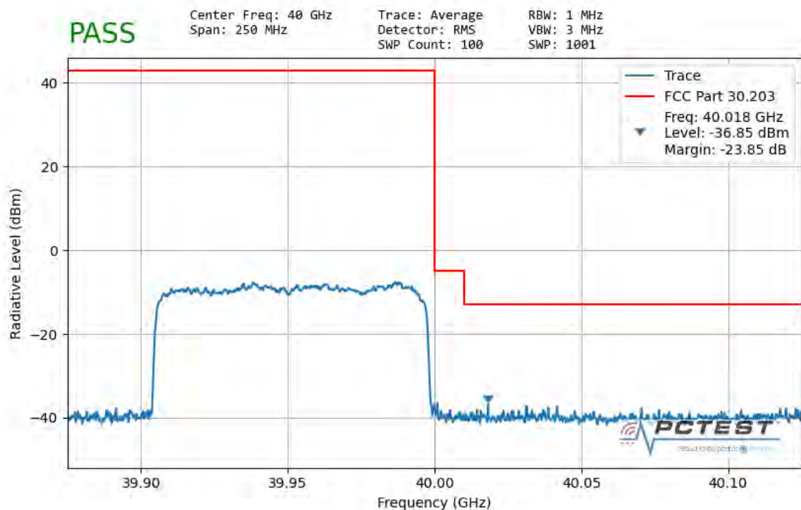
Plot 7-183. Ant2 Upper Band Edge (100MHz-1CC – QPSK Full RB)
