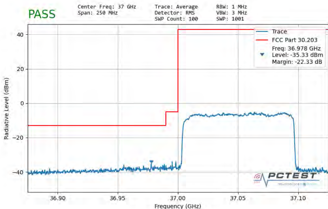
Plot 7-163. Ant1 Lower Band Edge (100MHz-1CC – QPSK Full RB)
