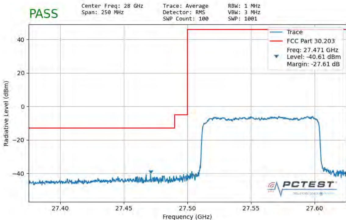
Plot 7-147. Ant2 Lower Band Edge (100MHz-1CC – QPSK Full RB)
