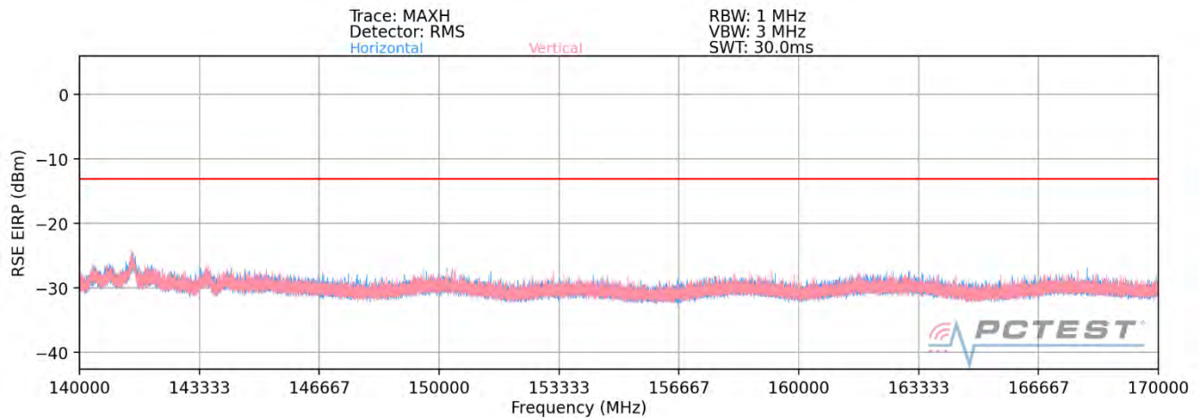
Plot 7-104. Ant1-n260 Radiated Spurious Plot (1CC QPSK Mid Channel V Beam – ENDC)
