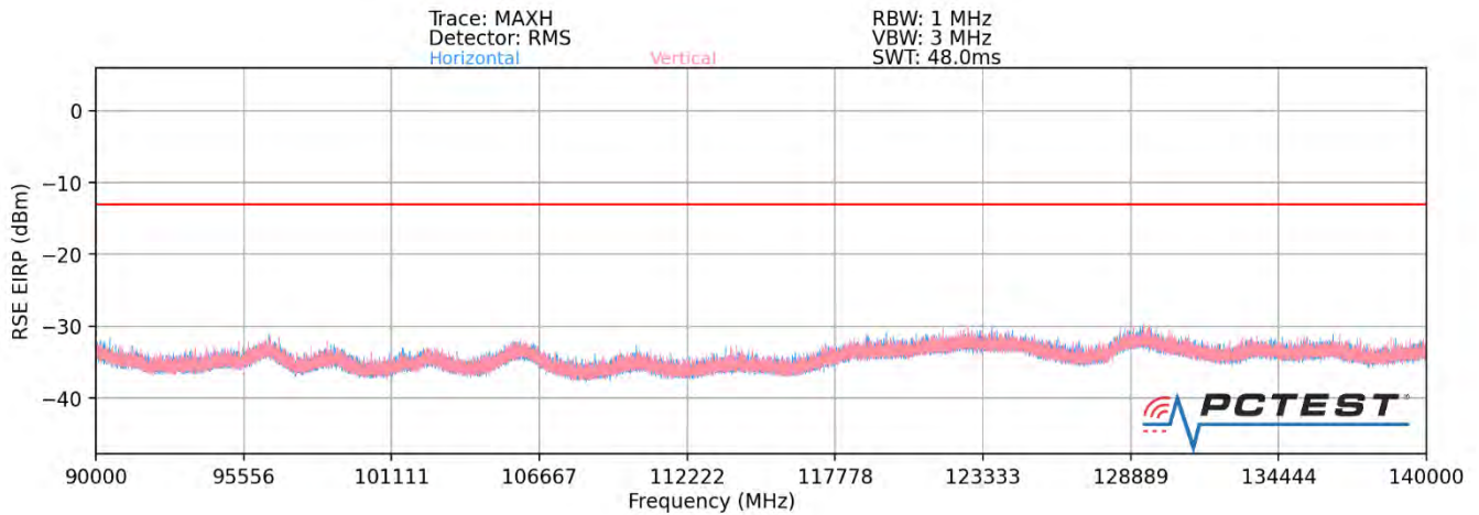
Plot 7-117. Ant2-n260 Radiated Spurious Plot (1CC QPSK Mid Channel H Beam – ENDC)
