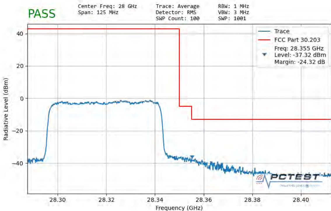
Plot 7-127. Ant1 Upper Band Edge (50MHz-1CC – QPSK Full RB)
