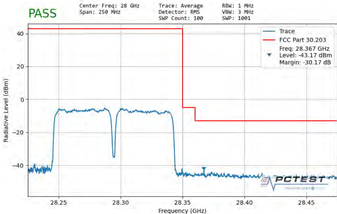
Plot 7-129. Ant1 Upper Band Edge (50MHz-2CC – QPSK Full RB)
