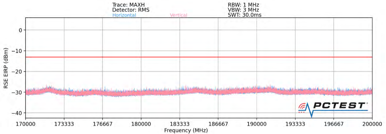
Plot 7-121. Ant2-n260 Radiated Spurious Plot (1CC QPSK Mid Channel H Beam – ENDC)
