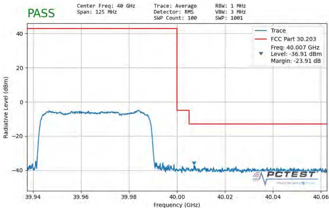
Plot 7-159. Ant1 Upper Band Edge (50MHz-1CC – QPSK Full RB)
