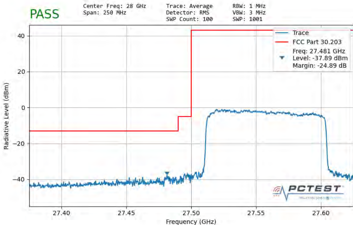
Plot 7-131. Ant1 Lower Band Edge (100MHz-1CC – QPSK Full RB)
