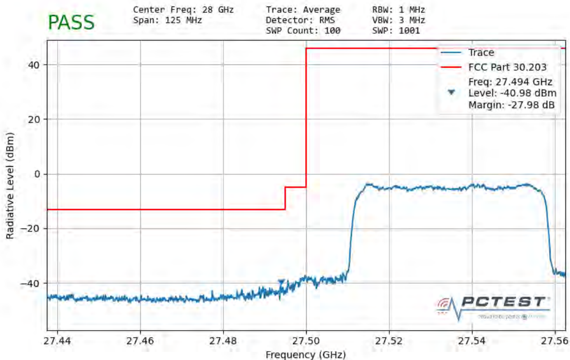
Plot 7-139. Ant2 Lower Band Edge (50MHz-1CC – QPSK Full RB)
