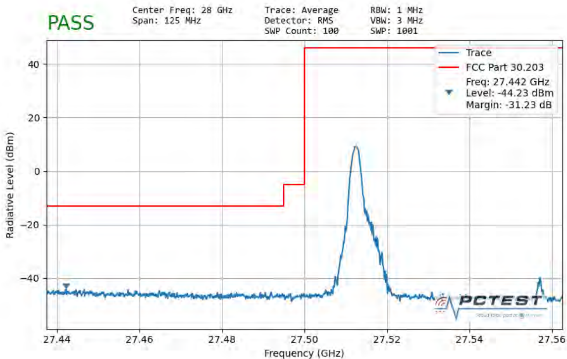
Plot 7-140. Ant2 Lower Band Edge (50MHz-1CC – QPSK 1 RB)
