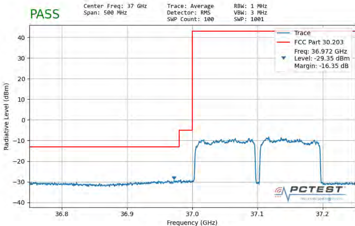
Plot 7-181. Ant2 Lower Band Edge (100MHz-2CC – QPSK Full RB)
