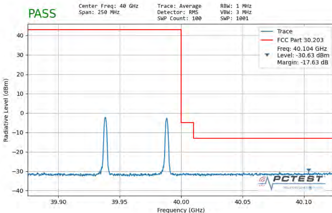
Plot 7-178. Ant2 Upper Band Edge (50MHz-2CC – QPSK 1 RB)
