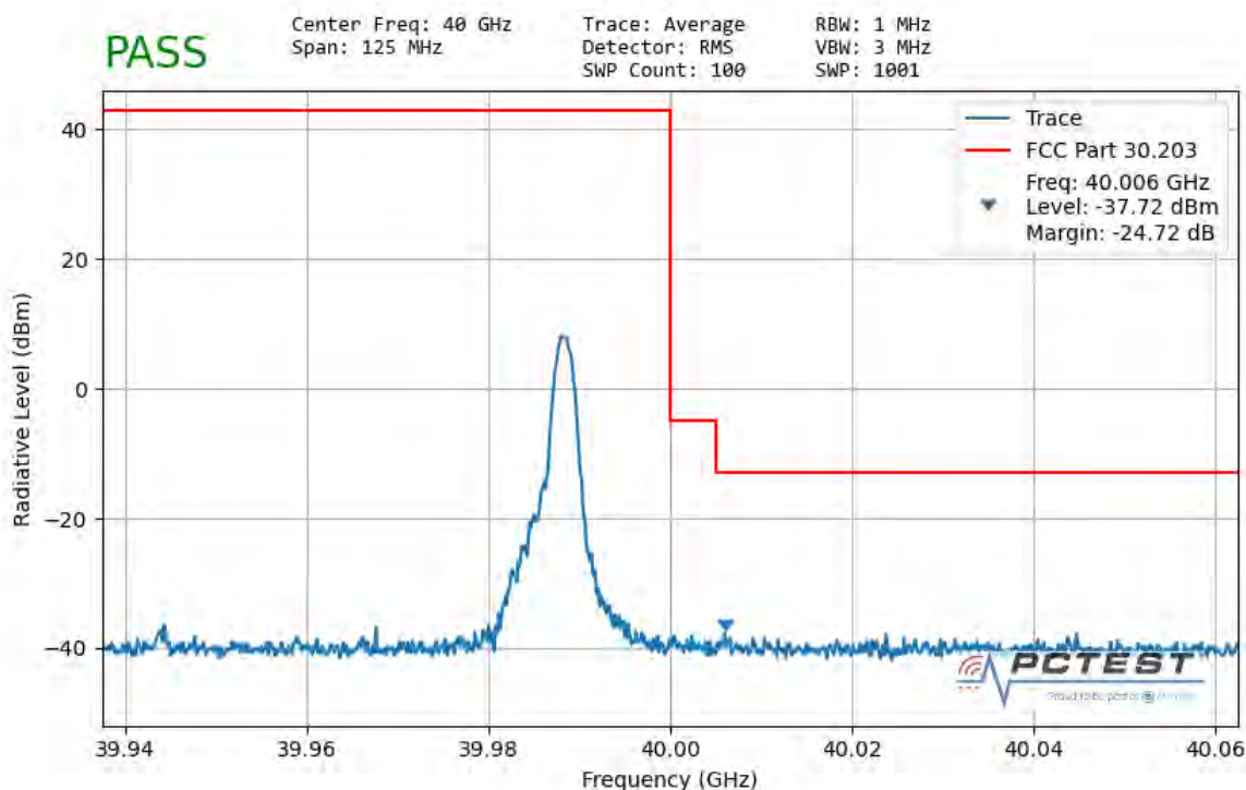
Plot 7-160. Ant1 Upper Band Edge (50MHz-1CC – QPSK 1 RB)
