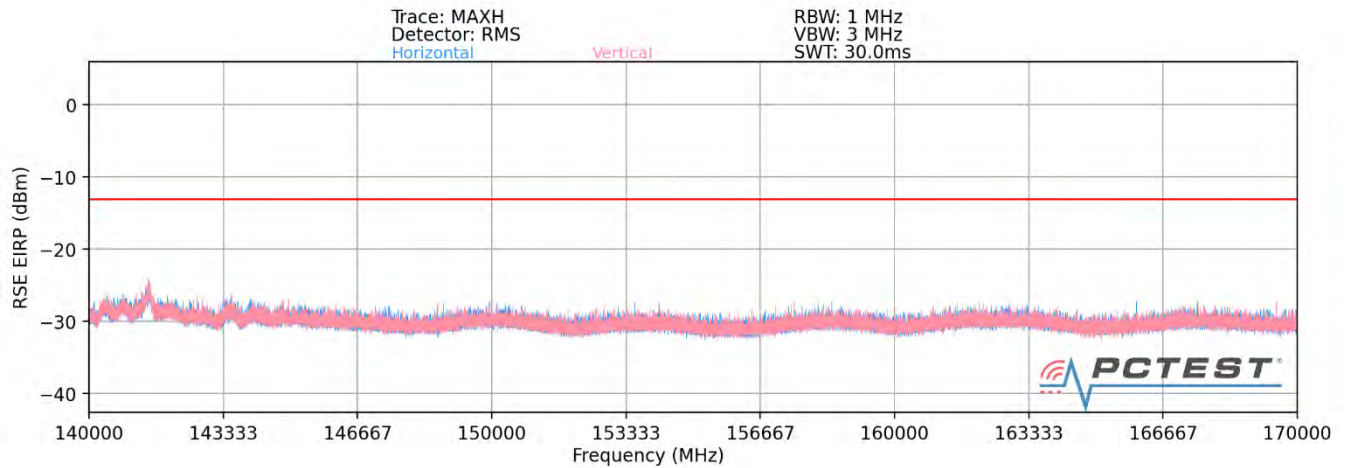
Plot 7-103. Ant1-n260 Radiated Spurious Plot (1CC QPSK Mid Channel H Beam – ENDC)
