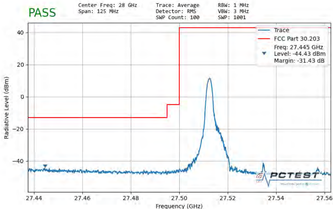
Plot 7-124. Ant1 Lower Band Edge (50MHz-1CC – QPSK 1 RB)
