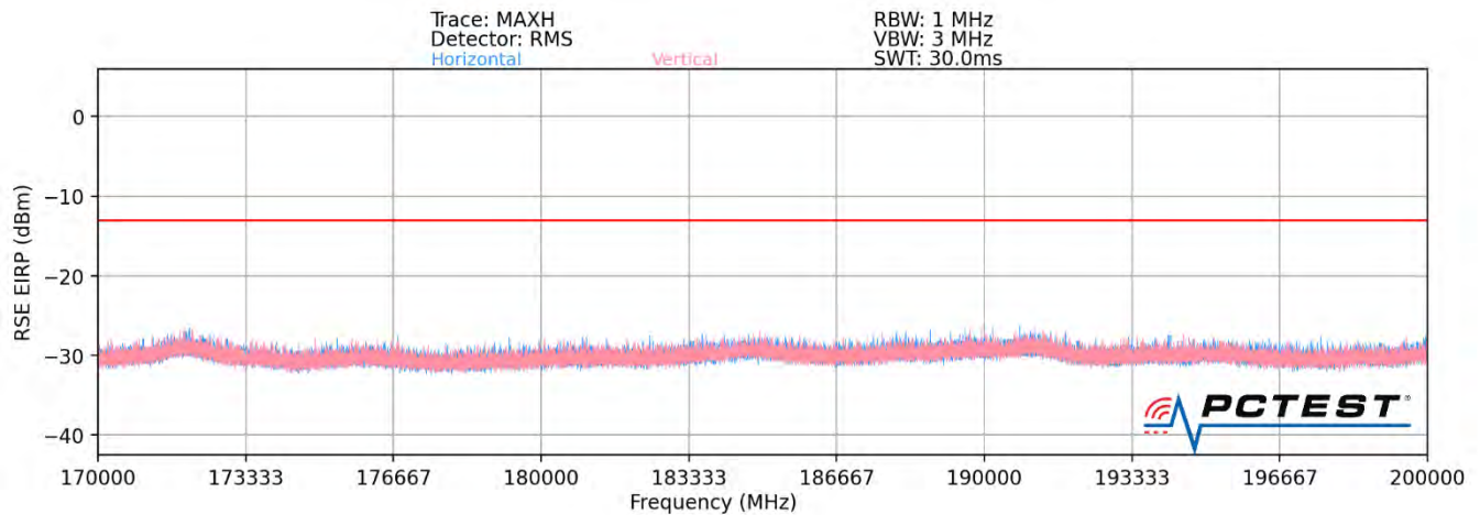
Plot 7-122. Ant2-n260 Radiated Spurious Plot (1CC QPSK Mid Channel V Beam – ENDC)
