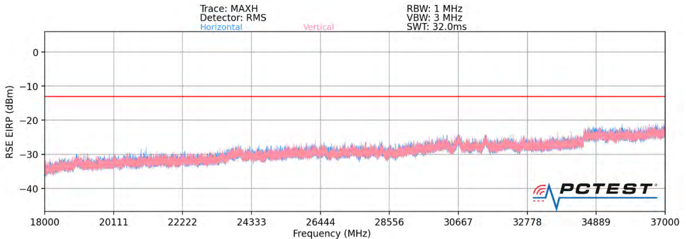
Plot 7-112. Ant2-n260 Radiated Spurious Plot (1CC QPSK Mid Channel V Beam – ENDC)
