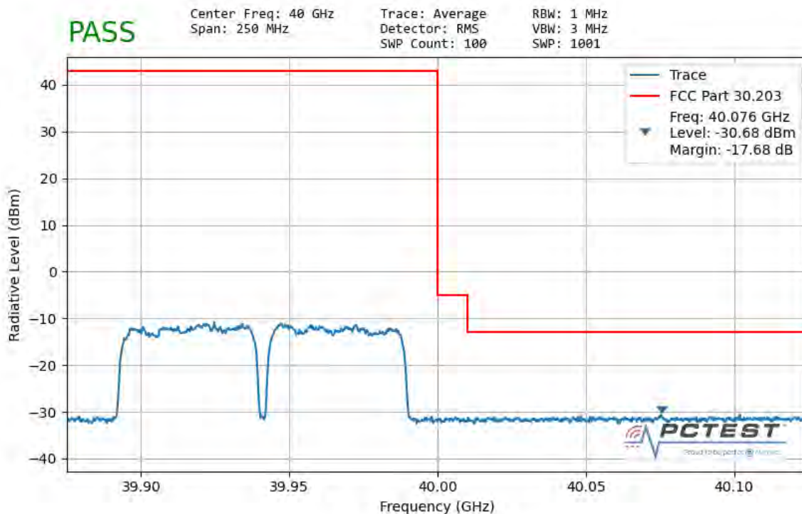
Plot 7-177. Ant2 Upper Band Edge (50MHz-2CC – QPSK Full RB)
