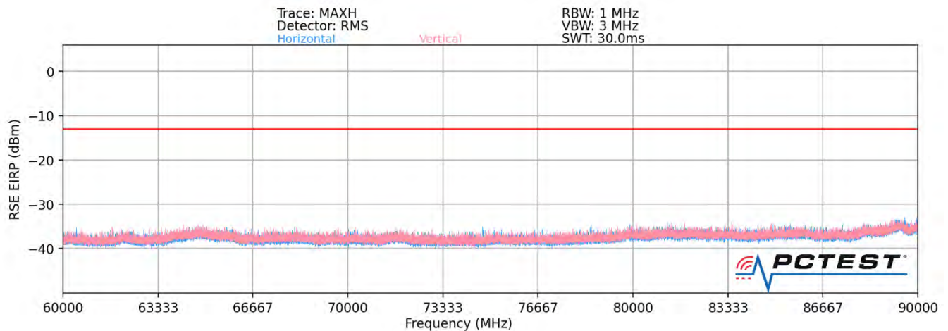
Plot 7-116. Ant2-n260 Radiated Spurious Plot (1CC QPSK Mid Channel V Beam – ENDC)
