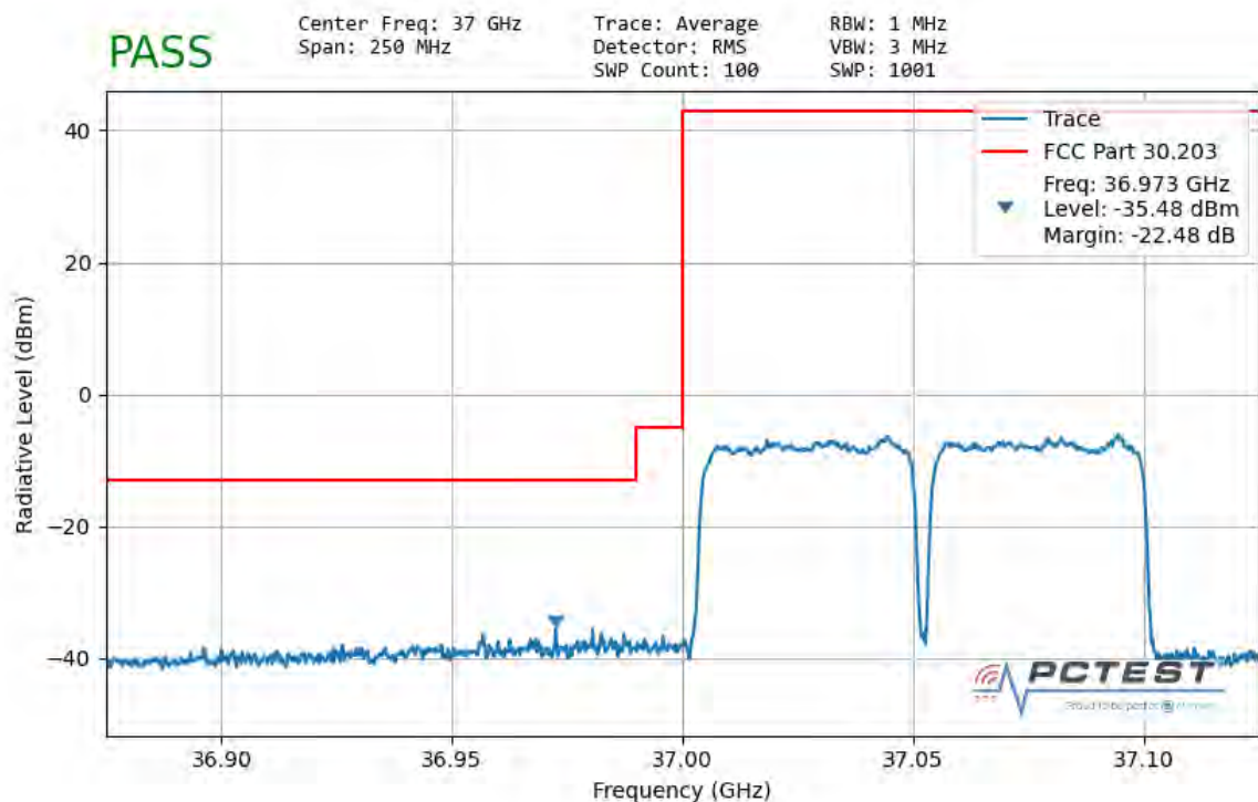
Plot 7-157. Ant1 Lower Band Edge (50MHz-2CC – QPSK Full RB)
