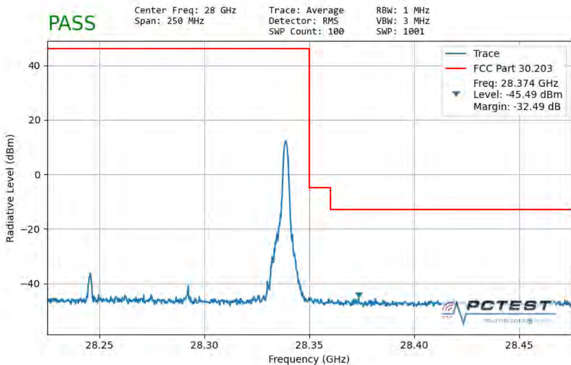
Plot 7-152. Ant2 Upper Band Edge (100MHz-1CC – QPSK 1 RB)
