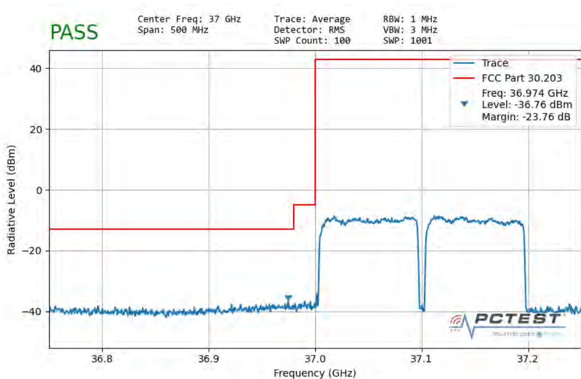
Plot 7-165. Ant1 Lower Band Edge (100MHz-2CC – QPSK Full RB)
