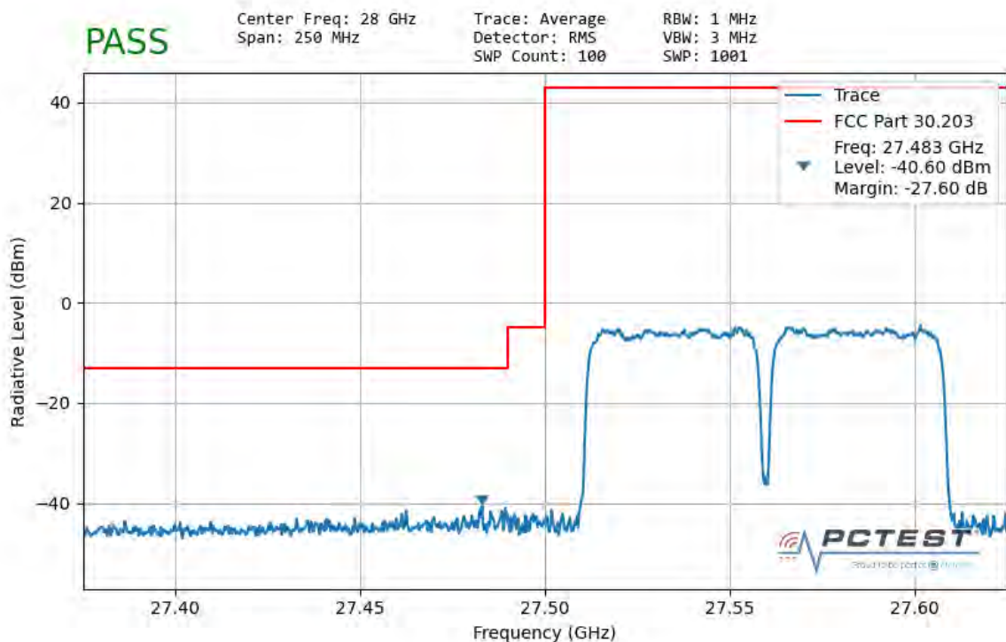
Plot 7-125. Ant1 Lower Band Edge (50MHz-2CC – QPSK Full RB)
