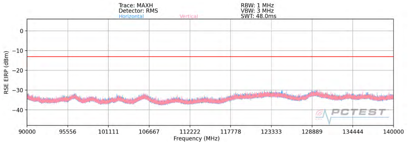
Plot 7-102. Ant1-n260 Radiated Spurious Plot (1CC QPSK Mid Channel V Beam – ENDC)
