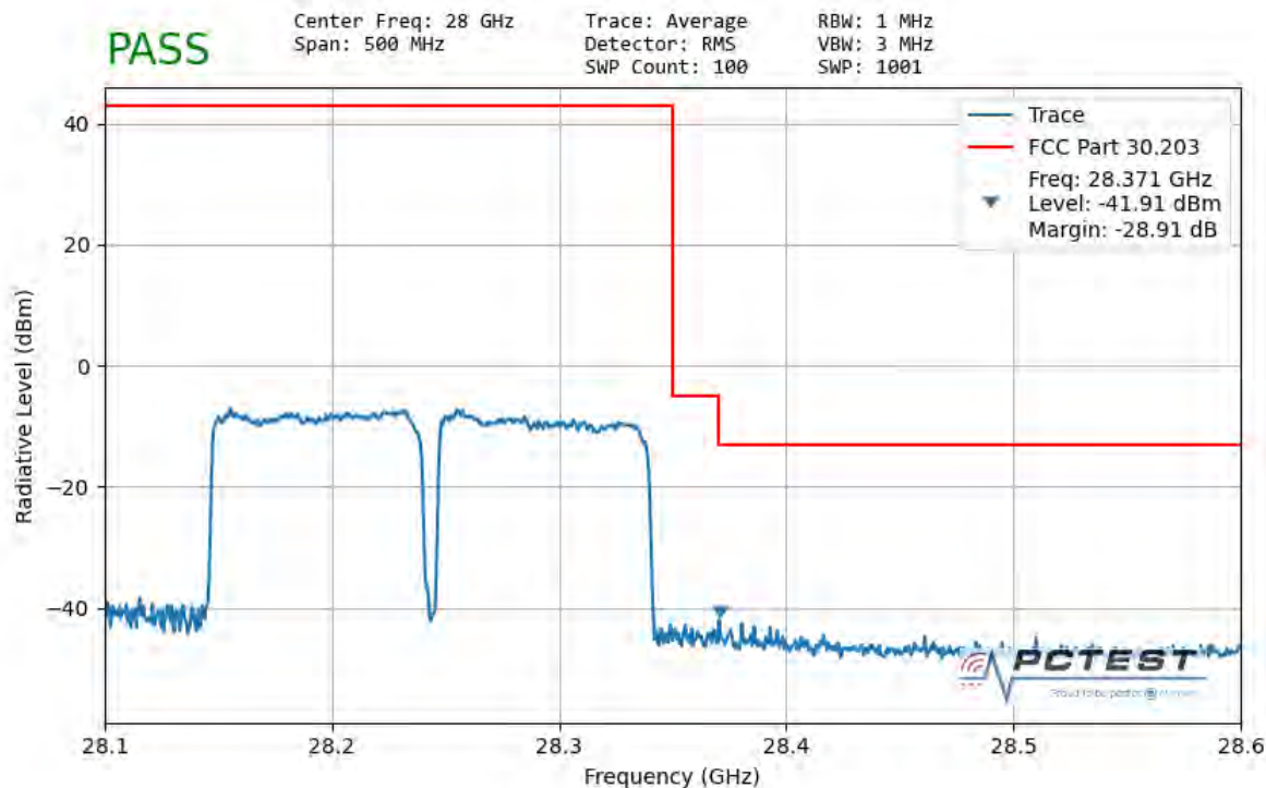
Plot 7-153. Ant2 Upper Band Edge (100MHz-2CC - QPSK Full RB)
