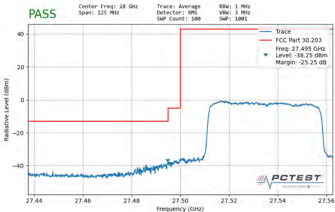
Plot 7-123. Ant1 Lower Band Edge (50MHz-1CC – QPSK Full RB)
