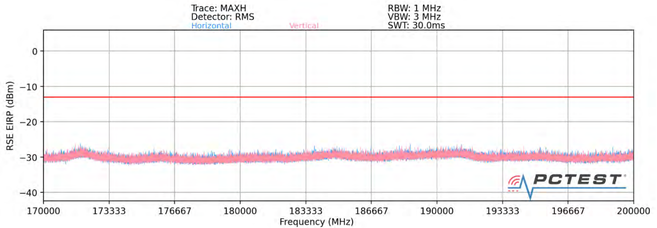
Plot 7-105. Ant1-n260 Radiated Spurious Plot (1CC QPSK Mid Channel H Beam – ENDC)
