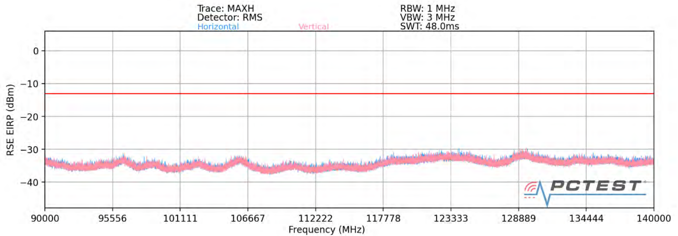
Plot 7-101. Ant1-n260 Radiated Spurious Plot (1CC QPSK Mid Channel H Beam – ENDC)
