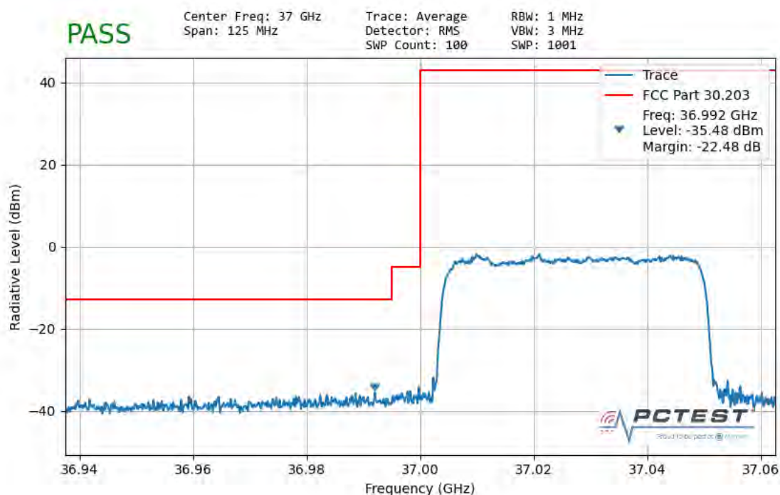
Plot 7-155. Ant1 Lower Band Edge (50MHz-1CC – QPSK Full RB)
