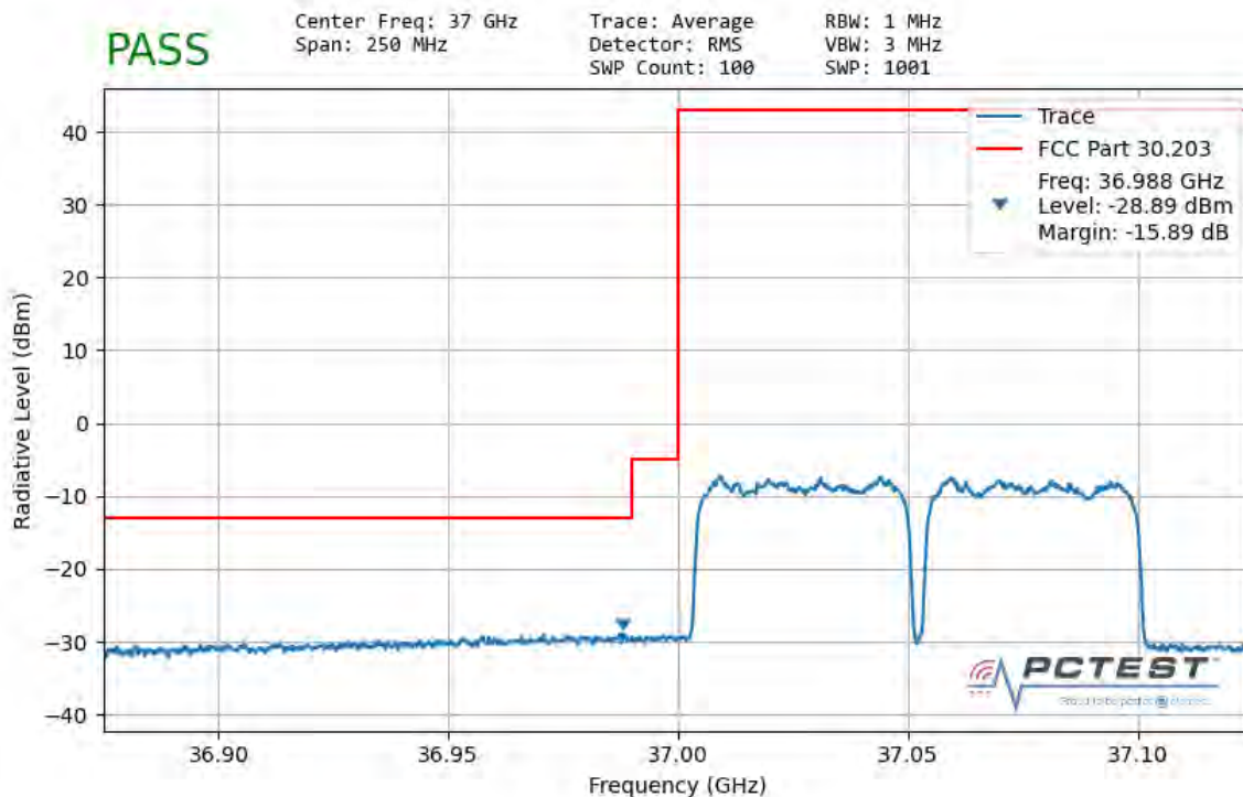
Plot 7-173. Ant2 Lower Band Edge (50MHz-2CC – QPSK Full RB)
