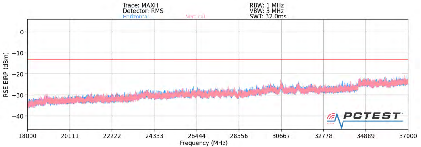
Plot 7-111. Ant2-n260 Radiated Spurious Plot (1CC QPSK Mid Channel H Beam – ENDC)
