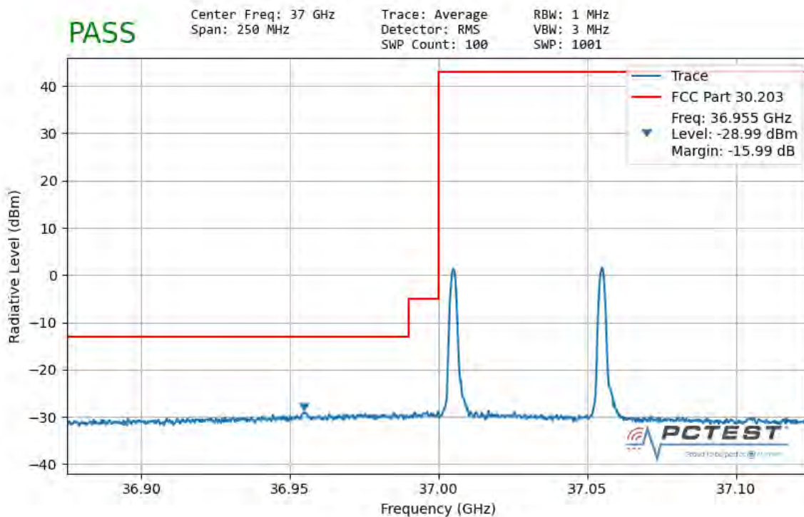
Plot 7-174. Ant2 Lower Band Edge (50MHz-2CC – QPSK 1 RB)
