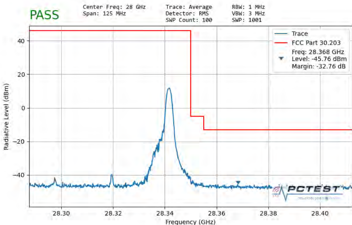
Plot 7-128. Ant1 Upper Band Edge (50MHz-1CC – QPSK 1 RB)
