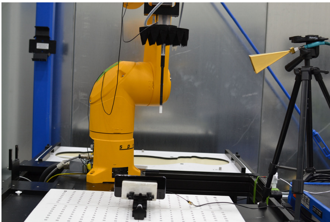
Test Setup Photo 7 – Power Density Setup (Figure 7-2)
