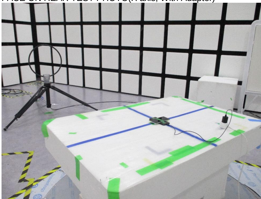
FACE ON REAR TEST PHOTO(X axis, With Adapter)
