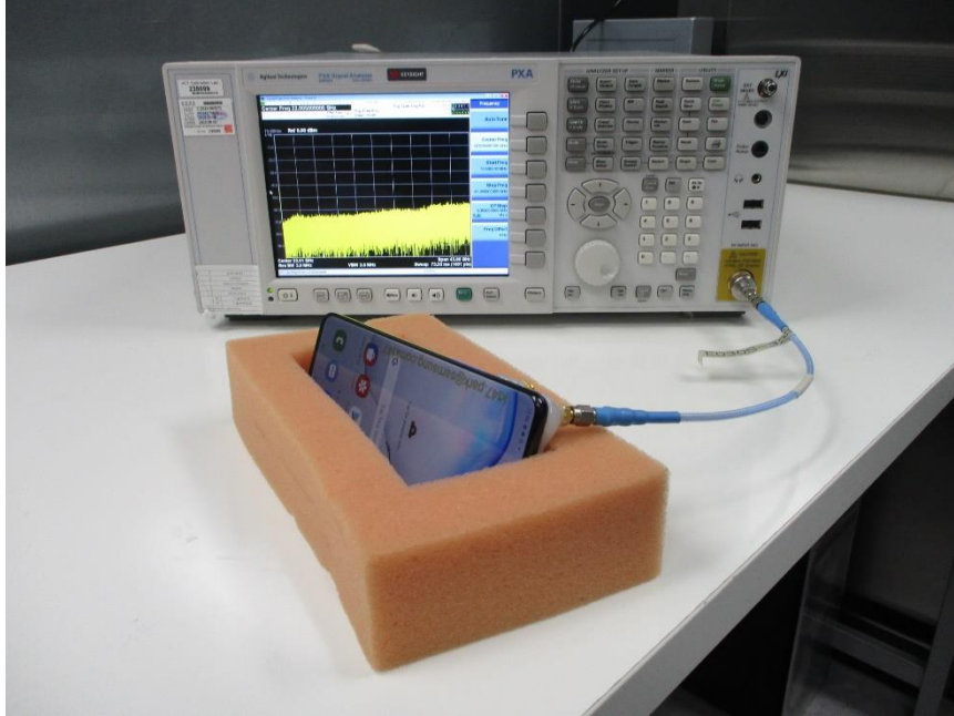
CONDUCTED TEST PHOTO
