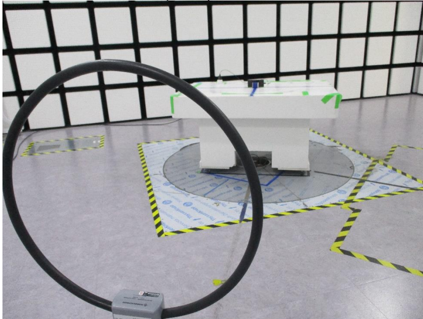
FACE ON TEST PHOTO(Y axis)
