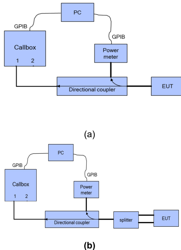
Figure 6-1 Conducted power measurement setup
