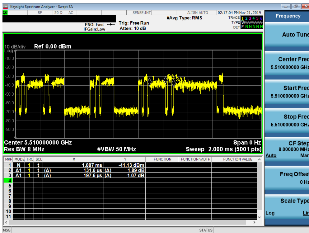
Figure 9-1. Band 2C Pulse Width & Period
