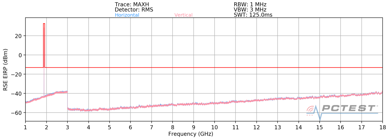
Plot 7-45. Radiated Spurious Plot above 1GHz (PCS GPRS Mode)
