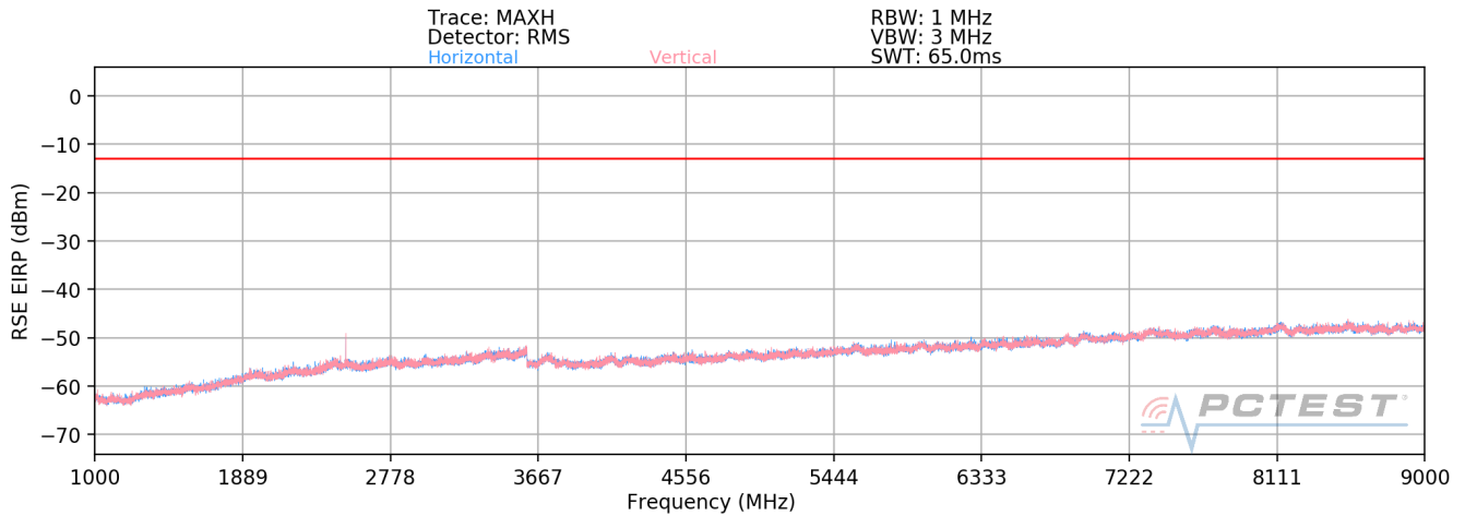
Plot 7-43. Radiated Spurious Plot above 1GHz (Cellular GPRS Mode)
