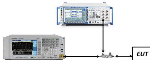
Figure 7-2. Test Instrument & Measurement Setup
