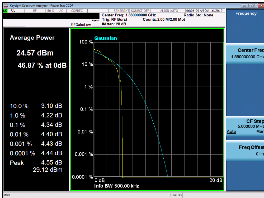
Plot 7-42. Peak-Average Ratio Plot (EDGE1900 Mode)
