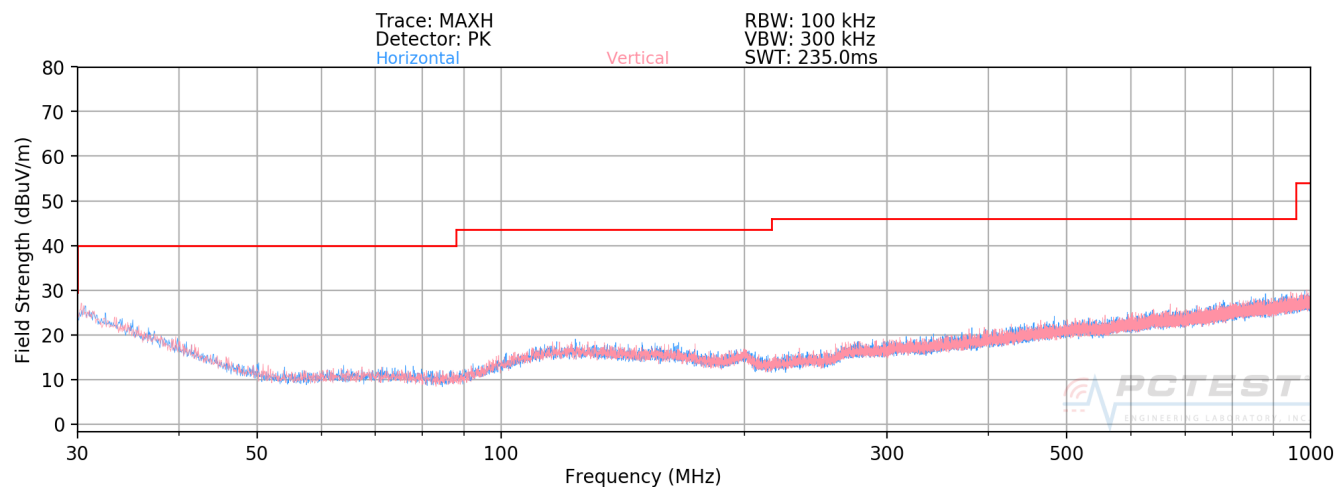
Plot 7-50. Radiated Spurious Plot below 1GHz
