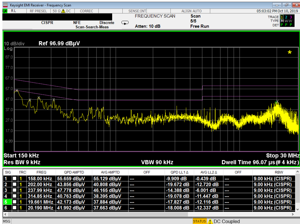
Plot 7-5. Line-Conducted Test Plot (N) - Device to Device WPT
