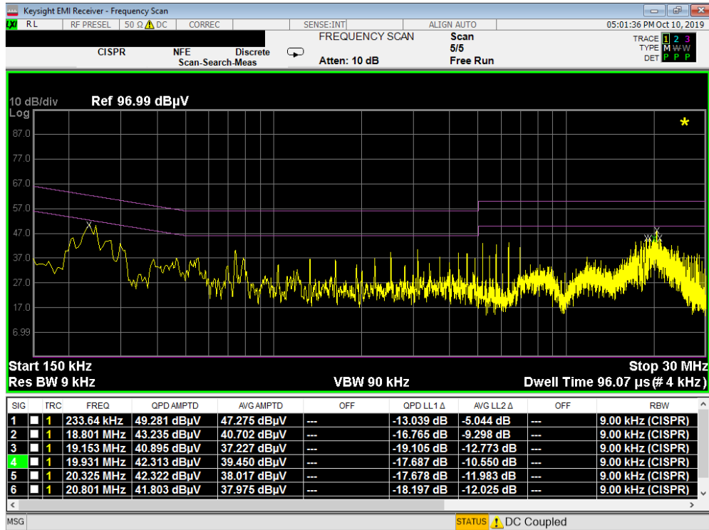
Plot 7-4. Line-Conducted Test Plot (L1) - Device to Device WPT
