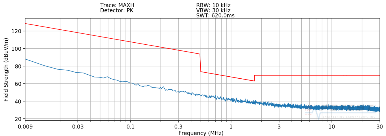
Plot 7-2 Radiated Spurious Plot 9kHz – 30MHz (Pol. Y – Device to Device WPT)
