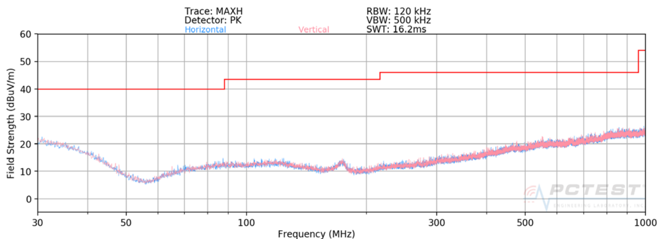
Plot 7-1. Radiated Spurious Plot below 1GHz
