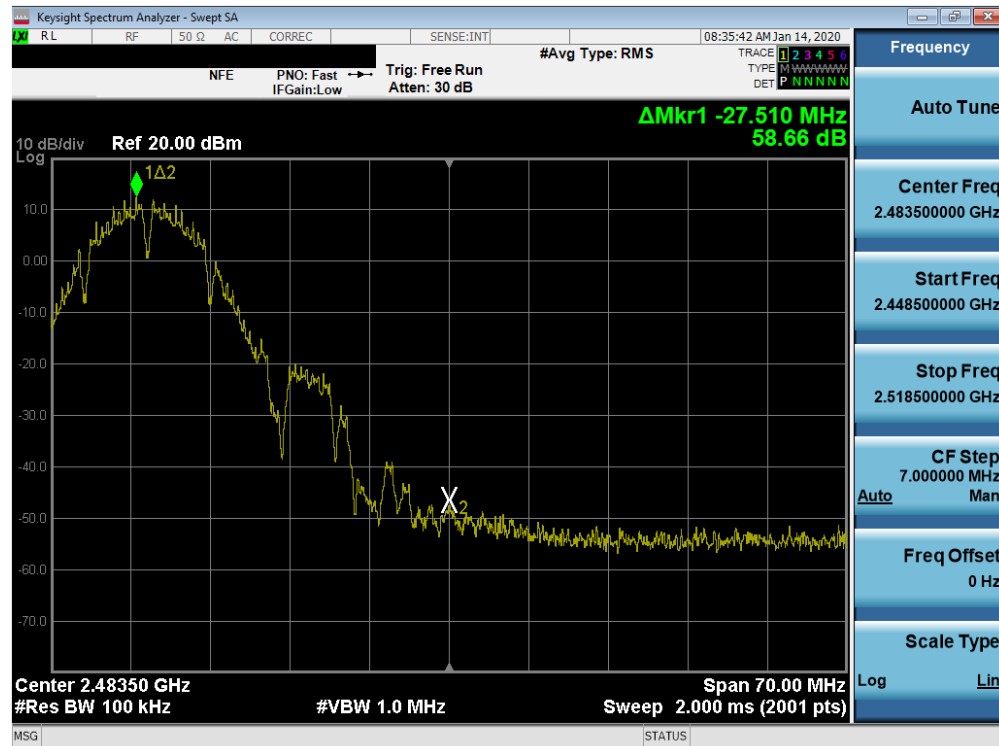
Plot 7-64. Band Edge Plot SISO ANT2 (802.11b – Ch. 10)
