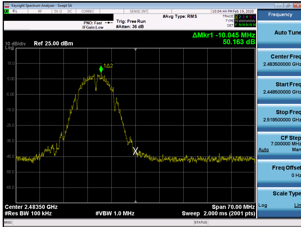
Plot 7-47. Band Edge Plot SISO ANT1 (802.11b – Ch. 13)
