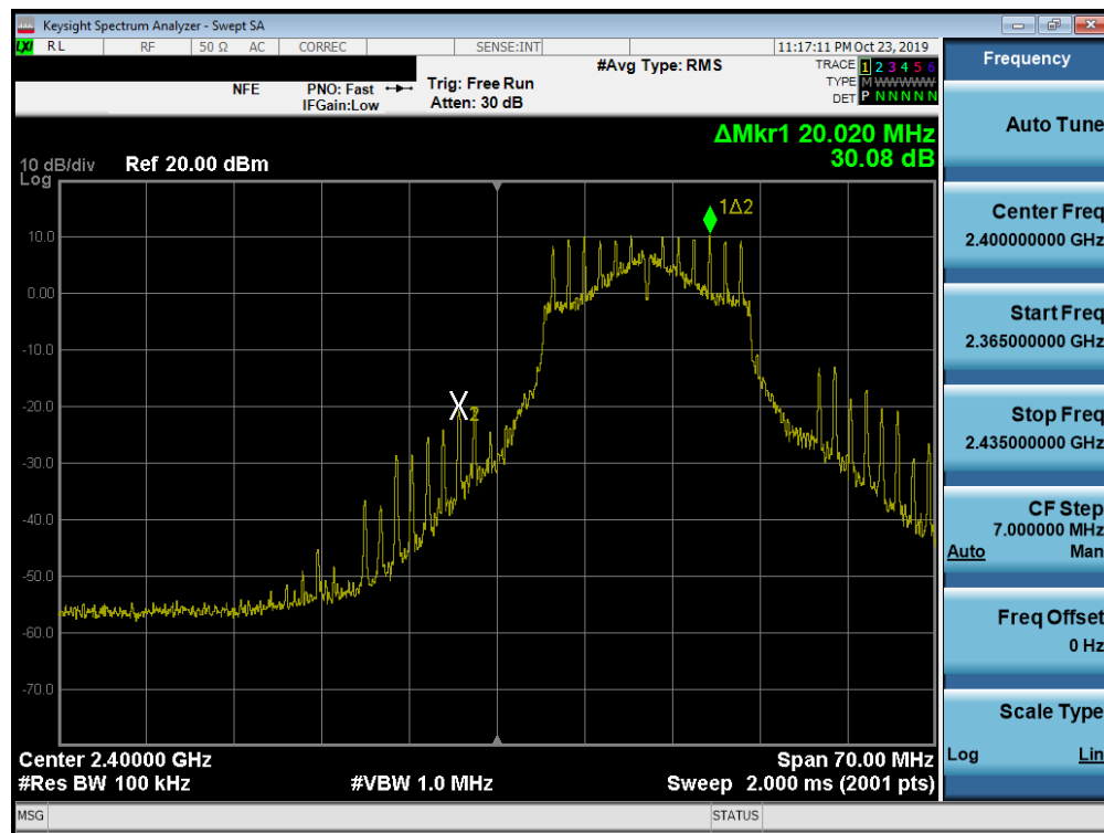
Plot 7-48. Band Edge Plot SISO ANT1 (802.11g- Ch. 1)
