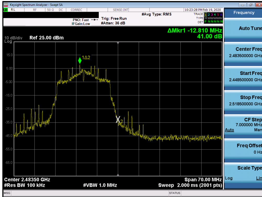
Plot 7-77. Band Edge Plot SISO ANT2 (802.11n - Ch. 13)
