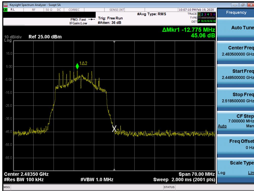
Plot 7-57. Band Edge Plot SISO ANT1 (802.11n (2.4GHz) – Ch. 13)
