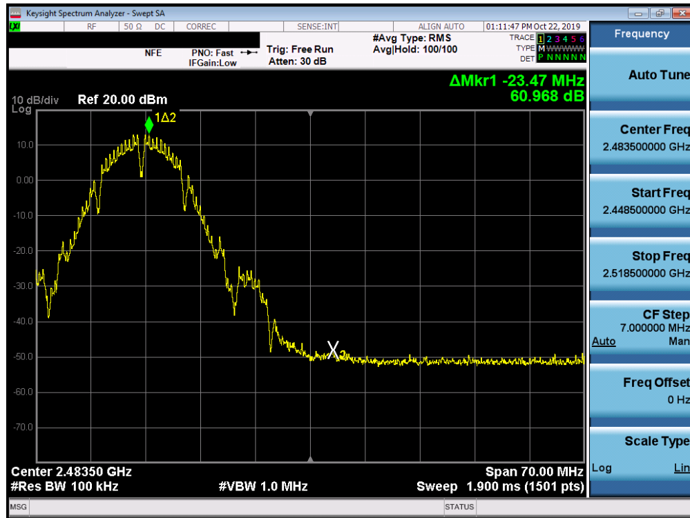
Plot 7-65. Band Edge Plot SISO ANT2 (802.11b – Ch. 11)
