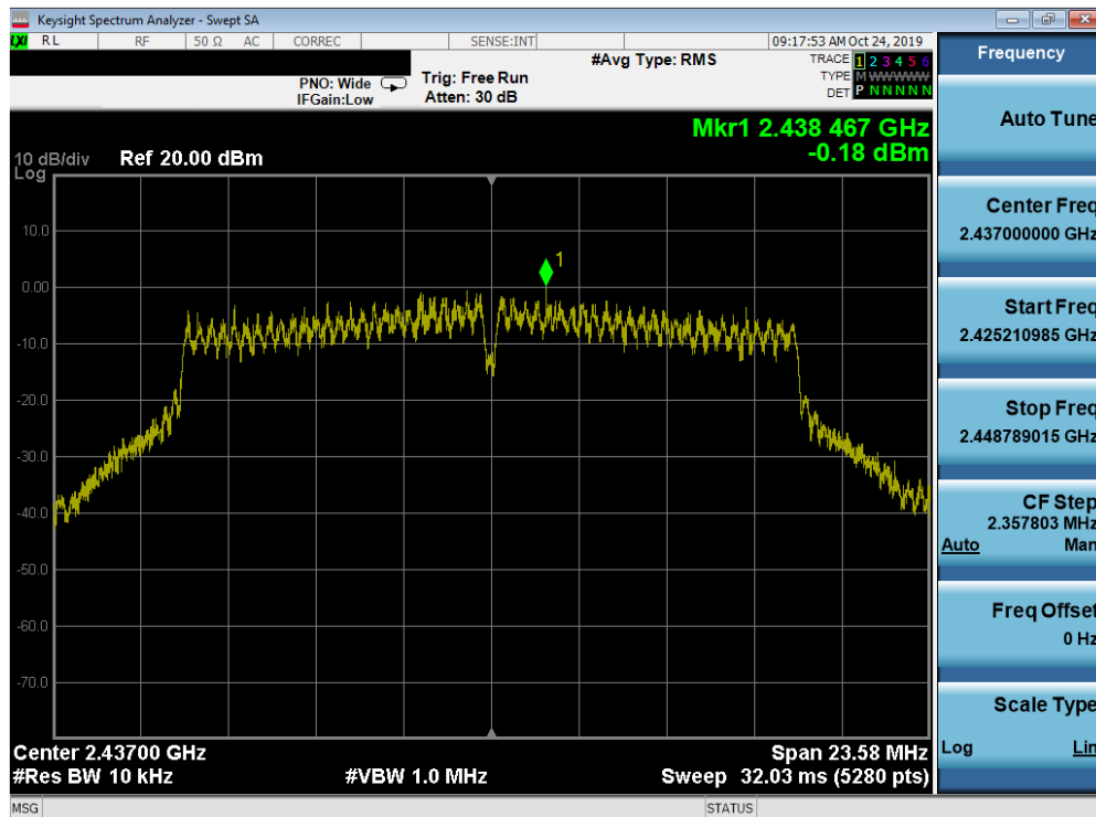
Plot 7-35. Power Spectral Density Plot SISO ANT2 (802.11g – Ch. 6)
