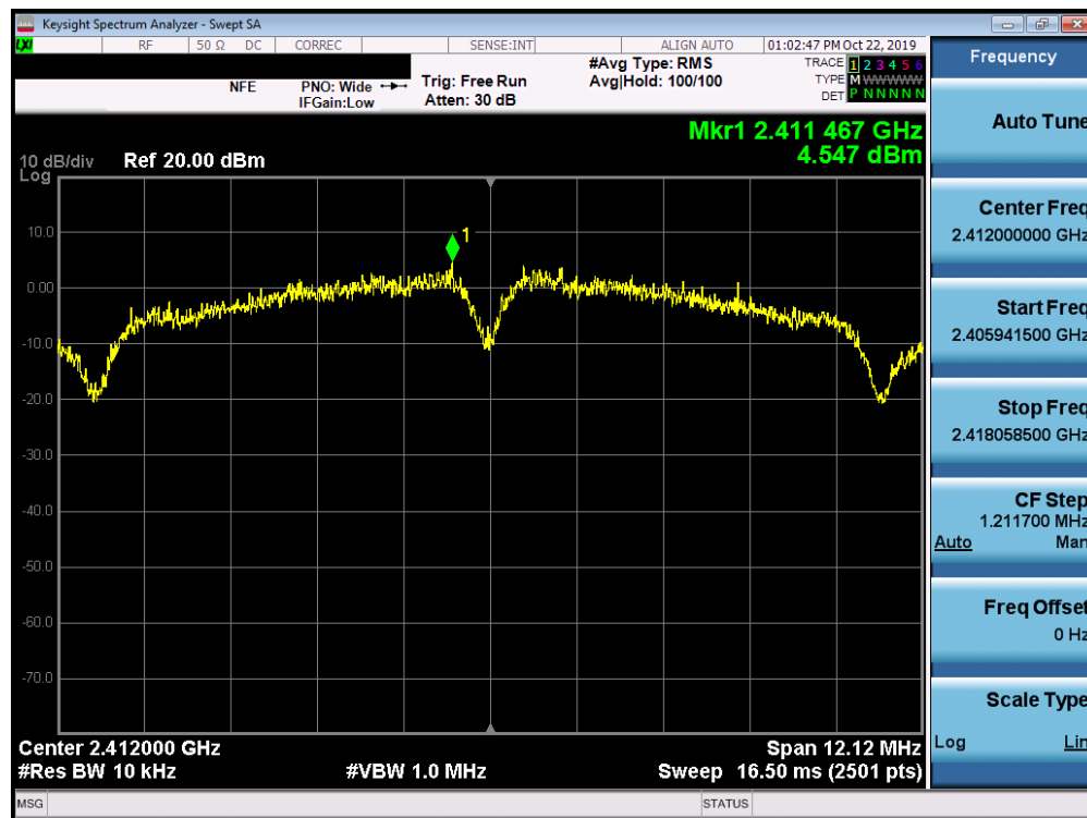
Plot 7-31. Power Spectral Density Plot SISO ANT2 (802.11b – Ch. 1)
