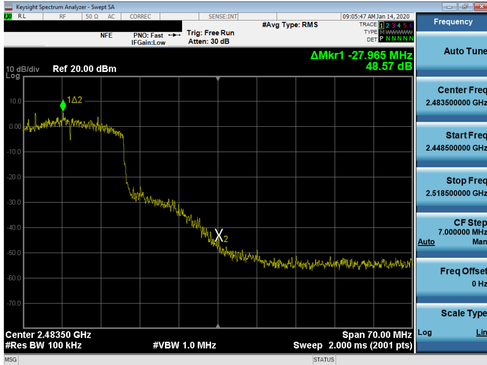
Plot 7-79. Band Edge Plot SISO ANT2 (802.11ax (2.4GHz) – Ch. 10)
