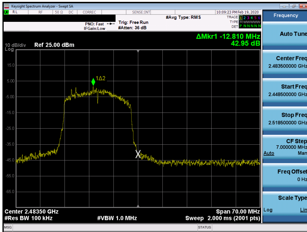
Plot 7-62. Band Edge Plot SISO ANT1 (802.11ax (2.4GHz) – Ch. 13)
