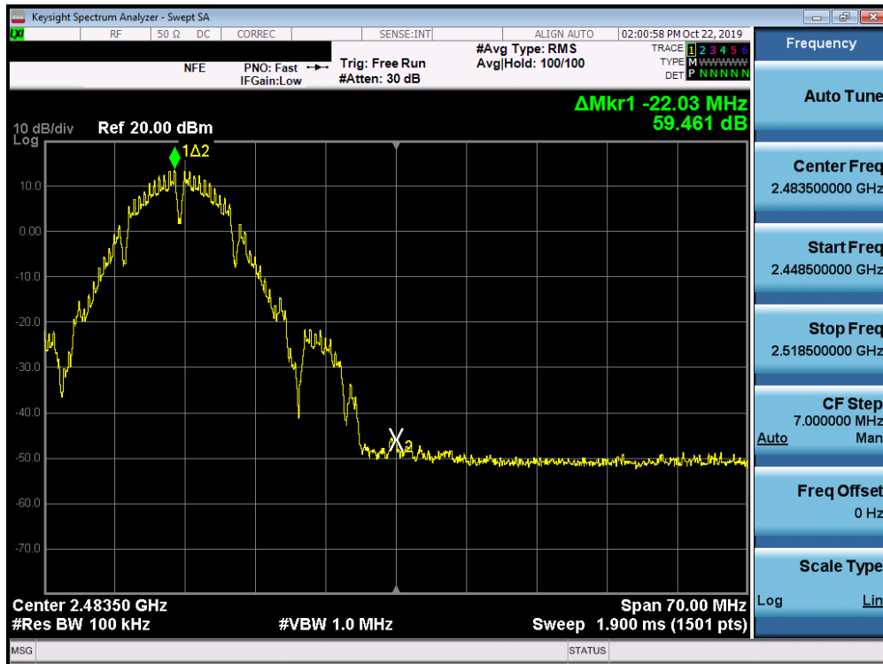
Plot 7-45. Band Edge Plot SISO ANT1 (802.11b – Ch. 11)
