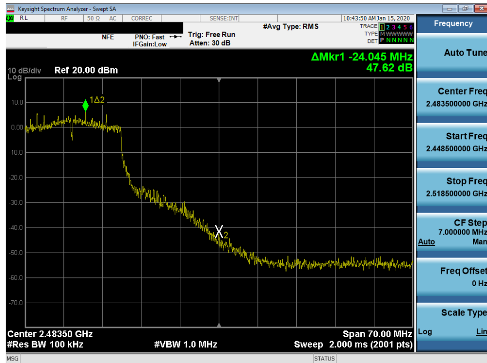
Plot 7-54. Band Edge Plot SISO ANT1 (802.11n (2.4GHz) – Ch. 11)
