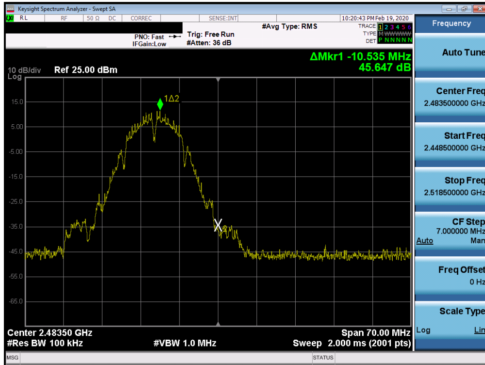
Plot 7-67. Band Edge Plot SISO ANT2 (802.11b – Ch. 13)
