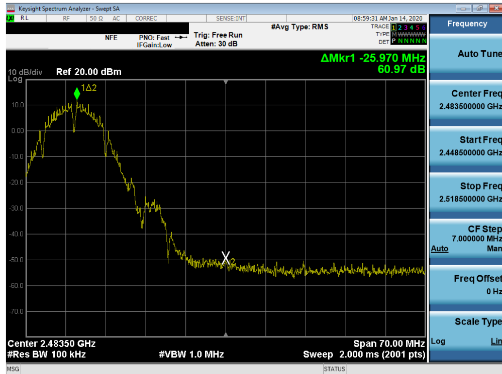
Plot 7-44. Band Edge Plot SISO ANT1 (802.11b – Ch. 10)
