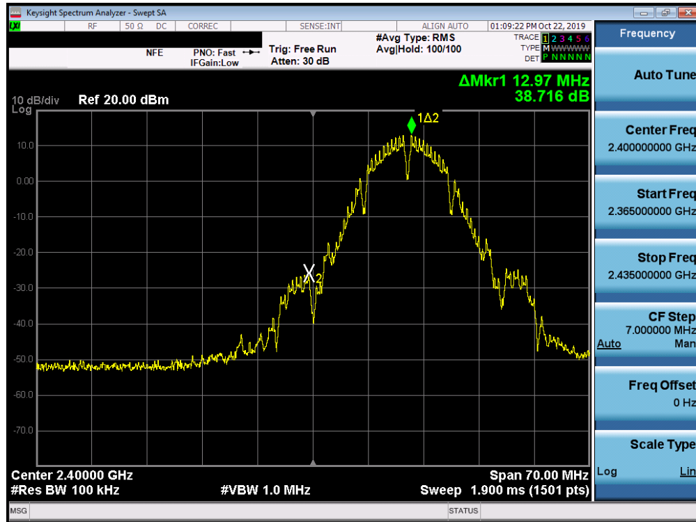
Plot 7-63. Band Edge Plot SISO ANT2 (802.11b – Ch. 1)
