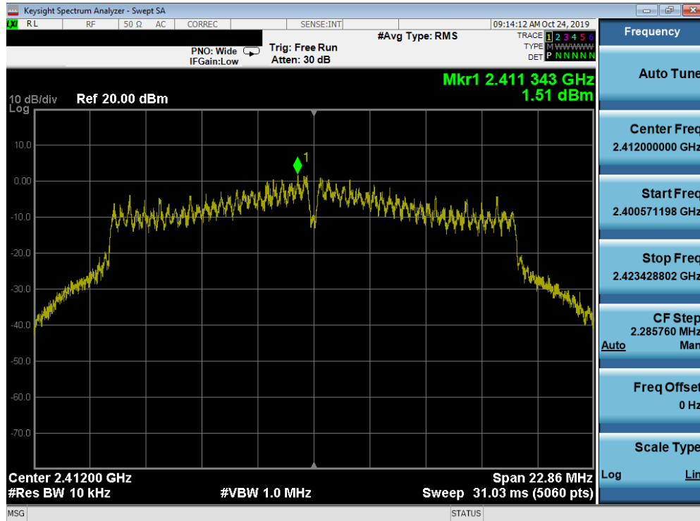
Plot 7-34. Power Spectral Density Plot SISO ANT2 (802.11g – Ch. 1)
