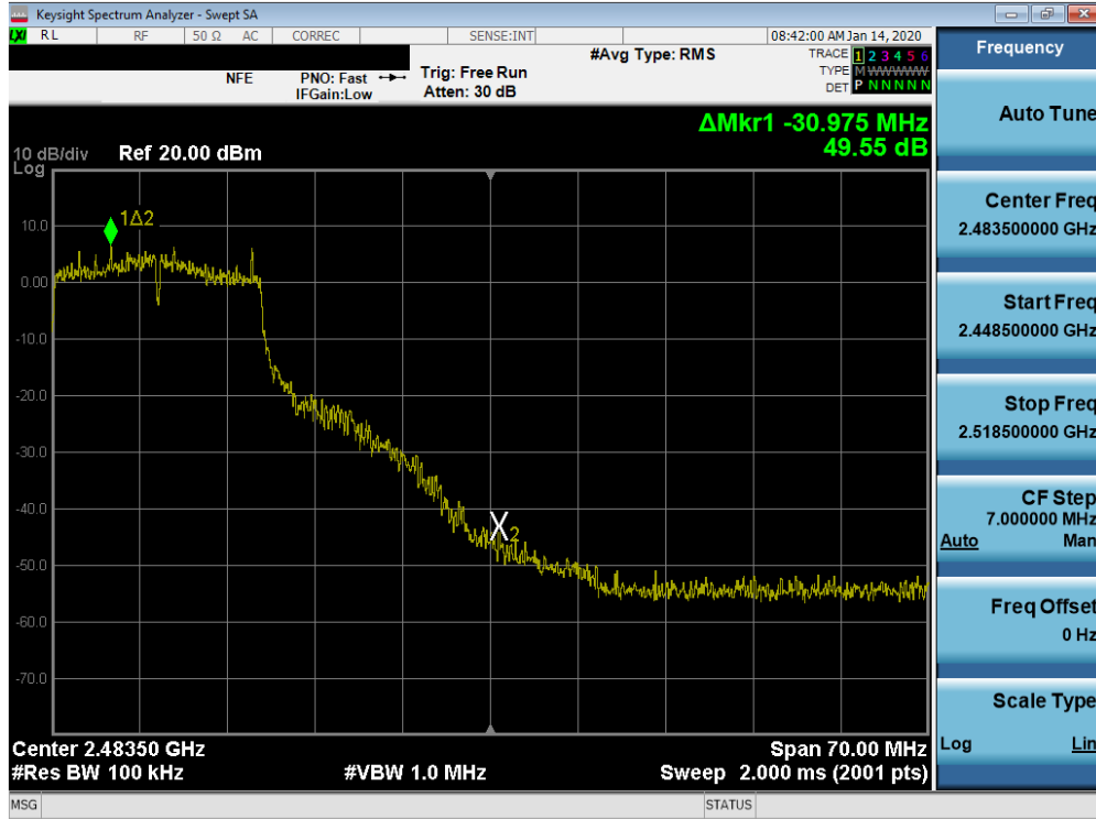
Plot 7-69. Band Edge Plot SISO ANT2 (802.11g – Ch. 11)
