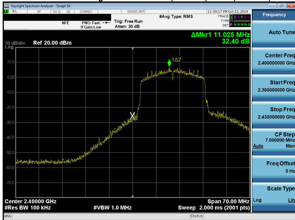
Plot 7-58. Band Edge Plot SISO ANT1 (802.11ax (2.4GHz) – Ch. 1)
