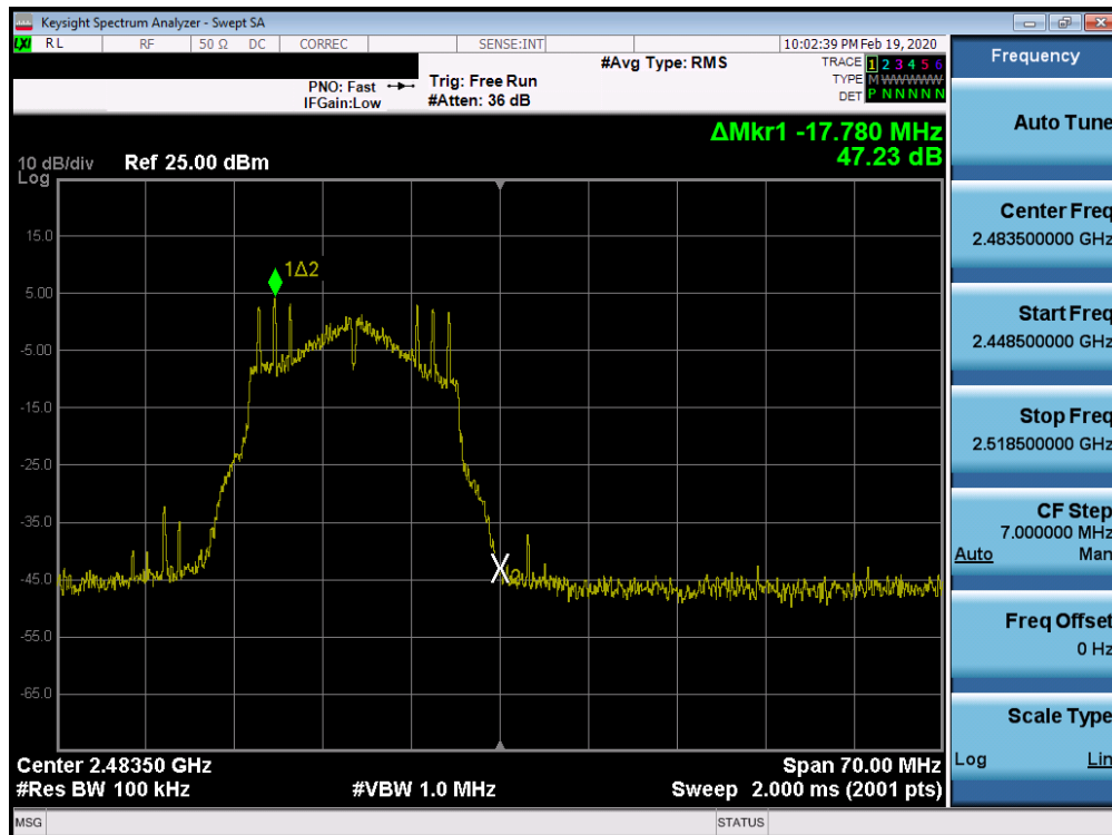
Plot 7-52. Band Edge Plot SISO ANT1 (802.11g – Ch. 13)
