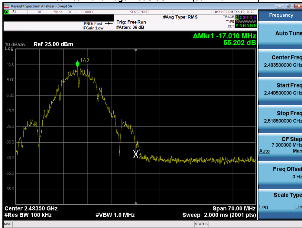
Plot 7-66. Band Edge Plot SISO ANT2 (802.11b – Ch. 12)
