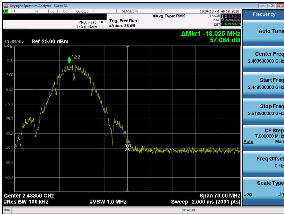
Plot 7-46. Band Edge Plot SISO ANT1 (802.11b – Ch. 12)
