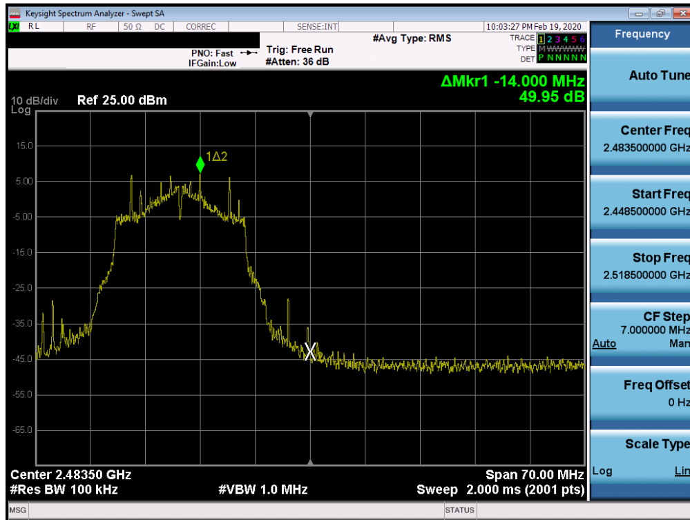
Plot 7-51. Band Edge Plot SISO ANT1 (802.11g – Ch. 12)
