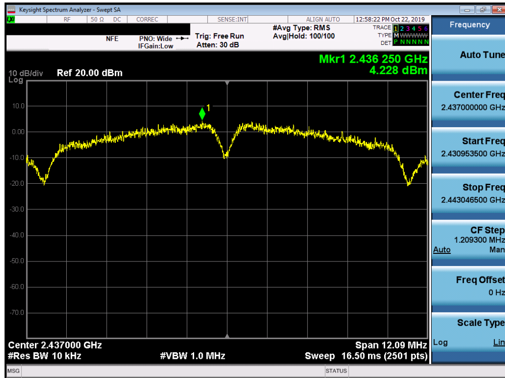
Plot 7-32. Power Spectral Density Plot SISO ANT2 (802.11b – Ch. 6)
