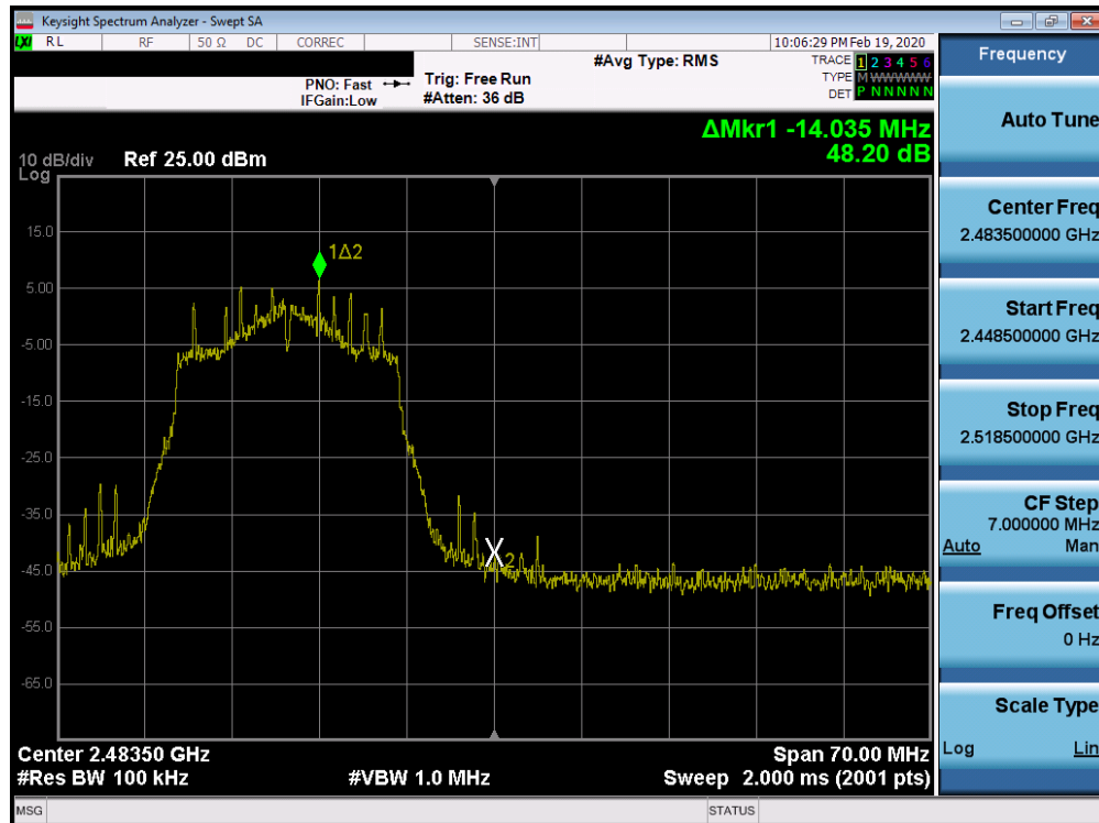
Plot 7-56. Band Edge Plot SISO ANT1 (802.11n (2.4GHz) – Ch. 12)
