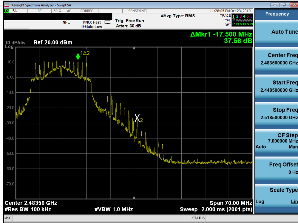
Plot 7-55. Band Edge Plot SISO ANT1 (802.11n (2.4GHz) – Ch. 11)
