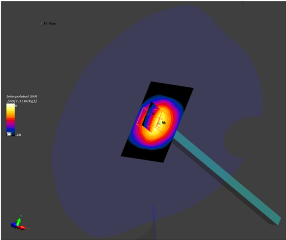
Figure C-3 SAR measurement system verification plot for 2450MHz performed on 12/2/2019. Input power = 10.0mW.
