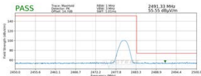
Plot 7-5. Radiated Restricted Upper Band Edge Measurement (Peak)
