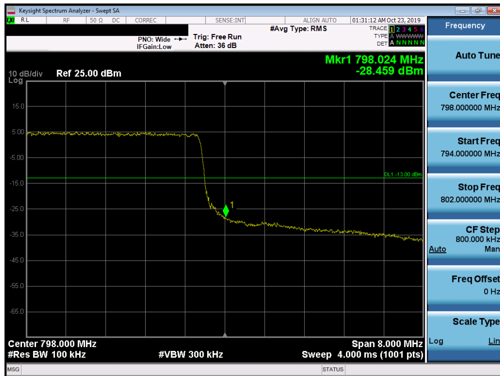
Plot 7-53. Upper Band Edge Plot (LTE Band 14, 10MHz QPSK - RB Size 50)
