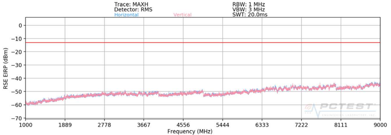
Plot 7-57. Radiated Spurious Plot (CDMA BC10)
