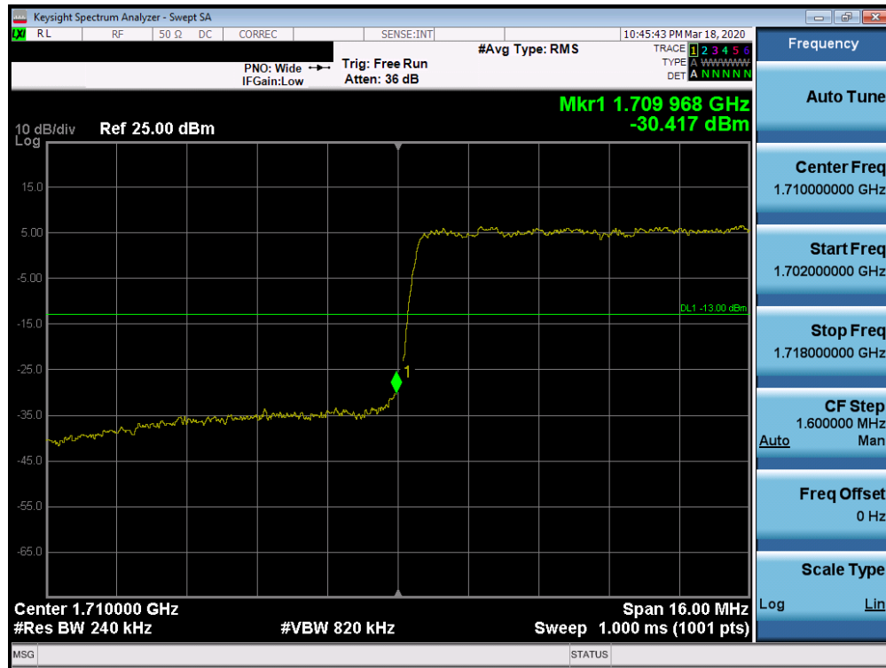
Plot 7-73. Lower Band Edge Plot (n66 - 20MHz DFT-s-OFDM-BPSK - Full RB Configuration)
