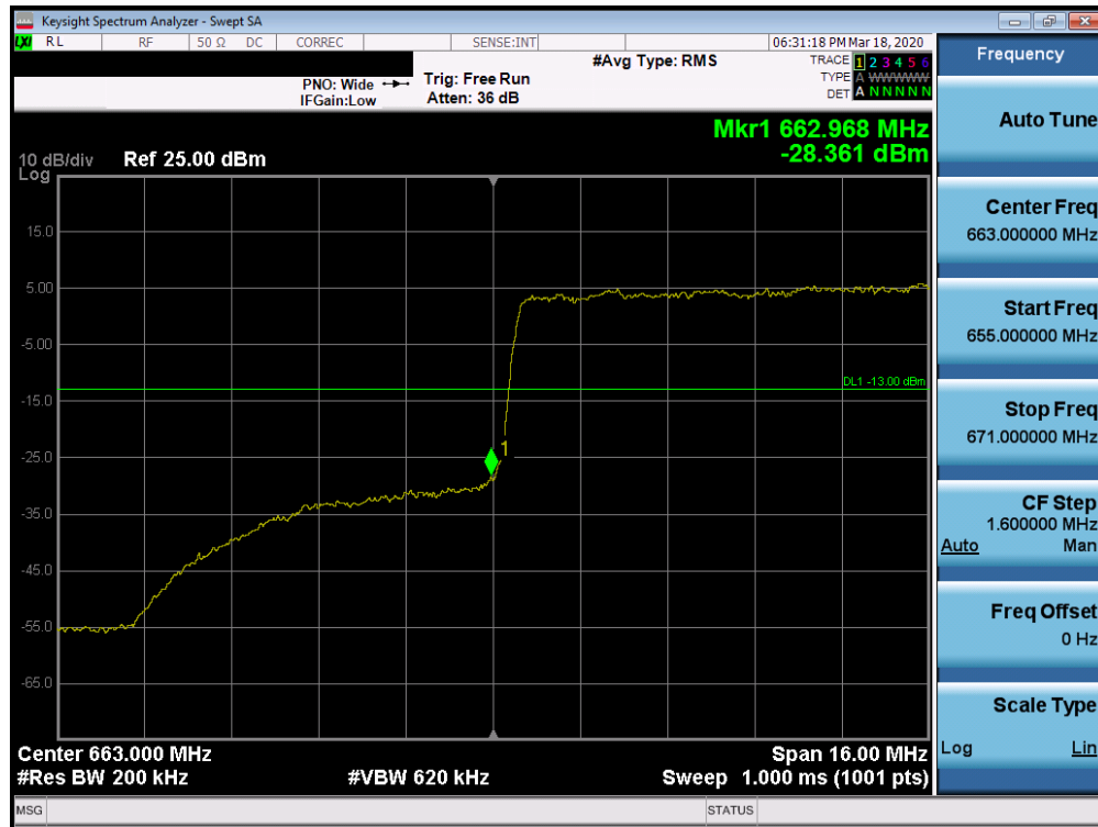
Plot 7-69. Lower Band Edge Plot (n71 - 20MHz DFT-s-OFDM-BPSK - Full RB Configuration)
