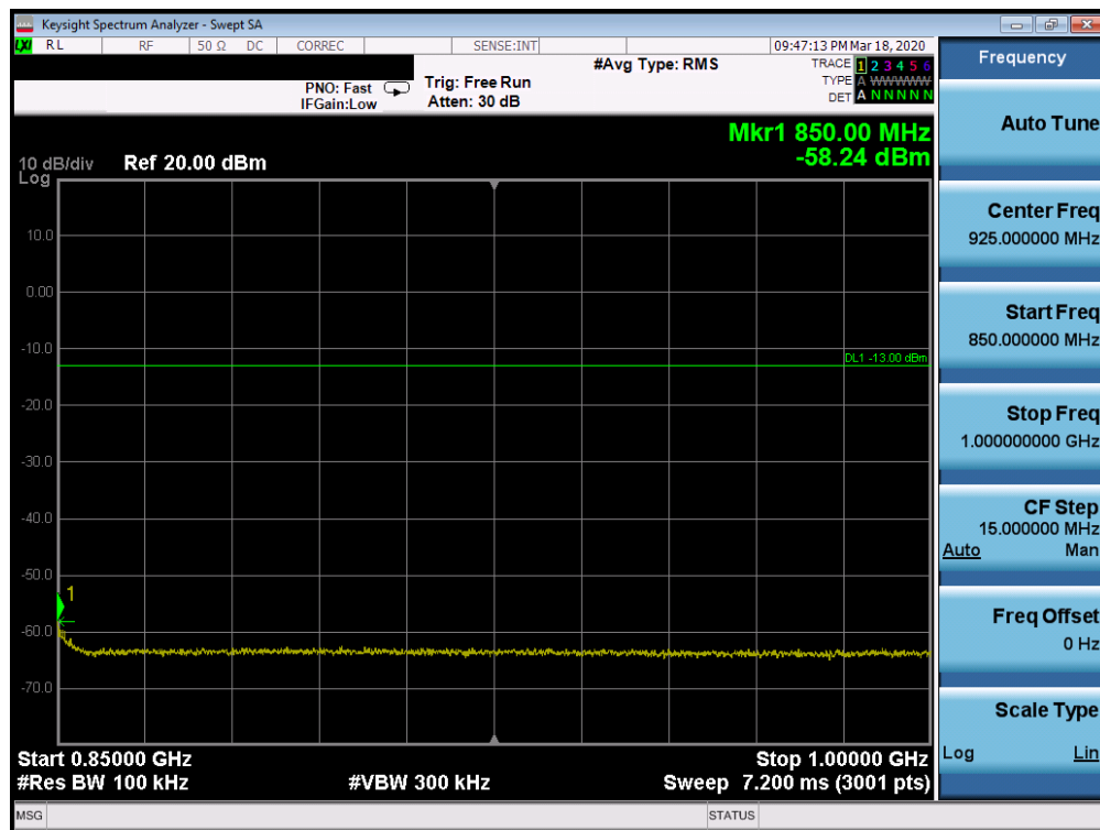
Plot 7-40. Conducted Spurious Plot (n5 - 20MHz DFT-s-OFDM-BPSK - RB Size 1, RB Offset 1 - High Channel)
