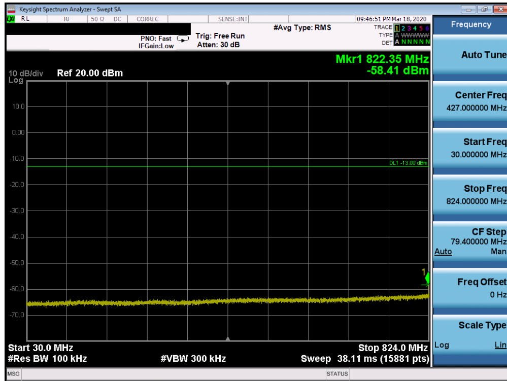
Plot 7-39. Conducted Spurious Plot (n5 - 20MHz DFT-s-OFDM-BPSK - RB Size 1, RB Offset 1 - High Channel)
