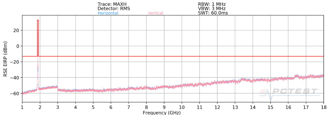
Plot 7-91. Radiated Spurious Plot above 1GHz (EN-DC n2+LTE B13)
