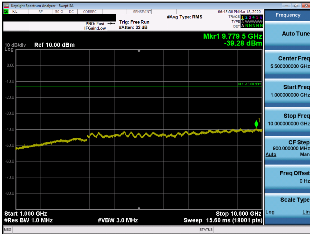
Plot 7-26. Conducted Spurious Plot (n71 - 20MHz DFT-s-OFDM-BPSK - RB Size 1, RB Offset 1 - Low Channel)
