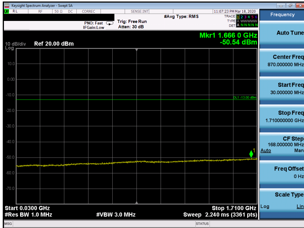
Plot 7-48. Conducted Spurious Plot (n66 - 20MHz DFT-s-OFDM-BPSK - RB Size 1, RB Offset 1 - High Channel)
