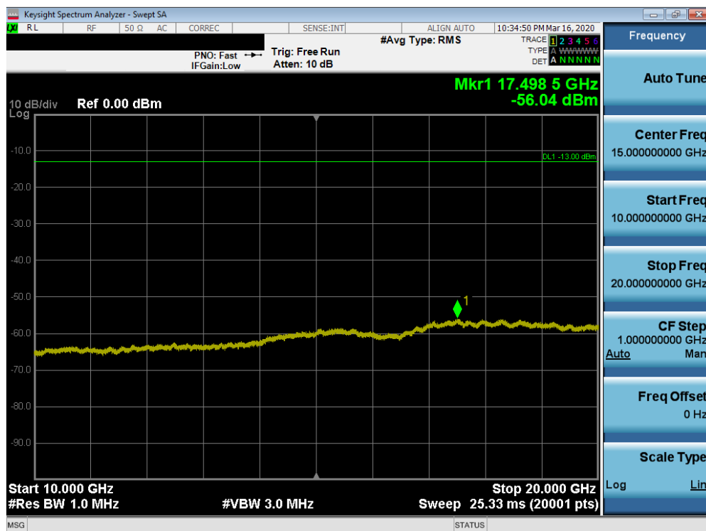
Plot 7-59. Conducted Spurious Plot (n2 - 20MHz DFT-s-OFDM-BPSK - RB Size 1, RB Offset 1 - High Channel)
