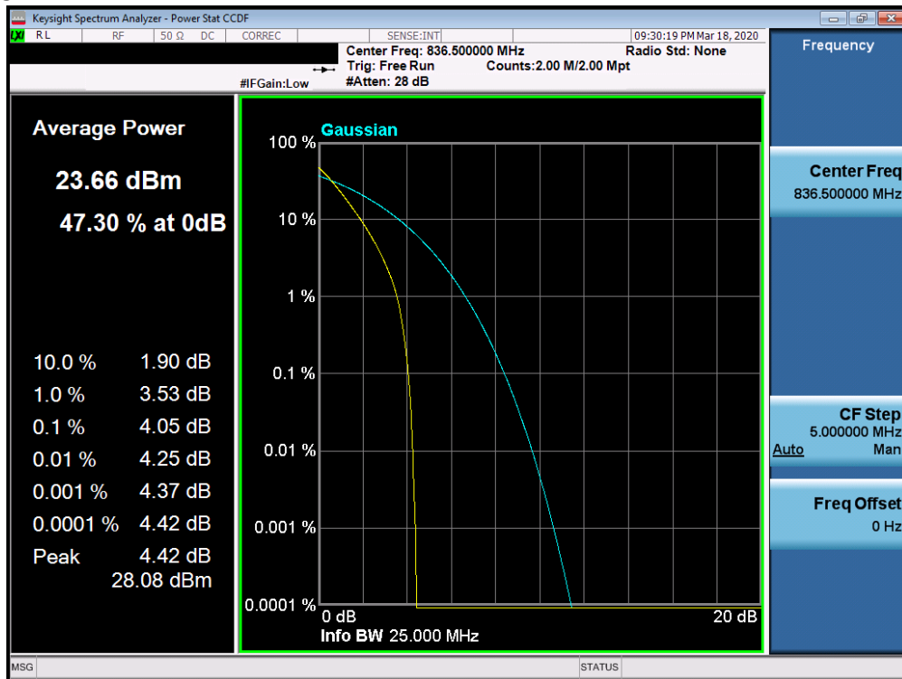
Plot 7-84. PAR Plot (Band n5 - 20.0MHz DFT-s-OFDM-BPSK - Full RB Configuration)
