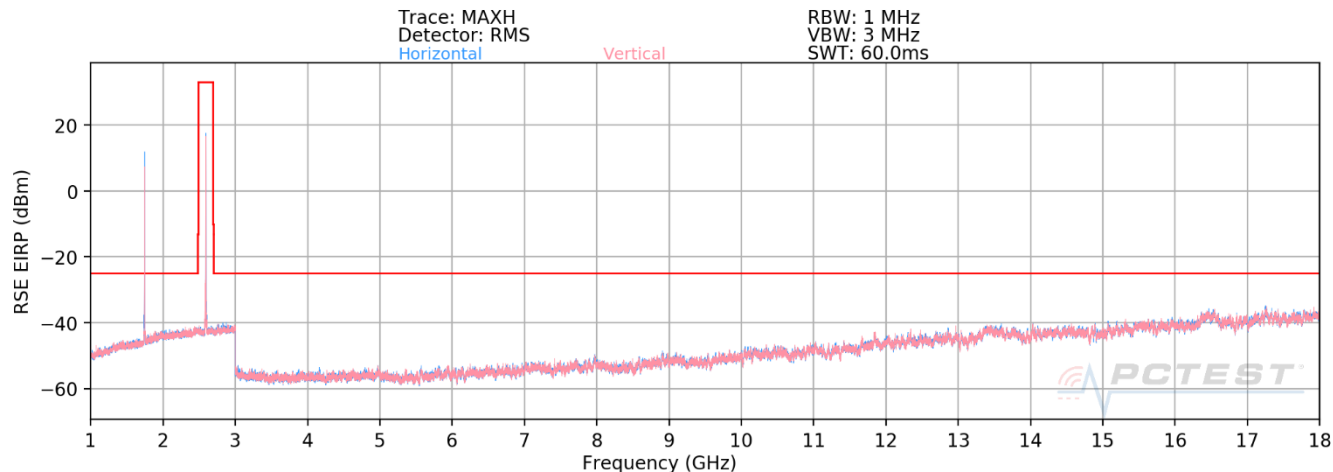
Plot 7-92. Radiated Spurious Plot 1GHz - 18GHz (EN-DC n41+ LTE B66)
