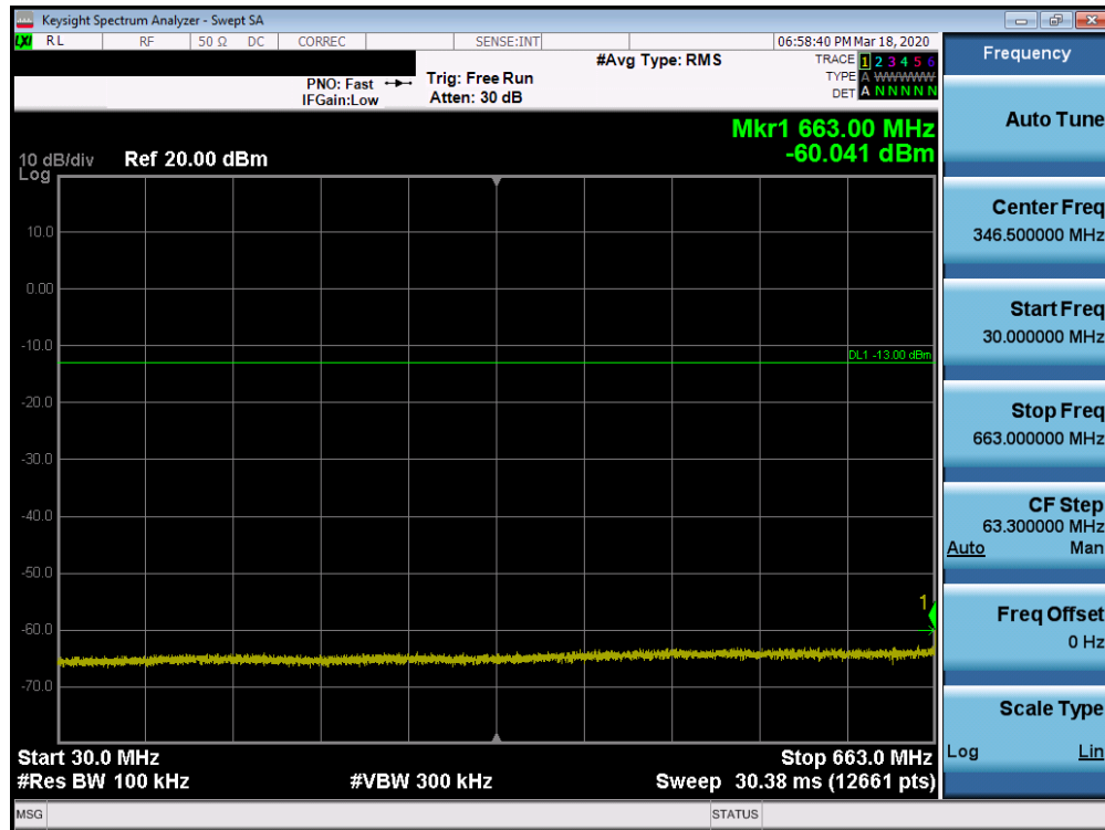
Plot 7-30. Conducted Spurious Plot (n71 - 20MHz DFT-s-OFDM-BPSK - RB Size 1, RB Offset 1 - High Channel)
