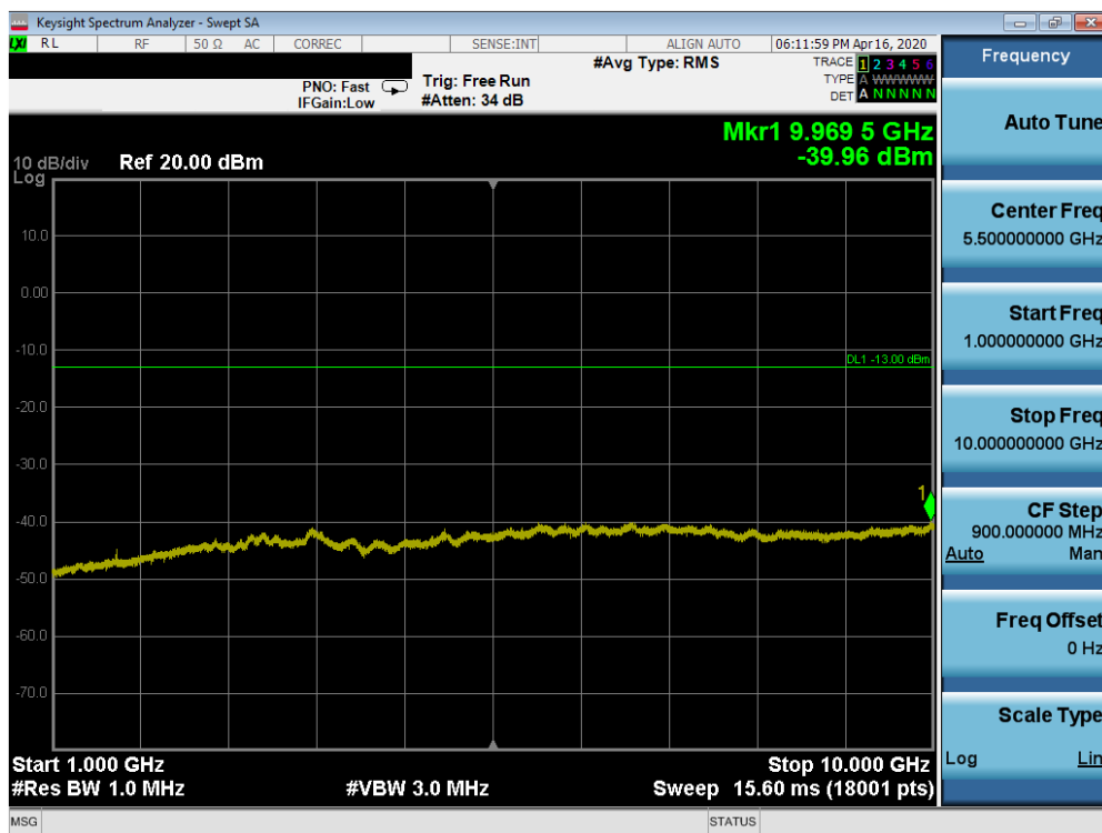
Plot 7-38. Conducted Spurious Plot (n5 - 20MHz DFT-s-OFDM-BPSK - RB Size 1, RB Offset 1 - Mid Channel)
