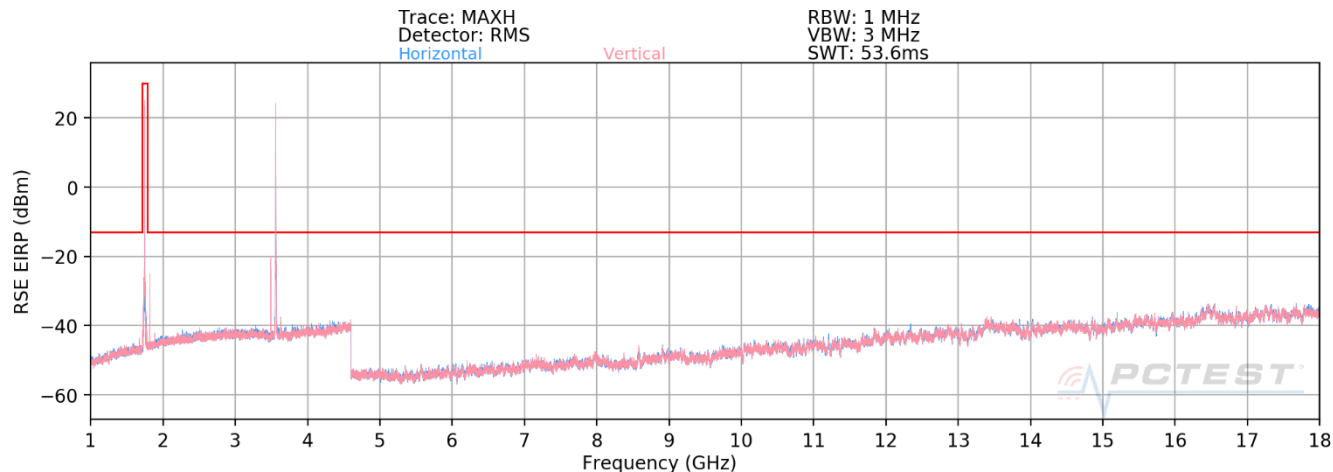
Plot 7-90. Radiated Spurious Plot above 1GHz (EN-DC n66+LTE B48)
