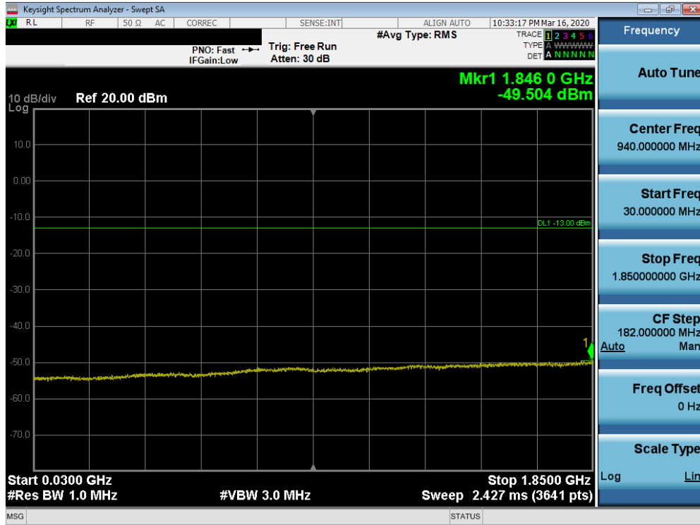
Plot 7-57. Conducted Spurious Plot (n2 - 20MHz DFT-s-OFDM-BPSK - RB Size 1, RB Offset 1 - High Channel)
