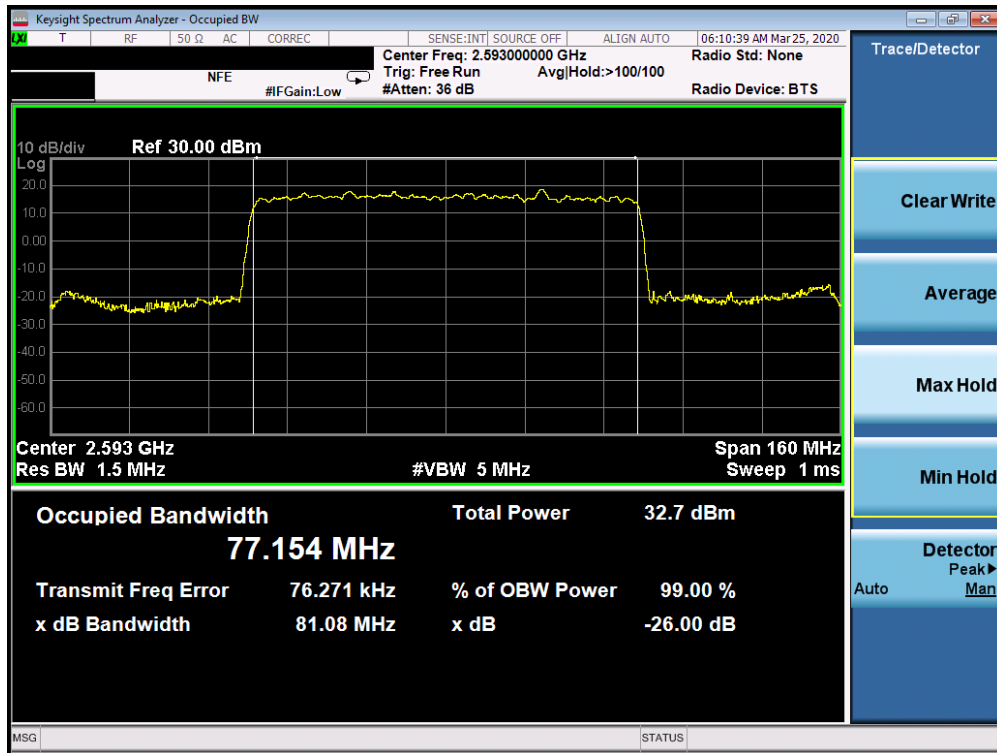
Plot 7-21. Occupied Bandwidth Plot (n41 80MHz DFT-s-OFDM-BPSK Full RB Configuration)
