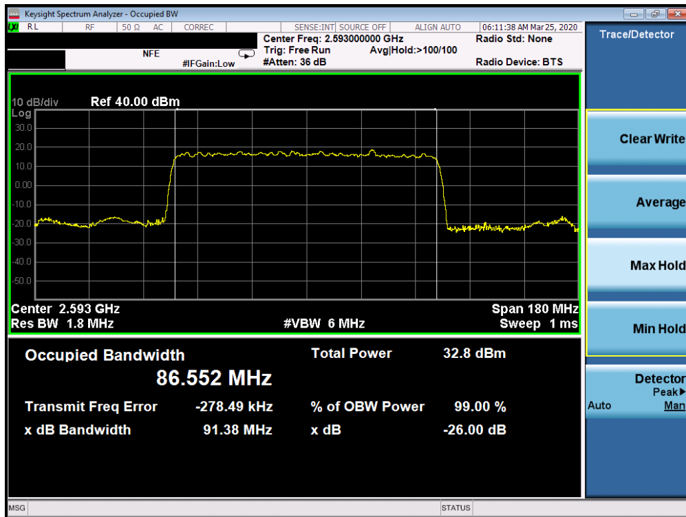
Plot 7-22. Occupied Bandwidth Plot (n41 90MHz DFT-s-OFDM-BPSK - Full RB Configuration)
