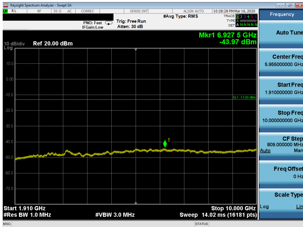
Plot 7-52. Conducted Spurious Plot (n2 - 20MHz DFT-s-OFDM-BPSK - RB Size 1, RB Offset 1 - Low Channel)
