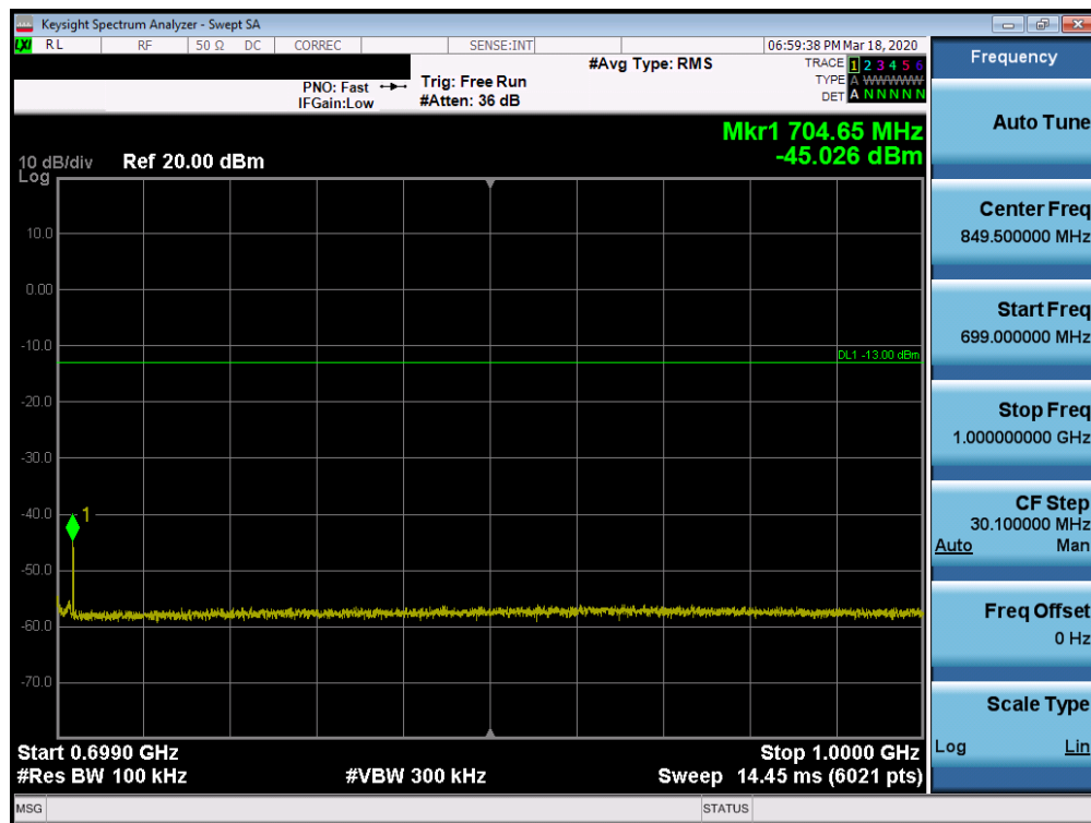
Plot 7-31. Conducted Spurious Plot (n71 - 20MHz DFT-s-OFDM-BPSK - RB Size 1, RB Offset 1 - High Channel)
