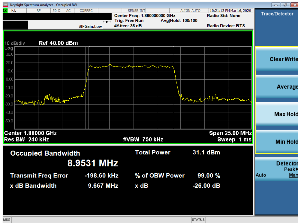
Plot 7-14. Occupied Bandwidth Plot (n2 10MHz DFT-s-OFDM-BPSK - Full RB Configuration)
