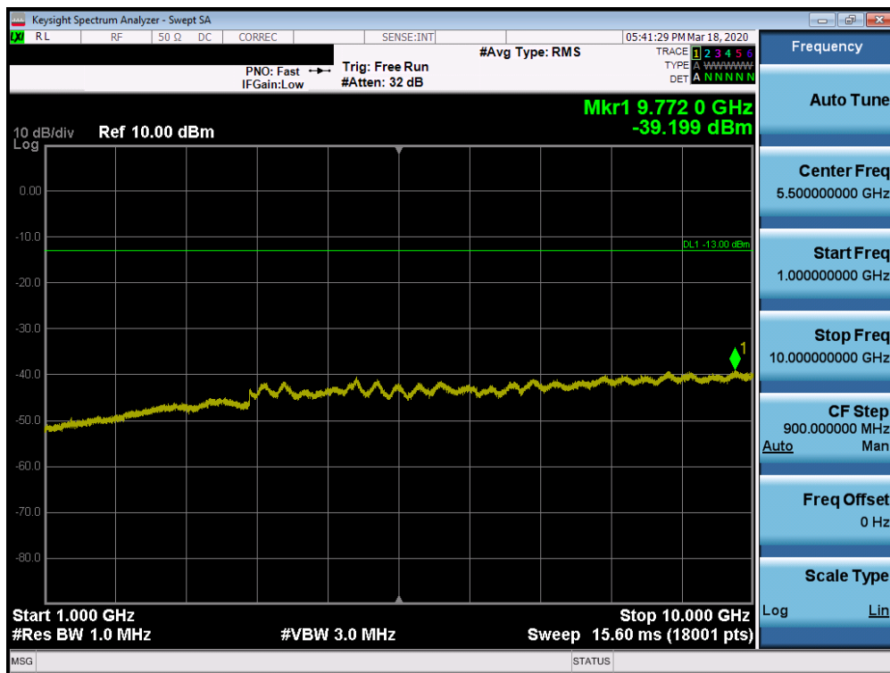
Plot 7-29. Conducted Spurious Plot (n71 - 20MHz DFT-s-OFDM-BPSK - RB Size 1, RB Offset 1 - Mid Channel)
