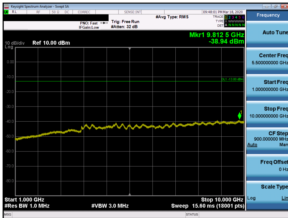
Plot 7-41. Conducted Spurious Plot (n5 - 20MHz DFT-s-OFDM-BPSK - RB Size 1, RB Offset 1 - High Channel)
