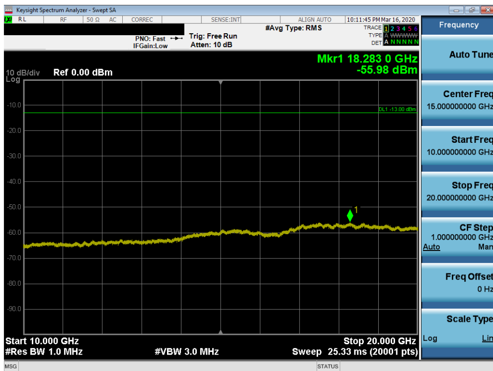
Plot 7-56. Conducted Spurious Plot (n2 - 20MHz DFT-s-OFDM-BPSK - RB Size 1, RB Offset 1 - Mid Channel)
