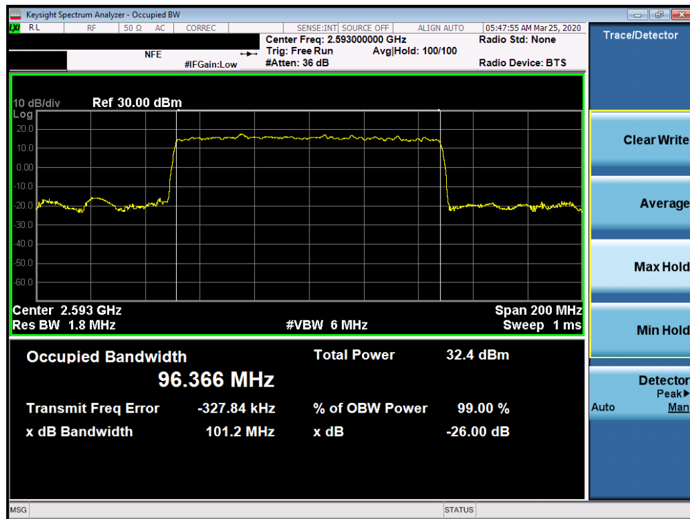
Plot 7-23. Occupied Bandwidth Plot (n41 100MHz DFT-s-OFDM-BPSK - Full RB Configuration)
