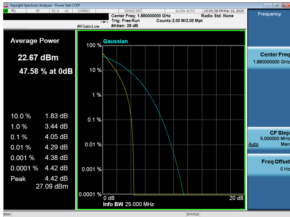
Plot 7-86. PAR Plot (Band n2 - 20.0MHz DFT-s-OFDM-BPSK - Full RB Configuration)
