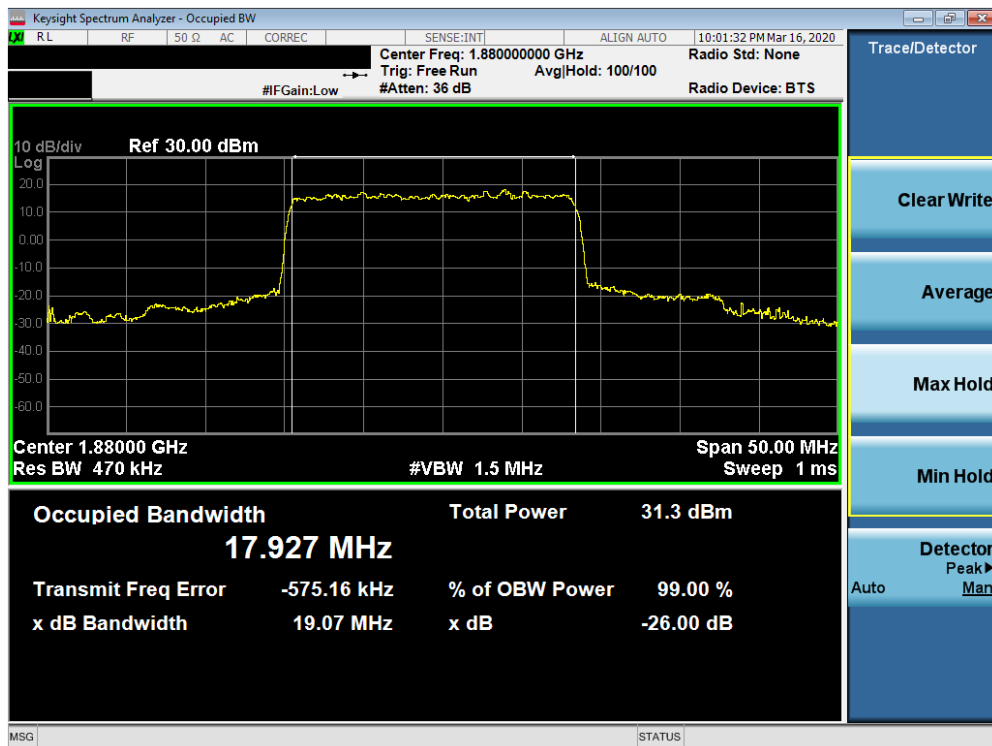
Plot 7-16. Occupied Bandwidth Plot (n2 20MHz DFT-s-OFDM-BPSK - Full RB Configuration)
