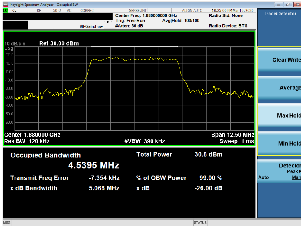
Plot 7-13. Occupied Bandwidth Plot (n2 5MHz DFT-s-OFDM-BPSK Full RB Configuration)
