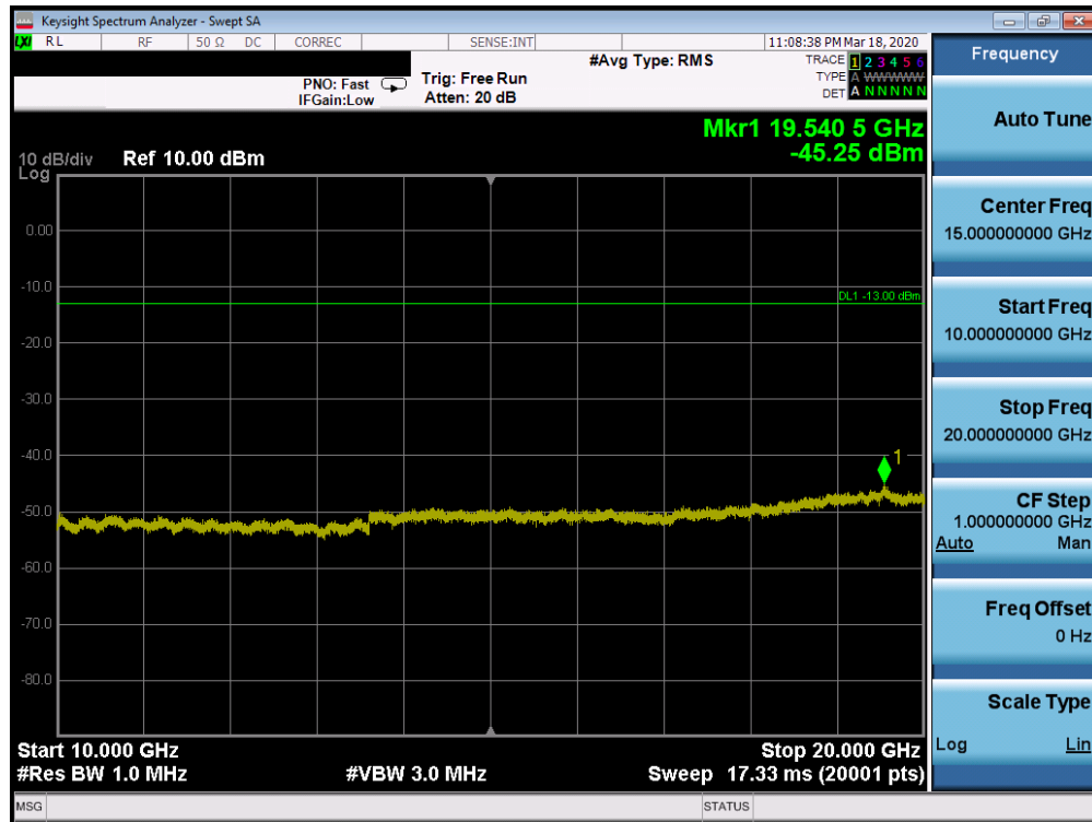
Plot 7-50. Conducted Spurious Plot (n66 - 20MHz DFT-s-OFDM-BPSK - RB Size 1, RB Offset 1 - High Channel)
