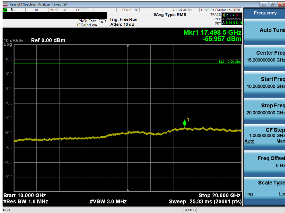
Plot 7-53. Conducted Spurious Plot (n2 - 20MHz DFT-s-OFDM-BPSK - RB Size 1, RB Offset 1 - Low Channel)
