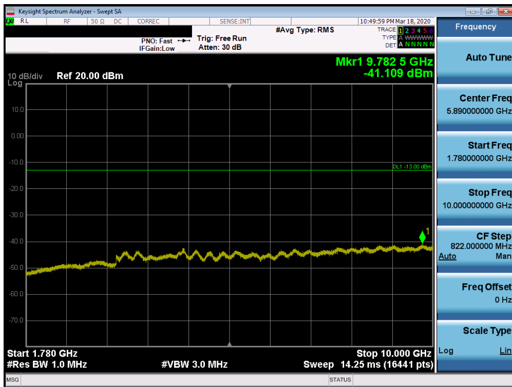
Plot 7-43. Conducted Spurious Plot (n66 - 20MHz DFT-s-OFDM-BPSK - RB Size 1, RB Offset 1 - Low Channel)
