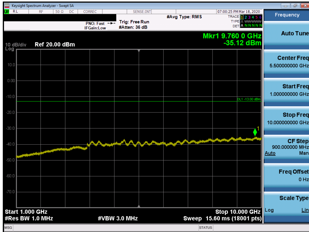
Plot 7-32. Conducted Spurious Plot (n71 - 20MHz DFT-s-OFDM-BPSK - RB Size 1, RB Offset 1 - High Channel)
