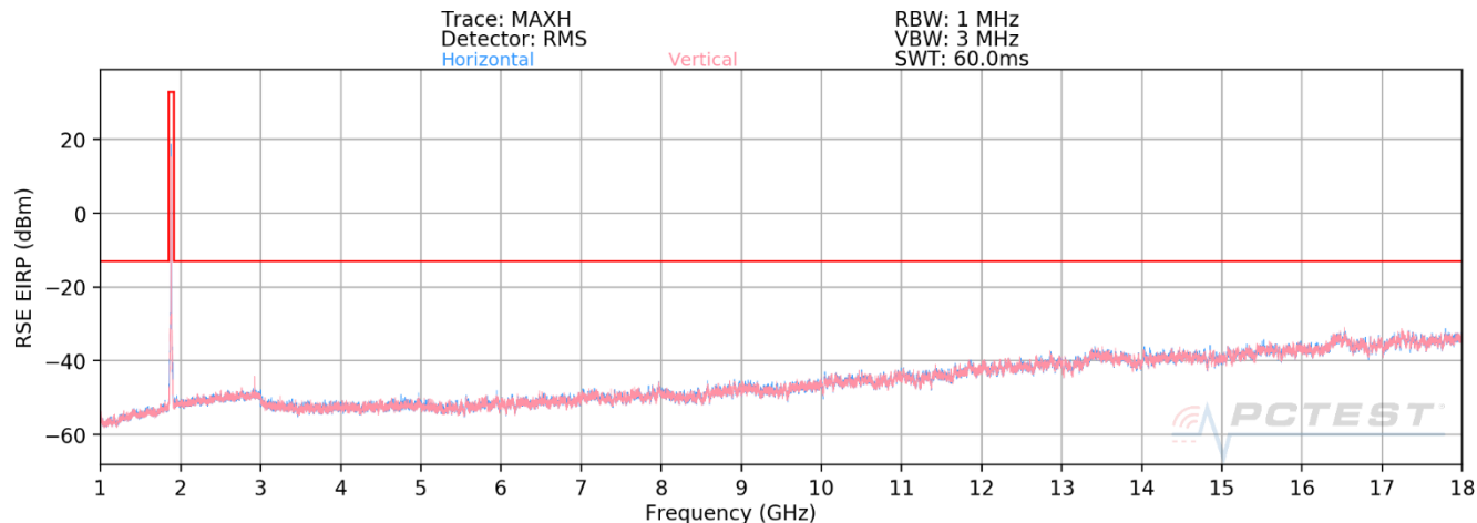
Plot 7-89. Radiated Spurious Plot above 1GHz (EN-DC n5+LTE B2)
