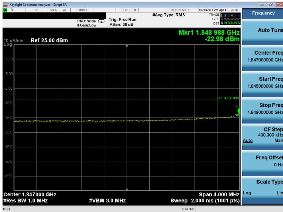
Plot 7-78. Lower Extended Band Edge Plot (n2 - 20MHz DFT-s-OFDM-BPSK - Full RB Configuration)
