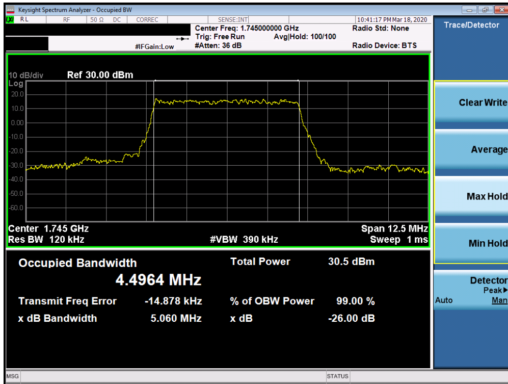
Plot 7-9. Occupied Bandwidth Plot (n66 5MHz DFT-s-OFDM-BPSK Full RB Configuration)
