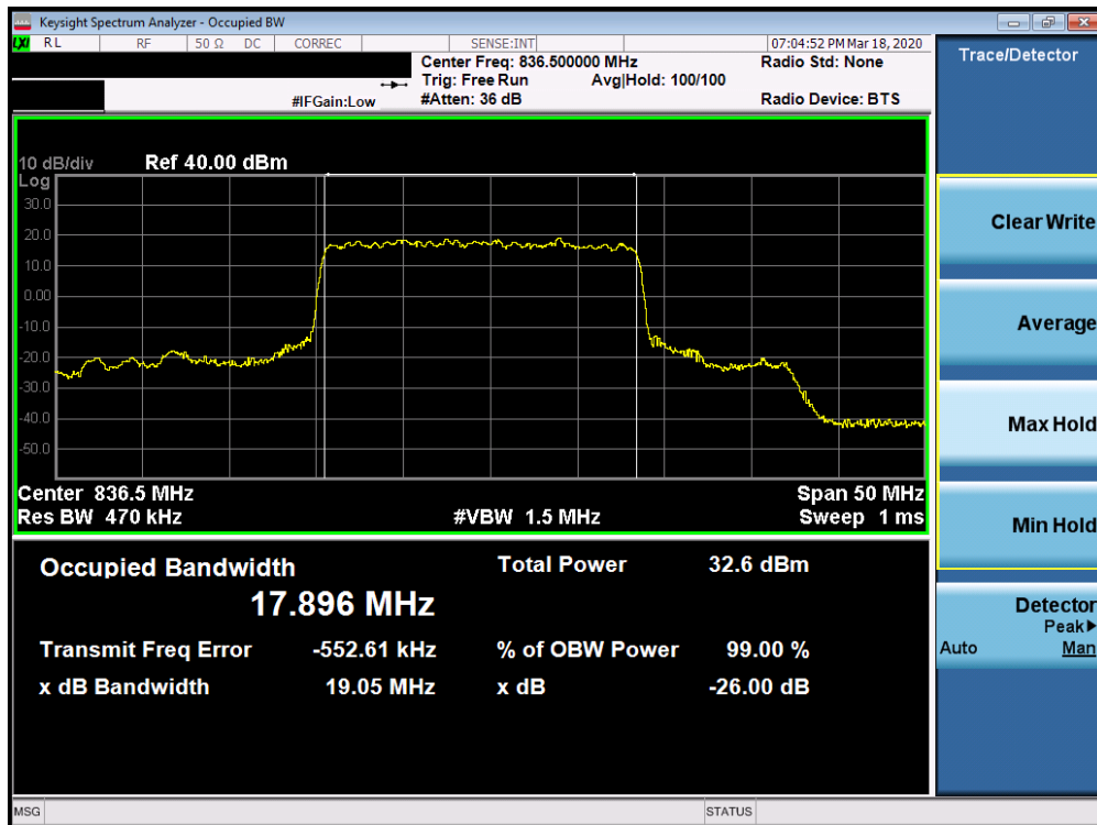
Plot 7-8. Occupied Bandwidth Plot (n5 20MHz DFT-s-OFDM-BPSK - Full RB Configuration)
