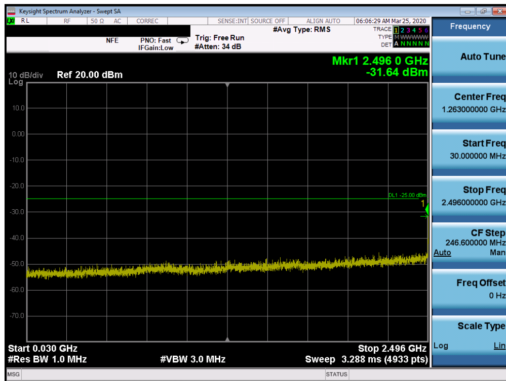
Plot 7-63. Conducted Spurious Plot (n41 - 100MHz DFT-s-OFDM-BPSK - RB Size 1, RB Offset 1 - Mid Channel)
