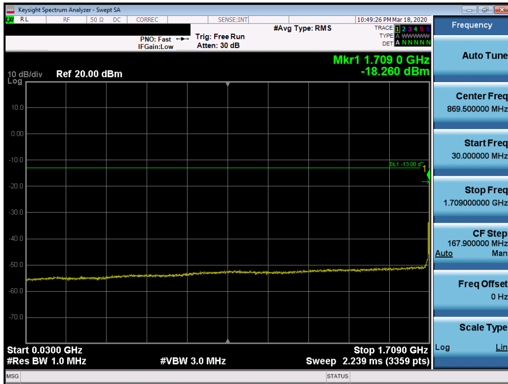
Plot 7-42. Conducted Spurious Plot (n66 - 20MHz DFT-s-OFDM-BPSK - RB Size 1, RB Offset 1 - Low Channel)
