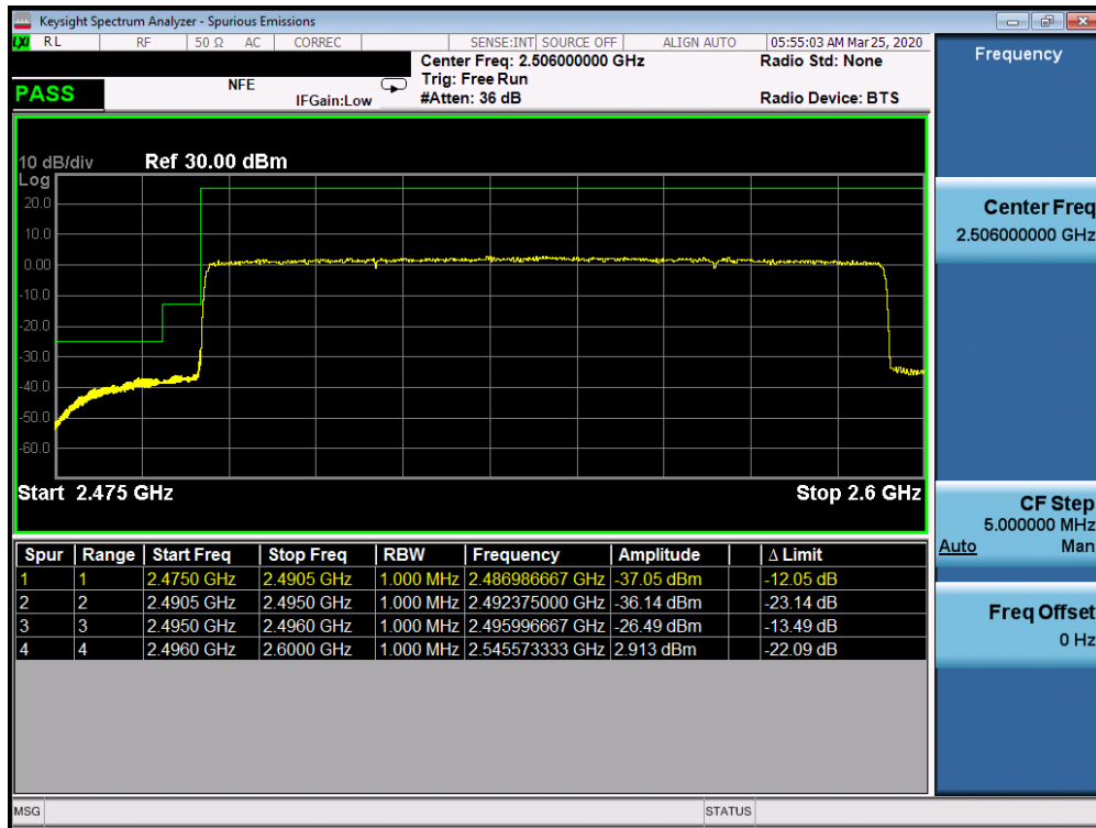
Plot 7-81. Lower Band Edge Plot (n41 - 100MHz DFT-s-OFDM-BPSK - Full RB Configuration)
