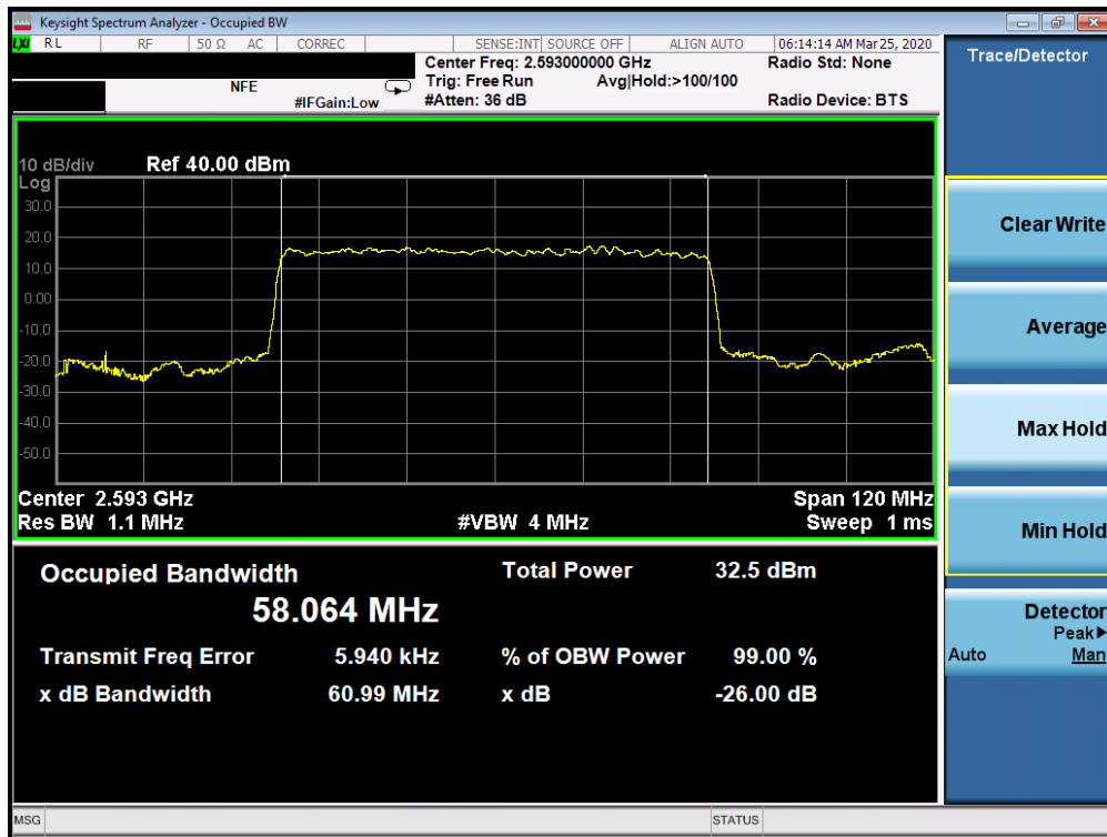
Plot 7-20. Occupied Bandwidth Plot (n41 60MHz DFT-s-OFDM-BPSK - Full RB Configuration)
