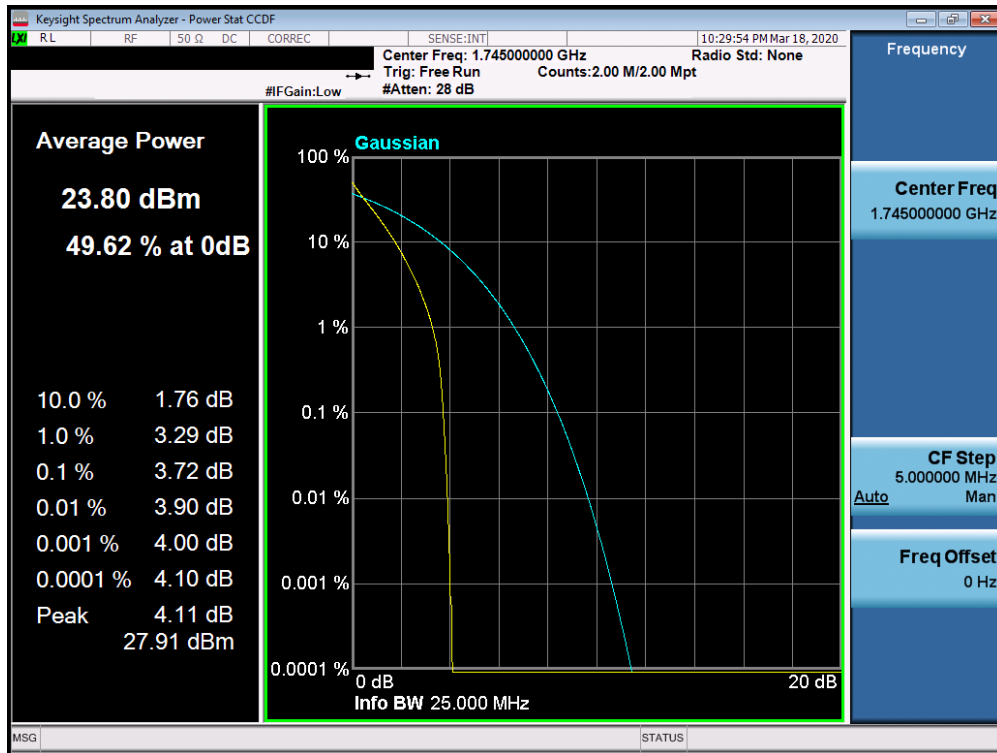
Plot 7-85. PAR Plot (Band n66 - 20.0MHz DFT-s-OFDM-BPSK - Full RB Configuration)
