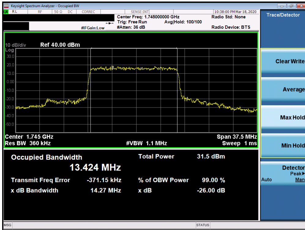
Plot 7-11. Occupied Bandwidth Plot (n66 15MHz DFT-s-OFDM-BPSK - Full RB Configuration)
