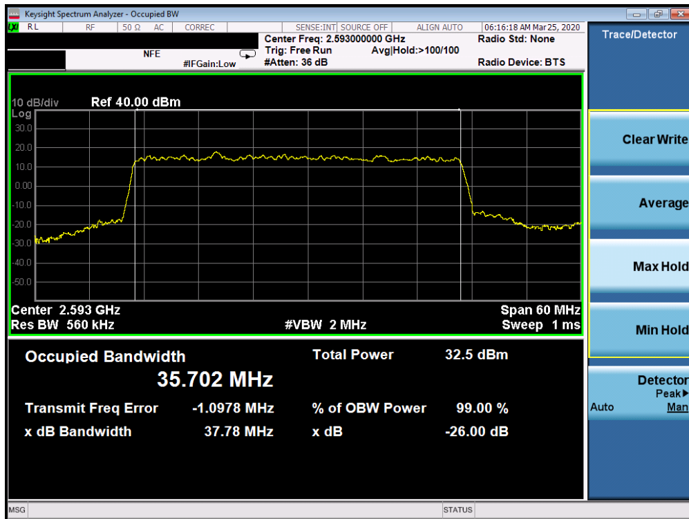
Plot 7-18. Occupied Bandwidth Plot (n41 40MHz DFT-s-OFDM-BPSK - Full RB Configuration)
