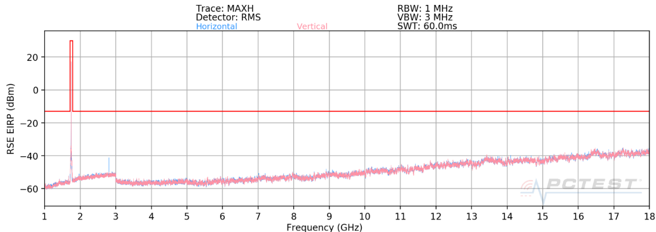
Plot 7-88. Radiated Spurious Plot above 1GHz (EN-DC n71 + LTE B66)
