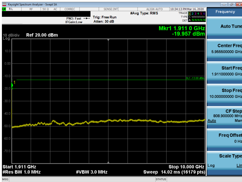
Plot 7-58. Conducted Spurious Plot (n2 - 20MHz DFT-s-OFDM-BPSK - RB Size 1, RB Offset 1 - High Channel)
