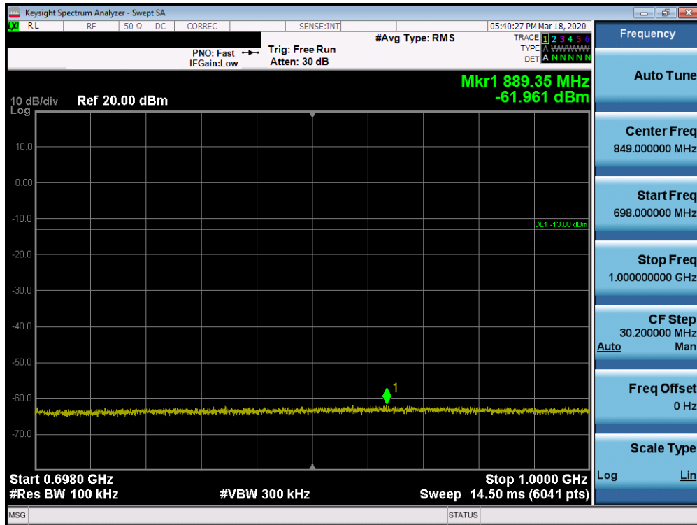
Plot 7-28. Conducted Spurious Plot (n71 - 20MHz DFT-s-OFDM-BPSK - RB Size 1, RB Offset 1 - Mid Channel)
