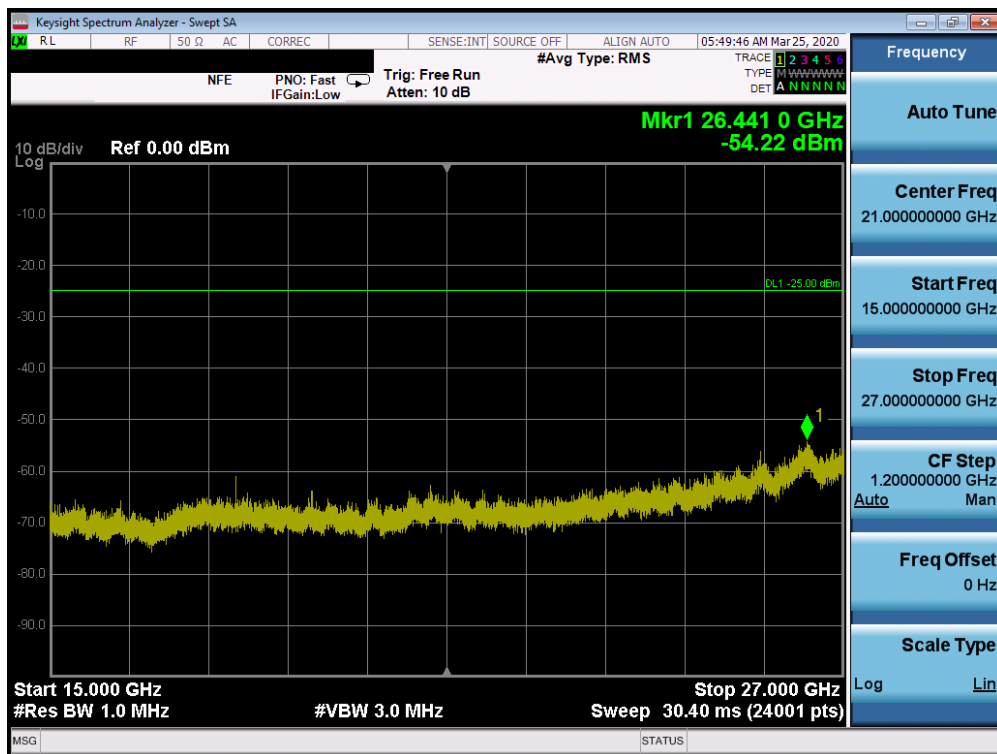
Plot 7-65. Conducted Spurious Plot (n41 - 100MHz DFT-s-OFDM-BPSK - RB Size 1, RB Offset 1 - Mid Channel)
