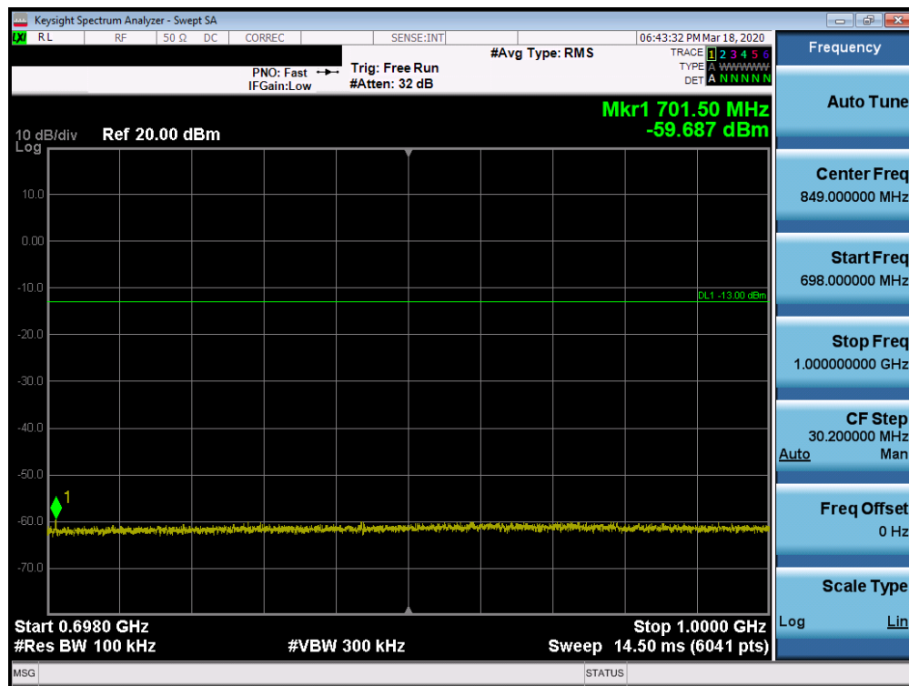
Plot 7-25. Conducted Spurious Plot (n71 - 20MHz DFT-s-OFDM-BPSK - RB Size 1, RB Offset 1 - Low Channel)
