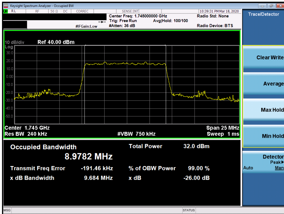
Plot 7-10. Occupied Bandwidth Plot (n66 10MHz DFT-s-OFDM-BPSK - Full RB Configuration)
