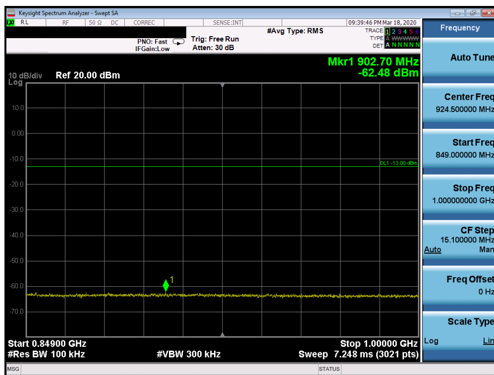
Plot 7-34. Conducted Spurious Plot (n5 - 20MHz DFT-s-OFDM-BPSK - RB Size 1, RB Offset 1 - Low Channel)
