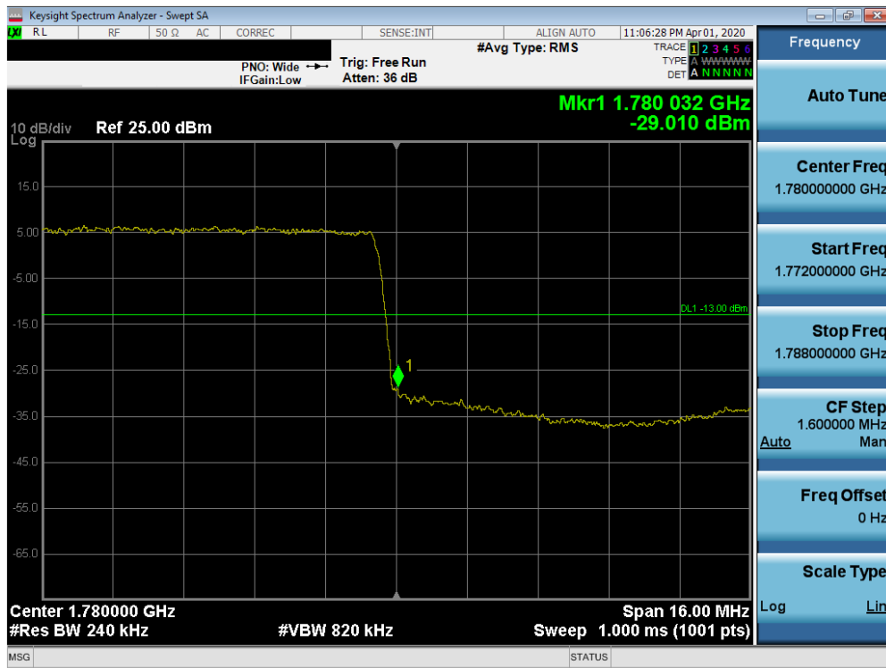
Plot 7-75. Upper Band Edge Plot (n66 - 20MHz DFT-s-OFDM-BPSK - Full RB Configuration)
