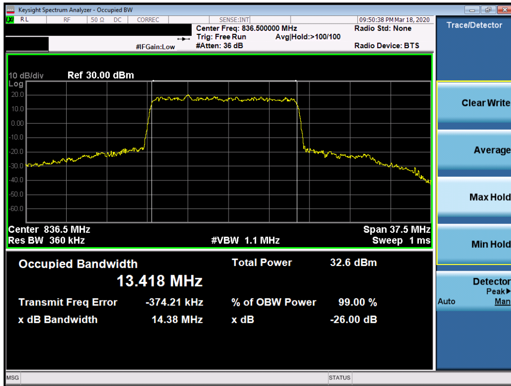
Plot 7-7. Occupied Bandwidth Plot (n5 15MHz DFT-s-OFDM-BPSK - Full RB Configuration)
