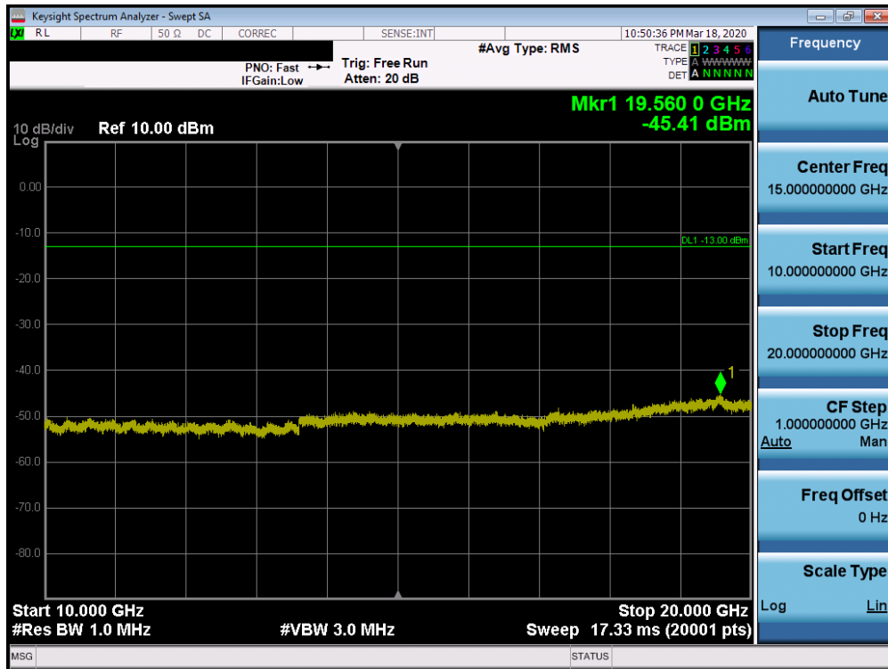
Plot 7-44. Conducted Spurious Plot (n66 - 20MHz DFT-s-OFDM-BPSK - RB Size 1, RB Offset 1 - Low Channel)
