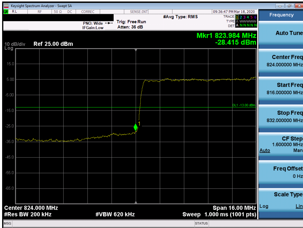
Plot 7-71. Lower Band Edge Plot (n5 - 20MHz DFT-s-OFDM-BPSK - Full RB Configuration)
