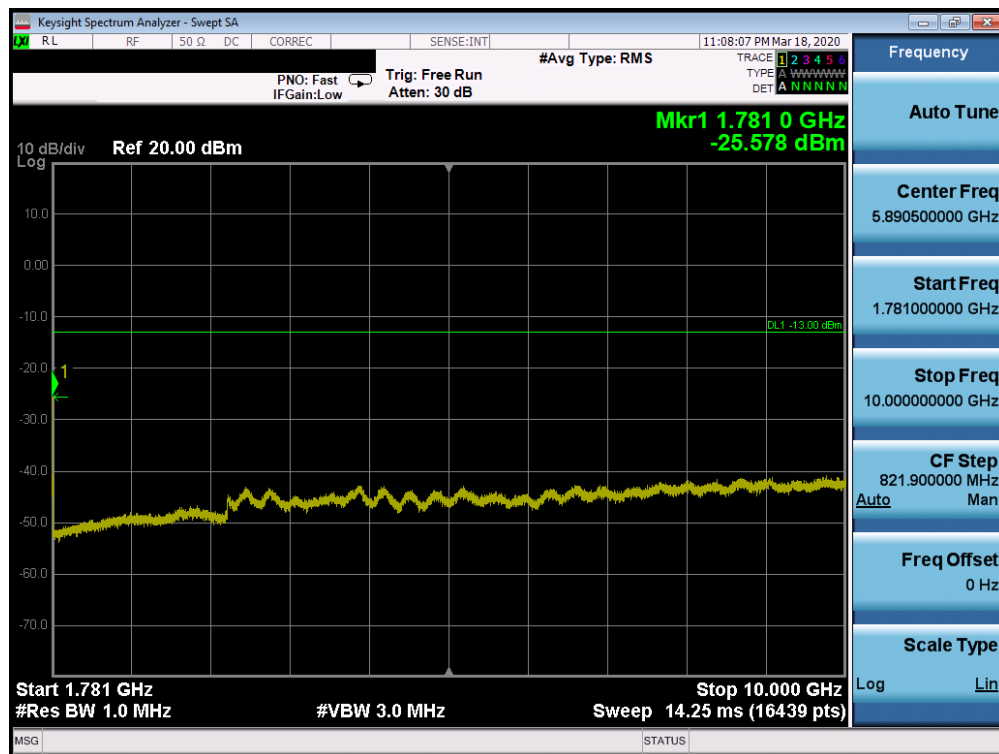
Plot 7-49. Conducted Spurious Plot (n66 - 20MHz DFT-s-OFDM-BPSK - RB Size 1, RB Offset 1 - High Channel)
