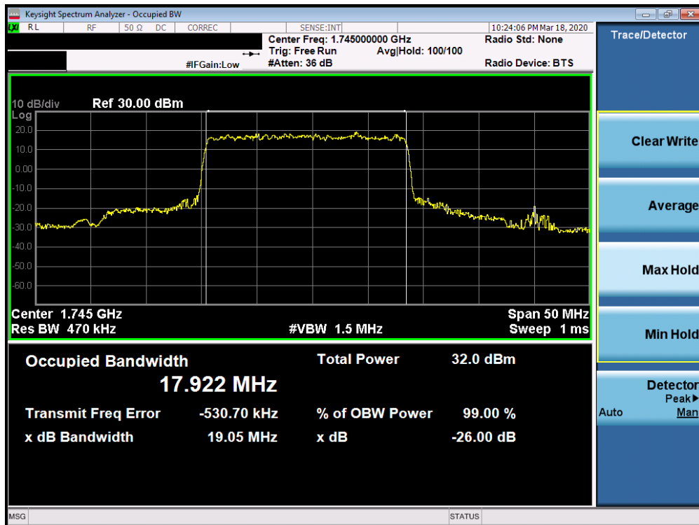
Plot 7-12. Occupied Bandwidth Plot (n66 20MHz DFT-s-OFDM-BPSK - Full RB Configuration)
