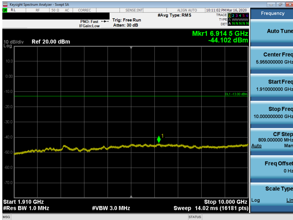
Plot 7-55. Conducted Spurious Plot (n2 - 20MHz DFT-s-OFDM-BPSK - RB Size 1, RB Offset 1 - Mid Channel)
