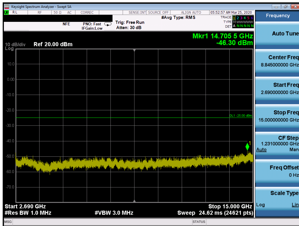
Plot 7-61. Conducted Spurious Plot (n41 - 100MHz DFT-s-OFDM-BPSK - RB Size 1, RB Offset 1 - Low Channel)
