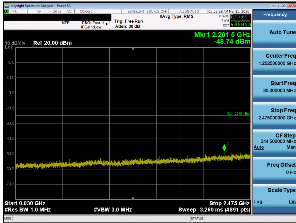
Plot 7-60. Conducted Spurious Plot (n41 - 100MHz DFT-s-OFDM-BPSK - RB Size 1, RB Offset 1 - Low Channel)
