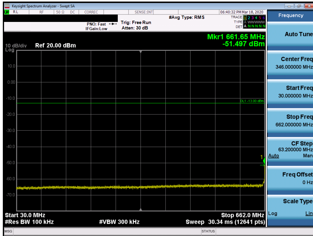
Plot 7-24. Conducted Spurious Plot (n71 - 20MHz DFT-s-OFDM-BPSK - RB Size 1, RB Offset 1 - Low Channel)
