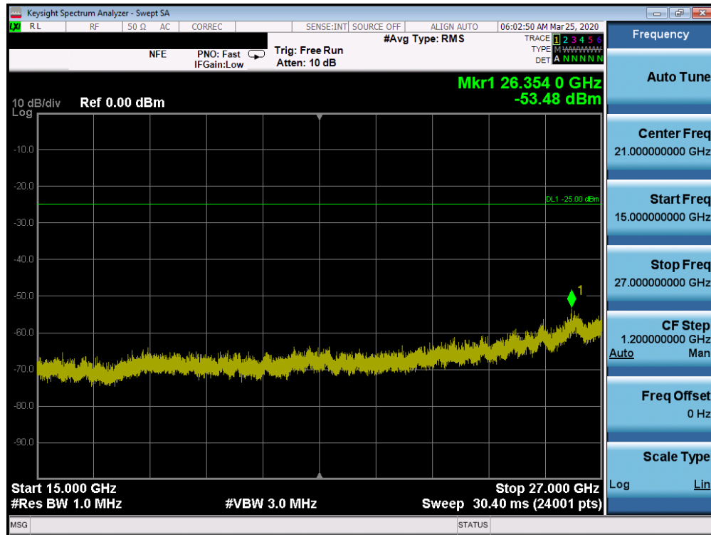
Plot 7-68. Conducted Spurious Plot (n41 - 100MHz DFT-s-OFDM-BPSK - RB Size 1, RB Offset 1 - High Channel)
