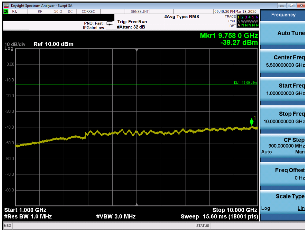
Plot 7-35. Conducted Spurious Plot (n5 - 20MHz DFT-s-OFDM-BPSK - RB Size 1, RB Offset 1 - Low Channel)
