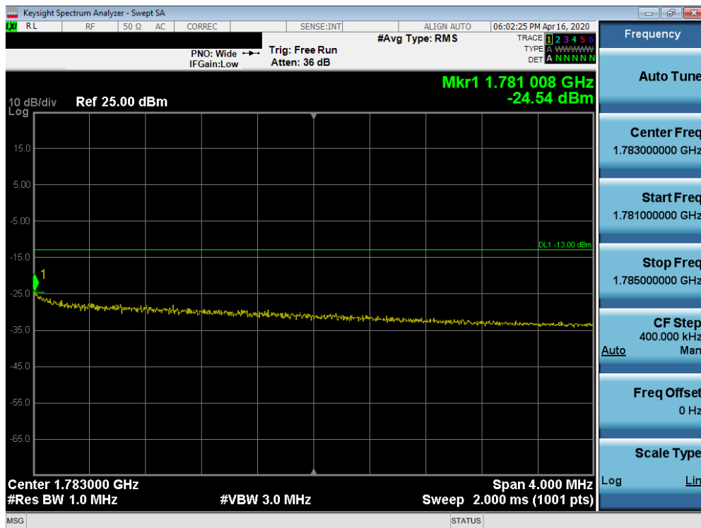
Plot 7-76. Upper Extended Band Edge Plot (n66 - 20MHz DFT-s-OFDM-BPSK - Full RB Configuration)
