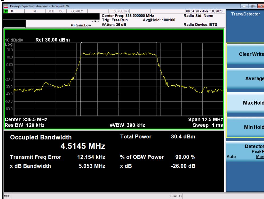
Plot 7-5. Occupied Bandwidth Plot (n5 5MHz DFT-s-OFDM-BPSK Full RB Configuration)
