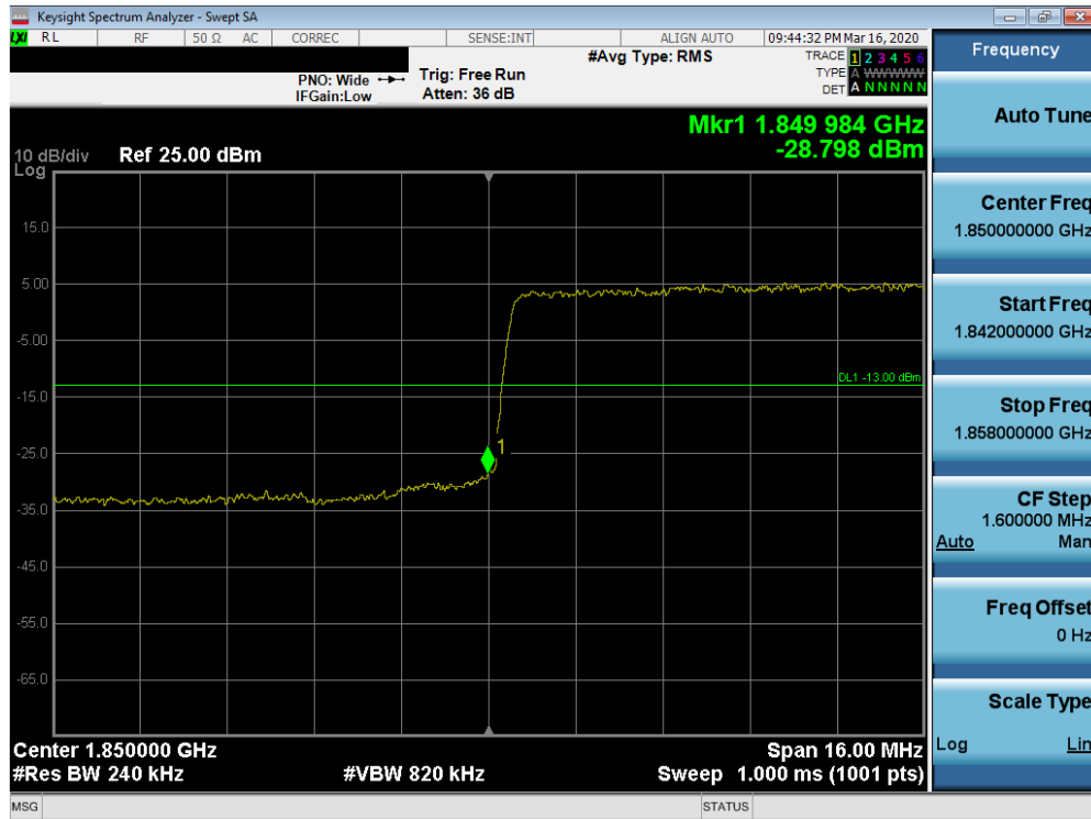
Plot 7-77. Lower Band Edge Plot (n2 - 20MHz DFT-s-OFDM-BPSK - Full RB Configuration)
