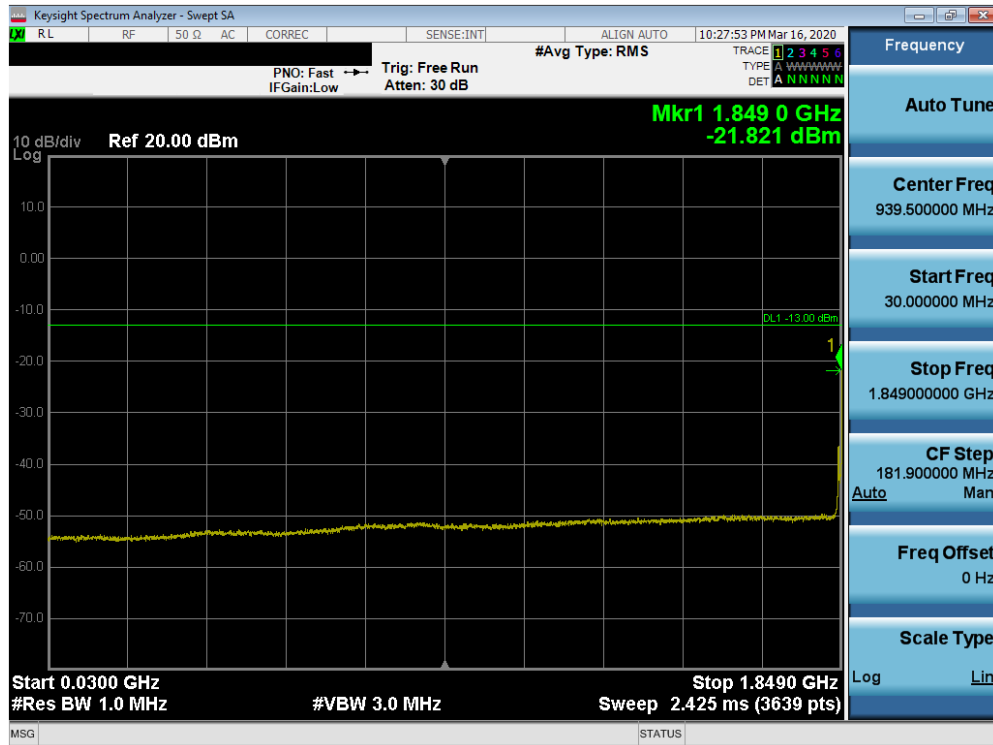
Plot 7-51. Conducted Spurious Plot (n2 - 20MHz DFT-s-OFDM-BPSK - RB Size 1, RB Offset 1 - Low Channel)
