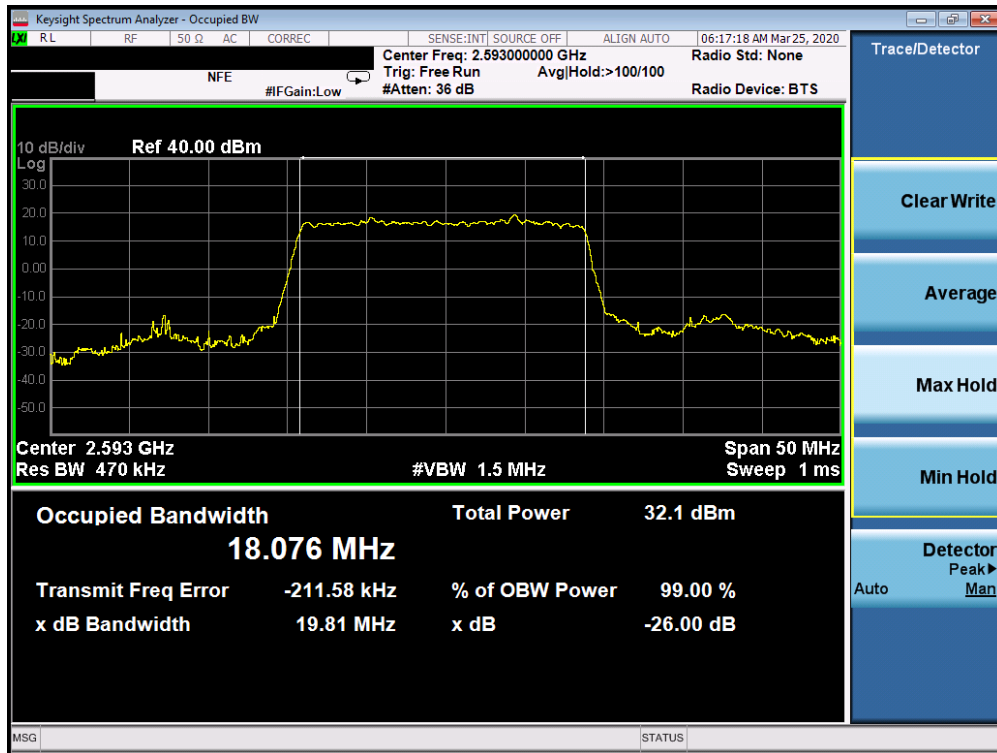
Plot 7-17. Occupied Bandwidth Plot (n41 20MHz DFT-s-OFDM-BPSK Full RB Configuration)
