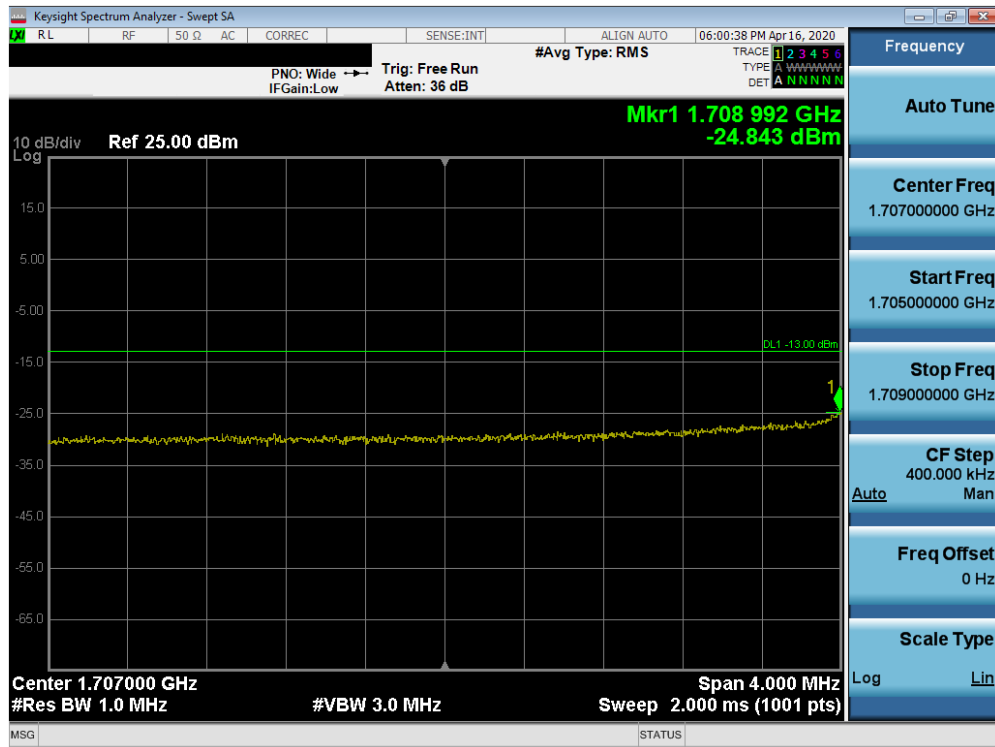
Plot 7-74. Lower Extended Band Edge Plot (n66 - 20MHz DFT-s-OFDM-BPSK - Full RB Configuration)
