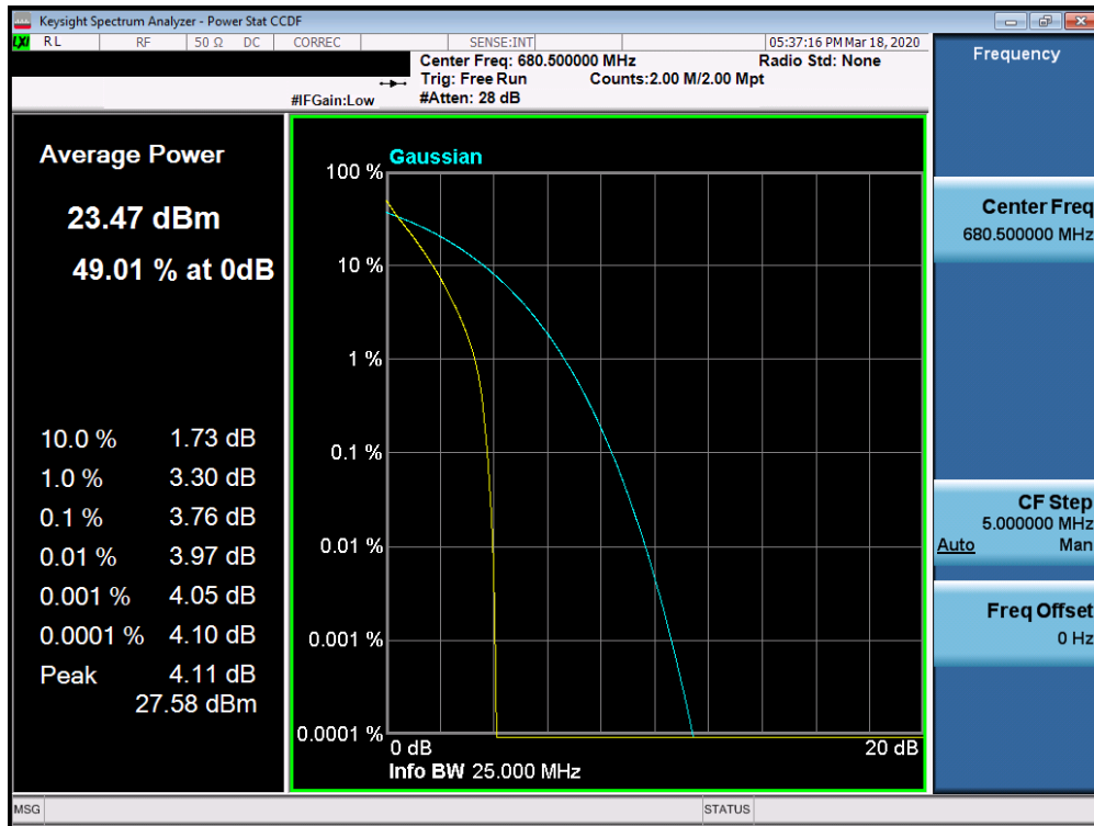
Plot 7-83. PAR Plot (Band n71 - 20.0MHz DFT-s-OFDM-BPSK - Full RB Configuration)
