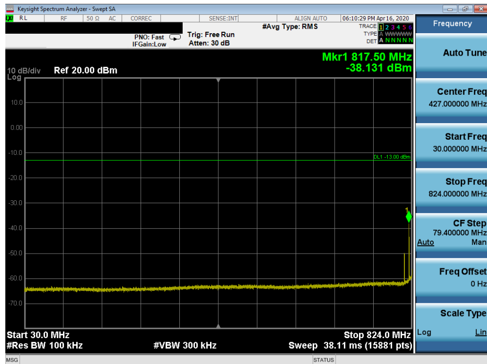
Plot 7-36. Conducted Spurious Plot (n5 - 20MHz DFT-s-OFDM-BPSK - RB Size 1, RB Offset 1 - Mid Channel)
