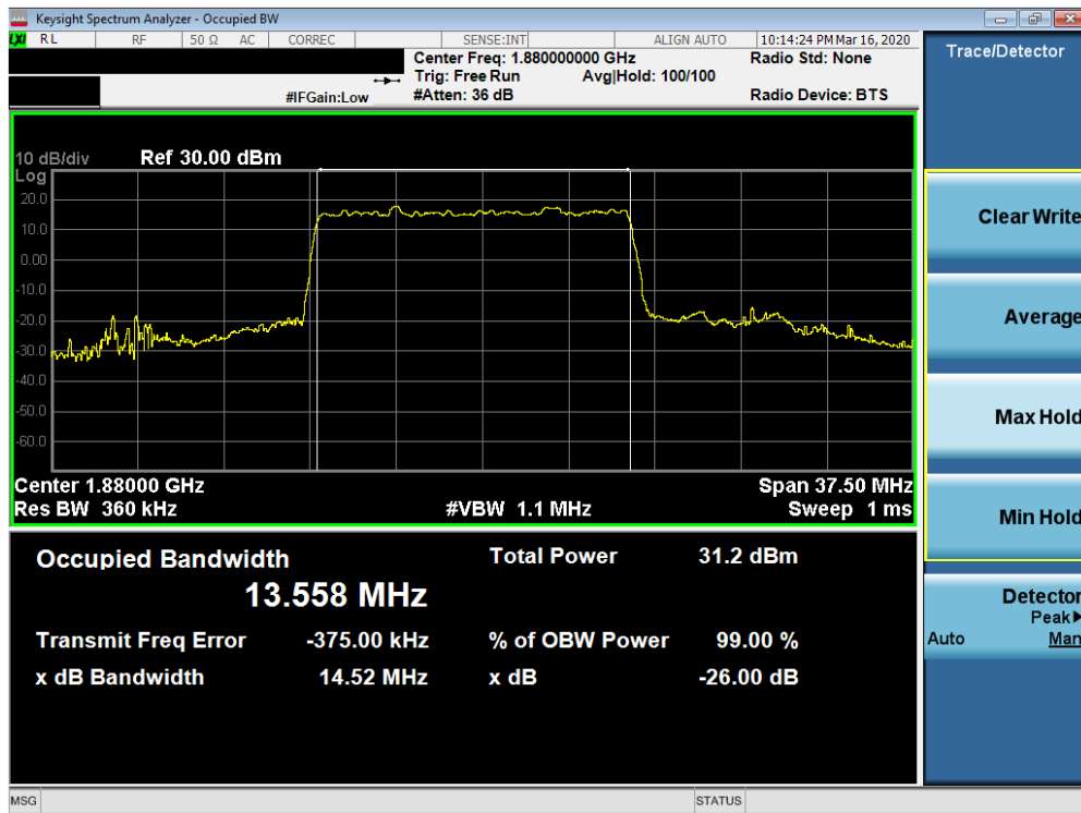
Plot 7-15. Occupied Bandwidth Plot (n2 15MHz DFT-s-OFDM-BPSK - Full RB Configuration)
