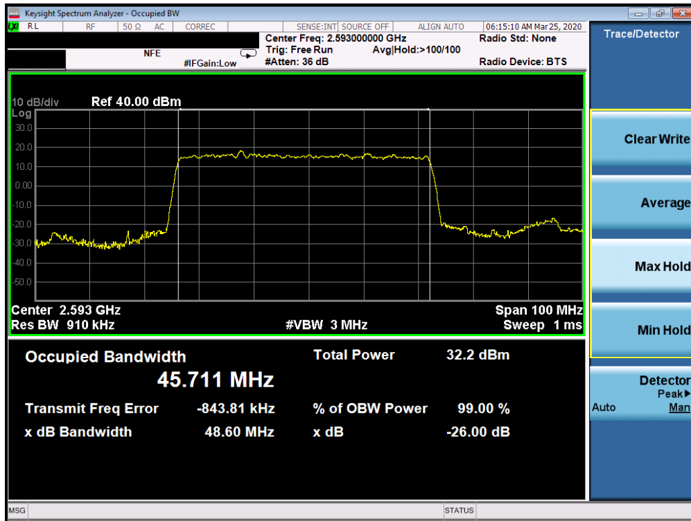
Plot 7-19. Occupied Bandwidth Plot (n41 50MHz DFT-s-OFDM-BPSK - Full RB Configuration)
