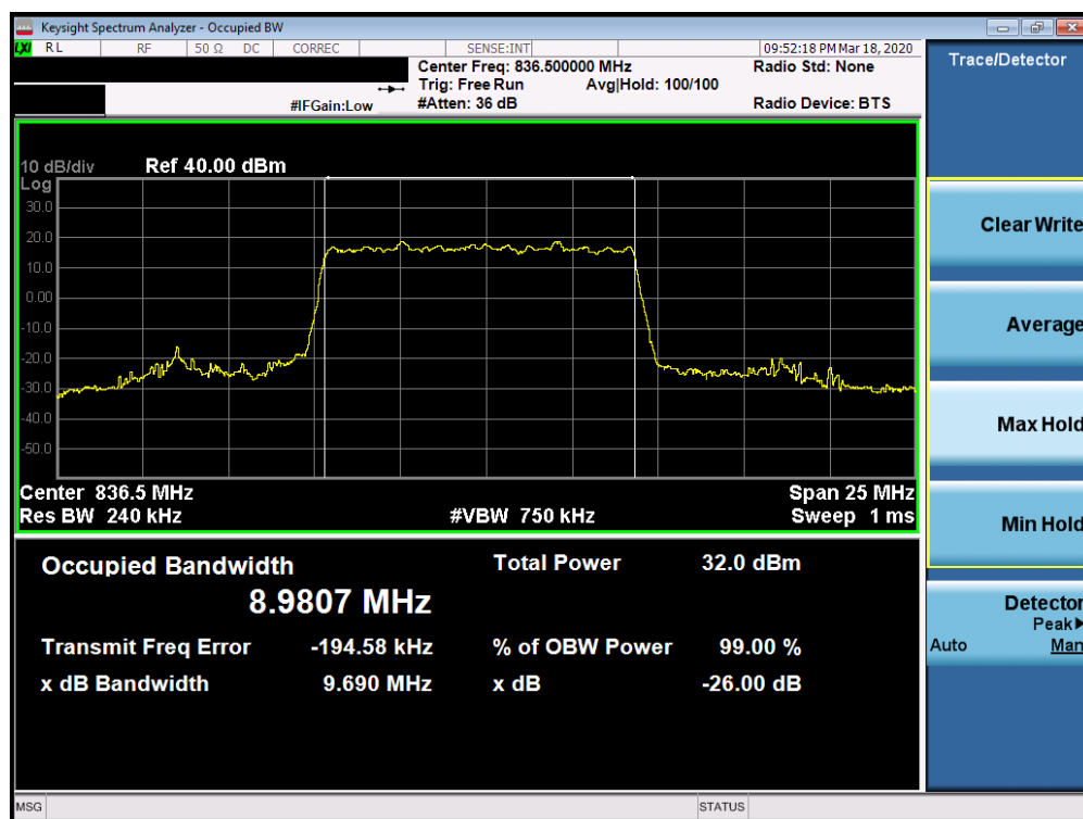
Plot 7-6. Occupied Bandwidth Plot (n5 10MHz DFT-s-OFDM-BPSK - Full RB Configuration)
