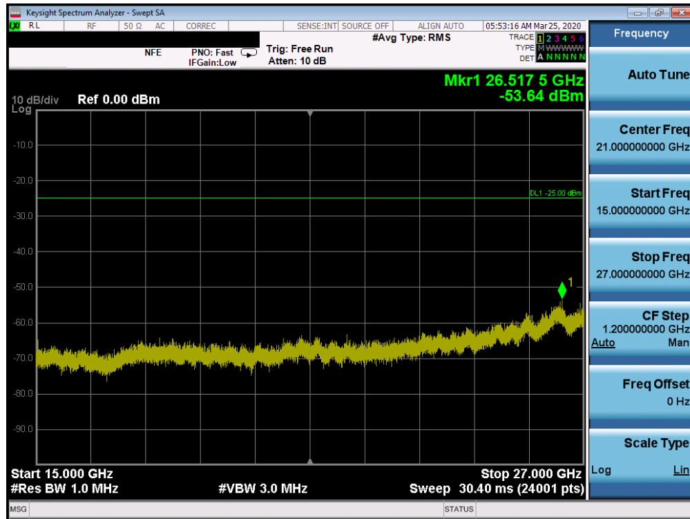
Plot 7-62. Conducted Spurious Plot (n41 - 100MHz DFT-s-OFDM-BPSK - RB Size 1, RB Offset 1 - Low Channel)
