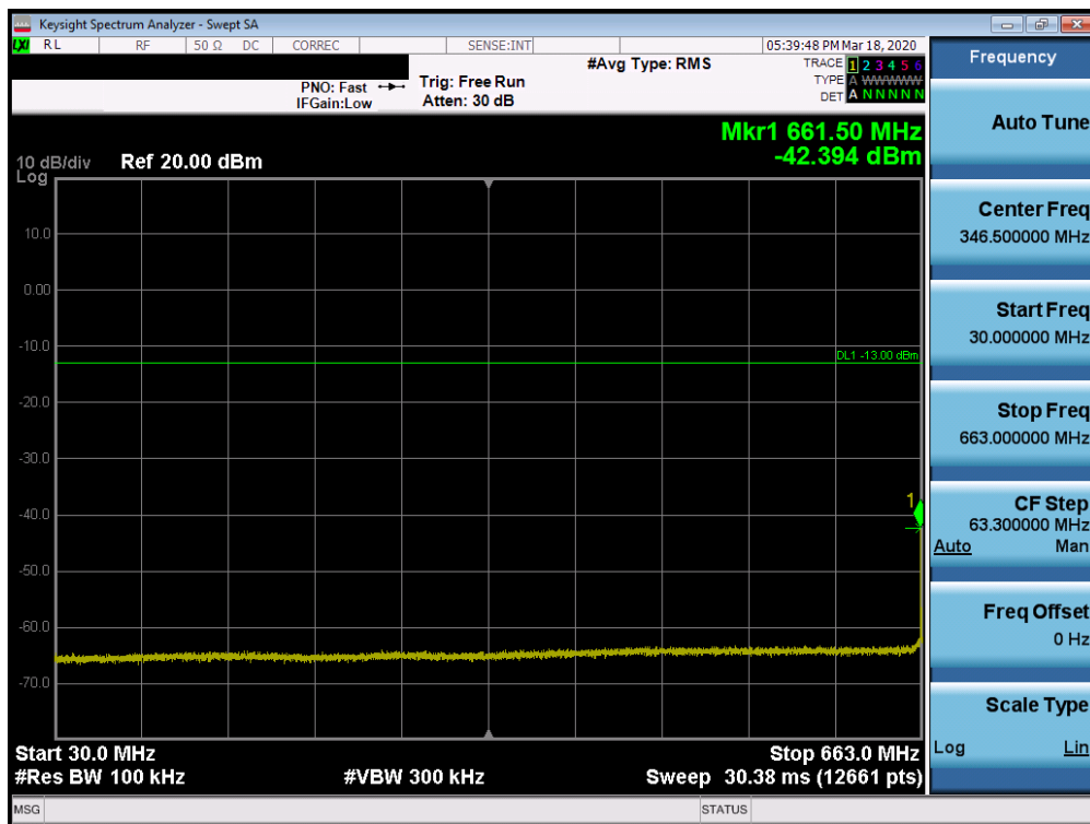
Plot 7-27. Conducted Spurious Plot (n71 - 20MHz DFT-s-OFDM-BPSK - RB Size 1, RB Offset 1 - Mid Channel)
