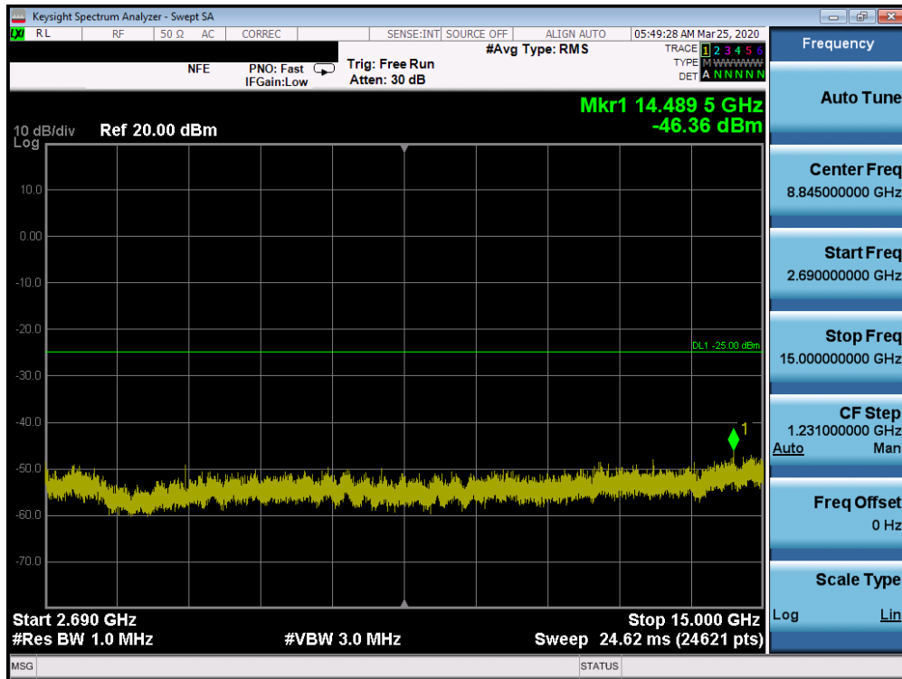
Plot 7-64. Conducted Spurious Plot (n41 - 100MHz DFT-s-OFDM-BPSK - RB Size 1, RB Offset 1 - Mid Channel)
