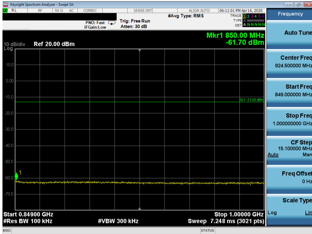
Plot 7-37. Conducted Spurious Plot (n5 - 20MHz DFT-s-OFDM-BPSK - RB Size 1, RB Offset 1 - Mid Channel)
