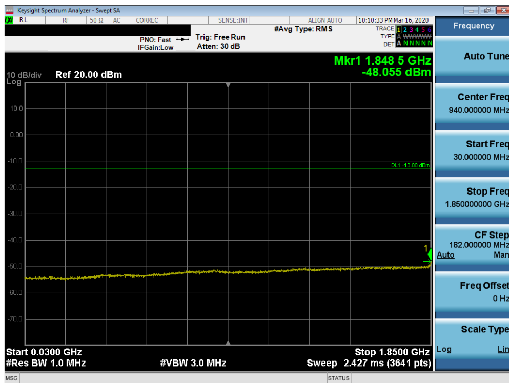
Plot 7-54. Conducted Spurious Plot (n2 - 20MHz DFT-s-OFDM-BPSK - RB Size 1, RB Offset 1 - Mid Channel)
