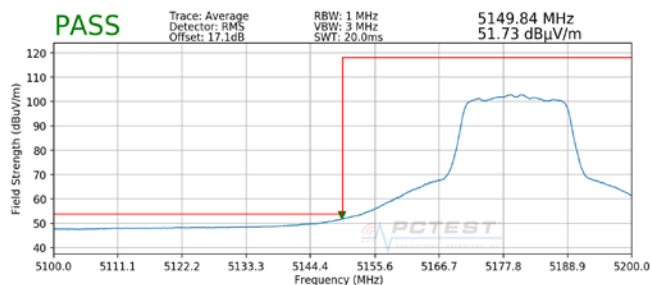
Plot 7-328. Radiated Lower Band Edge Plot MIMO (Average – UNII Band 1)
