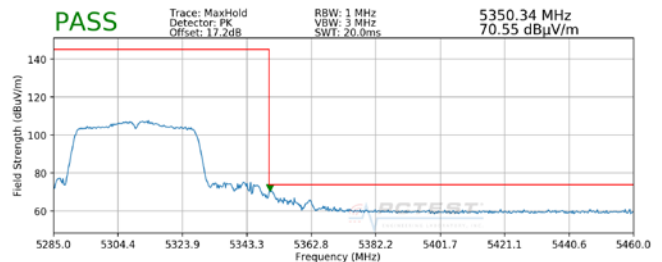
Plot 7-340. Radiated Upper Band Edge Plot MIMO (Peak – UNII Band 2A)
