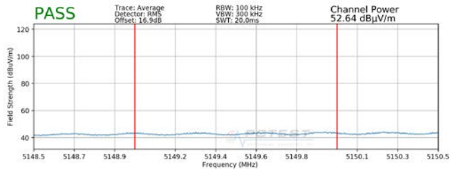
Plot 7-335. Radiated Band Edge Plot MIMO (Average – WCP)
