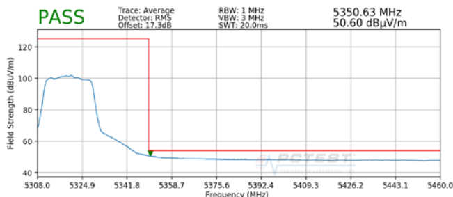
Plot 7-330. Radiated Upper Band Edge Plot MIMO (Average – UNII Band 2A)
