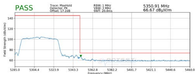
Plot 7-345. Radiated Band Edge Plot MIMO (Peak – WCP)
