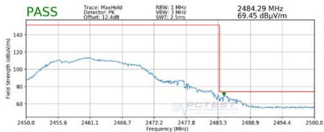
Plot 7-120. Radiated Restricted Upper Band Edge Measurement CDD (Peak)
