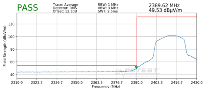
Plot 7-103. Radiated Restricted Lower Band Edge Measurement SISO ANT1 (Average)
