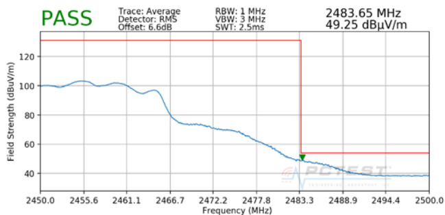
Plot 7-117. Radiated Restricted Upper Band Edge Measurement CDD (Average)
