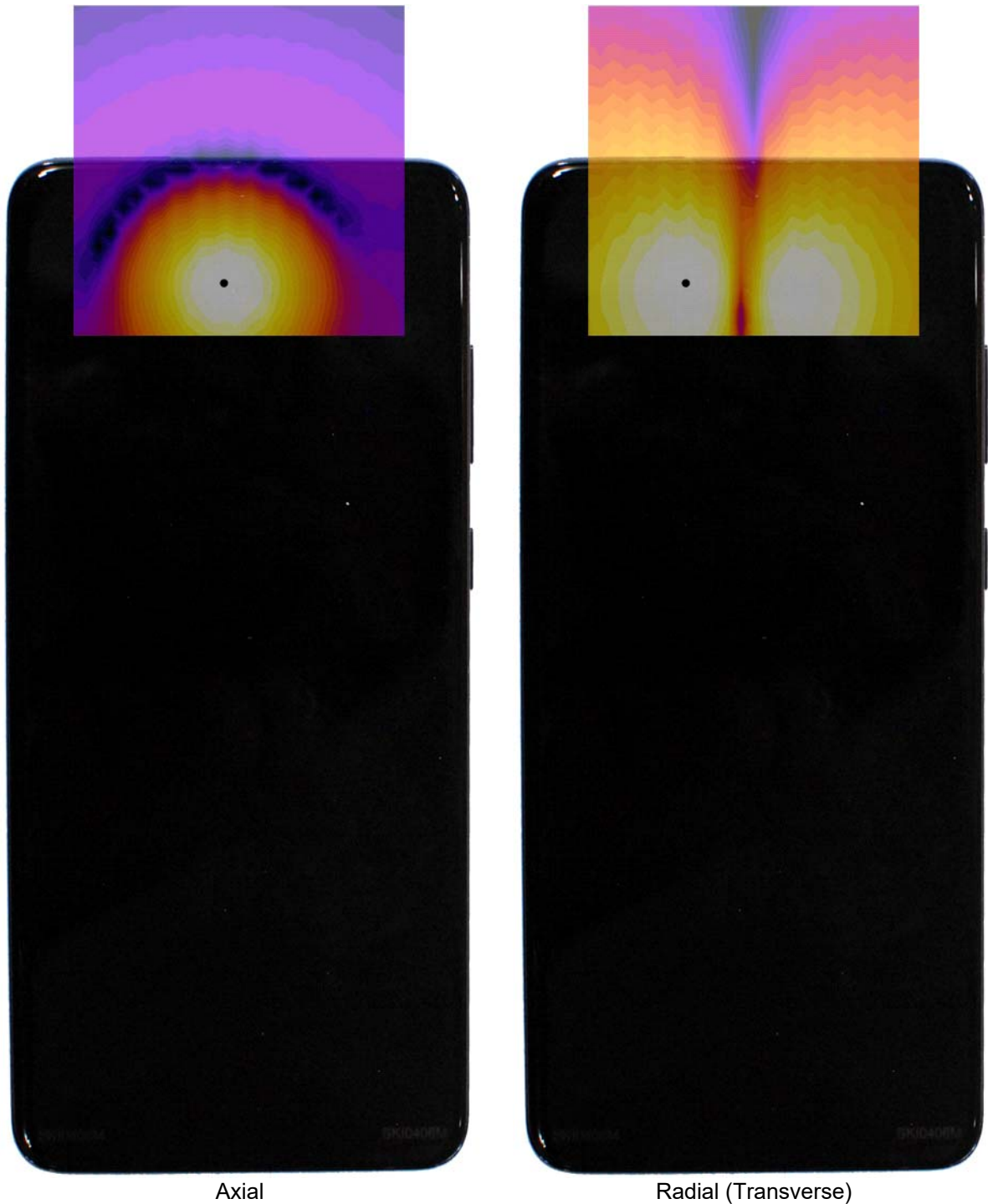
Figure 13-3 T-Coil Scan Overlay Magnetic Field Distributions
