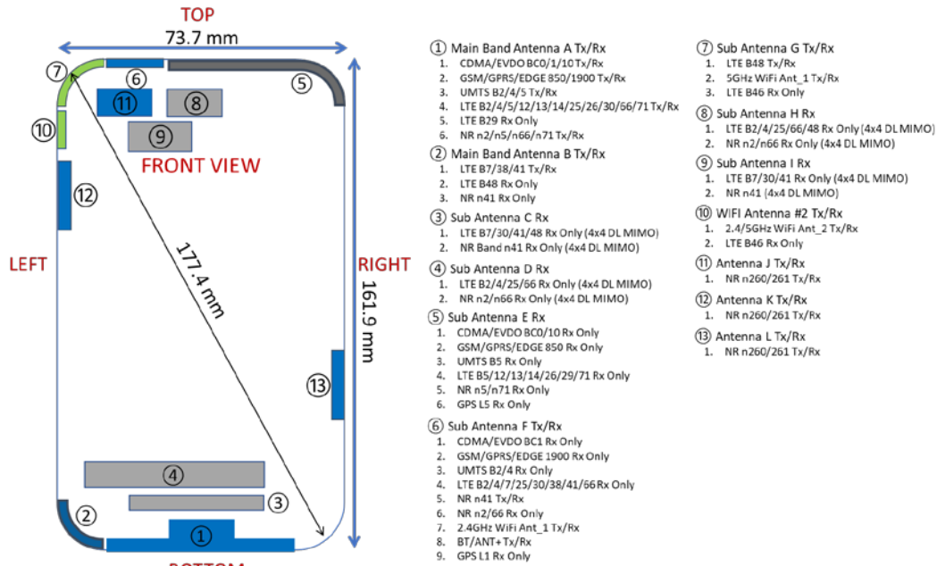
Figure E-1 DUT Antenna Locations
