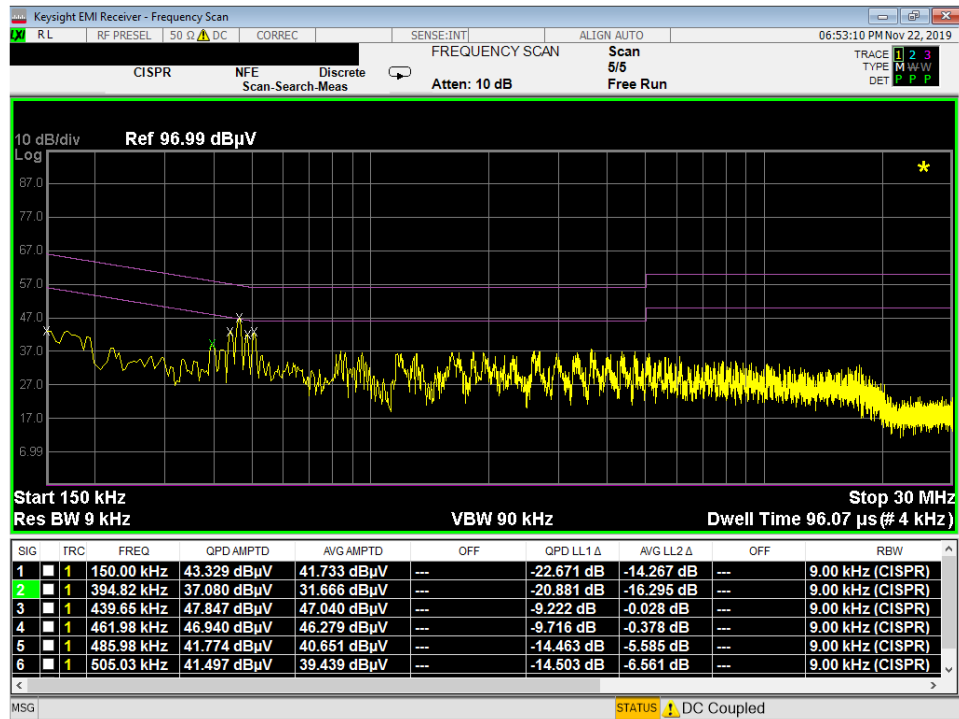
Plot 7-8. Line-Conducted Test Plot (L1) Terminated at 50 Ohms
