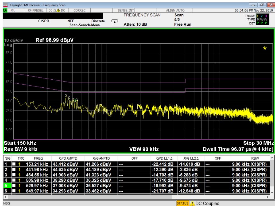
Plot 7-9. Line-Conducted Test Plot (N) Terminated at 50 Ohms
