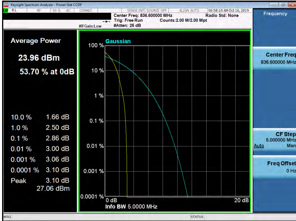
Plot 7-87. Peak-Average Ratio Plot (Cell WCDMA Mode)
