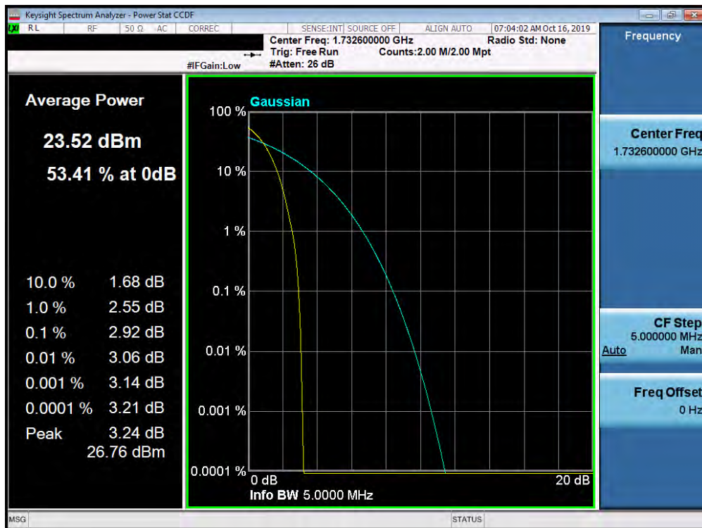
Plot 7-88. Peak-Average Ratio Plot (AWS WCDMA Mode)
