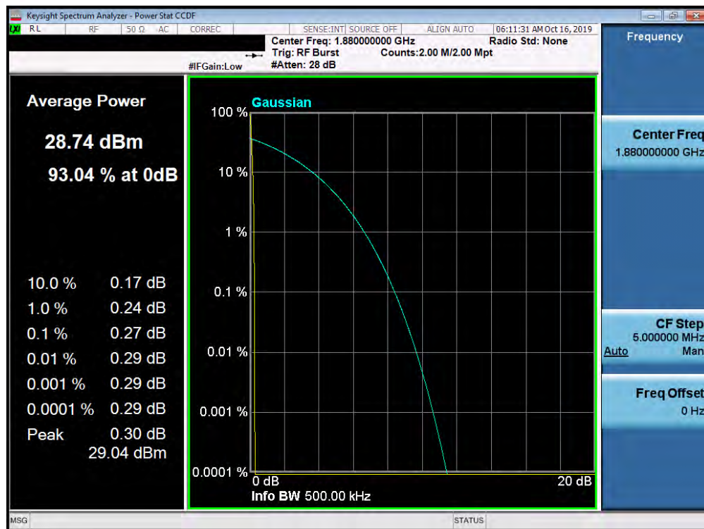
Plot 7-85. Peak-Average Ratio Plot (PCS GSM Mode)
