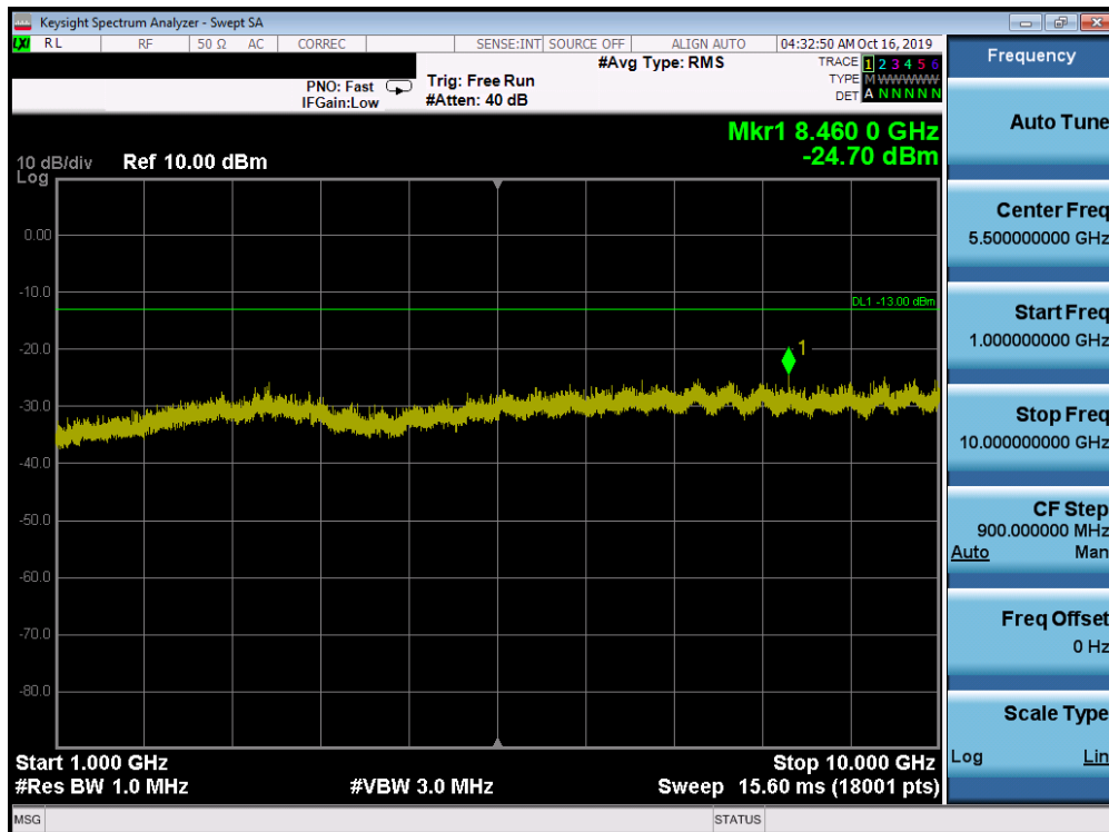
Plot 7-14. Conducted Spurious Plot (Cellular GSM Mode - Mid Channel)
