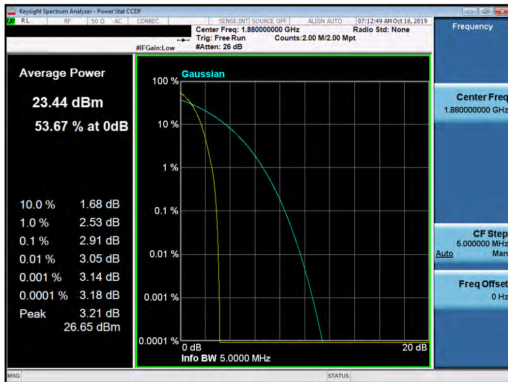
Plot 7-89. Peak-Average Ratio Plot (PCS WCDMA Mode)
