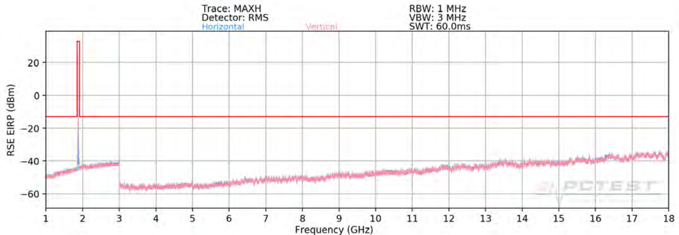
Plot 7-94. Radiated Spurious Plot above 1GHz (PCS GSM Mode)
