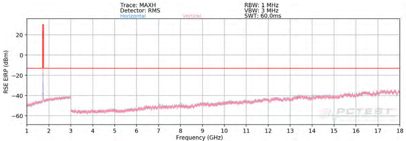
Plot 7-93. Radiated Spurious Plot above 1GHz (AWS WCDMA Mode)
