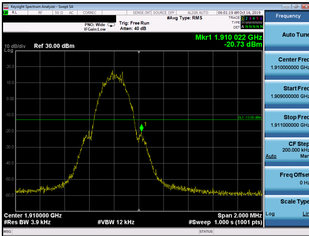
Plot 7-67. Band Edge Plot (PCS GSM Mode - High Channel)
