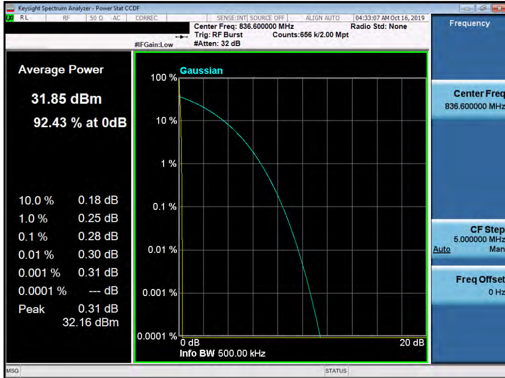
Plot 7-83. Peak-Average Ratio Plot (Cell GPRS Mode)
