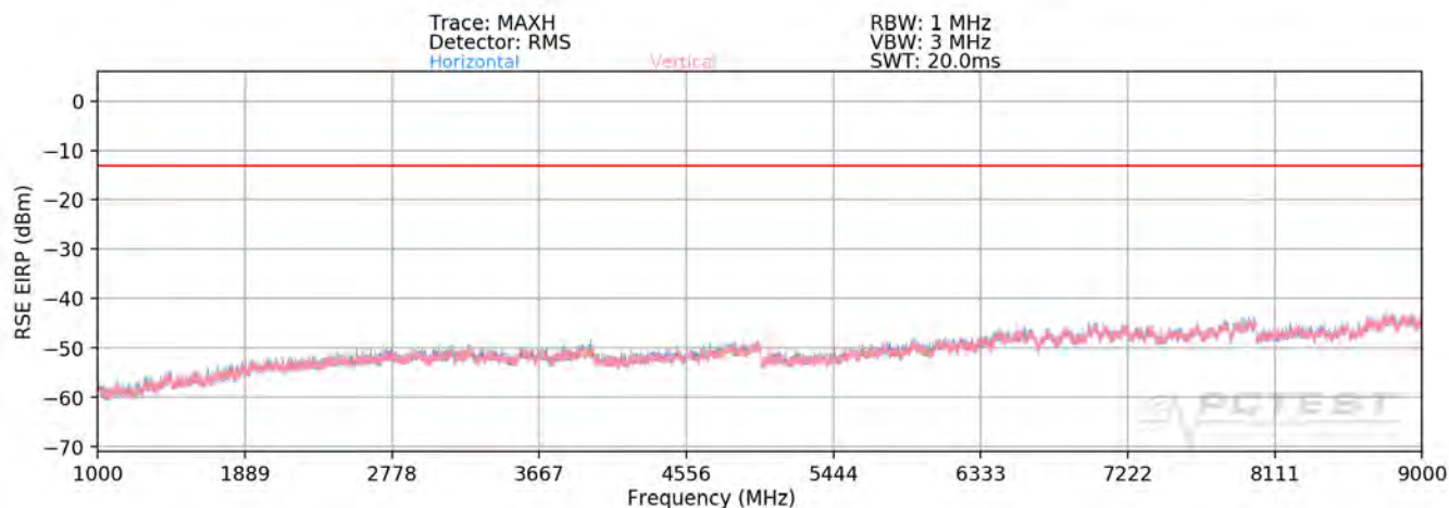
Plot 7-92. Radiated Spurious Plot above 1GHz (Cellular WCDMA Mode)
