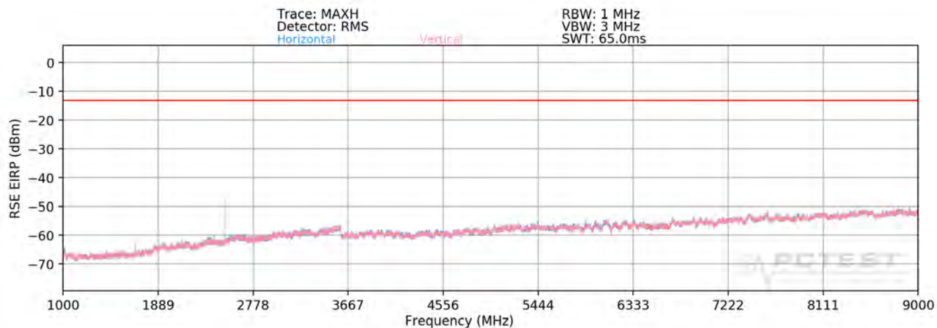
Plot 7-90. Radiated Spurious Plot above 1GHz (Cellular GSM Mode)
