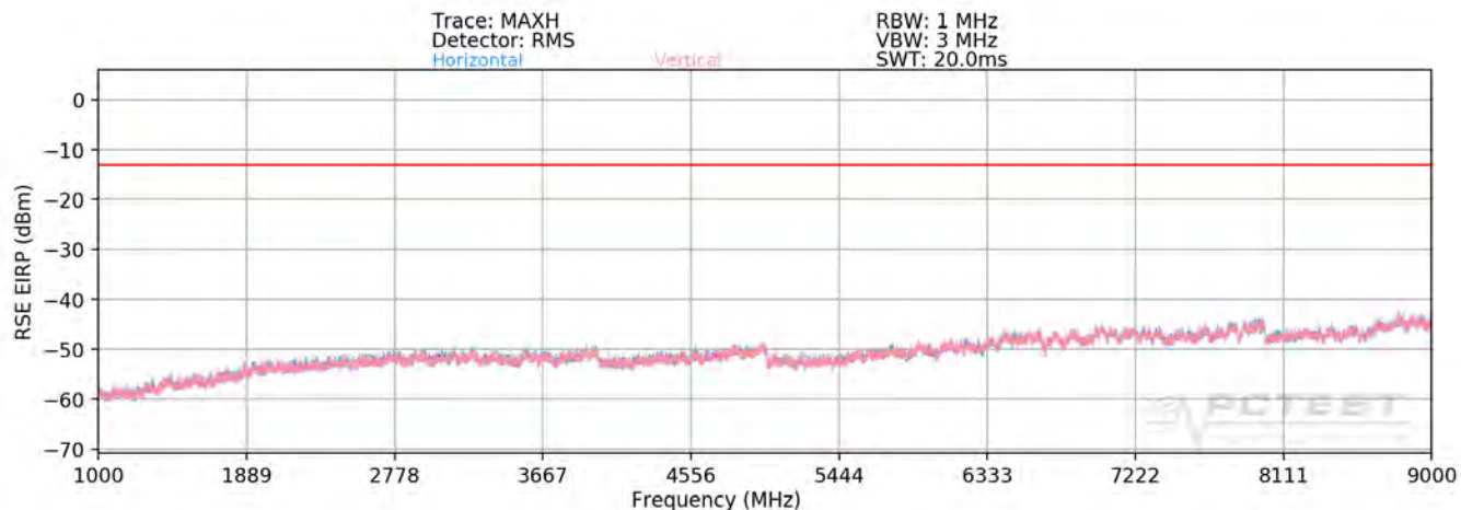
Plot 7-91. Radiated Spurious Plot above 1GHz (Cellular CDMA Mode)
