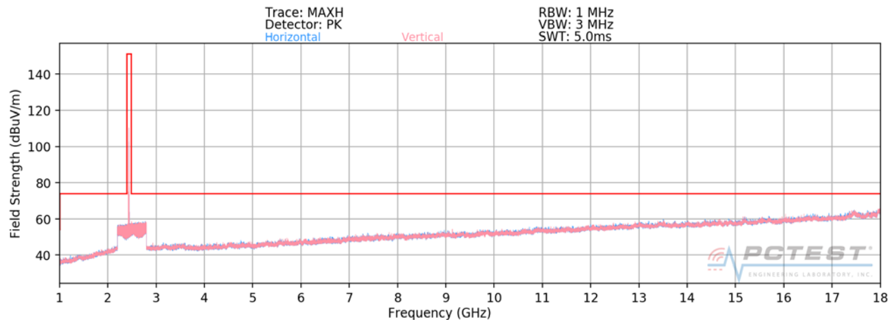
Plot 7-42. Radiated Spurious Plot above 1GHz (BT- Ch. 70)
