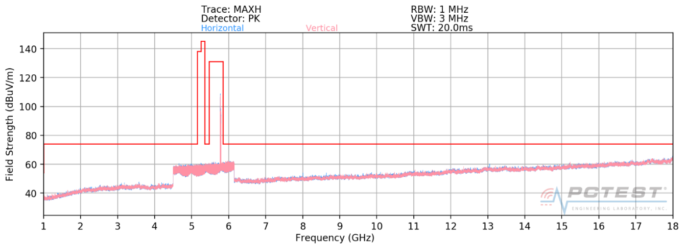
Plot 7-274. Radiated Spurious Plot above 1GHz SISO ANT1 (802.11ax – U3 Ch. 157 – 106 Tones)
