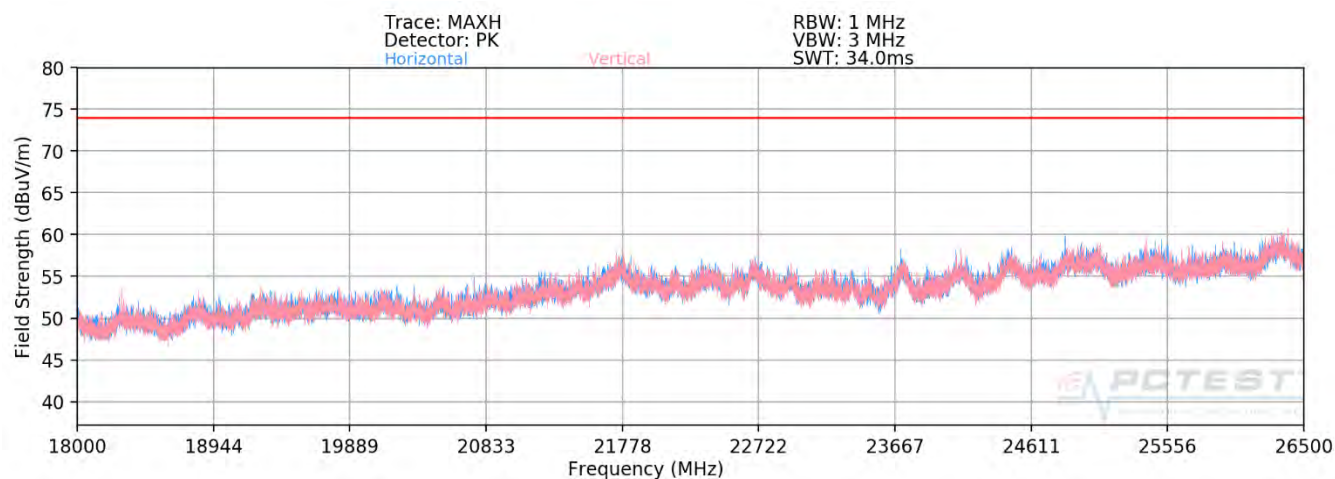
Plot 7-77. Radiated Spurious Plot above 18GHz SISO ANT1 (802.11ax OFDMA – 106 Tones)
