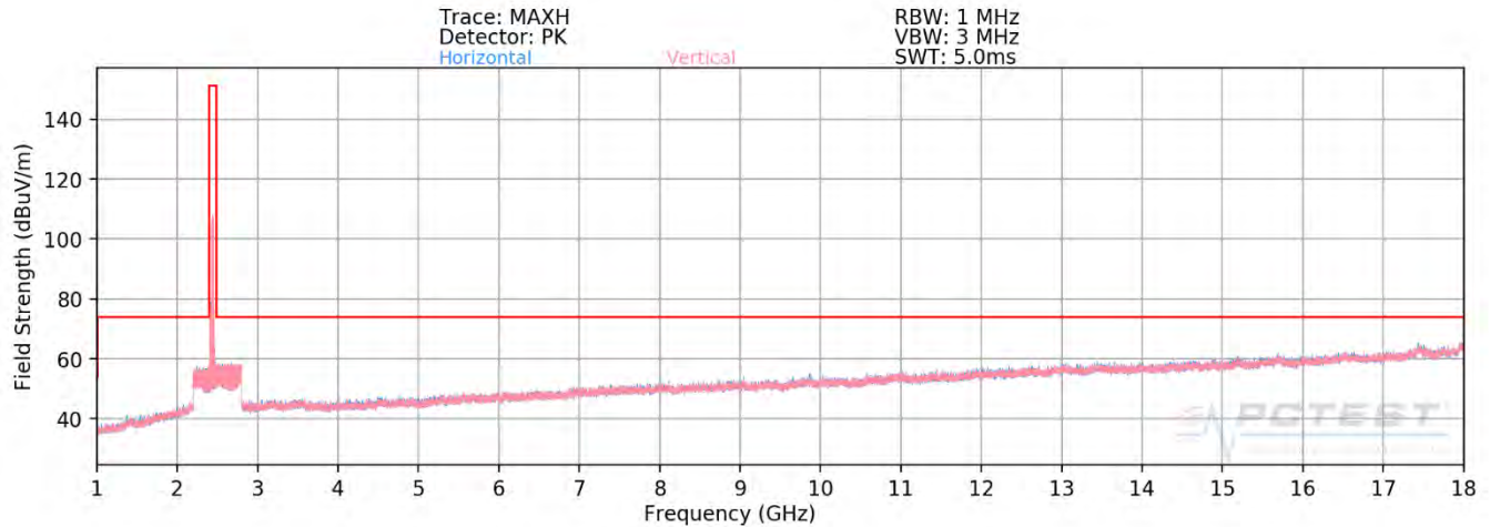
Plot 7-75. Radiated Spurious Plot above 1GHz SISO ANT1 (802.11ax OFDMA – 242 Tones – Ch. 6)
