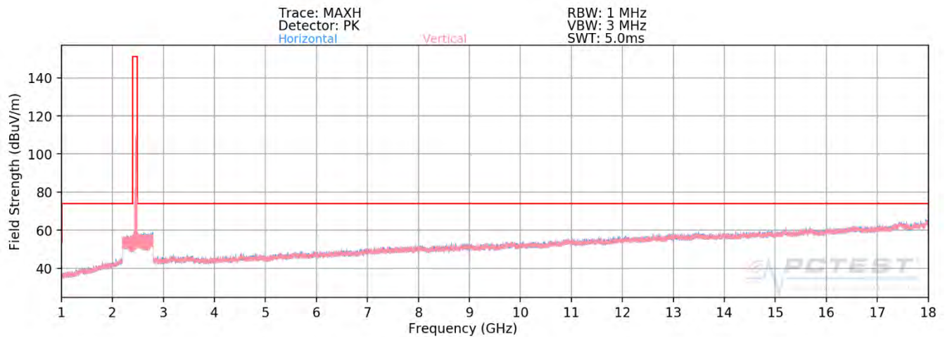
Plot 7-76. Radiated Spurious Plot above 1GHz SISO ANT1 (802.11ax OFDMA – 242 Tones – Ch. 11)
