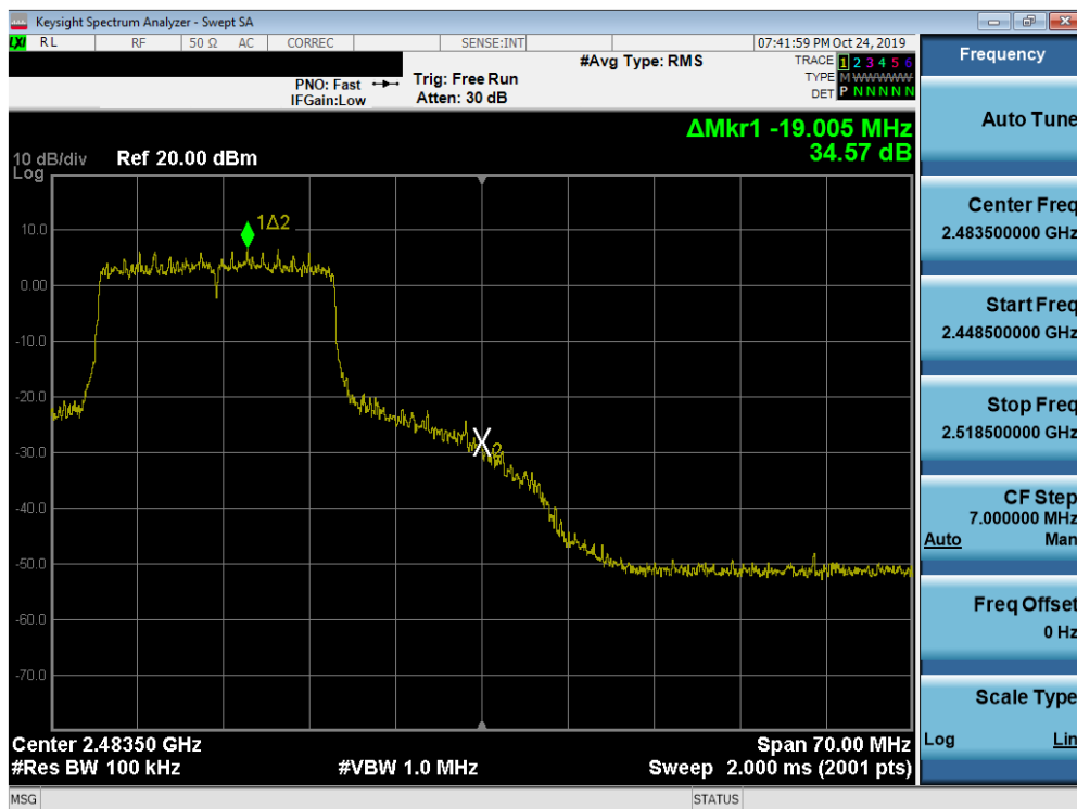
Plot 7-41. Band Edge Plot SISO ANT1 (802.11ax OFDMA – 242 Tones – Ch. 11)
