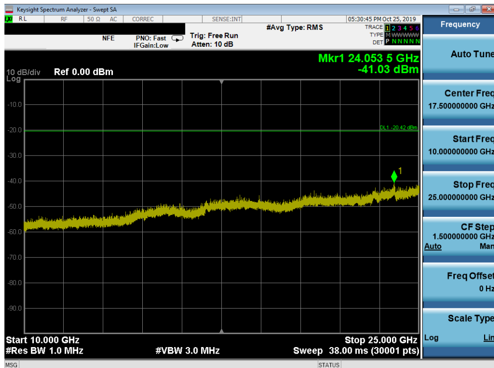
Plot 7-50. Conducted Spurious Plot SISO ANT1 (802.11ax OFDMA – 26 Tones – Ch. 6)
