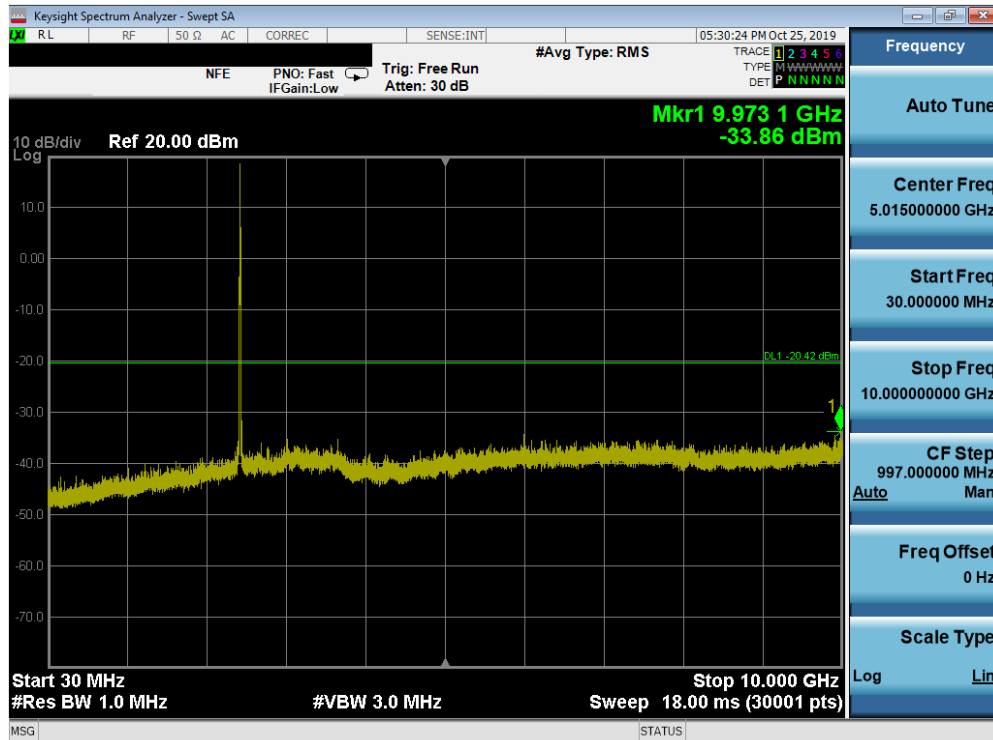
Plot 7-49. Conducted Spurious Plot SISO ANT1 (802.11ax OFDMA – 26 Tones – Ch. 6)
