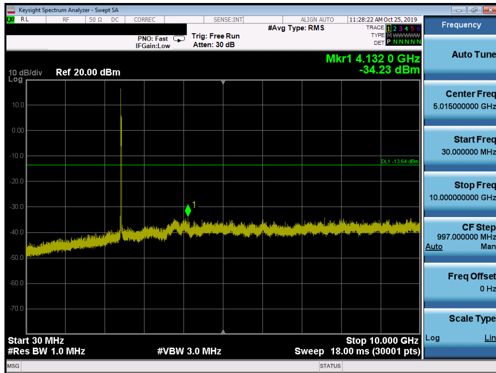
Plot 7-61. Conducted Spurious Plot SISO ANT2 (802.11ax OFDMA - 26 Tones - Ch. 6)
