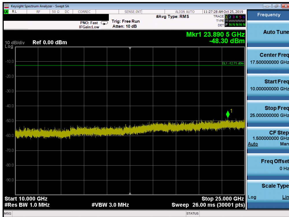
Plot 7-60. Conducted Spurious Plot SISO ANT2 (802.11ax OFDMA – 26 Tones – Ch. 1)
