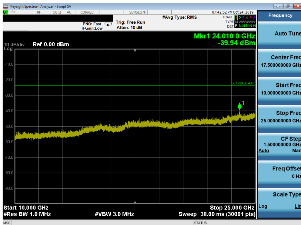
Plot 7-58. Conducted Spurious Plot SISO ANT1 (802.11ax OFDMA – 242 Tones – Ch. 11)
