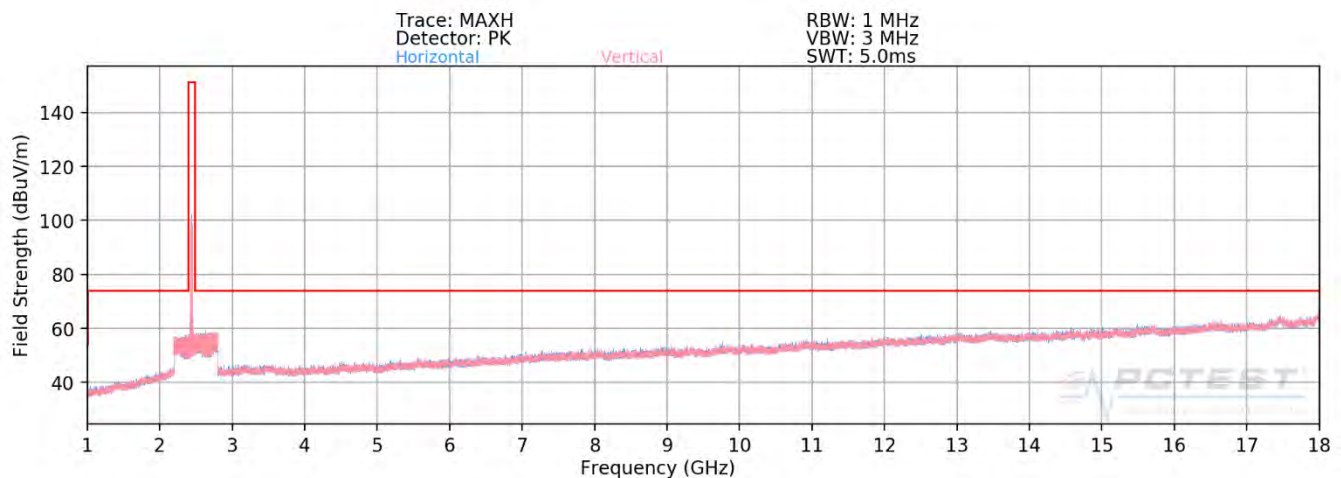
Plot 7-79. Radiated Spurious Plot above 1GHz SISO ANT2 (802.11ax OFDMA – 106 Tones – Ch. 6)
