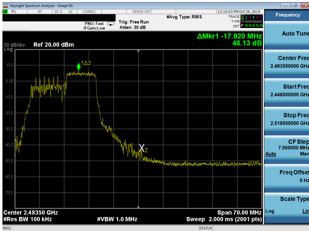
Plot 7-43. Band Edge Plot SISO ANT2 (802.11ax OFDMA – 106 Tones – Ch. 11)
