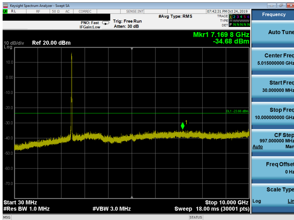
Plot 7-57. Conducted Spurious Plot SISO ANT1 (802.11ax OFDMA – 242 Tones – Ch. 11)
