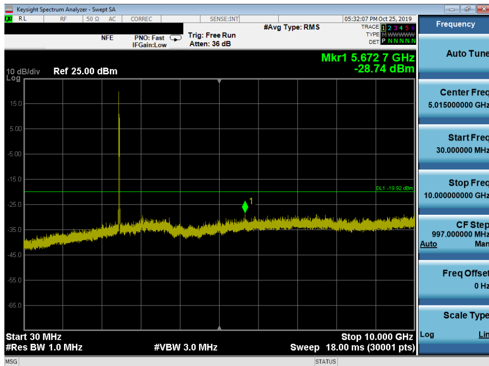
Plot 7-51. Conducted Spurious Plot SISO ANT1 (802.11ax OFDMA – 26 Tones – Ch. 11)
