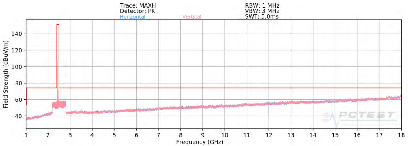
Plot 7-72. Radiated Spurious Plot above 1GHz SISO ANT1 (802.11ax OFDMA – 106 Tones – Ch. 6)
