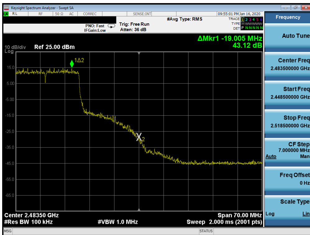
Plot 7-40. Band Edge Plot SISO ANT1 (802.11ax OFDMA – 242 Tones – Ch. 10)
