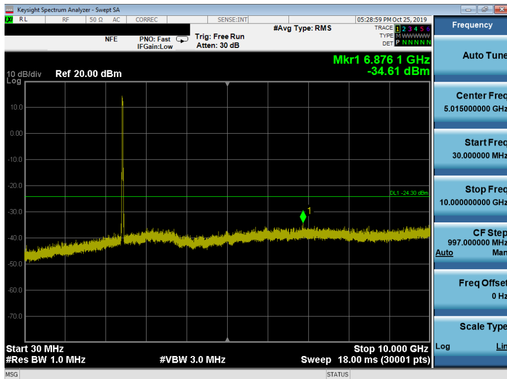
Plot 7-55. Conducted Spurious Plot SISO ANT1 (802.11ax OFDMA – 242 Tones – Ch. 6)
