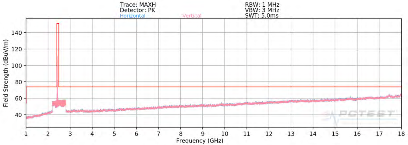
Plot 7-71. Radiated Spurious Plot above 1GHz SISO ANT1 (802.11ax OFDMA – 106 Tones – Ch. 1)
