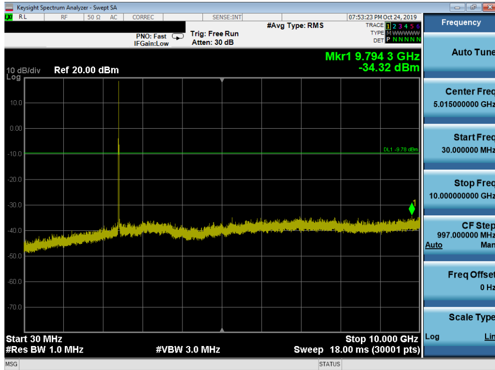
Plot 7-47. Conducted Spurious Plot SISO ANT1 (802.11ax OFDMA – 26 Tones – Ch. 1)
