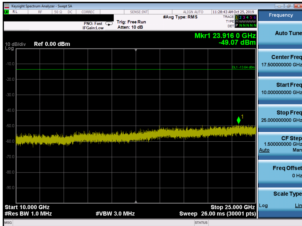
Plot 7-62. Conducted Spurious Plot SISO ANT2 (802.11ax OFDMA - 26 Tones - Ch. 6)
