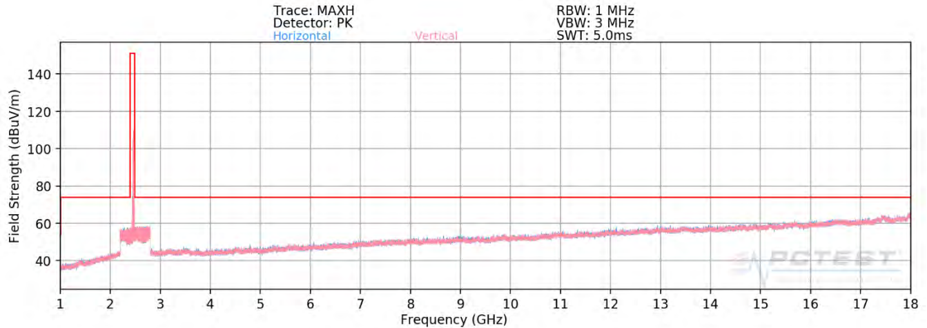
Plot 7-73. Radiated Spurious Plot above 1GHz SISO ANT1 (802.11ax OFDMA – 106 Tones – Ch. 11)
