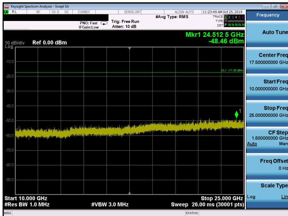
Plot 7-70. Conducted Spurious Plot SISO ANT2 (802.11ax OFDMA – 242 Tones – Ch. 11)
