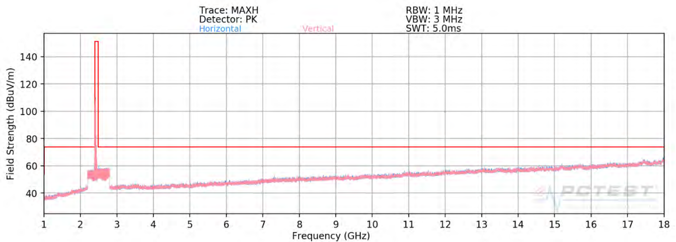
Plot 7-74. Radiated Spurious Plot above 1GHz SISO ANT1 (802.11ax OFDMA – 242 Tones – Ch. 1)
