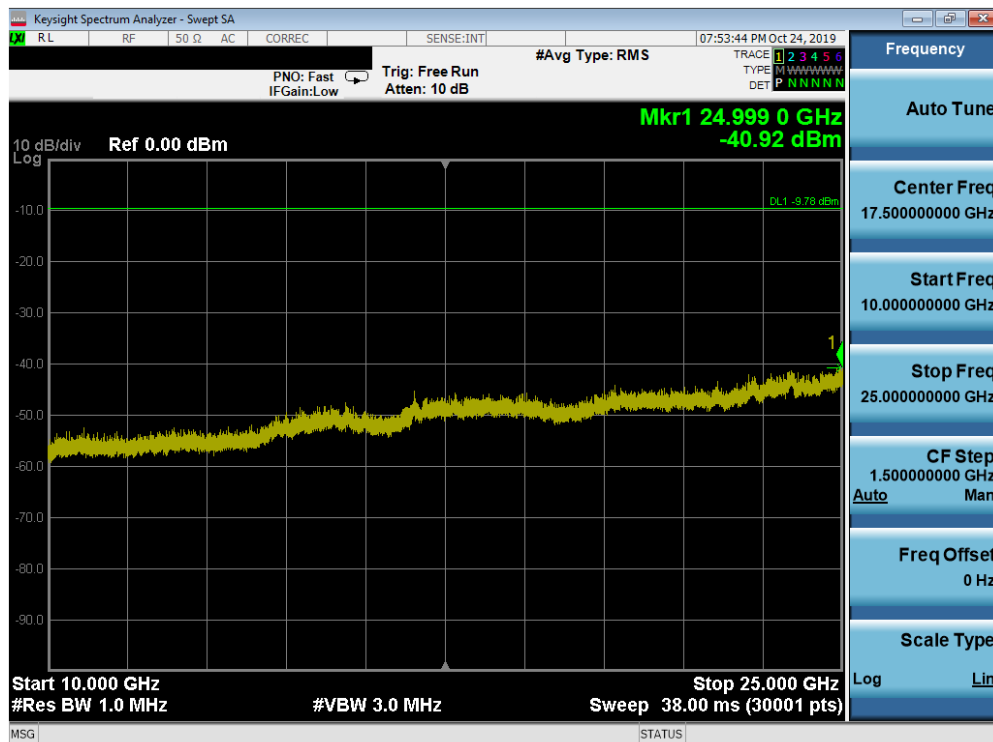
Plot 7-48. Conducted Spurious Plot SISO ANT1 (802.11ax OFDMA – 26 Tones – Ch. 1)
