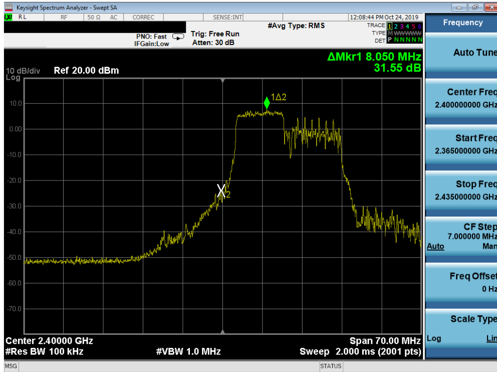
Plot 7-42. Band Edge Plot SISO ANT2 (802.11ax OFDMA – 106 Tones – Ch. 1)
