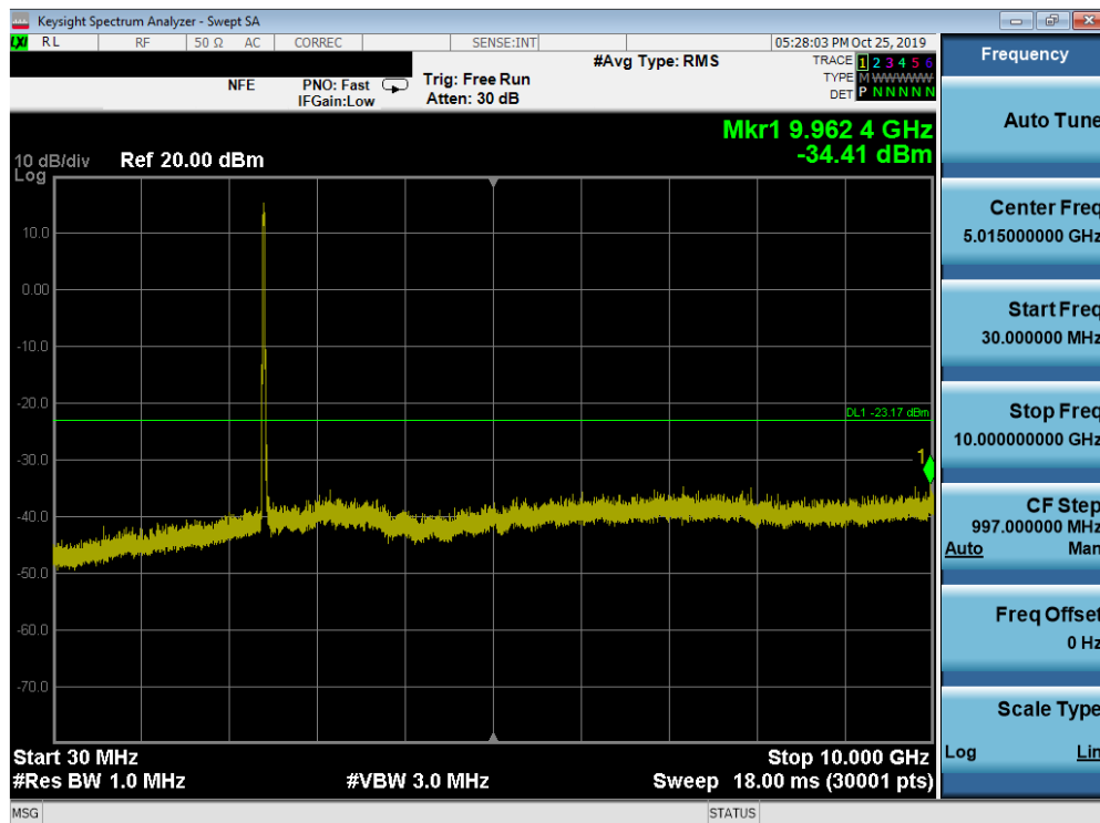
Plot 7-53. Conducted Spurious Plot SISO ANT1 (802.11ax OFDMA – 242 Tones – Ch. 1)
