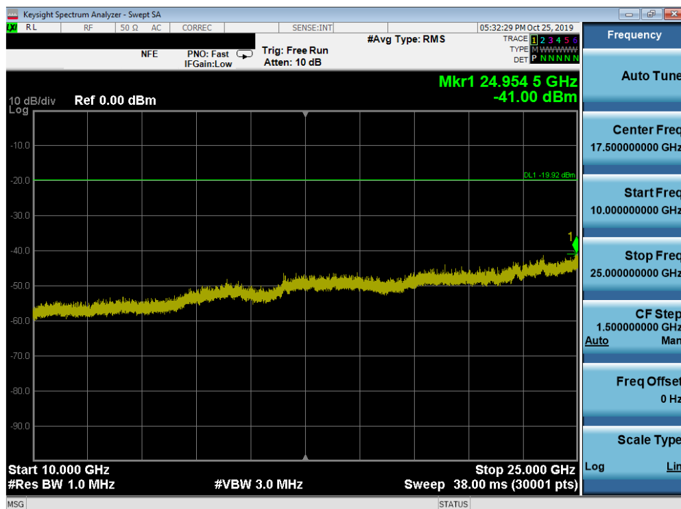
Plot 7-52. Conducted Spurious Plot SISO ANT1 (802.11ax OFDMA – 26 Tones – Ch. 11)
