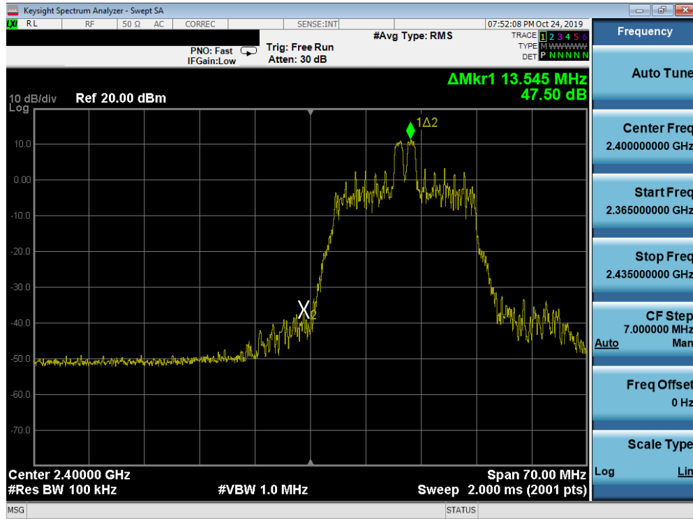
Plot 7-37. Band Edge Plot SISO ANT1 (802.11ax OFDMA – 26 Tones – Ch. 1)
