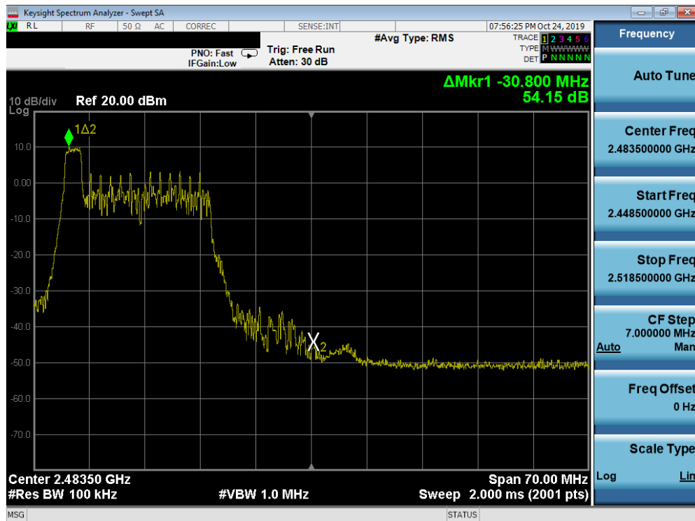
Plot 7-38. Band Edge Plot SISO ANT1 (802.11ax OFDMA – 26 Tones – Ch. 11)
