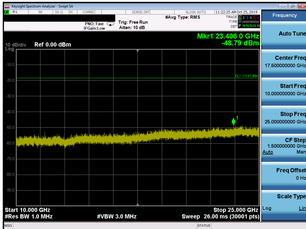
Plot 7-68. Conducted Spurious Plot SISO ANT2 (802.11ax OFDMA – 242 Tones – Ch. 6)
