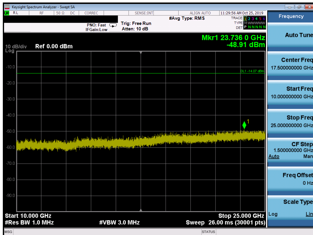
Plot 7-64. Conducted Spurious Plot SISO ANT2 (802.11ax OFDMA – 26 Tones – Ch. 11)
