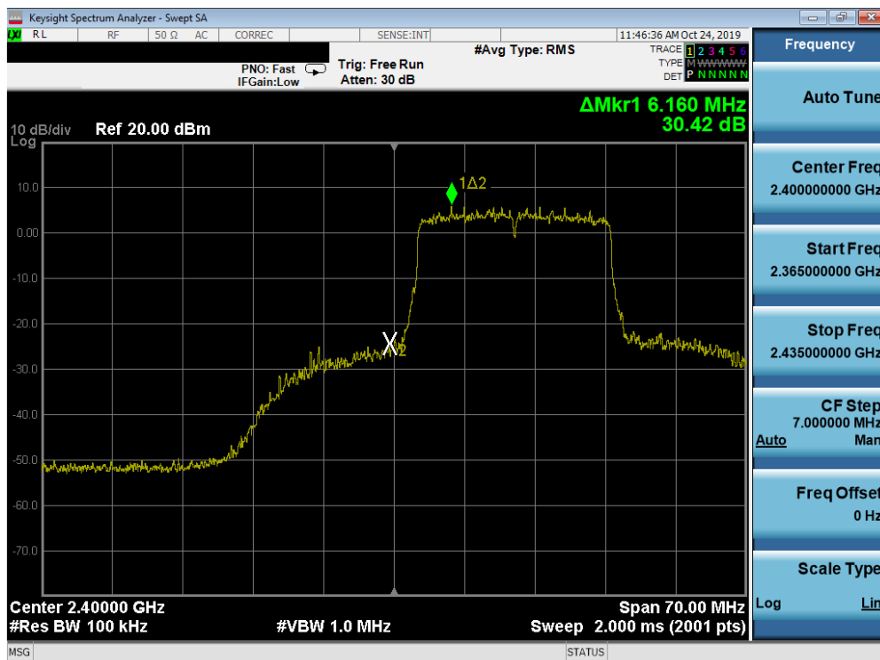
Plot 7-44. Band Edge Plot SISO ANT2 (802.11ax OFDMA – 242 Tones – Ch. 1)
