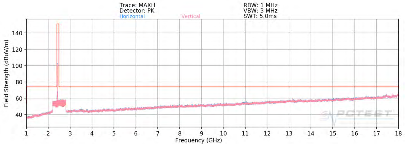
Plot 7-78. Radiated Spurious Plot above 1GHz SISO ANT2 (802.11ax OFDMA – 106 Tones – Ch. 1)
