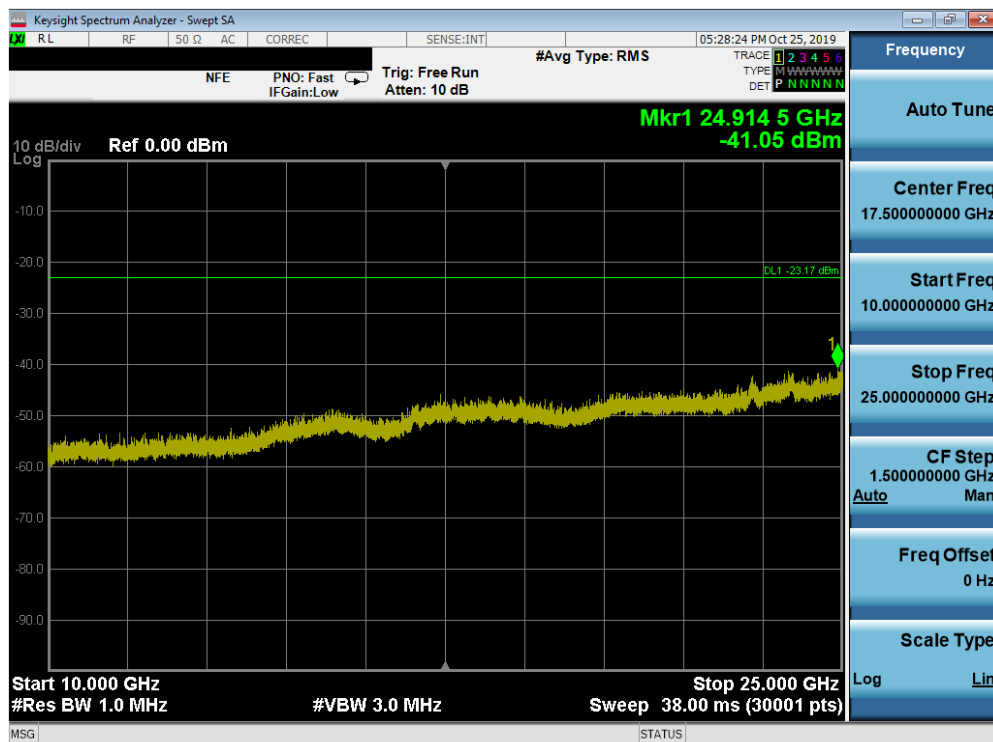
Plot 7-54. Conducted Spurious Plot SISO ANT1 (802.11ax OFDMA – 242 Tones – Ch. 1)
