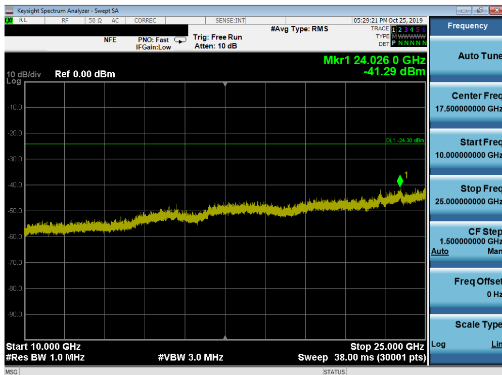
Plot 7-56. Conducted Spurious Plot SISO ANT1 (802.11ax OFDMA – 242 Tones – Ch. 6)
