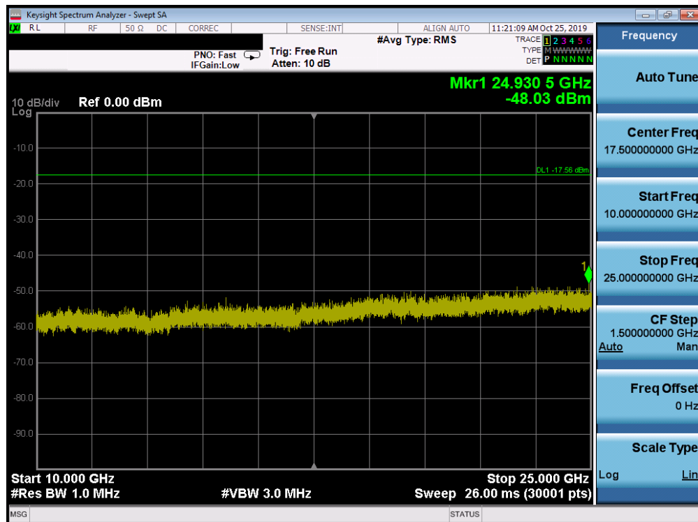
Plot 7-66. Conducted Spurious Plot SISO ANT2 (802.11ax OFDMA – 242 Tones – Ch. 1)
