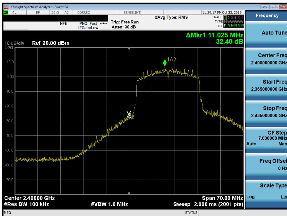
Plot 7-64. Band Edge Plot SISO ANT1 (802.11ax (2.4GHz) – Ch. 1)
