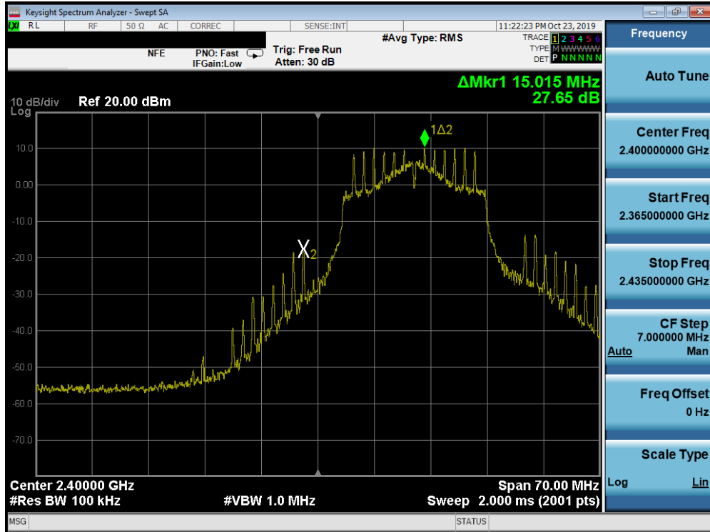
Plot 7-61. Band Edge Plot SISO ANT1 (802.11n (2.4GHz) – Ch. 1)
