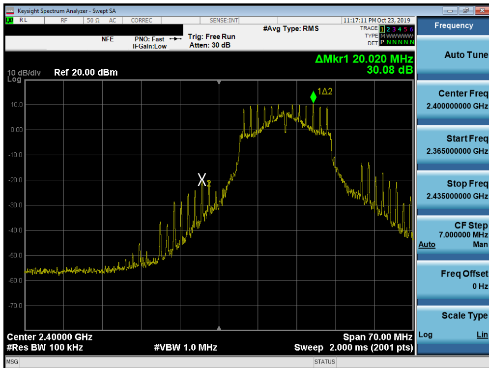
Plot 7-58. Band Edge Plot SISO ANT1 (802.11g- Ch. 1)
