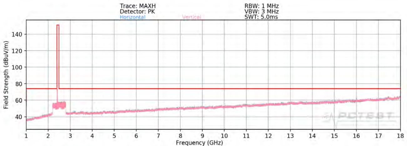
Plot 7-91. Radiated Spurious Plot above 1GHz SISO ANT1 (802.11b – Ch. 1)
