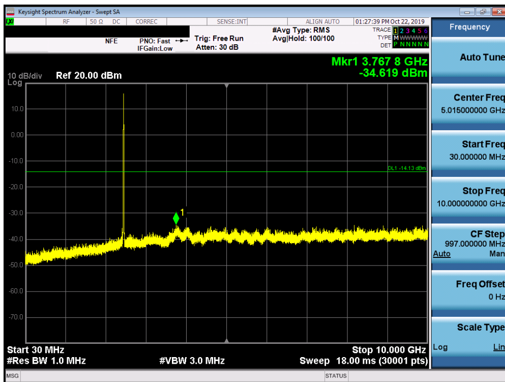
Plot 7-89. Conducted Spurious Plot SISO ANT2 (802.11b – Ch. 11)
