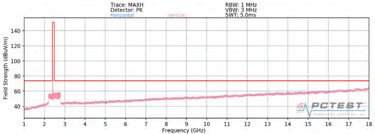
Plot 7-95. Radiated Spurious Plot above 1GHz SISO ANT2 (802.11b – Ch. 1)
