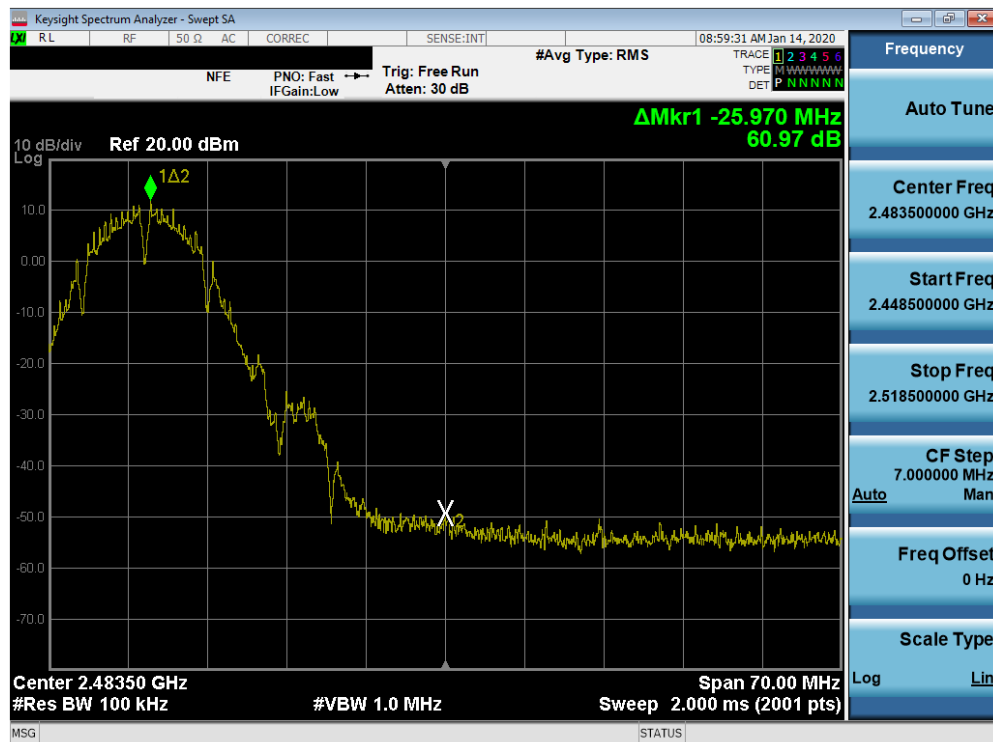
Plot 7-56. Band Edge Plot SISO ANT1 (802.11b - Ch. 10)
