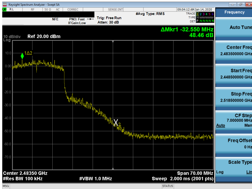
Plot 7-65. Band Edge Plot SISO ANT1 (802.11ax (2.4GHz) – Ch. 10)
