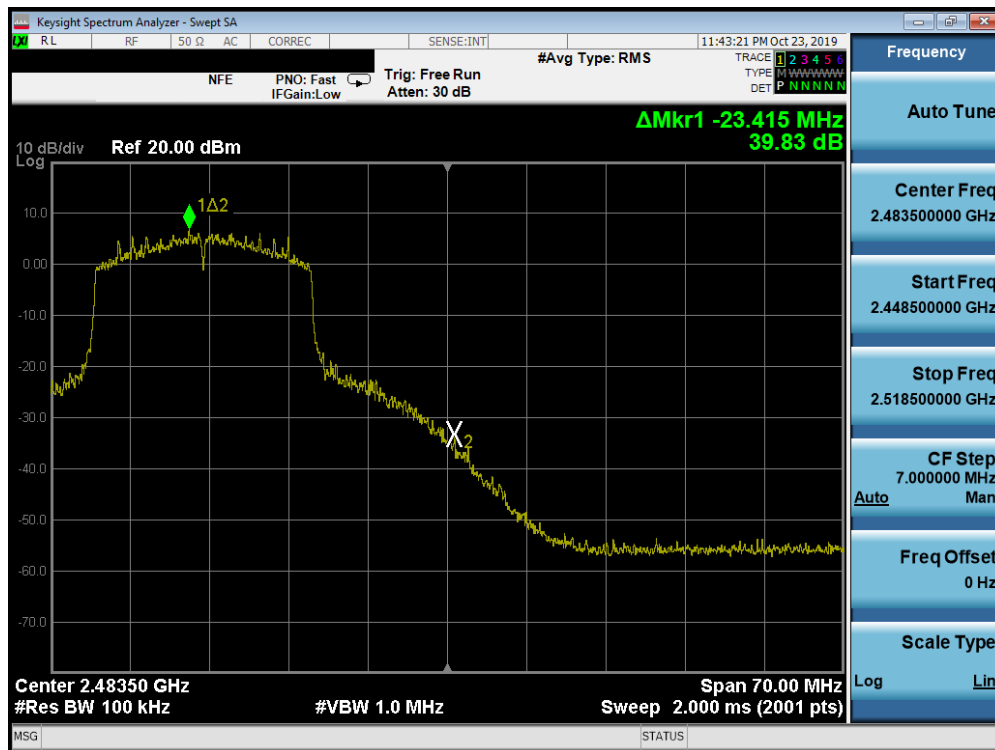
Plot 7-66. Band Edge Plot SISO ANT1 (802.11ax (2.4GHz) – Ch. 11)
