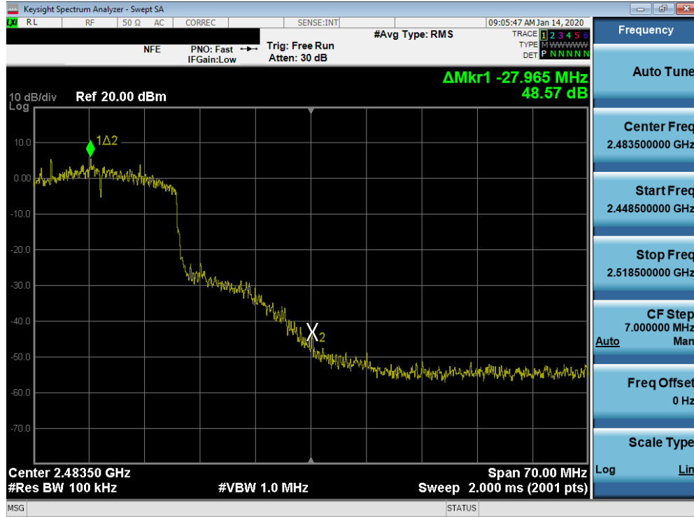
Plot 7-77. Band Edge Plot SISO ANT2 (802.11ax (2.4GHz) – Ch. 10)
