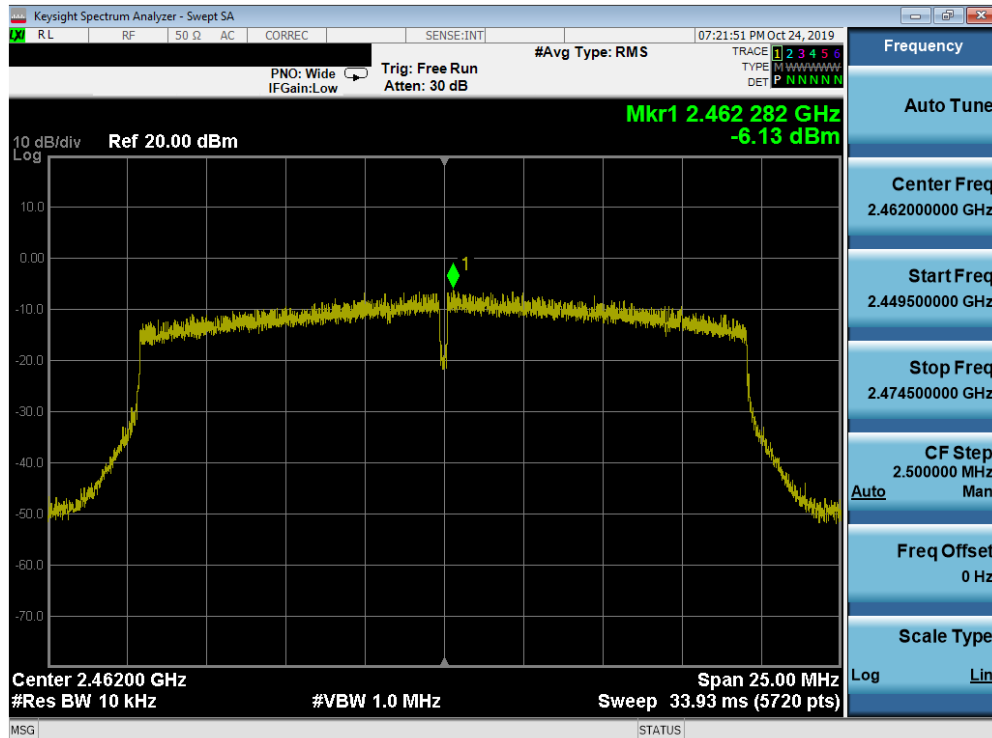
Plot 7-54. Power Spectral Density Plot MIMO ANT2 (802.11ax (2.4GHz) – Ch. 11)
