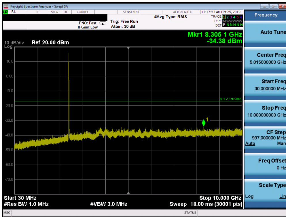
Plot 7-85. Conducted Spurious Plot SISO ANT2 (802.11b – Ch. 1)
