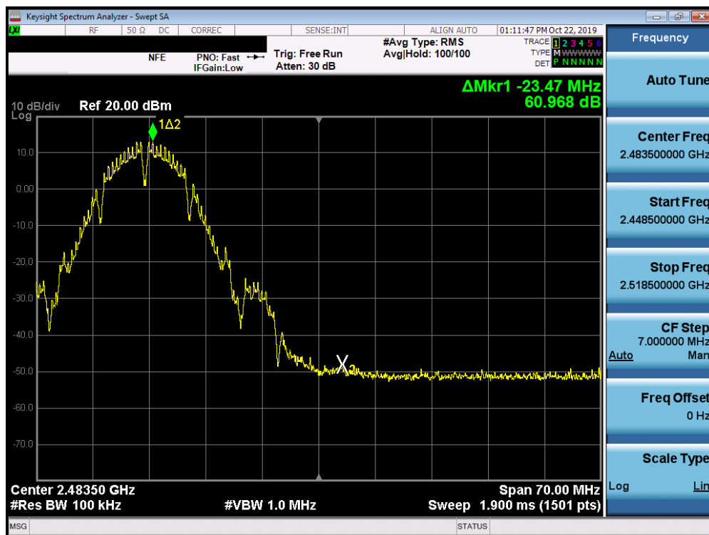
Plot 7-69. Band Edge Plot SISO ANT2 (802.11b – Ch. 11)
