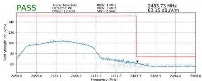
Plot 7-114. Radiated Restricted Upper Band Edge Measurement SISO ANT2 (Peak)
