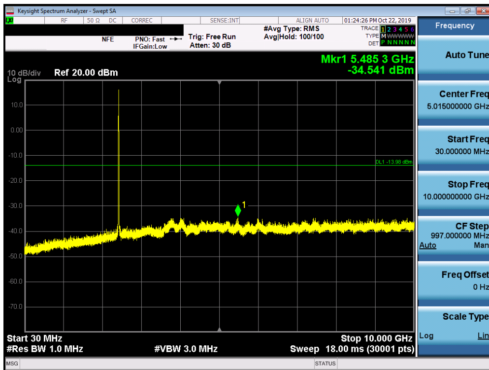
Plot 7-87. Conducted Spurious Plot SISO ANT2 (802.11b – Ch. 6)
