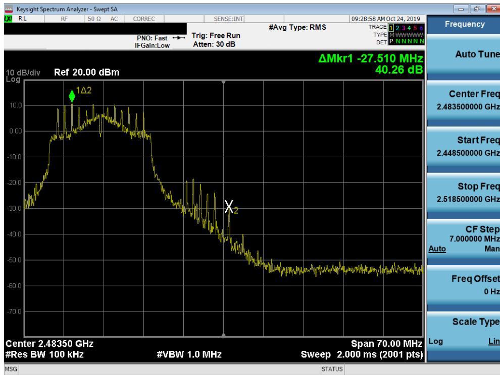
Plot 7-75. Band Edge Plot SISO ANT2 (802.11n (2.4GHz) – Ch. 11)
