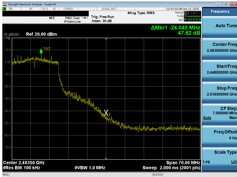
Plot 7-62. Band Edge Plot SISO ANT1 (802.11n (2.4GHz) – Ch. 10)
