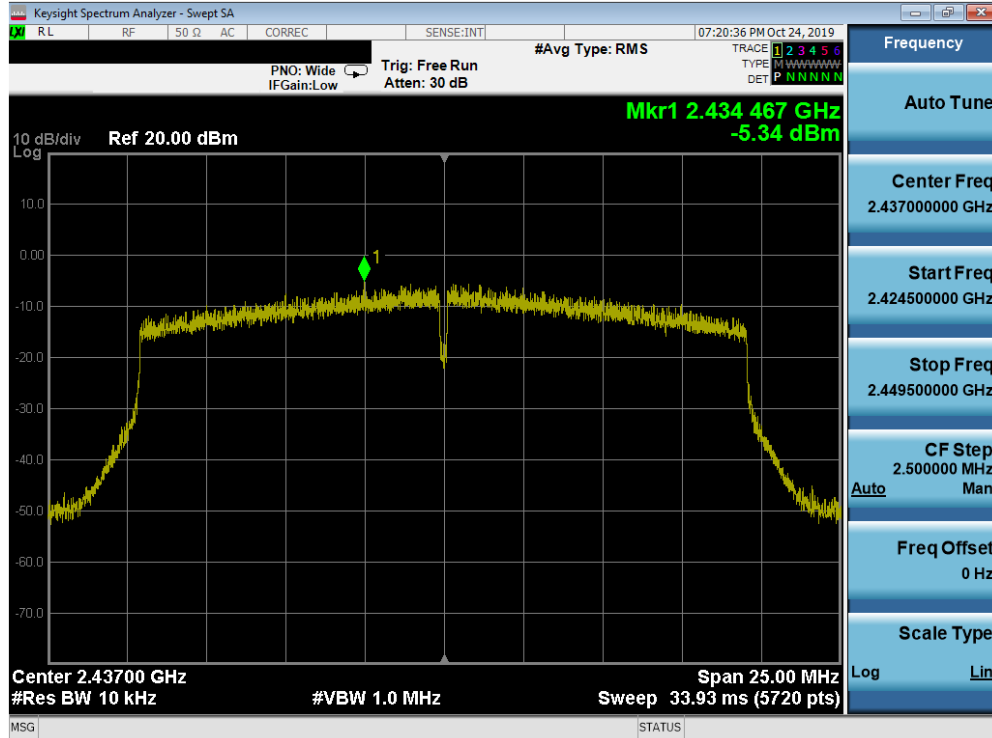
Plot 7-53. Power Spectral Density Plot MIMO ANT2 (802.11ax (2.4GHz) – Ch. 6)
