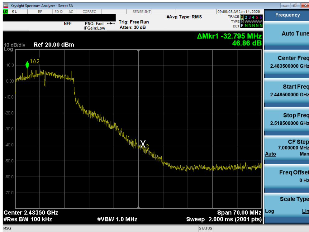
Plot 7-59. Band Edge Plot SISO ANT1 (802.11g – Ch. 10)
