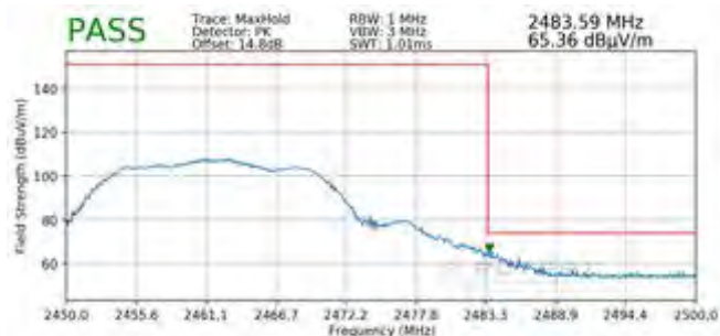
Plot 7-128. Radiated Restricted Band Edge Measurement MIMO with WCP (Peak)
