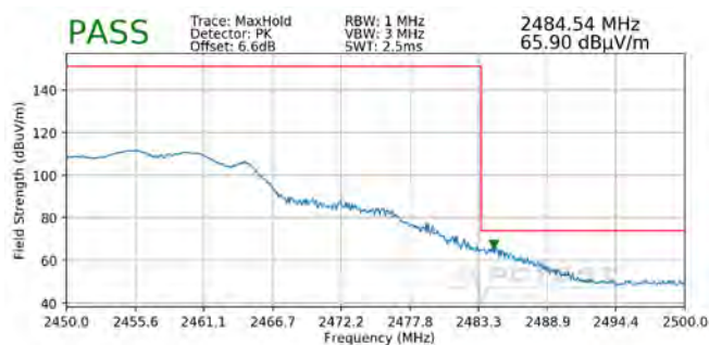
Plot 7-118. Radiated Restricted Upper Band Edge Measurement CDD (Peak)
