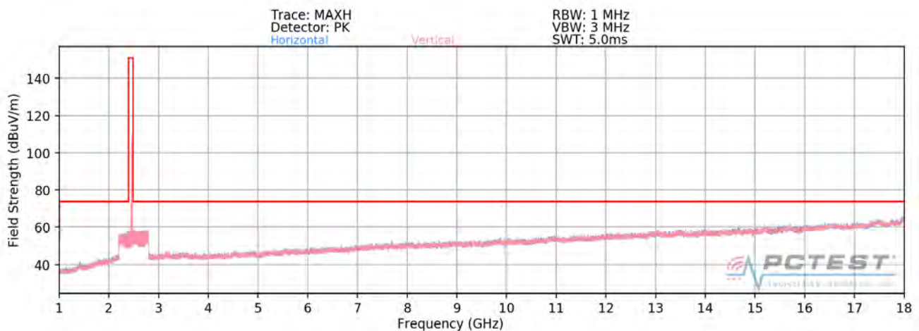
Plot 7-93. Radiated Spurious Plot above 1GHz SISO ANT1 (802.11b – Ch. 11)
