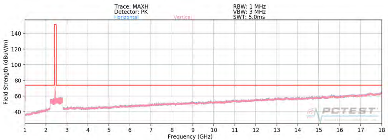
Plot 7-92. Radiated Spurious Plot above 1GHz SISO ANT1 (802.11b – Ch. 6)
