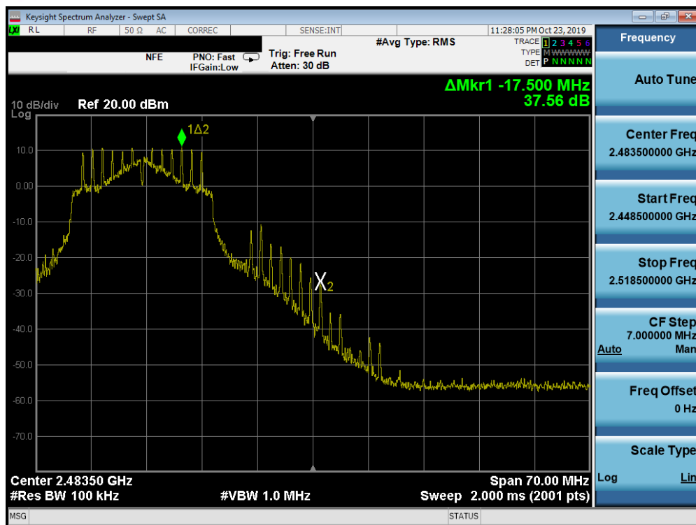
Plot 7-63. Band Edge Plot SISO ANT1 (802.11n (2.4GHz) – Ch. 11)
