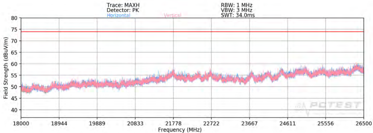
Plot 7-94. Radiated Spurious Plot above 18GHz SISO ANT1
