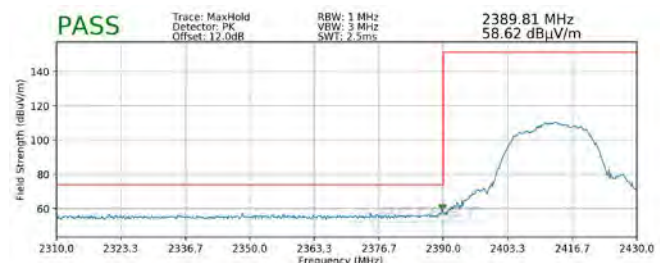
Plot 7-104. Radiated Restricted Lower Band Edge Measurement SISO ANT1 (Peak)
