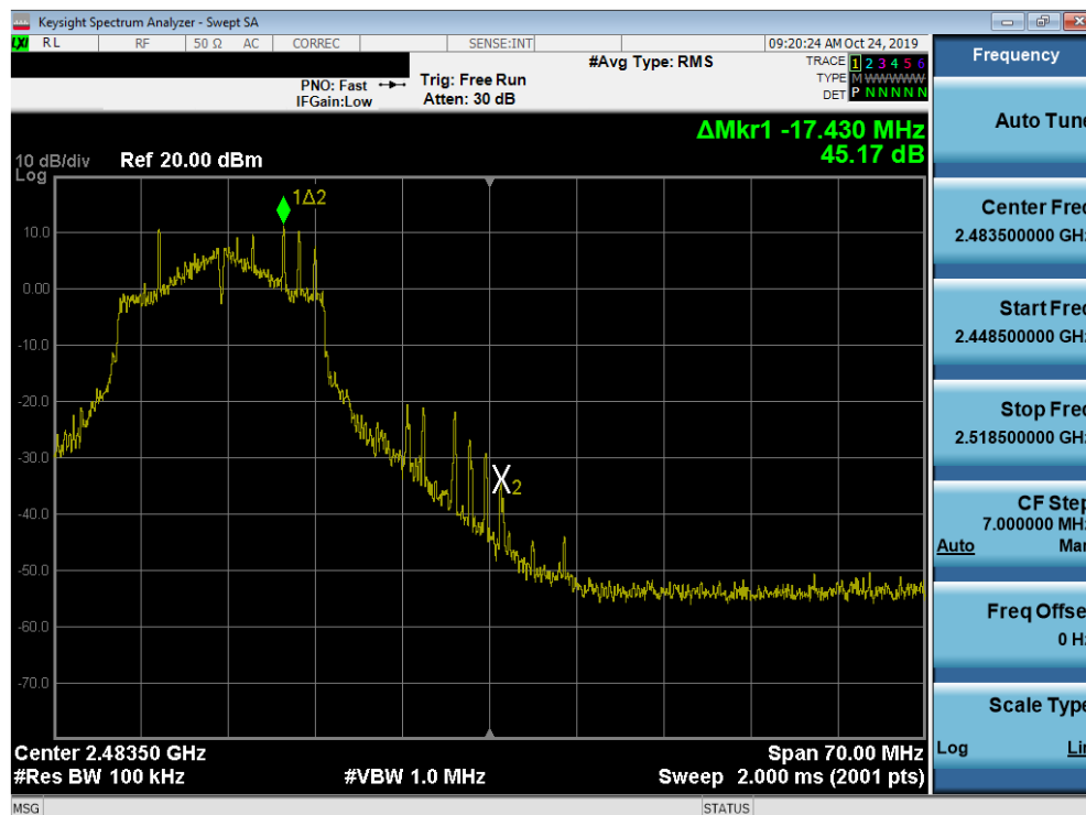
Plot 7-72. Band Edge Plot SISO ANT2 (802.11g – Ch. 11)
