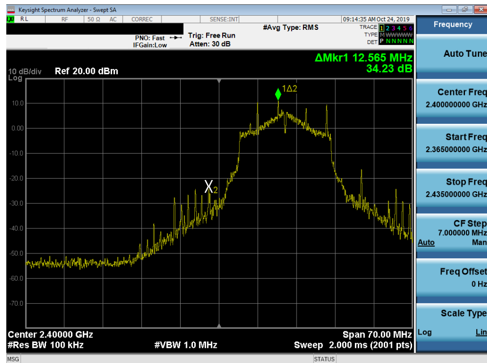
Plot 7-70. Band Edge Plot SISO ANT2 (802.11g- Ch. 1)
