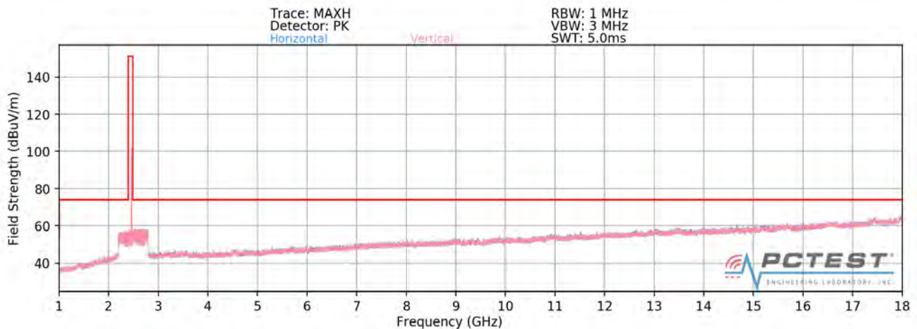
Plot 7-97. Radiated Spurious Plot above 1GHz SISO ANT2 (802.11b – Ch. 11)
