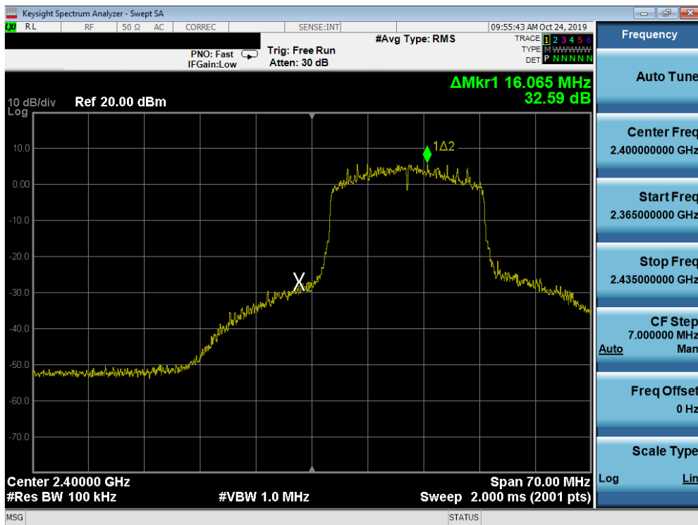
Plot 7-76. Band Edge Plot SISO ANT2 (802.11ax (2.4GHz) – Ch. 1)
