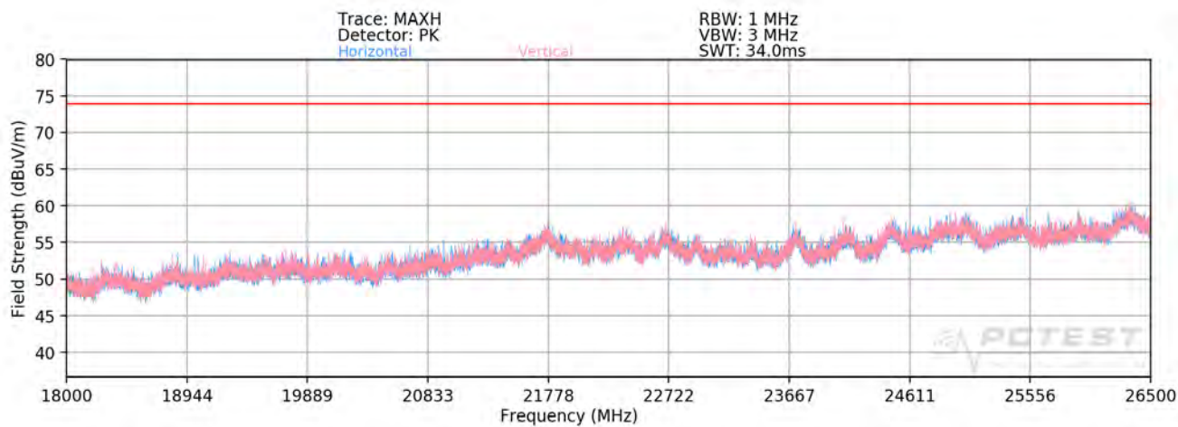
Plot 7-98. Radiated Spurious Plot above 18GHz SISO ANT2
