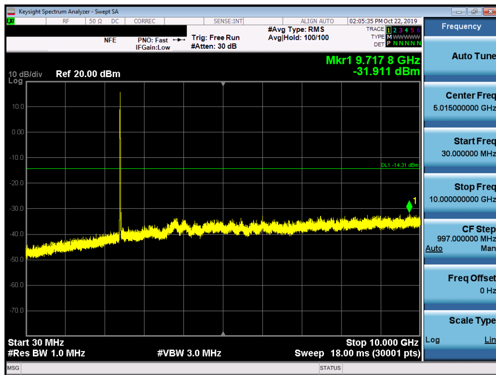
Plot 7-79. Conducted Spurious Plot SISO ANT1 (802.11b – Ch. 1)
