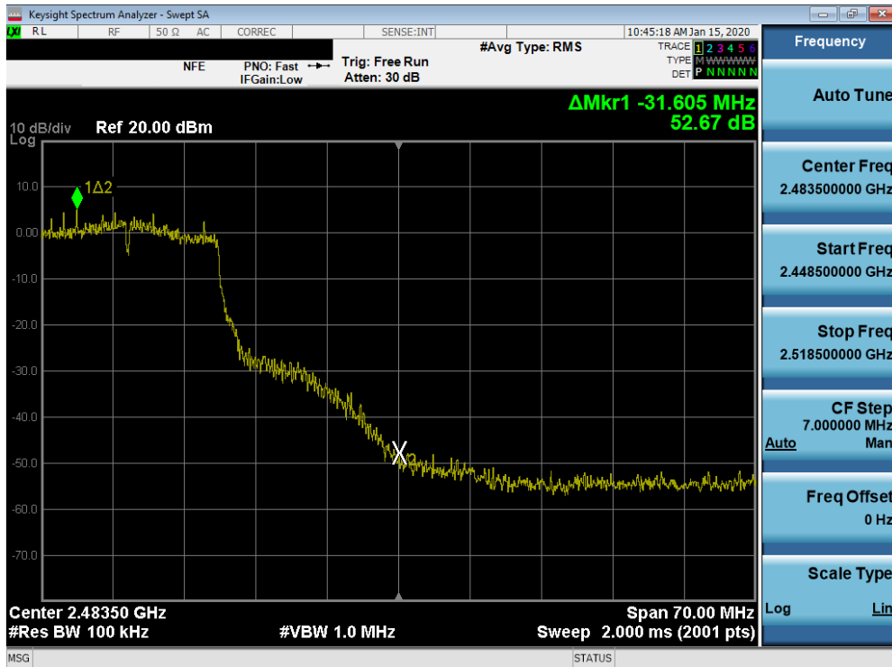
Plot 7-74. Band Edge Plot SISO ANT2 (802.11n (2.4GHz) – Ch. 10)
