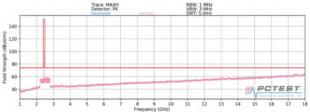
Plot 7-96. Radiated Spurious Plot above 1GHz SISO ANT2 (802.11b – Ch. 6)
