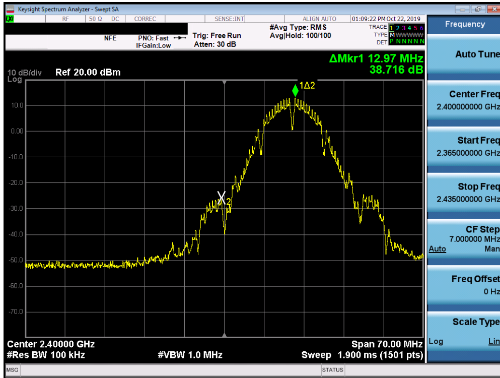
Plot 7-67. Band Edge Plot SISO ANT2 (802.11b - Ch. 1)
