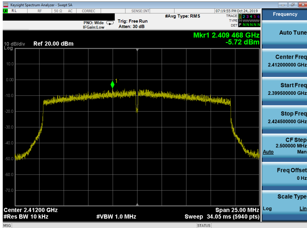
Plot 7-52. Power Spectral Density Plot MIMO ANT2 (802.11ax (2.4GHz) – Ch. 1)
