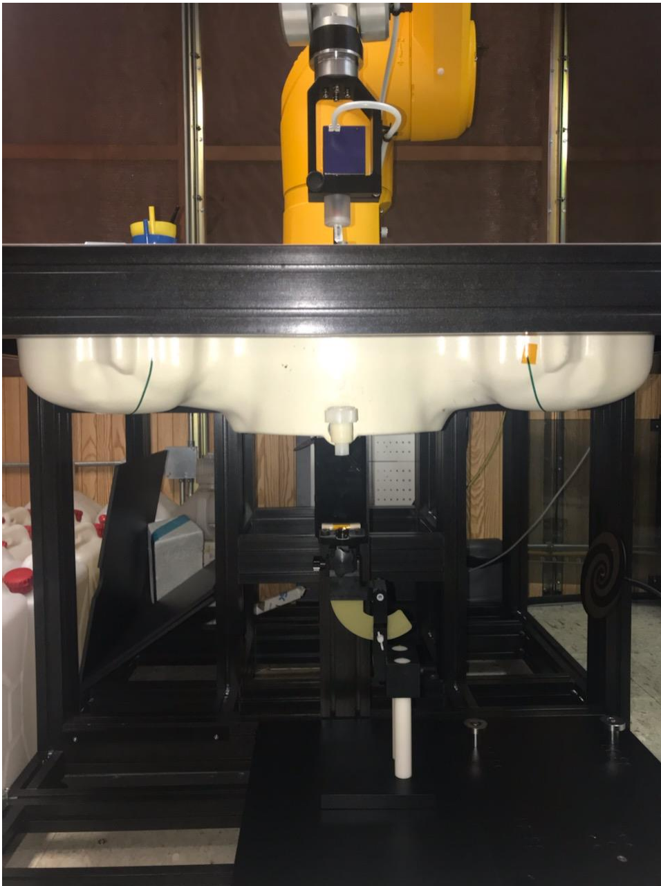
Figure 7-1 SAR measurement setup
