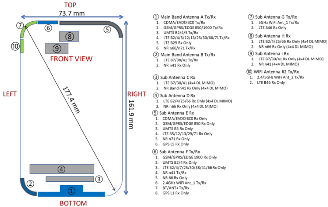
Figure E-1 DUT Antenna Locations
