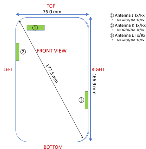
Figure 1: Location of mmW antenna modules looking from front of the DUT
