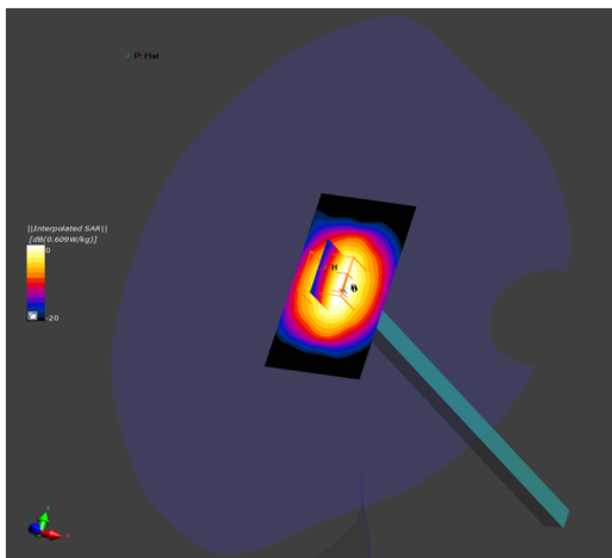
Figure C-4 SAR measurement system verification plot for 2300MHz performed on 1/13/2020. Input power = 10.0mW.
