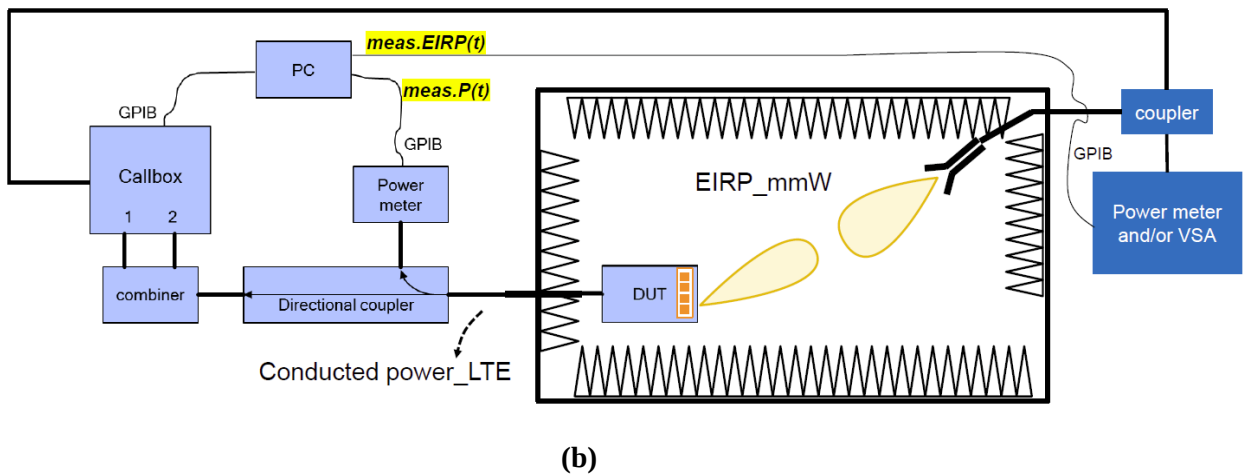
Figure 8-1 mmW NR radiated power measurement setup (see Appendix E for missing figures)
