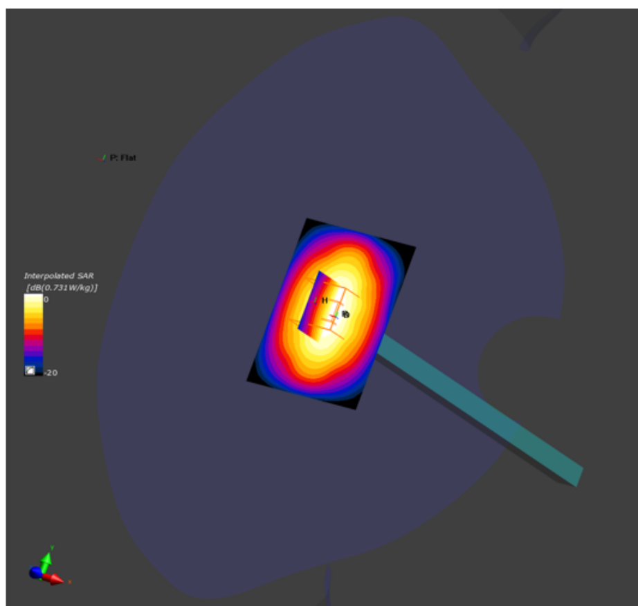
Figure C-2 SAR measurement system verification plot for 1800MHz performed on 1/8/2020. Input power = 10.0mW.
