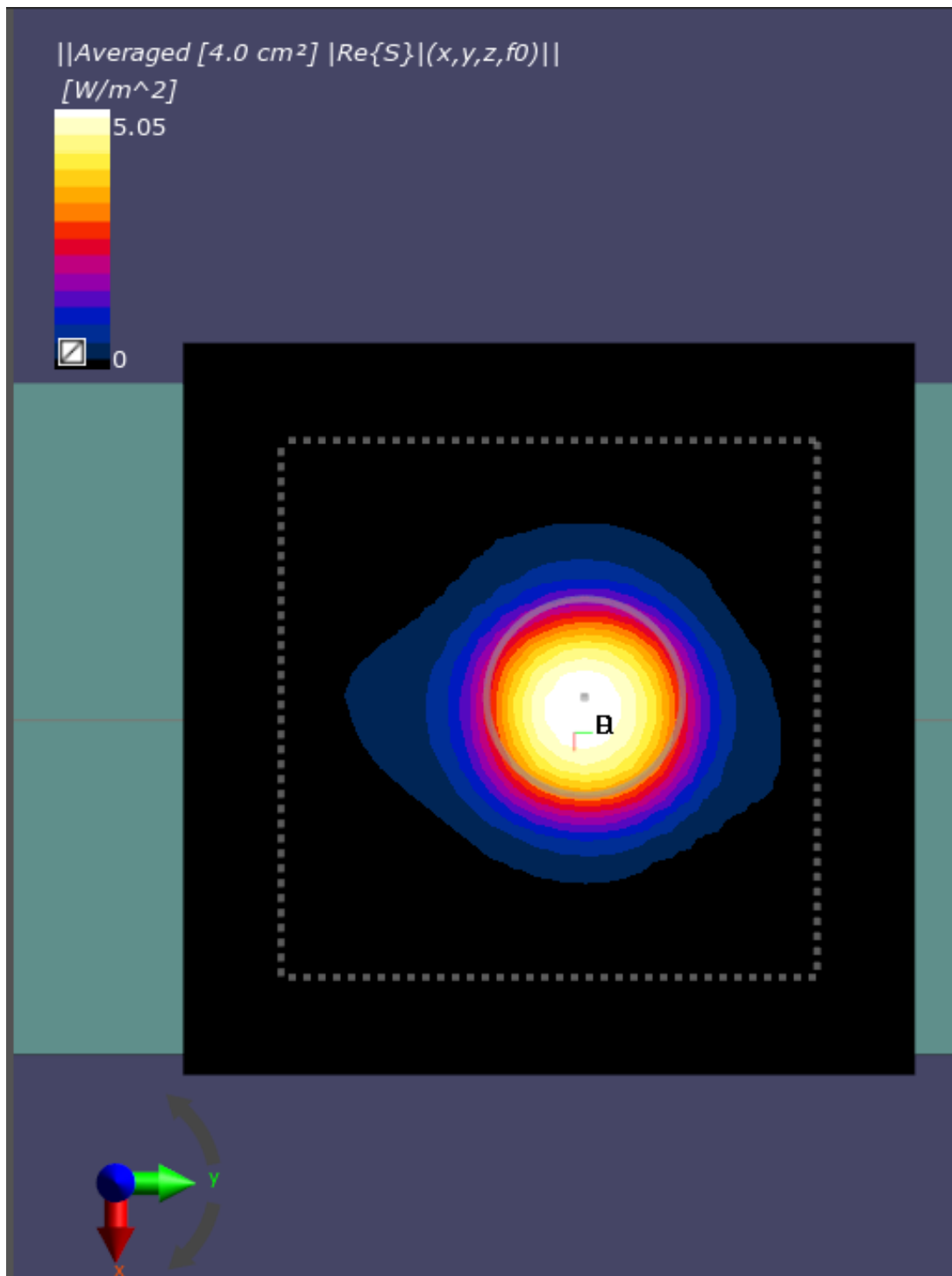
Figure 8-2: 4cm 2 -averaged power density distribution measured at input.power.limit of 3.1dBm on the back surface for n261 beam 26
