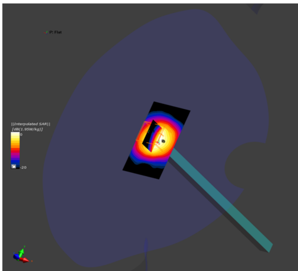
Figure C-3 SAR measurement system verification plot for 3700MHz performed on 01/08/2020. Input power = 10.0mW.
