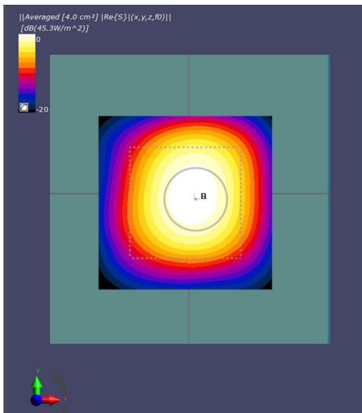
Figure C-6 4cm 2 PD for source validation on 1/17/2020
