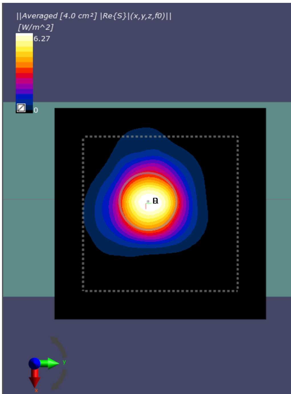
Figure 8-3: 4cm 2 -averaged power density distribution measured at target power of 4.7dBm on the back surface for n260 beam 41
