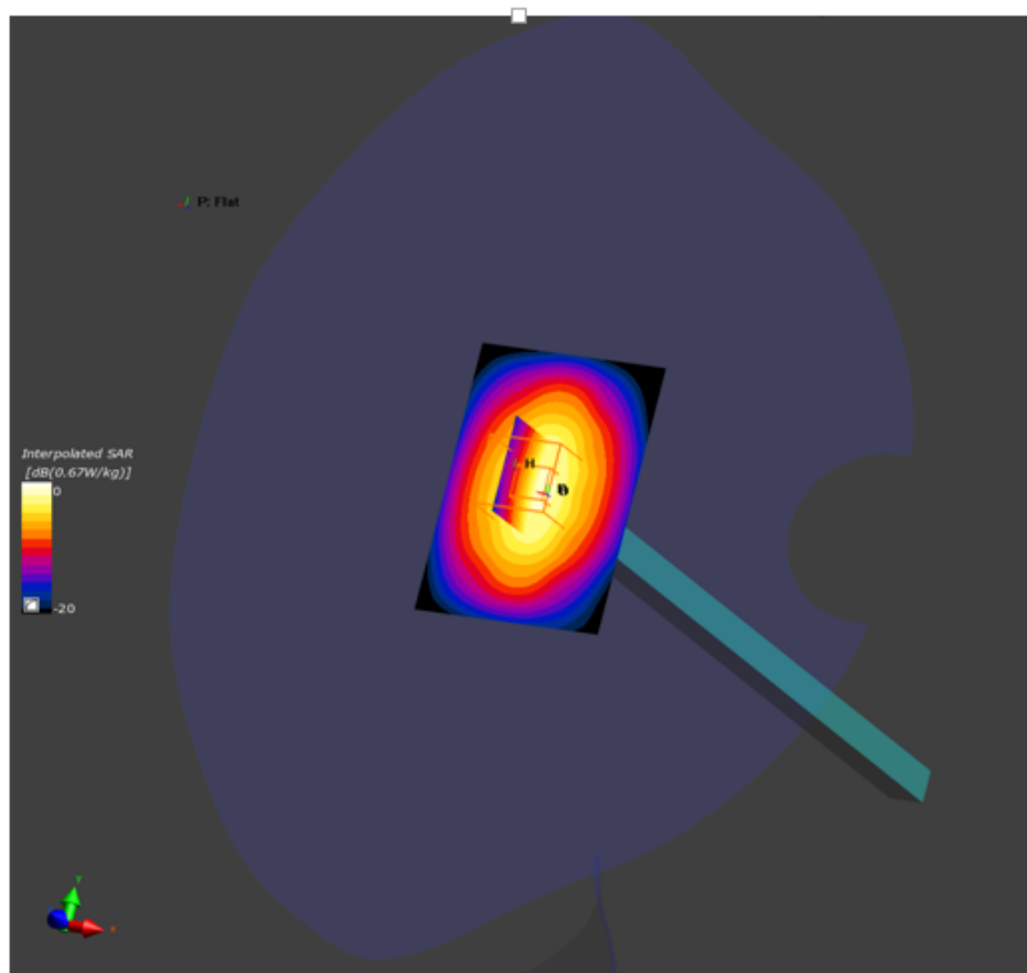
Figure C-5 SAR measurement system verification plot for 1800MHz performed on 2/2/2020. Input power = 10.0mW.
