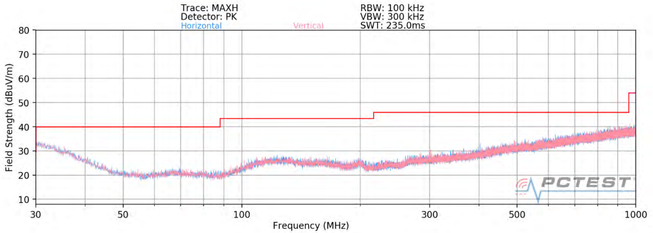
Plot 7-125. Radiated Spurious Plot below 1GHz MIMO (52 Tones)
