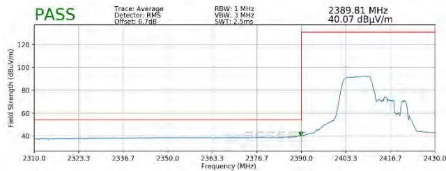
Plot 7-105. Radiated Restricted Lower Band Edge Measurement SISO ANT2 (Average – 106 Tones)
