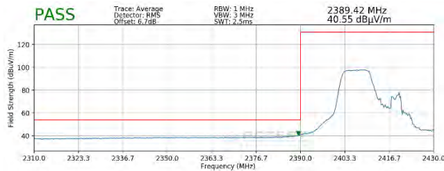
Plot 7-115. Radiated Restricted Lower Band Edge Measurement MIMO (Average – 106 Tones)
