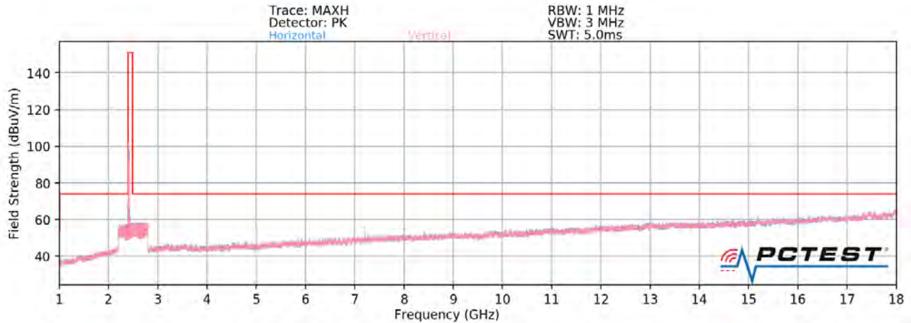
Plot 7-79. Radiated Spurious Plot above 1GHz SISO ANT2 (802.11ax OFDMA – 26 Tones – Ch. 1)
