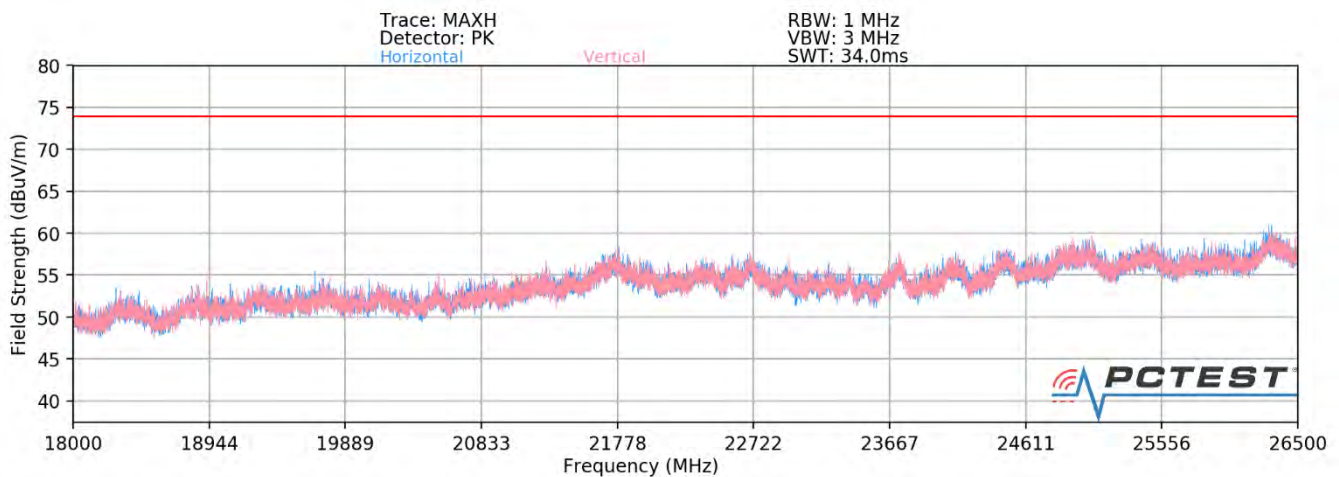
Plot 7-78. Radiated Spurious Plot above 18GHz SISO ANT1 (802.11ax OFDMA – 242 Tones)
