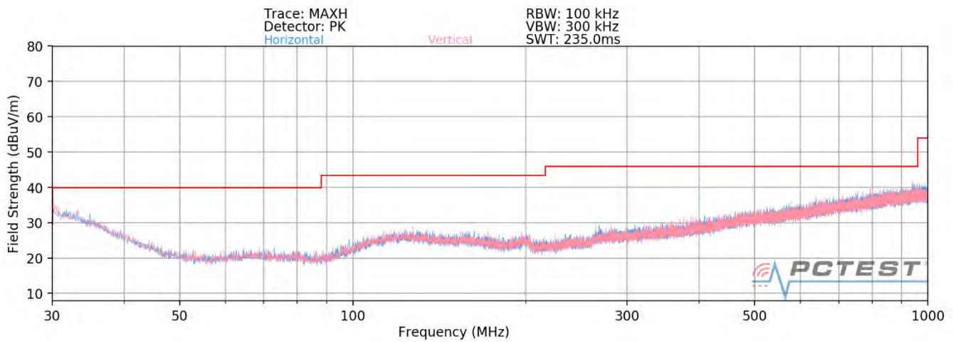
Plot 7-126. Radiated Spurious Plot below 1GHz MIMO (242 Tones)
