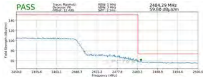
Plot 7-122. Radiated Restricted Upper Band Edge Measurement MIMO (Peak – 242 Tones)
