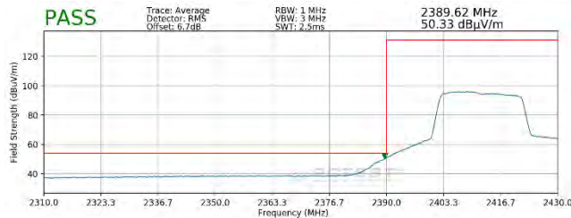
Plot 7-99. Radiated Restricted Lower Band Edge Measurement SISO ANT1 (Average – 242 Tones)
