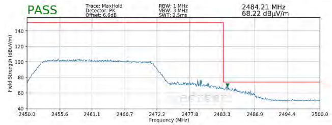
Plot 7-114. Radiated Restricted Upper Band Edge Measurement SISO ANT2 (Peak – 242 Tones)
