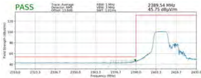
Plot 7-95. Radiated Restricted Lower Band Edge Measurement SISO ANT1 (Average – 106 Tones)
