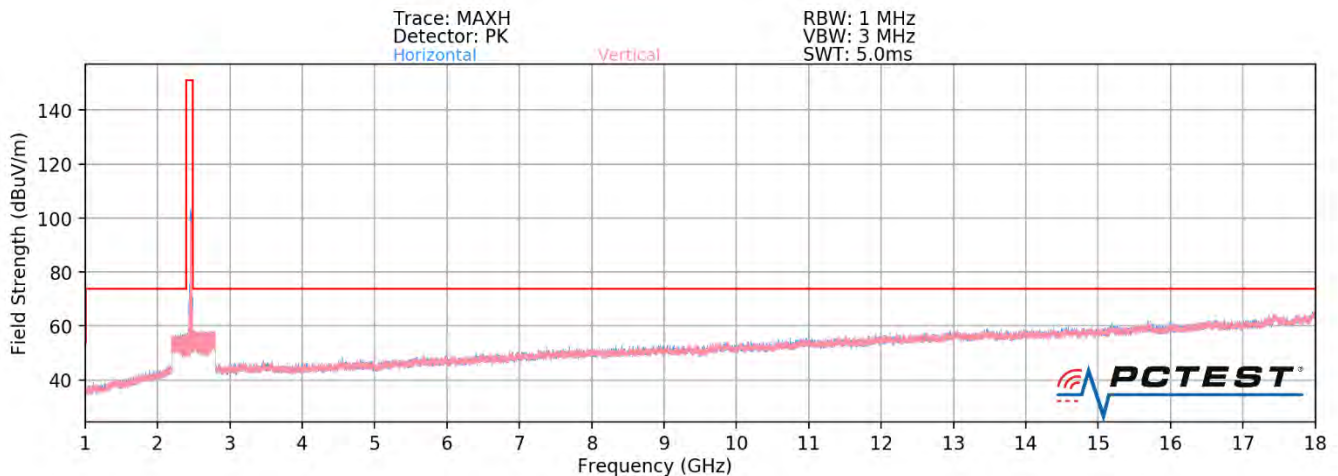
Plot 7-84. Radiated Spurious Plot above 1GHz SISO ANT2 (802.11ax OFDMA – 242 Tones – Ch. 11)
