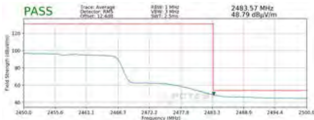
Plot 7-101. Radiated Restricted Upper Band Edge Measurement SISO ANT1 (Average – 242 Tones)
