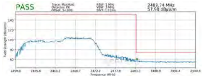
Plot 7-108. Radiated Restricted Upper Band Edge Measurement SISO ANT2 (Peak – 106 Tones)
