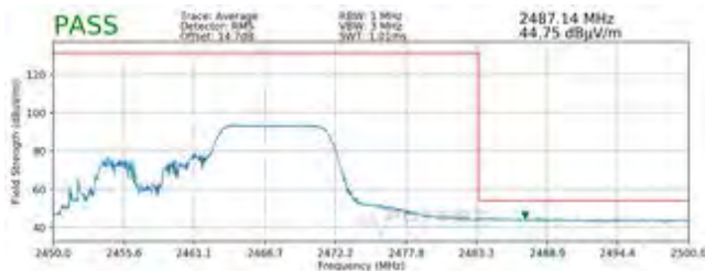
Plot 7-107. Radiated Restricted Upper Band Edge Measurement SISO ANT2 (Average – 106 Tones)
