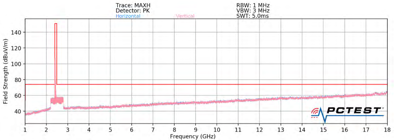
Plot 7-90. Radiated Spurious Plot above 1GHz MIMO (802.11ax OFDMA – 242 Tones – Ch. 1)
