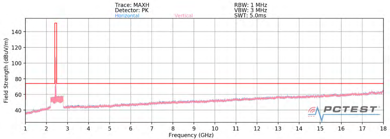
Plot 7-75. Radiated Spurious Plot above 1GHz SISO ANT1 (802.11ax OFDMA – 26T Tones – Ch. 6)
