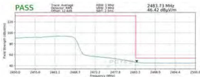
Plot 7-111. Radiated Restricted Upper Band Edge Measurement SISO ANT2 (Average – 242 Tones)
