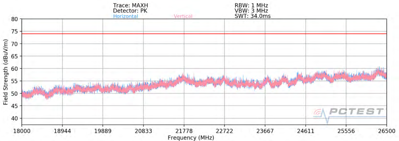
Plot 7-94. Radiated Spurious Plot above 18GHz MIMO (802.11ax OFDMA – 242 Tones)
