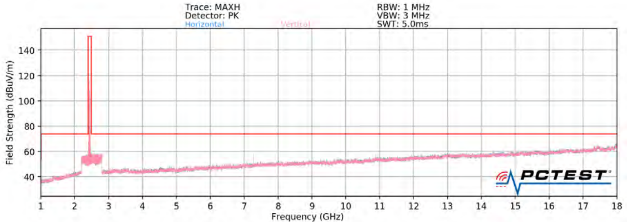
Plot 7-88. Radiated Spurious Plot above 1GHz MIMO (802.11ax OFDMA – 106 Tones – Ch. 6)
