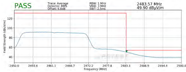
Plot 7-113. Radiated Restricted Upper Band Edge Measurement SISO ANT2 (Average – 242 Tones)
