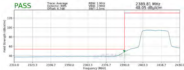
Plot 7-119. Radiated Restricted Lower Band Edge Measurement MIMO (Average – 242 Tones)
