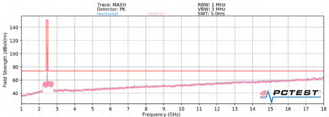
Plot 7-81. Radiated Spurious Plot above 1GHz SISO ANT2 (802.11ax OFDMA – 26 Tones – Ch. 11)
