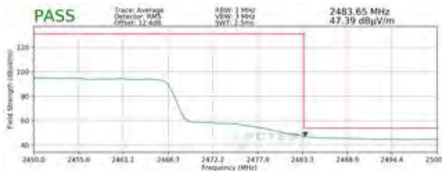
Plot 7-121. Radiated Restricted Upper Band Edge Measurement MIMO (Average – 242 Tones)
