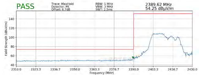
Plot 7-116. Radiated Restricted Lower Band Edge Measurement MIMO (Peak – 106 Tones)
