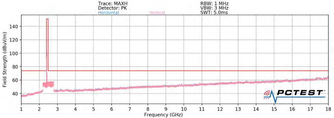
Plot 7-82. Radiated Spurious Plot above 1GHz SISO ANT2 (802.11ax OFDMA – 242 Tones – Ch. 1)
