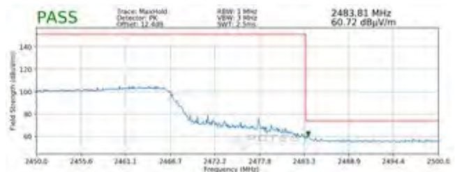
Plot 7-112. Radiated Restricted Upper Band Edge Measurement SISO ANT2 (Peak – 242 Tones)
