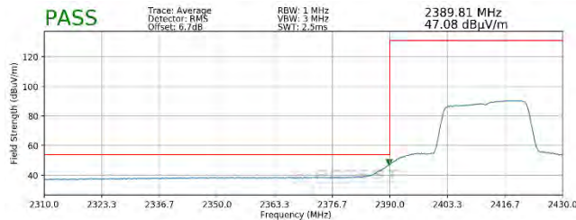
Plot 7-109. Radiated Restricted Lower Band Edge Measurement SISO ANT2 (Average – 242 Tones)
