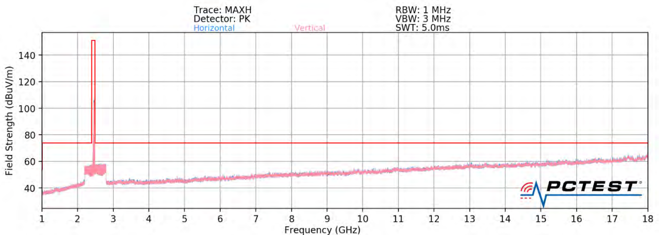
Plot 7-92. Radiated Spurious Plot above 1GHz MIMO (802.11ax OFDMA – 242 Tones – Ch. 11)
