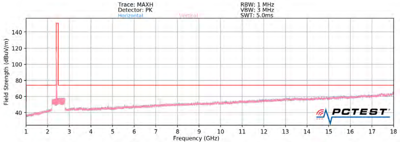
Plot 7-87. Radiated Spurious Plot above 1GHz MIMO (802.11ax OFDMA – 106 Tones – Ch. 1)
