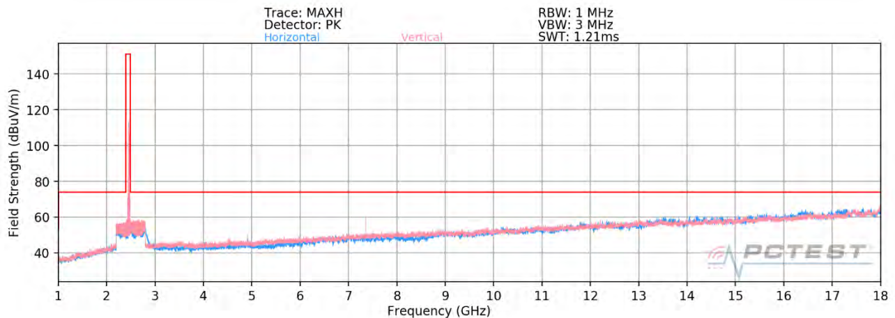
Plot 7-89. Radiated Spurious Plot above 1GHz MIMO (802.11ax OFDMA – 106 Tones – Ch. 11)
