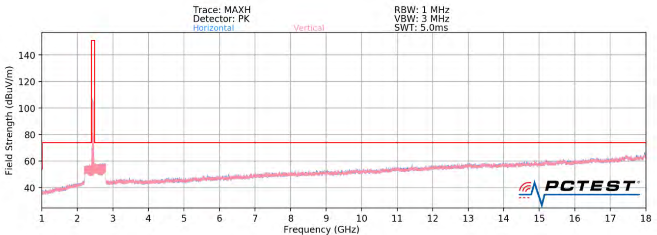
Plot 7-91. Radiated Spurious Plot above 1GHz MIMO (802.11ax OFDMA – 242 Tones – Ch. 6)
