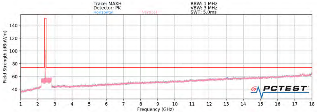
Plot 7-80. Radiated Spurious Plot above 1GHz SISO ANT2 (802.11ax OFDMA – 26 Tones – Ch. 6)
