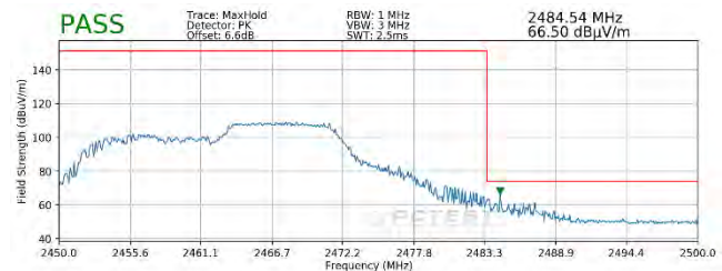
Plot 7-98. Radiated Restricted Upper Band Edge Measurement SISO ANT1 (Peak – 106 Tones)
