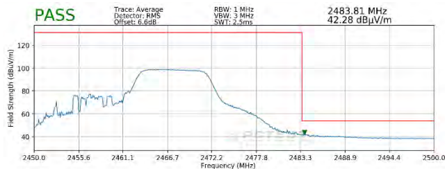
Plot 7-97. Radiated Restricted Upper Band Edge Measurement SISO ANT1 (Average – 106 Tones)
