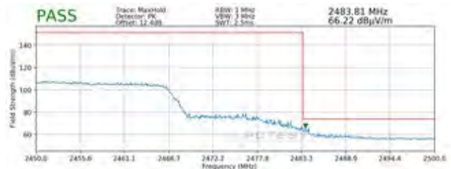
Plot 7-102. Radiated Restricted Upper Band Edge Measurement SISO ANT1 (Peak – 242 Tones)
