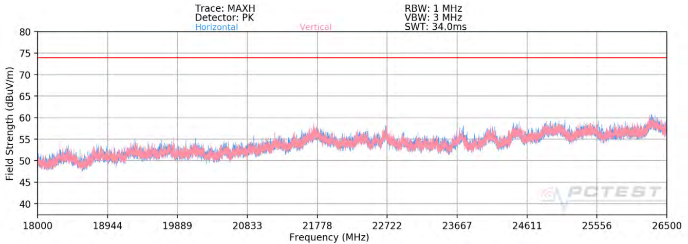
Plot 7-93. Radiated Spurious Plot above 18GHz MIMO (802.11ax OFDMA – 52 Tones)
