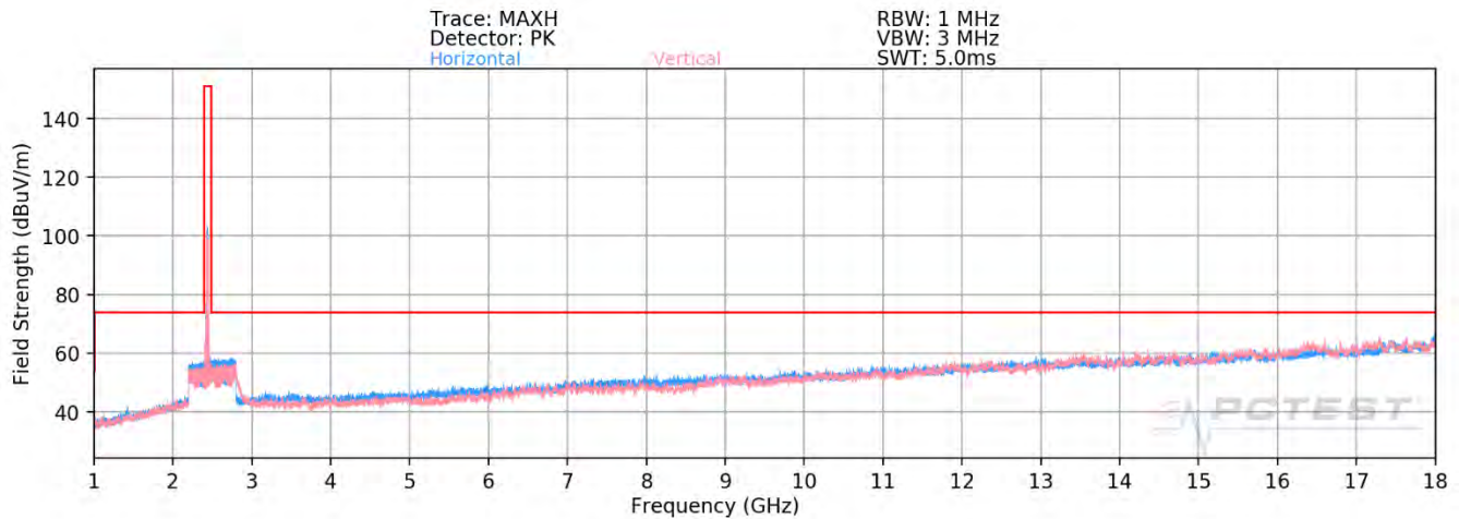
Plot 7-83. Radiated Spurious Plot above 1GHz SISO ANT2 (802.11ax OFDMA – 242 Tones – Ch. 6)
