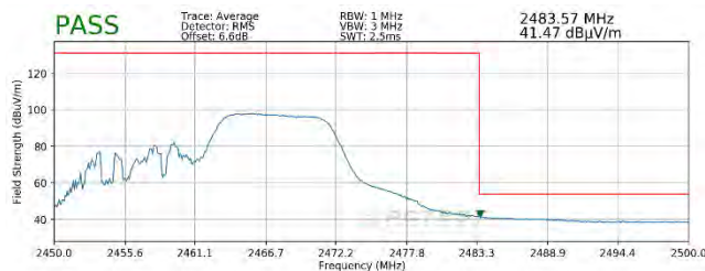
Plot 7-117. Radiated Restricted Upper Band Edge Measurement MIMO (Average – 106 Tones)
