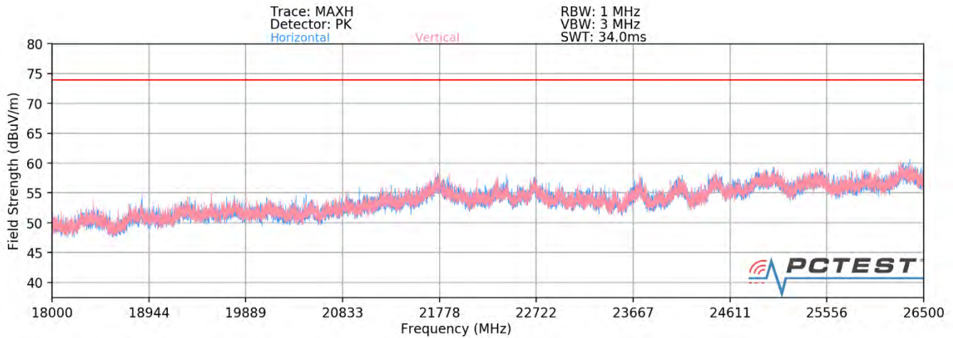
Plot 7-77. Radiated Spurious Plot above 18GHz SISO ANT1 (802.11ax OFDMA – 26 Tones)
