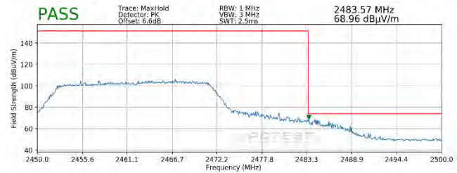
Plot 7-104. Radiated Restricted Upper Band Edge Measurement SISO ANT1 (Peak – 242 Tones)
