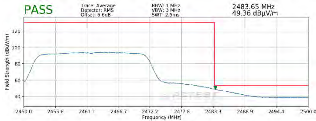
Plot 7-123. Radiated Restricted Upper Band Edge Measurement MIMO (Average – 242 Tones)
