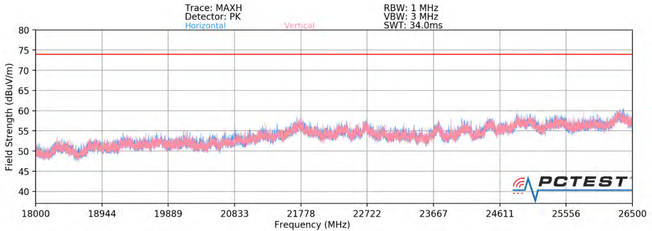
Plot 7-85. Radiated Spurious Plot above 18GHz SISO ANT2 (802.11ax OFDMA – 26 Tones)
