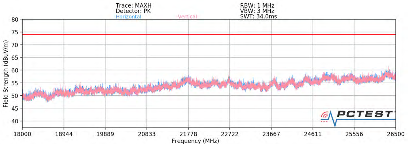
Plot 7-86. Radiated Spurious Plot above 18GHz SISO ANT2 (802.11ax OFDMA – 242 Tones)
