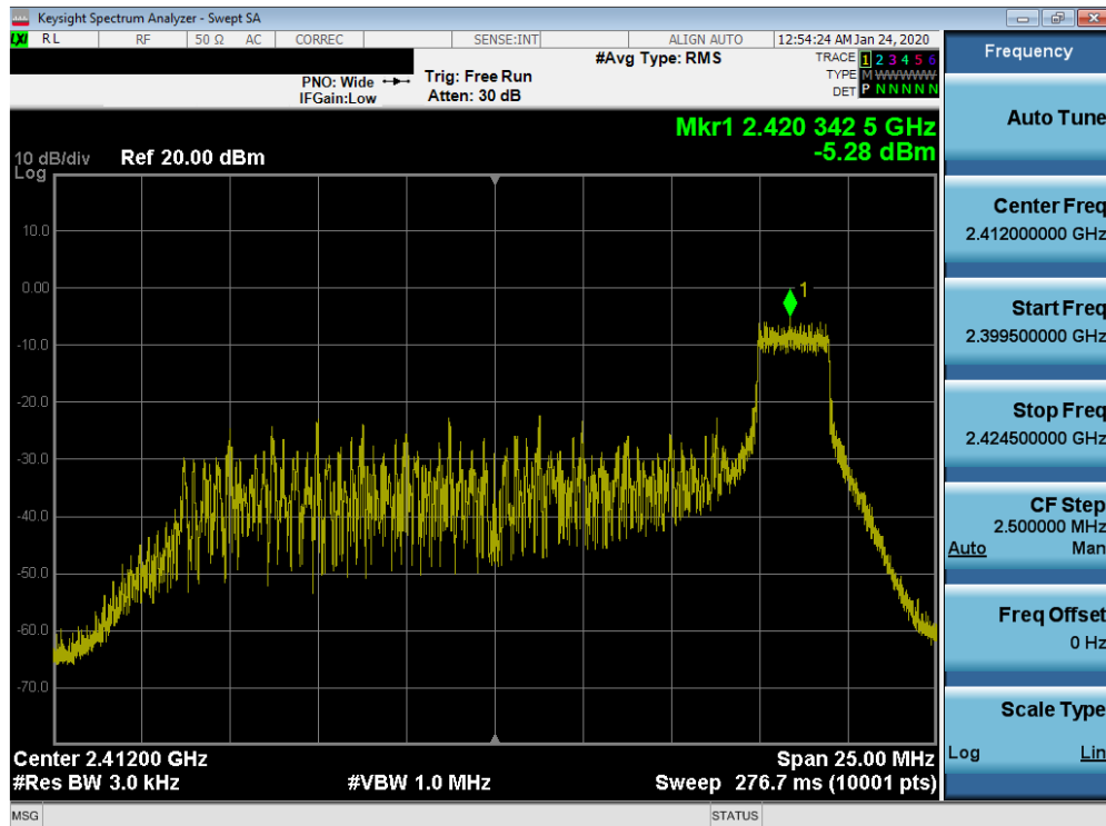
Plot 7-25. Power Spectral Density Plot MIMO ANT1 (802.11ax OFDMA – 6 Tones – Ch. 1)
