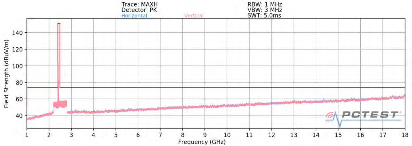
Plot 7-74. Radiated Spurious Plot above 1GHz SISO ANT1 (802.11ax OFDMA – 26T Tones – Ch. 1)
