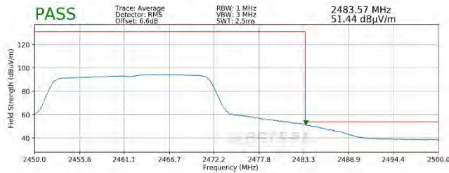
Plot 7-103. Radiated Restricted Upper Band Edge Measurement SISO ANT1 (Average – 242 Tones)
