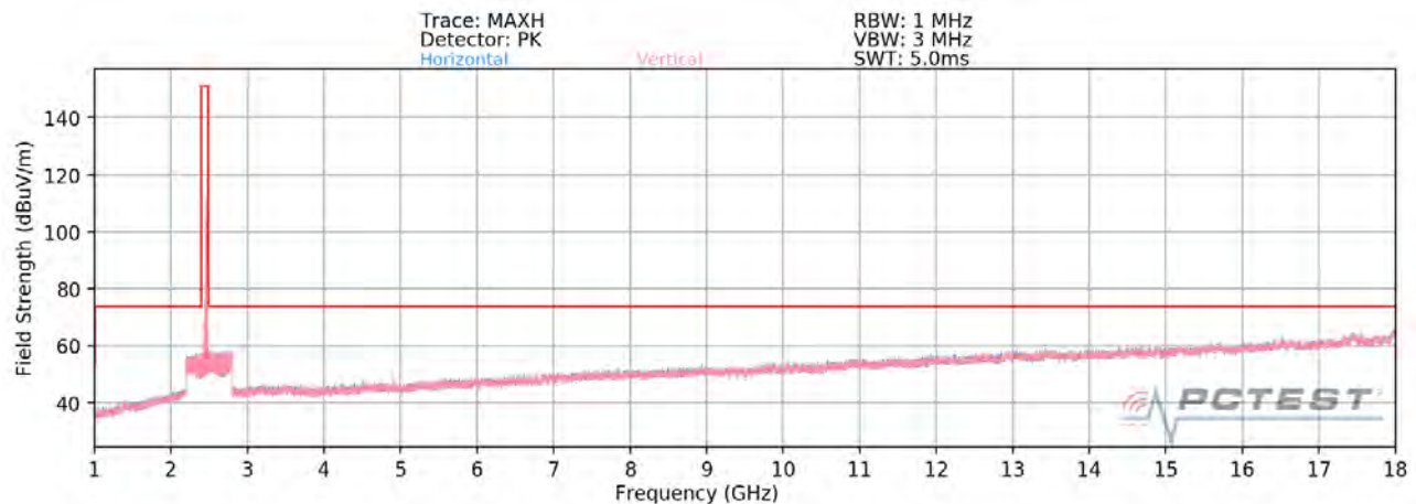
Plot 7-73. Radiated Spurious Plot above 1GHz SISO ANT1 (802.11ax OFDMA - 26T Tones - Ch. 11)
