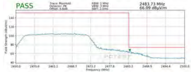
Plot 7-124. Radiated Restricted Upper Band Edge Measurement MIMO (Peak – 242 Tones)
