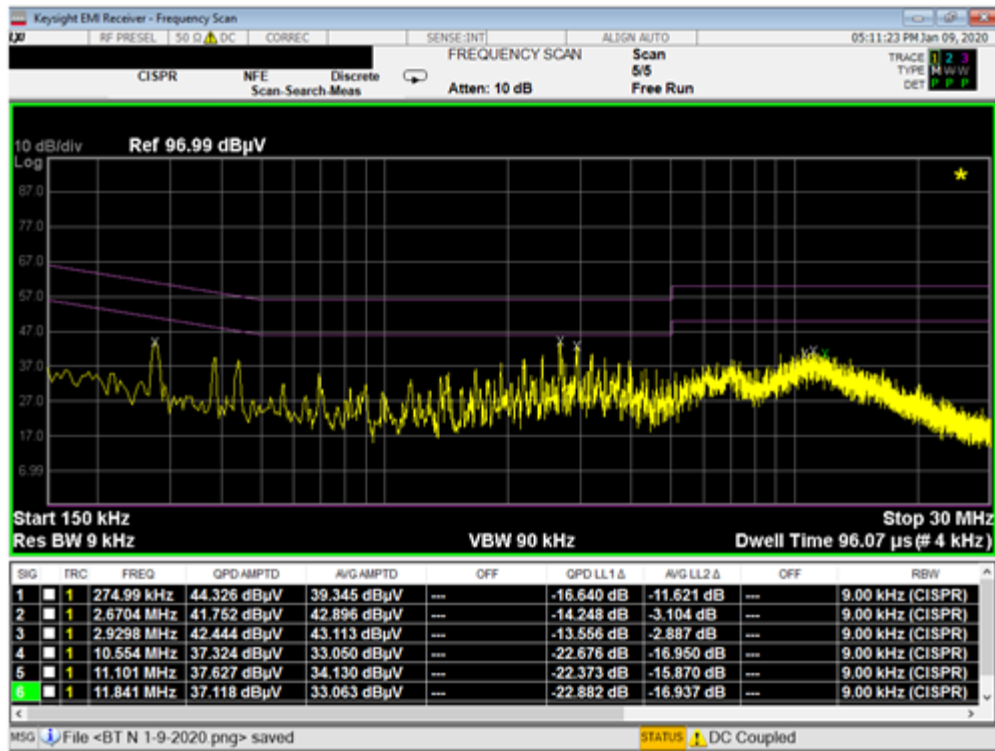
Plot 7-54. Line-Conducted Test with WCP (N)
