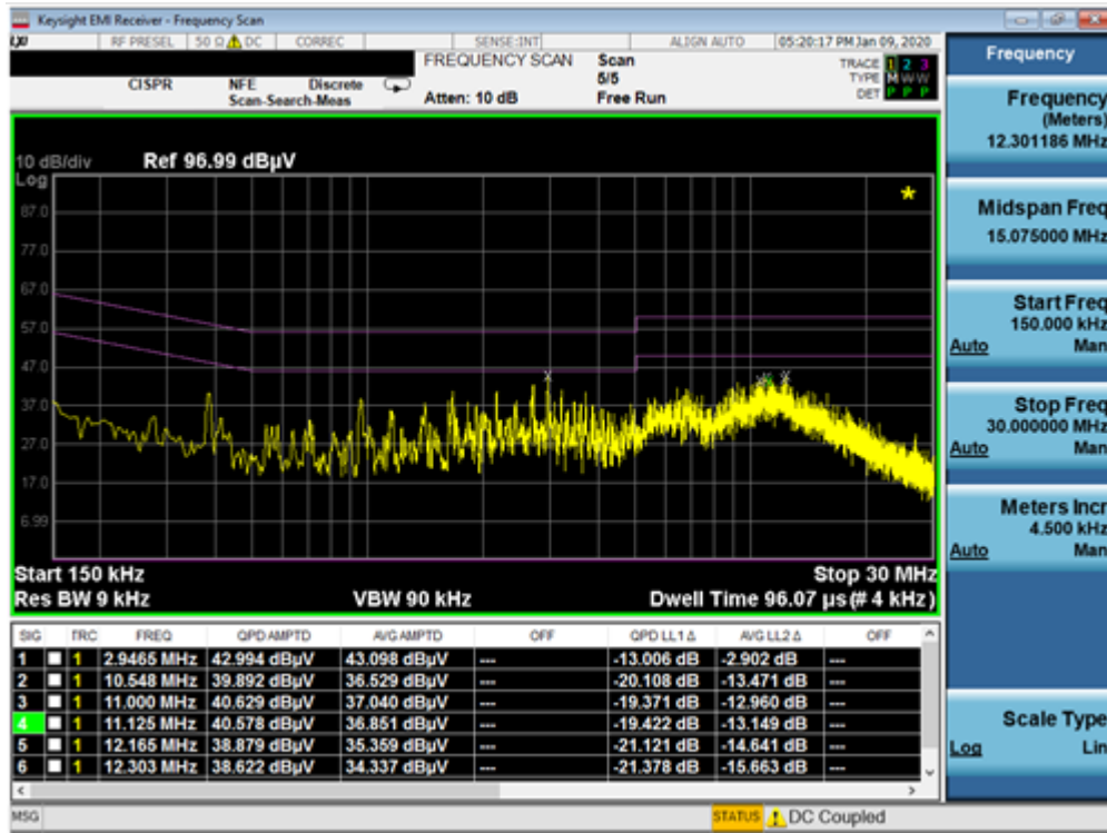
Plot 7-53. Line-Conducted Test with WCP (L1)
