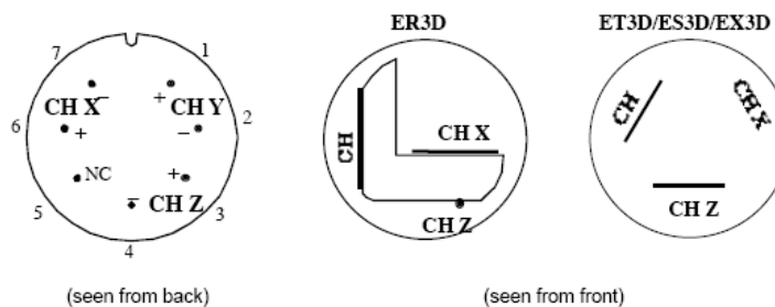
Connector Plan
