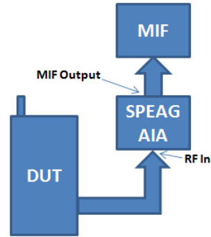
Figure 4-1 MIF Measurement Setup
