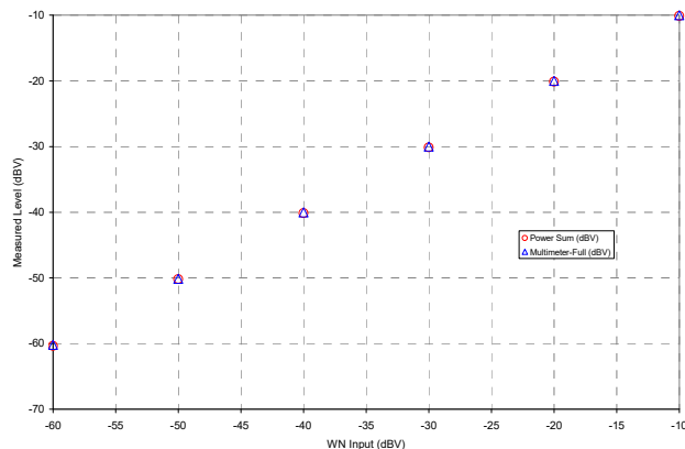
Figure 4-9 ABM2 Power Sum Validation
