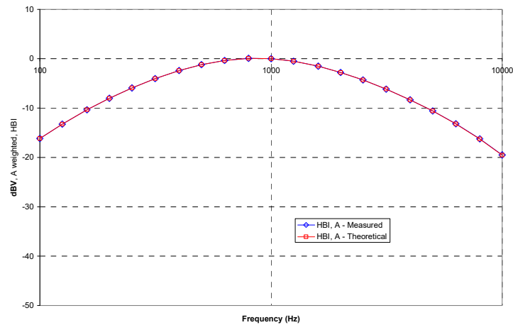
Figure 4-7 ABM2 Frequency Response Validation
