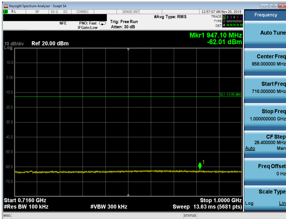
Plot 7-175. Conducted Spurious Plot (Band 12 - 10.0MHz QPSK - RB Size 1, RB Offset 0 - Low Channel)
