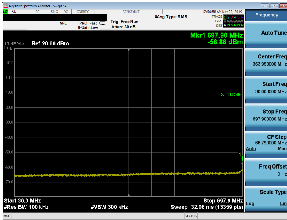
Plot 7-174. Conducted Spurious Plot (Band 12 - 10.0MHz QPSK - RB Size 1, RB Offset 0 - Low Channel)
