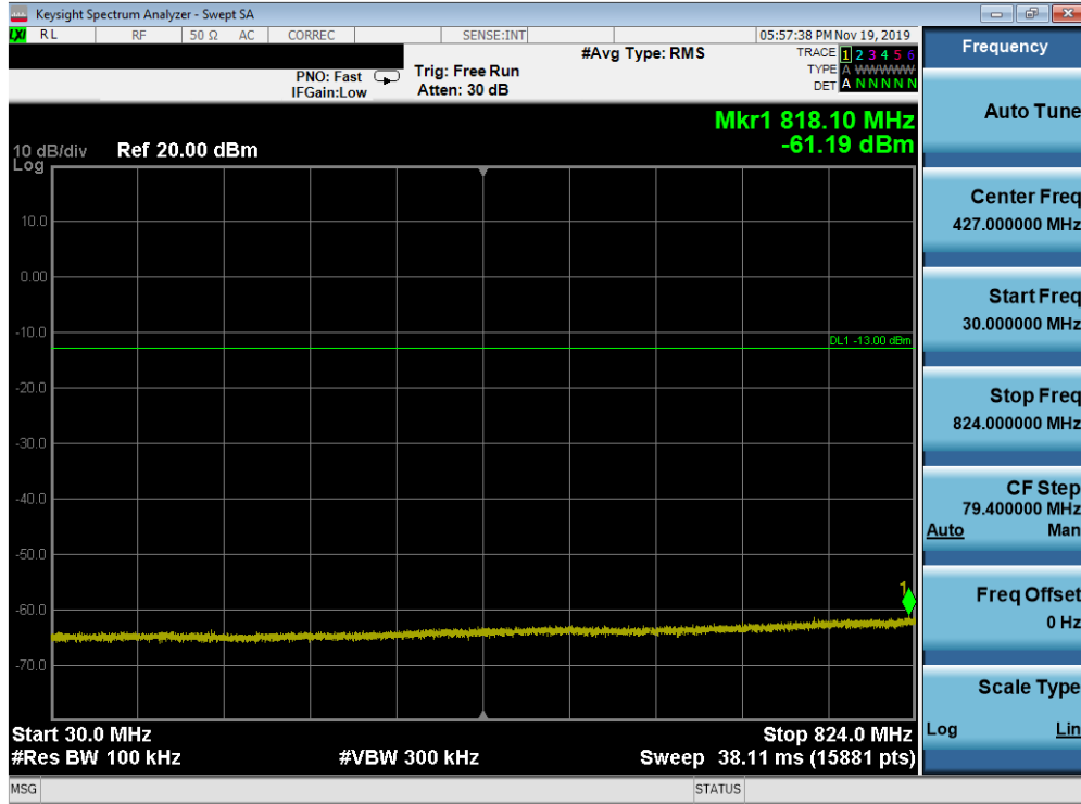
Plot 7-192. Conducted Spurious Plot (Band 20 - 15.0MHz QPSK - RB Size 1, RB Offset 0 - High Channel)
