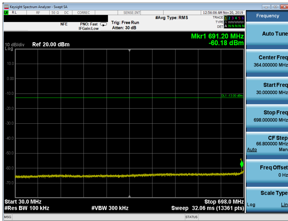
Plot 7-177. Conducted Spurious Plot (Band 12 - 10.0MHz QPSK - RB Size 1, RB Offset 0 - Mid Channel)
