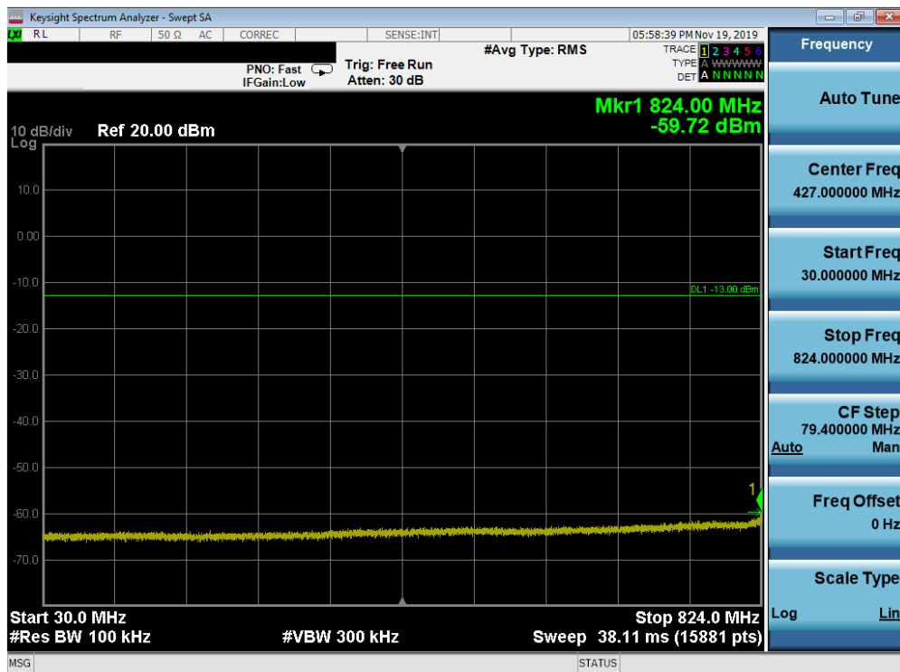
Plot 7-189. Conducted Spurious Plot (Band 26/5 - 10.0MHz QPSK - RB Size 1, RB Offset 0 - Mid Channel)
