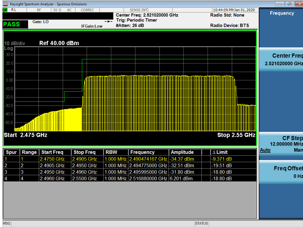
Plot 7-704. Lower ACP Plot at 2496 MHz (n41 - 50MHz DFT-s-OFDM-QPSK - Full RB Configuration)
