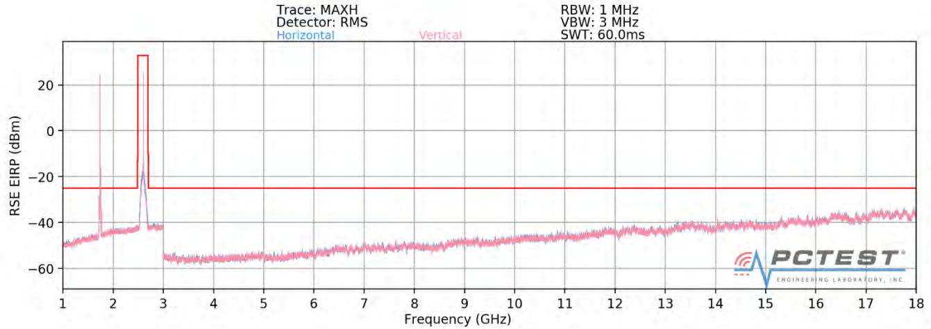
Plot 7-750. Radiated Spurious Plot above 1GHz (n41 - ANCHOR B66)
