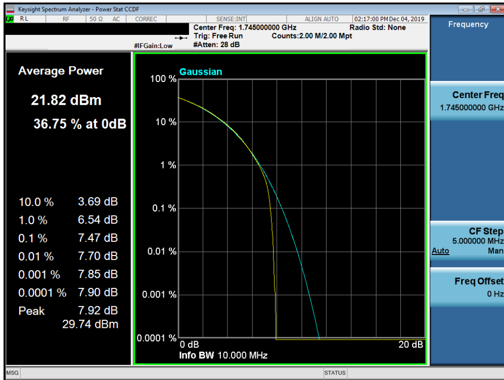
Plot 7-736. PAR Plot (Band n66 - 10.0MHz CP-OFDM- 64-QAM - Full RB Configuration)
