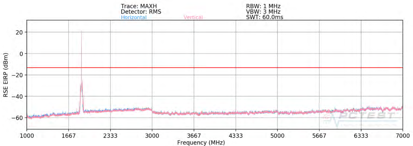
Plot 7-746. Radiated Spurious Plot above 1GHz (n71 ENDC - ANCHOR B2)
