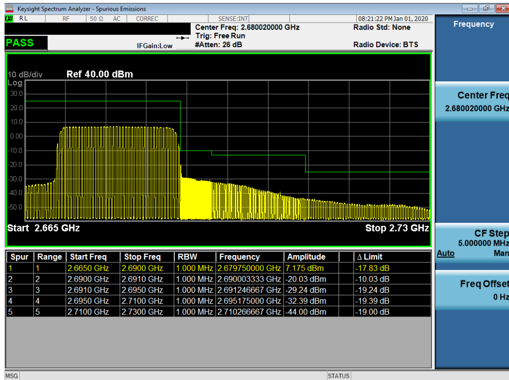
Plot 7-701. Upper ACP Plot (n41 - 20MHz CP-OFDM-QPSK - Full RB Configuration)
