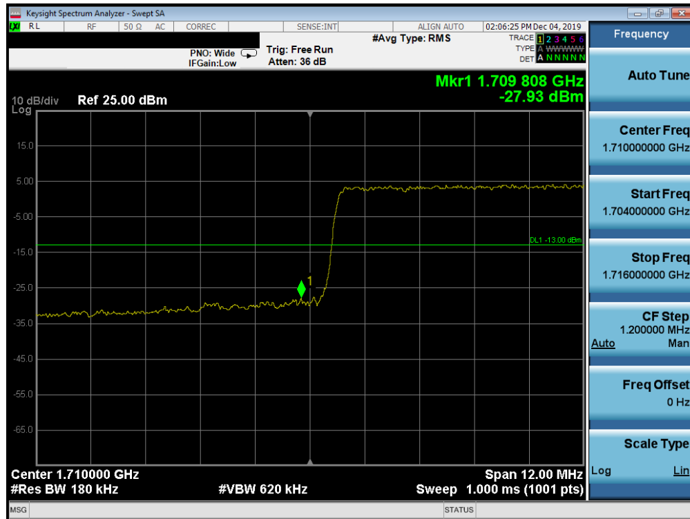
Plot 7-676. Lower Band Edge Plot (Band n66 - 15.0MHz CP-OFDM-QPSK - Full RB Configuration)
