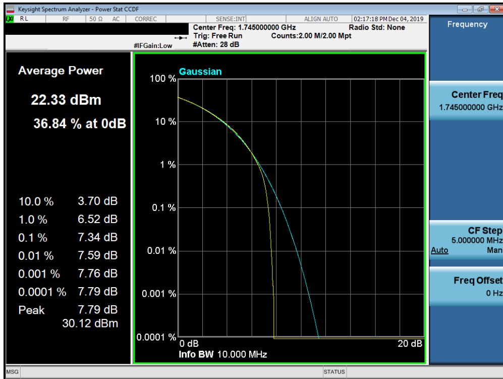
Plot 7-734. PAR Plot (Band n66 - 10.0MHz CP-OFDM-QPSK - Full RB Configuration)
