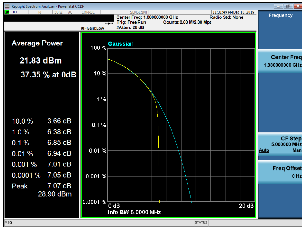
Plot 7-714. PAR Plot (Band n2 - 5.0MHz CP-OFDM-QPSK - Full RB Configuration)
