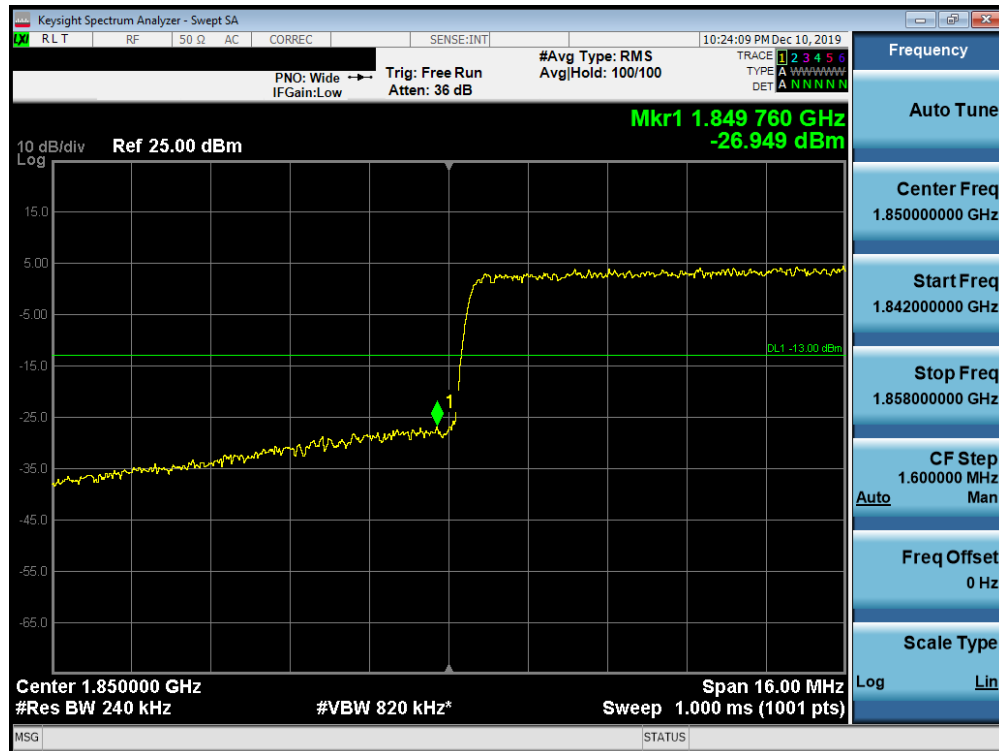
Plot 7-696. Lower Band Edge Plot (Band n2 - 20.0MHz CP-OFDM-QPSK - Full RB Configuration)
