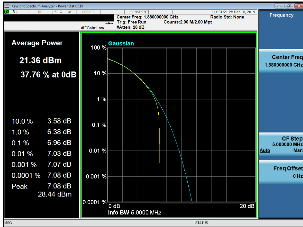
Plot 7-716. PAR Plot (Band n2 - 5.0MHz CP-OFDM-64-QAM - Full RB Configuration)
