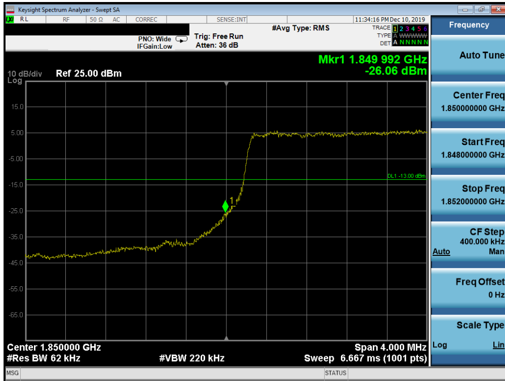
Plot 7-684. Lower Band Edge Plot (Band n2 - 5.0MHz DFT-s-OFDM-QPSK - Full RB Configuration)
