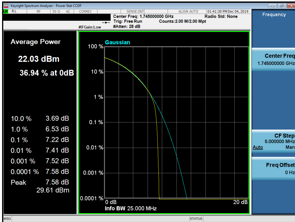
Plot 7-743. PAR Plot (Band n66 - 20.0MHz CP-OFDM- 16-QAM - Full RB Configuration)
