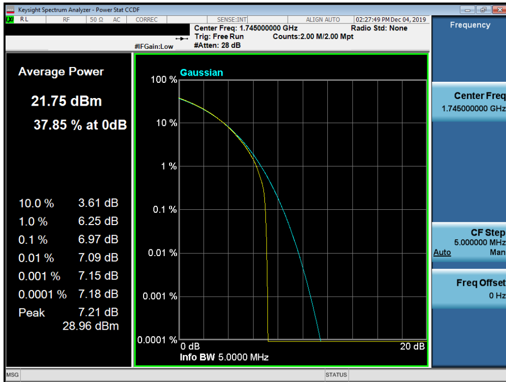
Plot 7-732. PAR Plot (Band n66 - 5.0MHz CP-OFDM- 64-QAM - Full RB Configuration)
