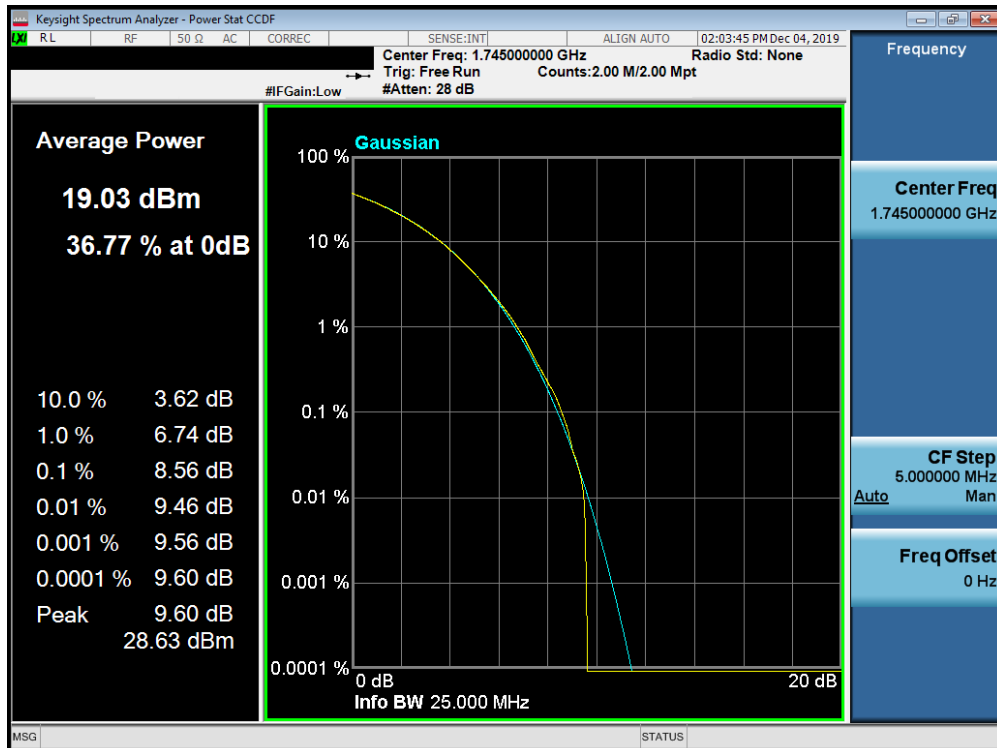
Plot 7-741. PAR Plot (Band n66 - 15.0MHz CP-OFDM- 256-QAM - Full RB Configuration)
