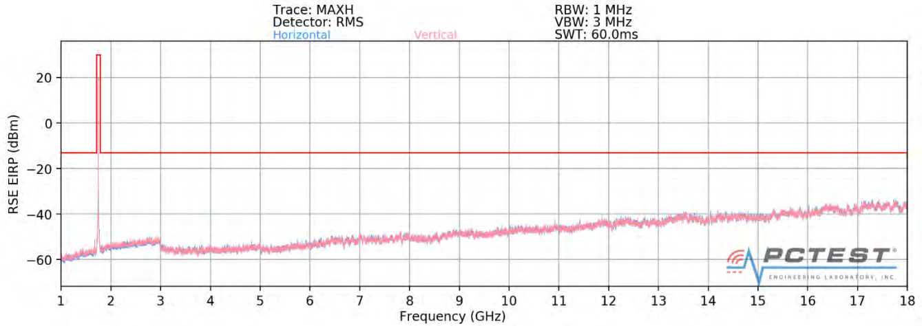
Plot 7-748. Radiated Spurious Plot above 1GHz (n66 ENDC – ANCHOR B13)
