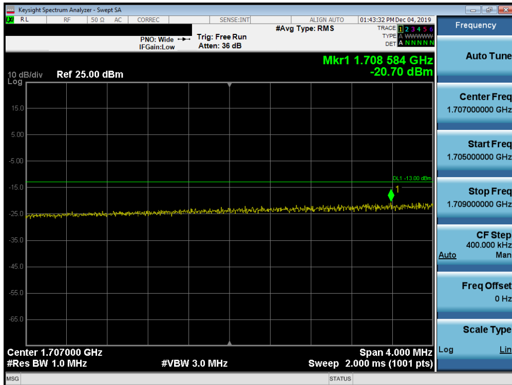
Plot 7-681. Lower Extended Band Edge Plot (Band n66 - 20.0MHz DFT-s-OFDM-QPSK - Full RB Configuration)
