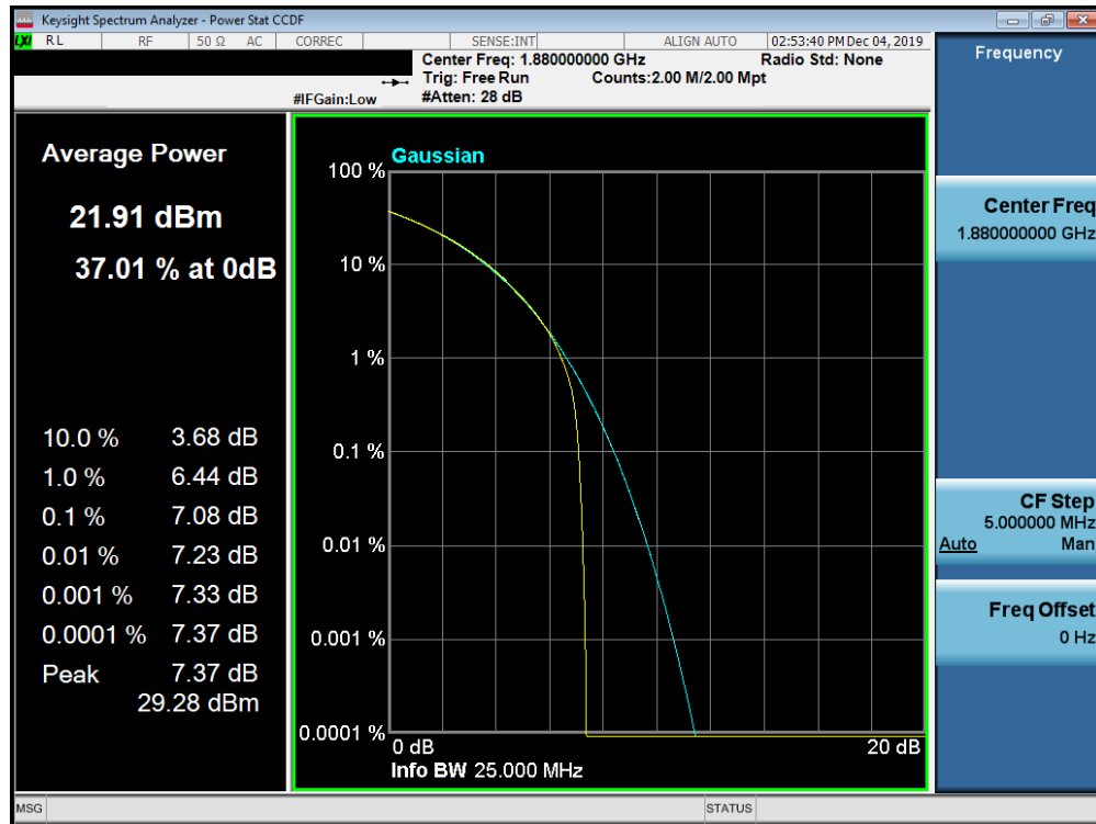
Plot 7-729. PAR Plot (Band n2 - 20.0MHz CP-OFDM- 256-QAM - Full RB Configuration)
