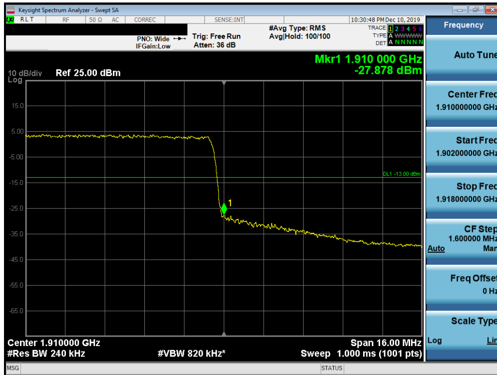
Plot 7-698. Upper Band Edge Plot (Band n2 - 20.0MHz CP-OFDM-QPSK - Full RB Configuration)
