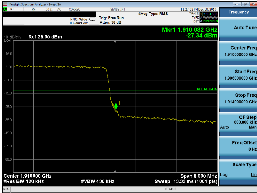
Plot 7-690. Upper Band Edge Plot (Band n2 - 10.0MHz DFT-s-OFDM-QPSK - Full RB Configuration)
