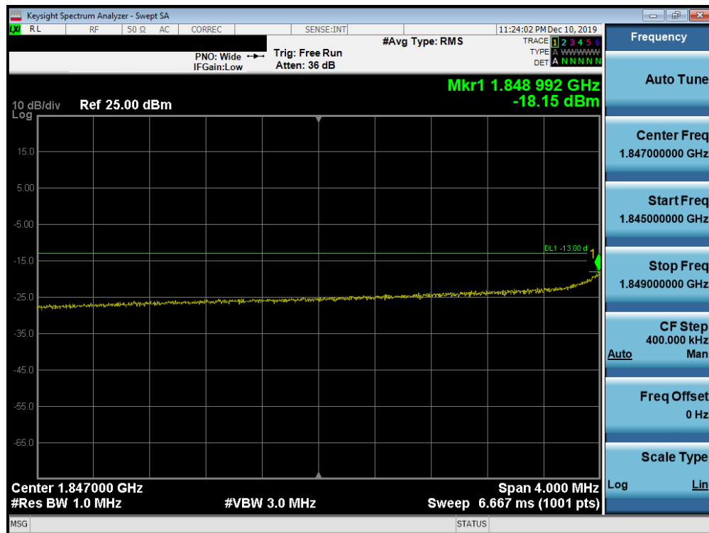
Plot 7-689. Lower Extended Band Edge Plot (Band n2 - 10.0MHz CP-OFDM-QPSK - Full RB Configuration)
