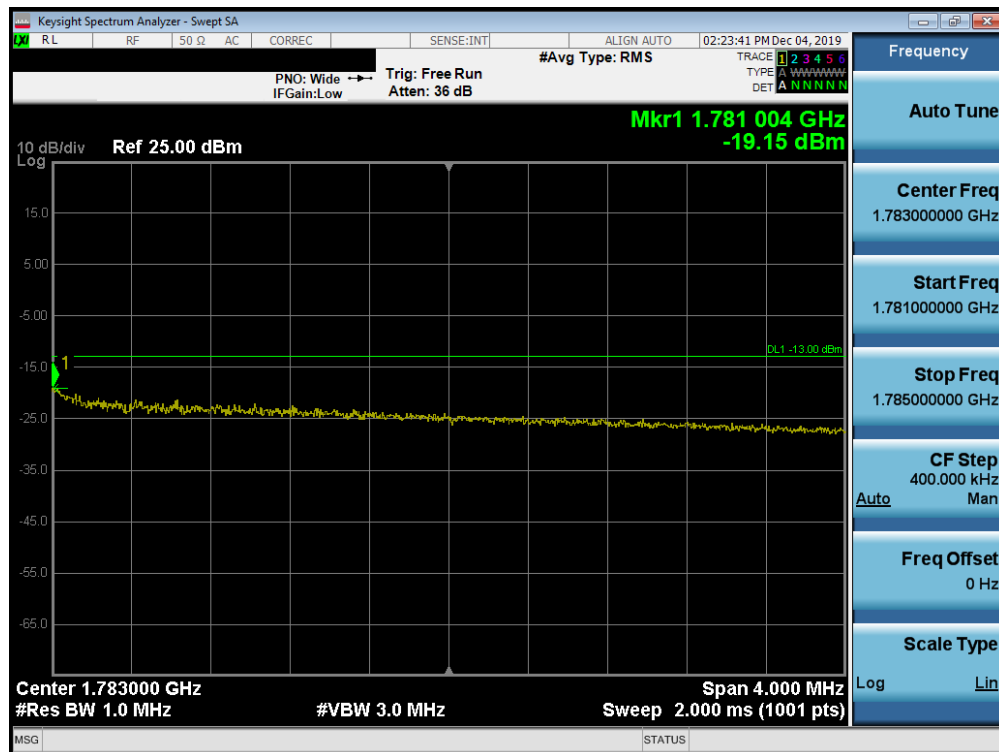
Plot 7-675. Upper Extended Band Edge Plot (Band n66 - 10.0MHz CP-OFDM-QPSK - Full RB Configuration)
