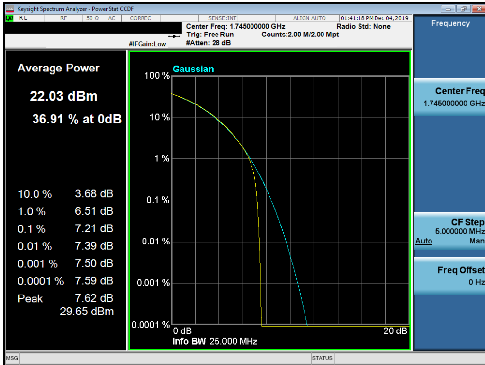
Plot 7-744. PAR Plot (Band n66 - 20.0MHz CP-OFDM- 64-QAM - Full RB Configuration)
