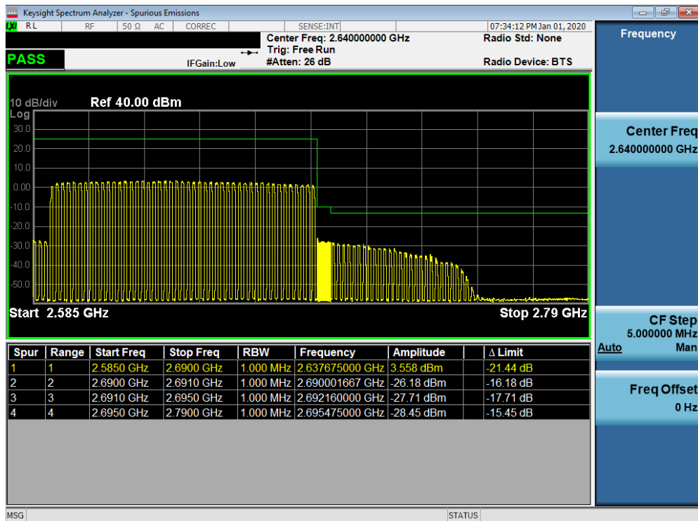
Plot 7-713. Upper ACP Plot (n41 - 100MHz CP-OFDM-QPSK - Full RB Configuration)
