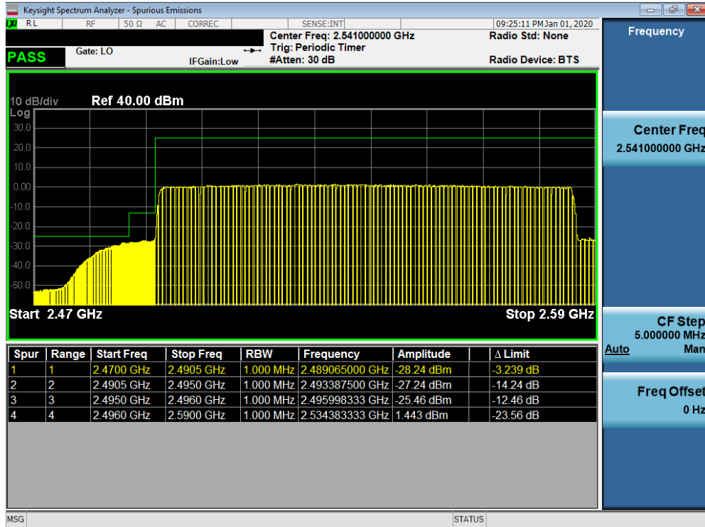
Plot 7-710. Lower ACP Plot at 2496 MHz (n41 - 90MHz CP-OFDM-QPSK - Full RB Configuration)
