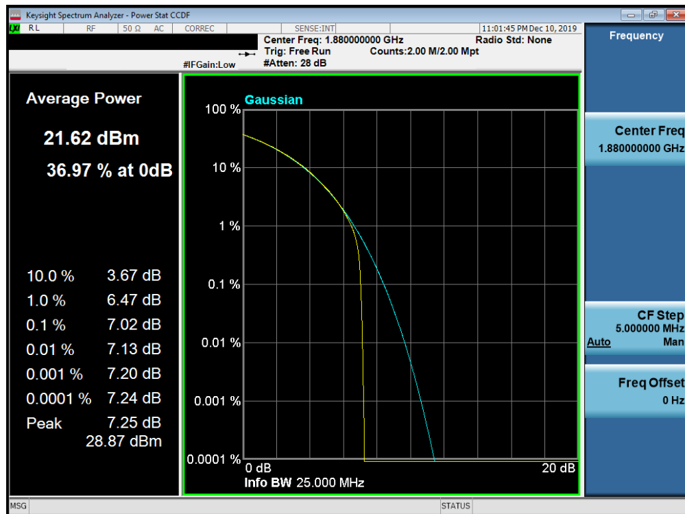
Plot 7-724. PAR Plot (Band n2 - 15.0MHz CP-OFDM-64-QAM - Full RB Configuration)
