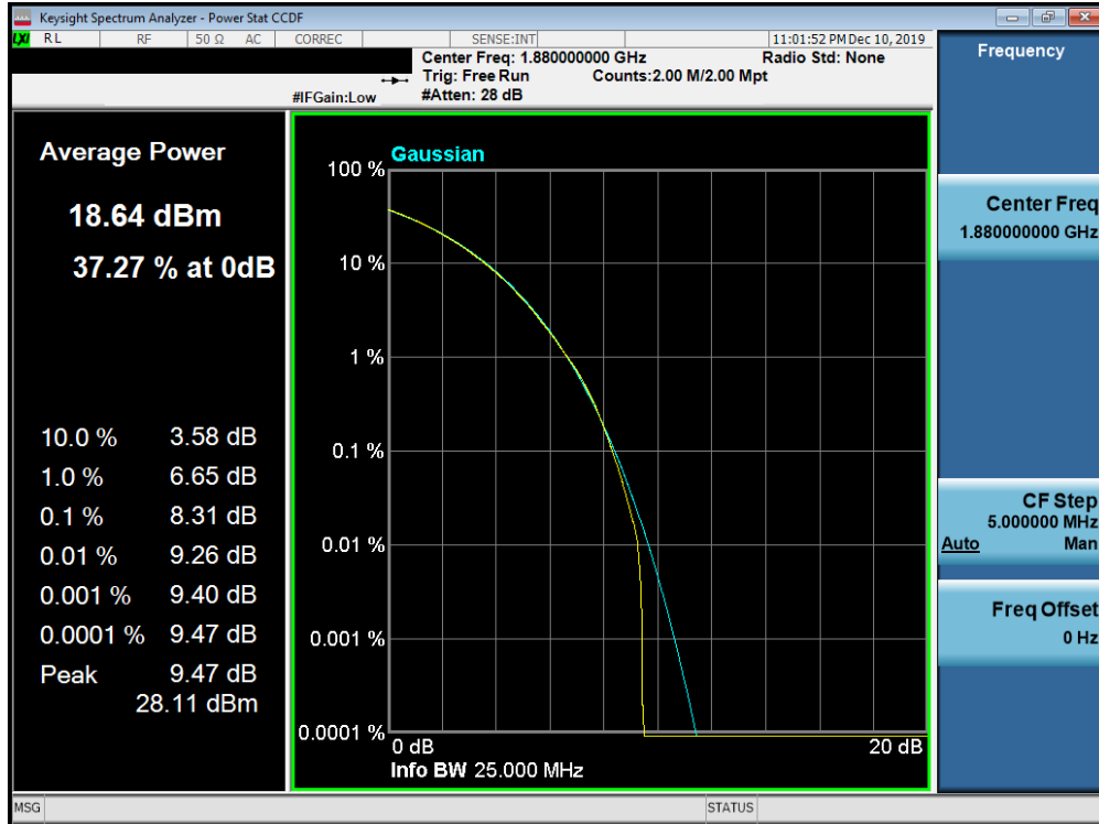
Plot 7-725. PAR Plot (Band n2 - 15.0MHz CP-OFDM 256-QAM - Full RB Configuration)
