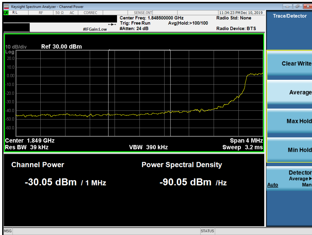
Plot 7-685. Lower Extended Band Edge Plot (Band n2 - 5.0MHz DFT-s-OFDM-QPSK - Full RB Configuration)
