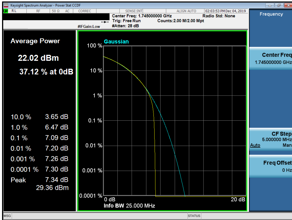
Plot 7-740. PAR Plot (Band n66 - 15.0MHz CP-OFDM- 64-QAM - Full RB Configuration)
