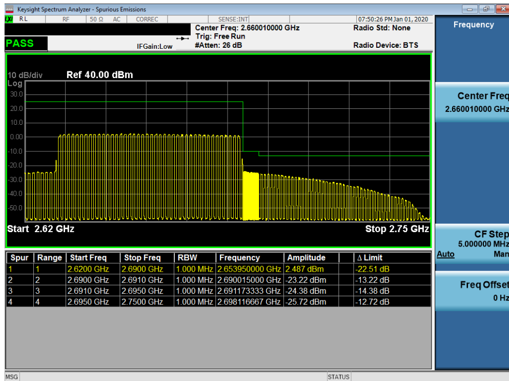
Plot 7-707. Upper ACP Plot (n41 - 60MHz DFT-s-OFDM-QPSK - Full RB Configuration)
