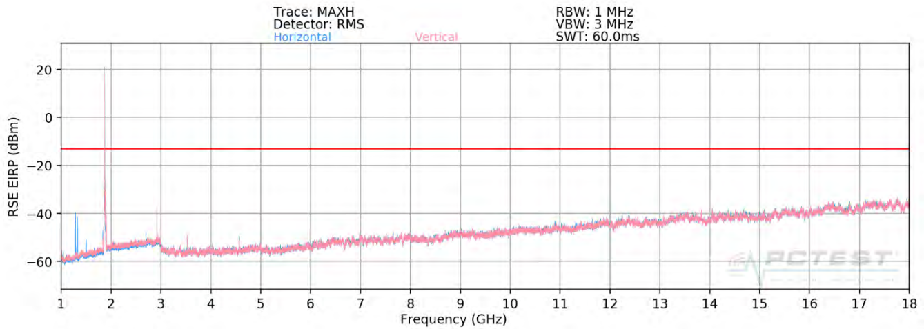
Plot 7-747. Radiated Spurious Plot above 1GHz (n5 EN-DC – ANCHOR B2)
