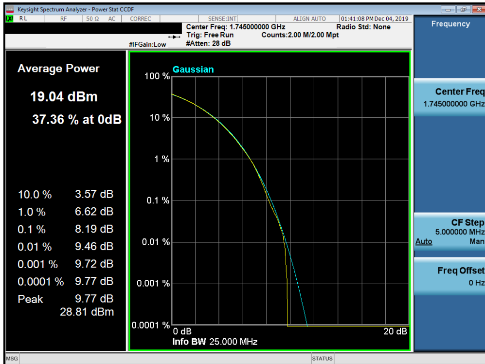
Plot 7-745. PAR Plot (Band n66 - 20.0MHz CP-OFDM- 256-QAM - Full RB Configuration)
