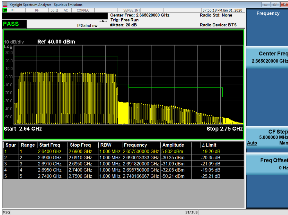
Plot 7-705. Upper ACP Plot (n41 - 50MHz DFT-s-OFDM-QPSK - Full RB Configuration)
