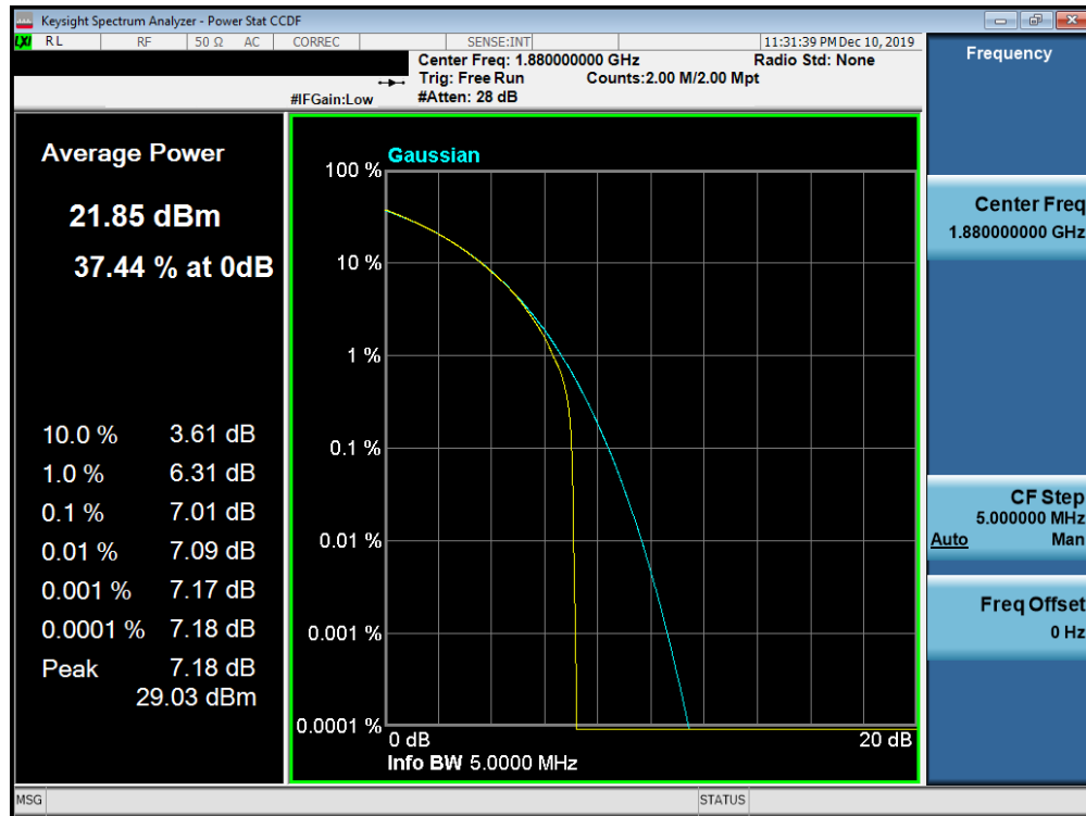
Plot 7-715. PAR Plot (Band n2 - 5.0MHz CP-OFDM-16-QAM - Full RB Configuration)
