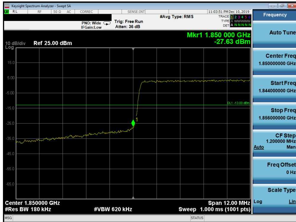
Plot 7-692. Lower Band Edge Plot (Band n2 - 15.0MHz CP-OFDM-QPSK - Full RB Configuration)
