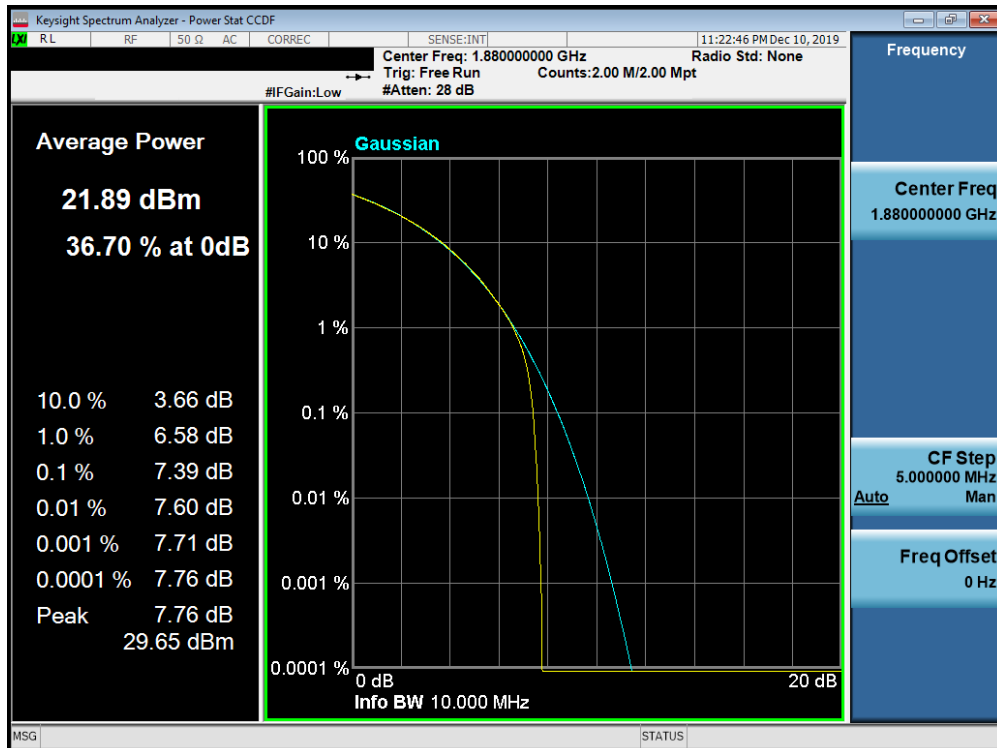
Plot 7-718. PAR Plot (Band n2 - 10.0MHz CP-OFDM-QPSK - Full RB Configuration)
