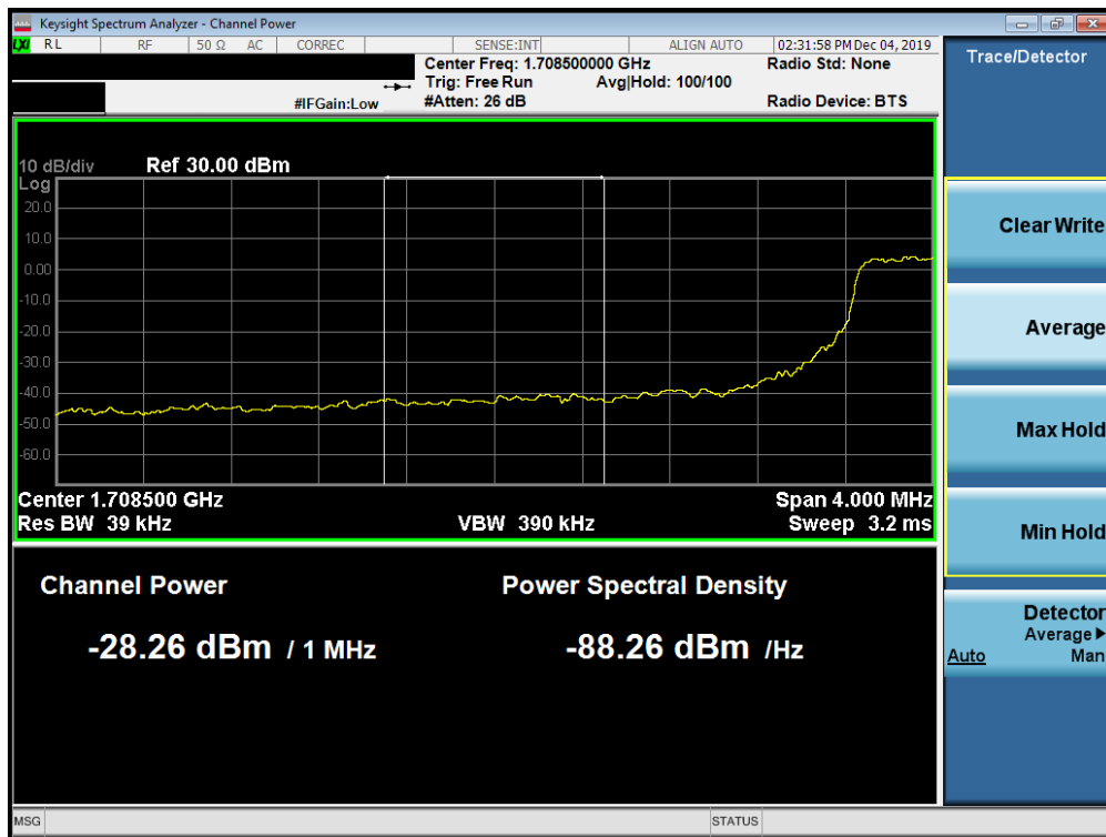
Plot 7-669. Lower Extended Band Edge Plot (Band n66 - 5.0MHz DFT-s-OFDM-QPSK - Full RB Configuration)
