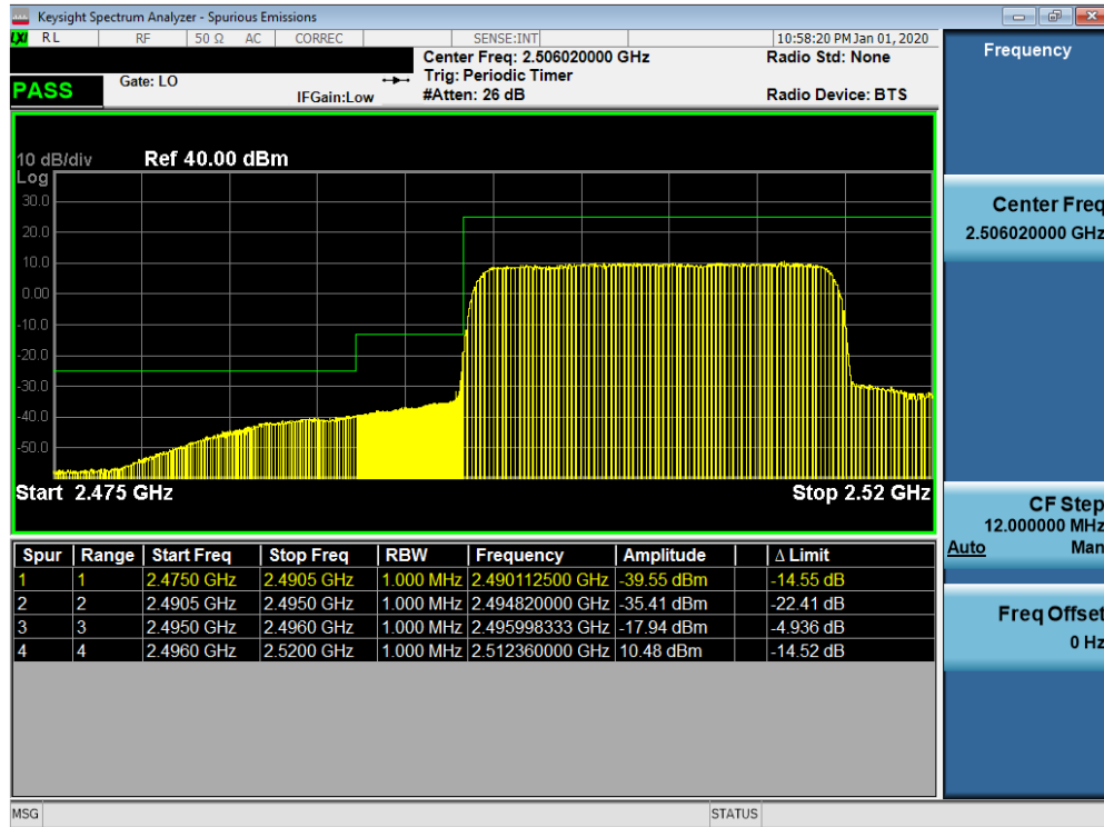
Plot 7-700. Lower ACP Plot at 2496 MHz (n41 - 20MHz DFT-s-OFDM-QPSK - Full RB Configuration)
