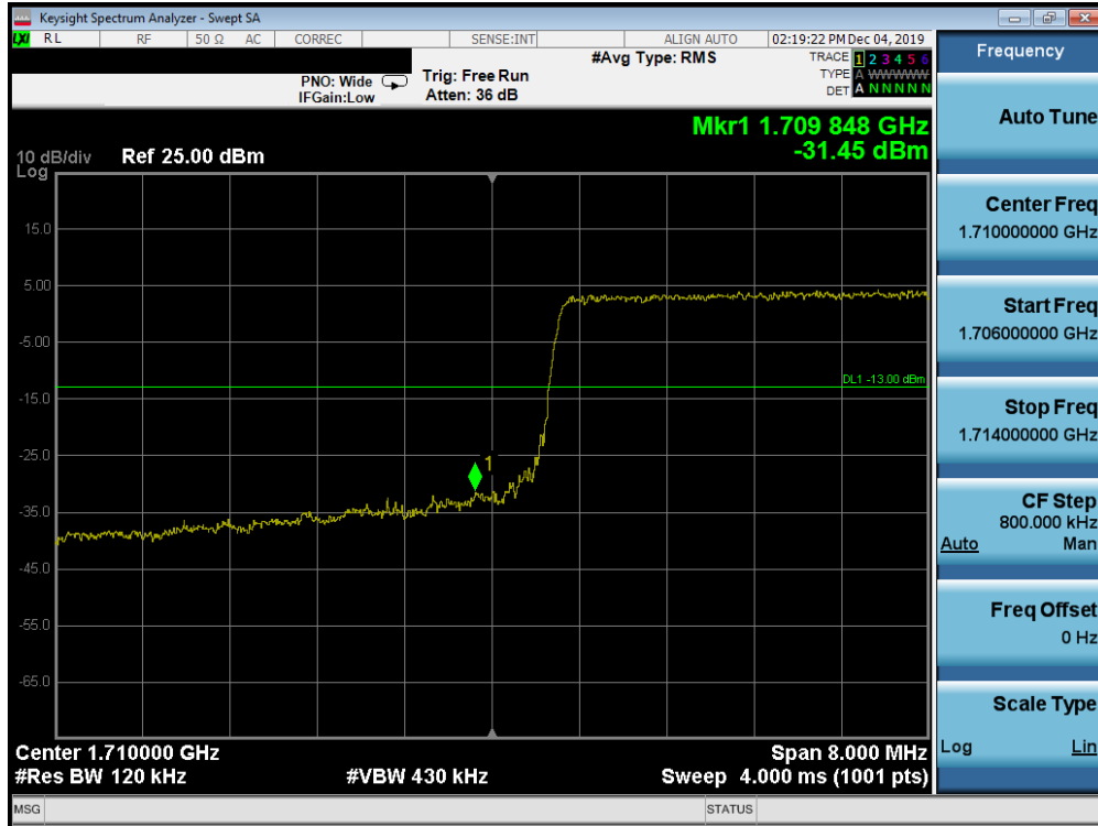
Plot 7-672. Lower Band Edge Plot (Band n66 - 10.0MHz CP-OFDM-QPSK - Full RB Configuration)
