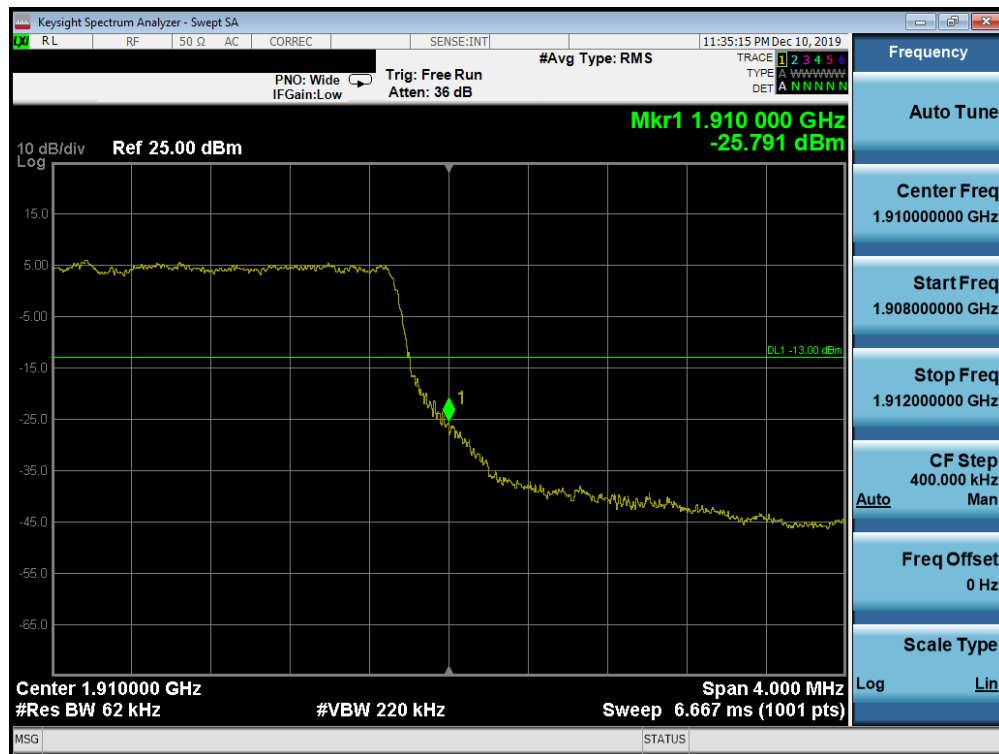
Plot 7-686. Upper Band Edge Plot (Band n2 - 5.0MHz DFT-s-OFDM-QPSK - Full RB Configuration)
