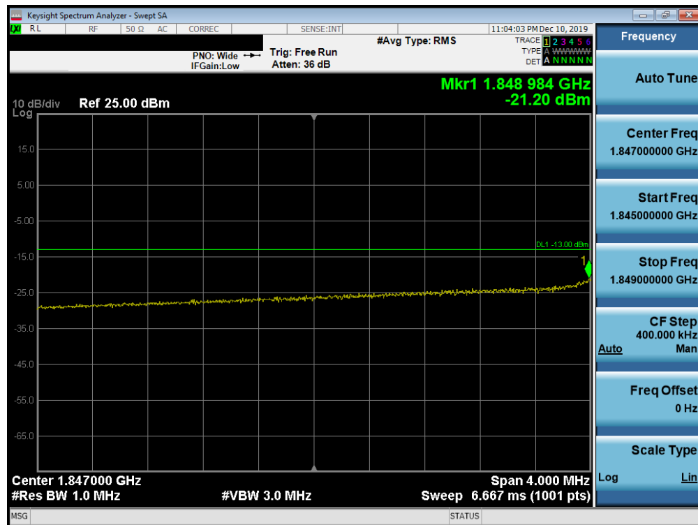
Plot 7-693. Lower Extended Band Edge Plot (Band n2 - 15.0MHz CP-OFDM-QPSK - Full RB Configuration)
