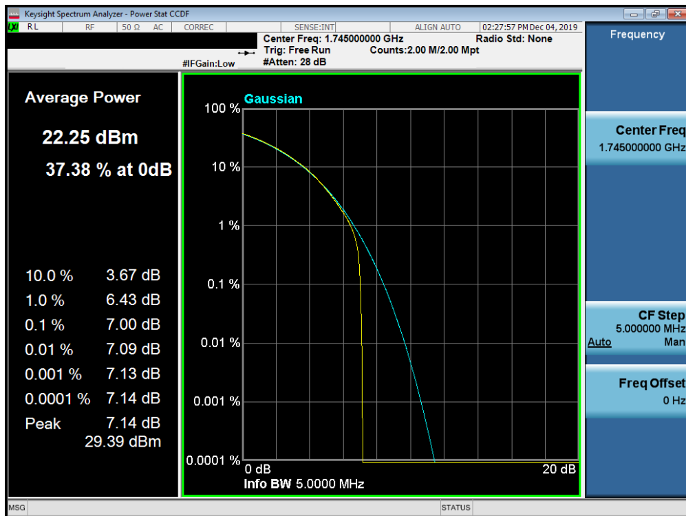
Plot 7-731. PAR Plot (Band n66 - 5.0MHz CP-OFDM- 16-QAM - Full RB Configuration)
