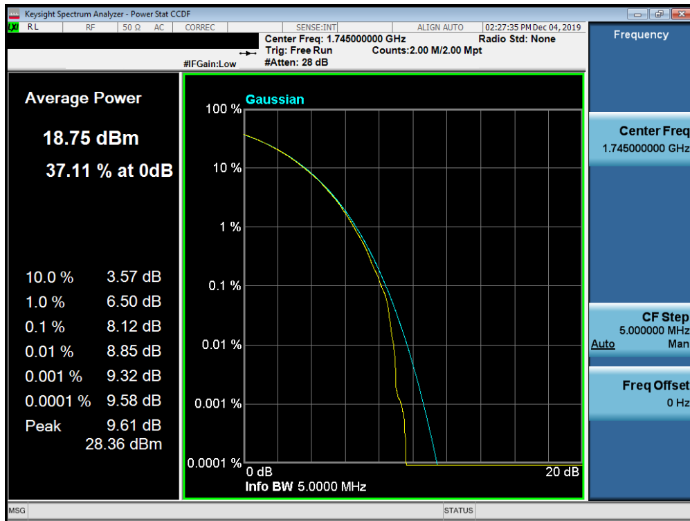
Plot 7-733. PAR Plot (Band n66 - 5.0MHz CP-OFDM- 256-QAM - Full RB Configuration)
