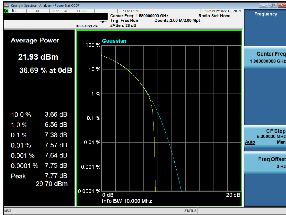
Plot 7-719. PAR Plot (Band n2 - 10.0MHz CP-OFDM-16-QAM - Full RB Configuration)
