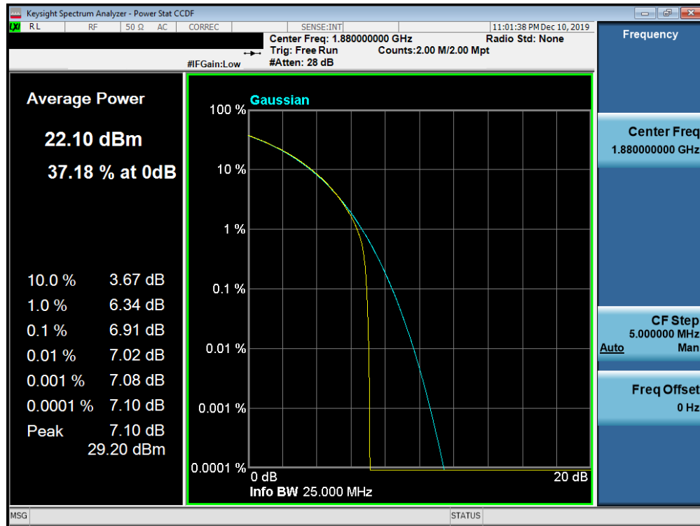
Plot 7-723. PAR Plot (Band n2 - 15.0MHz CP-OFDM -16-QAM - Full RB Configuration)
