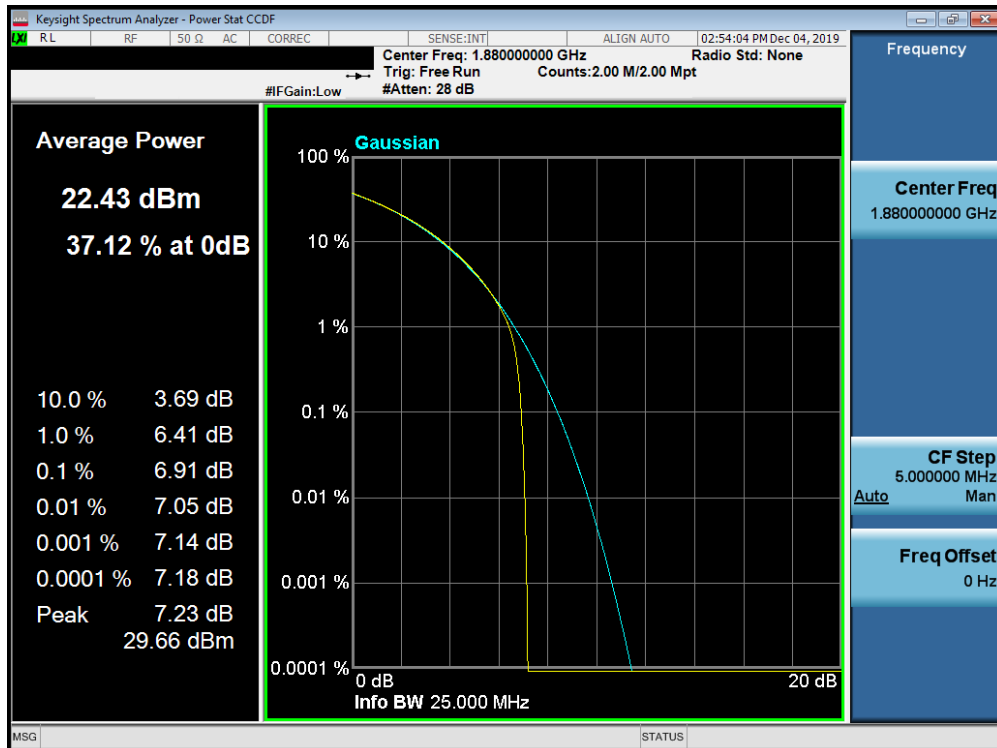
Plot 7-726. PAR Plot (Band n2 - 20.0MHz CP-OFDM-QPSK - Full RB Configuration)
