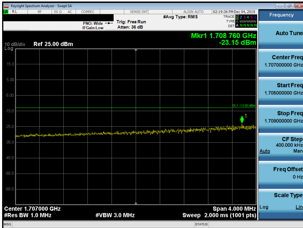
Plot 7-673. Lower Extended Band Edge Plot (Band n66 - 10.0MHz CP-OFDM-QPSK - Full RB Configuration)
