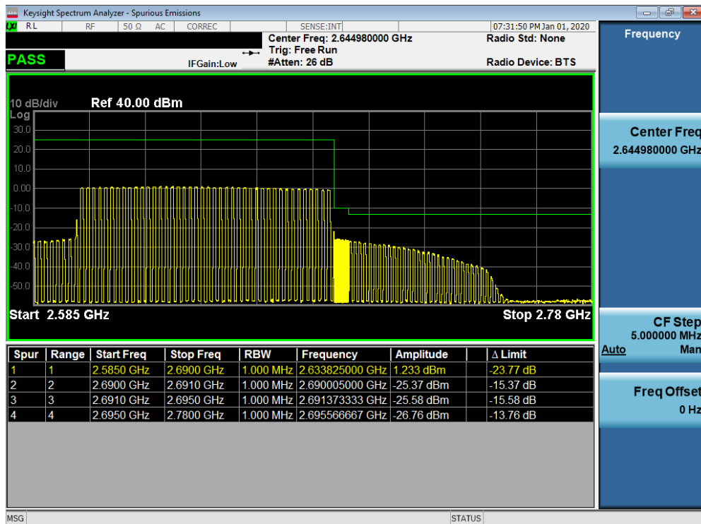
Plot 7-711. Upper ACP Plot (n41 - 90MHz CP-OFDM-QPSK - Full RB Configuration)
