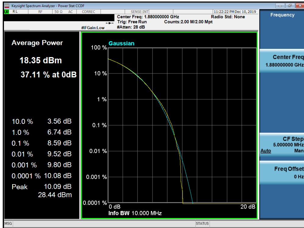
Plot 7-721. PAR Plot (Band n2 - 10.0MHz CP-OFDM - 256-QAM - Full RB Configuration)
