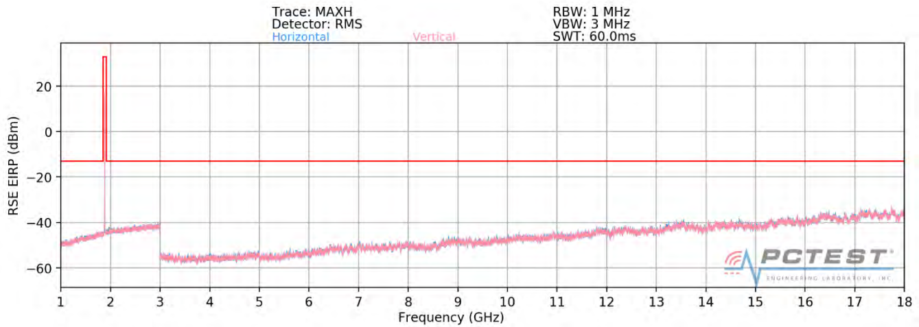
Plot 7-749. Radiated Spurious Plot above 1GHz (n2 ENDC - ANCHOR B13)
