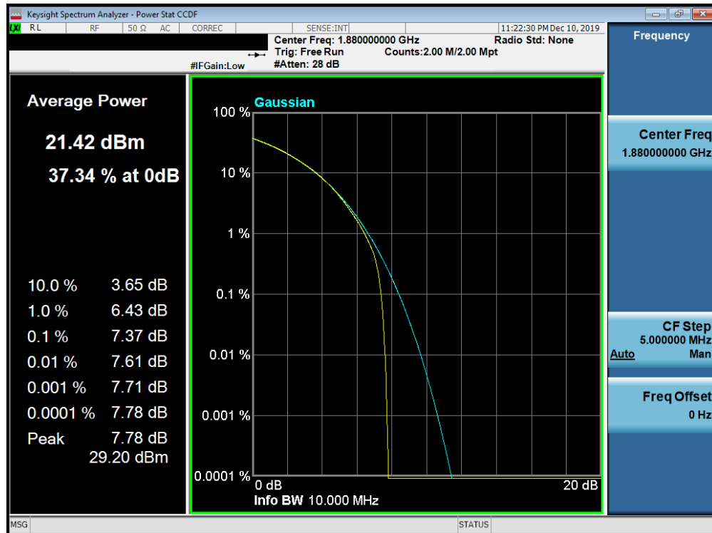
Plot 7-720. PAR Plot (Band n2 - 10.0MHz CP-OFDM- 64-QAM - Full RB Configuration)
