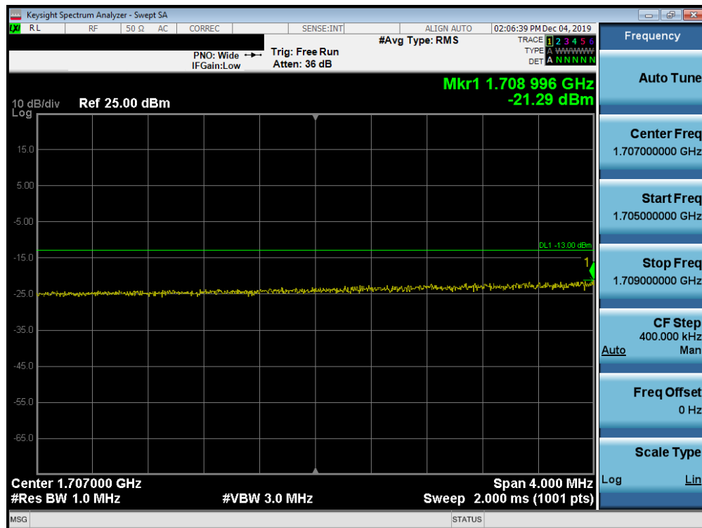
Plot 7-677. Lower Extended Band Edge Plot (Band n66 - 15.0MHz CP-OFDM-QPSK - Full RB Configuration)
