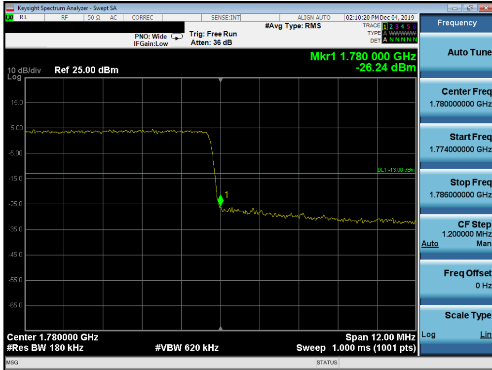
Plot 7-678. Upper Band Edge Plot (Band n66 - 15.0MHz CP-OFDM-QPSK - Full RB Configuration)
