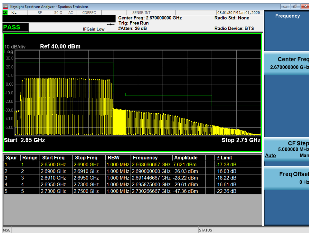
Plot 7-703. Upper ACP Plot (n41 - 40MHz DFT-s-OFDM-QPSK - Full RB Configuration)
