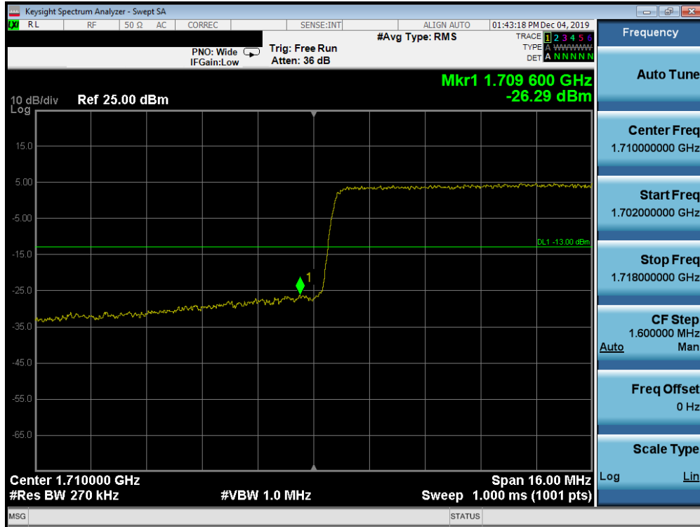
Plot 7-680. Lower Band Edge Plot (Band n66 - 20.0MHz DFT-s-OFDM-QPSK - Full RB Configuration)
