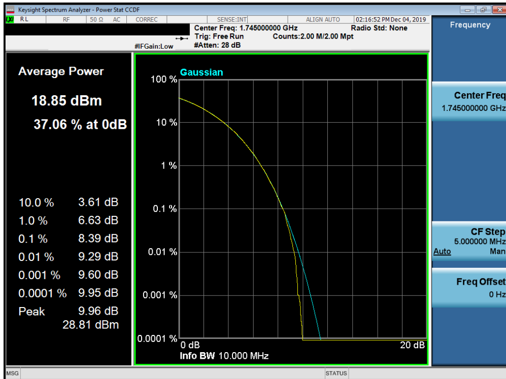
Plot 7-737. PAR Plot (Band n66 - 10.0MHz CP-OFDM- 256-QAM - Full RB Configuration)
