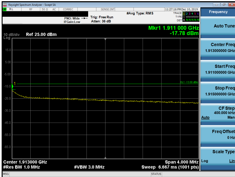
Plot 7-691. Upper Extended Band Edge Plot (Band n2 - 10.0MHz DFT-s-OFDM-QPSK - Full RB Configuration)
