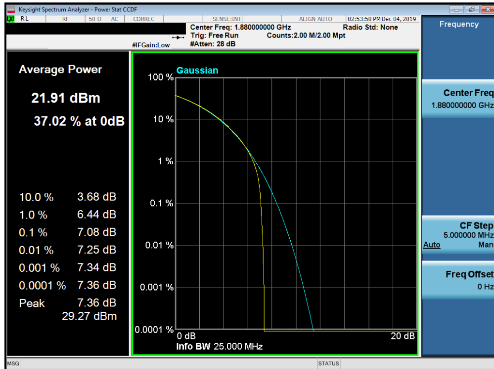
Plot 7-728. PAR Plot (Band n2 - 20.0MHz CP-OFDM-64-QAM - Full RB Configuration)
