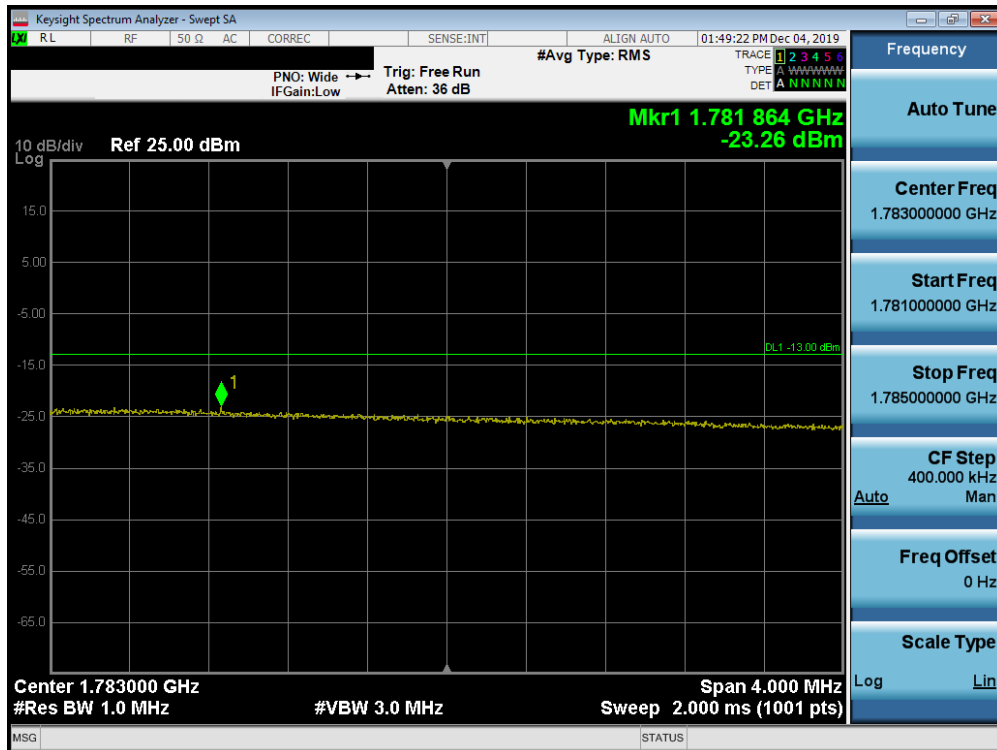
Plot 7-683. Upper Extended Band Edge Plot (Band n66 - 20.0MHz DFT-s-OFDM-QPSK - Full RB Configuration)
