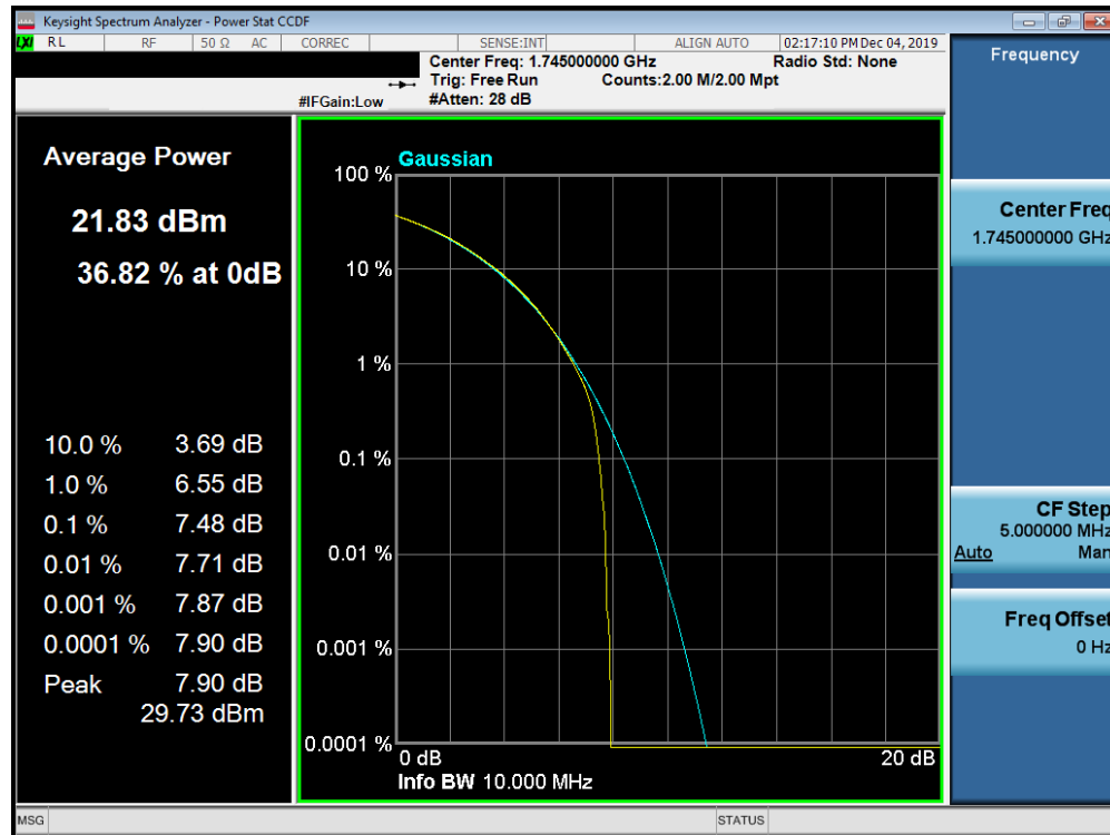
Plot 7-735. PAR Plot (Band n66 - 10.0MHz CP-OFDM- 16-QAM - Full RB Configuration)
