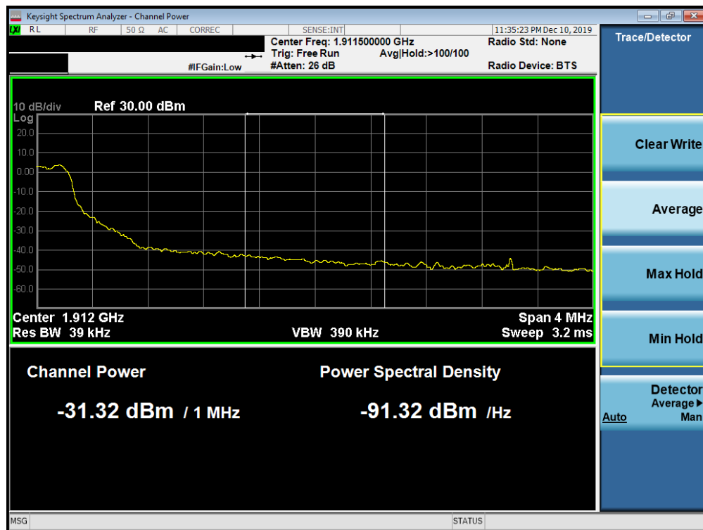
Plot 7-687. Upper Extended Band Edge Plot (Band n2 - 5.0MHz DFT-s-OFDM-QPSK - Full RB Configuration)
