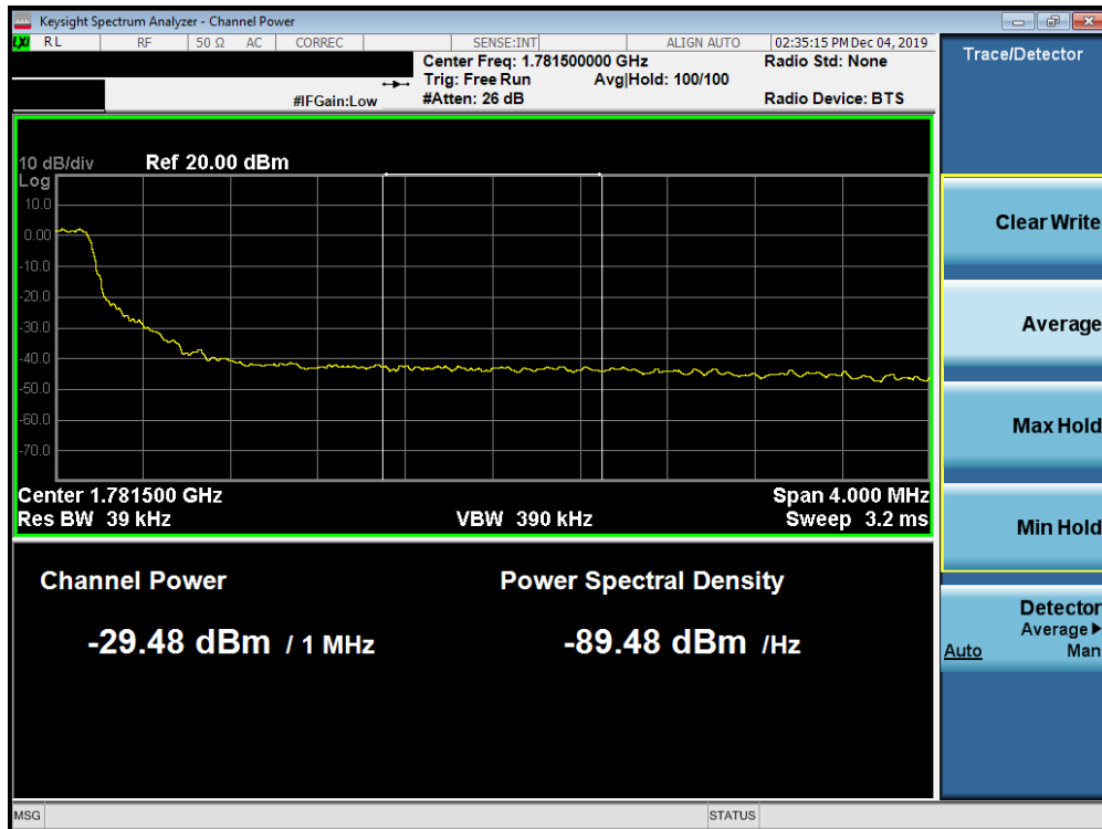
Plot 7-671. Upper Extended Band Edge Plot (Band n66 - 5.0MHz CP-OFDM-QPSK - Full RB Configuration)
