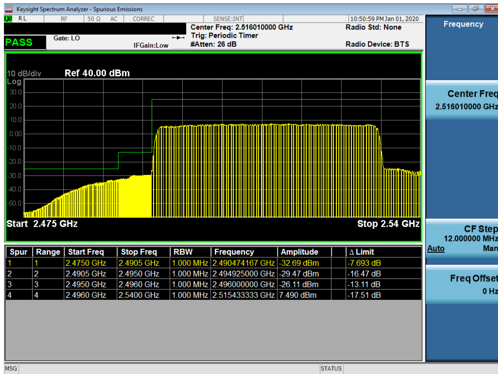
Plot 7-702. Lower ACP Plot at 2496 MHz (n41 - 40MHz DFT-s-OFDM-QPSK - Full RB Configuration)
