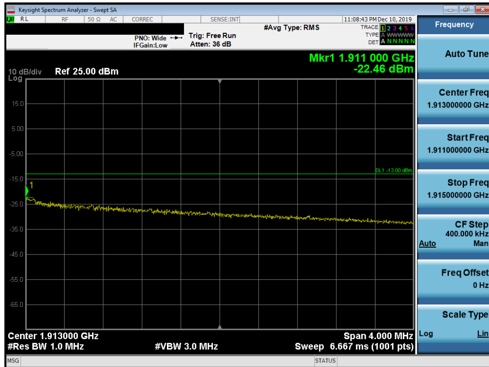
Plot 7-695. Upper Extended Band Edge Plot (Band n2 - 15.0MHz CP-OFDM-QPSK - Full RB Configuration)
