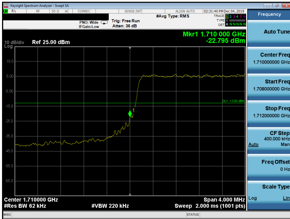
Plot 7-668. Lower Band Edge Plot (Band n66 - 5.0MHz DFT-s-OFDM-QPSK - Full RB Configuration)
