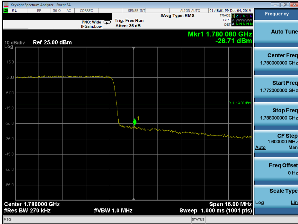
Plot 7-682. Upper Band Edge Plot (Band n66 - 20.0MHz DFT-s-OFDM-QPSK - Full RB Configuration)
