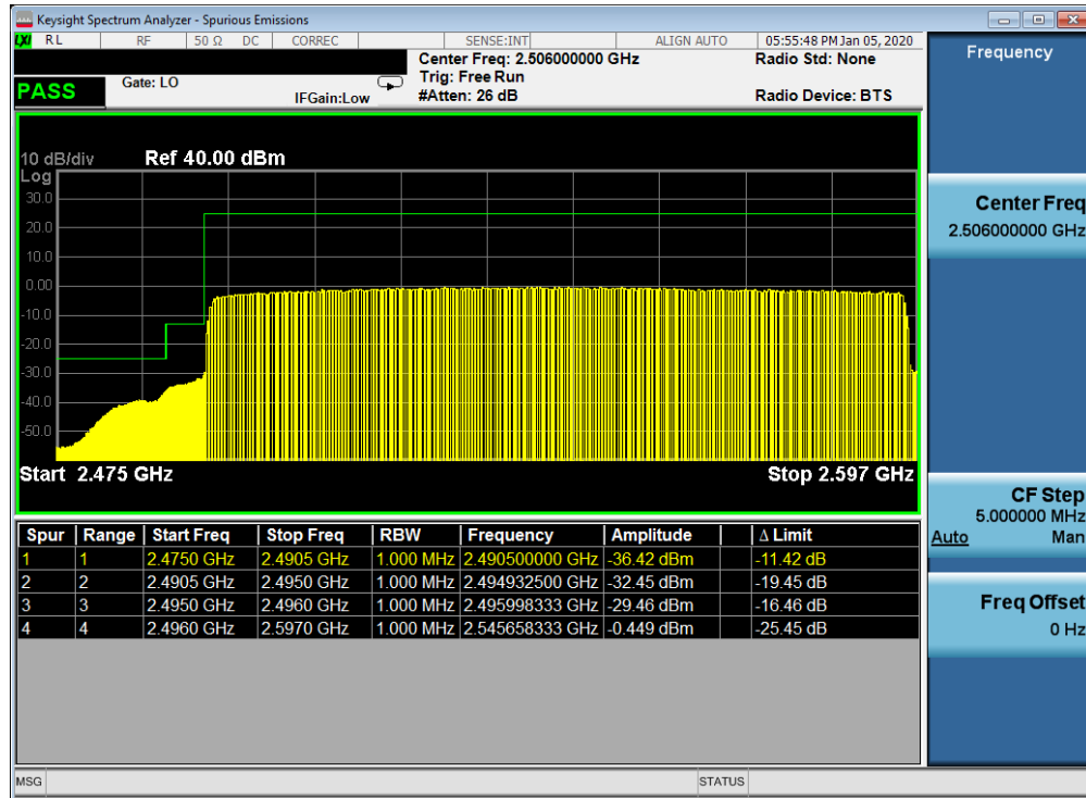
Plot 7-712. Lower ACP Plot at 2496 MHz (n41 - 100MHz CP-OFDM-QPSK - Full RB Configuration)
