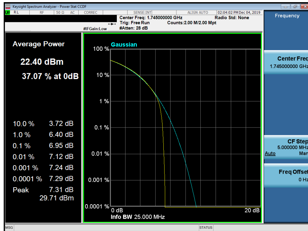
Plot 7-739. PAR Plot (Band n66 - 15.0MHz CP-OFDM- 16-QAM - Full RB Configuration)
