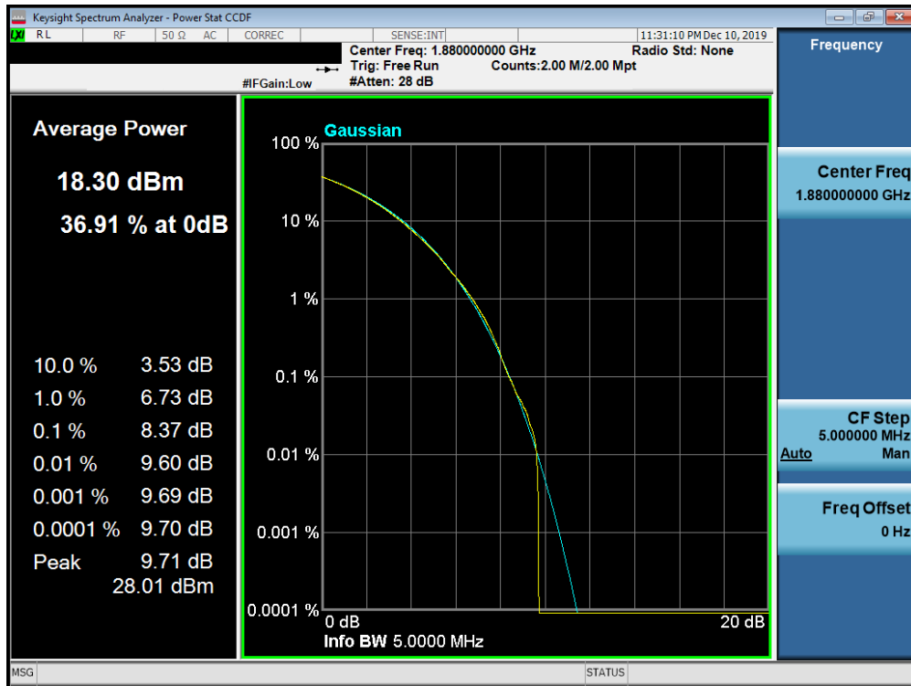
Plot 7-717. PAR Plot (Band n2 - 5.0MHz CP-OFDM- 256-QAM - Full RB Configuration)
