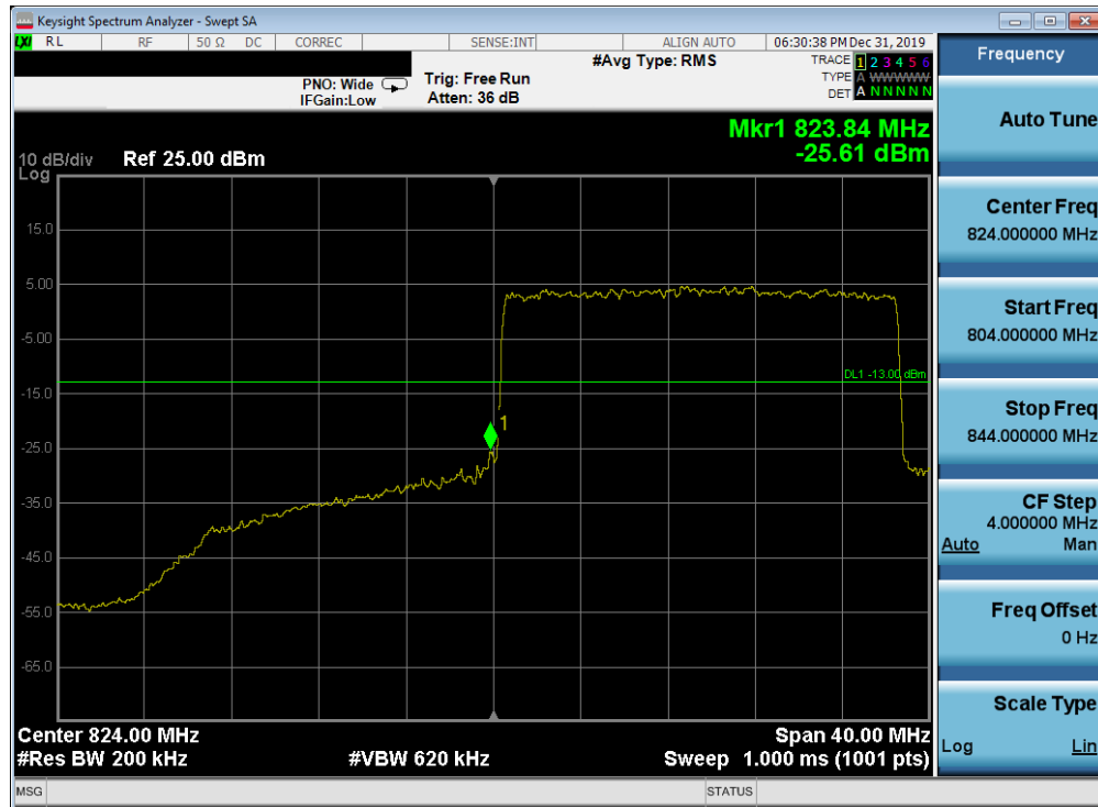
Plot 7-666. Lower Band Edge Plot (n5 - 20MHz DFT-s-OFDM-QPSK - Full RB Configuration)
