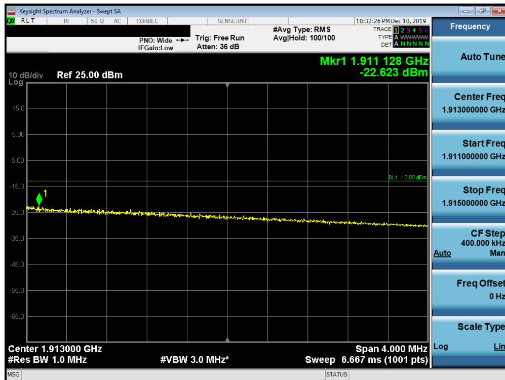
Plot 7-699. Upper Extended Band Edge Plot (Band n2 - 20.0MHz CP-OFDM-QPSK - Full RB Configuration)
