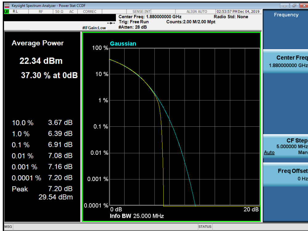
Plot 7-727. PAR Plot (Band n2 - 20.0MHz CP-OFDM-16-QAM - Full RB Configuration)
