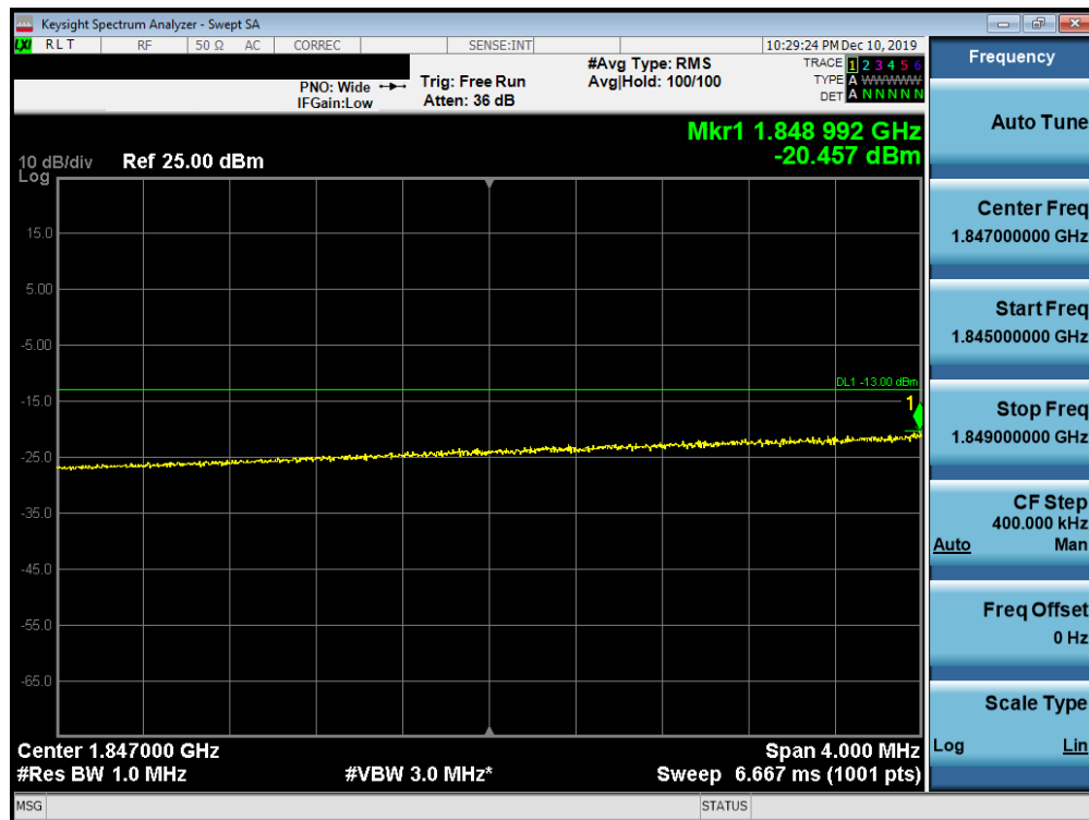
Plot 7-697. Lower Extended Band Edge Plot (Band n2 - 20.0MHz CP-OFDM-QPSK - Full RB Configuration)
