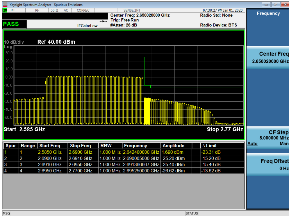
Plot 7-709. Upper ACP Plot (n41 - 80MHz DFT-s-OFDM-QPSK - Full RB Configuration)
