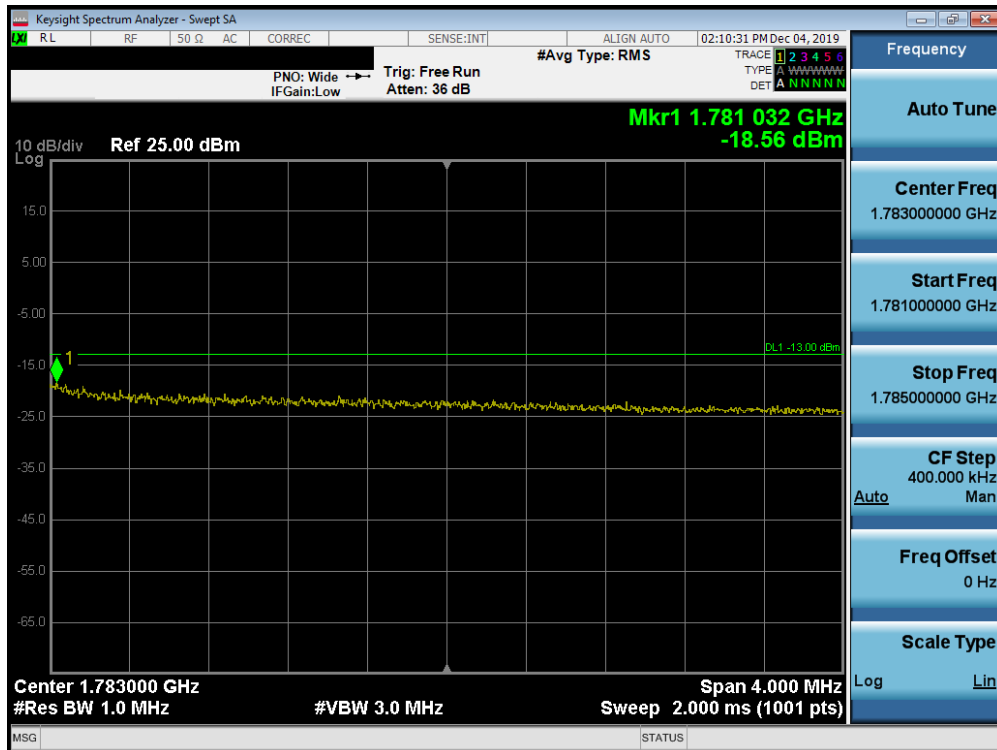
Plot 7-679. Upper Extended Band Edge Plot (Band n66 - 15.0MHz CP-OFDM-QPSK - Full RB Configuration)
