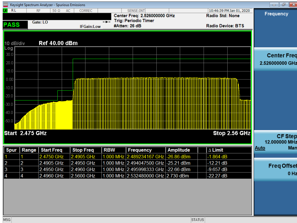
Plot 7-706. Lower ACP Plot at 2496 MHz (n41 - 60MHz CP-OFDM-QPSK - Full RB Configuration)
