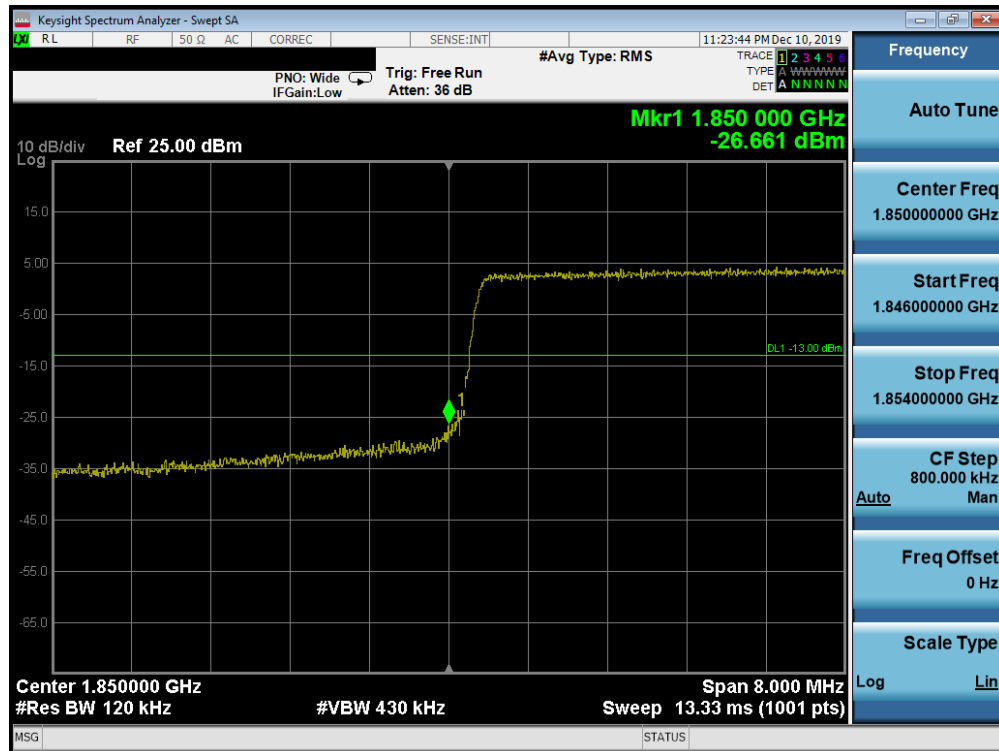
Plot 7-688. Lower Band Edge Plot (Band n2 - 10.0MHz CP-OFDM-QPSK - Full RB Configuration)
