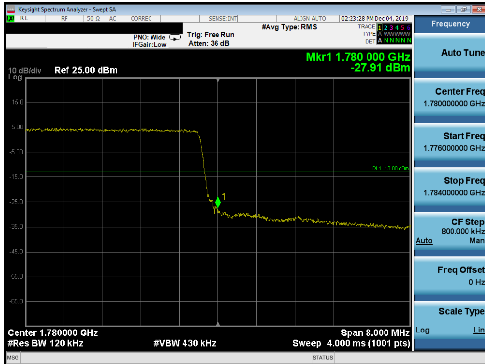
Plot 7-674. Upper Band Edge Plot (Band n66 - 10.0MHz CP-OFDM-QPSK - Full RB Configuration)
