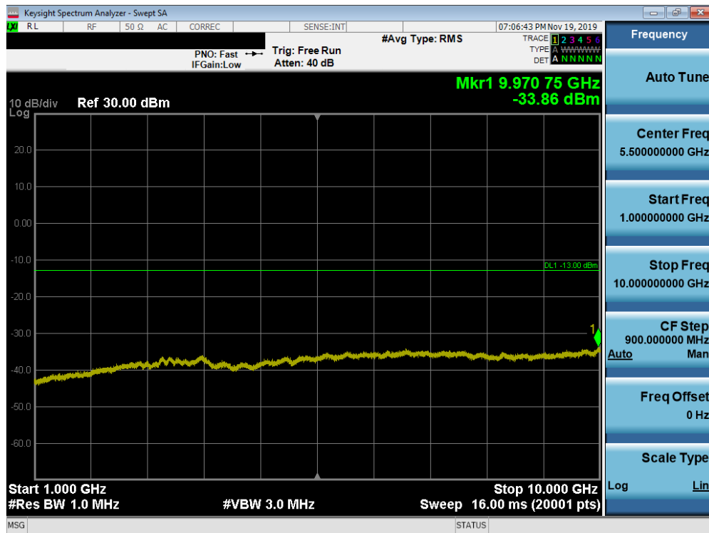
Plot 7-33. Conducted Spurious Plot (LTE Band 26 - 15MHz QPSK - RB Size 1, RB Offset 0 - Mid Channel)
