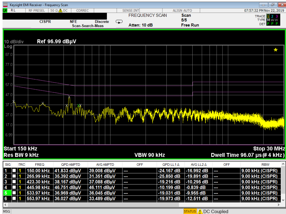
Plot 7-16. Line Conducted Plot (N)
