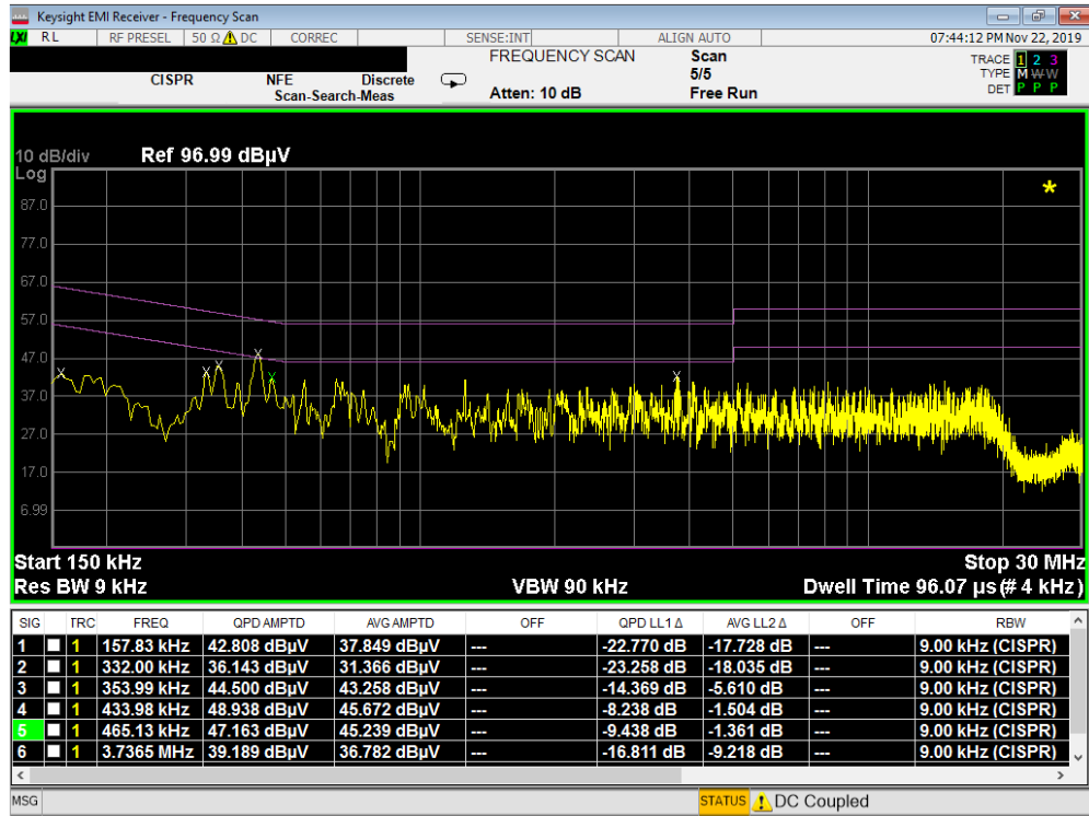
Plot 7-11. Line Conducted Plot (L1)
