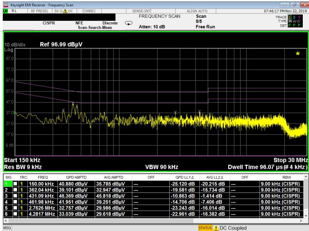
Plot 7-12. Line Conducted Plot (N)
