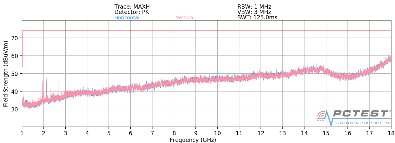
Plot 7-8. Radiated Spurious Plot above 1GHz [Radiated Test Config. 4]
