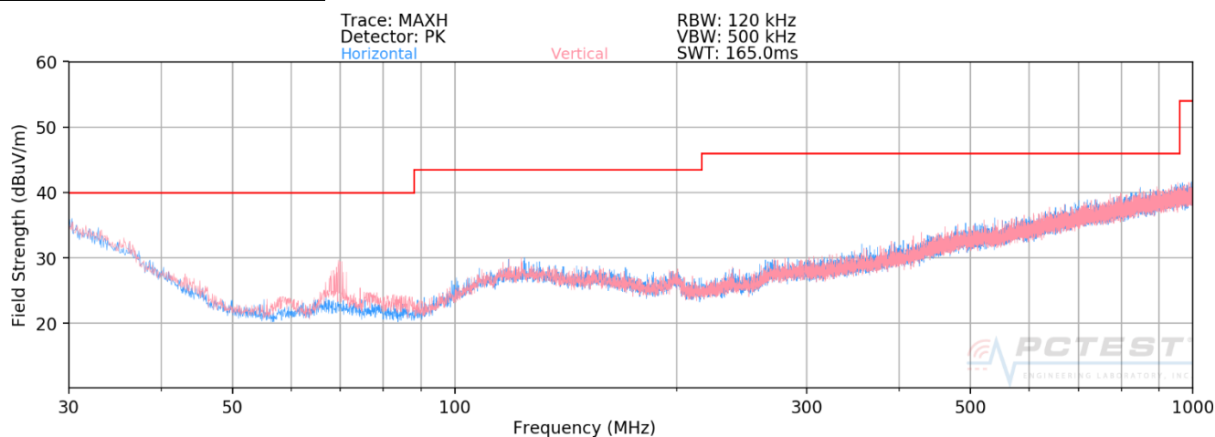
Plot 7-9. Radiated Spurious Plot below 1GHz [Radiated Test Config. 5]
