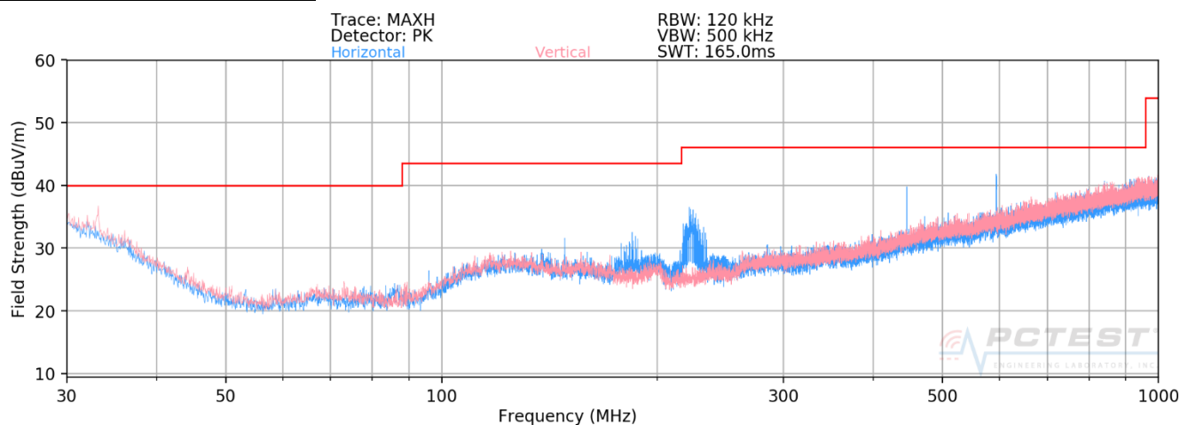
Plot 7-5. Radiated Spurious Plot below 1GHz [Radiated Test Config. 3]
