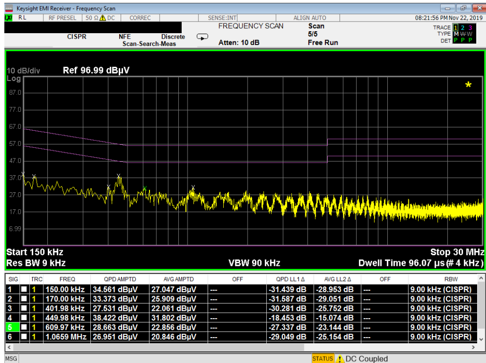
Plot 7-20. Line Conducted Plot (N)
