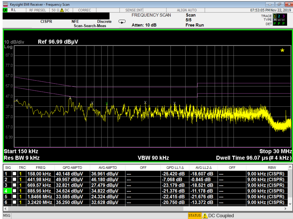
Plot 7-13. Line Conducted Plot (L1)
