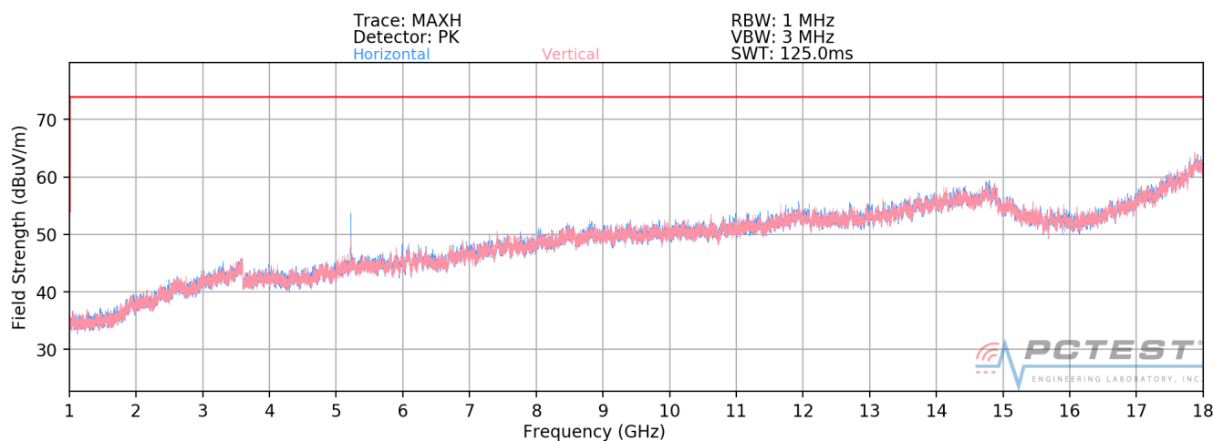
Plot 7-10. Radiated Spurious Plot above 1GHz [Radiated Test Config. 5]
