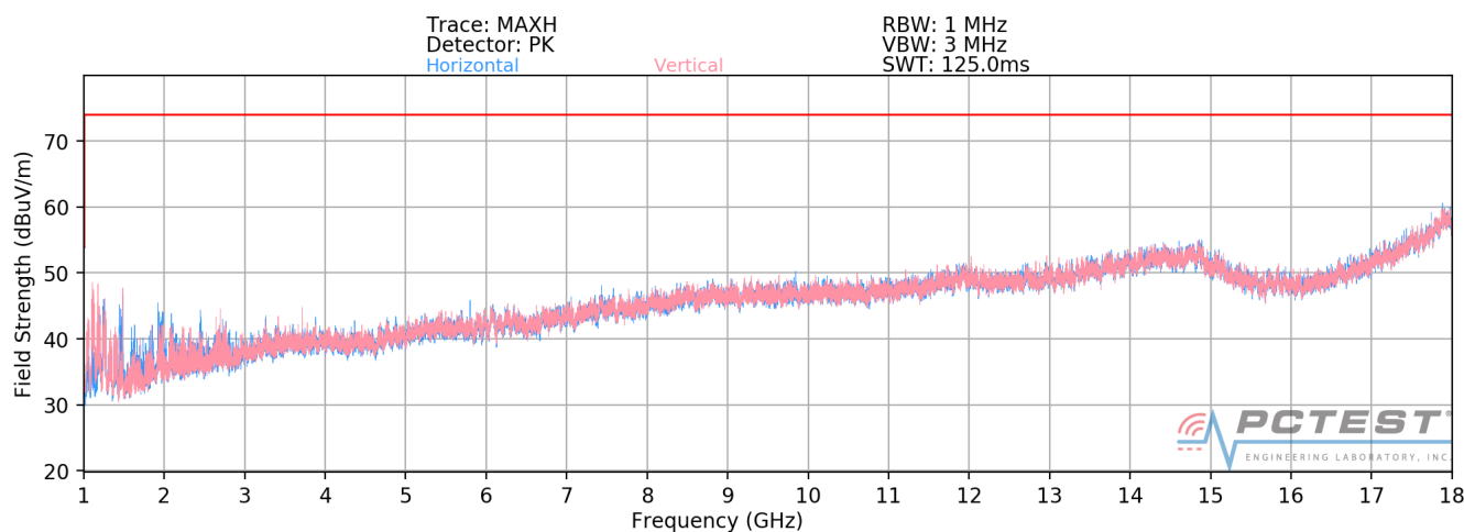
Plot 7-6. Radiated Spurious Plot above 1GHz [Radiated Test Config. 3]
