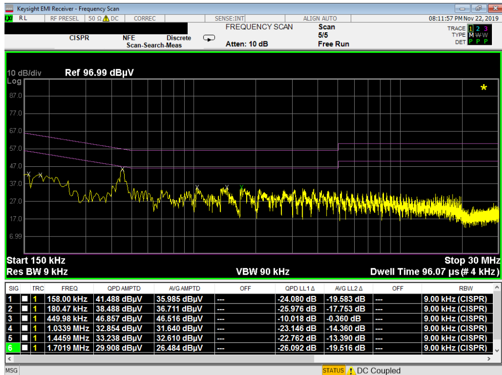
Plot 7-18. Line Conducted Plot (N)
