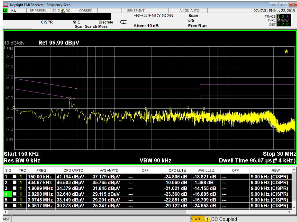
Plot 7-14. Line Conducted Plot (N)
