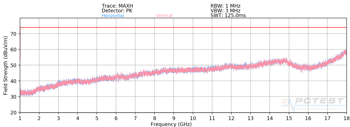
Plot 7-2. Radiated Spurious Plot above 1GHz [Radiated Test Config. 1]
