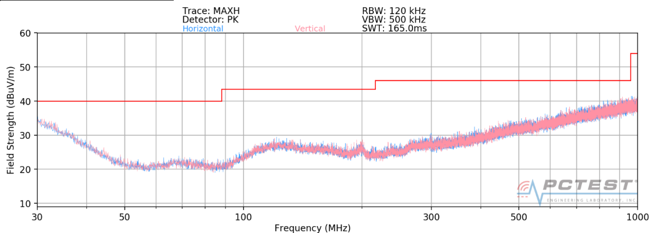
Plot 7-3. Radiated Spurious Plot below 1GHz [Radiated Test Config. 2]
