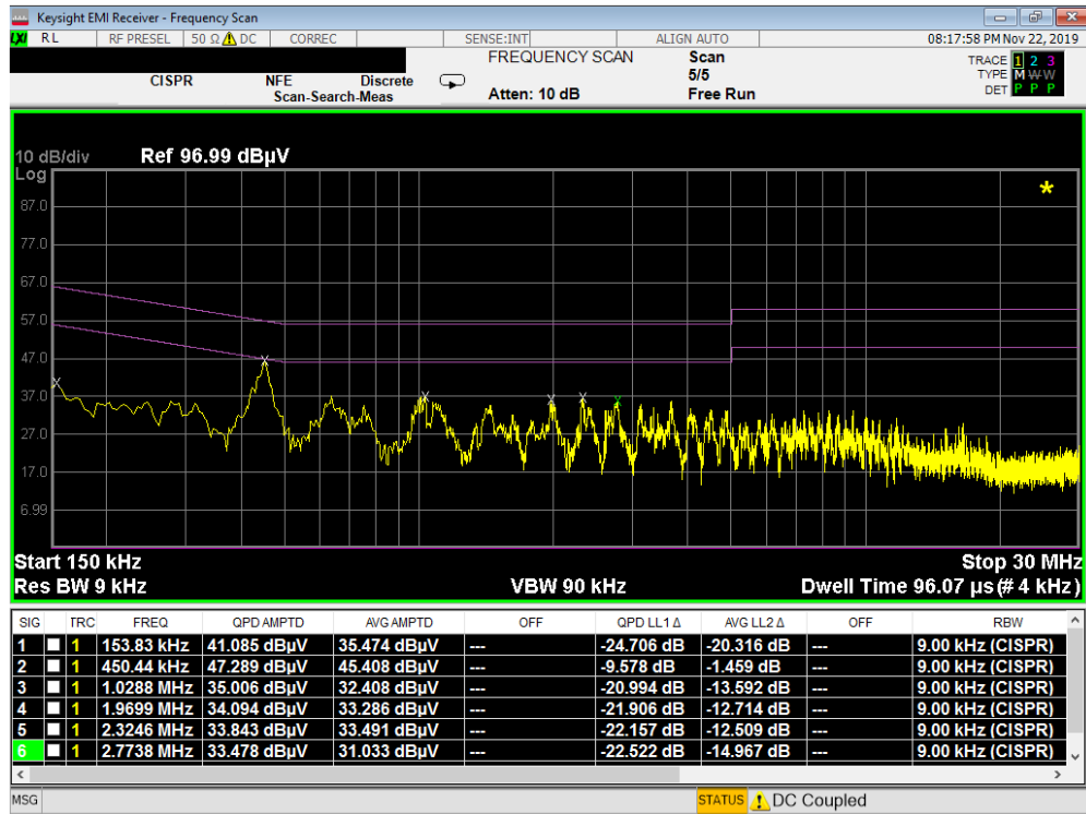
Plot 7-17. Line Conducted Plot (L1)
