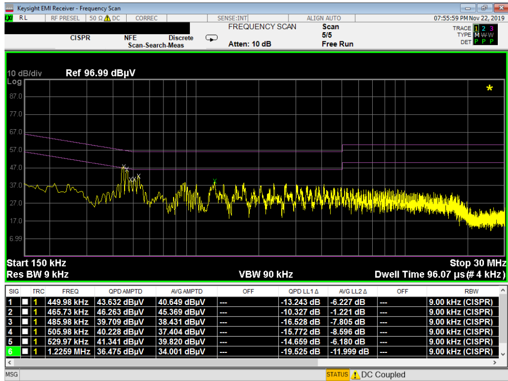
Plot 7-15. Line Conducted Plot (L1)
