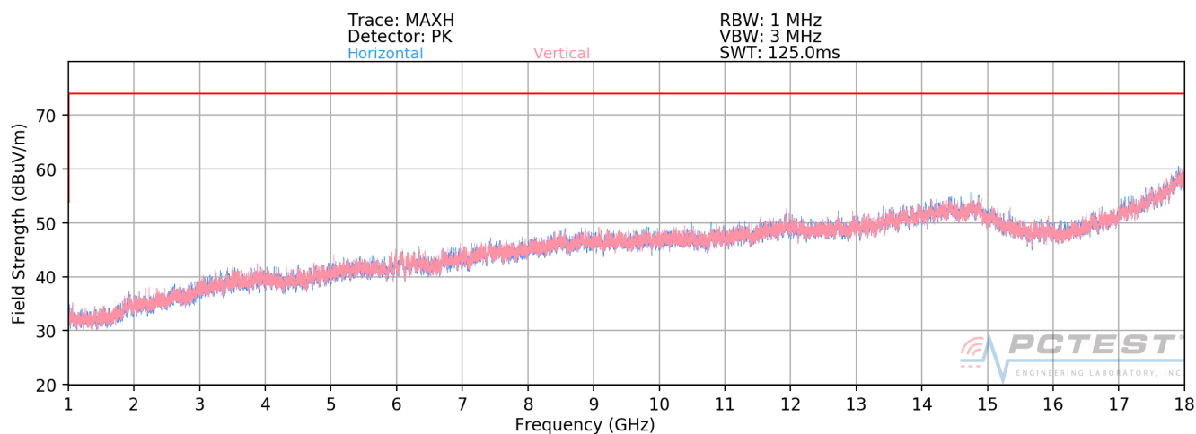
Plot 7-4. Radiated Spurious Plot above 1GHz [Radiated Test Config. 2]
