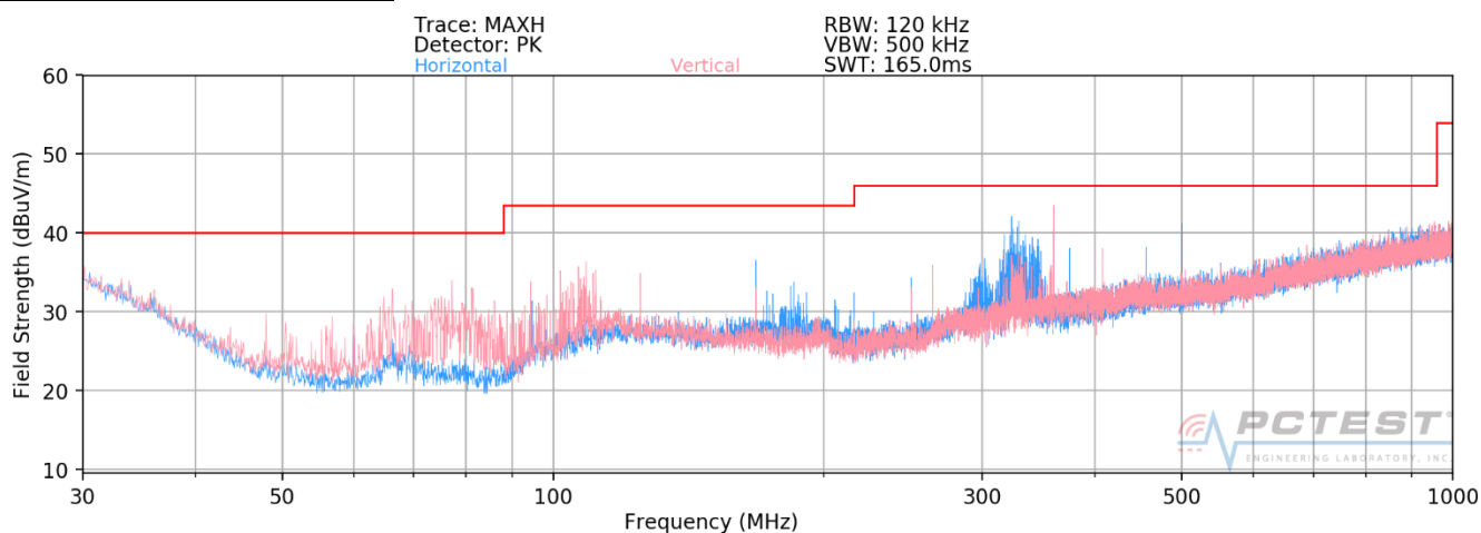
Plot 7-7. Radiated Spurious Plot below 1GHz [Radiated Test Config. 4]
