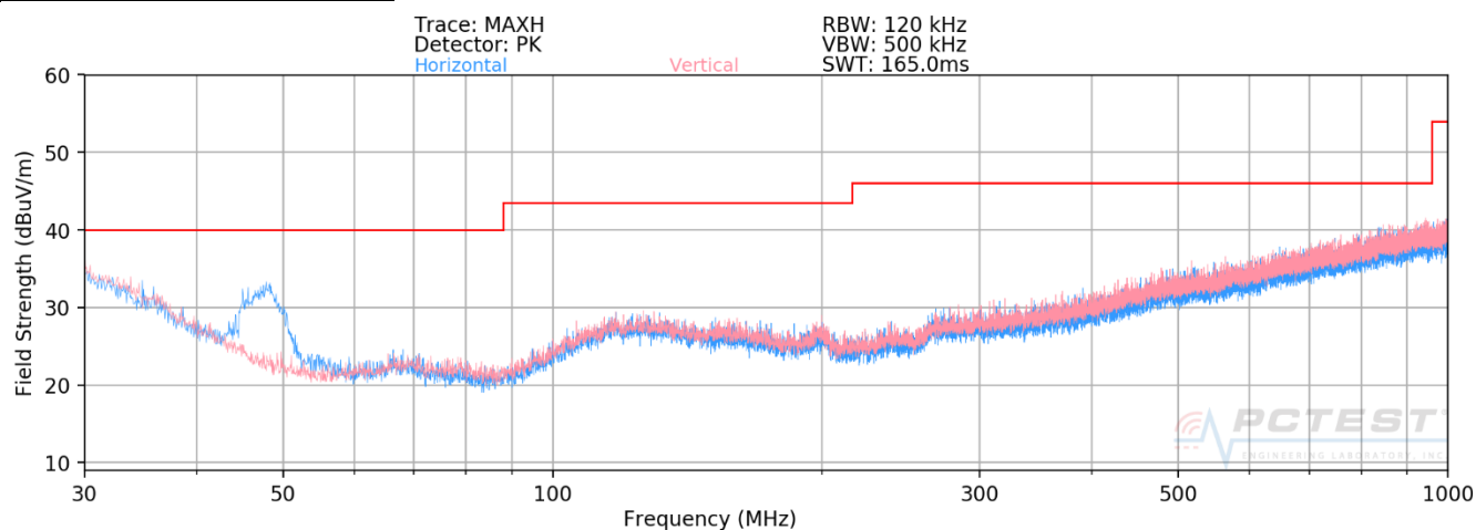
Plot 7-1. Radiated Spurious Plot below 1GHz [Radiated Test Config. 1]
