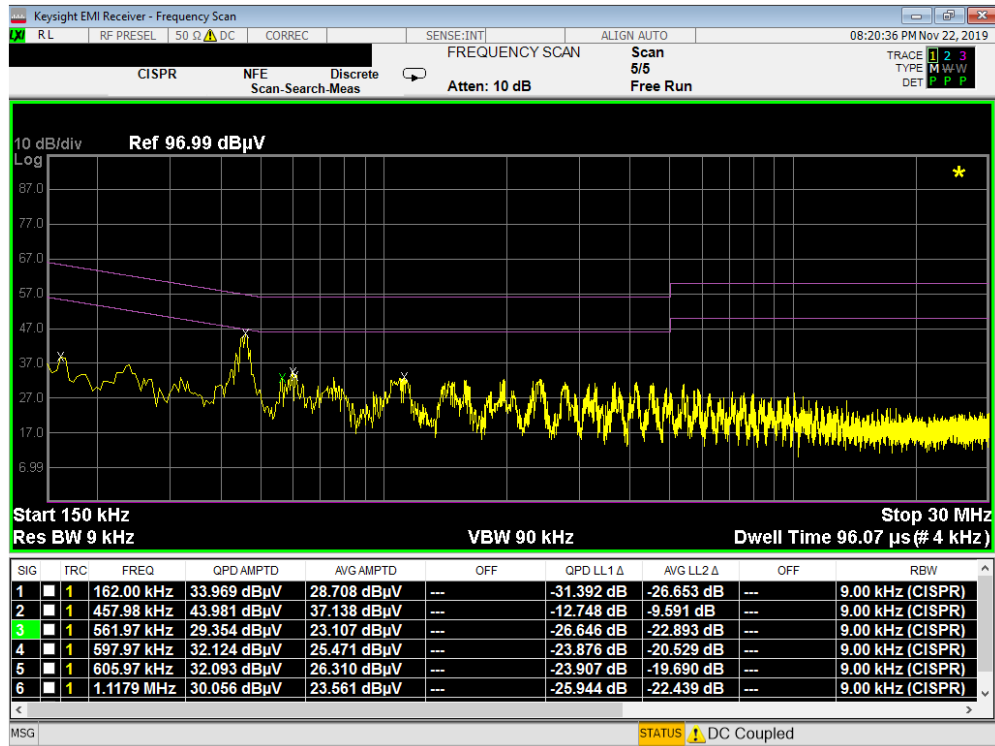
Plot 7-19. Line Conducted Plot (L1)
