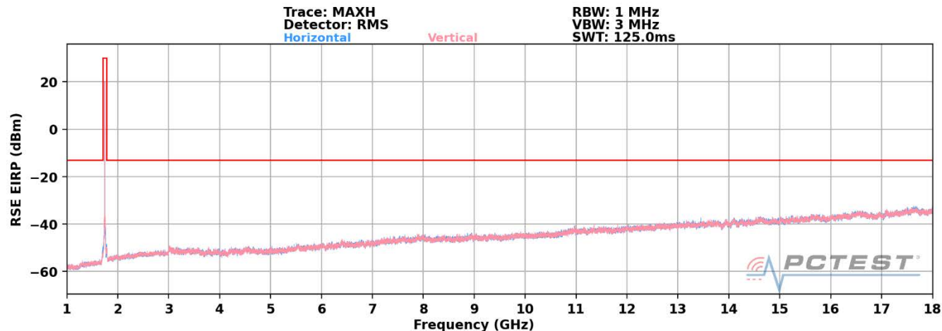
Plot 7-90. Radiated Spurious Plot above 1GHz (EN-DC n66+LTE B13)
