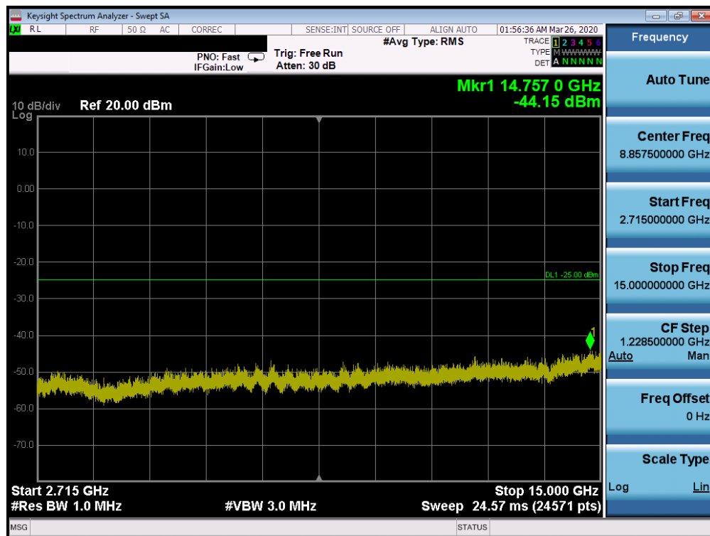
Plot 7-67. Conducted Spurious Plot (n41 - 100MHz DFT-s-OFDM-BPSK - RB Size 1, RB Offset 1 - High Channel)
