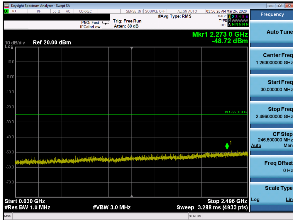
Plot 7-66. Conducted Spurious Plot (n41 - 100MHz DFT-s-OFDM-BPSK - RB Size 1, RB Offset 1 - High Channel)
