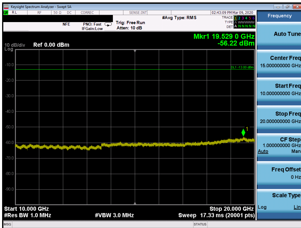
Plot 7-47. Conducted Spurious Plot (n66 - 20MHz DFT-s-OFDM-BPSK - RB Size 1, RB Offset 1 - Mid Channel)
