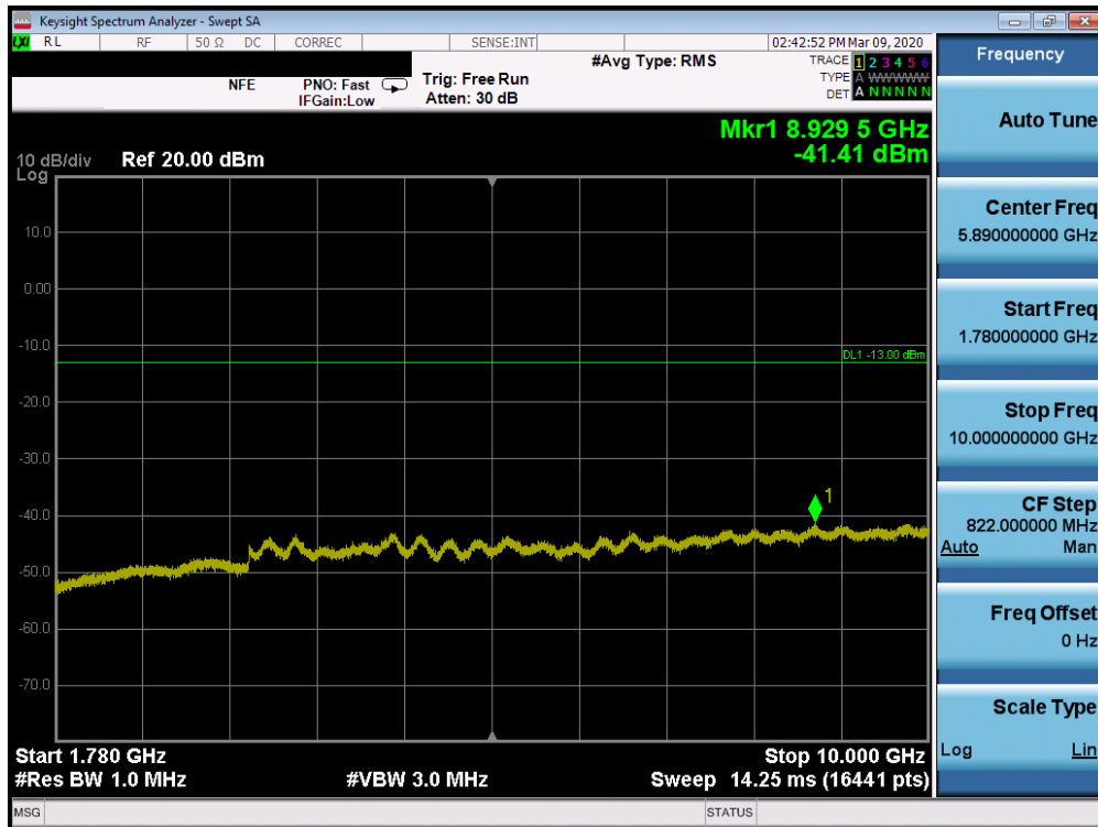
Plot 7-46. Conducted Spurious Plot (n66 - 20MHz DFT-s-OFDM-BPSK - RB Size 1, RB Offset 1 - Mid Channel)
