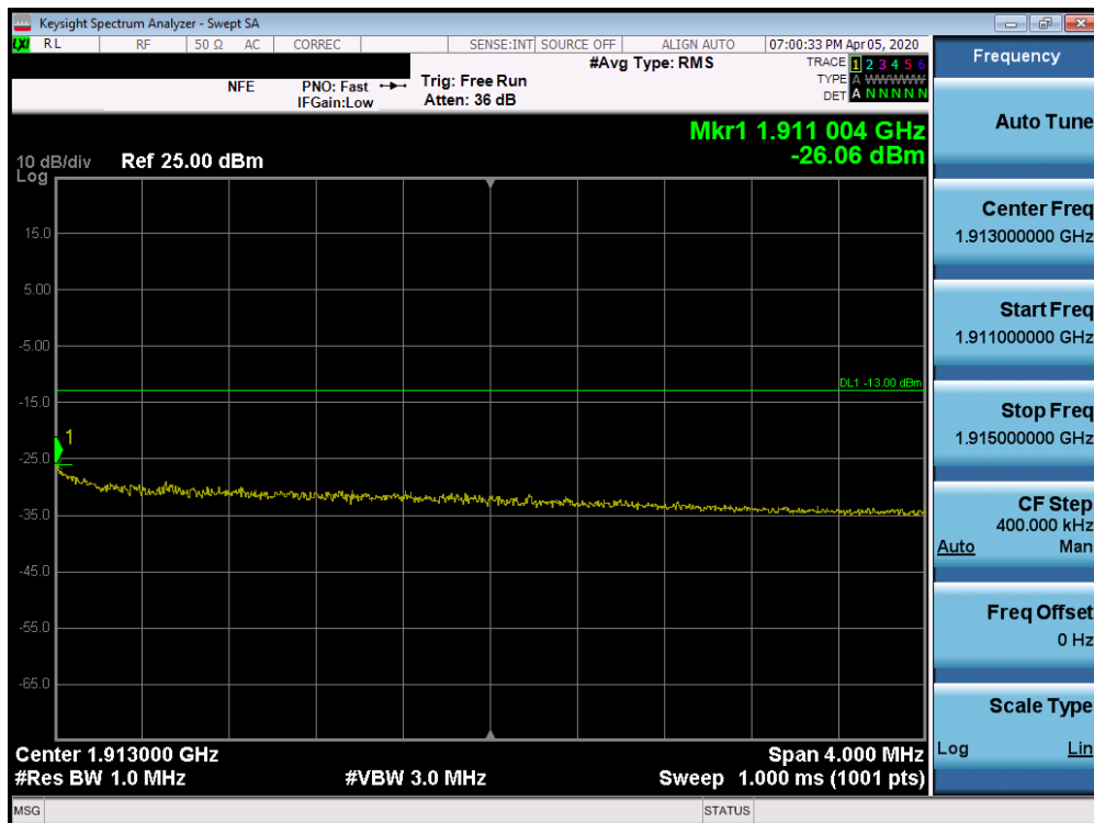
Plot 7-80. Upper Extended Band Edge Plot (n2 - 20MHz DFT-s-OFDM-BPSK - Full RB Configuration)
