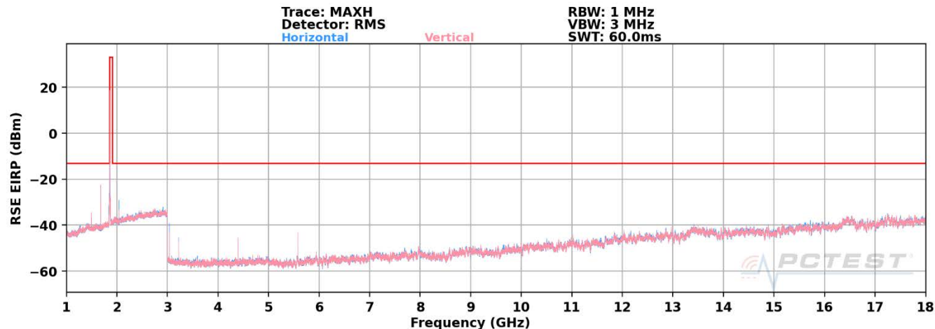
Plot 7-88. Radiated Spurious Plot above 1GHz (EN-DC n71 + LTE B2)
