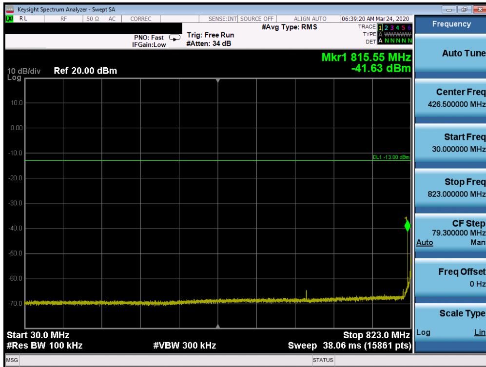
Plot 7-33. Conducted Spurious Plot (n5 - 20MHz DFT-s-OFDM-QPSK - RB Size 1, RB Offset 1 – Low Channel)
