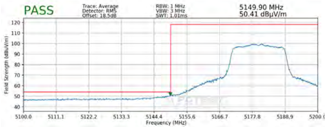
Plot 7-328. Radiated Lower Band Edge Plot MIMO (Average – UNII Band 1)
