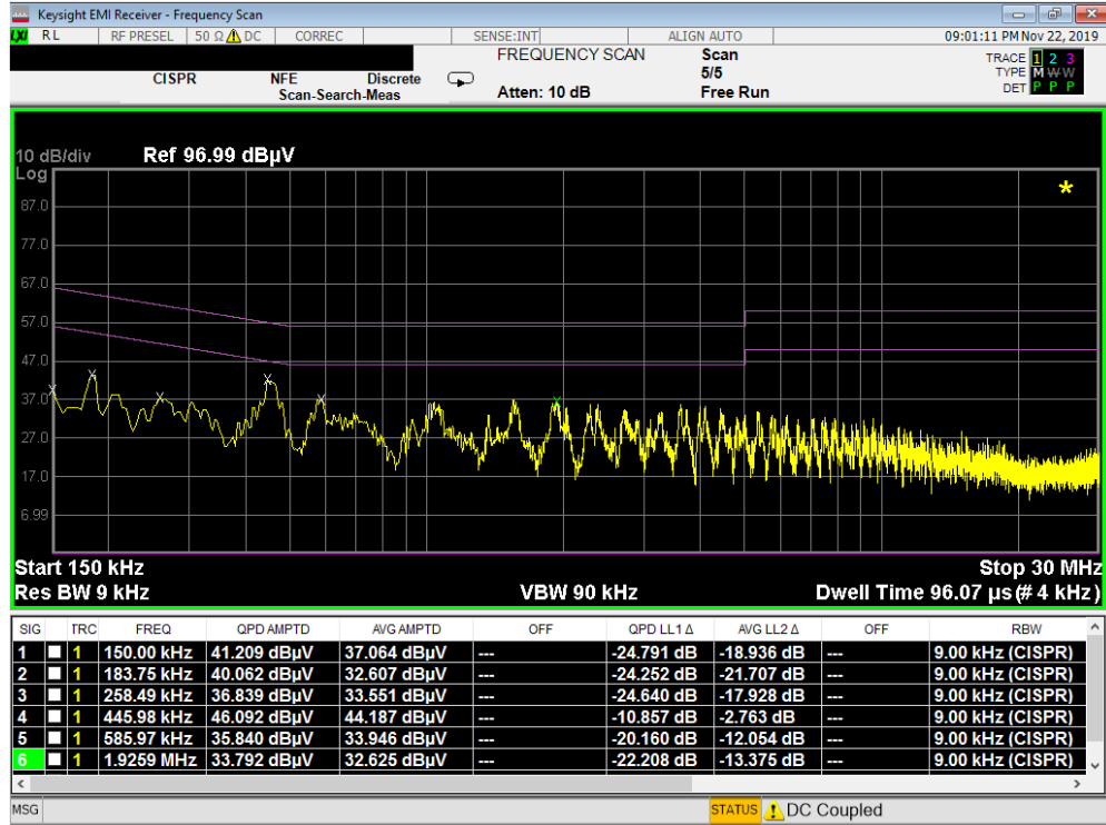
Plot 7-364. Line Conducted Plot with 802.11a UNII Band 3 (L1)
