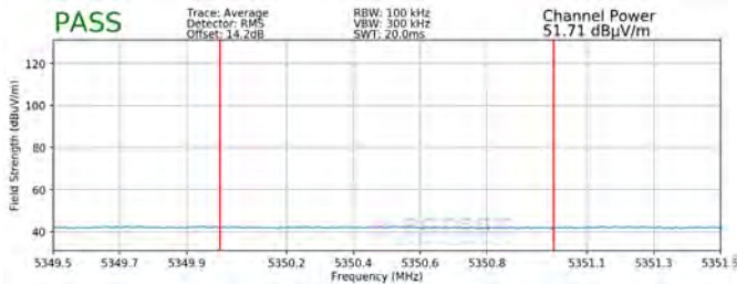
Plot 7-302. Radiated Upper Band Edge Plot SISO ANT1 (Average - UNII Band 2A)
