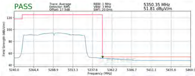
Plot 7-323. Radiated Upper Band Edge Plot SISO ANT2 (Average – UNII Band 2A)
