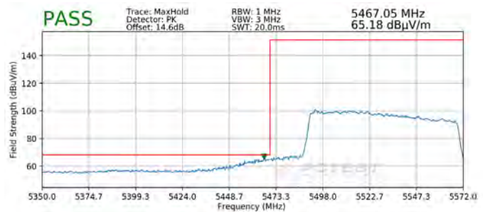
Plot 7-351. Radiated Lower Band Edge Plot MIMO (Peak – UNII Band 2C)
