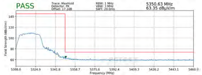
Plot 7-331. Radiated Upper Band Edge Plot MIMO (Peak – UNII Band 2A)
