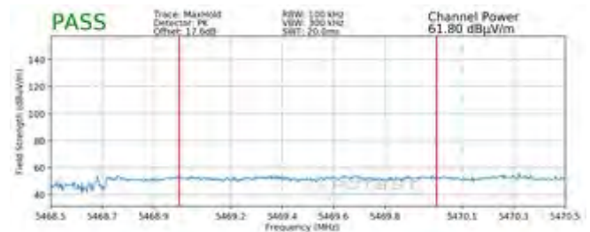
Plot 7-336. Radiated Band Edge Plot MIMO (Peak – WCP)
