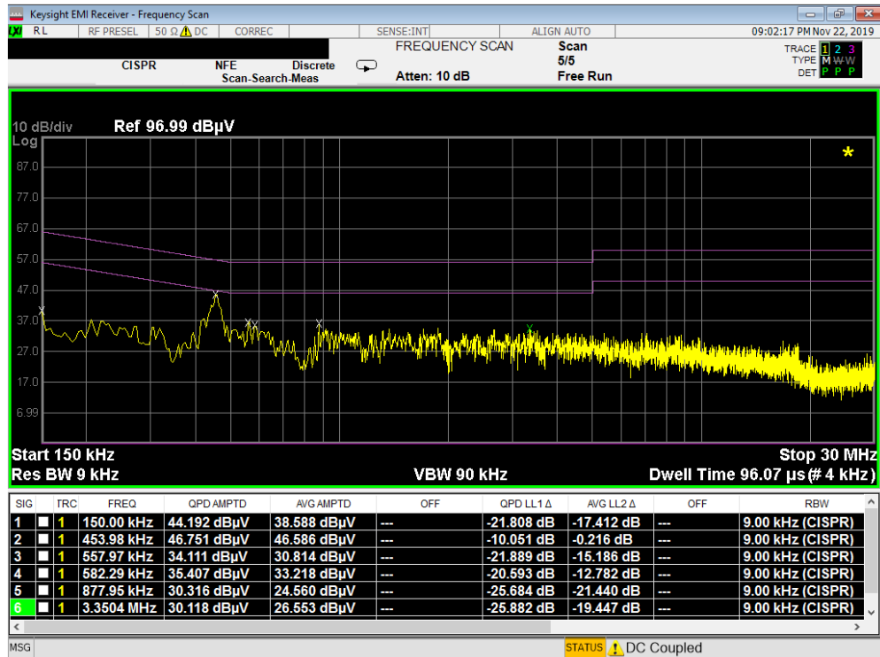
Plot 7-365. Line Conducted Plot with 802.11a UNII Band 3 (N)
