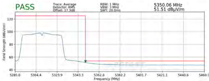
Plot 7-316. Radiated Upper Band Edge Plot SISO ANT2 (Average – UNII Band 2A)
