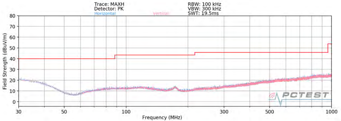
Plot 7-356. Radiated Spurious Plot below 1GHz (2.4GHz – 5GHz)
