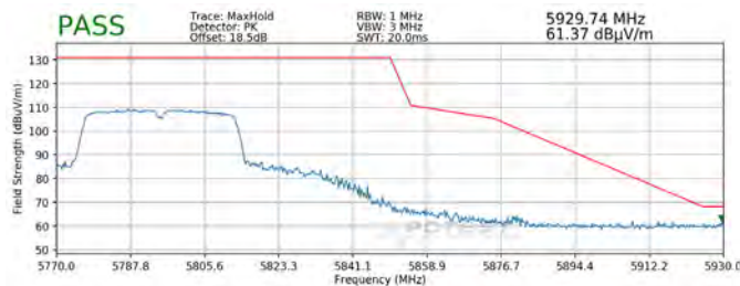
Plot 7-320. Radiated Upper Band Edge Plot SISO ANT2 (Peak – UNII Band 3)
