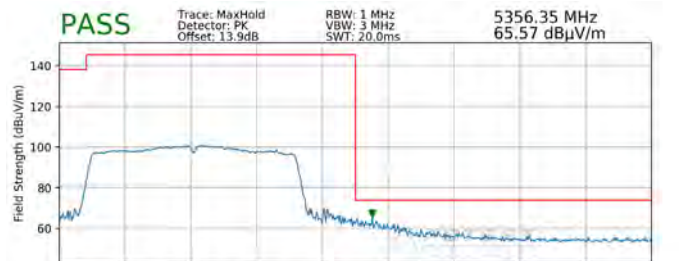
Plot 7-324. Radiated Upper Band Edge Plot SISO ANT2 (Peak – UNII Band 2A)
