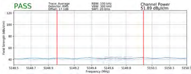
Plot 7-314. Radiated Lower Band Edge Plot SISO ANT2 (Average – UNII Band 1)
