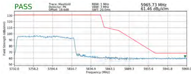
Plot 7-352. Radiated Upper Band Edge Plot MIMO (Peak – UNII Band 3)
