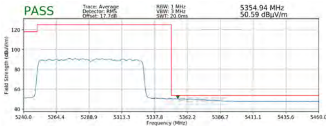
Plot 7-348. Radiated Upper Band Edge Plot MIMO (Average – UNII Band 2A)
