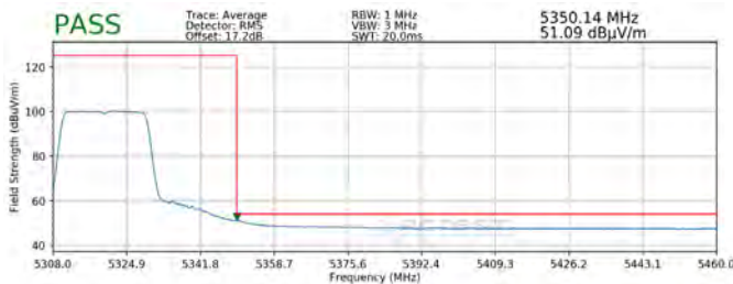
Plot 7-309. Radiated Upper Band Edge Plot SISO ANT2 (Average – UNII Band 2A)
