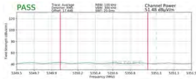
Plot 7-344. Radiated Band Edge Plot MIMO (Average – WCP)
