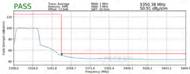
Plot 7-288. Radiated Upper Band Edge Plot SISO ANT1 (Average – UNII Band 2A)
