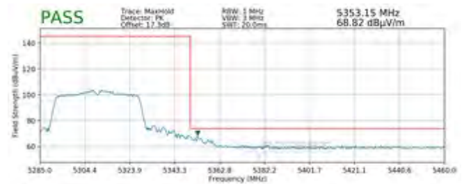
Plot 7-345. Radiated Band Edge Plot MIMO (Peak – WCP)
