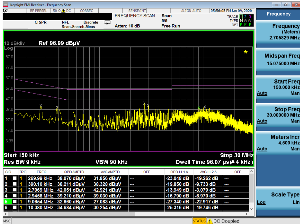
Plot 7-371. Line Conducted Plot with 802.11a UNII Band 2C with WCP (N)
