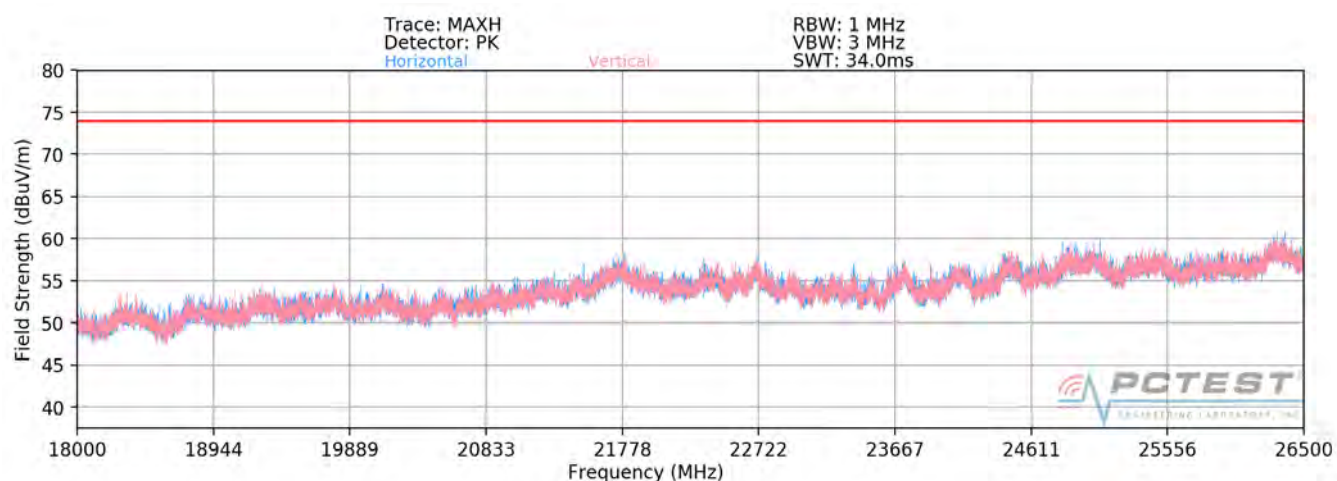
Plot 7-278. Radiated Spurious Plot 18GHz – 26.5GHz (2.4GHz – 5GHz)
