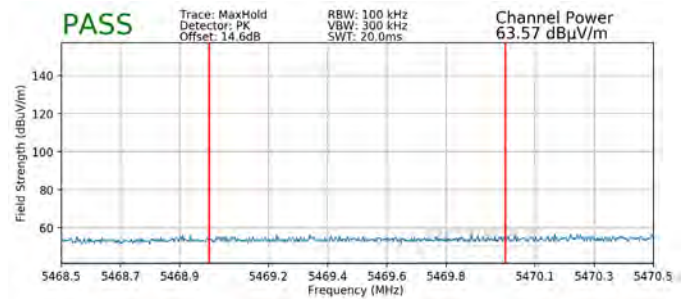
Plot 7-312. Radiated Lower Band Edge Plot SISO ANT2 (Peak - UNII Band 2C)
