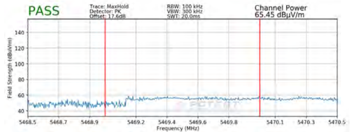
Plot 7-319. Radiated Lower Band Edge Plot SISO ANT2 (Peak – UNII Band 2C)
