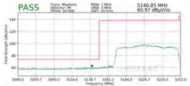
Plot 7-354. Radiated Band Edge Plot MIMO (Peak – WCP)
