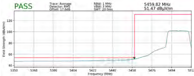
Plot 7-311. Radiated Lower Band Edge Plot SISO ANT2 (Average - UNII Band 2C)
