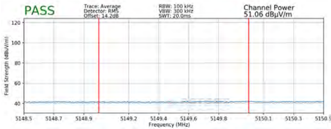
Plot 7-300. Radiated Lower Band Edge Plot SISO ANT1 (Average - UNII Band 1)
