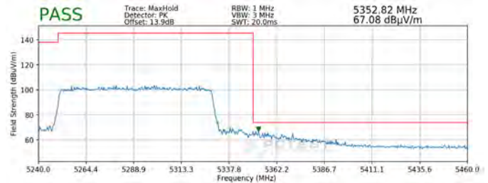
Plot 7-303. Radiated Upper Band Edge Plot SISO ANT1 (Peak - UNII Band 2A)
