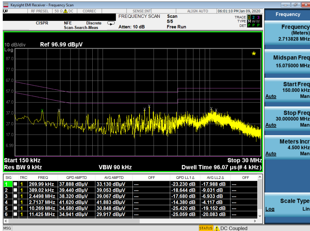
Plot 7-373. Line Conducted Plot with 802.11a UNII Band 3 with WCP (N)
