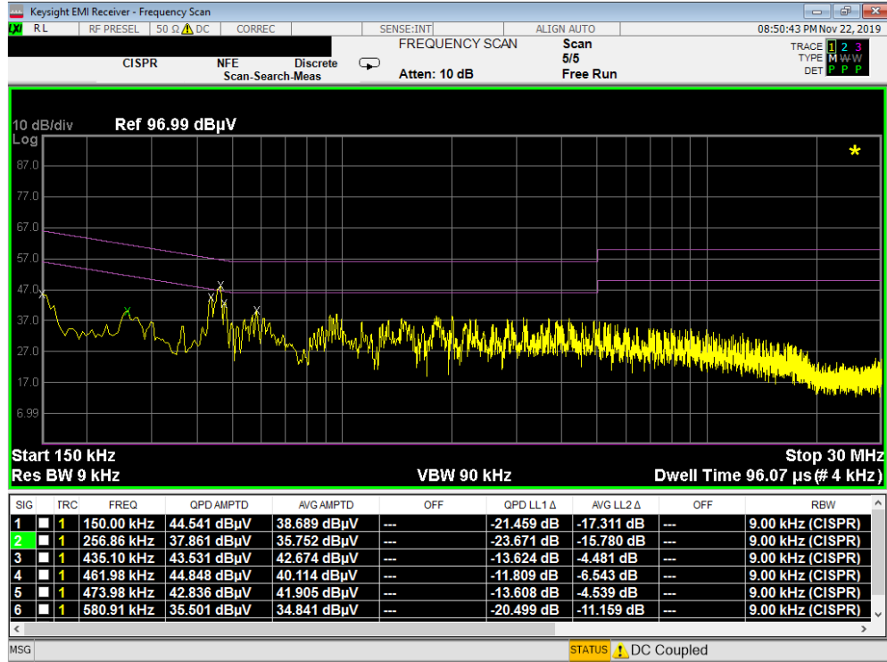
Plot 7-360. Line Conducted Plot with 802.11a UNII Band 2A (L1)
