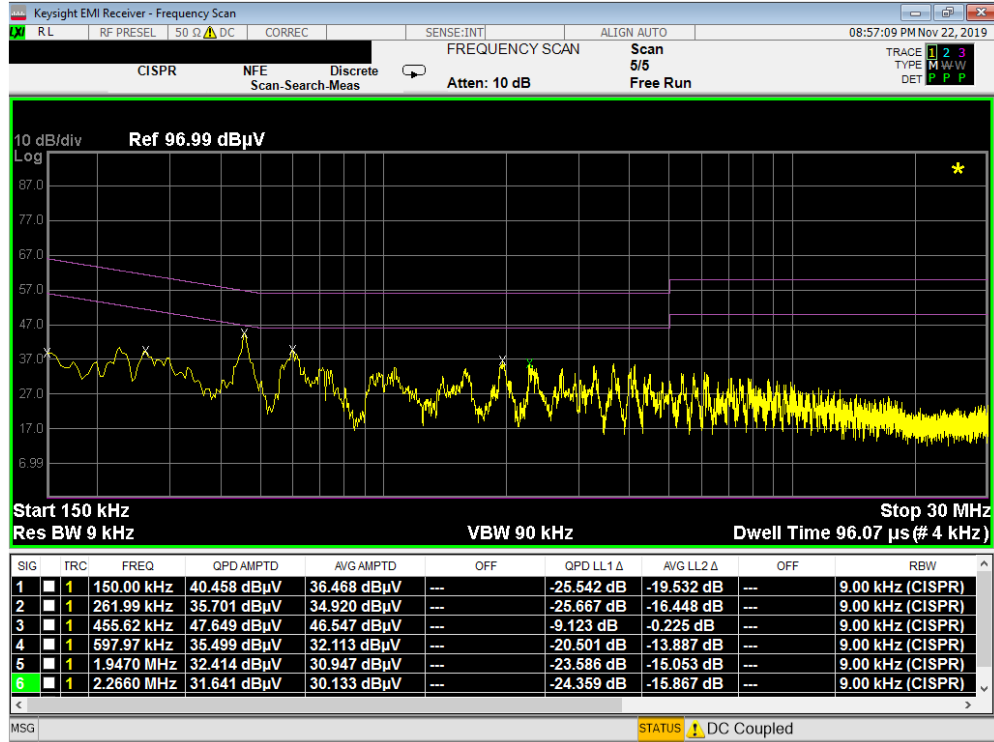
Plot 7-362. Line Conducted Plot with 802.11a UNII Band 2C (L1)
