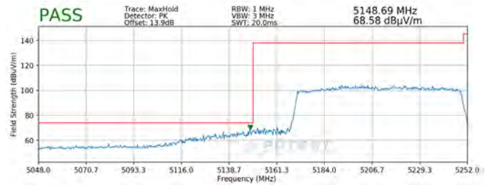
Plot 7-301. Radiated Lower Band Edge Plot SISO ANT1 (Peak - UNII Band 1)
