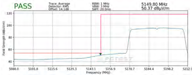
Plot 7-293. Radiated Lower Band Edge Plot SISO ANT1 (Average – UNII Band 1)
