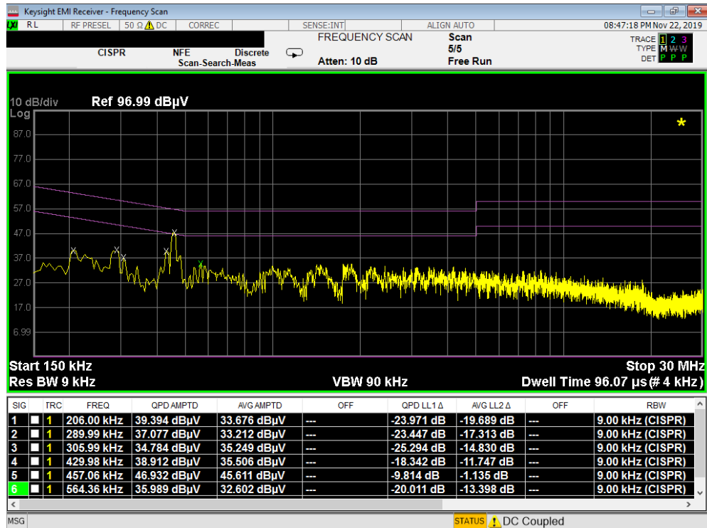
Plot 7-361. Line Conducted Plot with 802.11a UNII Band 2A (N)
