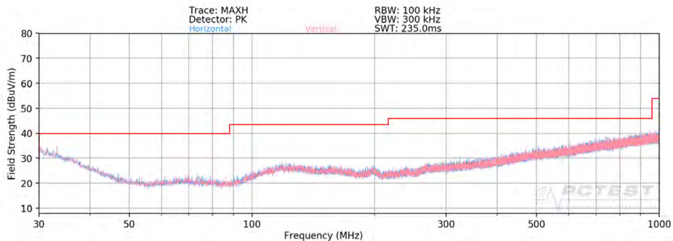
Plot 7-355. Radiated Spurious Plot below 1GHz MIMO (802.11a – U3 Ch. 157)
