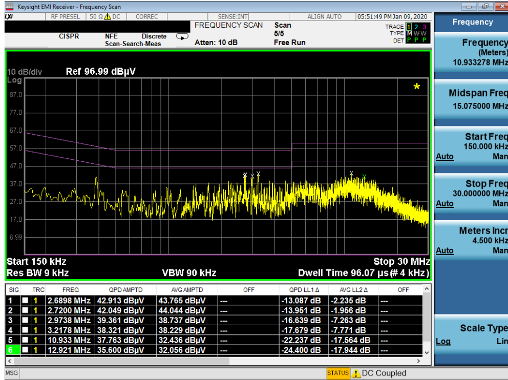
Plot 7-368. Line Conducted Plot with 802.11a UNII Band 2A with WCP (L1)
