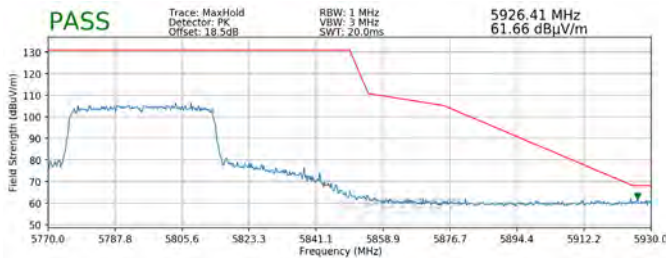
Plot 7-299. Radiated Upper Band Edge Plot SISO ANT1 (Peak - UNII Band 3)
