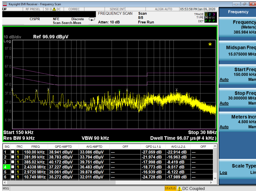
Plot 7-369. Line Conducted Plot with 802.11a UNII Band 2A with WCP (N)
