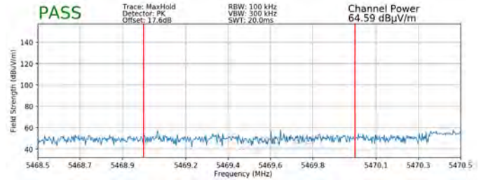
Plot 7-333. Radiated Lower Band Edge Plot MIMO (Peak – UNII Band 2C)
