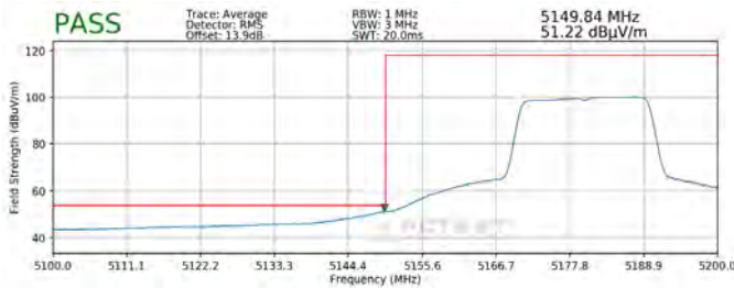
Plot 7-286. Radiated Lower Band Edge Plot SISO ANT1 (Average – UNII Band 1)
