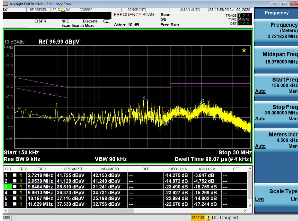
Plot 7-366. Line Conducted Plot with 802.11a UNII Band 1 with WCP (L1)
