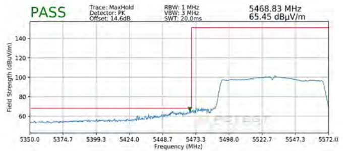
Plot 7-326. Radiated Lower Band Edge Plot SISO ANT2 (Peak - UNII Band 2C)
