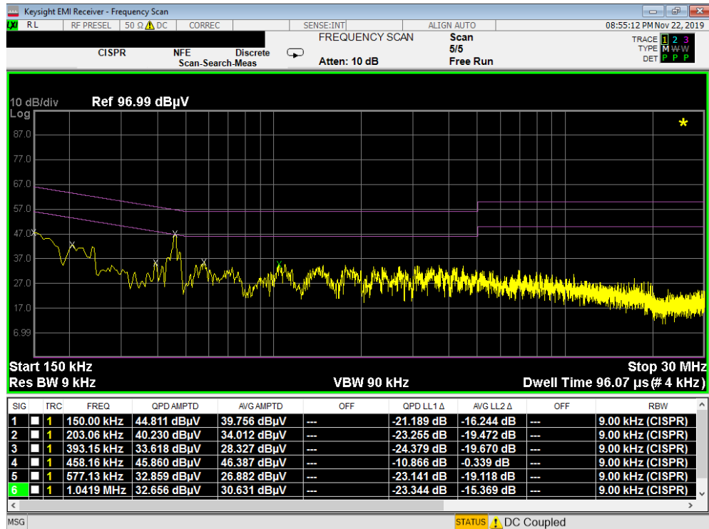
Plot 7-363. Line Conducted Plot with 802.11a UNII Band 2C (N)
