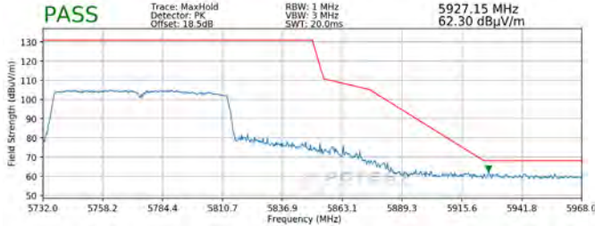
Plot 7-327. Radiated Upper Band Edge Plot SISO ANT2 (Peak - UNII Band 3)
