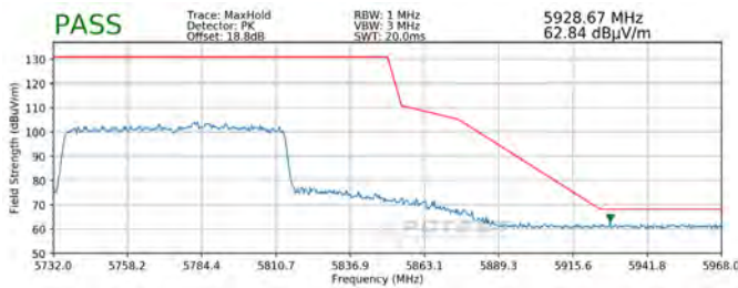
Plot 7-306. Radiated Upper Band Edge Plot SISO ANT1 (Peak – UNII Band 3)
