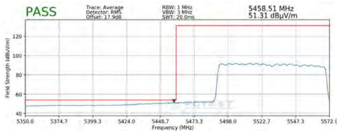
Plot 7-350. Radiated Lower Band Edge Plot MIMO (Average – UNII Band 2C)
