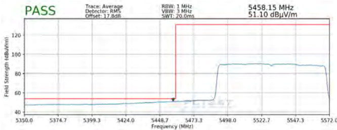
Plot 7-304. Radiated Lower Band Edge Plot SISO ANT1 (Average – UNII Band 2C)
