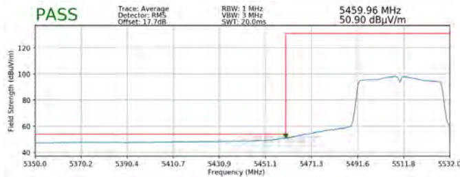
Plot 7-318. Radiated Lower Band Edge Plot SISO ANT2 (Average – UNII Band 2C)
