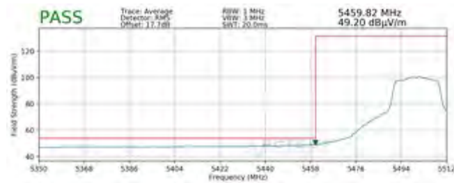
Plot 7-335. Radiated Band Edge Plot MIMO (Average – WCP)
