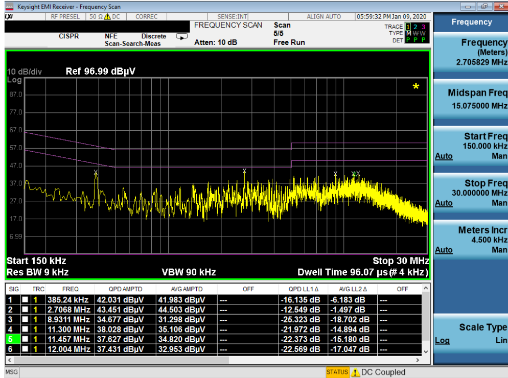
Plot 7-372. Line Conducted Plot with 802.11a UNII Band 3 with WCP (L1)
