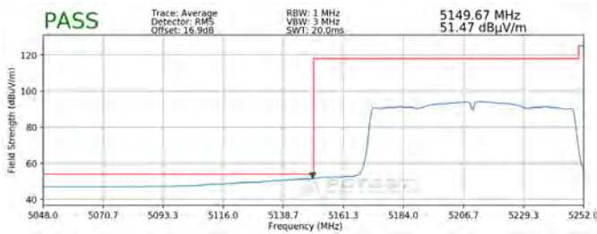
Plot 7-321. Radiated Lower Band Edge Plot SISO ANT2 (Average – UNII Band 1)
