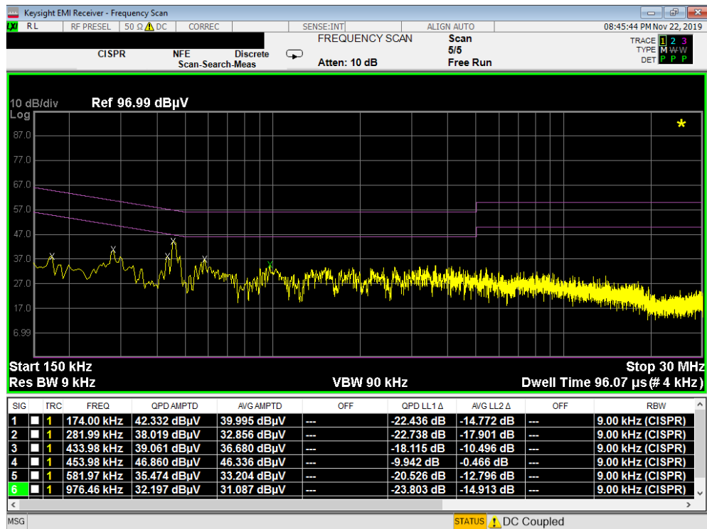
Plot 7-359. Line Conducted Plot with 802.11a UNII Band 1 (N)
