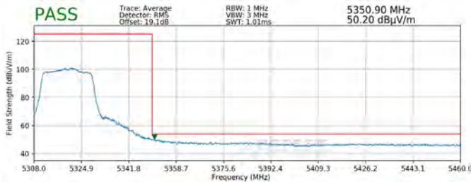
Plot 7-330. Radiated Upper Band Edge Plot MIMO (Average – UNII Band 2A)
