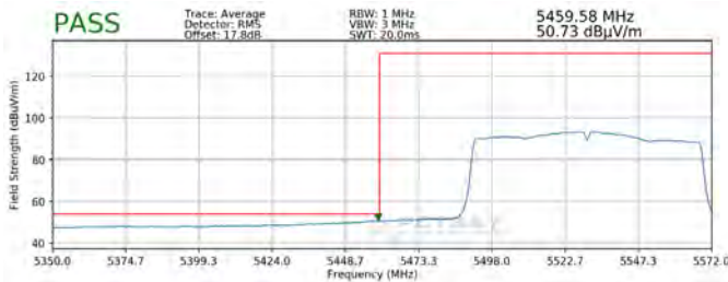
Plot 7-325. Radiated Lower Band Edge Plot SISO ANT2 (Average - UNII Band 2C)
