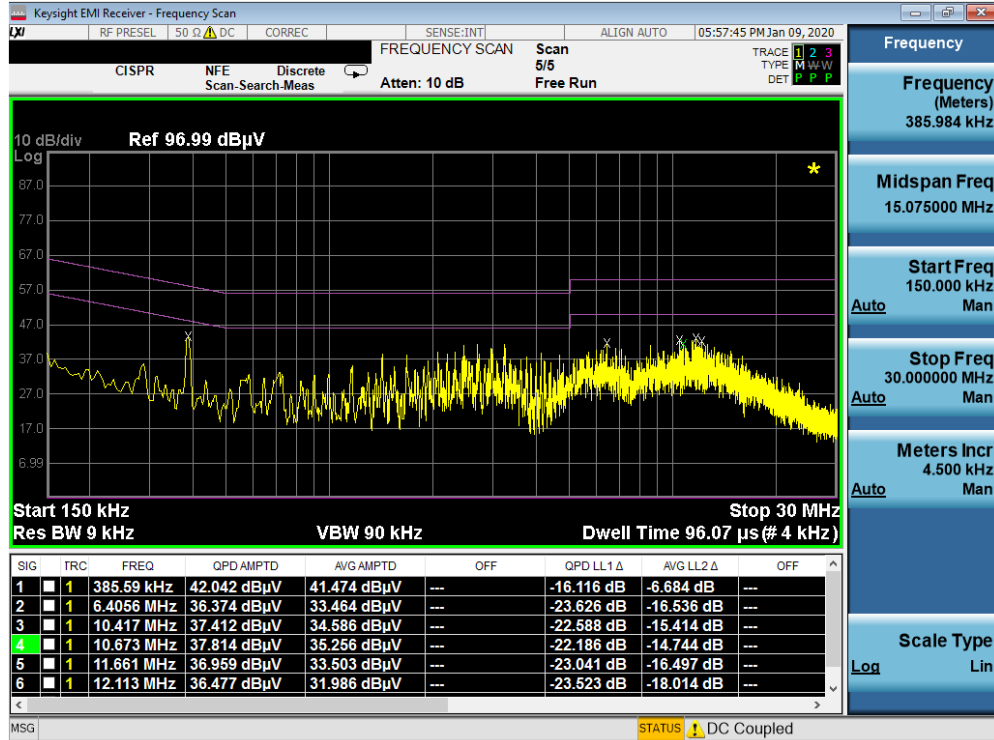
Plot 7-370. Line Conducted Plot with 802.11a UNII Band 2C with WCP (L1)
