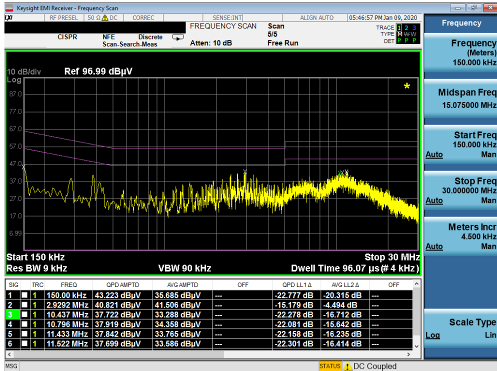
Plot 7-367. Line Conducted Plot with 802.11a UNII Band 1 with WCP (N)
