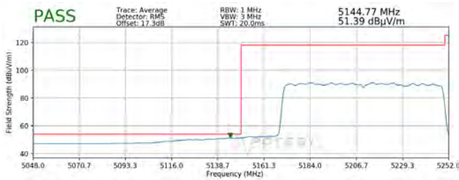
Plot 7-346. Radiated Lower Band Edge Plot MIMO (Average – UNII Band 1)
