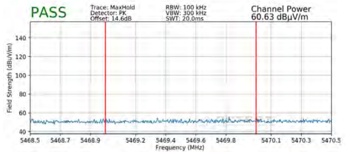
Plot 7-298. Radiated Lower Band Edge Plot SISO ANT1 (Peak - UNII Band 2C)
