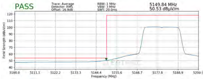
Plot 7-307. Radiated Lower Band Edge Plot SISO ANT2 (Average – UNII Band 1)
