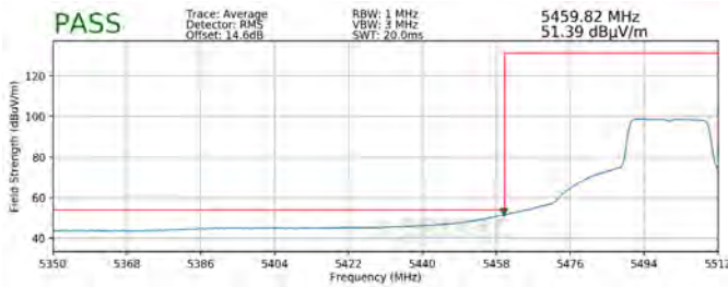
Plot 7-290. Radiated Lower Band Edge Plot SISO ANT1 (Average - UNII Band 2C)
