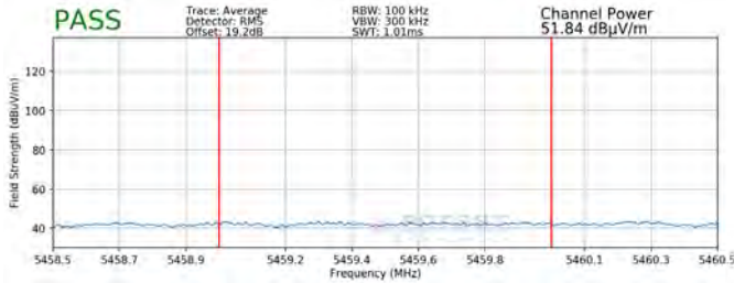
Plot 7-332. Radiated Lower Band Edge Plot MIMO (Average – UNII Band 2C)
