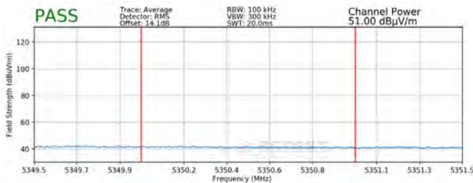
Plot 7-295. Radiated Upper Band Edge Plot SISO ANT1 (Average – UNII Band 2A)
