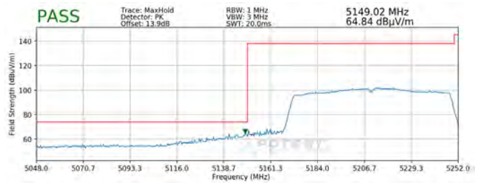
Plot 7-322. Radiated Lower Band Edge Plot SISO ANT2 (Peak – UNII Band 1)
