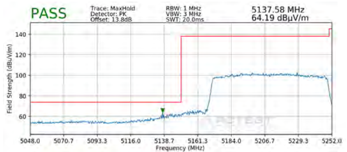
Plot 7-347. Radiated Lower Band Edge Plot MIMO (Peak – UNII Band 1)
