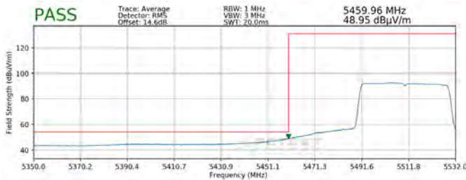
Plot 7-297. Radiated Lower Band Edge Plot SISO ANT1 (Average - UNII Band 2C)
