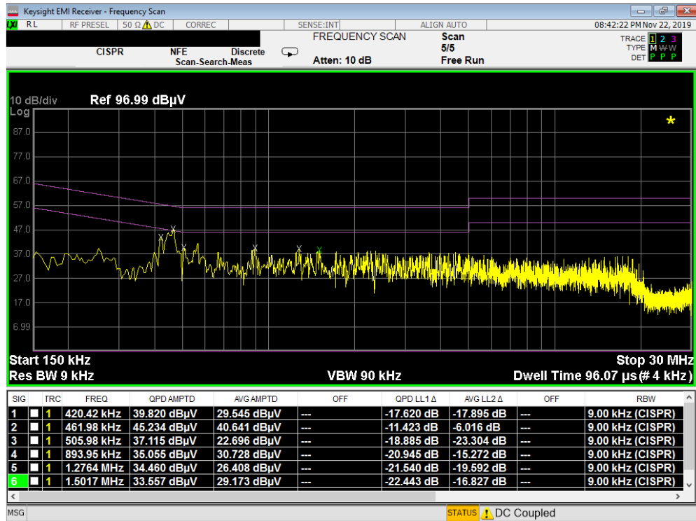
Plot 7-358. Line Conducted Plot with 802.11a UNII Band 1 (L1)
