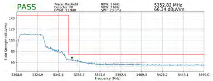
Plot 7-289. Radiated Upper Band Edge Plot SISO ANT1 (Peak – UNII Band 2A)
