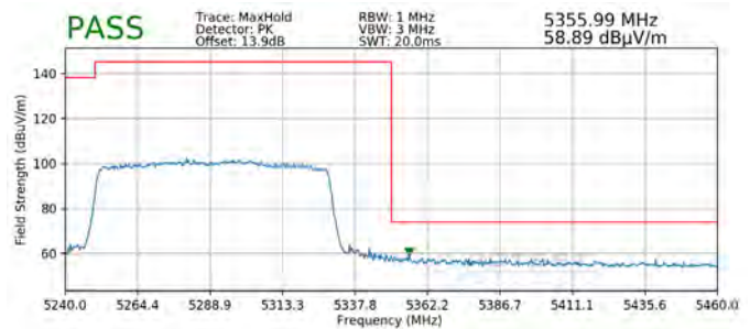
Plot 7-349. Radiated Upper Band Edge Plot MIMO (Peak – UNII Band 2A)
