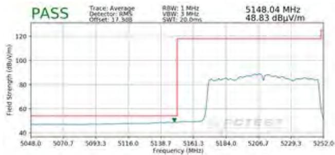
Plot 7-353. Radiated Band Edge Plot MIMO (Average – WCP)
