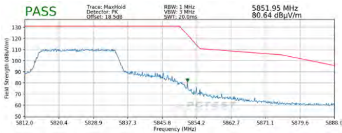
Plot 7-292. Radiated Upper Band Edge Plot SISO ANT1 (Peak - UNII Band 3)
