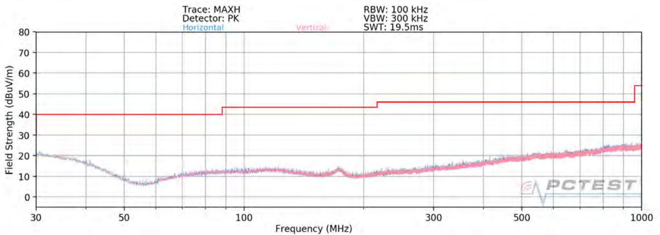
Plot 7-357. Radiated Spurious Plot below 1GHz (5GHz – 2.4 GHz)
