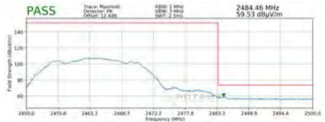
Plot 7-106. Radiated Restricted Upper Band Edge Measurement MIMO (Peak)
