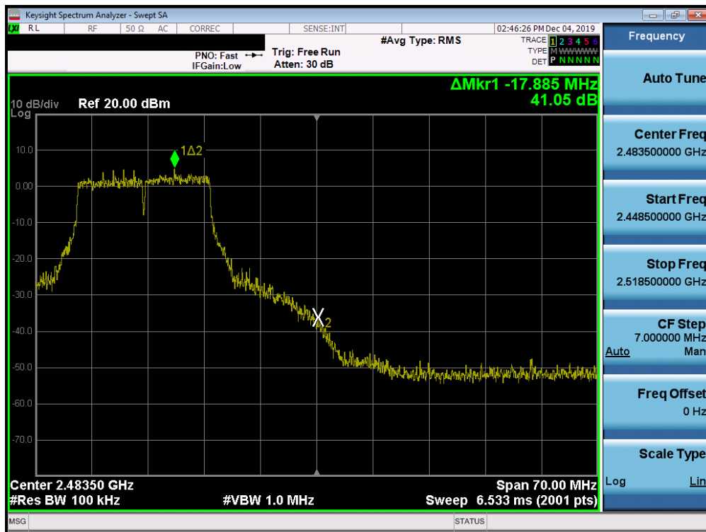
Plot 7-66. Band Edge Plot SISO ANT2 (802.11g - Ch. 11)
