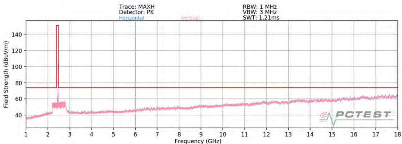
Plot 7-85. Radiated Spurious Plot above 1GHz SISO ANT1 (802.11b – Ch. 11)
