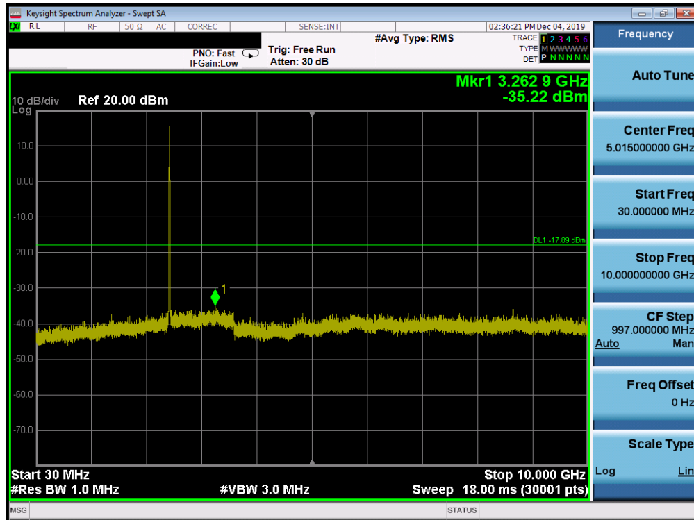
Plot 7-79. Conducted Spurious Plot SISO ANT2 (802.11b – Ch. 6)
