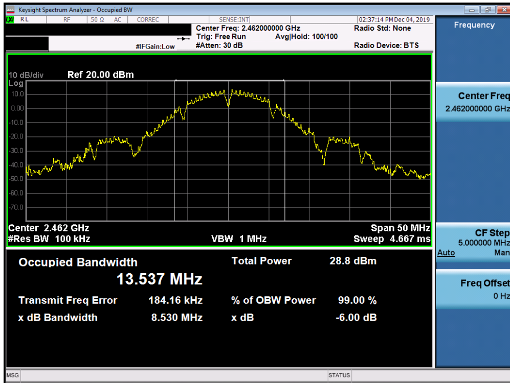
Plot 7-15. 6dB Bandwidth Plot SISO ANT1 (802.11b – Ch. 11)
