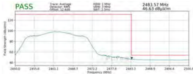
Plot 7-105. Radiated Restricted Upper Band Edge Measurement MIMO (Average)
