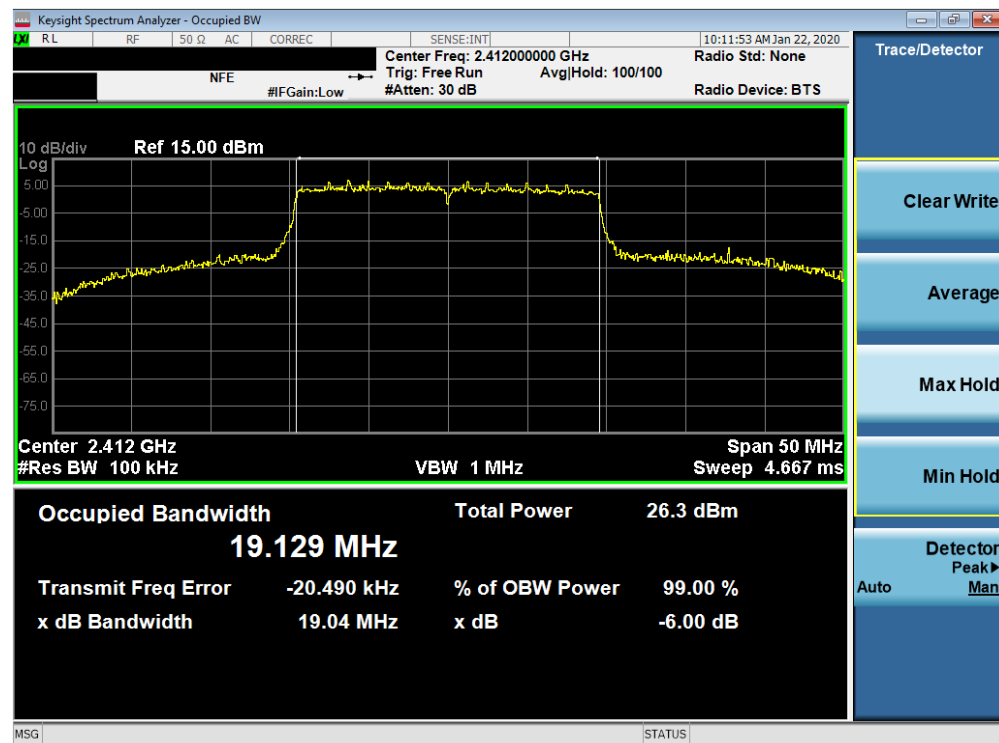
Plot 7-22. 6dB Bandwidth Plot SISO ANT1 (802.11ax (2.4GHz) – Ch. 1)
