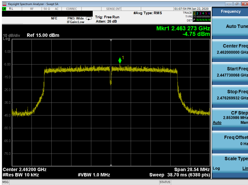
Plot 7-48. Power Spectral Density Plot SISO ANT1 (802.11ax (2.4GHz) – Ch. 11)
