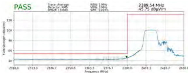
Plot 7-95. Radiated Restricted Lower Band Edge Measurement SISO ANT1 (Average)
