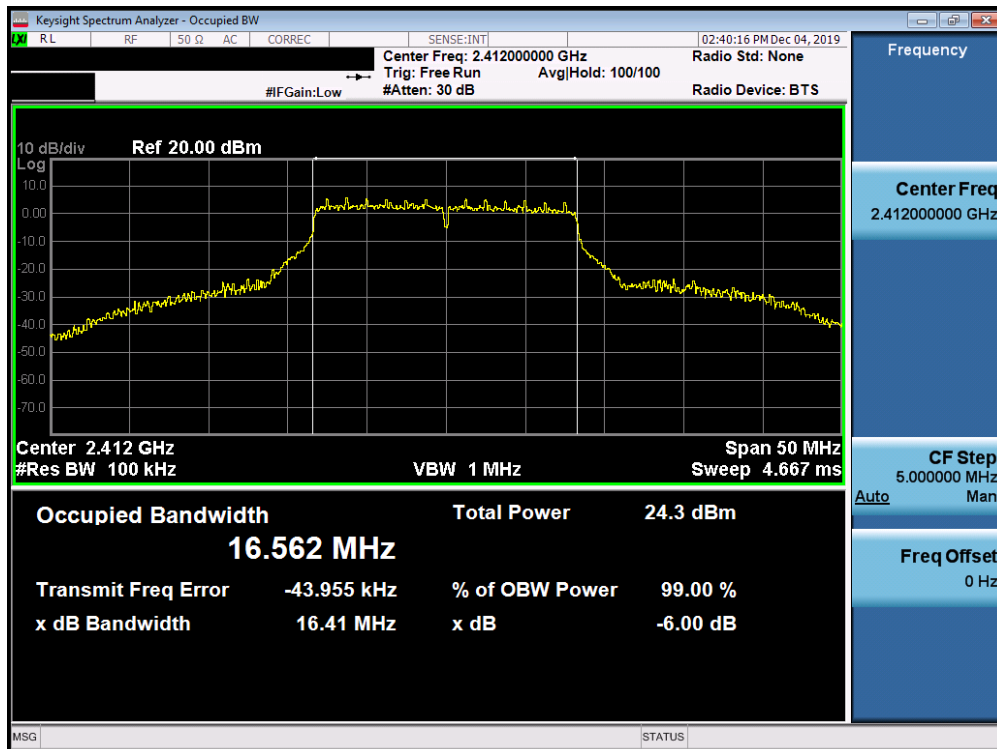
Plot 7-16. 6dB Bandwidth Plot SISO ANT1 (802.11g – Ch. 1)
