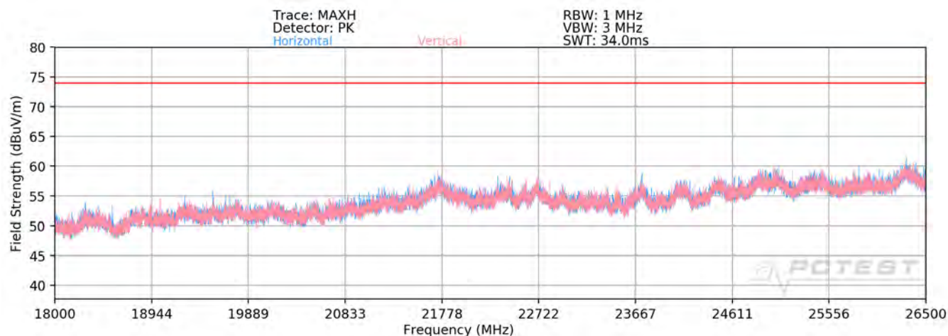
Plot 7-94. Radiated Spurious Plot above 18GHz MIMO/CDD
