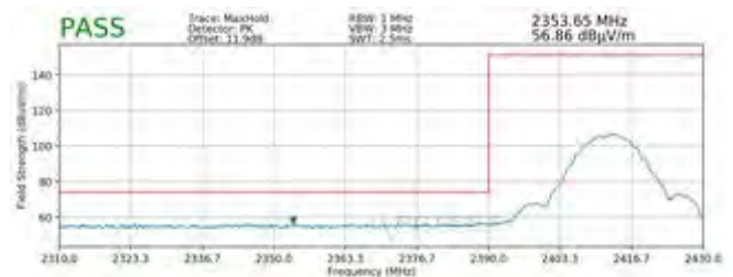
Plot 7-100. Radiated Restricted Lower Band Edge Measurement SISO ANT2 (Peak)
