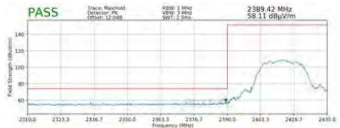
Plot 7-104. Radiated Restricted Lower Band Edge Measurement MIMO (Peak)
