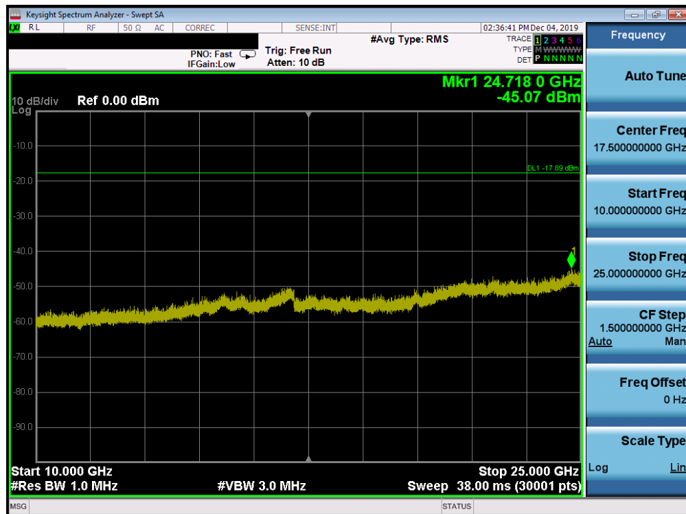
Plot 7-80. Conducted Spurious Plot SISO ANT2 (802.11b – Ch. 6)
