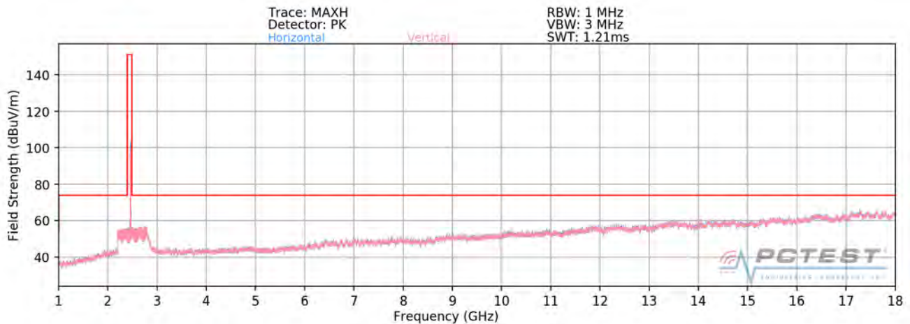
Plot 7-93. Radiated Spurious Plot above 1GHz MIMO/CDD (802.11g – Ch. 11)
