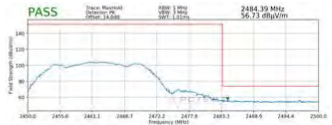
Plot 7-108. Radiated Restricted Band Edge Measurement MIMO with WCP (Peak)
