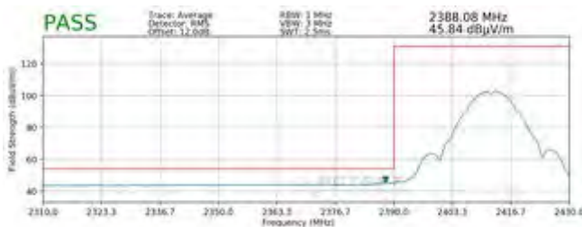
Plot 7-99. Radiated Restricted Lower Band Edge Measurement SISO ANT2 (Average)
