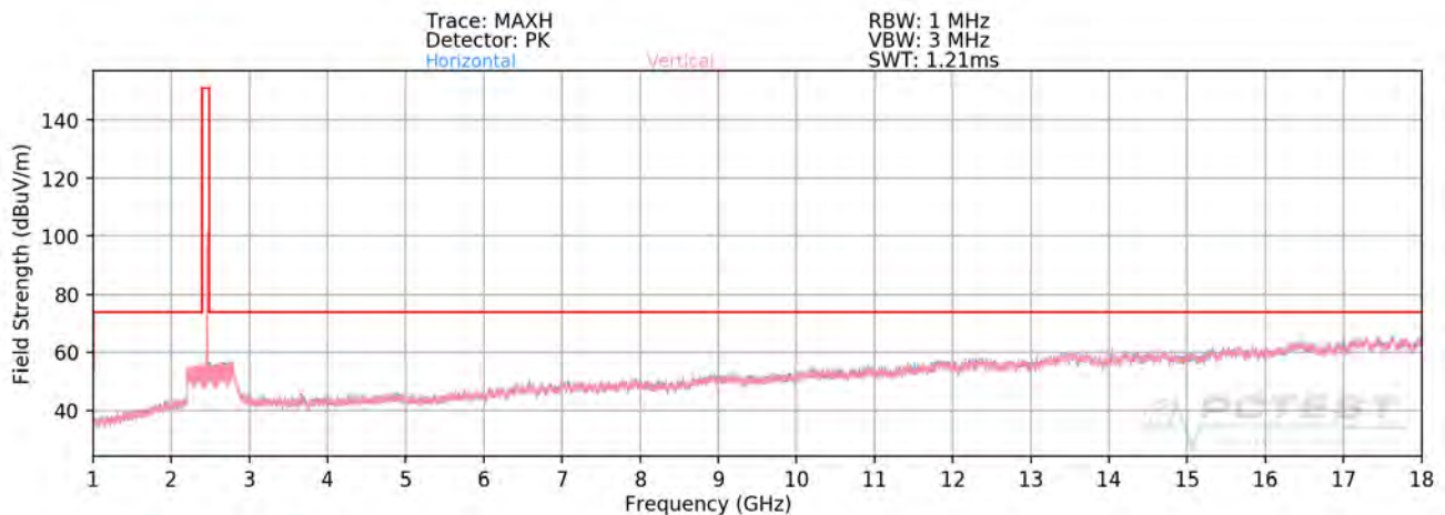
Plot 7-89. Radiated Spurious Plot above 1GHz SISO ANT2 (802.11b – Ch. 11)
