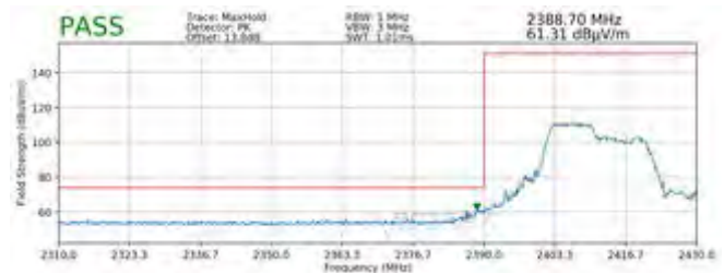
Plot 7-96. Radiated Restricted Lower Band Edge Measurement SISO ANT1 (Peak)
