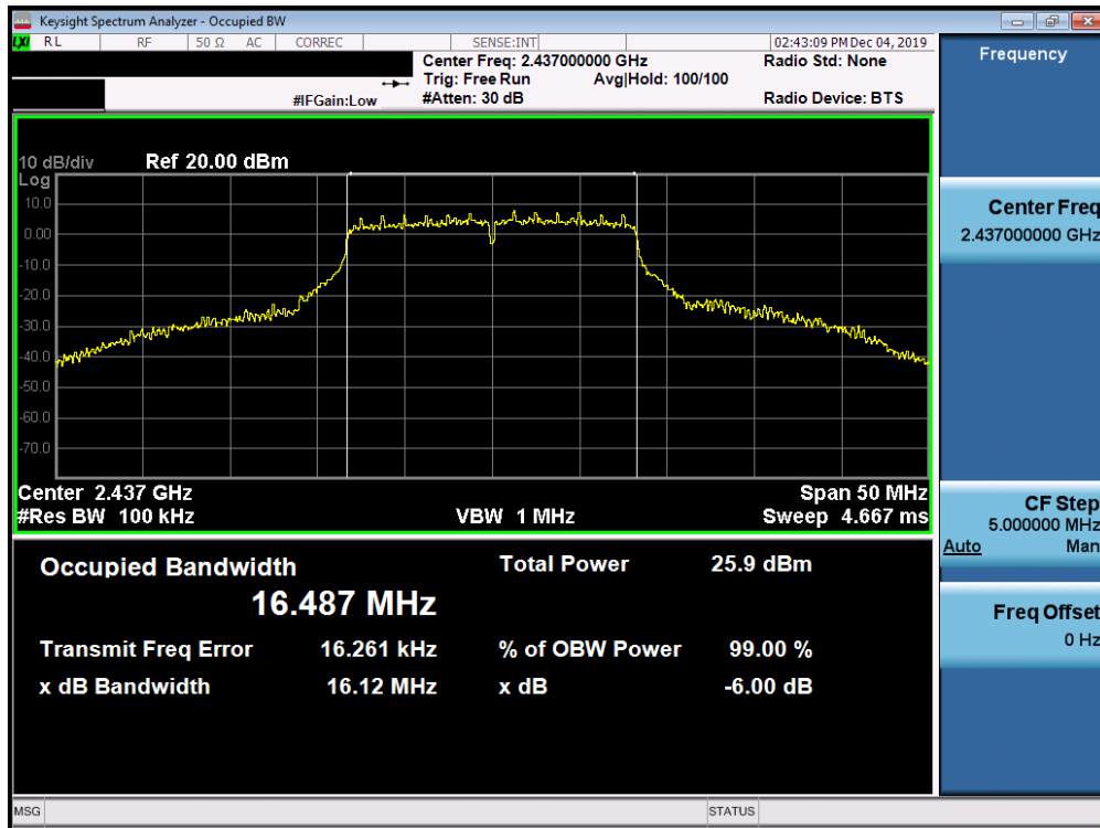
Plot 7-17. 6dB Bandwidth Plot SISO ANT1 (802.11g – Ch. 6)
