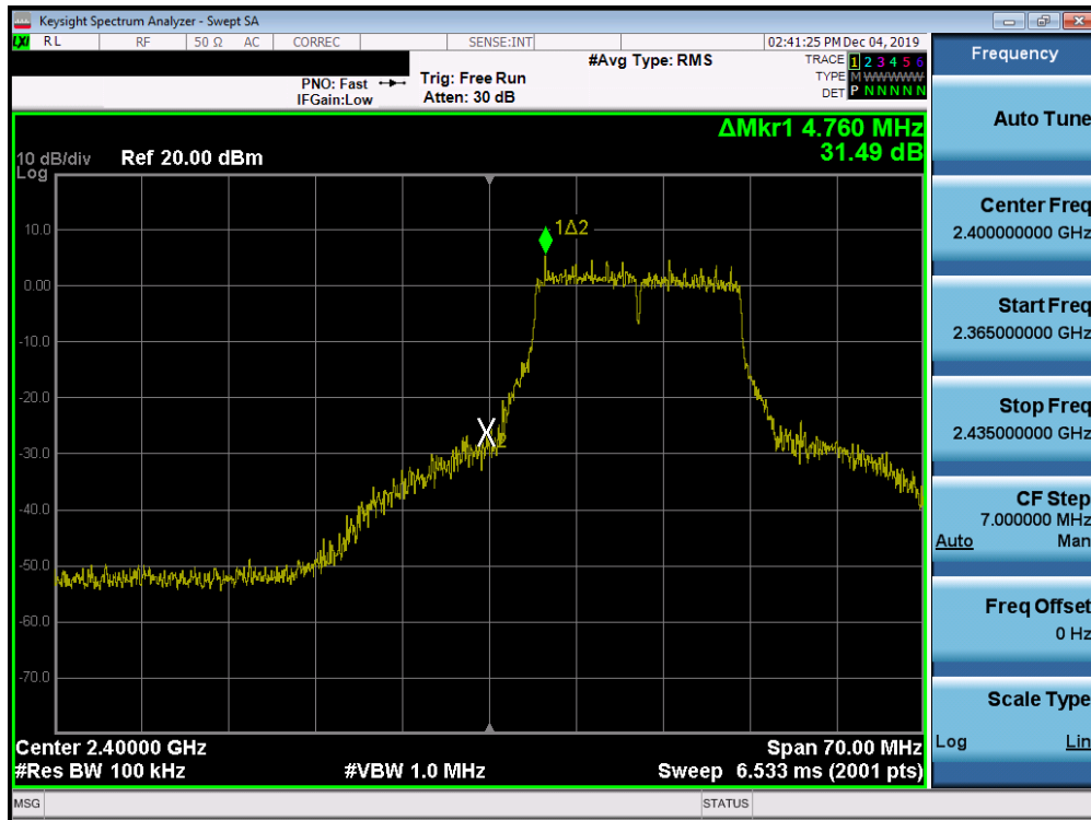
Plot 7-65. Band Edge Plot SISO ANT2 (802.11g- Ch. 1)
