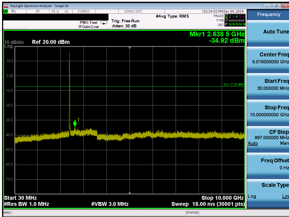
Plot 7-77. Conducted Spurious Plot SISO ANT2 (802.11b - Ch. 1)
