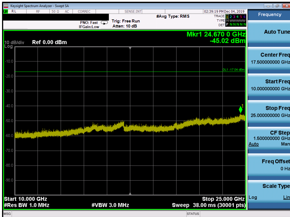
Plot 7-82. Conducted Spurious Plot SISO ANT2 (802.11b – Ch. 11)
