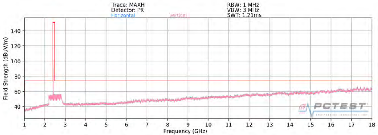
Plot 7-87. Radiated Spurious Plot above 1GHz SISO ANT2 (802.11b – Ch. 1)
