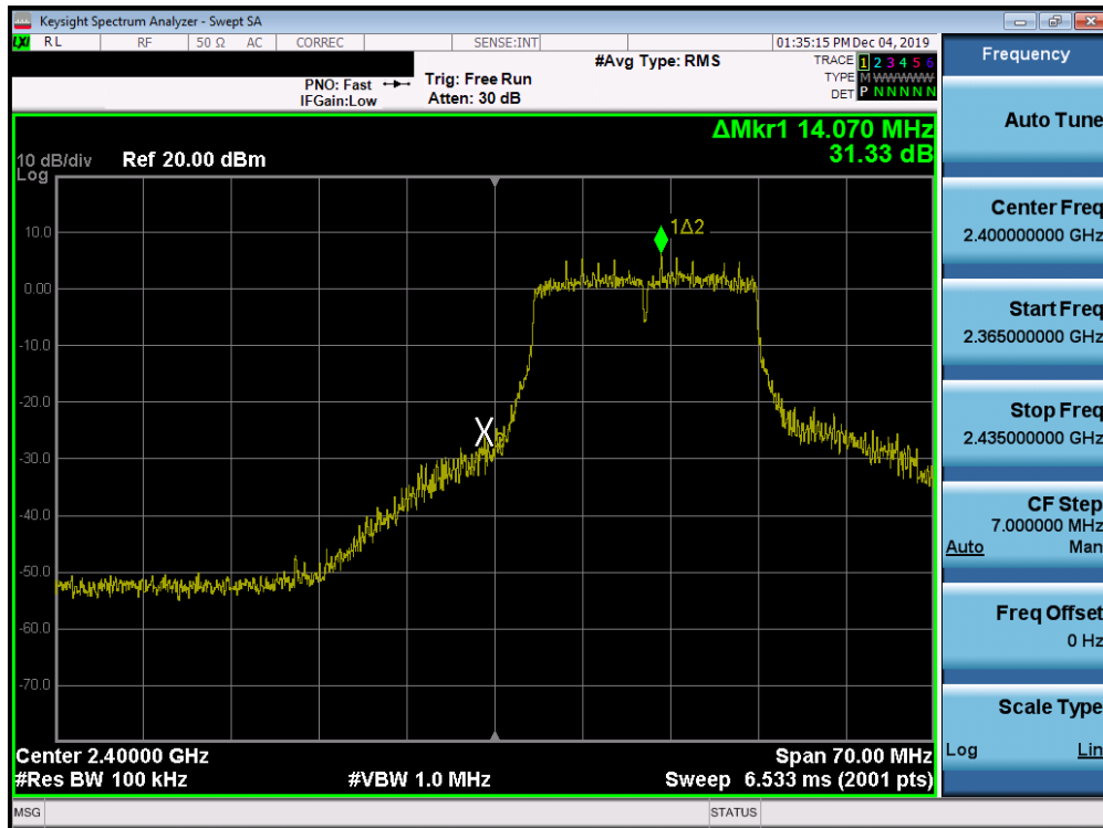
Plot 7-59. Band Edge Plot SISO ANT1 (802.11n (2.4GHz) – Ch. 1)
