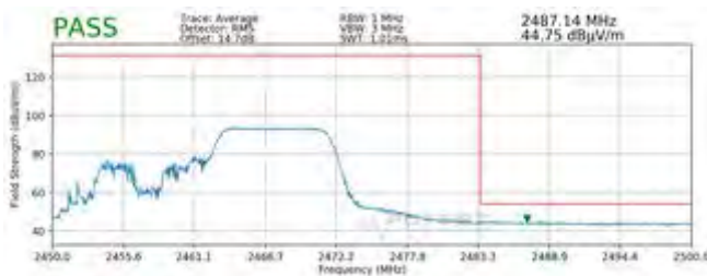
Plot 7-101. Radiated Restricted Upper Band Edge Measurement SISO ANT2 (Average)
