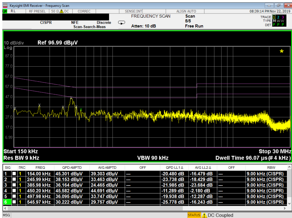
Plot 7-111. Line Conducted Plot with 802.11b (N)
