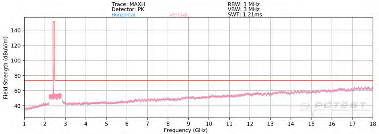
Plot 7-91. Radiated Spurious Plot above 1GHz MIMO/CDD (802.11g – Ch. 1)
