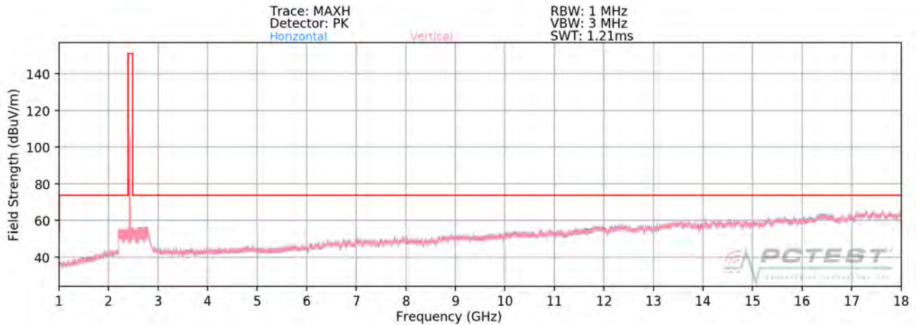
Plot 7-92. Radiated Spurious Plot above 1GHz MIMO/CDD (802.11g – Ch. 6)
