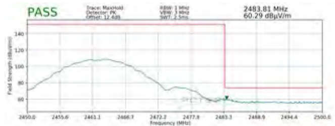
Plot 7-98. Radiated Restricted Upper Band Edge Measurement SISO ANT1 (Peak)
