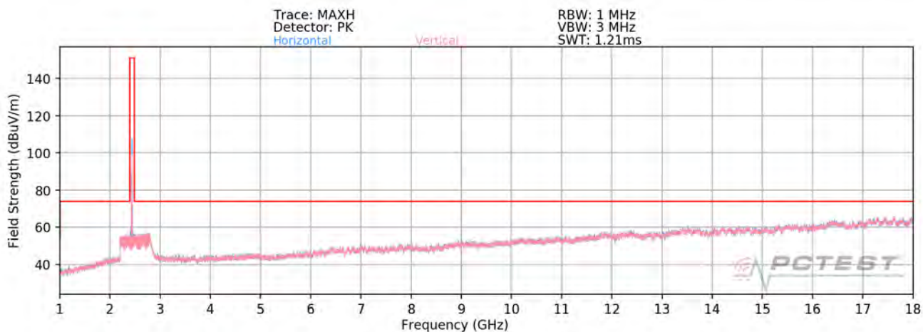
Plot 7-84. Radiated Spurious Plot above 1GHz SISO ANT1 (802.11b – Ch. 6)
