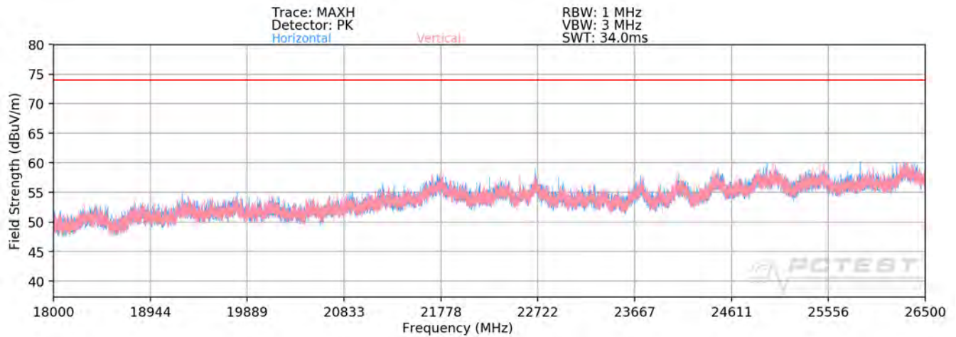
Plot 7-90. Radiated Spurious Plot above 18GHz SISO ANT2
