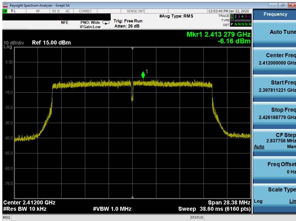
Plot 7-46. Power Spectral Density Plot SISO ANT1 (802.11ax (2.4GHz) – Ch. 1)
