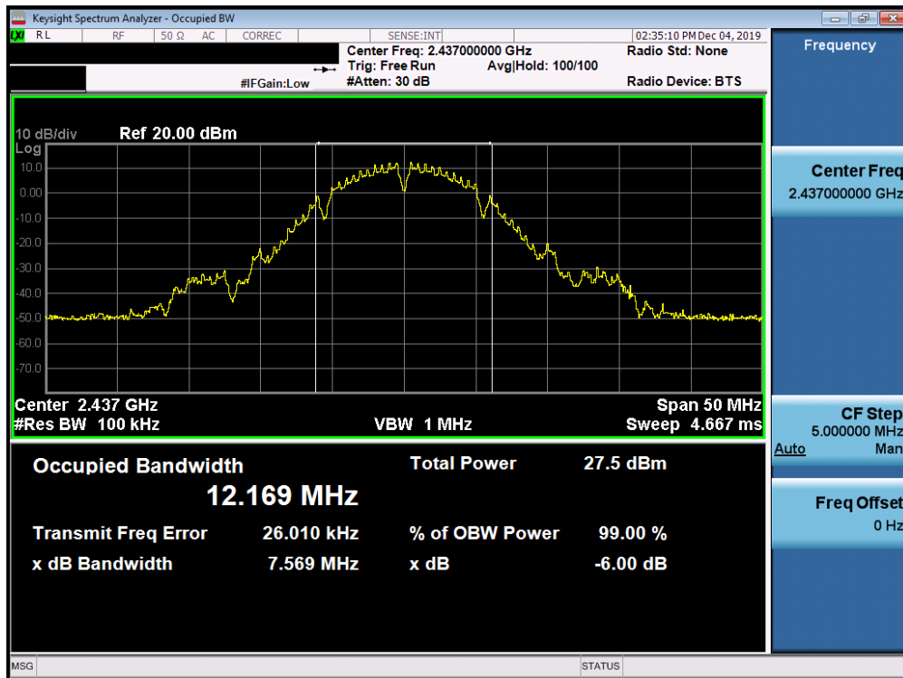
Plot 7-14. 6dB Bandwidth Plot SISO ANT1 (802.11b – Ch. 6)
