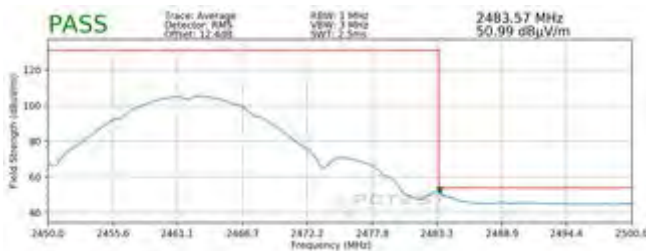
Plot 7-97. Radiated Restricted Upper Band Edge Measurement SISO ANT1 (Average)
