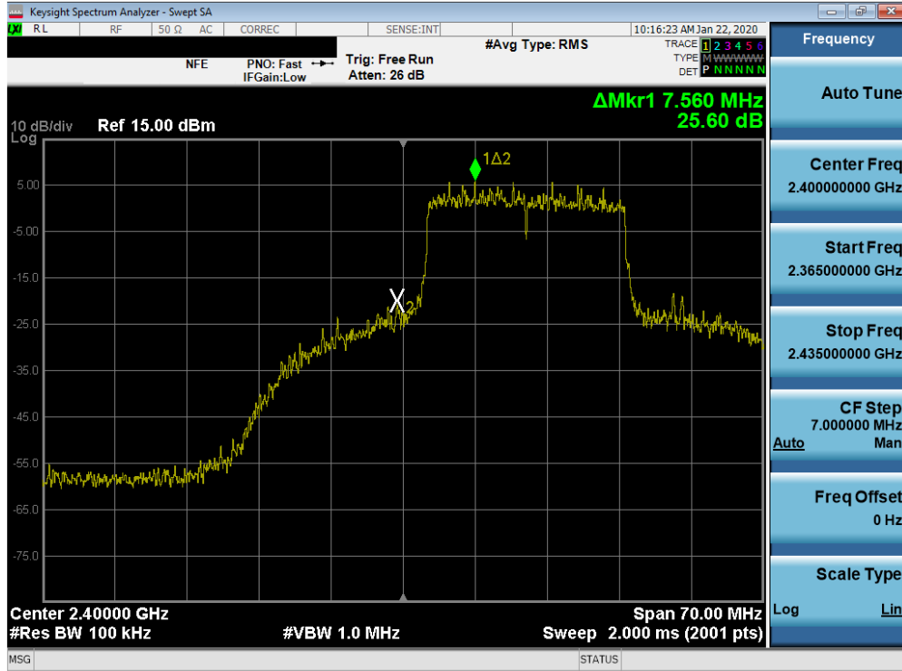
Plot 7-69. Band Edge Plot SISO ANT2 (802.11ax (2.4GHz) – Ch. 1)
