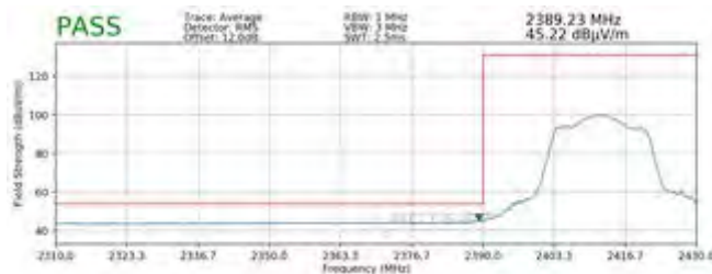
Plot 7-103. Radiated Restricted Lower Band Edge Measurement MIMO (Average)
