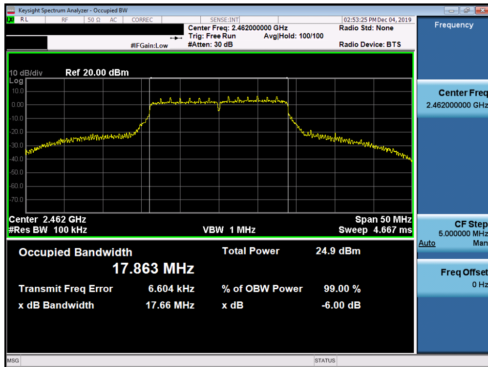
Plot 7-21. 6dB Bandwidth Plot SISO ANT1 (802.11n (2.4GHz) – Ch. 11)
