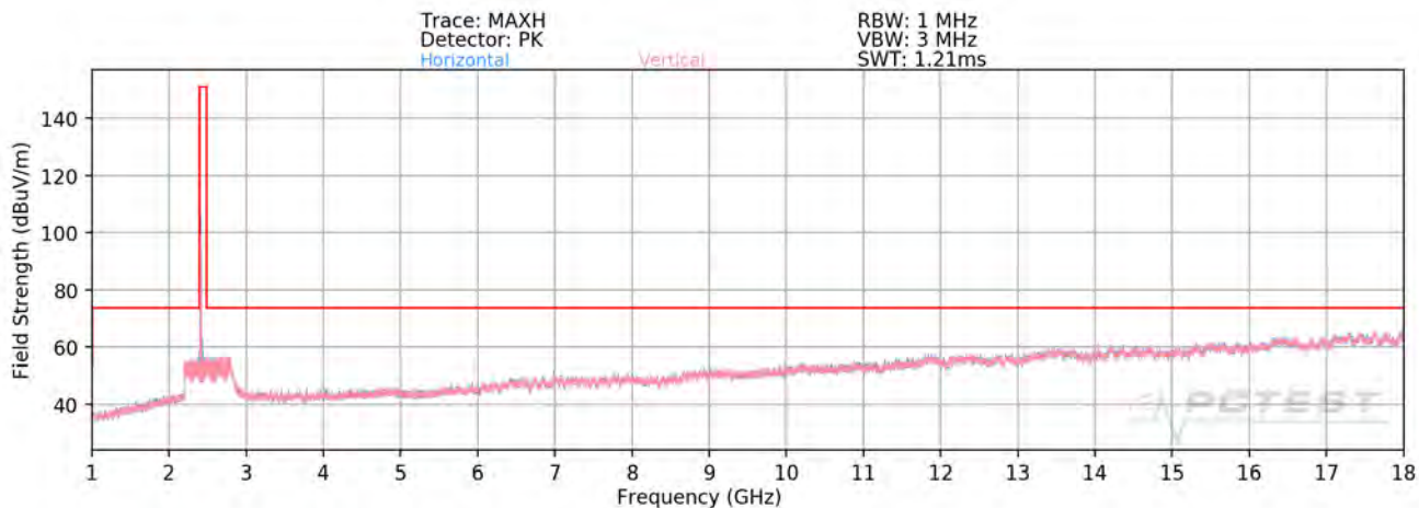
Plot 7-83. Radiated Spurious Plot above 1GHz SISO ANT1 (802.11b – Ch. 1)
