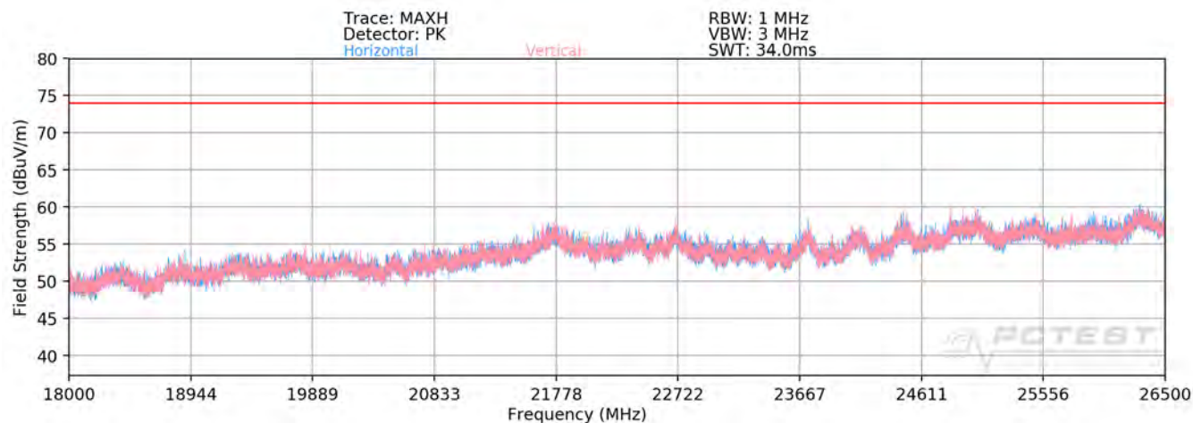
Plot 7-86. Radiated Spurious Plot above 18GHz SISO ANT1
