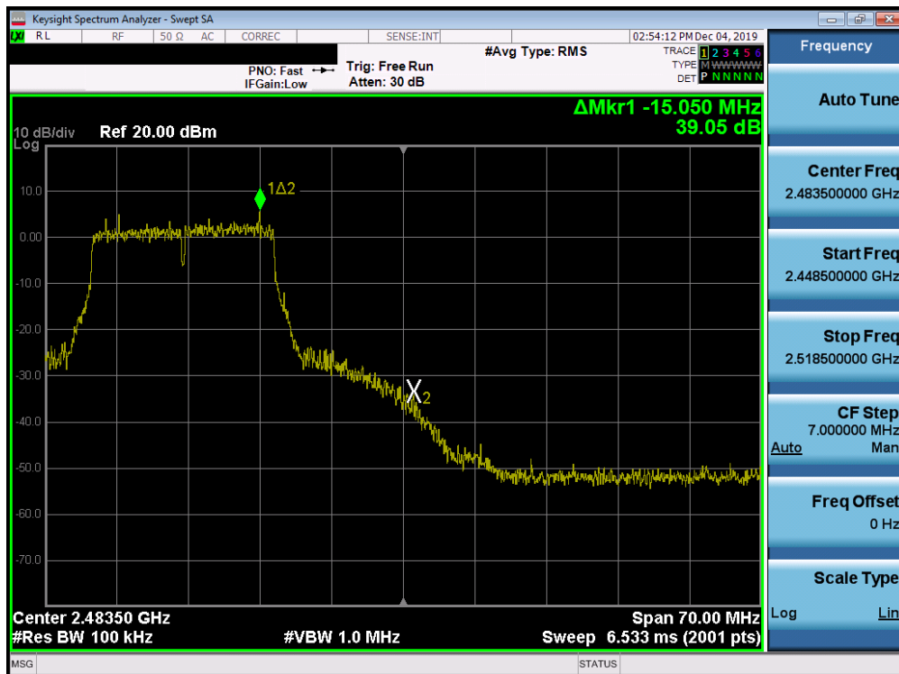
Plot 7-68. Band Edge Plot SISO ANT2 (802.11n (2.4GHz) – Ch. 11)
