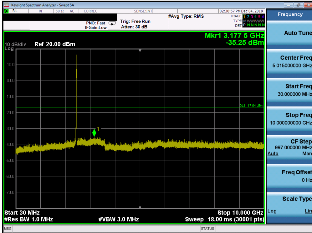
Plot 7-81. Conducted Spurious Plot SISO ANT2 (802.11b – Ch. 11)
