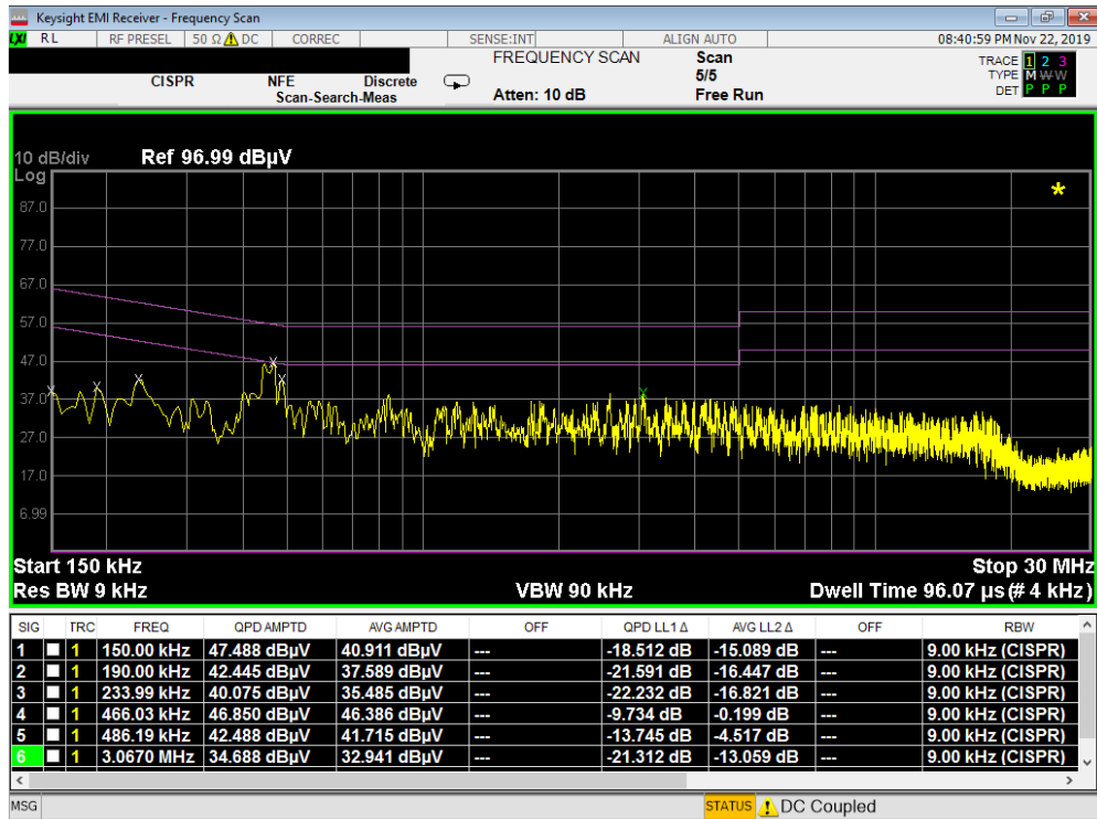
Plot 7-110. Line Conducted Plot with 802.11b (L1)
