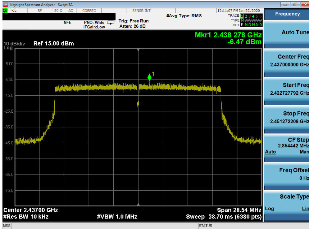
Plot 7-47. Power Spectral Density Plot SISO ANT1 (802.11ax (2.4GHz) – Ch. 6)
