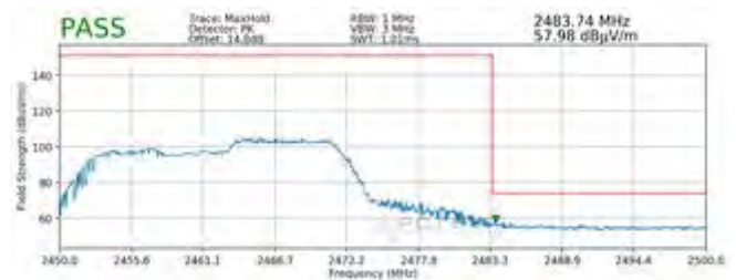
Plot 7-102. Radiated Restricted Upper Band Edge Measurement SISO ANT2 (Peak)
