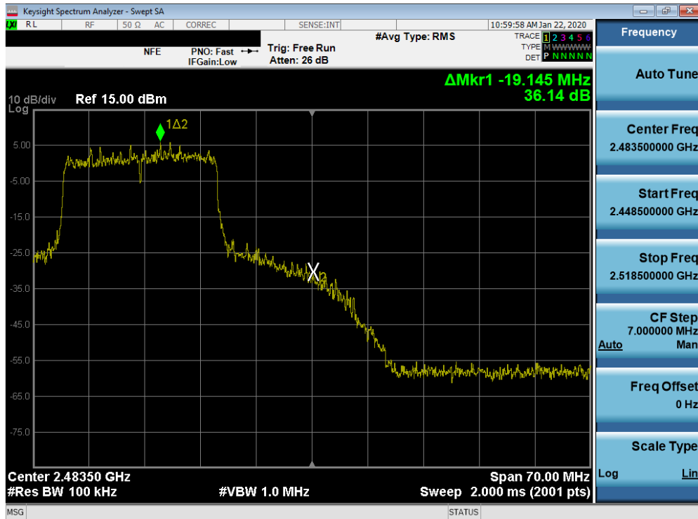
Plot 7-70. Band Edge Plot SISO ANT2 (802.11ax (2.4GHz) – Ch. 11)
