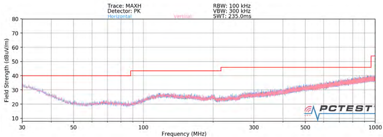
Plot 7-109. Radiated Spurious Plot below 1GHz MIMO
