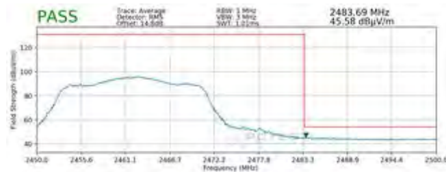
Plot 7-107. Radiated Restricted Band Edge Measurement MIMO with WCP (Average)
