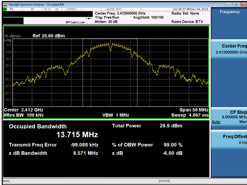
Plot 7-13. 6dB Bandwidth Plot SISO ANT1 (802.11b – Ch. 1)
