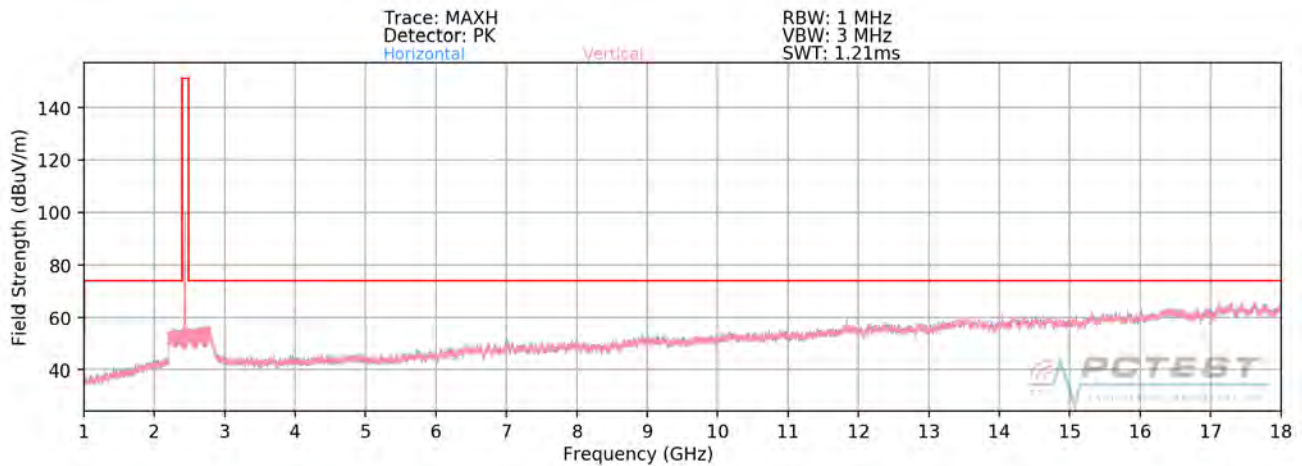
Plot 7-88. Radiated Spurious Plot above 1GHz SISO ANT2 (802.11b – Ch. 6)
