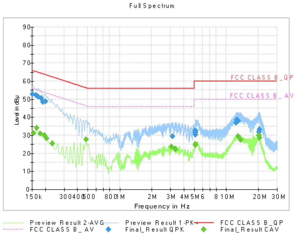
Figure 7: Conducted Emission, Wireless Charging (PHONE TO WATCH), Line (L1)
