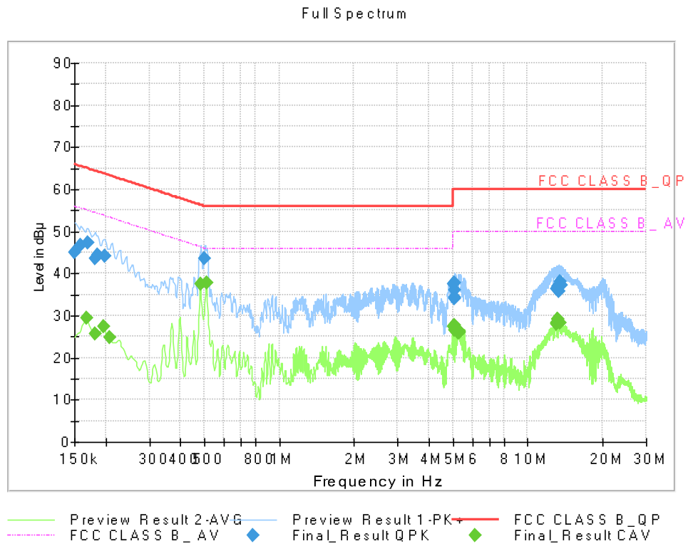
Figure 11: Conducted Emission, LTE B29 Middle ch Idle + Rear Camera, Line (L1)
