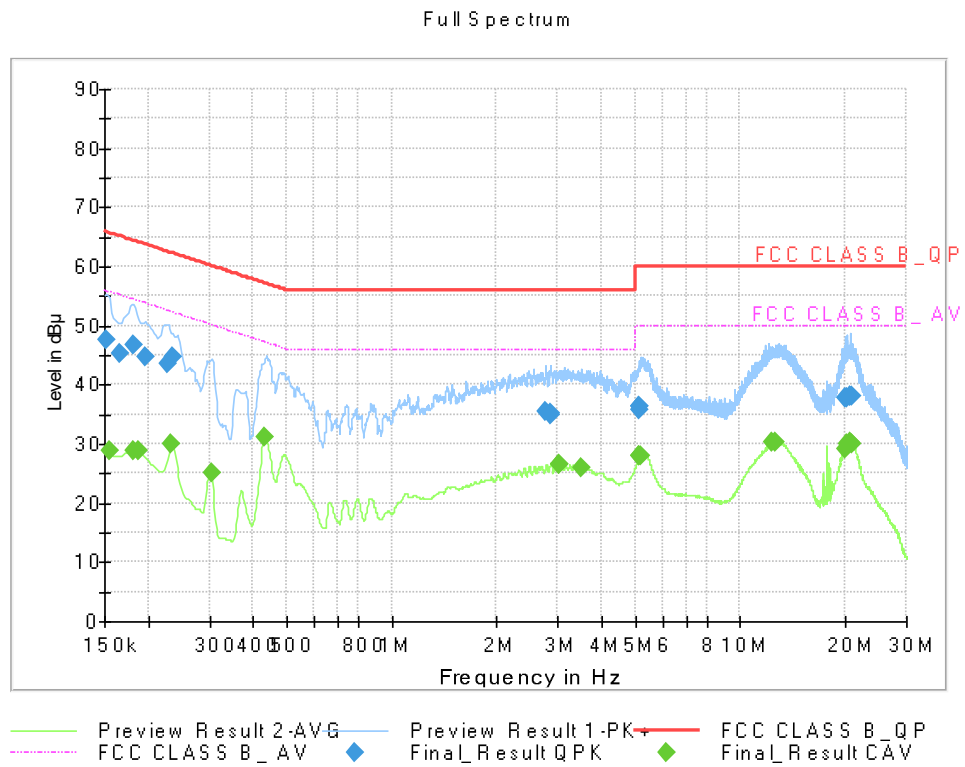
Figure 3: Conducted Emission, Video + Audio, Line (L1)
