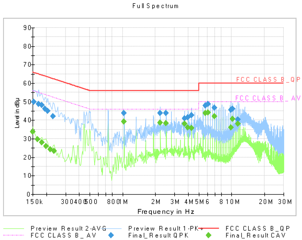
Figure 5: Conducted Emission, Wireless Charging (PHONE TO PHONE), Line (L1)
