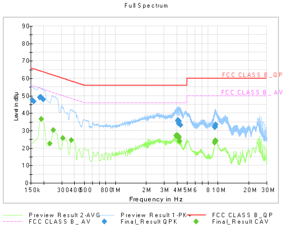
Figure 1: Conducted Emission, Data Communication (Internal), Line (L1)
