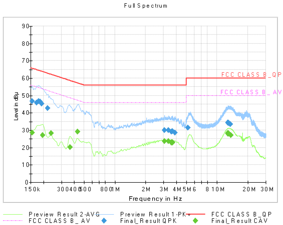
Figure 4: Conducted Emission, Video + Audio, Line (N)
