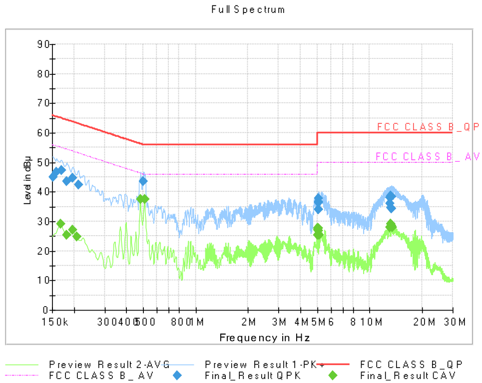
Figure 9: Conducted Emission, LTE B14 Middle ch Idle + Front Camera, Line (L1)
