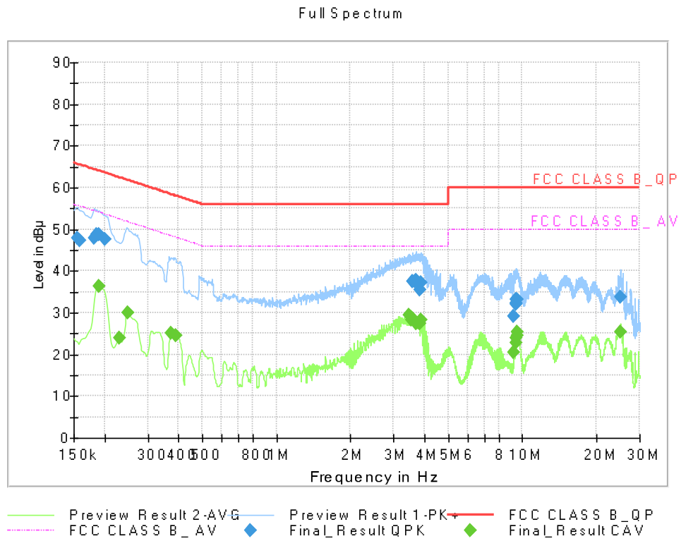
Figure 2: Conducted Emission, Data Communication (Internal), Line (N)
