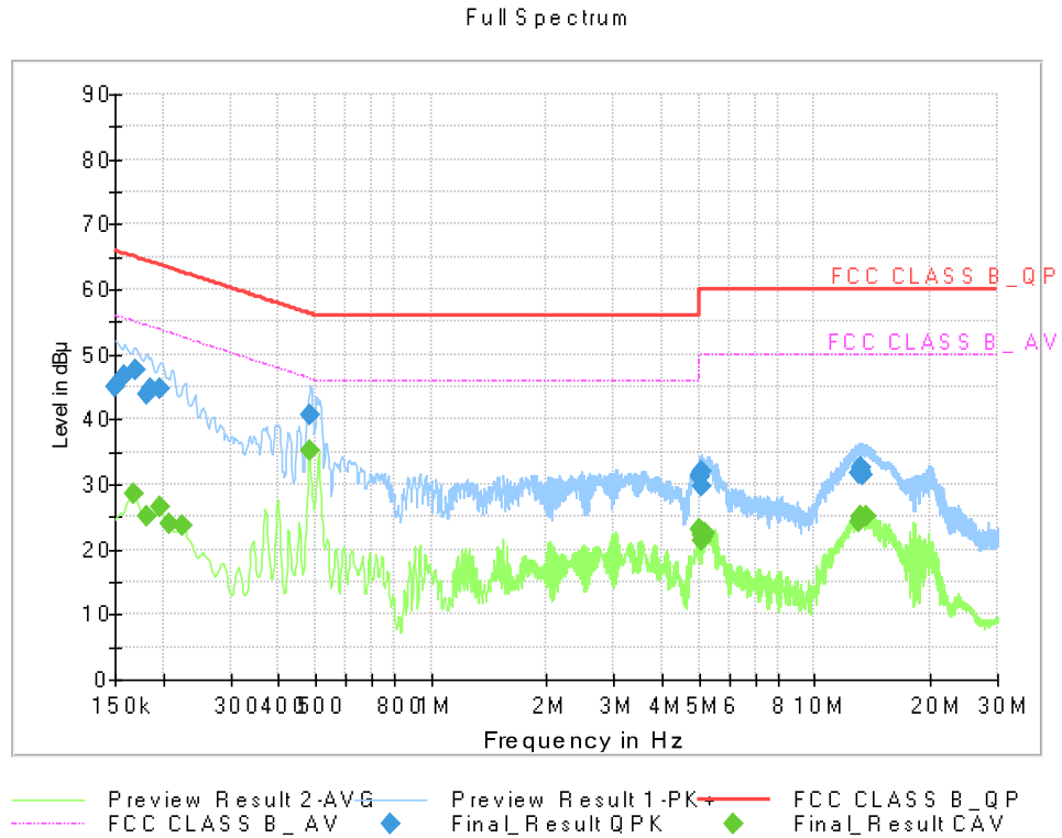
Figure 12: Conducted Emission, LTE B29 Middle ch Idle + Rear Camera, Line (N)
