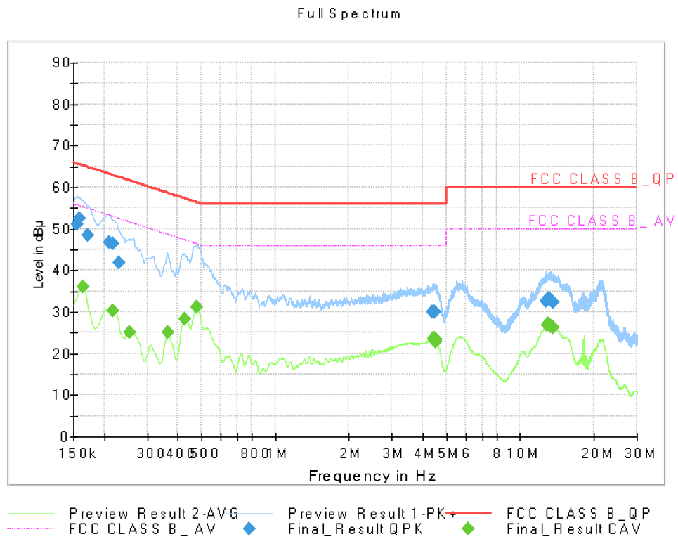
Figure 10: Conducted Emission, LTE B14 Middle ch Idle + Front Camera, Line (N)
