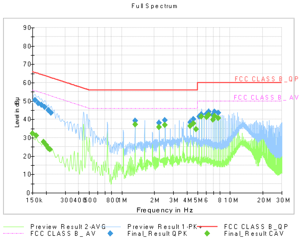
Figure 6: Conducted Emission, Wireless Charging (PHONE TO PHONE), Line (N)
