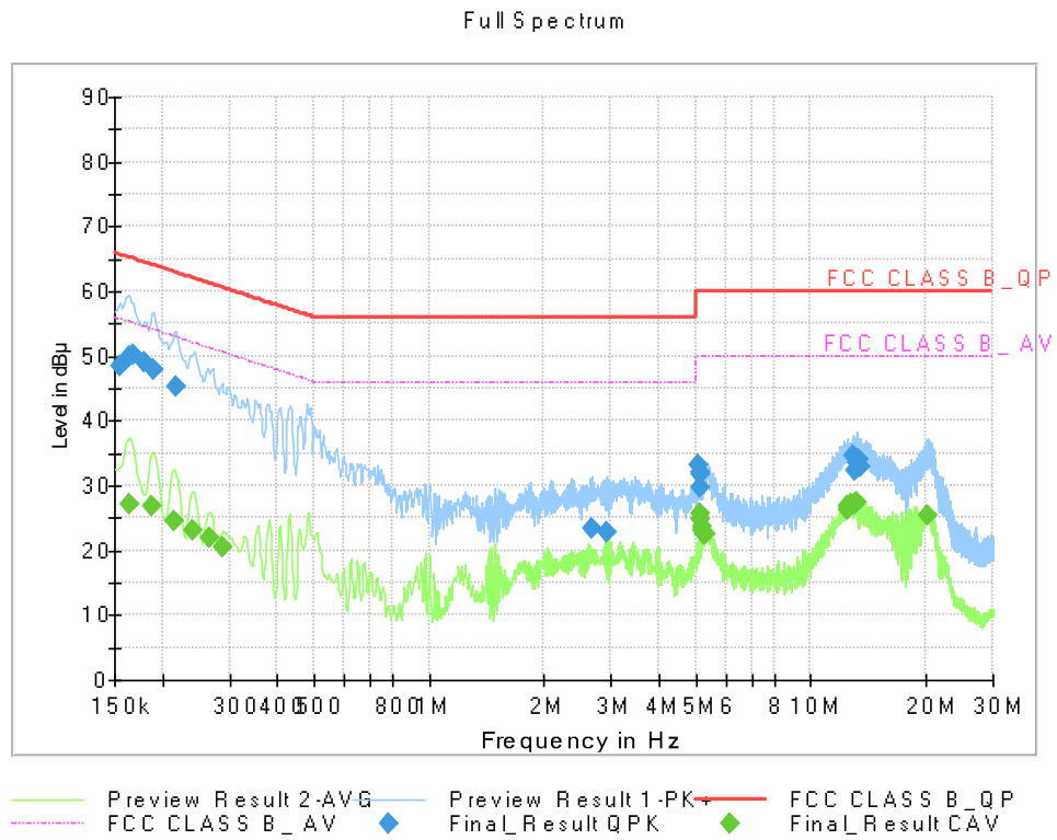
Figure 8: Conducted Emission, Wireless Charging (PHONE TO WATCH), Line (N)
