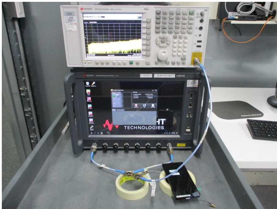
LICENSED BAND TEST PHOTO(Sub-6)
