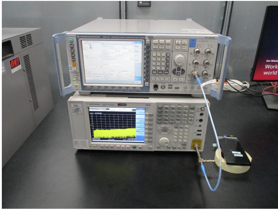
LICENSED BAND TEST PHOTO
